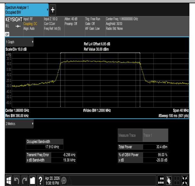
Band25-20MHz-16QAM-26140-100RB#0-PASS
