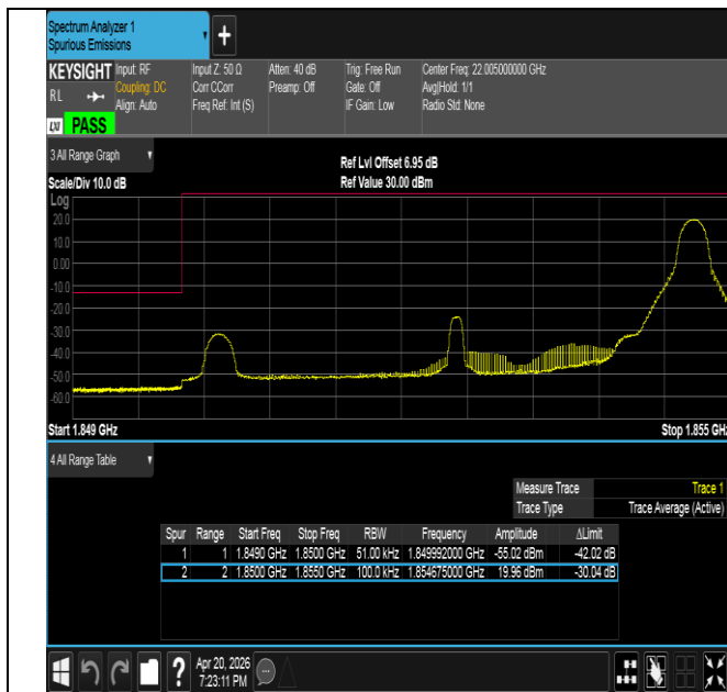
Band25-5MHz-16QAM-26065-1RB#24-PASS
