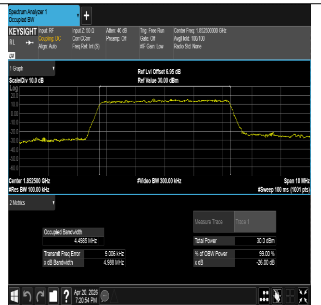
Band25-5MHz-16QAM-26065-25RB#0-PASS
