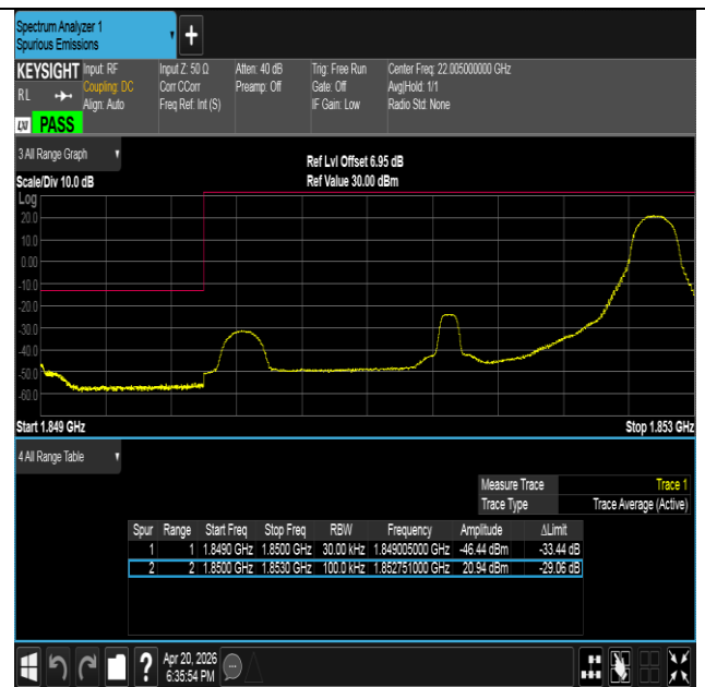
Band25-3MHz-QPSK-26055-1RB#14-PASS
