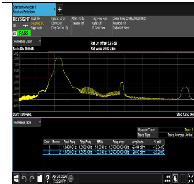
Band25-5MHz-QPSK-26065-1RB#0-PASS
