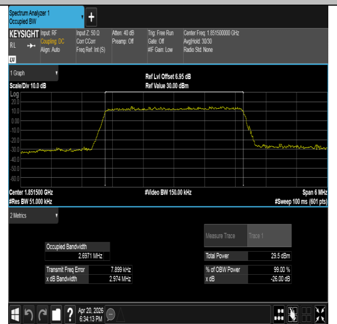
Band25-3MHz-16QAM-26055-15RB#0-PASS
