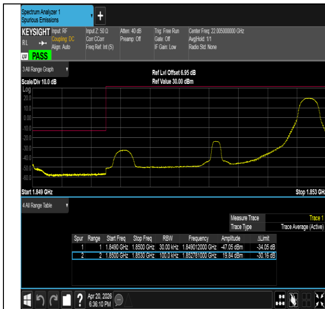
Band25-3MHz-16QAM-26055-1RB#14-PASS
