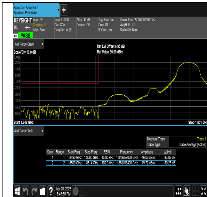
Band25-1.4MHz-16QAM-26047-1RB#5-PASS
