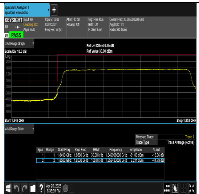
Band25-3MHz-16QAM-26055-15RB#0-PASS
