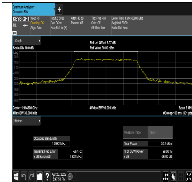
Band25-1.4MHz-QPSK-26683-6RB#0-PASS
