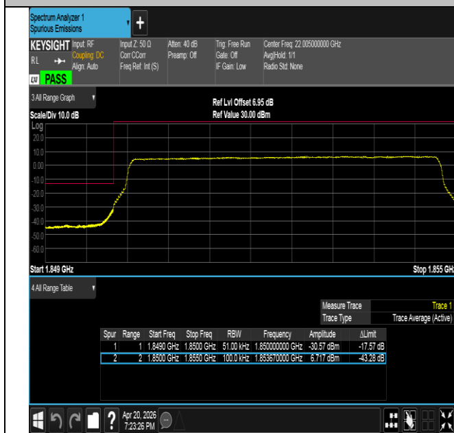
Band25-5MHz-QPSK-26065-25RB#0-PASS
