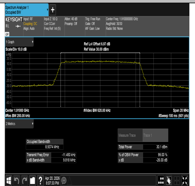
Band25-10MHz-16QAM-26640-50RB#0-PASS
