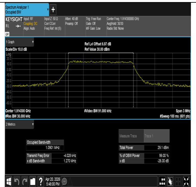
Band25-1.4MHz-16QAM-26683-6RB#0-PASS
