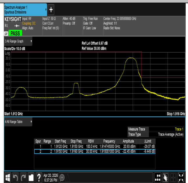
Band25-3MHz-QPSK-26675-1RB#14-PASS
