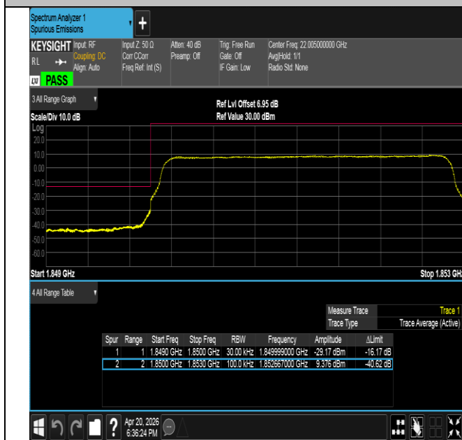
Band25-3MHz-QPSK-26055-15RB#0-PASS
