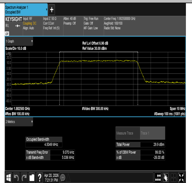
Band25-5MHz-16QAM-26365-25RB#0-PASS
