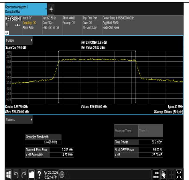
Band25-15MHz-16QAM-26115-75RB#0-PASS
