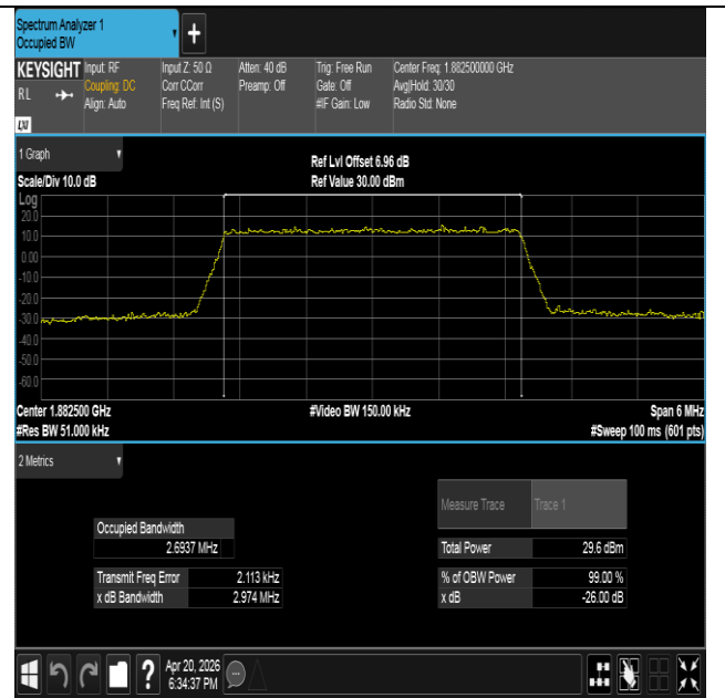
Band25-3MHz-16QAM-26365-15RB#0-PASS
