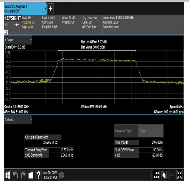
Band25-3MHz-16QAM-26675-15RB#0-PASS
