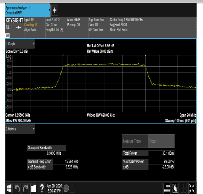
Band25-10MHz-16QAM-26090-50RB#0-PASS
