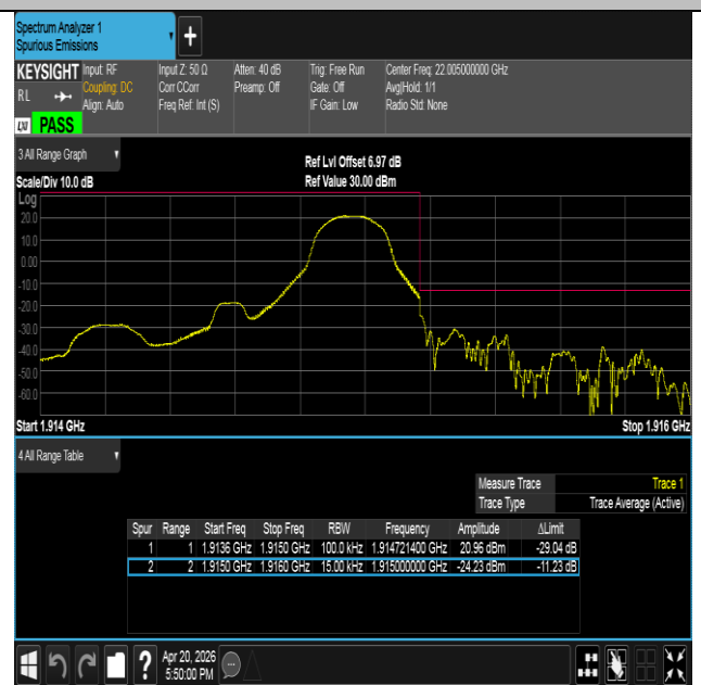
Band25-1.4MHz-QPSK-26683-1RB#5-PASS
