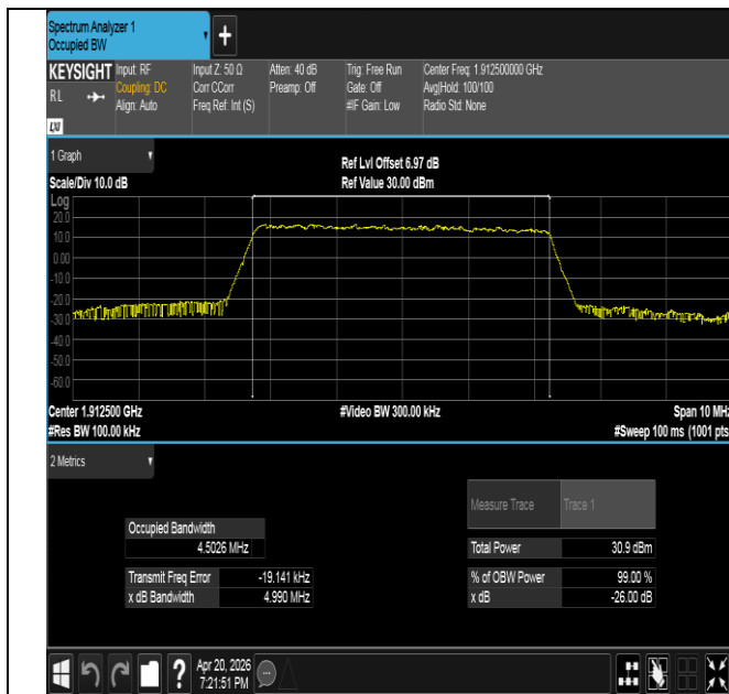
Band25-5MHz-QPSK-26665-25RB#0-PASS
