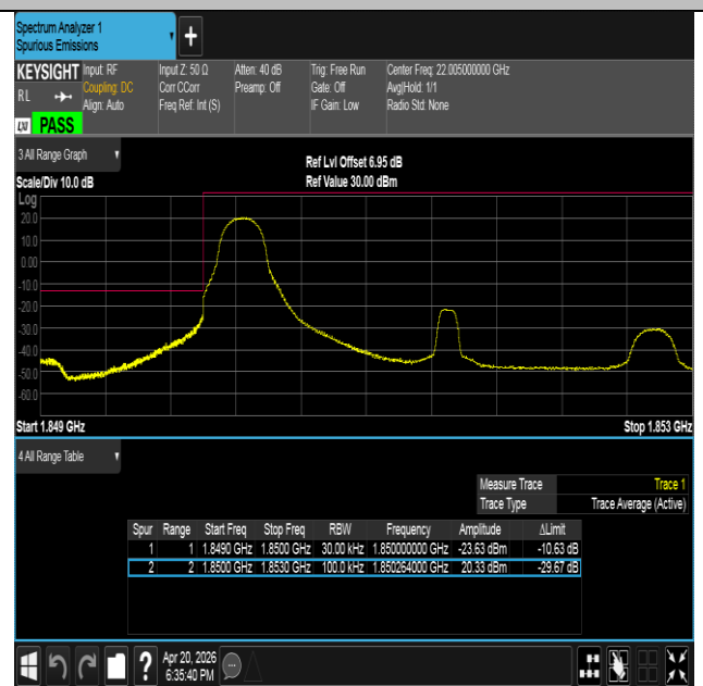
Band25-3MHz-16QAM-26055-1RB#0-PASS
