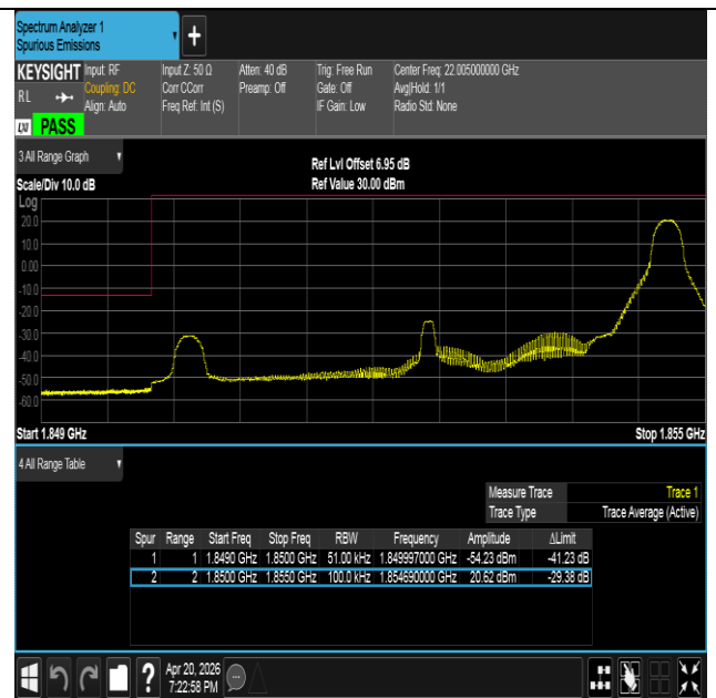
Band25-5MHz-QPSK-26065-1RB#24-PASS
