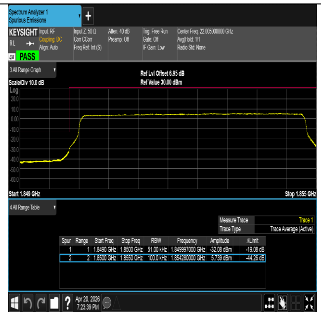
Band25-5MHz-16QAM-26065-25RB#0-PASS
