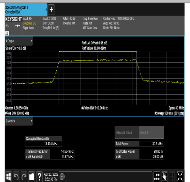
Band25-15MHz-16QAM-26365-75RB#0-PASS
