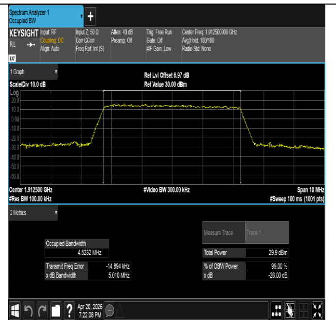
Band25-5MHz-16QAM-26665-25RB#0-PASS
