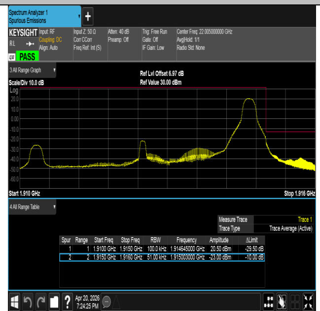
Band25-5MHz-QPSK-26665-1RB#24-PASS
