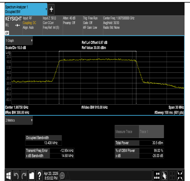
Band25-15MHz-16QAM-26615-75RB#0-PASS
