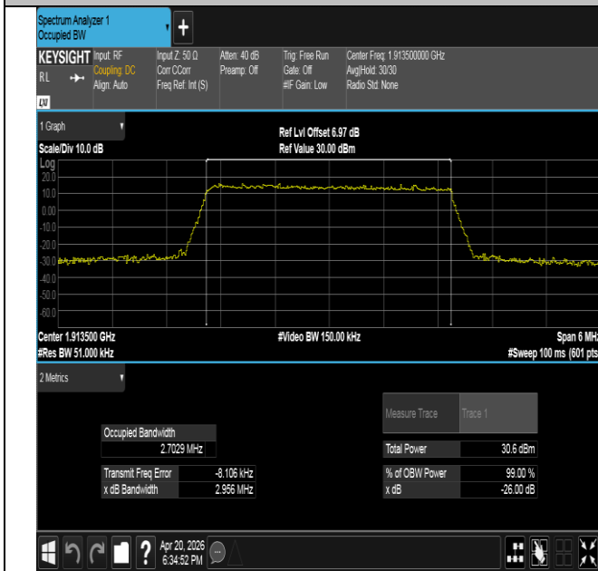
Band25-3MHz-QPSK-26675-15RB#0-PASS
