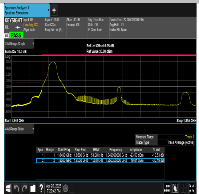
Band25-5MHz-16QAM-26065-1RB#0-PASS
