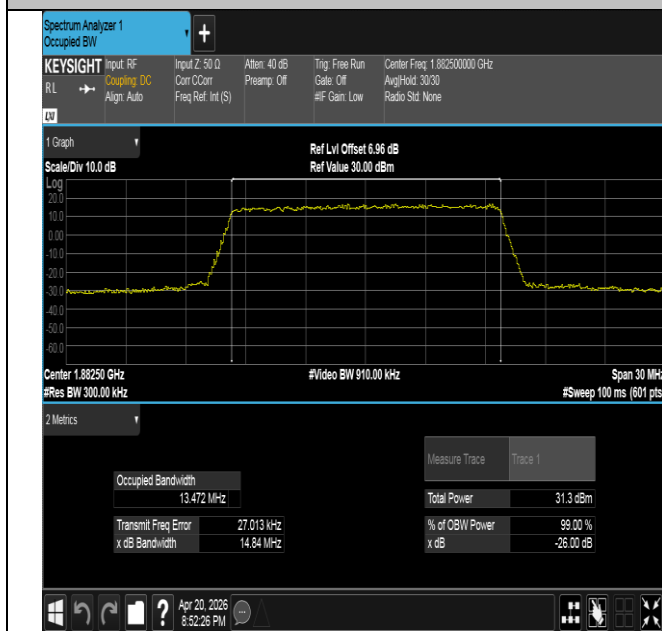
Band25-15MHz-QPSK-26365-75RB#0-PASS
