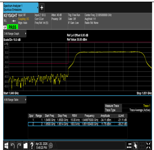
Band25-1.4MHz-16QAM-26047-6RB#0-PASS
