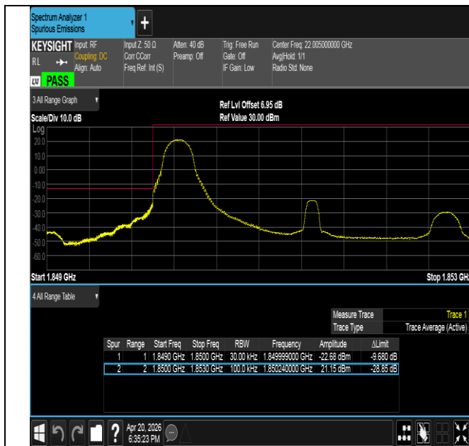
Band25-3MHz-QPSK-26055-1RB#0-PASS
