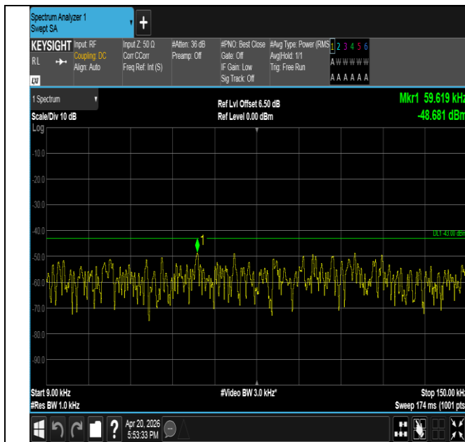
Band25-1.4MHz-16QAM-26047-1RB#5-0.009~0.15-PASS
