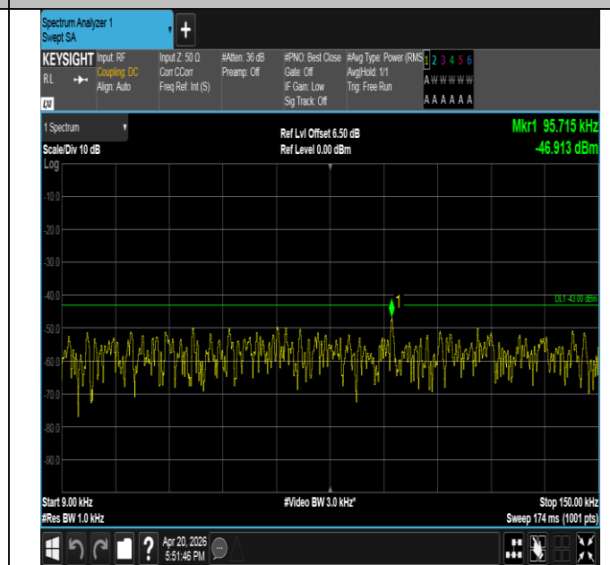
Band25-1.4MHz-16QAM-26047-1RB#0-0.009~0.15-PASS
