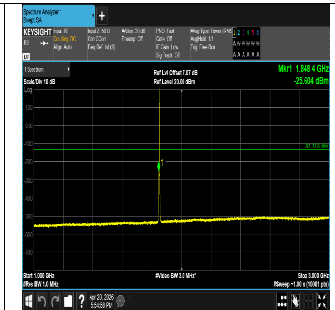
Band25-1.4MHz-QPSK-26047-6RB#0-1000~3000-PASS
