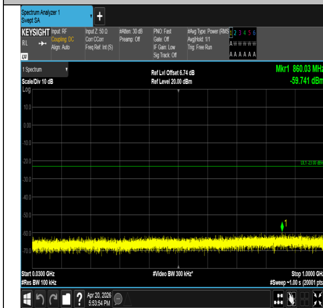
Band25-1.4MHz-16QAM-26047-1RB#5-30~1000-PASS
