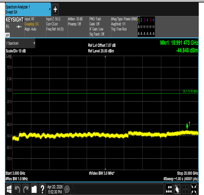
Band25-1.4MHz-16QAM-26047-1RB#0-3000~20000-PASS
