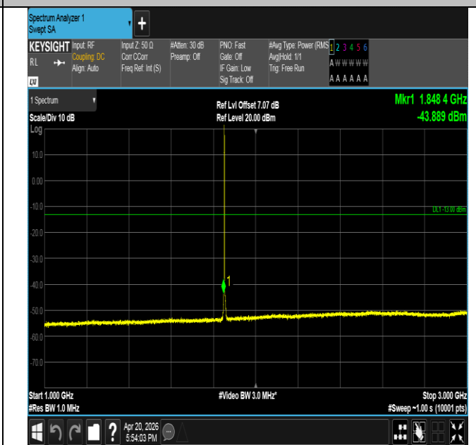
Band25-1.4MHz-16QAM-26047-1RB#5-1000~3000-PASS
