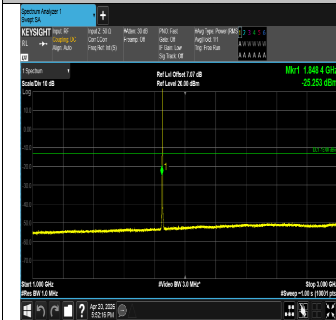
Band25-1.4MHz-16QAM-26047-1RB#0-1000~3000-PASS
