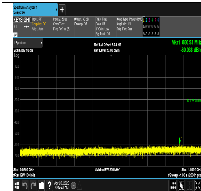
Band25-1.4MHz-QPSK-26047-6RB#0-30~1000-PASS
