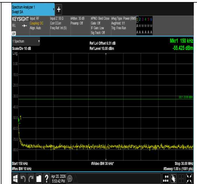
Band25-1.4MHz-16QAM-26047-1RB#5-0.15~30-PASS
