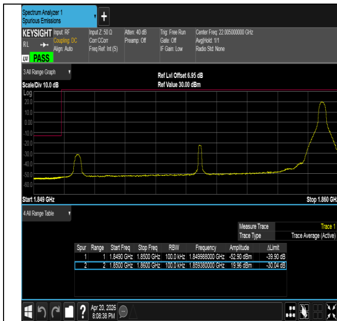
Band25-10MHz-16QAM-26090-1RB#49-PASS
