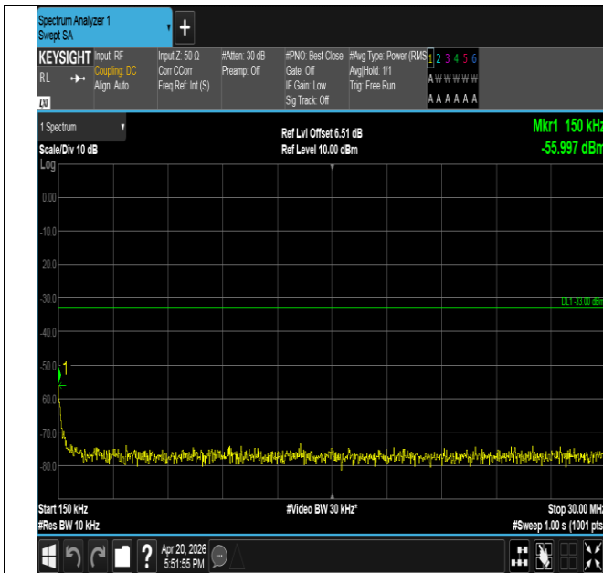
Band25-1.4MHz-16QAM-26047-1RB#0-0.15~30-PASS
