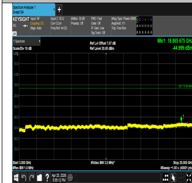
Band25-1.4MHz-QPSK-26047-6RB#0-3000~20000-PASS
