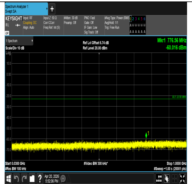
Band25-1.4MHz-16QAM-26047-1RB#0-30~1000-PASS
