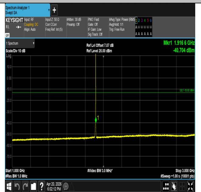
Band25-1.4MHz-QPSK-26683-1RB#0-1000~3000-PASS
