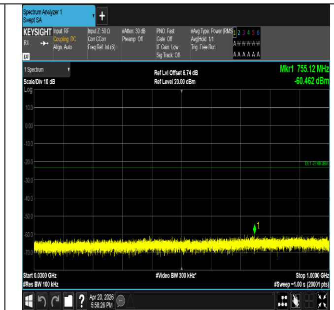
Band25-1.4MHz-QPSK-26365-1RB#5-30~1000-PASS
