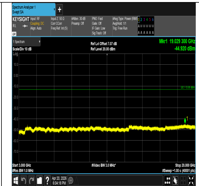
Band25-1.4MHz-QPSK-26683-1RB#5-3000~20000-PASS
