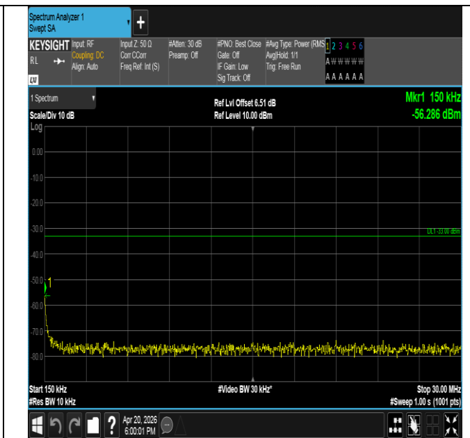
Band25-1.4MHz-QPSK-26365-6RB#0-0.15~30-PASS
