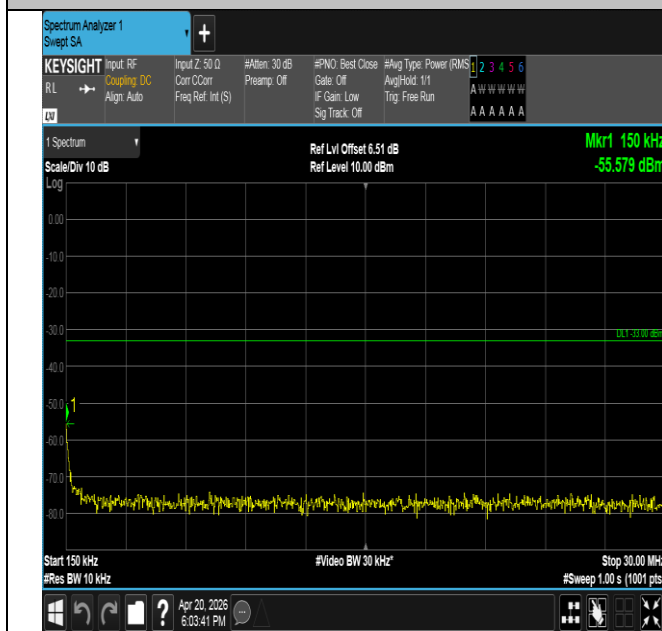
Band25-1.4MHz-QPSK-26683-1RB#5-0.15~30-PASS
