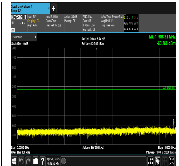
Band25-1.4MHz-16QAM-26683-1RB#0-30~1000-PASS
