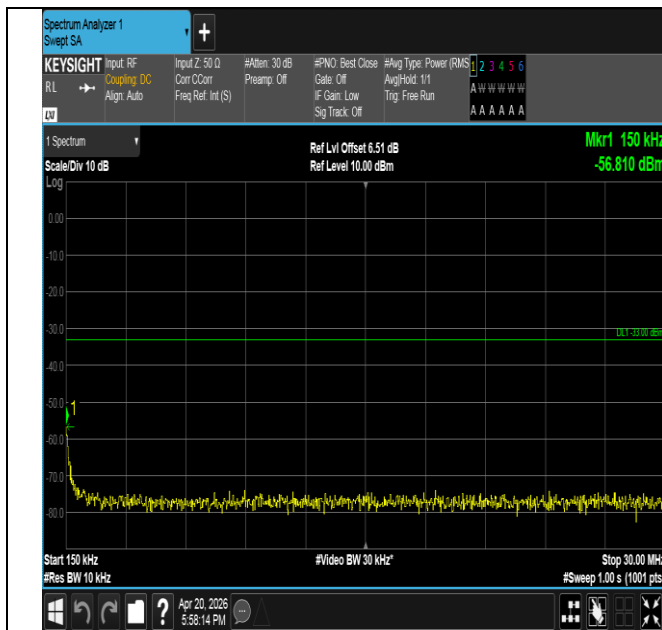
Band25-1.4MHz-QPSK-26365-1RB#5-0.15~30-PASS
