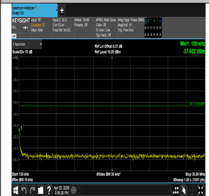
Band25-1.4MHz-QPSK-26365-1RB#0-0.15~30-PASS
