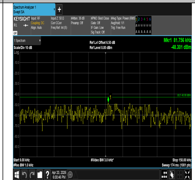
Band25-1.4MHz-16QAM-26365-6RB#0-0.009~0.15-PASS
