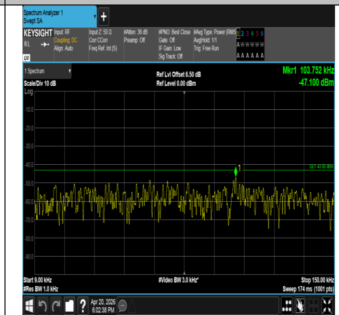
Band25-1.4MHz-16QAM-26683-1RB#0-0.009~0.15-PASS
