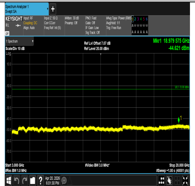
Band25-1.4MHz-16QAM-26365-6RB#0-3000~20000-PASS
