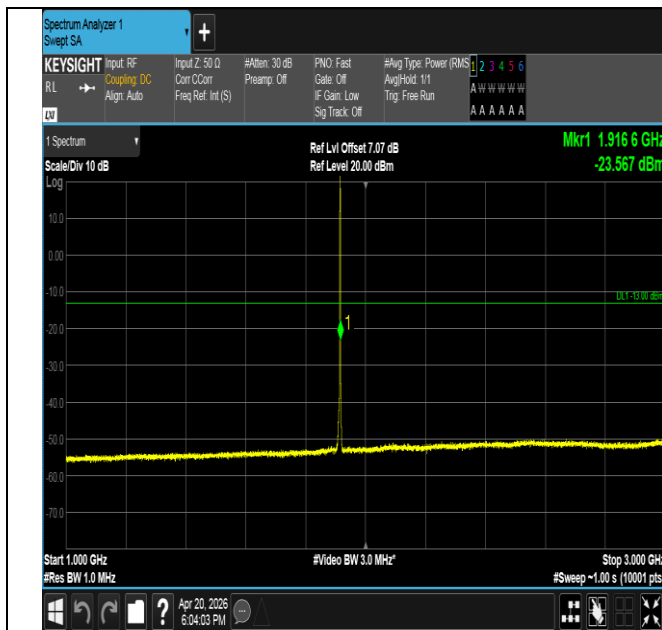
Band25-1.4MHz-QPSK-26683-1RB#5-1000~3000-PASS
