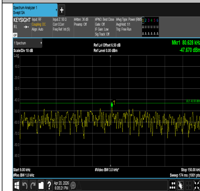
Band25-1.4MHz-QPSK-26683-6RB#0-0.009~0.15-PASS
