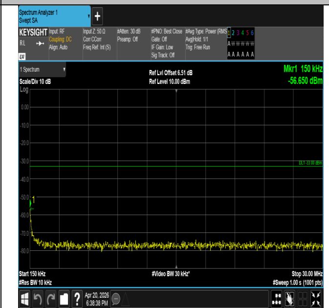
Band25-3MHz-QPSK-26055-1RB#0-0.15~30-PASS
