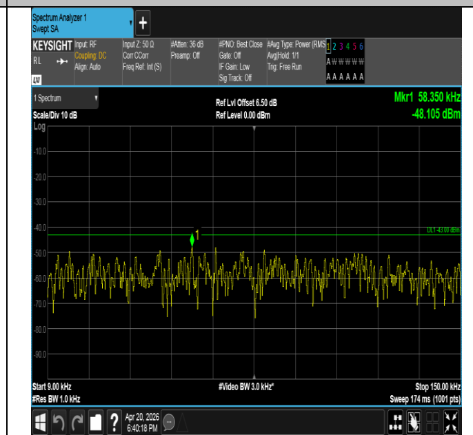
Band25-3MHz-QPSK-26055-1RB#14-0.009~0.15-PASS
