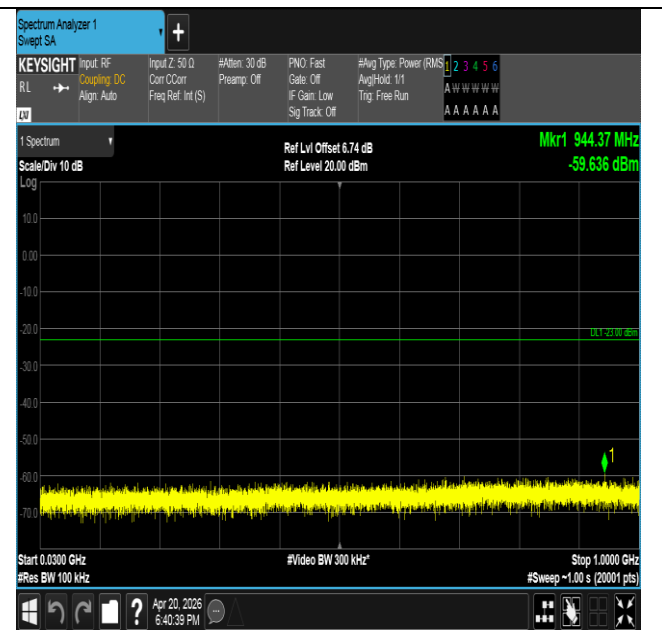
Band25-3MHz-QPSK-26055-1RB#14-30~1000-PASS
