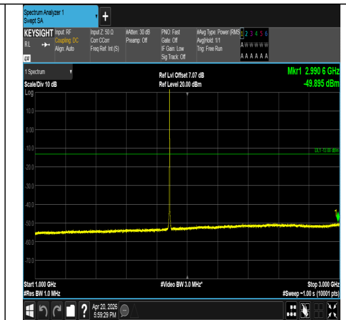
Band25-1.4MHz-16QAM-26365-1RB#5-1000~3000-PASS
