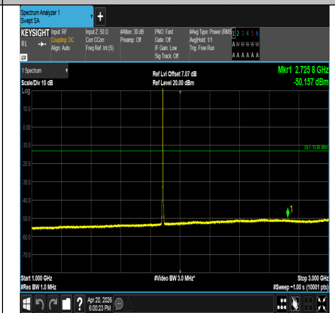
Band25-1.4MHz-QPSK-26365-6RB#0-1000~3000-PASS
