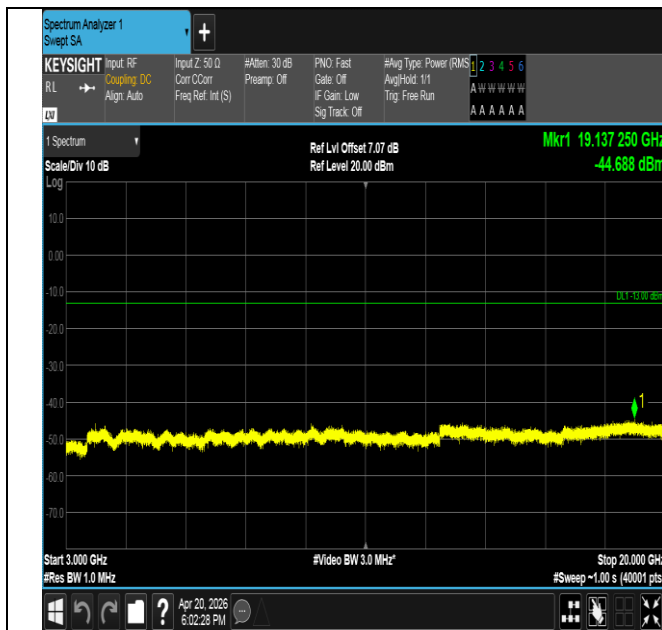
Band25-1.4MHz-QPSK-26683-1RB#0-3000~20000-PASS
