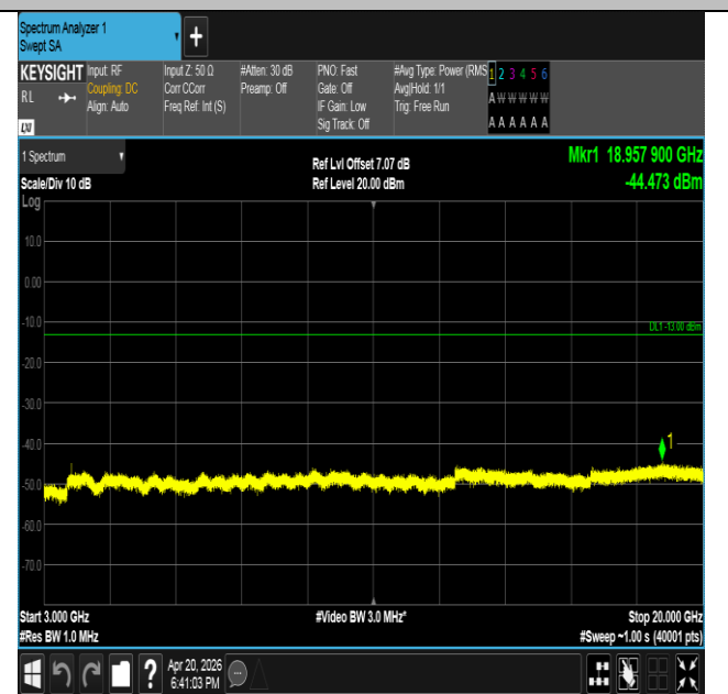
Band25-3MHz-QPSK-26055-1RB#14-3000~20000-PASS
