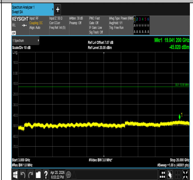
Band25-1.4MHz-16QAM-26683-1RB#0-3000~20000-PASS
