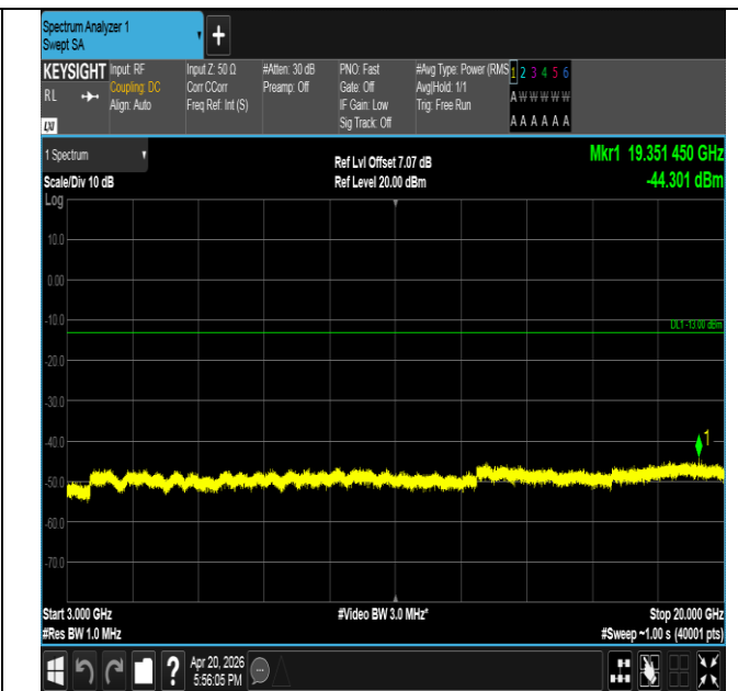
Band25-1.4MHz-16QAM-26047-6RB#0-3000~20000-PASS
