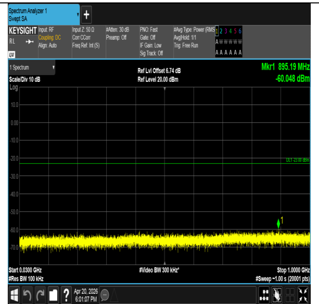
Band25-1.4MHz-16QAM-26365-6RB#0-30~1000-PASS
