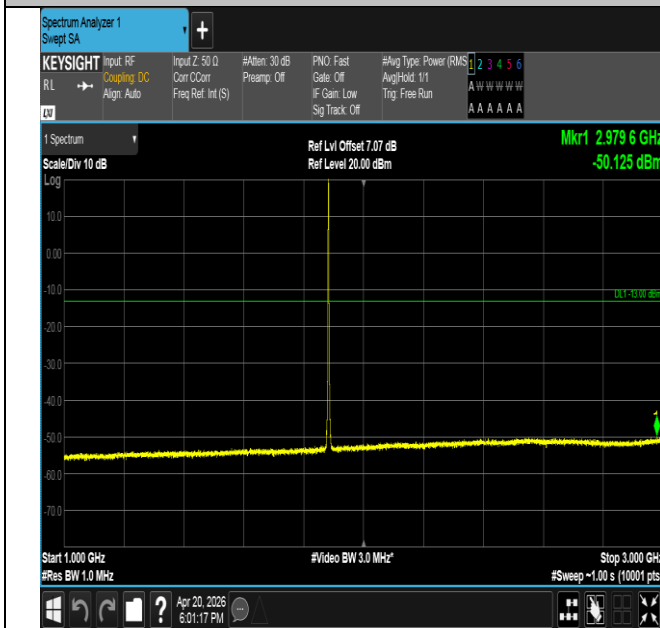
Band25-1.4MHz-16QAM-26365-6RB#0-1000~3000-PASS
