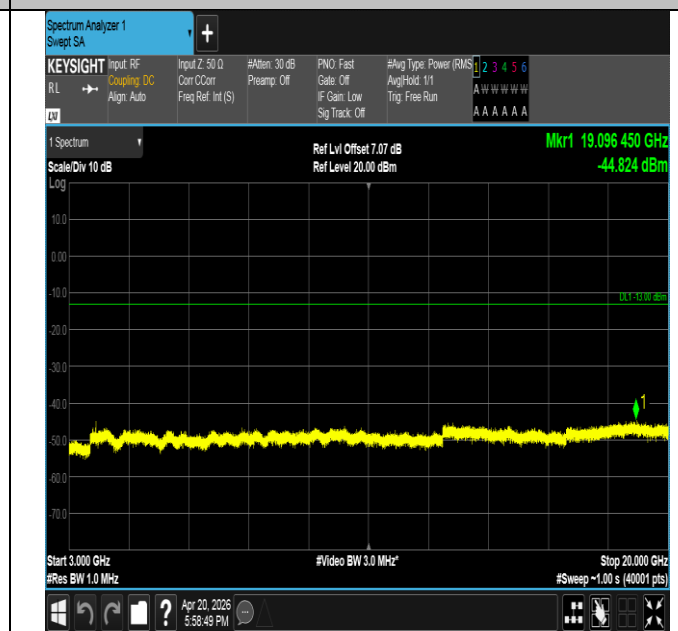
Band25-1.4MHz-QPSK-26365-1RB#5-3000~20000-PASS
