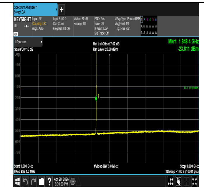
Band25-3MHz-QPSK-26055-1RB#0-1000~3000-PASS
