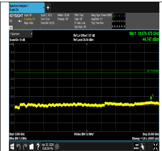
Band25-1.4MHz-16QAM-26683-6RB#0-3000~20000-PASS
