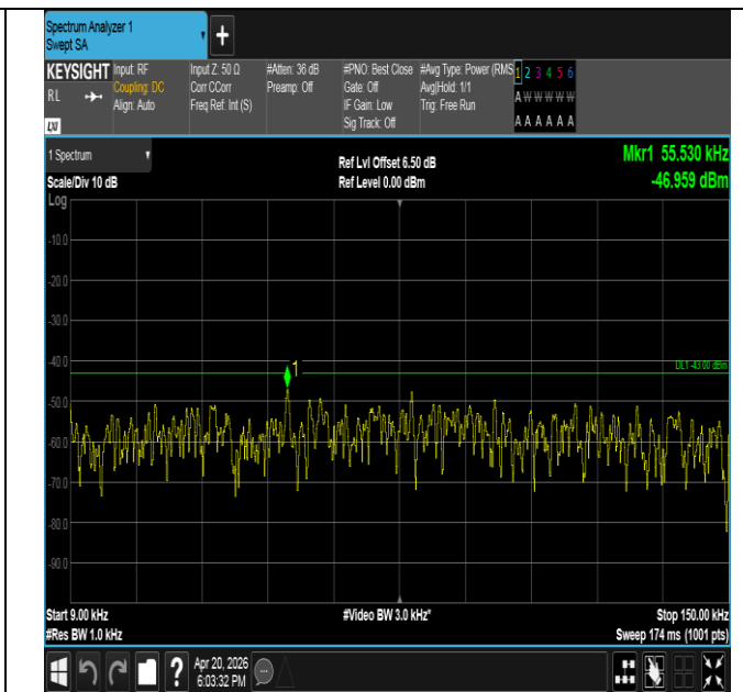
Band25-1.4MHz-QPSK-26683-1RB#5-0.009~0.15-PASS
