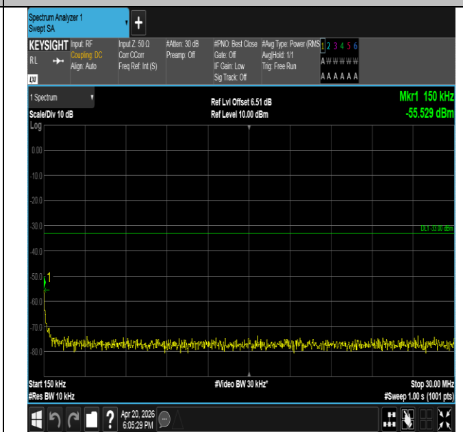
Band25-1.4MHz-QPSK-26683-6RB#0-0.15~30-PASS
