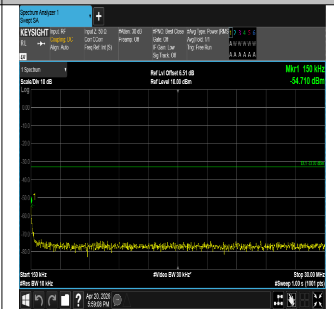
Band25-1.4MHz-16QAM-26365-1RB#5-0.15~30-PASS
