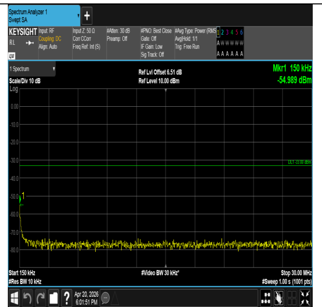
Band25-1.4MHz-QPSK-26683-1RB#0-0.15~30-PASS
