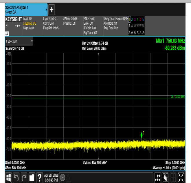
Band25-3MHz-16QAM-26675-1RB#0-30~1000-PASS
