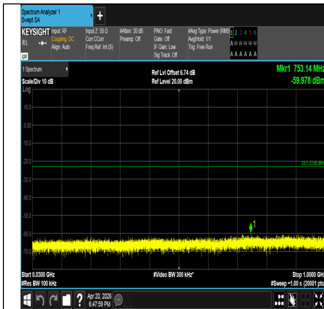
Band25-3MHz-QPSK-26365-15RB#0-30~1000-PASS
