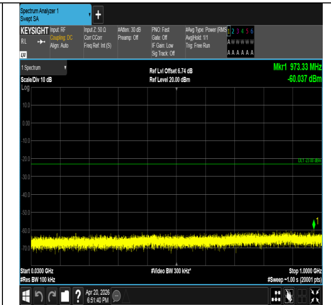
Band25-3MHz-QPSK-26675-1RB#14-30~1000-PASS
