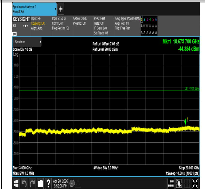
Band25-3MHz-QPSK-26675-1RB#14-3000~20000-PASS
