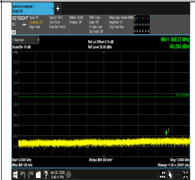
Band25-3MHz-QPSK-26365-1RB#14-30~1000-PASS
