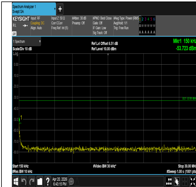
Band25-3MHz-16QAM-26055-15RB#0-0.15~30-PASS
