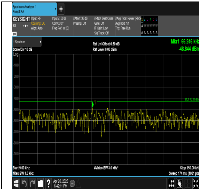
Band25-3MHz-QPSK-26055-15RB#0-0.009~0.15-PASS
