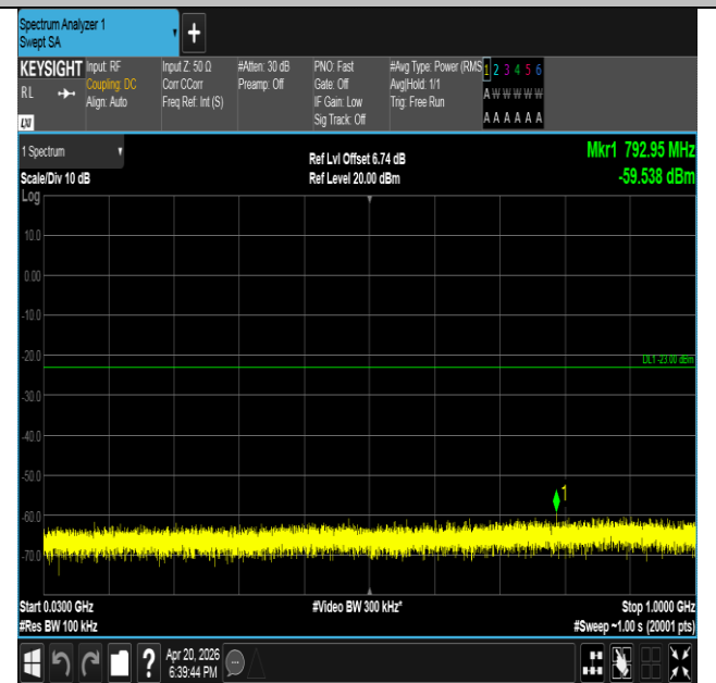
Band25-3MHz-16QAM-26055-1RB#0-30~1000-PASS
