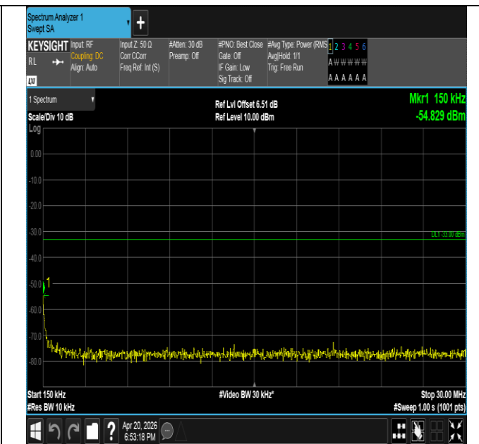
Band25-3MHz-QPSK-26675-15RB#0-0.15~30-PASS
