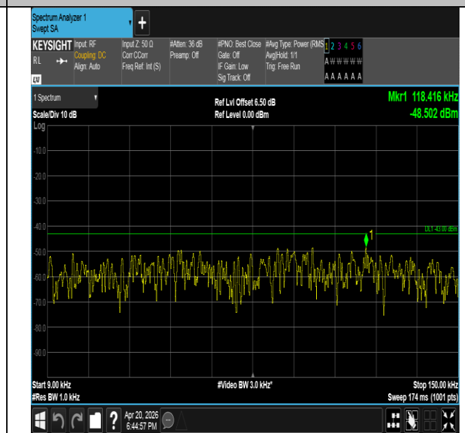
Band25-3MHz-16QAM-26365-1RB#0-0.009~0.15-PASS
