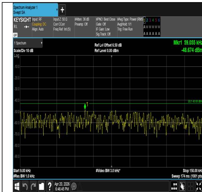
Band25-3MHz-16QAM-26365-1RB#14-0.009~0.15-PASS
