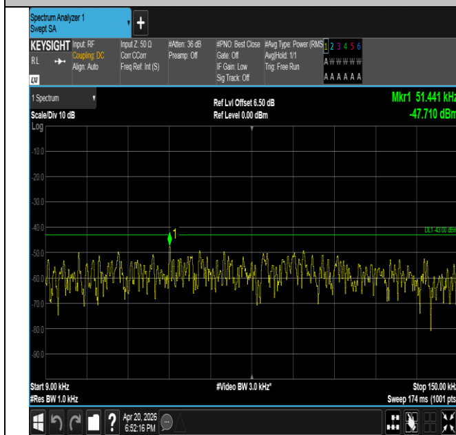
Band25-3MHz-16QAM-26675-1RB#14-0.009~0.15-PASS
