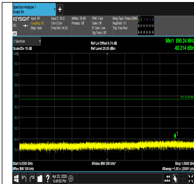
Band25-3MHz-QPSK-26675-1RB#0-30~1000-PASS
