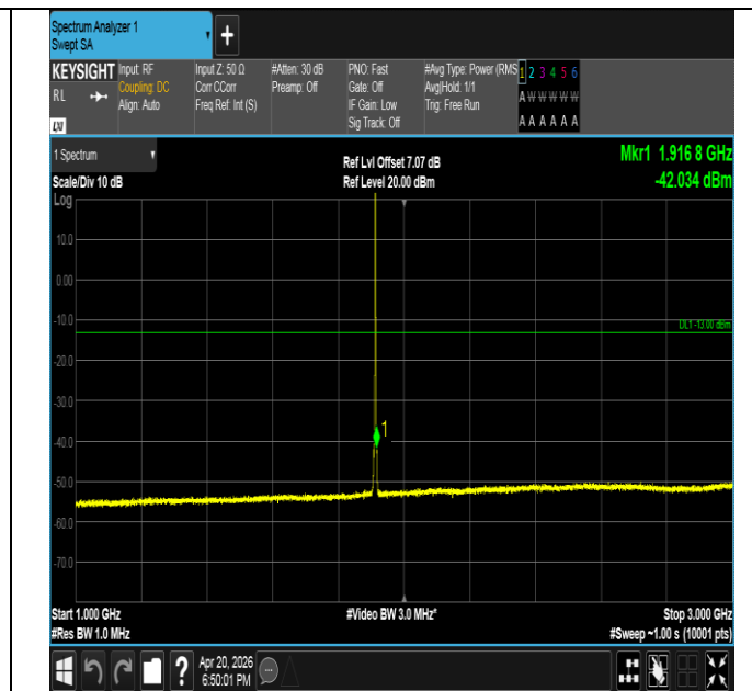
Band25-3MHz-QPSK-26675-1RB#0-1000~3000-PASS
