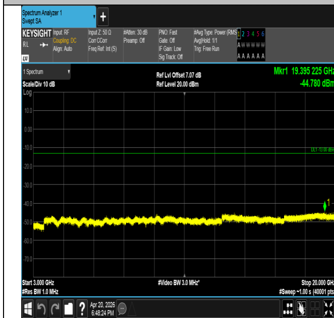
Band25-3MHz-QPSK-26365-15RB#0-3000~20000-PASS
