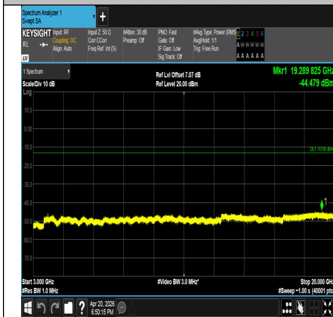
Band25-3MHz-QPSK-26675-1RB#0-3000~20000-PASS
