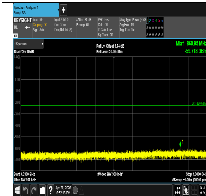
Band25-3MHz-16QAM-26675-1RB#14-30~1000-PASS
