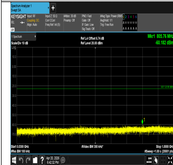
Band25-3MHz-QPSK-26055-15RB#0-30~1000-PASS
