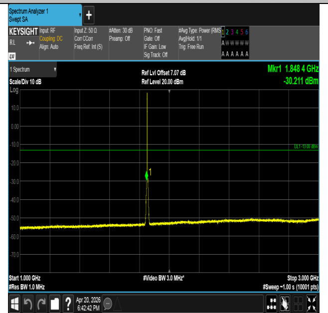
Band25-3MHz-QPSK-26055-15RB#0-1000~3000-PASS
