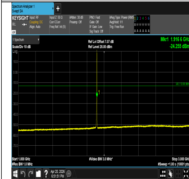
Band25-3MHz-QPSK-26675-1RB#14-1000~3000-PASS
