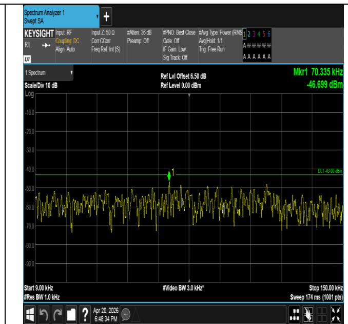
Band25-3MHz-16QAM-26365-15RB#0-0.009~0.15-PASS
