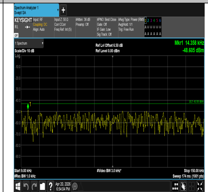
Band25-3MHz-16QAM-26675-15RB#0-0.009~0.15-PASS
