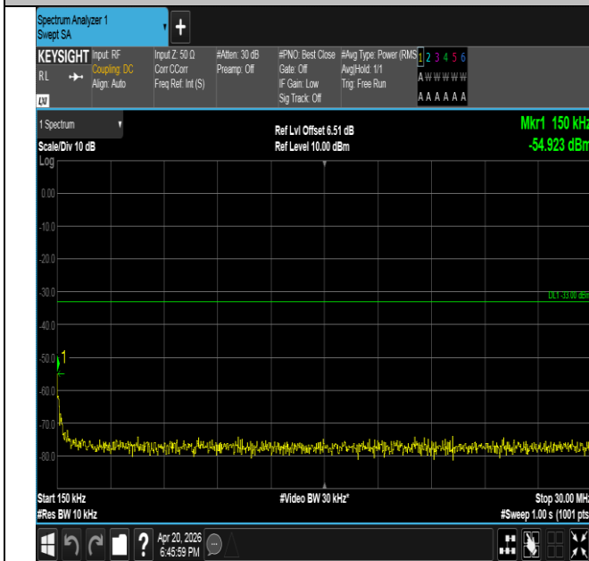
Band25-3MHz-QPSK-26365-1RB#14-0.15~30-PASS
