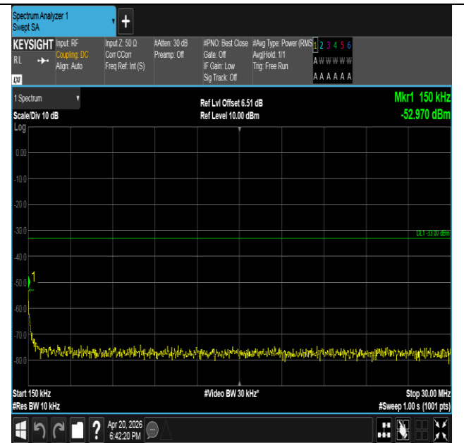
Band25-3MHz-QPSK-26055-15RB#0-0.15~30-PASS
