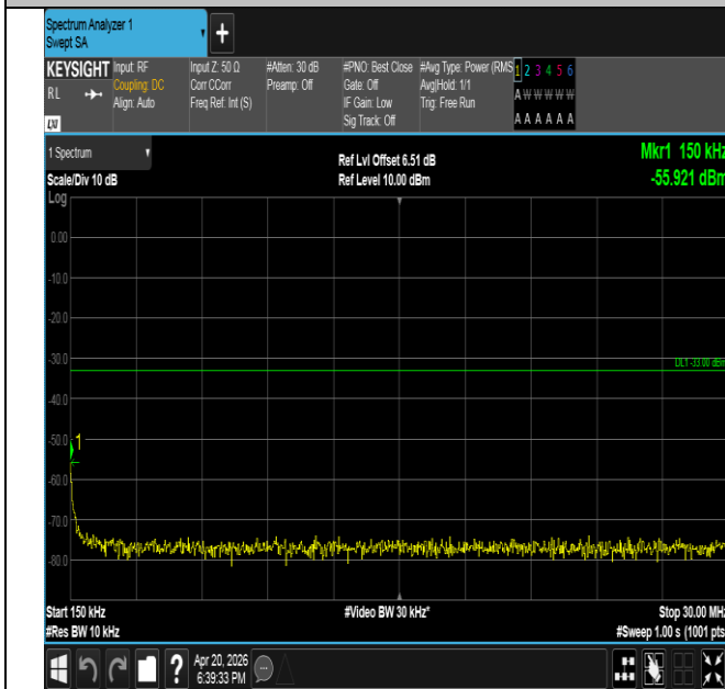
Band25-3MHz-16QAM-26055-1RB#0-0.15~30-PASS
