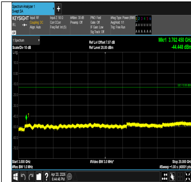
Band25-3MHz-QPSK-26365-1RB#0-3000~20000-PASS
