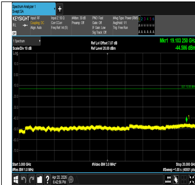
Band25-3MHz-QPSK-26055-15RB#0-3000~20000-PASS
