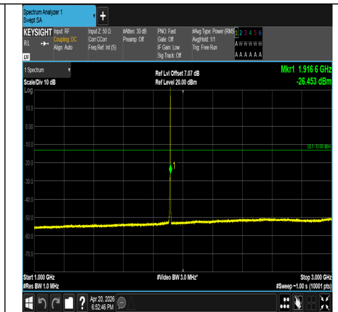
Band25-3MHz-16QAM-26675-1RB#14-1000~3000-PASS
