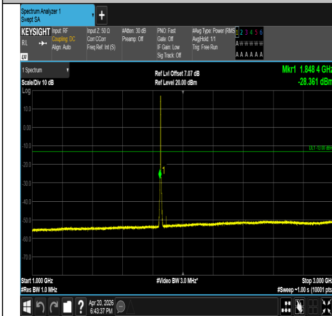
Band25-3MHz-16QAM-26055-15RB#0-1000~3000-PASS
