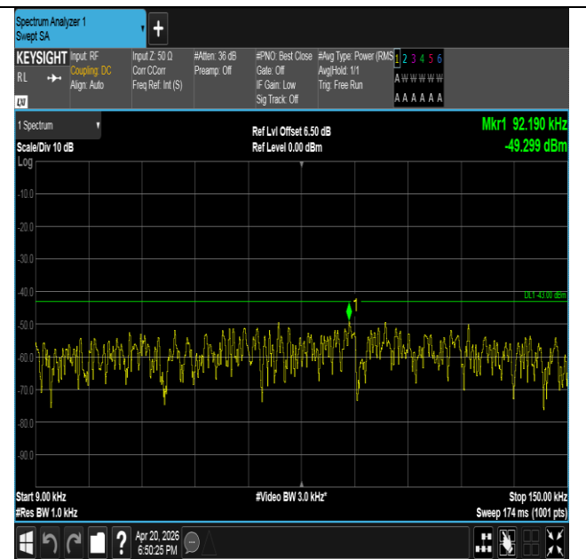
Band25-3MHz-16QAM-26675-1RB#0-0.009~0.15-PASS
