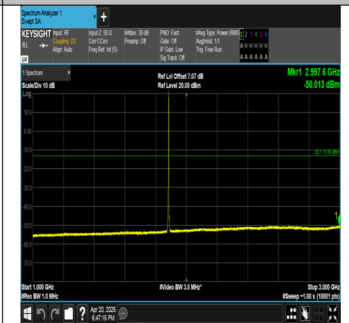
Band25-3MHz-16QAM-26365-1RB#14-1000~3000-PASS
