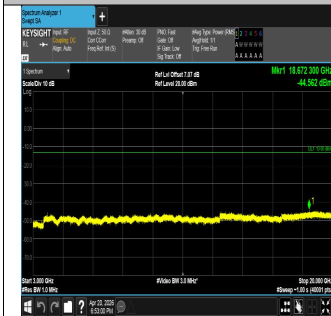
Band25-3MHz-16QAM-26675-1RB#14-3000~20000-PASS
