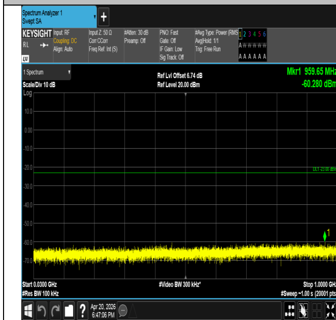
Band25-3MHz-16QAM-26365-1RB#14-30~1000-PASS
