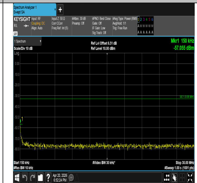
Band25-3MHz-16QAM-26675-1RB#14-0.15~30-PASS
