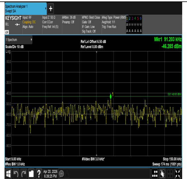
Band25-3MHz-16QAM-26055-1RB#0-0.009~0.15-PASS
