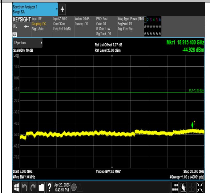
Band25-3MHz-16QAM-26055-15RB#0-3000~20000-PASS
