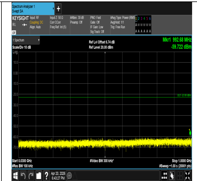
Band25-3MHz-16QAM-26055-15RB#0-30~1000-PASS
