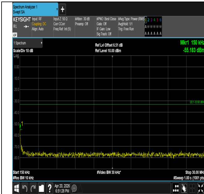
Band25-3MHz-QPSK-26675-1RB#14-0.15~30-PASS
