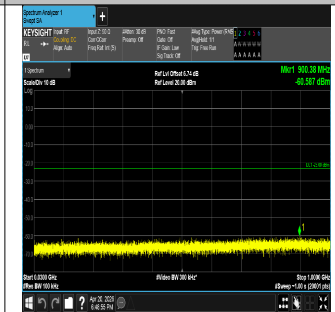
Band25-3MHz-16QAM-26365-15RB#0-30~1000-PASS
