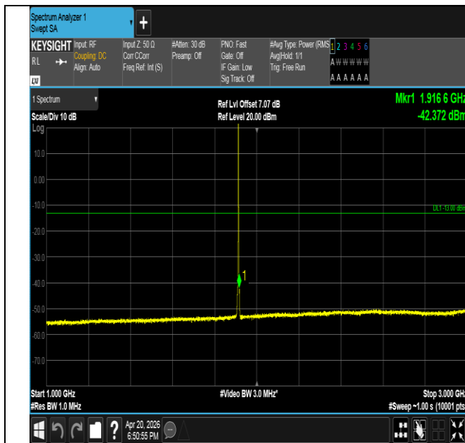
Band25-3MHz-16QAM-26675-1RB#0-1000~3000-PASS
