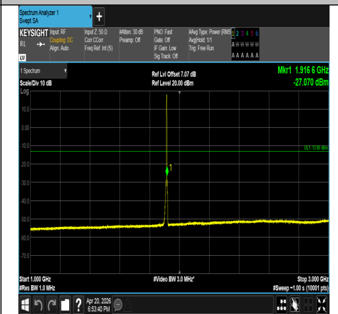
Band25-3MHz-QPSK-26675-15RB#0-1000~3000-PASS
