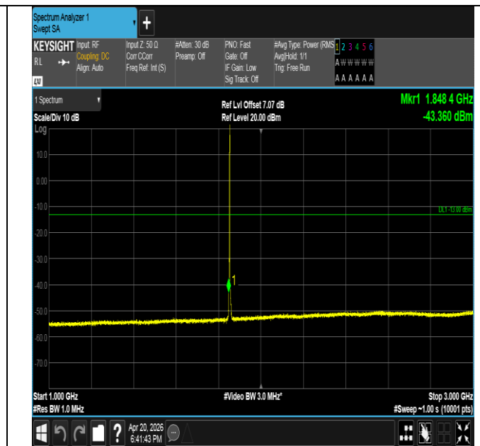
Band25-3MHz-16QAM-26055-1RB#14-1000~3000-PASS
