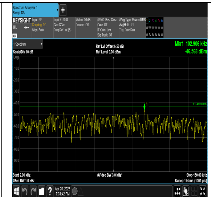
Band25-5MHz-16QAM-26365-1RB#0-0.009~0.15-PASS
