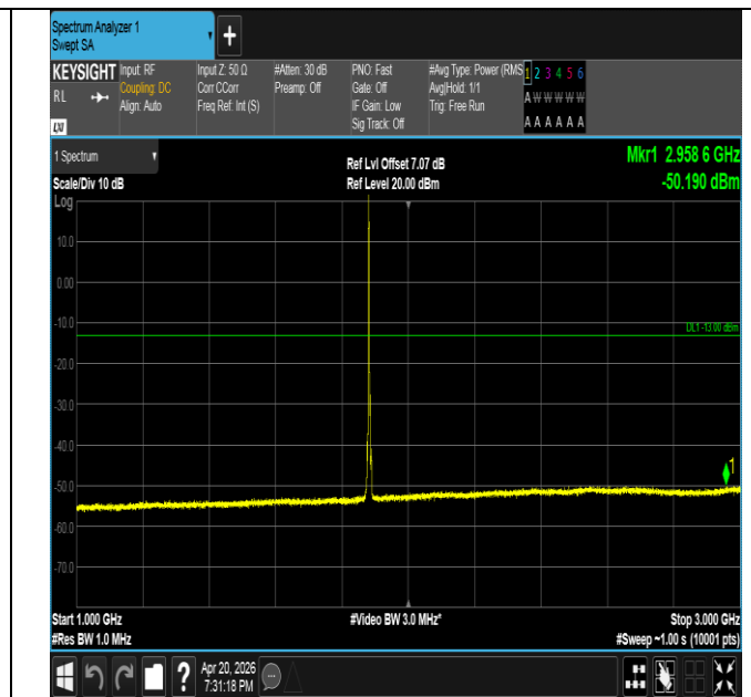
Band25-5MHz-QPSK-26365-1RB#0-1000~3000-PASS
