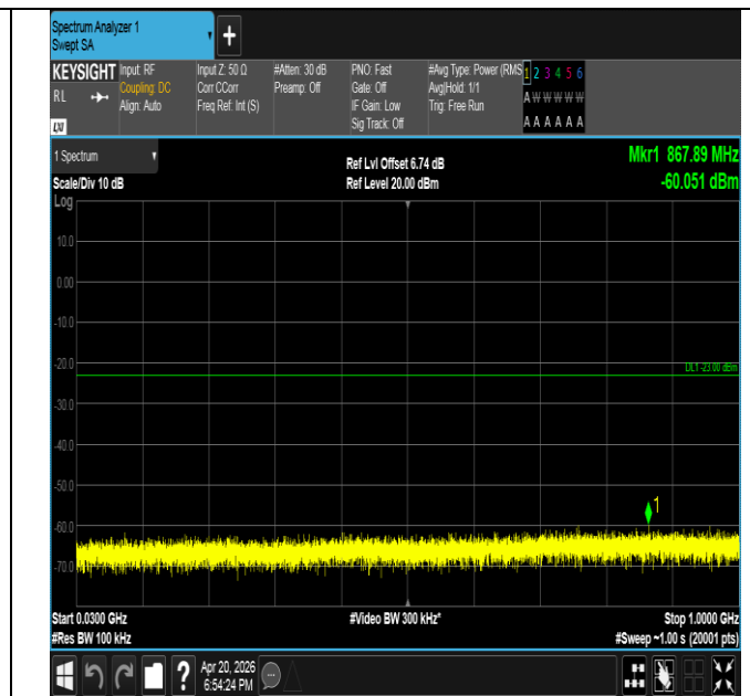
Band25-3MHz-16QAM-26675-15RB#0-30~1000-PASS
