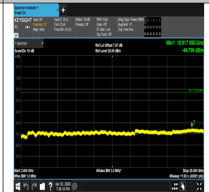
Band25-5MHz-16QAM-26365-25RB#0-3000~20000-PASS
