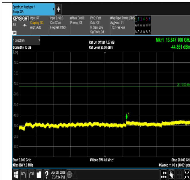
Band25-5MHz-QPSK-26665-1RB#0-3000~20000-PASS
