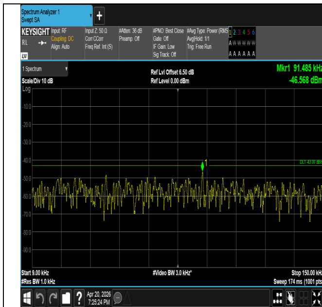
Band25-5MHz-QPSK-26065-1RB#0-0.009~0.15-PASS
