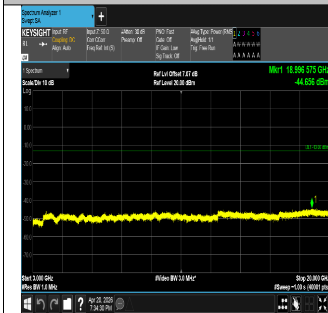
Band25-5MHz-16QAM-26365-1RB#24-3000~20000-PASS
