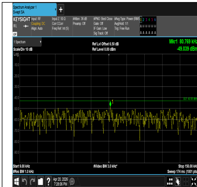
Band25-5MHz-16QAM-26065-1RB#24-0.009~0.15-PASS
