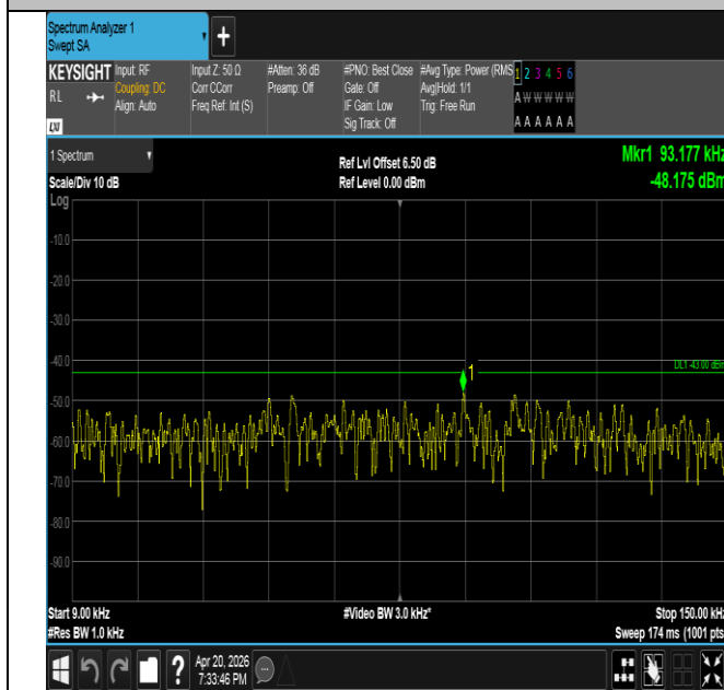
Band25-5MHz-16QAM-26365-1RB#24-0.009~0.15-PASS
