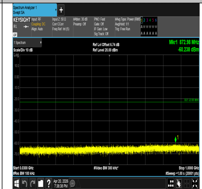
Band25-5MHz-QPSK-26665-1RB#24-30~1000-PASS
