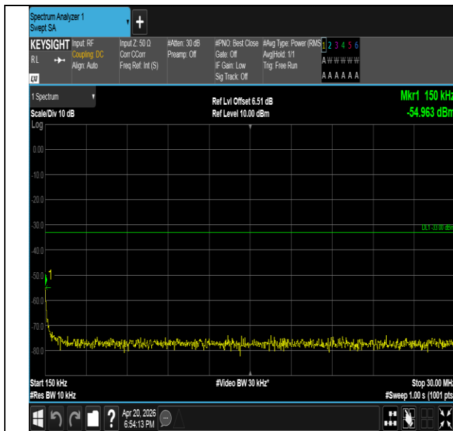
Band25-3MHz-16QAM-26675-15RB#0-0.15~30-PASS
