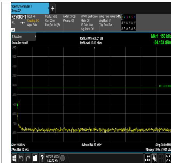
Band25-5MHz-16QAM-26365-25RB#0-0.15~30-PASS
