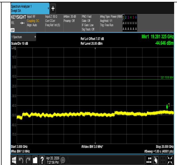
Band25-5MHz-QPSK-26065-1RB#24-3000~20000-PASS
