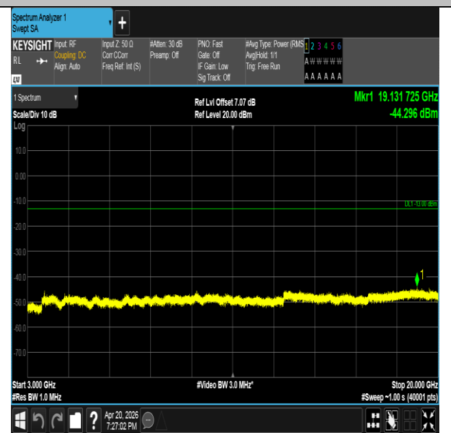
Band25-5MHz-16QAM-26065-1RB#0-3000~20000-PASS
