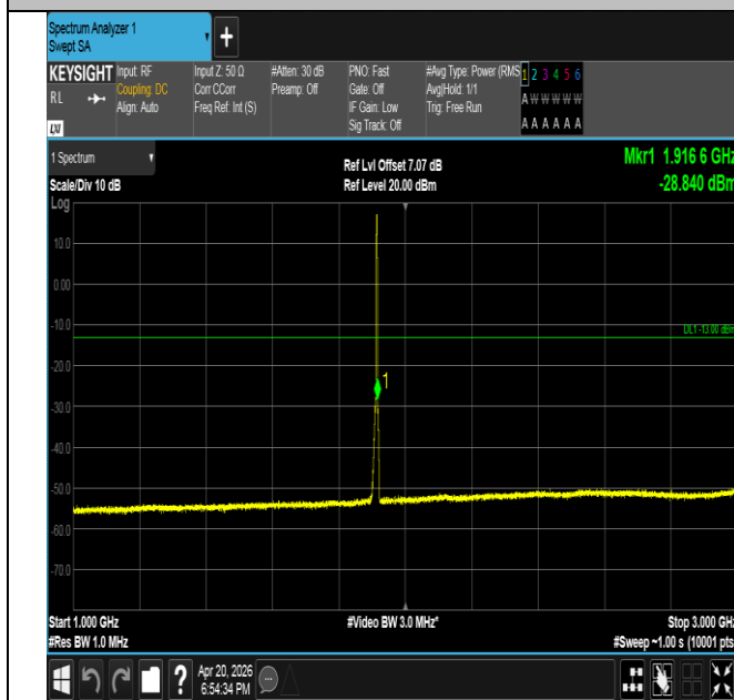
Band25-3MHz-16QAM-26675-15RB#0-1000~3000-PASS
