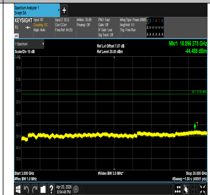
Band25-3MHz-16QAM-26675-15RB#0-3000~20000-PASS
