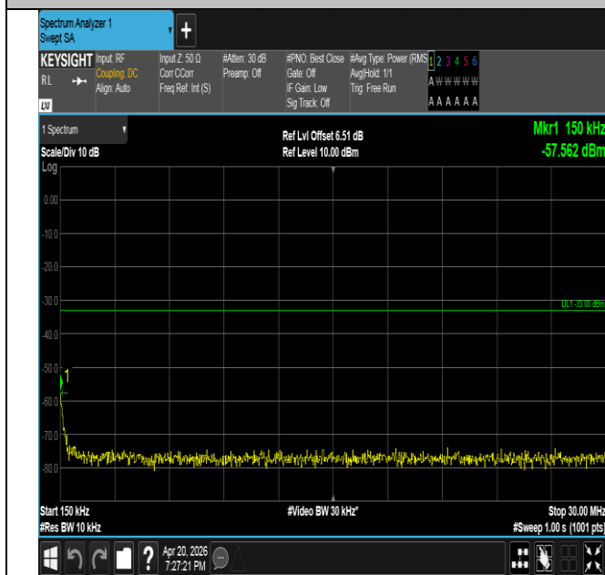
Band25-5MHz-QPSK-26065-1RB#24-0.15~30-PASS
