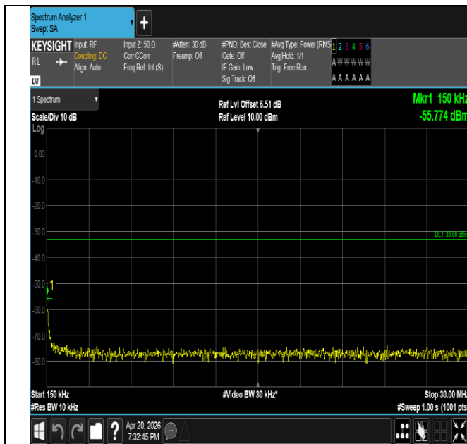
Band25-5MHz-QPSK-26365-1RB#24-0.15~30-PASS
