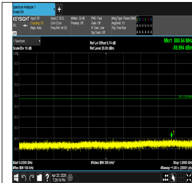
Band25-5MHz-QPSK-26065-25RB#0-30~1000-PASS
