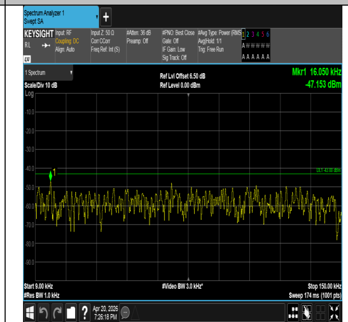
Band25-5MHz-16QAM-26065-1RB#0-0.009~0.15-PASS
