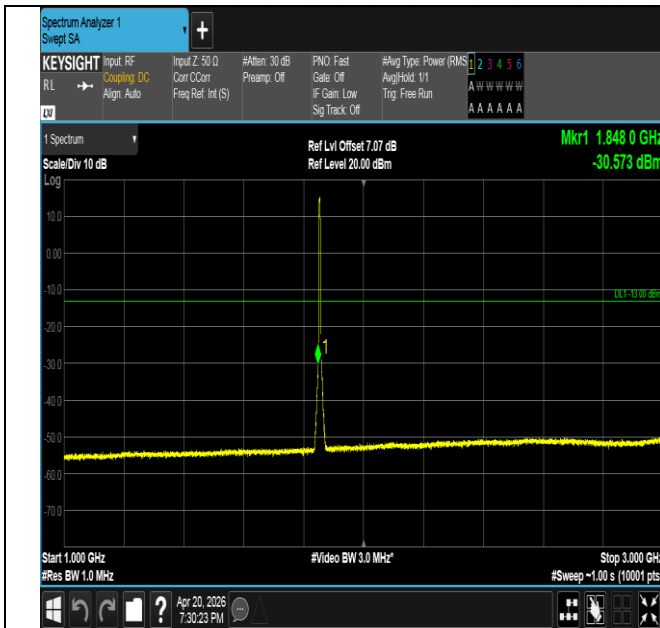
Band25-5MHz-16QAM-26065-25RB#0-1000~3000-PASS
