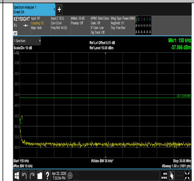
Band25-5MHz-16QAM-26365-1RB#24-0.15~30-PASS
