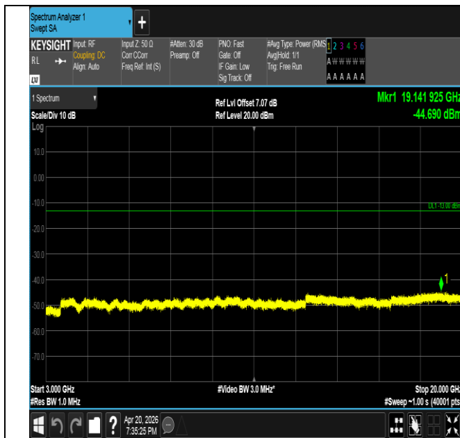
Band25-5MHz-QPSK-26365-25RB#0-3000~20000-PASS
