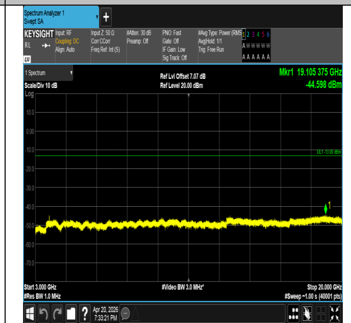
Band25-5MHz-QPSK-26365-1RB#24-3000~20000-PASS
