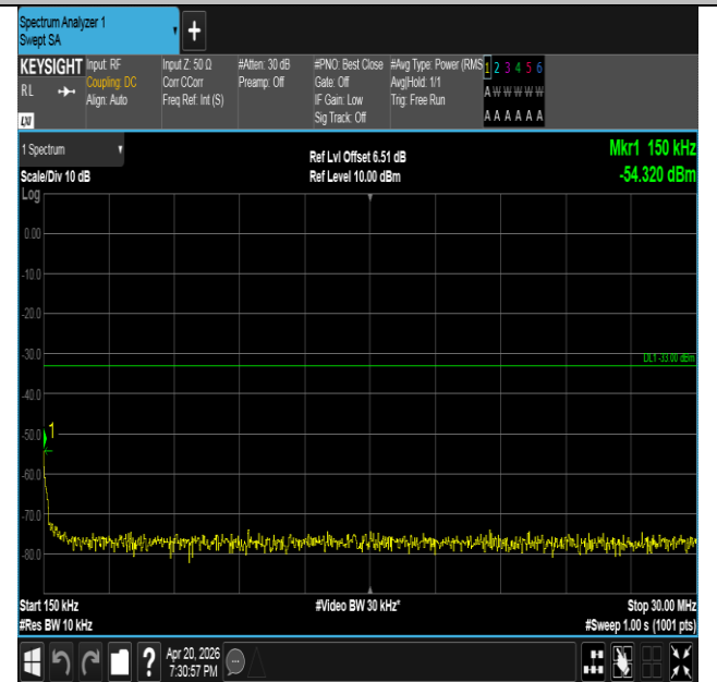
Band25-5MHz-QPSK-26365-1RB#0-0.15~30-PASS
