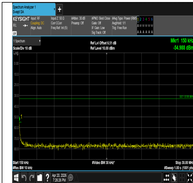
Band25-5MHz-16QAM-26065-1RB#0-0.15~30-PASS
