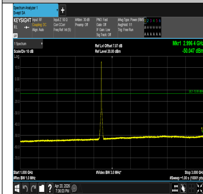
Band25-5MHz-16QAM-26365-25RB#0-1000~3000-PASS
