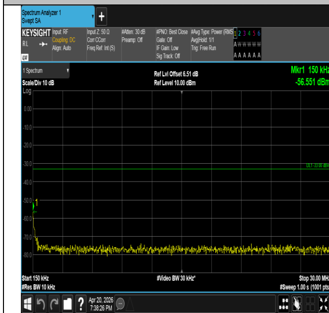
Band25-5MHz-QPSK-26665-1RB#24-0.15~30-PASS
