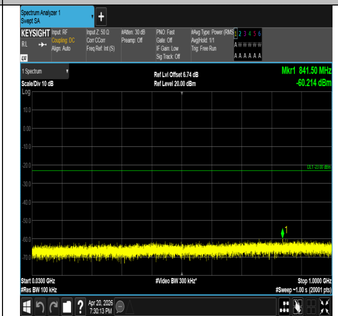
Band25-5MHz-16QAM-26065-25RB#0-30~1000-PASS
