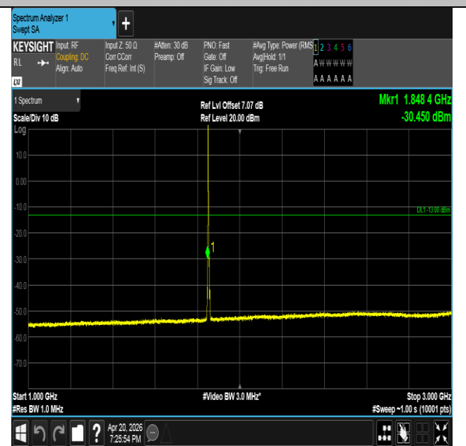
Band25-5MHz-QPSK-26065-1RB#0-1000~3000-PASS
