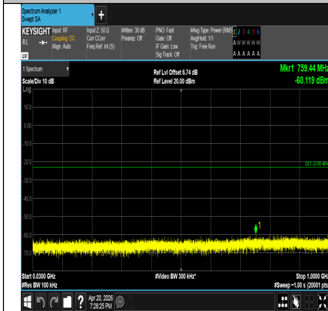
Band25-5MHz-16QAM-26065-1RB#24-30~1000-PASS
