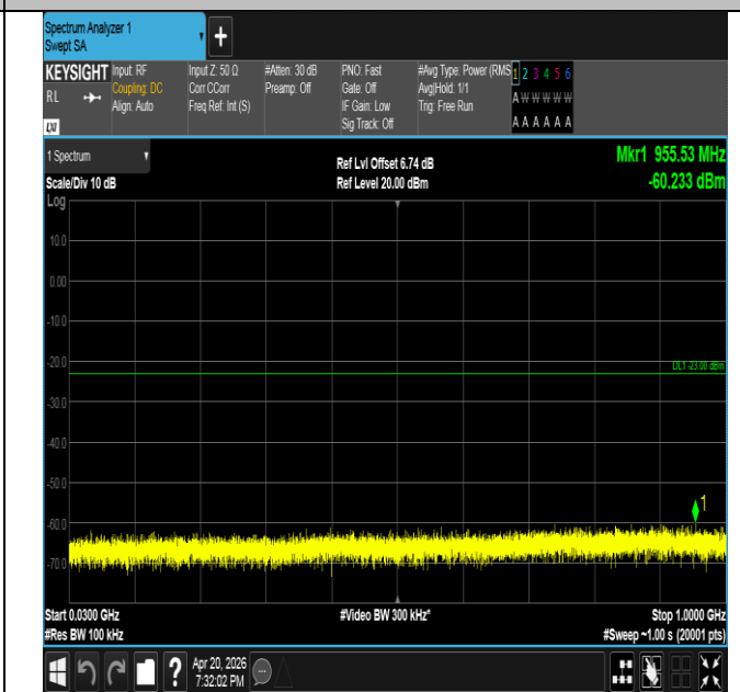
Band25-5MHz-16QAM-26365-1RB#0-30~1000-PASS
