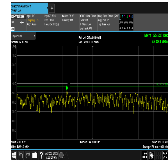
Band25-5MHz-QPSK-26665-1RB#0-0.009~0.15-PASS
