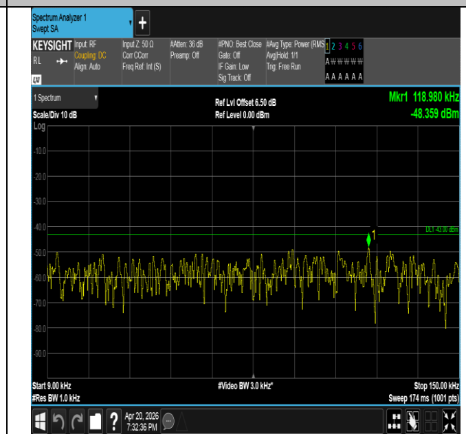
Band25-5MHz-QPSK-26365-1RB#24-0.009~0.15-PASS
