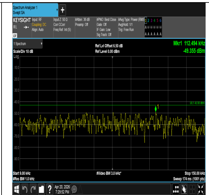
Band25-5MHz-16QAM-26065-25RB#0-0.009~0.15-PASS
