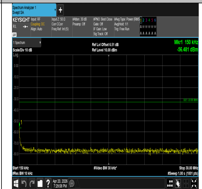
Band25-5MHz-QPSK-26065-25RB#0-0.15~30-PASS
