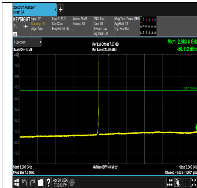
Band25-5MHz-16QAM-26365-1RB#0-1000~3000-PASS
