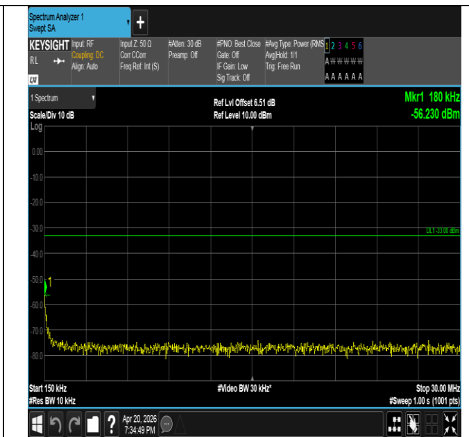
Band25-5MHz-QPSK-26365-25RB#0-0.15~30-PASS
