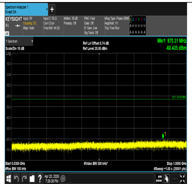
Band25-5MHz-16QAM-26065-1RB#0-30~1000-PASS
