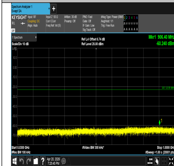
Band25-5MHz-QPSK-26065-1RB#0-30~1000-PASS
