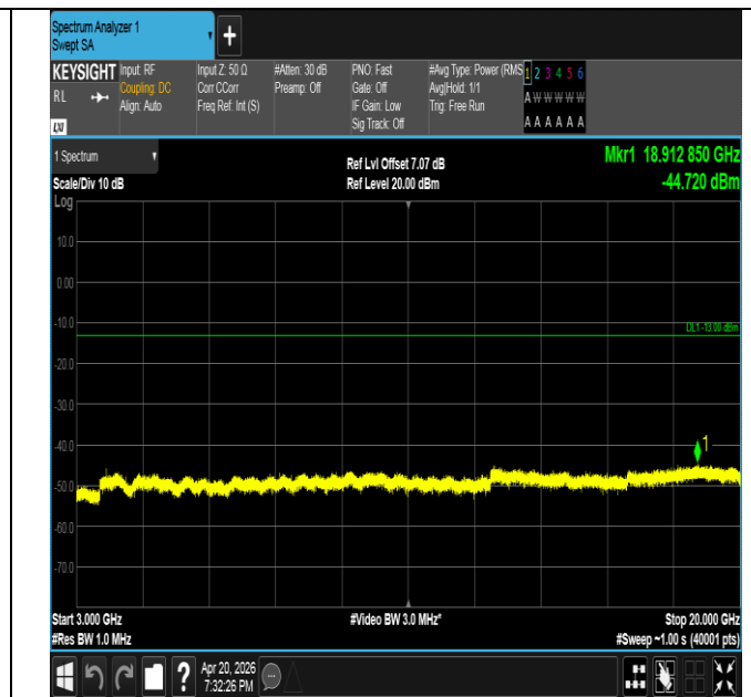
Band25-5MHz-16QAM-26365-1RB#0-3000~20000-PASS
