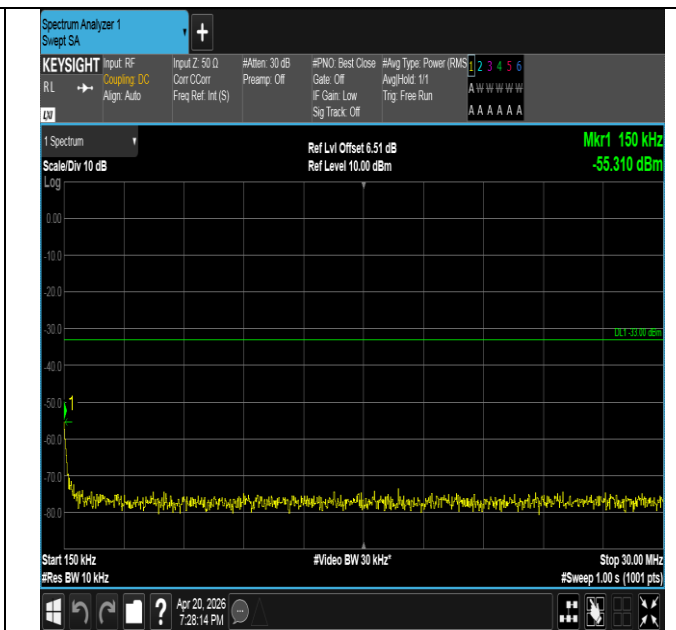
Band25-5MHz-16QAM-26065-1RB#24-0.15~30-PASS
