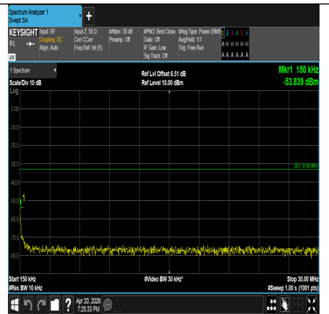
Band25-5MHz-QPSK-26065-1RB#0-0.15~30-PASS
