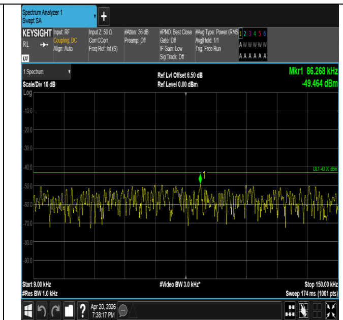
Band25-5MHz-QPSK-26665-1RB#24-0.009~0.15-PASS
