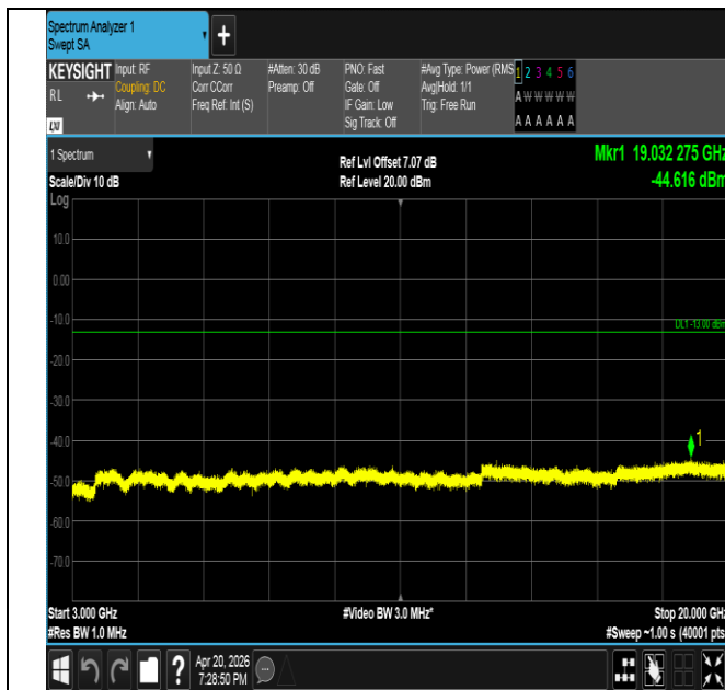
Band25-5MHz-16QAM-26065-1RB#24-3000~20000-PASS
