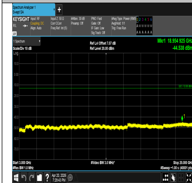
Band25-5MHz-QPSK-26065-25RB#0-3000~20000-PASS
