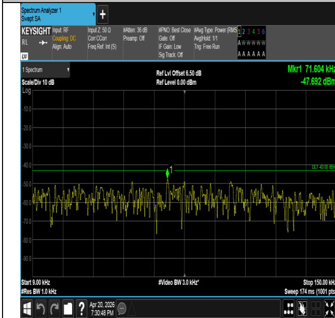
Band25-5MHz-QPSK-26365-1RB#0-0.009~0.15-PASS
