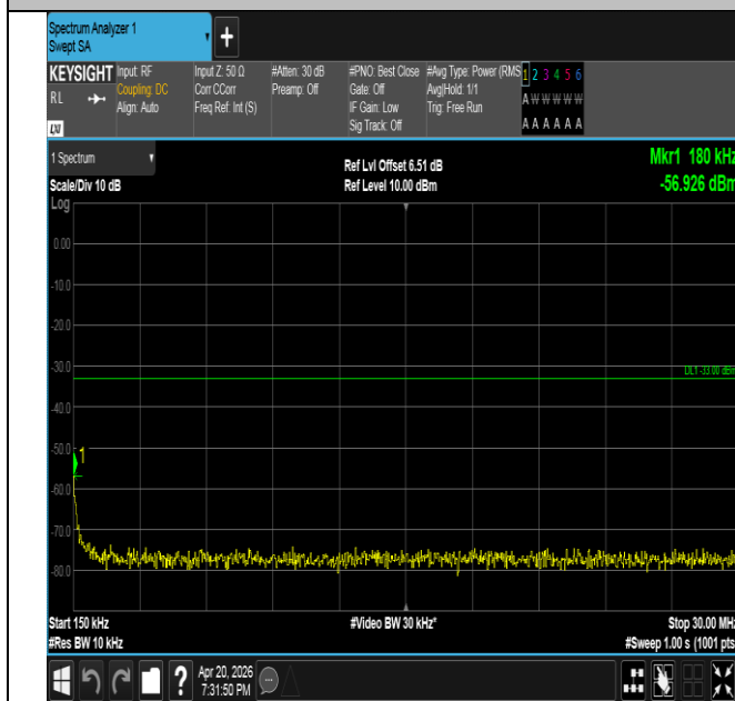
Band25-5MHz-16QAM-26365-1RB#0-0.15~30-PASS
