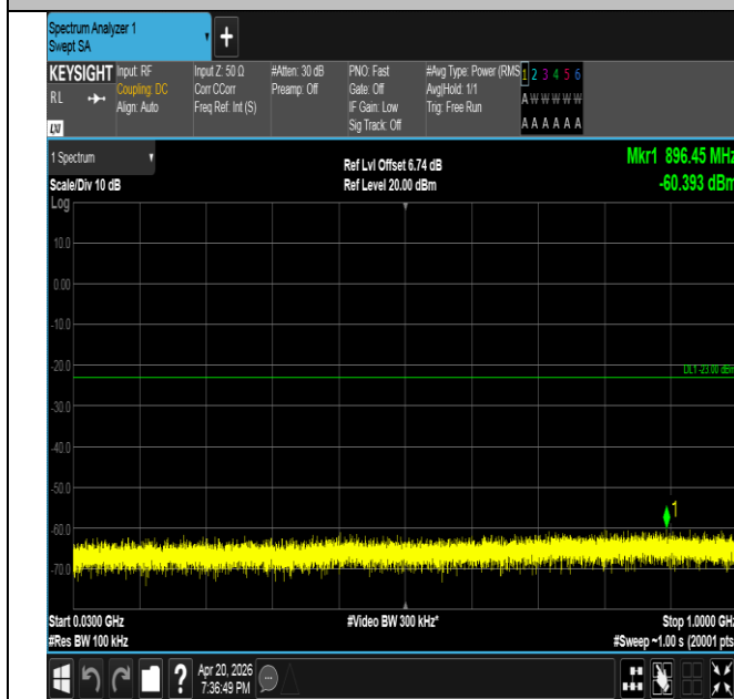
Band25-5MHz-QPSK-26665-1RB#0-30~1000-PASS
