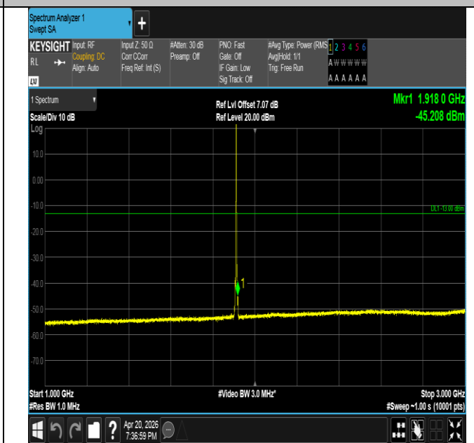
Band25-5MHz-QPSK-26665-1RB#0-1000~3000-PASS
