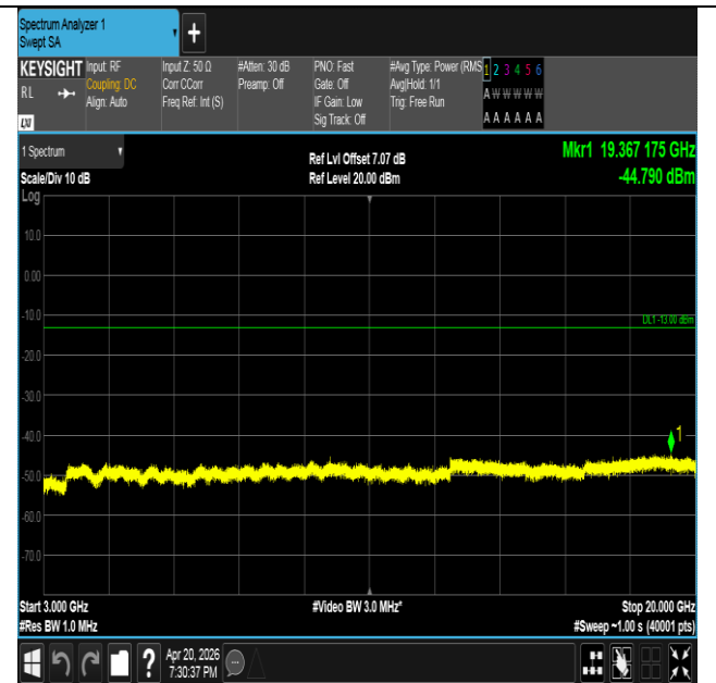
Band25-5MHz-16QAM-26065-25RB#0-3000~20000-PASS
