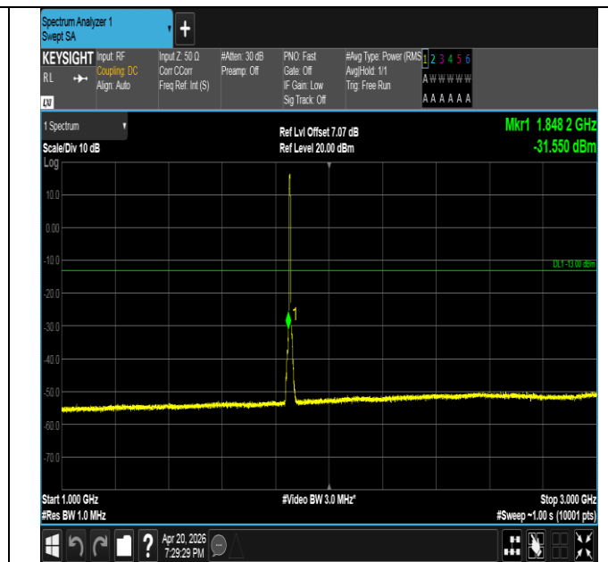
Band25-5MHz-QPSK-26065-25RB#0-1000~3000-PASS
