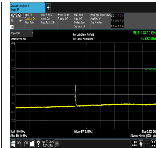
Band25-5MHz-QPSK-26065-1RB#24-1000~3000-PASS
