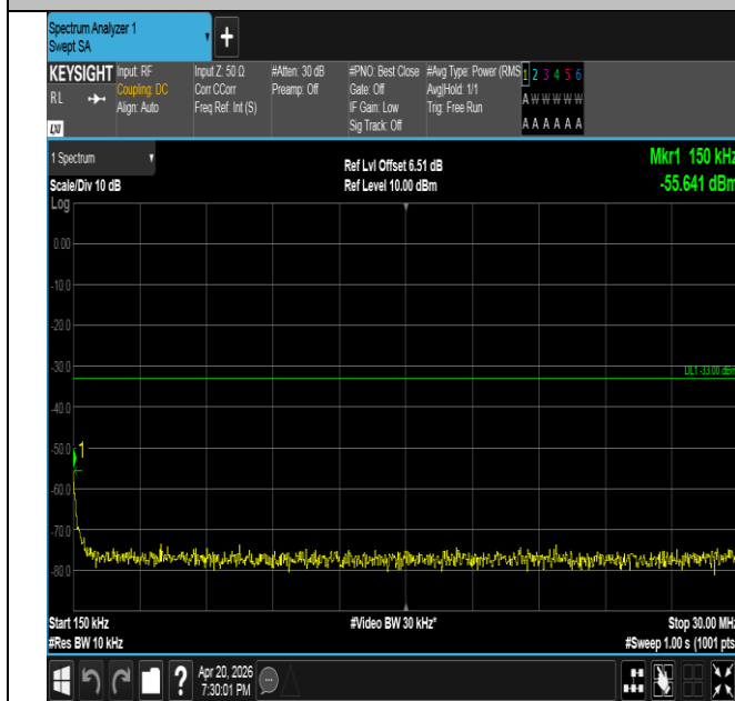
Band25-5MHz-16QAM-26065-25RB#0-0.15~30-PASS
