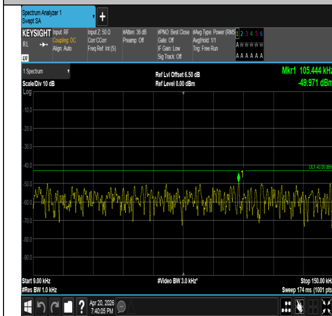
Band25-5MHz-QPSK-26665-25RB#0-0.009~0.15-PASS
