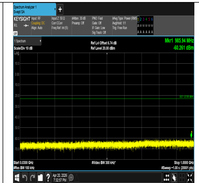
Band25-5MHz-QPSK-26365-1RB#24-30~1000-PASS
