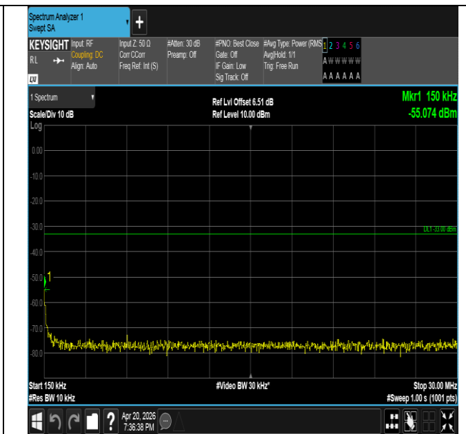
Band25-5MHz-QPSK-26665-1RB#0-0.15~30-PASS
