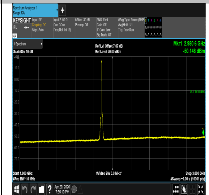
Band25-5MHz-QPSK-26365-25RB#0-1000~3000-PASS
