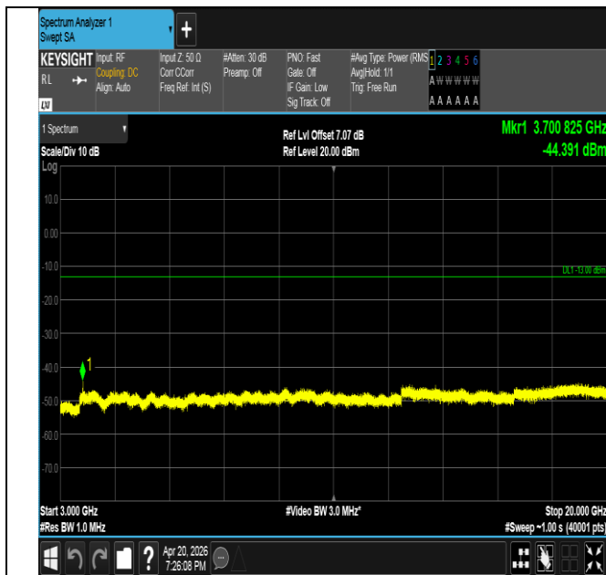
Band25-5MHz-QPSK-26065-1RB#0-3000~20000-PASS
