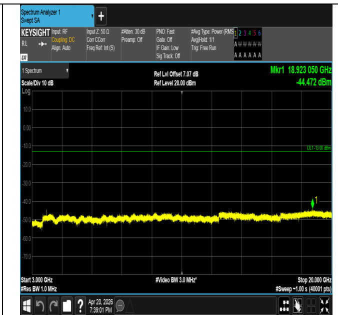
Band25-5MHz-QPSK-26665-1RB#24-3000~20000-PASS
