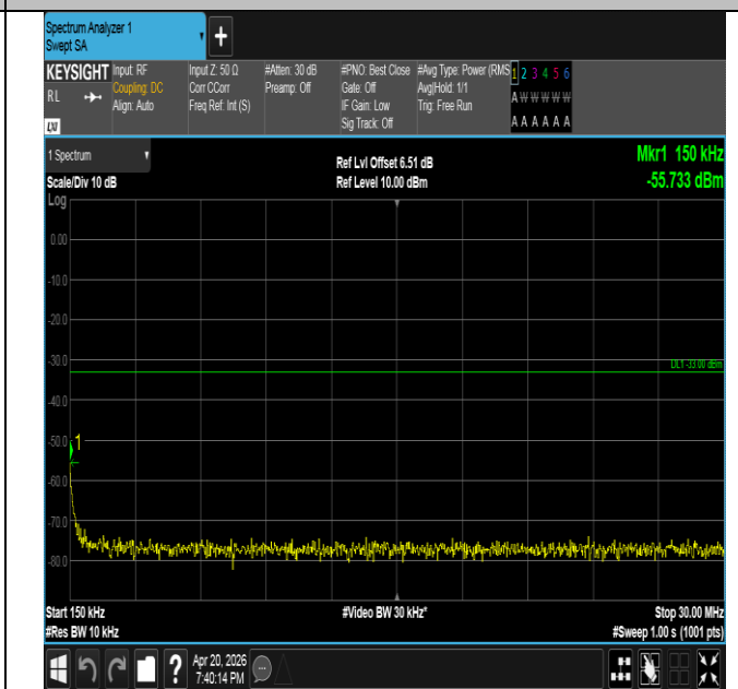
Band25-5MHz-QPSK-26665-25RB#0-0.15~30-PASS
