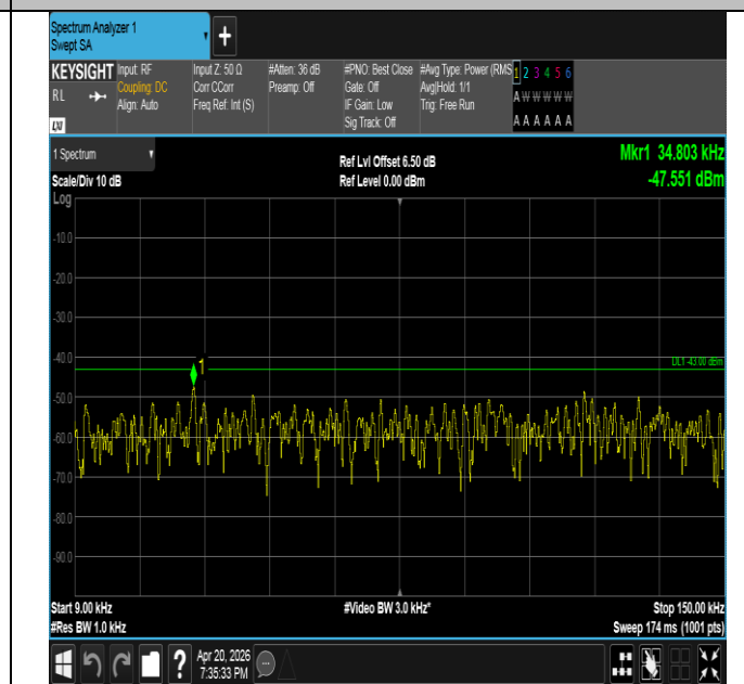
Band25-5MHz-16QAM-26365-25RB#0-0.009~0.15-PASS
