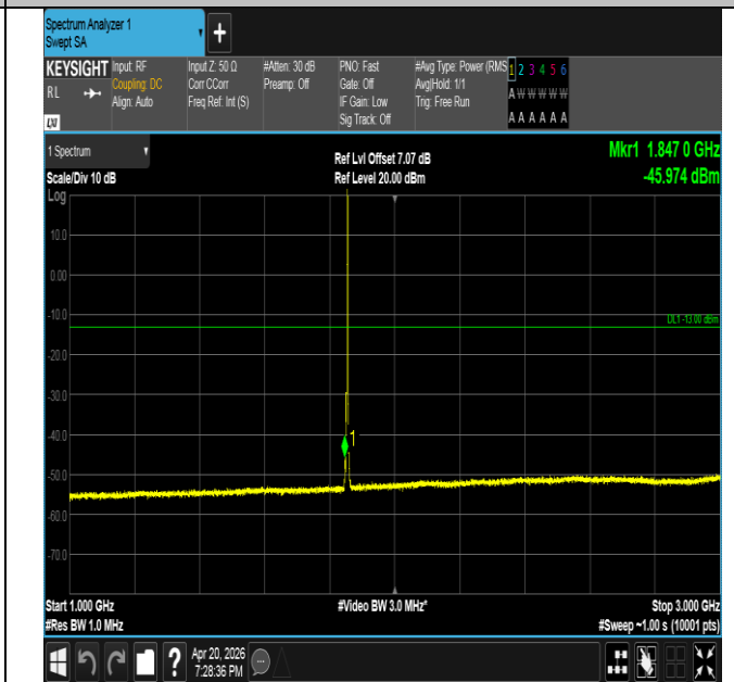
Band25-5MHz-16QAM-26065-1RB#24-1000~3000-PASS
