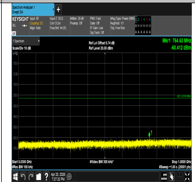
Band25-5MHz-QPSK-26065-1RB#24-30~1000-PASS
