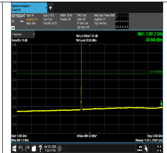
Band25-5MHz-16QAM-26365-1RB#24-1000~3000-PASS
