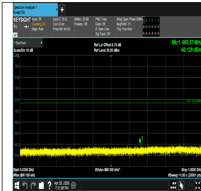
Band25-5MHz-QPSK-26365-1RB#0-30~1000-PASS
