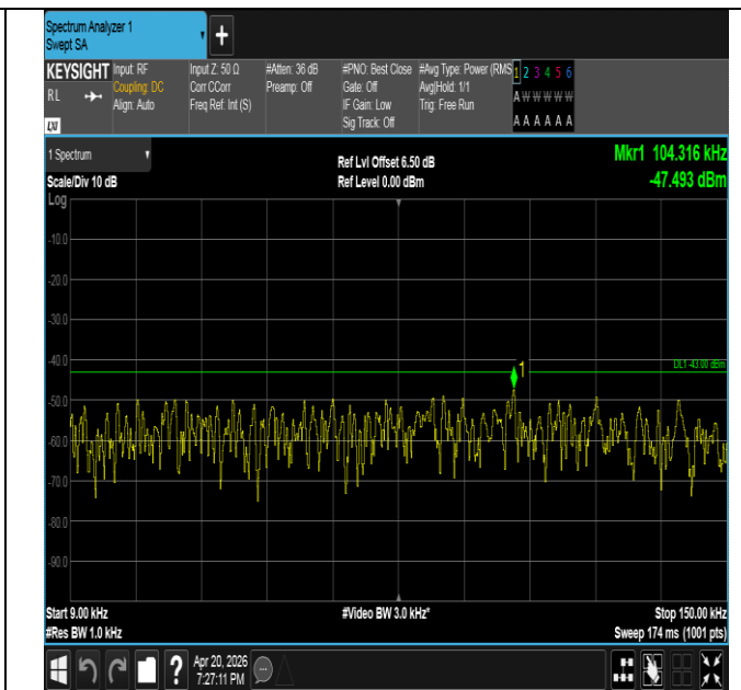
Band25-5MHz-QPSK-26065-1RB#24-0.009~0.15-PASS
