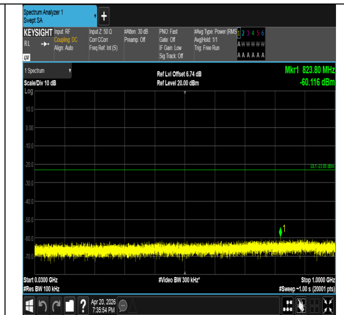
Band25-5MHz-16QAM-26365-25RB#0-30~1000-PASS
