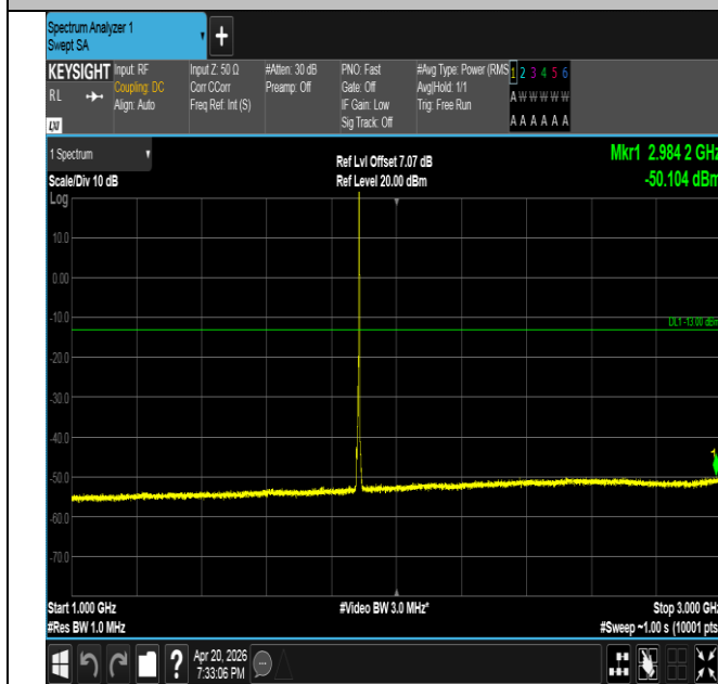
Band25-5MHz-QPSK-26365-1RB#24-1000~3000-PASS
