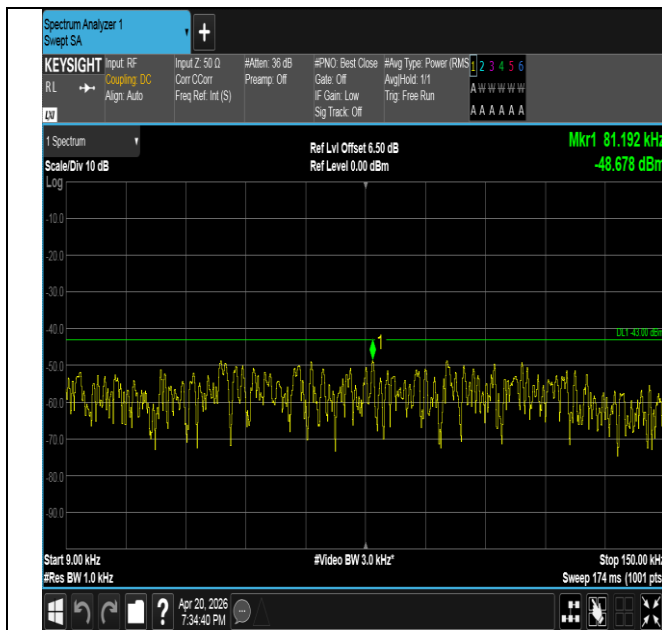
Band25-5MHz-QPSK-26365-25RB#0-0.009~0.15-PASS
