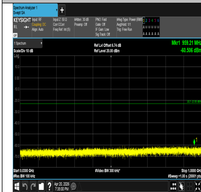
Band25-5MHz-QPSK-26365-25RB#0-30~1000-PASS
