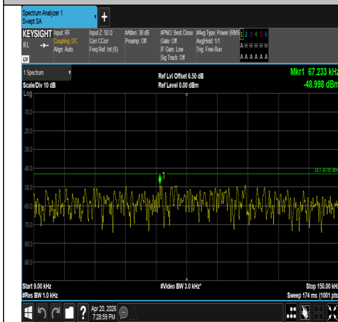
Band25-5MHz-QPSK-26065-25RB#0-0.009~0.15-PASS
