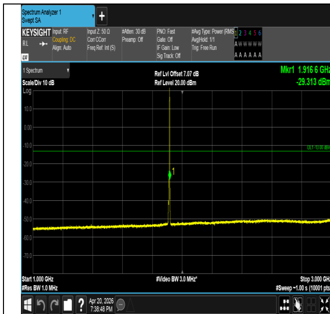
Band25-5MHz-QPSK-26665-1RB#24-1000~3000-PASS
