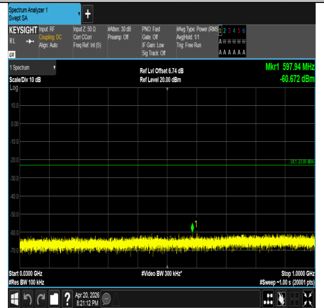
Band25-10MHz-16QAM-26365-50RB#0-30~1000-PASS
