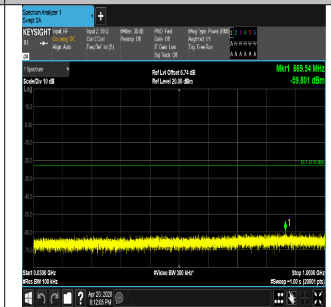
Band25-10MHz-16QAM-26090-1RB#0-30~1000-PASS
