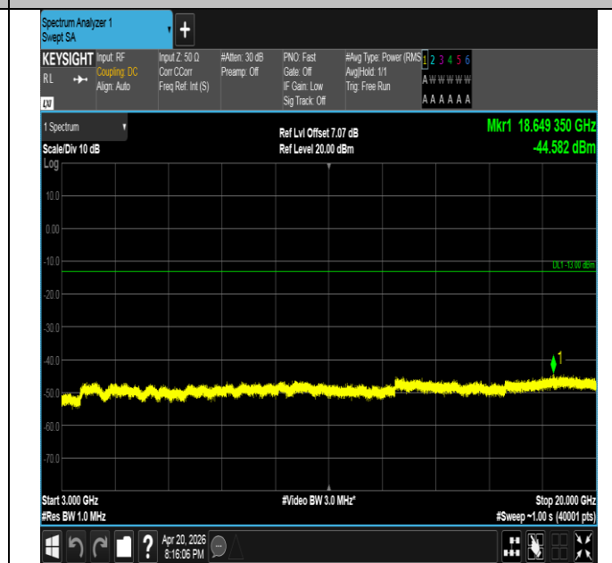
Band25-10MHz-16QAM-26090-50RB#0-3000~20000-PASS
