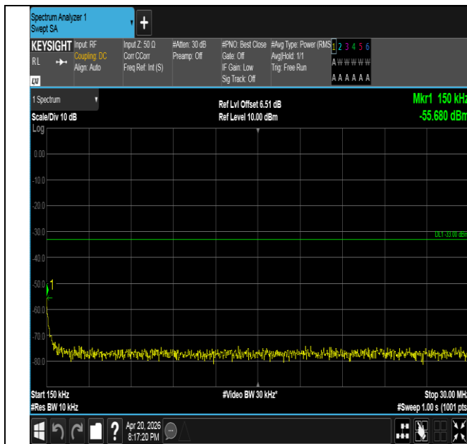
Band25-10MHz-16QAM-26365-1RB#0-0.15~30-PASS
