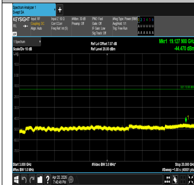
Band25-5MHz-QPSK-26665-25RB#0-3000~20000-PASS
