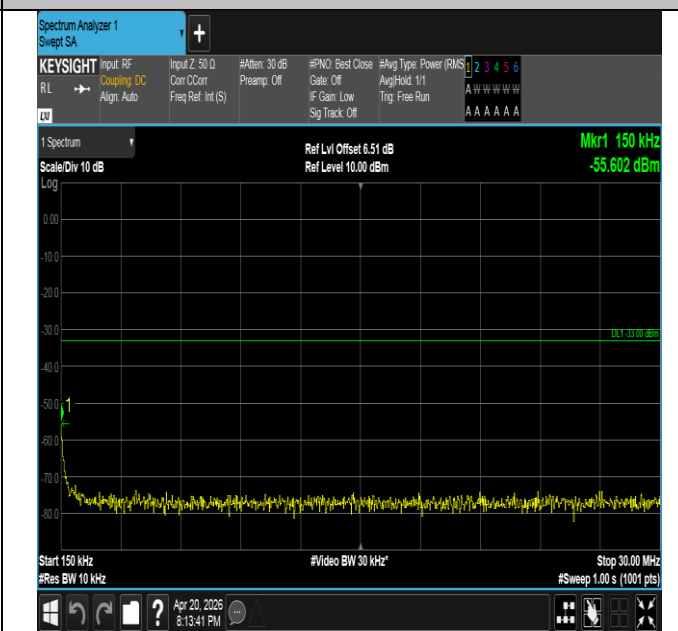
Band25-10MHz-16QAM-26090-1RB#49-0.15~30-PASS
