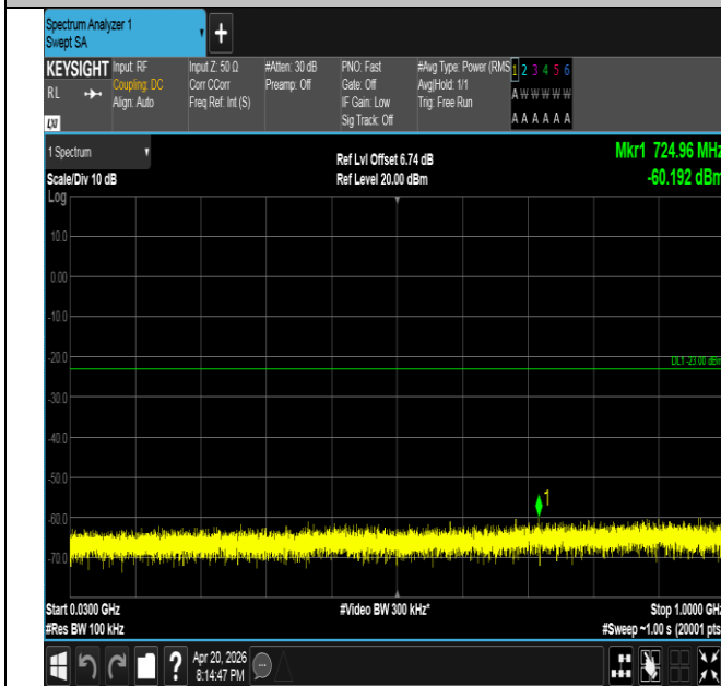
Band25-10MHz-QPSK-26090-50RB#0-30~1000-PASS
