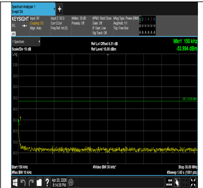
Band25-10MHz-QPSK-26090-50RB#0-0.15~30-PASS
