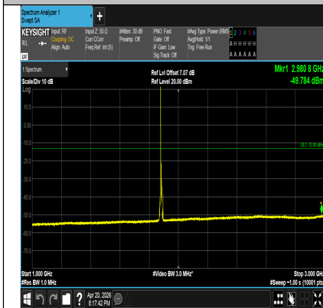
Band25-10MHz-16QAM-26365-1RB#0-1000~3000-PASS
