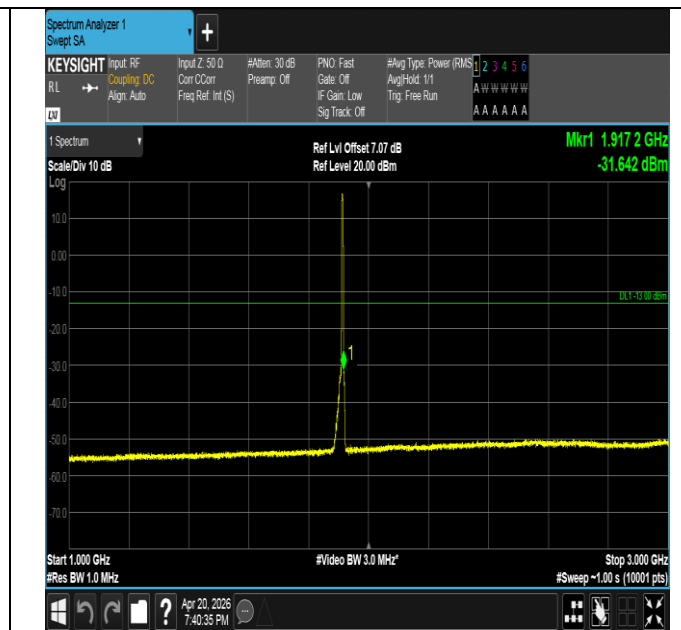
Band25-5MHz-QPSK-26665-25RB#0-1000~3000-PASS
