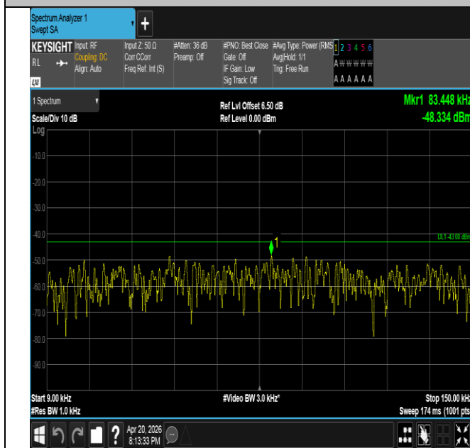
Band25-10MHz-16QAM-26090-1RB#49-0.009~0.15-PASS
