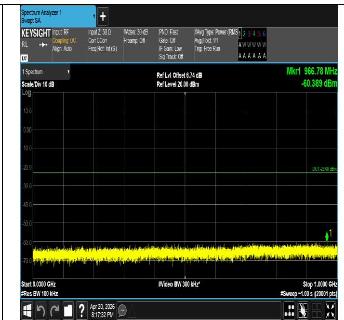
Band25-10MHz-16QAM-26365-1RB#0-30~1000-PASS
