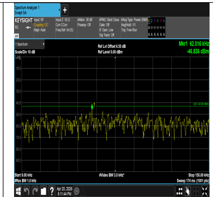
Band25-10MHz-16QAM-26090-1RB#0-0.009~0.15-PASS
