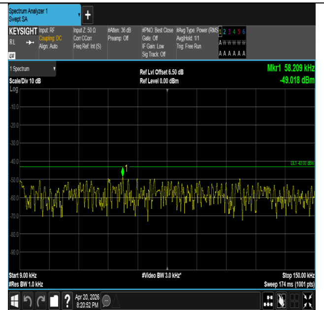
Band25-10MHz-16QAM-26365-50RB#0-0.009~0.15-PASS
