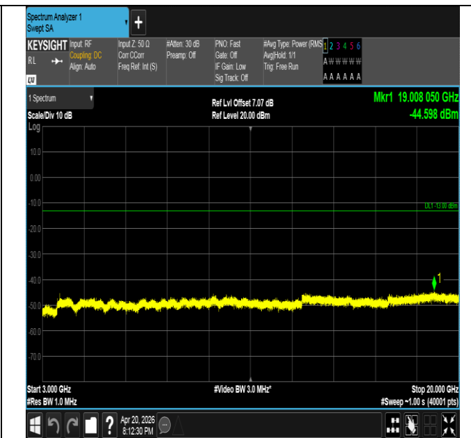
Band25-10MHz-16QAM-26090-1RB#0-3000~20000-PASS
