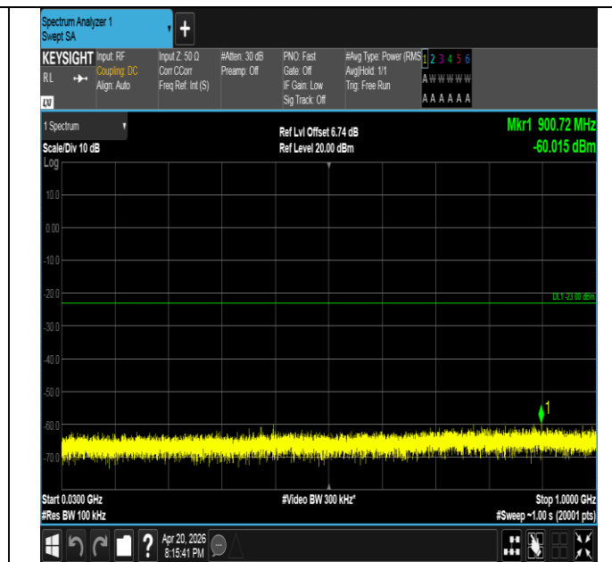
Band25-10MHz-16QAM-26090-50RB#0-30~1000-PASS
