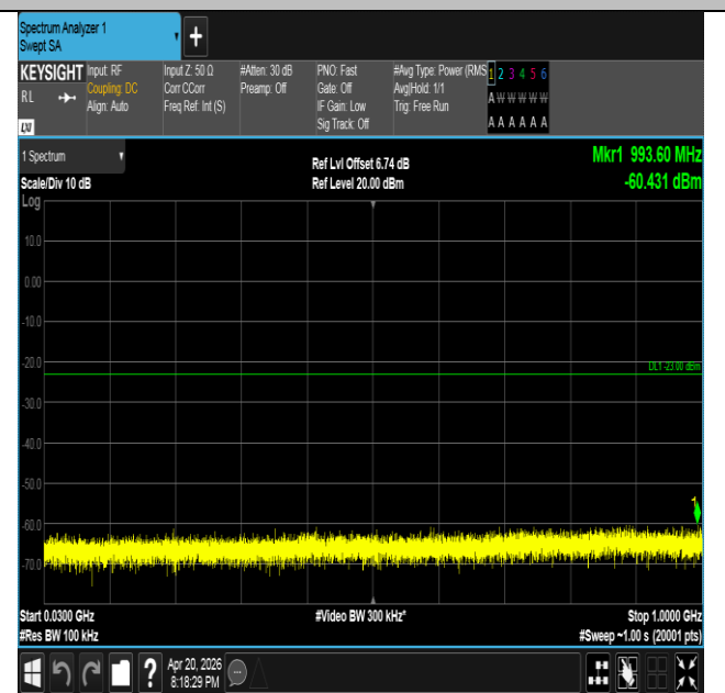
Band25-10MHz-QPSK-26365-1RB#49-30~1000-PASS
