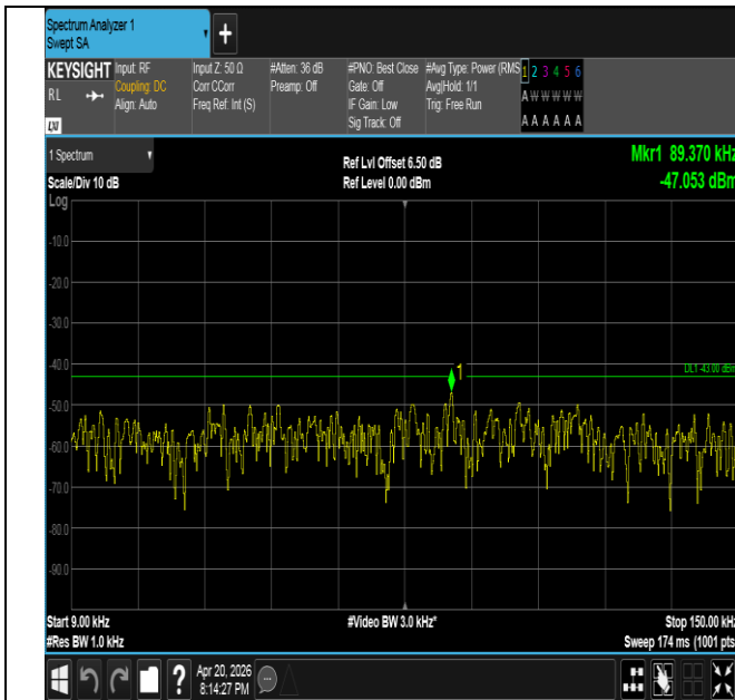
Band25-10MHz-QPSK-26090-50RB#0-0.009~0.15-PASS
