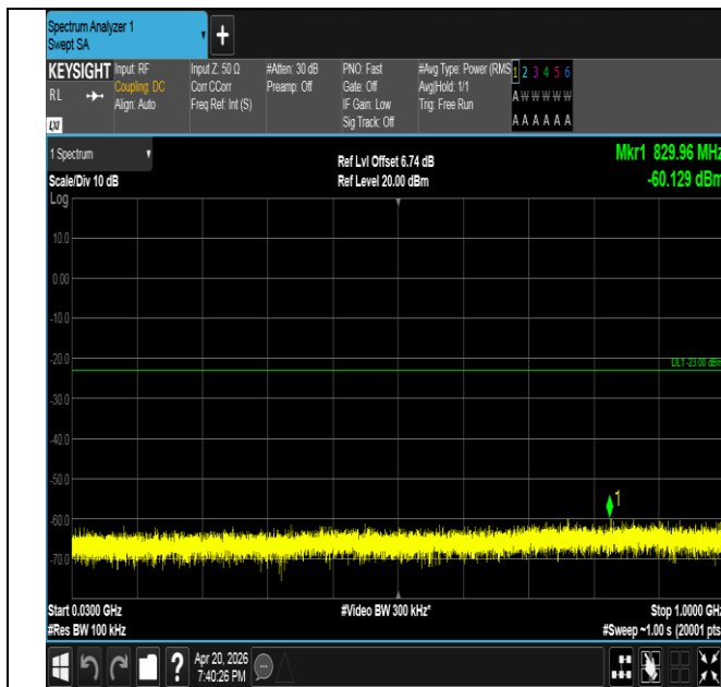
Band25-5MHz-QPSK-26665-25RB#0-30~1000-PASS
