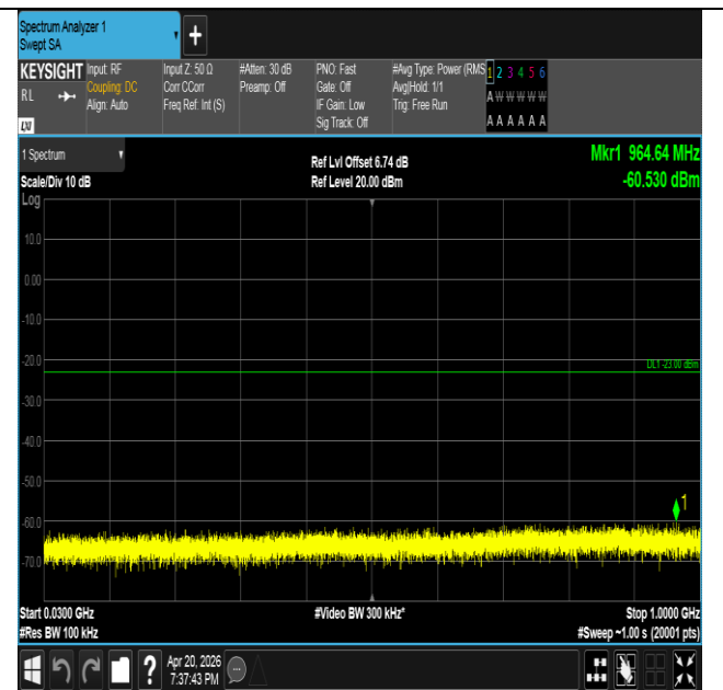
Band25-5MHz-16QAM-26665-1RB#0-30~1000-PASS
