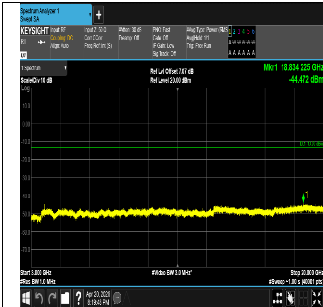
Band25-10MHz-16QAM-26365-1RB#49-3000~20000-PASS
