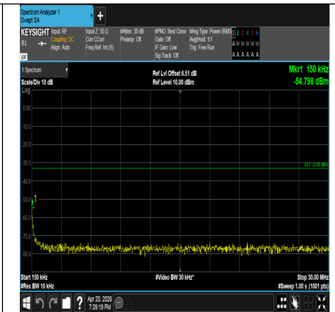
Band25-5MHz-16QAM-26665-1RB#24-0.15~30-PASS
