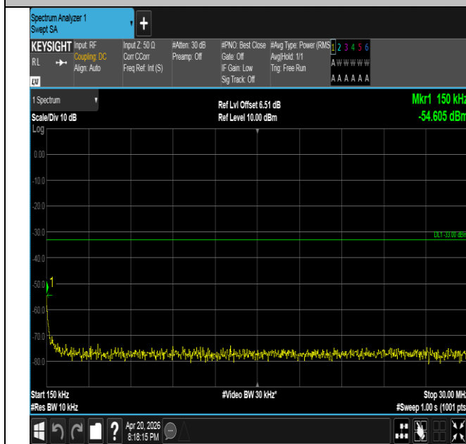
Band25-10MHz-QPSK-26365-1RB#49-0.15~30-PASS
