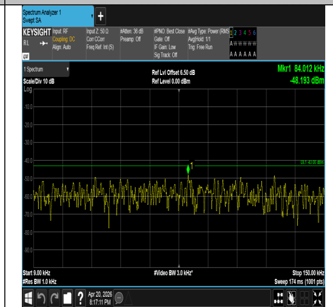
Band25-10MHz-16QAM-26365-1RB#0-0.009~0.15-PASS
