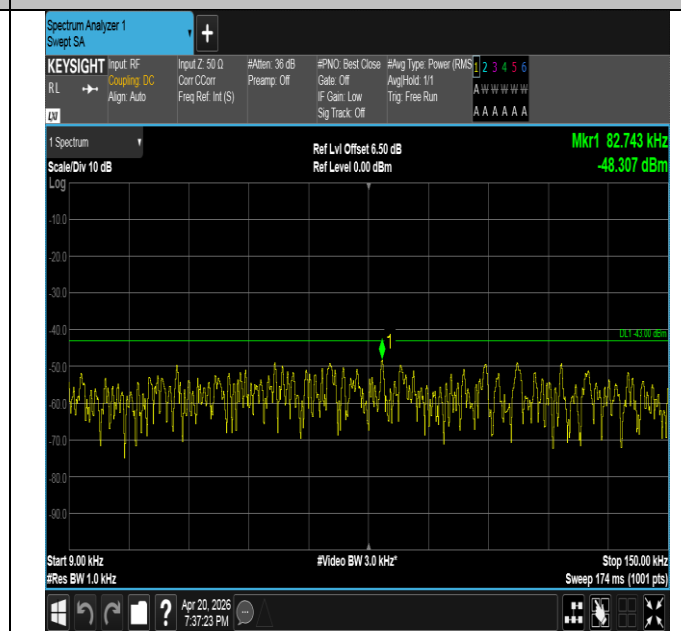
Band25-5MHz-16QAM-26665-1RB#0-0.009~0.15-PASS
