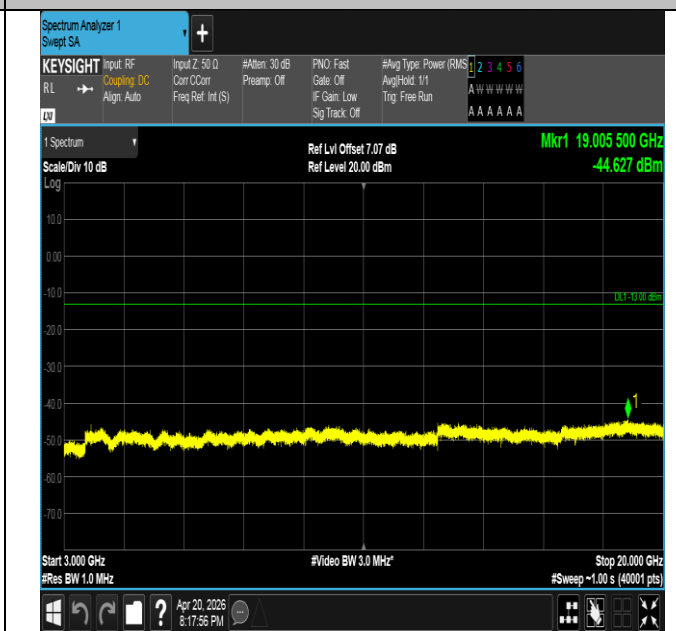
Band25-10MHz-16QAM-26365-1RB#0-3000~20000-PASS
