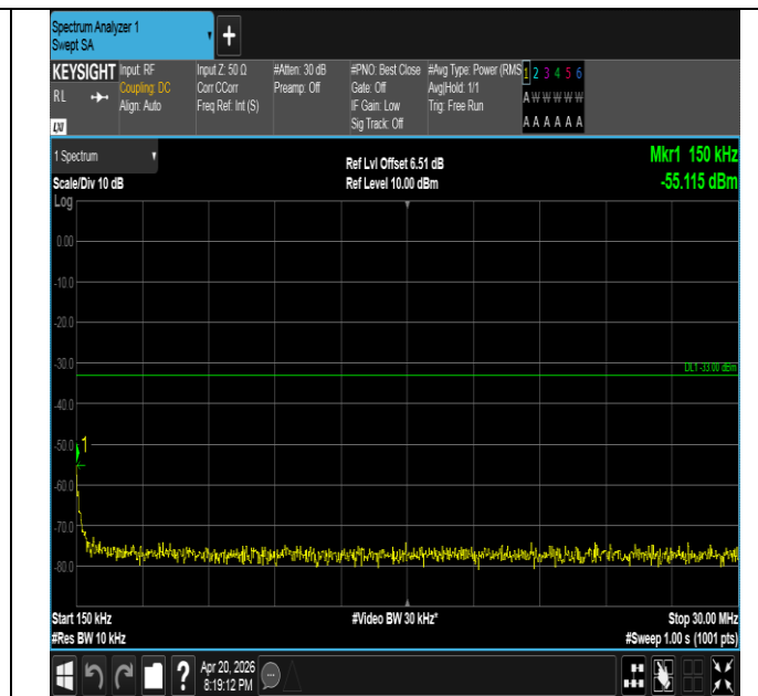
Band25-10MHz-16QAM-26365-1RB#49-0.15~30-PASS
