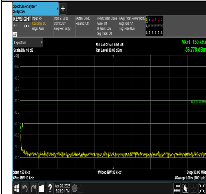
Band25-10MHz-16QAM-26365-50RB#0-0.15~30-PASS
