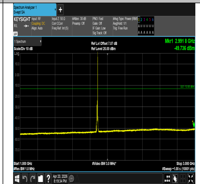
Band25-10MHz-16QAM-26365-1RB#49-1000~3000-PASS
