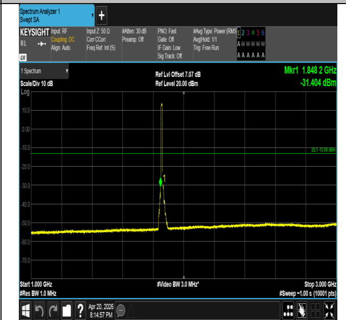
Band25-10MHz-QPSK-26090-50RB#0-1000~3000-PASS
