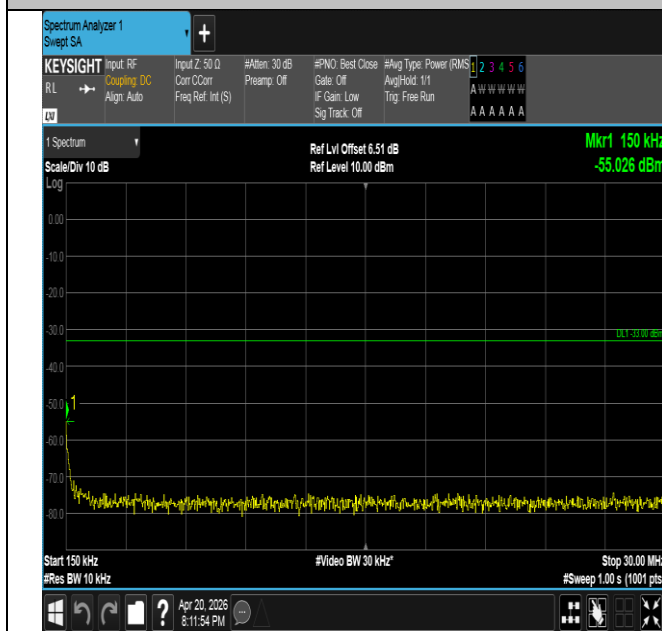
Band25-10MHz-16QAM-26090-1RB#0-0.15~30-PASS
