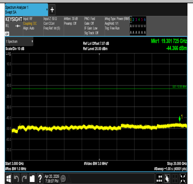
Band25-5MHz-16QAM-26665-1RB#0-3000~20000-PASS
