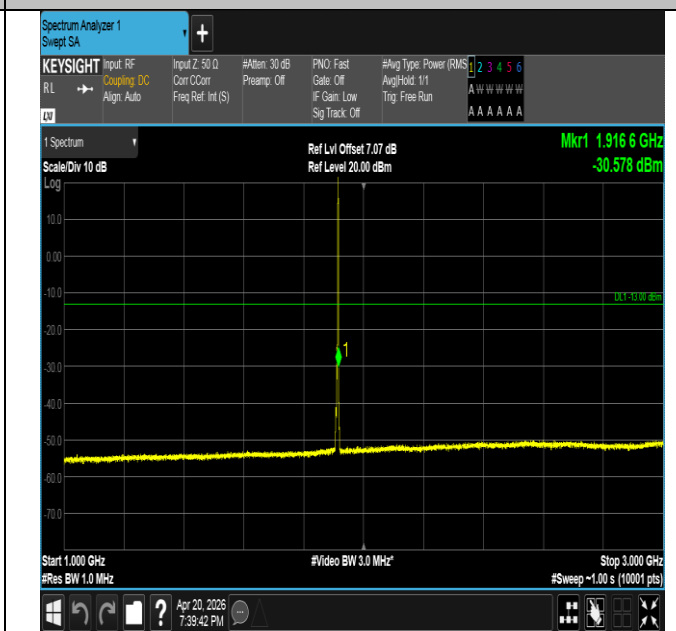
Band25-5MHz-16QAM-26665-1RB#24-1000~3000-PASS
