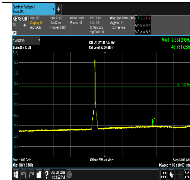
Band25-10MHz-16QAM-26365-50RB#0-1000~3000-PASS
