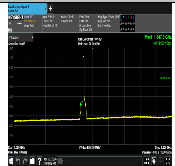
Band25-15MHz-QPSK-26365-75RB#0-1000~3000-PASS
