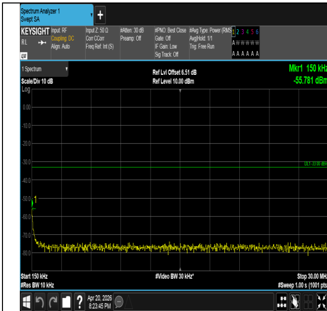
Band25-10MHz-QPSK-26640-1RB#49-0.15~30-PASS
