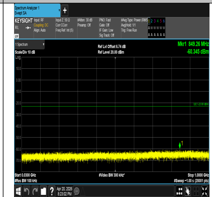
Band25-10MHz-16QAM-26640-1RB#0-30~1000-PASS
