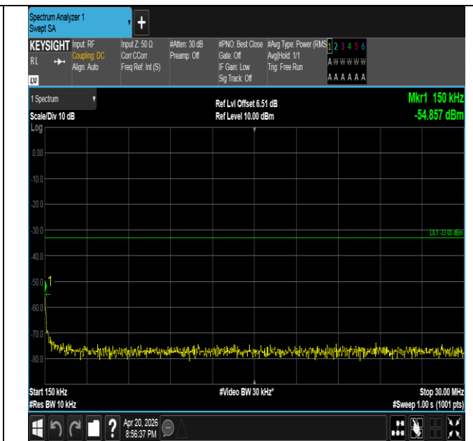
Band25-15MHz-QPSK-26115-1RB#0-0.15~30-PASS
