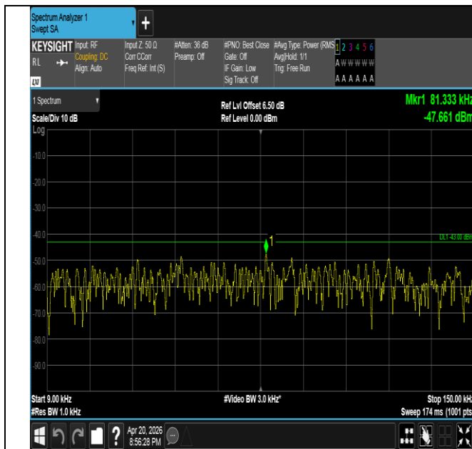
Band25-15MHz-QPSK-26115-1RB#0-0.009~0.15-PASS
