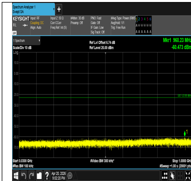
Band25-15MHz-QPSK-26365-1RB#0-30~1000-PASS
