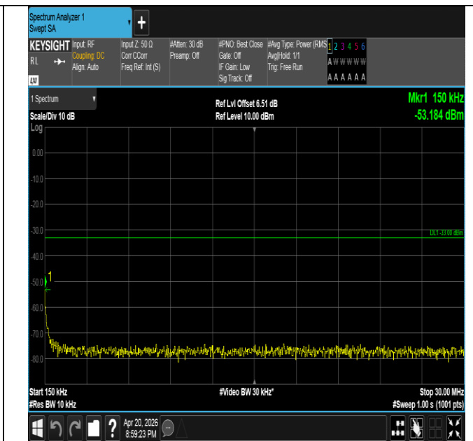
Band25-15MHz-16QAM-26115-1RB#74-0.15~30-PASS
