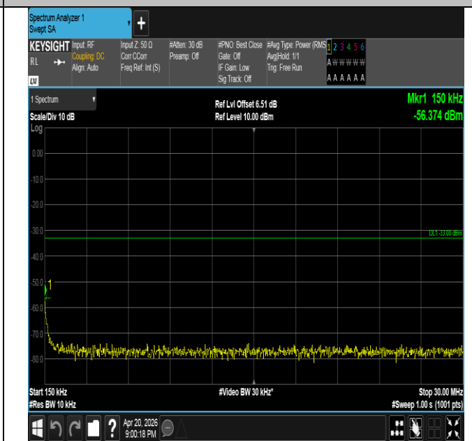
Band25-15MHz-QPSK-26115-75RB#0-0.15~30-PASS
