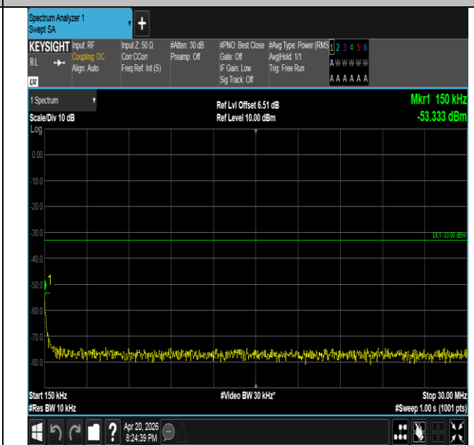
Band25-10MHz-16QAM-26640-1RB#49-0.15~30-PASS
