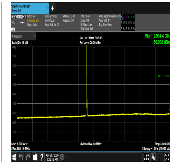
Band25-10MHz-16QAM-26640-1RB#0-1000~3000-PASS
