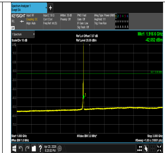
Band25-10MHz-16QAM-26640-1RB#49-1000~3000-PASS
