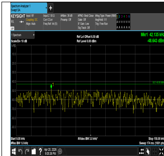
Band25-15MHz-QPSK-26365-75RB#0-0.009~0.15-PASS
