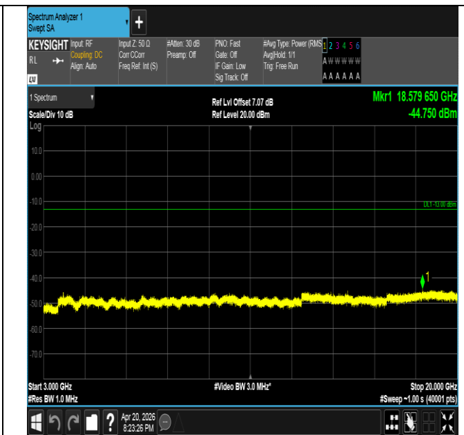
Band25-10MHz-16QAM-26640-1RB#0-3000~20000-PASS
