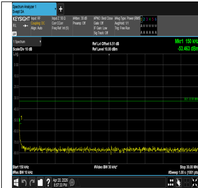
Band25-15MHz-16QAM-26115-1RB#0-0.15~30-PASS
