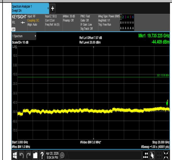
Band25-15MHz-QPSK-26365-1RB#74-3000~20000-PASS
