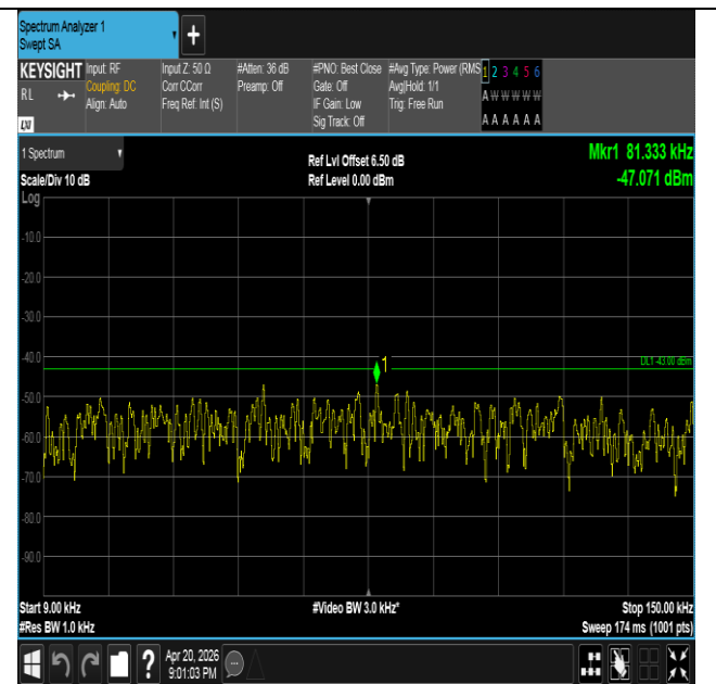
Band25-15MHz-16QAM-26115-75RB#0-0.009~0.15-PASS
