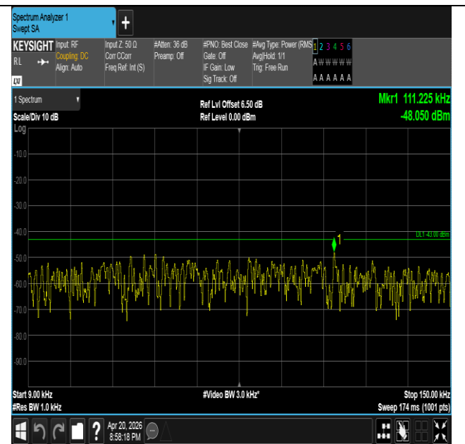
Band25-15MHz-QPSK-26115-1RB#74-0.009~0.15-PASS
