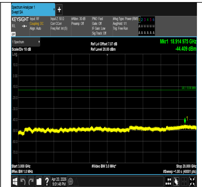
Band25-15MHz-16QAM-26115-75RB#0-3000~20000-PASS
