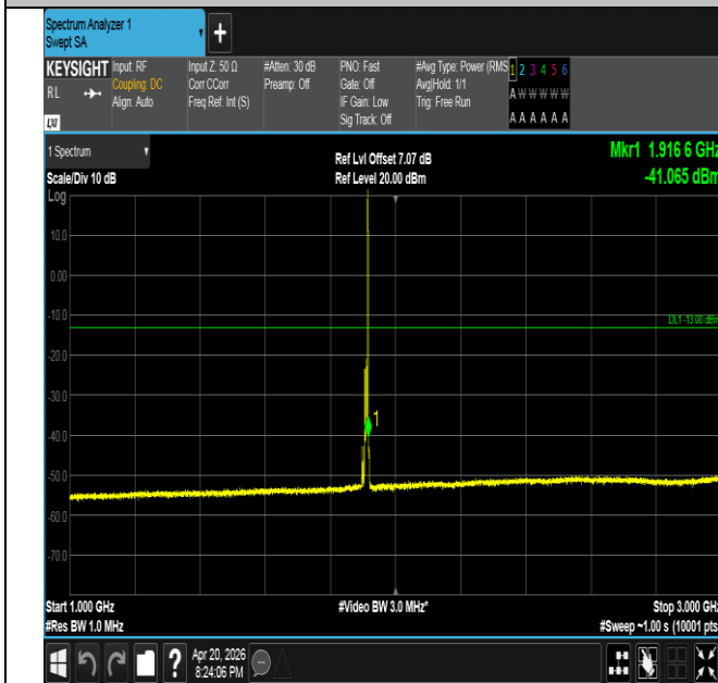
Band25-10MHz-QPSK-26640-1RB#49-1000~3000-PASS
