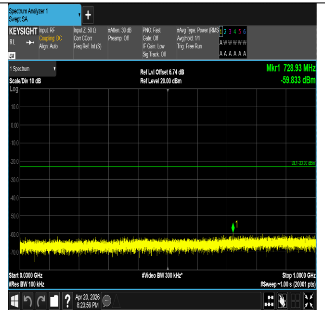
Band25-10MHz-QPSK-26640-1RB#49-30~1000-PASS
