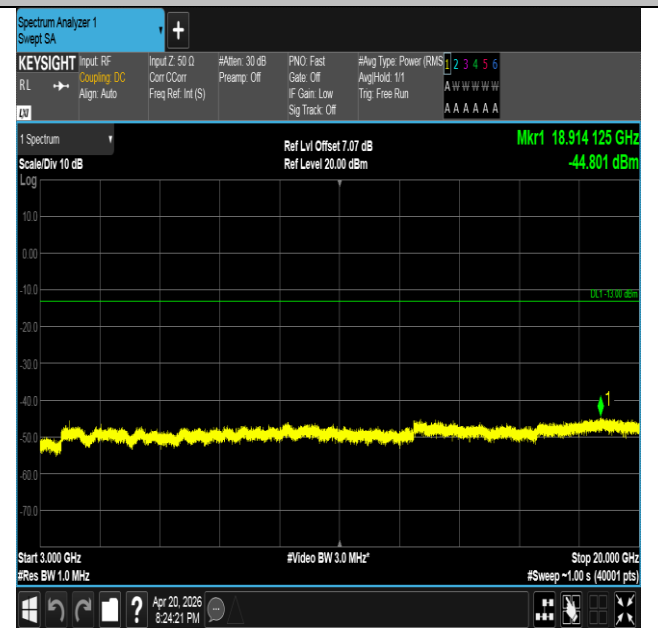
Band25-10MHz-QPSK-26640-1RB#49-3000~20000-PASS
