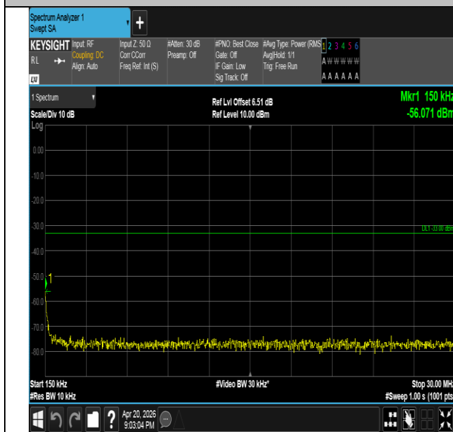
Band25-15MHz-16QAM-26365-1RB#0-0.15~30-PASS
