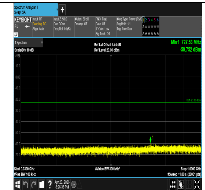
Band25-10MHz-16QAM-26640-50RB#0-30~1000-PASS
