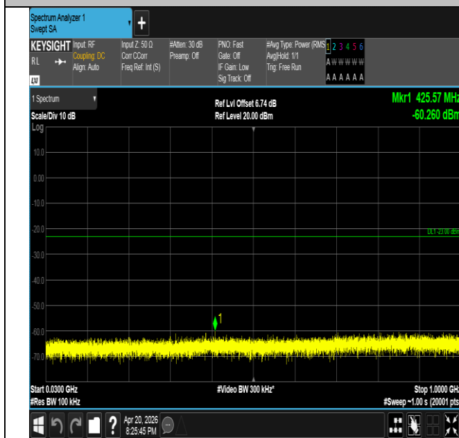
Band25-10MHz-QPSK-26640-50RB#0-30~1000-PASS
