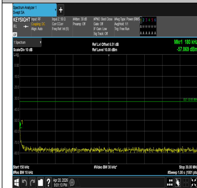
Band25-15MHz-16QAM-26115-75RB#0-0.15~30-PASS
