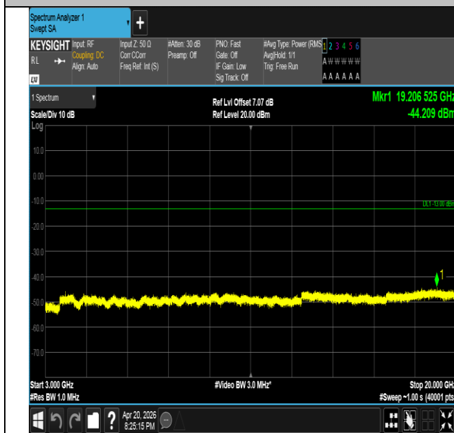
Band25-10MHz-16QAM-26640-1RB#49-3000~20000-PASS
