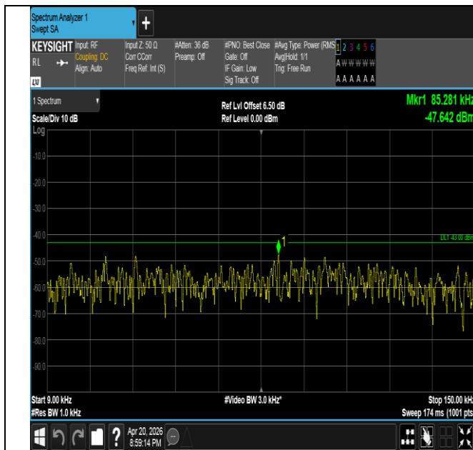
Band25-15MHz-16QAM-26115-1RB#74-0.009~0.15-PASS
