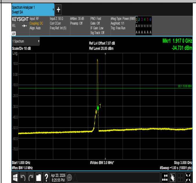
Band25-10MHz-QPSK-26640-50RB#0-1000~3000-PASS
