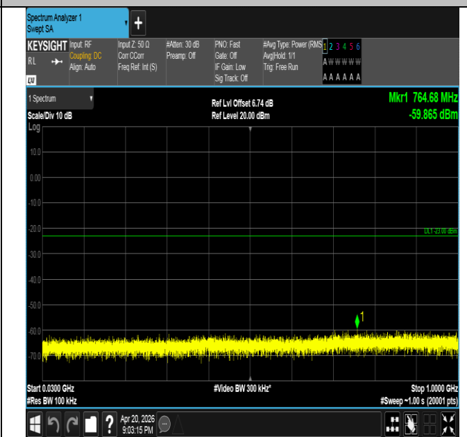
Band25-15MHz-16QAM-26365-1RB#0-30~1000-PASS
