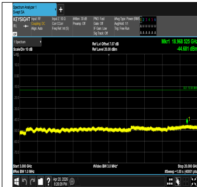
Band25-10MHz-QPSK-26640-50RB#0-3000~20000-PASS
