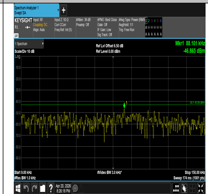
Band25-10MHz-16QAM-26640-50RB#0-0.009~0.15-PASS
