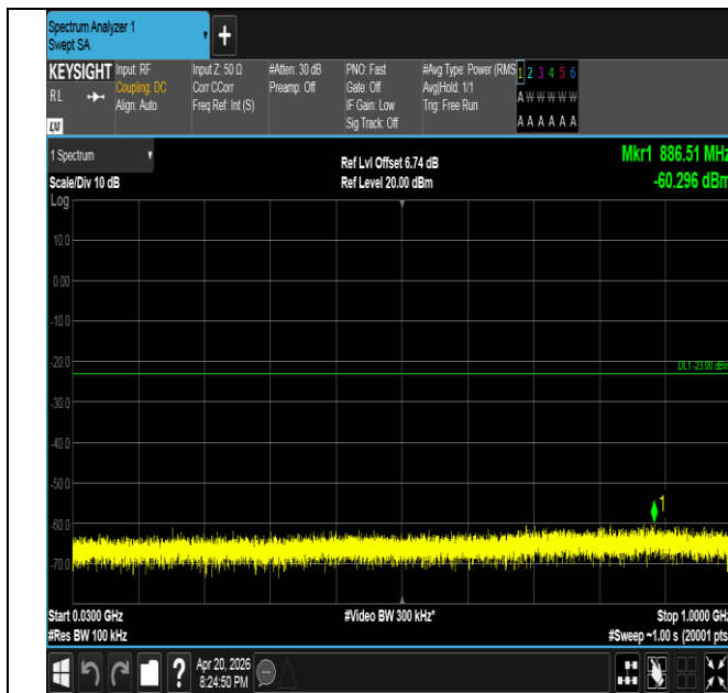
Band25-10MHz-16QAM-26640-1RB#49-30~1000-PASS
