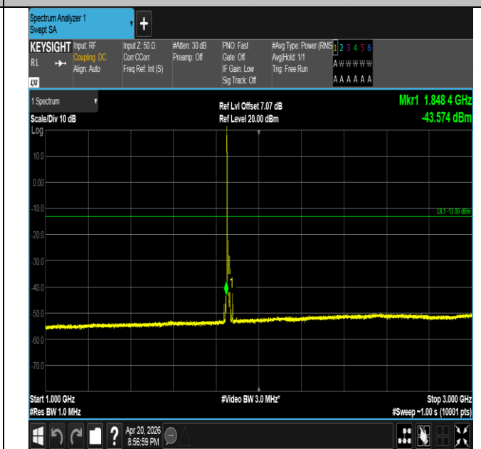
Band25-15MHz-QPSK-26115-1RB#0-1000~3000-PASS
