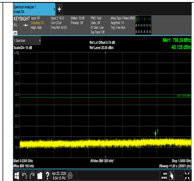
Band25-15MHz-QPSK-26365-1RB#74-30~1000-PASS
