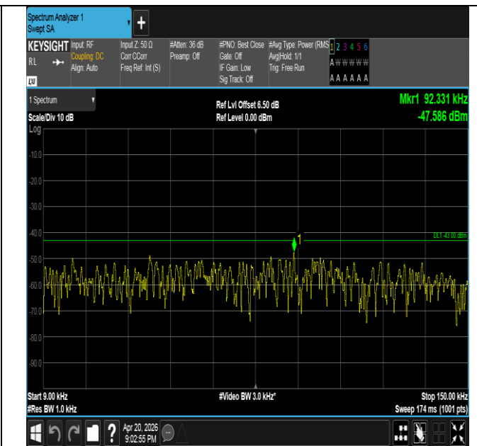
Band25-15MHz-16QAM-26365-1RB#0-0.009~0.15-PASS
