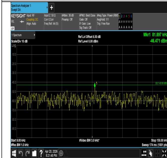
Band25-10MHz-QPSK-26640-1RB#0-0.009~0.15-PASS
