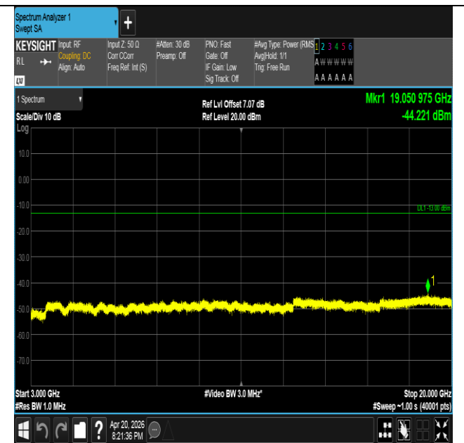
Band25-10MHz-16QAM-26365-50RB#0-3000~20000-PASS
