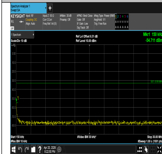
Band25-10MHz-16QAM-26640-1RB#0-0.15~30-PASS
