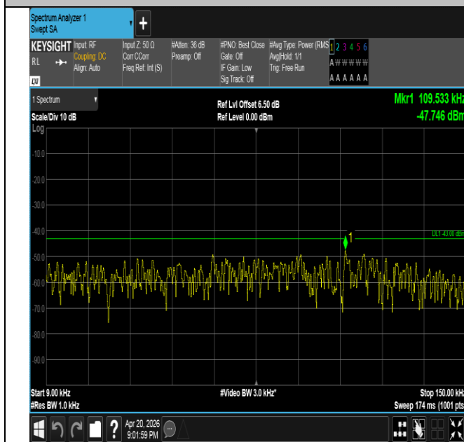
Band25-15MHz-QPSK-26365-1RB#0-0.009~0.15-PASS
