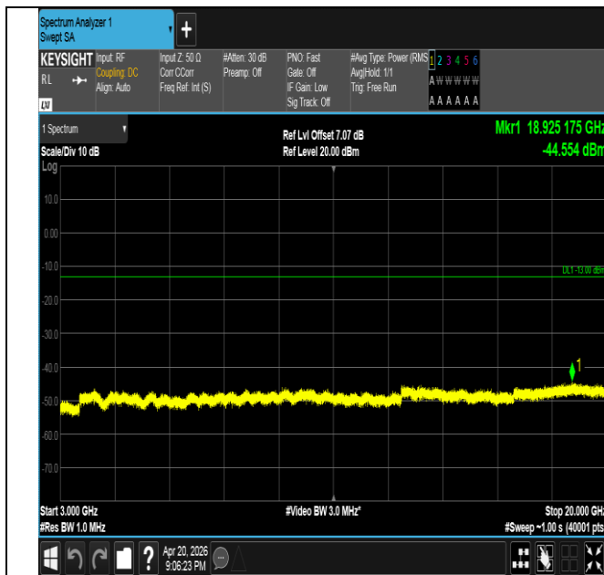
Band25-15MHz-QPSK-26365-75RB#0-3000~20000-PASS
