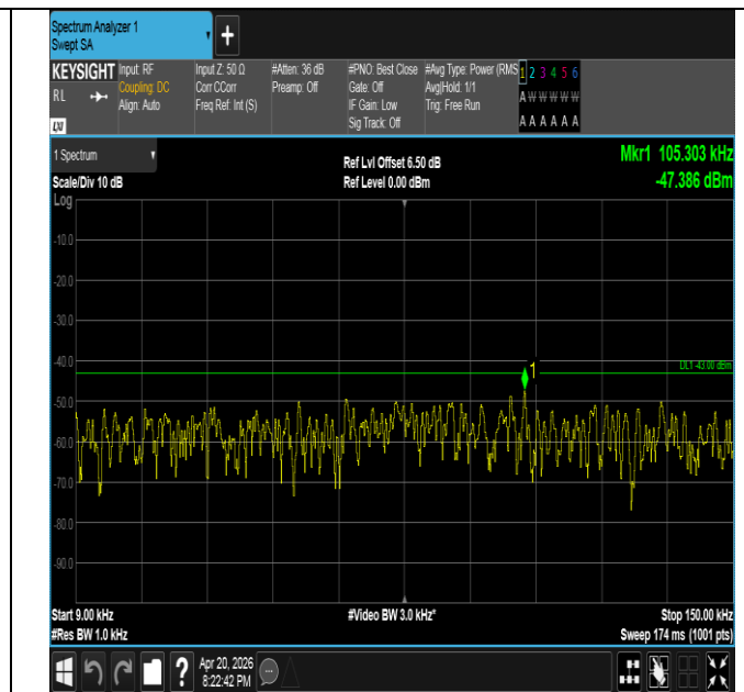
Band25-10MHz-16QAM-26640-1RB#0-0.009~0.15-PASS
