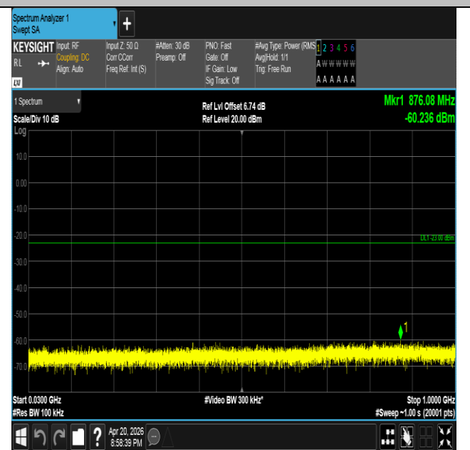
Band25-15MHz-QPSK-26115-1RB#74-30~1000-PASS
