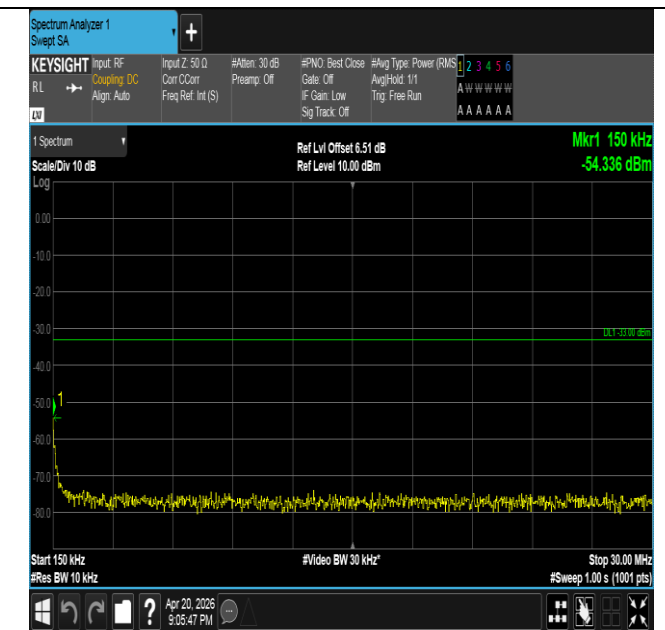
Band25-15MHz-QPSK-26365-75RB#0-0.15~30-PASS
