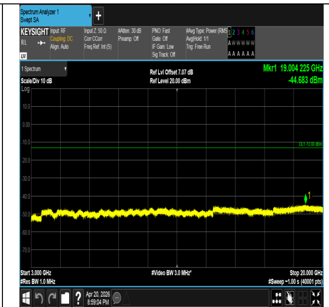
Band25-15MHz-QPSK-26115-1RB#74-3000~20000-PASS
