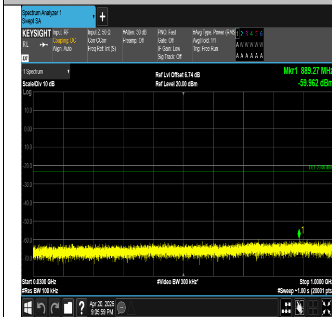
Band25-15MHz-QPSK-26365-75RB#0-30~1000-PASS
