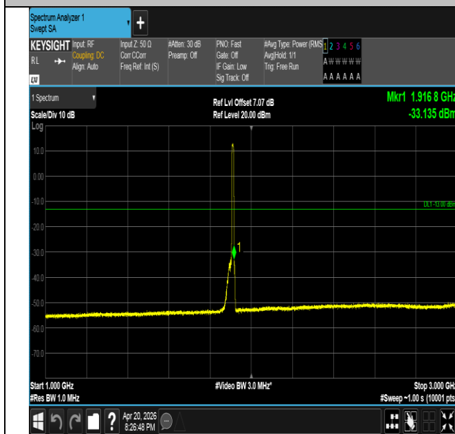
Band25-10MHz-16QAM-26640-50RB#0-1000~3000-PASS
