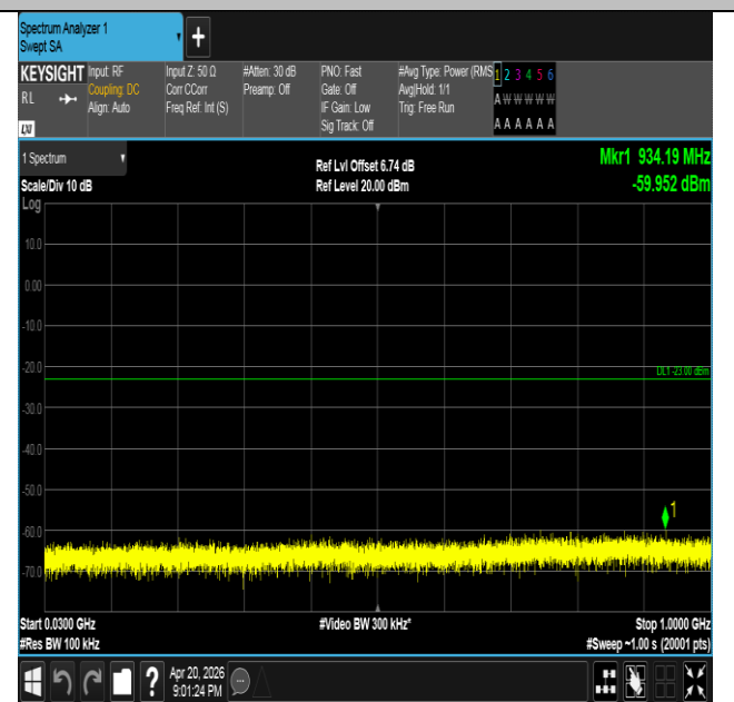
Band25-15MHz-16QAM-26115-75RB#0-30~1000-PASS
