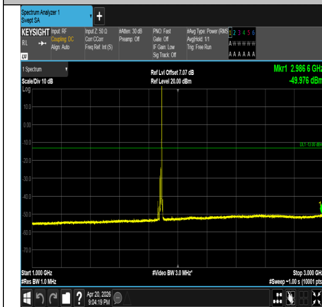
Band25-15MHz-QPSK-26365-1RB#74-1000~3000-PASS
