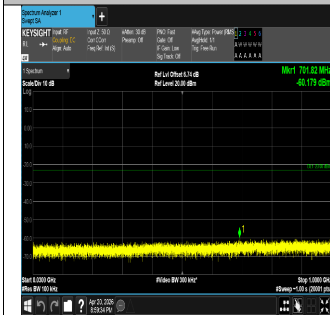
Band25-15MHz-16QAM-26115-1RB#74-30~1000-PASS
