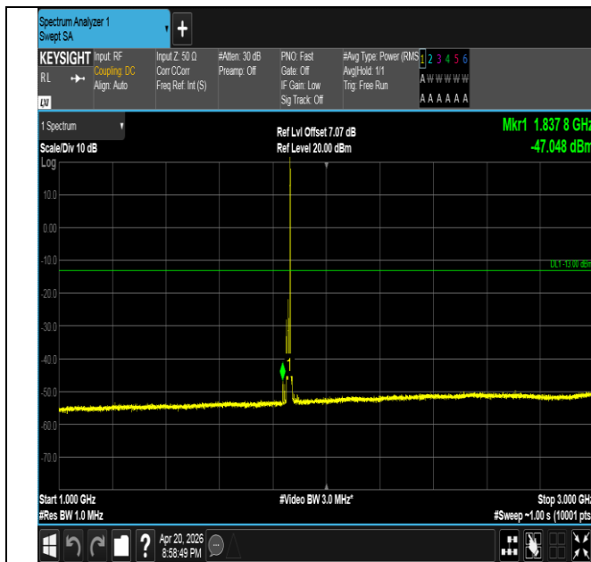
Band25-15MHz-QPSK-26115-1RB#74-1000~3000-PASS
