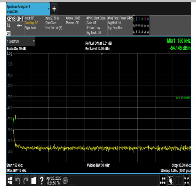
Band25-10MHz-QPSK-26640-1RB#0-0.15~30-PASS
