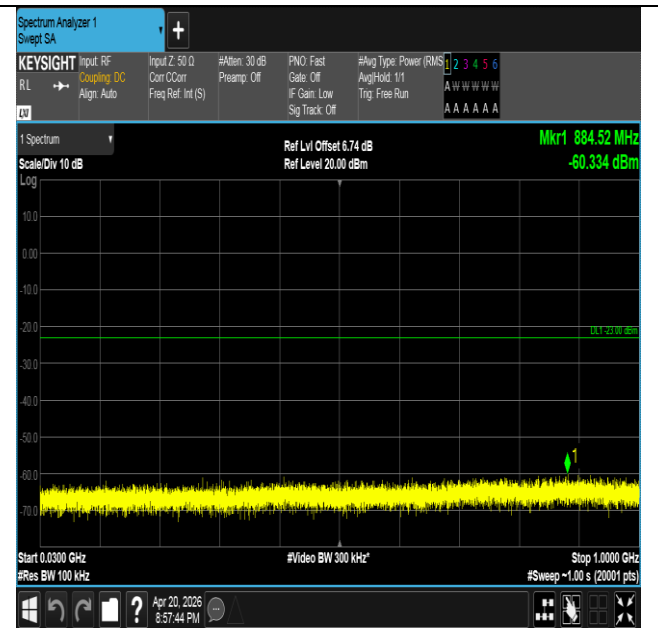
Band25-15MHz-16QAM-26115-1RB#0-30~1000-PASS
