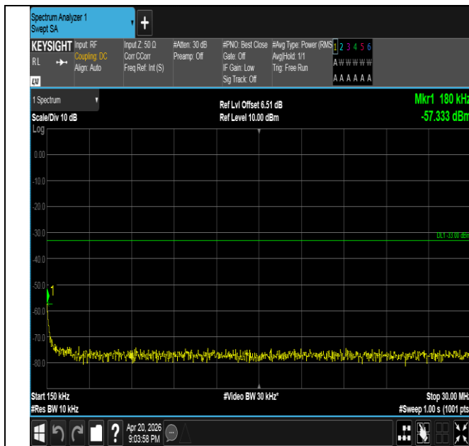
Band25-15MHz-QPSK-26365-1RB#74-0.15~30-PASS
