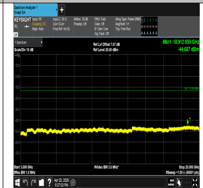
Band25-10MHz-16QAM-26640-50RB#0-3000~20000-PASS
