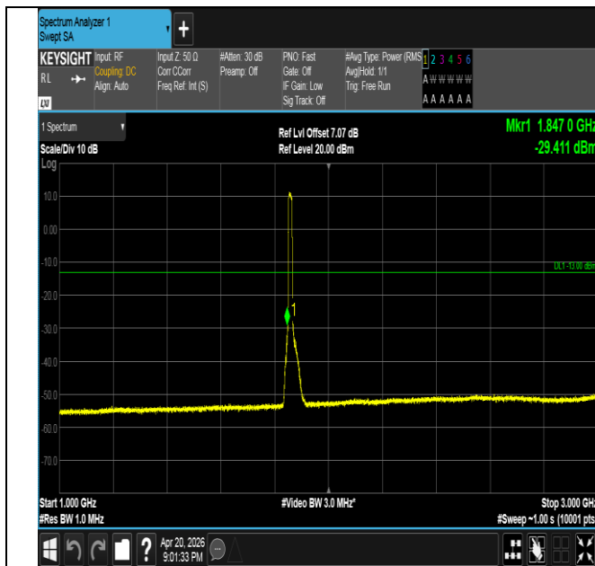
Band25-15MHz-16QAM-26115-75RB#0-1000~3000-PASS
