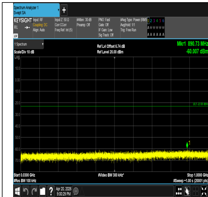
Band25-15MHz-QPSK-26115-75RB#0-30~1000-PASS
