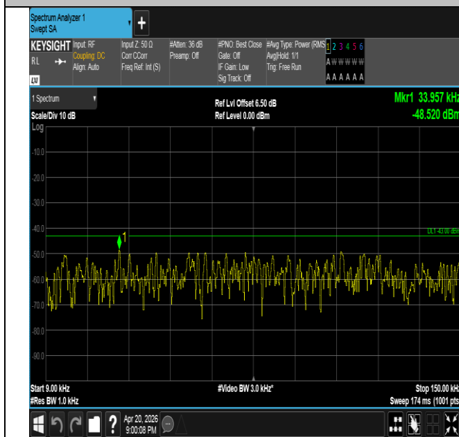
Band25-15MHz-QPSK-26115-75RB#0-0.009~0.15-PASS
