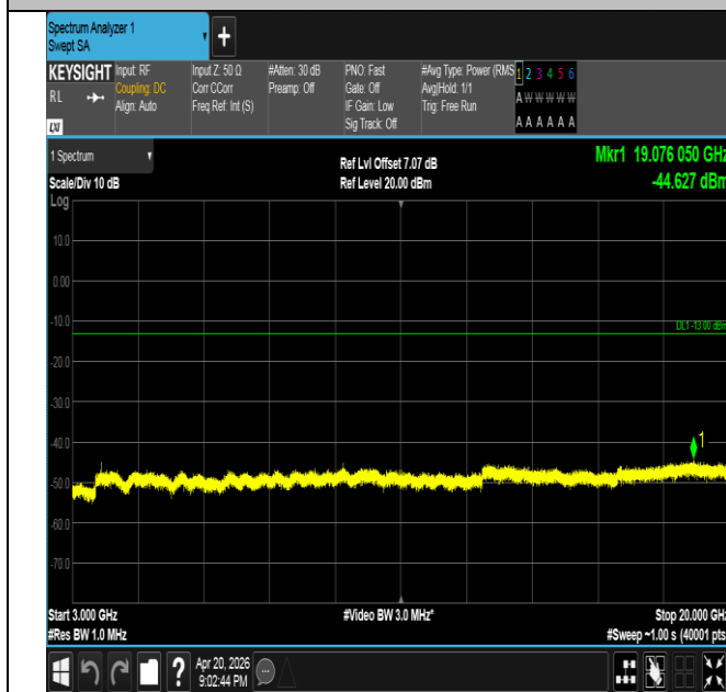
Band25-15MHz-QPSK-26365-1RB#0-3000~20000-PASS
