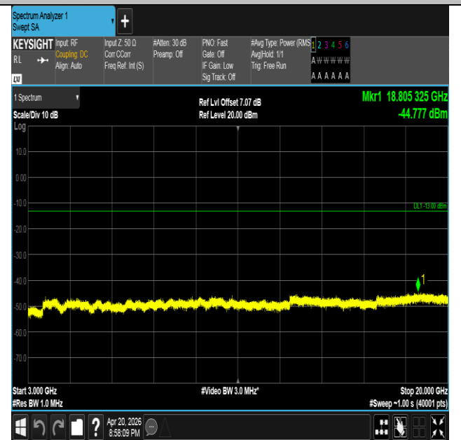
Band25-15MHz-16QAM-26115-1RB#0-3000~20000-PASS
