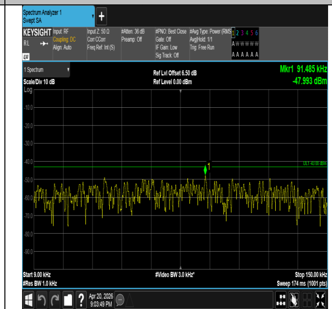
Band25-15MHz-QPSK-26365-1RB#74-0.009~0.15-PASS
