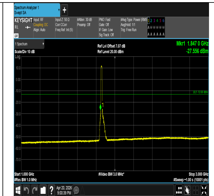
Band25-15MHz-QPSK-26115-75RB#0-1000~3000-PASS
