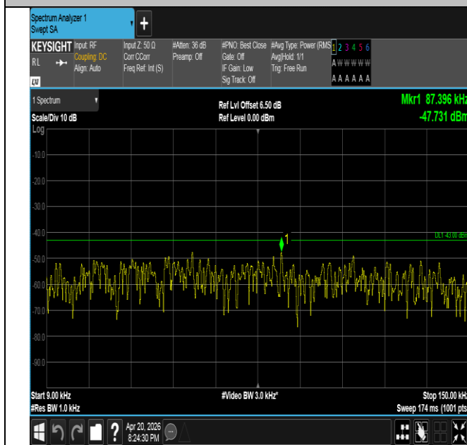
Band25-10MHz-16QAM-26640-1RB#49-0.009~0.15-PASS
