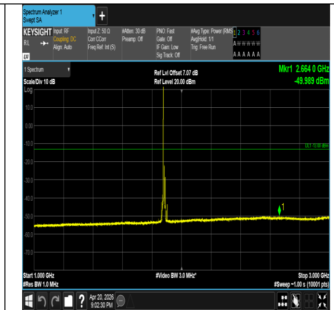
Band25-15MHz-QPSK-26365-1RB#0-1000~3000-PASS
