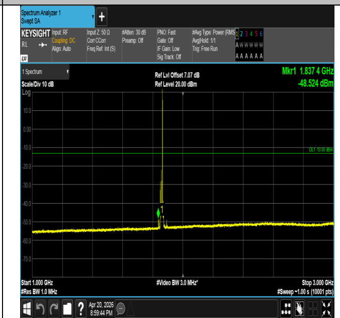
Band25-15MHz-16QAM-26115-1RB#74-1000~3000-PASS
