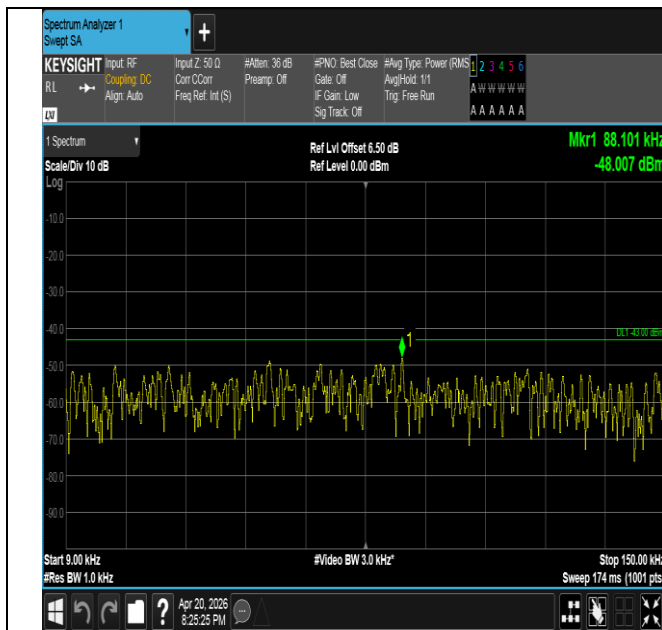
Band25-10MHz-QPSK-26640-50RB#0-0.009~0.15-PASS
