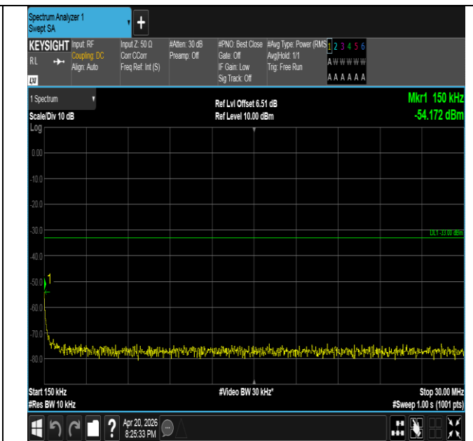
Band25-10MHz-QPSK-26640-50RB#0-0.15~30-PASS
