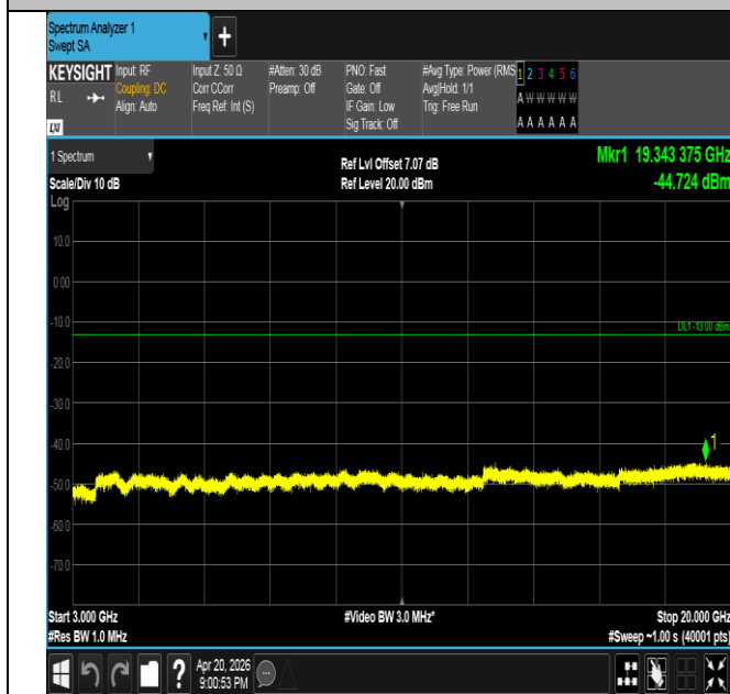
Band25-15MHz-QPSK-26115-75RB#0-3000~20000-PASS
