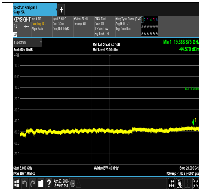
Band25-15MHz-16QAM-26115-1RB#74-3000~20000-PASS
