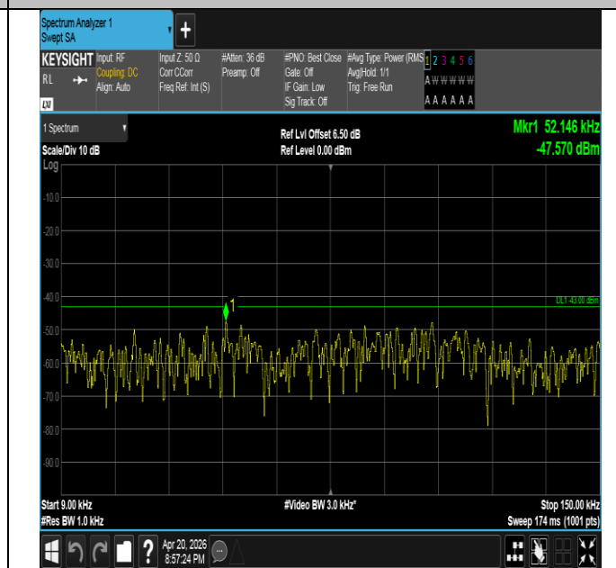
Band25-15MHz-16QAM-26115-1RB#0-0.009~0.15-PASS
