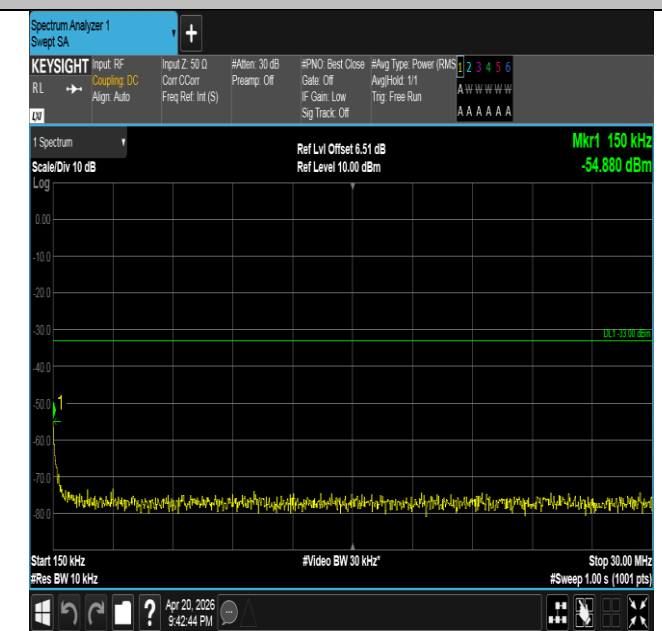
Band25-20MHz-QPSK-26140-1RB#0-0.15~30-PASS
