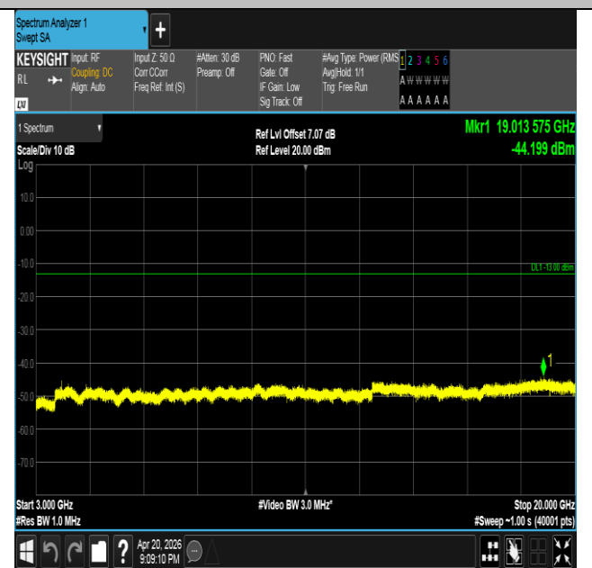
Band25-15MHz-16QAM-26615-1RB#0-3000~20000-PASS
