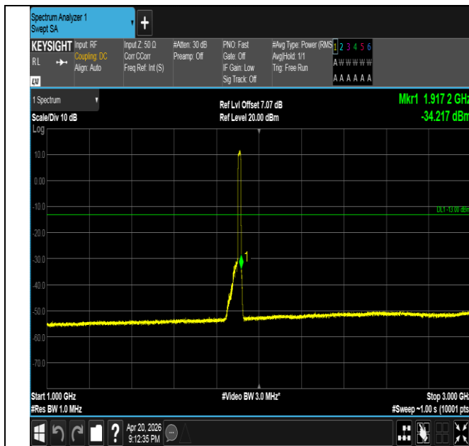
Band25-15MHz-16QAM-26615-75RB#0-1000~3000-PASS
