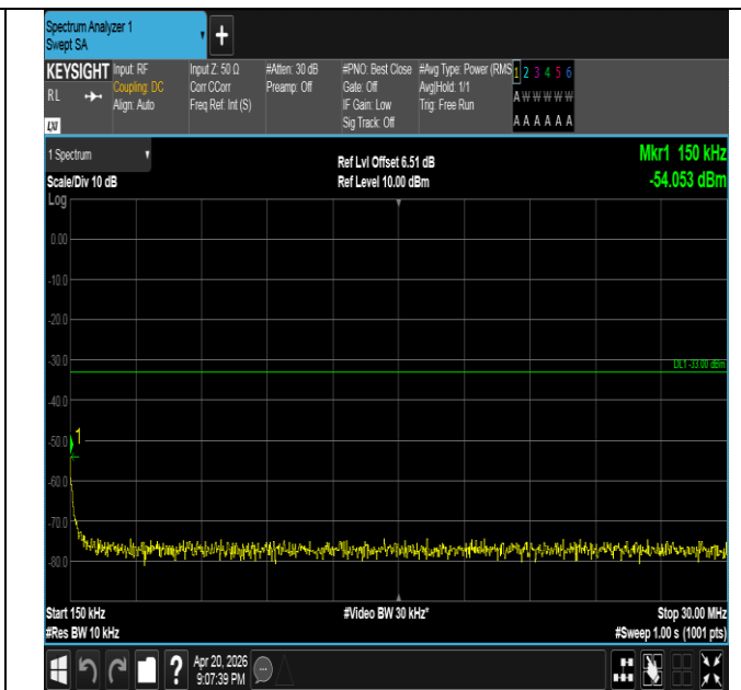
Band25-15MHz-QPSK-26615-1RB#0-0.15~30-PASS
