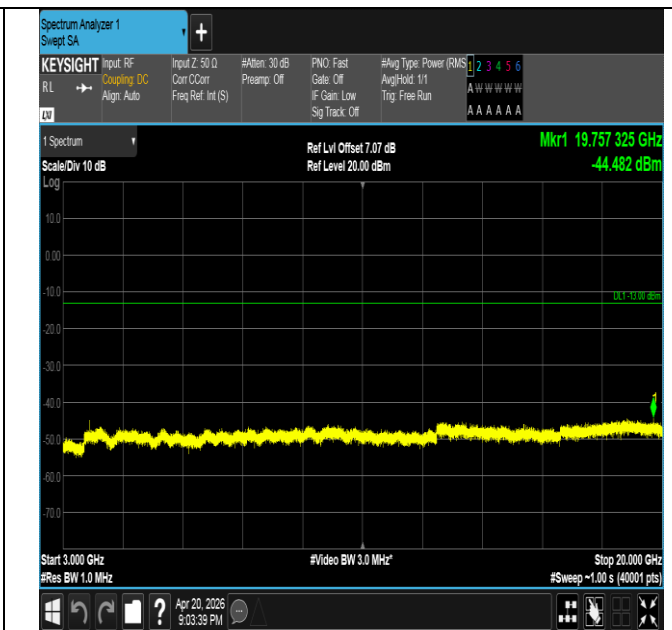
Band25-15MHz-16QAM-26365-1RB#0-3000~20000-PASS
