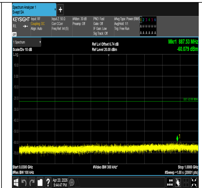
Band25-20MHz-QPSK-26140-1RB#99-30~1000-PASS
