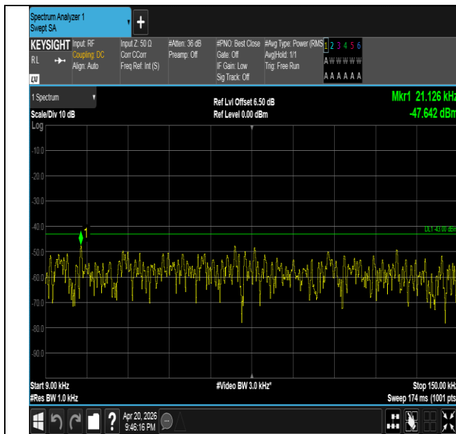
Band25-20MHz-QPSK-26140-100RB#0-0.009~0.15-PASS
