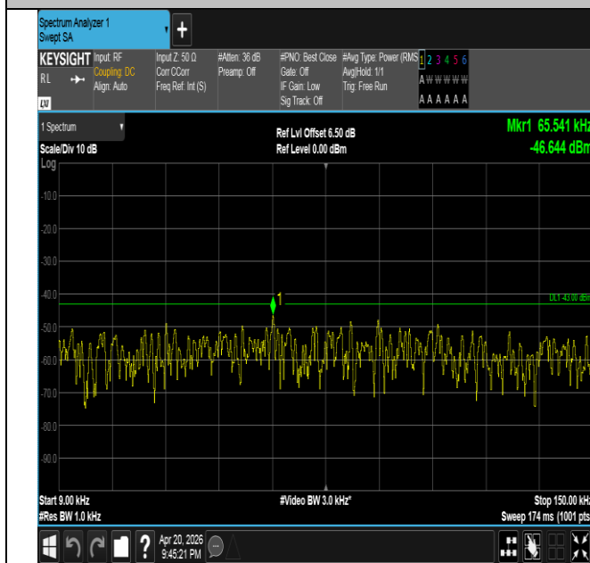
Band25-20MHz-16QAM-26140-1RB#99-0.009~0.15-PASS
