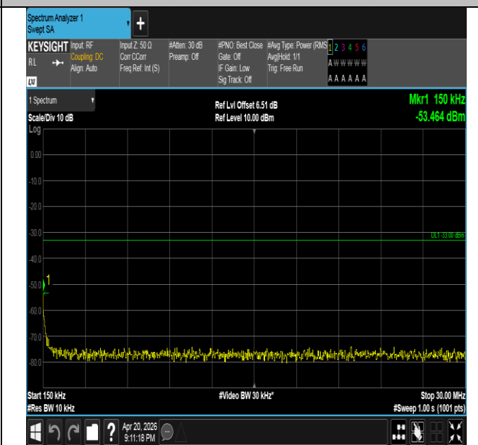
Band25-15MHz-QPSK-26615-75RB#0-0.15~30-PASS
