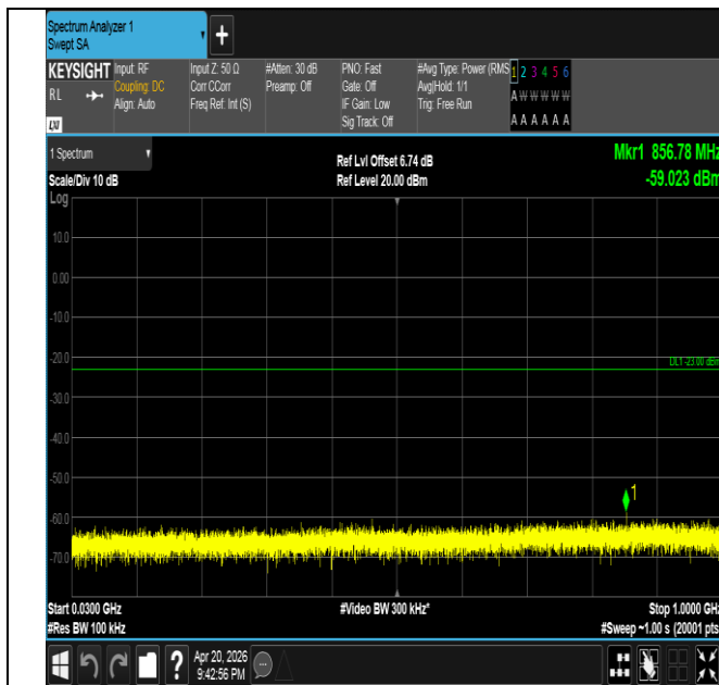
Band25-20MHz-QPSK-26140-1RB#0-30~1000-PASS
