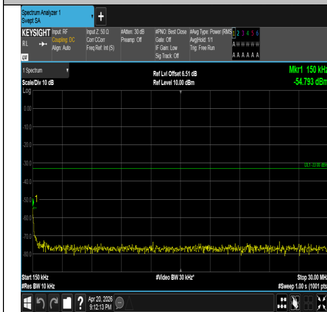
Band25-15MHz-16QAM-26615-75RB#0-0.15~30-PASS
