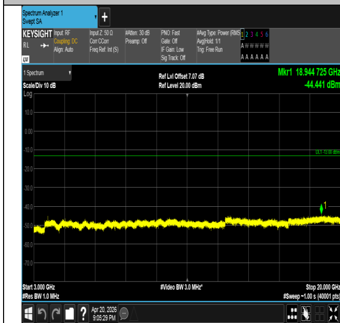
Band25-15MHz-16QAM-26365-1RB#74-3000~20000-PASS
