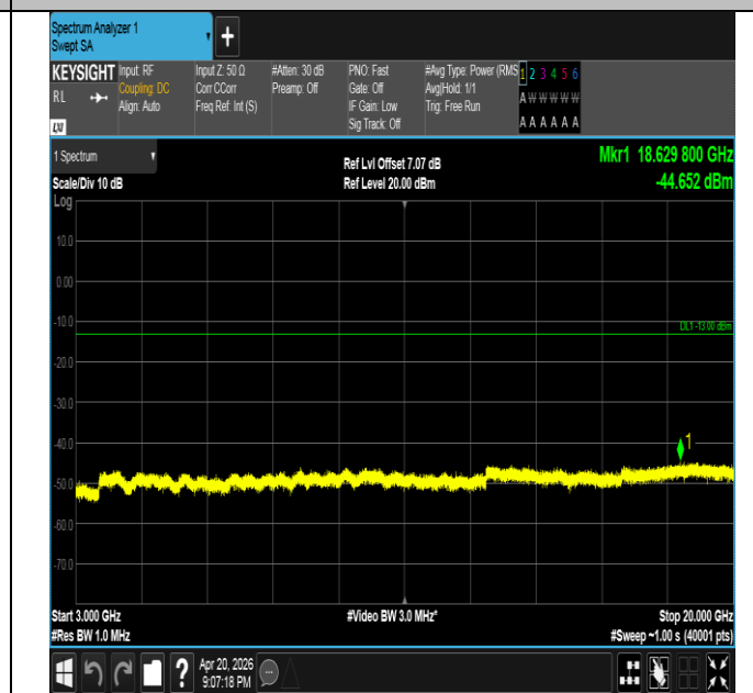
Band25-15MHz-16QAM-26365-75RB#0-3000~20000-PASS
