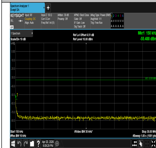
Band25-15MHz-QPSK-26615-1RB#74-0.15~30-PASS
