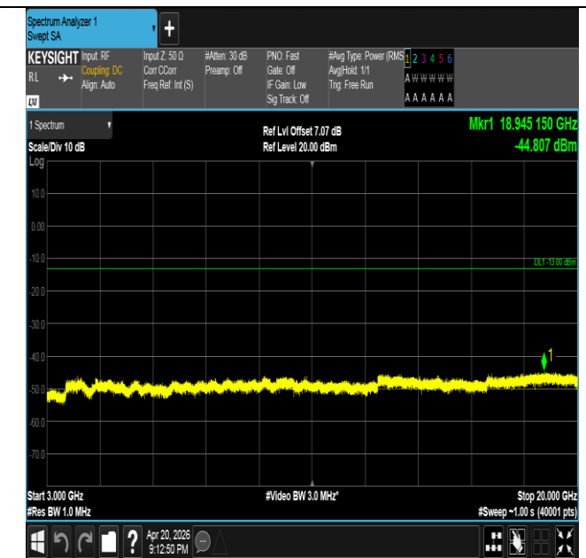
Band25-15MHz-16QAM-26615-75RB#0-3000~20000-PASS
