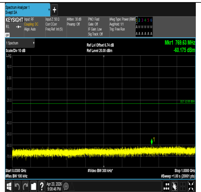
Band25-15MHz-16QAM-26615-1RB#0-30~1000-PASS
