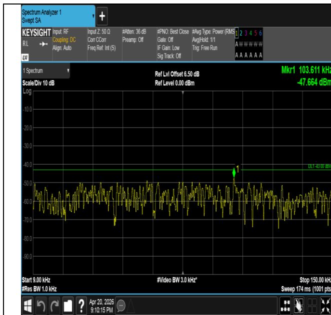
Band25-15MHz-16QAM-26615-1RB#74-0.009~0.15-PASS
