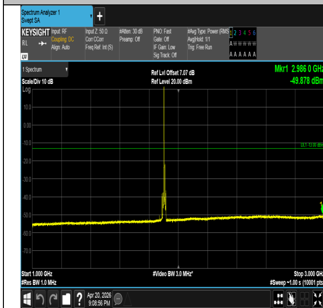
Band25-15MHz-16QAM-26615-1RB#0-1000~3000-PASS
