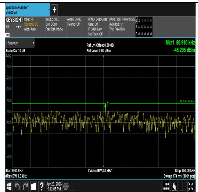
Band25-15MHz-16QAM-26615-75RB#0-0.009~0.15-PASS
