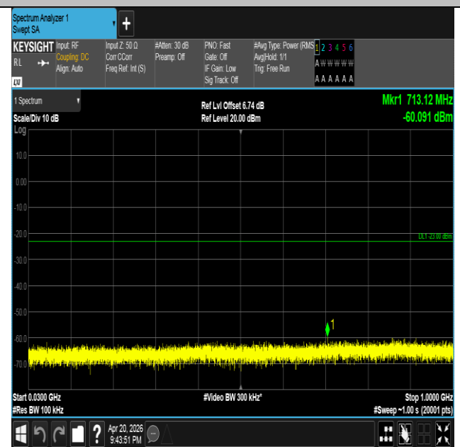
Band25-20MHz-16QAM-26140-1RB#0-30~1000-PASS
