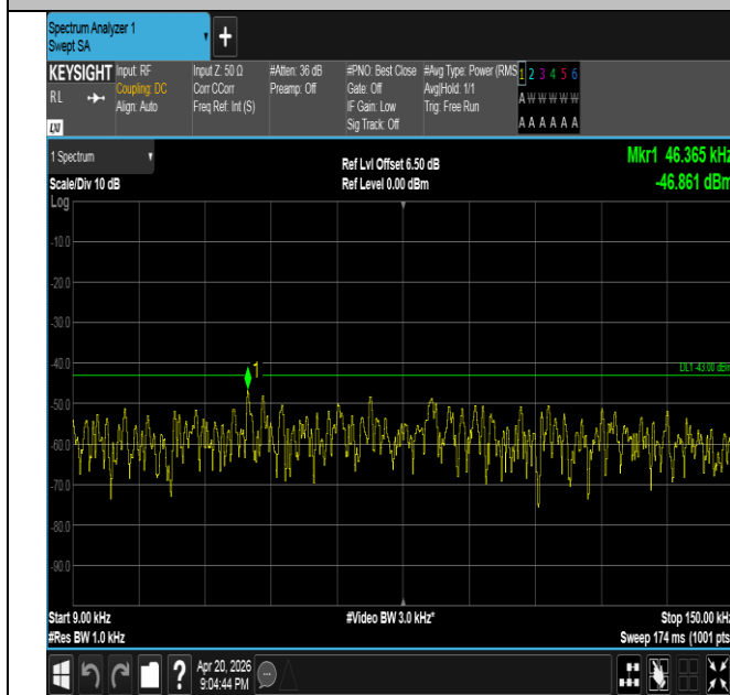
Band25-15MHz-16QAM-26365-1RB#74-0.009~0.15-PASS
