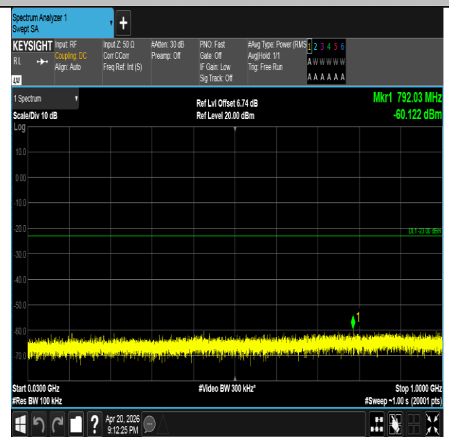
Band25-15MHz-16QAM-26615-75RB#0-30~1000-PASS
