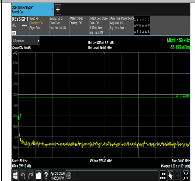
Band25-20MHz-16QAM-26140-1RB#99-0.15~30-PASS
