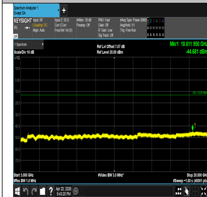
Band25-20MHz-QPSK-26140-1RB#0-3000~20000-PASS
