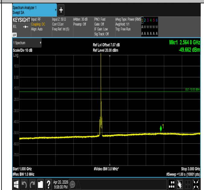
Band25-15MHz-QPSK-26615-1RB#0-1000~3000-PASS
