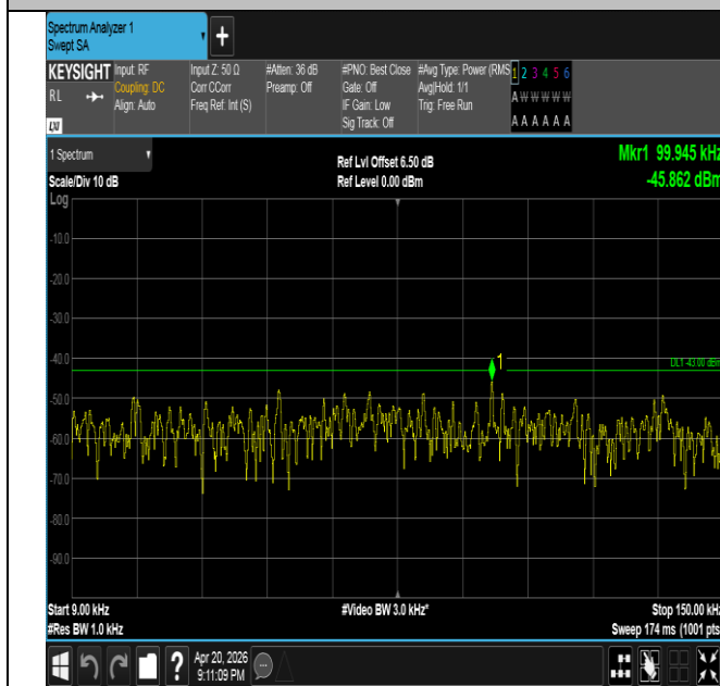
Band25-15MHz-QPSK-26615-75RB#0-0.009~0.15-PASS
