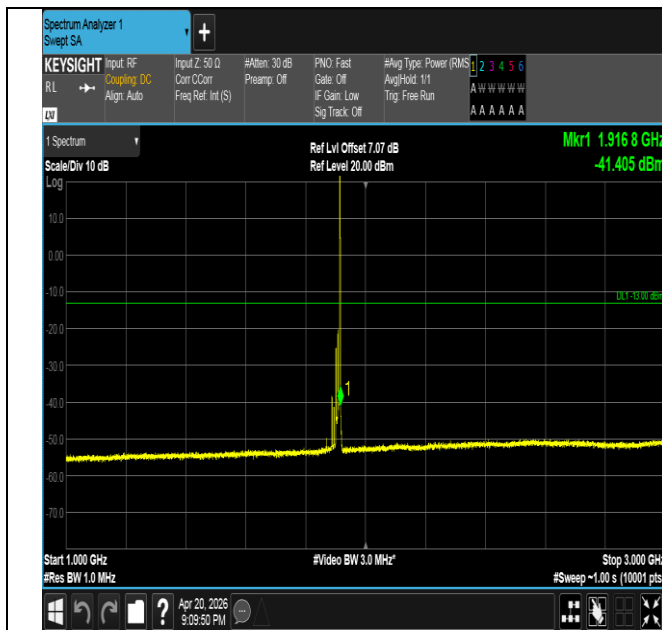
Band25-15MHz-QPSK-26615-1RB#74-1000~3000-PASS
