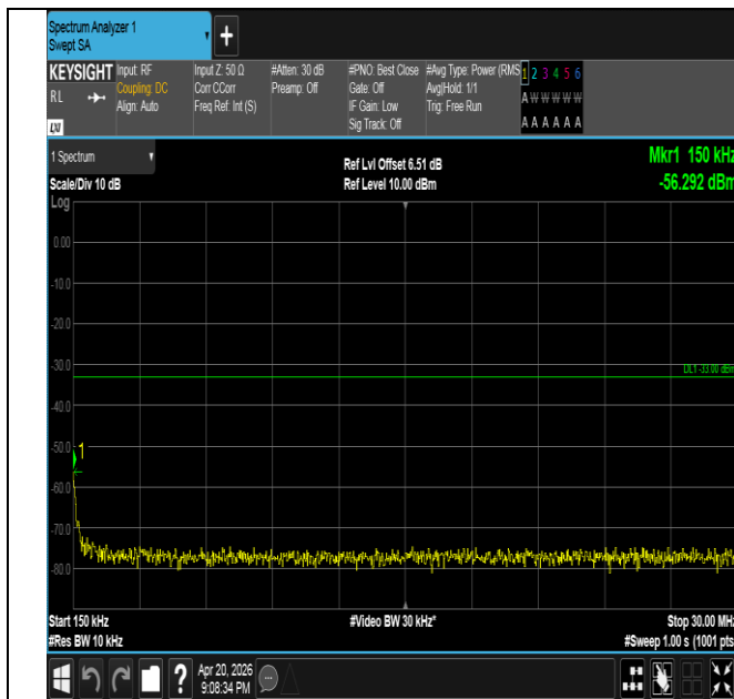
Band25-15MHz-16QAM-26615-1RB#0-0.15~30-PASS
