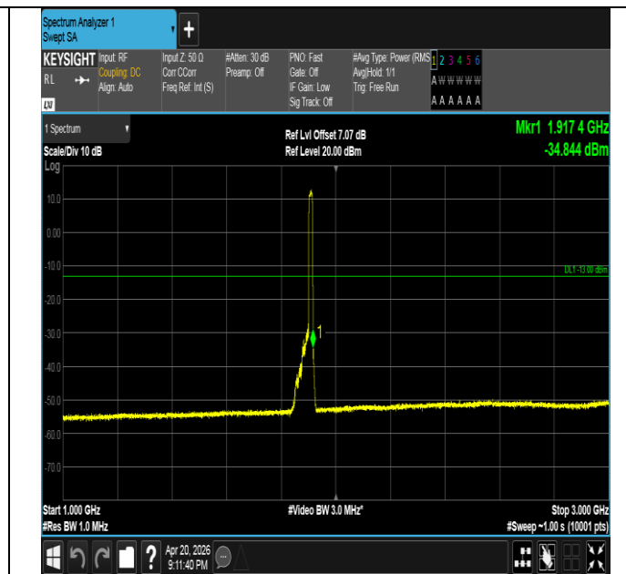
Band25-15MHz-QPSK-26615-75RB#0-1000~3000-PASS
