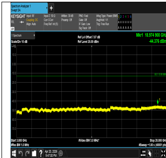
Band25-20MHz-QPSK-26140-100RB#0-3000~20000-PASS
