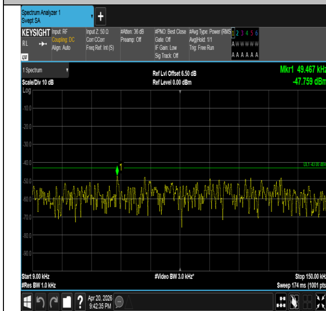
Band25-20MHz-QPSK-26140-1RB#0-0.009~0.15-PASS
