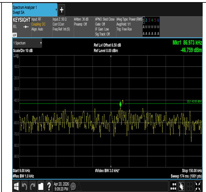
Band25-15MHz-QPSK-26615-1RB#74-0.009~0.15-PASS
