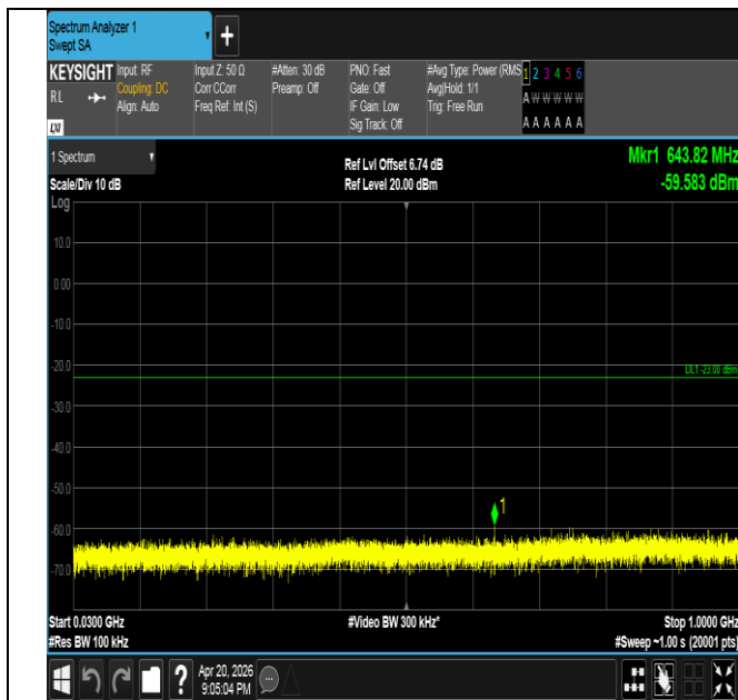
Band25-15MHz-16QAM-26365-1RB#74-30~1000-PASS
