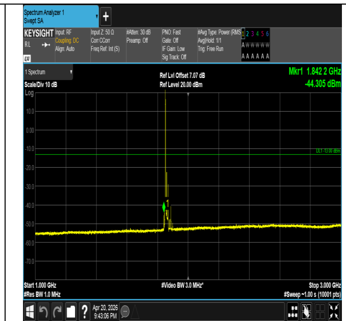
Band25-20MHz-QPSK-26140-1RB#0-1000~3000-PASS
