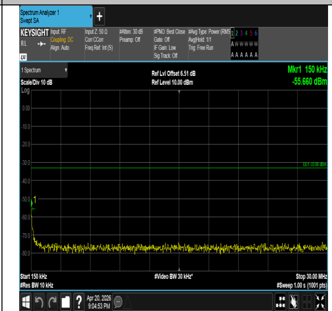
Band25-15MHz-16QAM-26365-1RB#74-0.15~30-PASS
