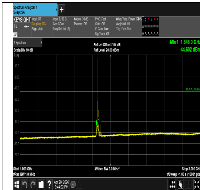
Band25-20MHz-16QAM-26140-1RB#0-1000~3000-PASS
