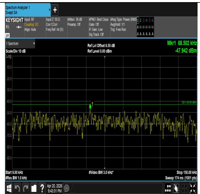
Band25-20MHz-16QAM-26140-1RB#0-0.009~0.15-PASS
