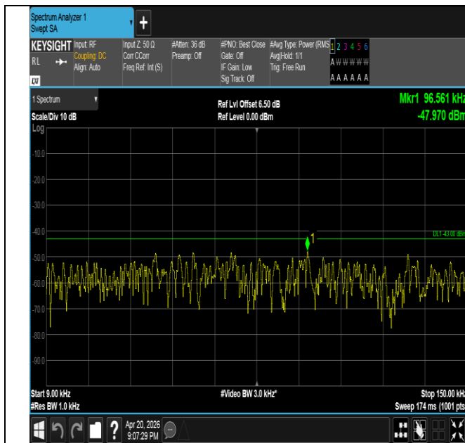
Band25-15MHz-QPSK-26615-1RB#0-0.009~0.15-PASS
