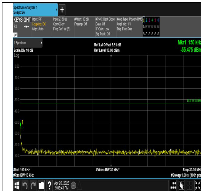
Band25-15MHz-16QAM-26365-75RB#0-0.15~30-PASS
