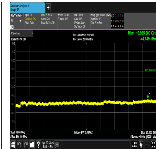
Band25-15MHz-QPSK-26615-1RB#0-3000~20000-PASS
