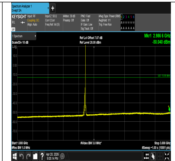
Band25-15MHz-16QAM-26365-1RB#74-1000~3000-PASS
