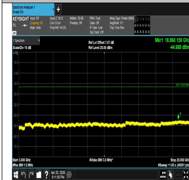
Band25-15MHz-QPSK-26615-75RB#0-3000~20000-PASS
