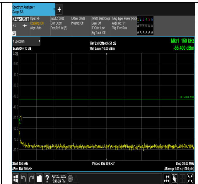
Band25-20MHz-QPSK-26140-100RB#0-0.15~30-PASS
