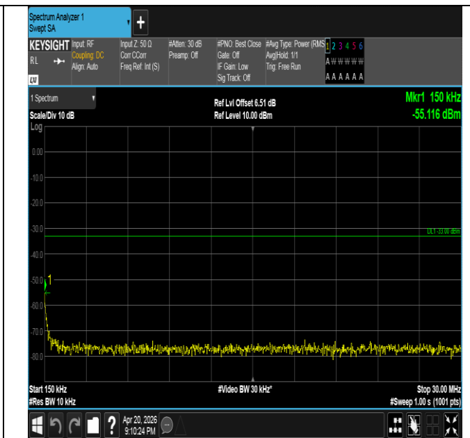
Band25-15MHz-16QAM-26615-1RB#74-0.15~30-PASS
