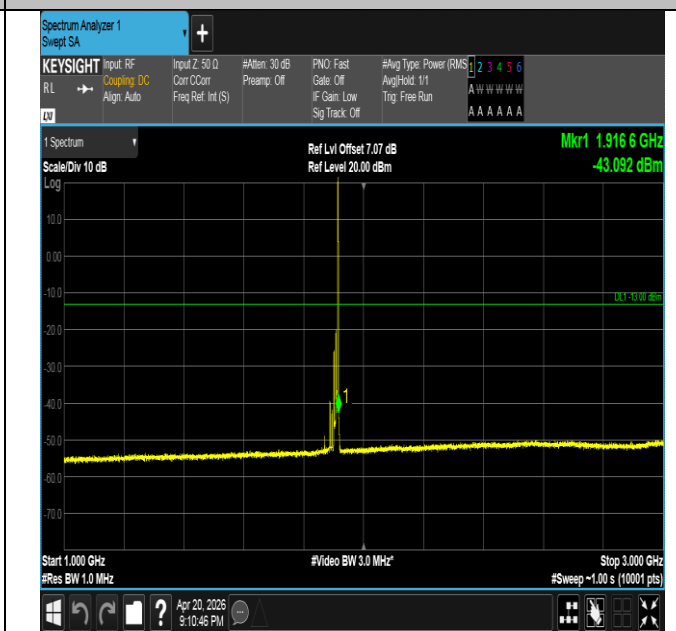
Band25-15MHz-16QAM-26615-1RB#74-1000~3000-PASS
