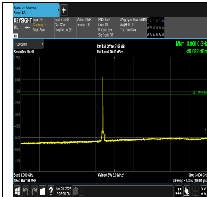
Band25-15MHz-16QAM-26365-1RB#0-1000~3000-PASS
