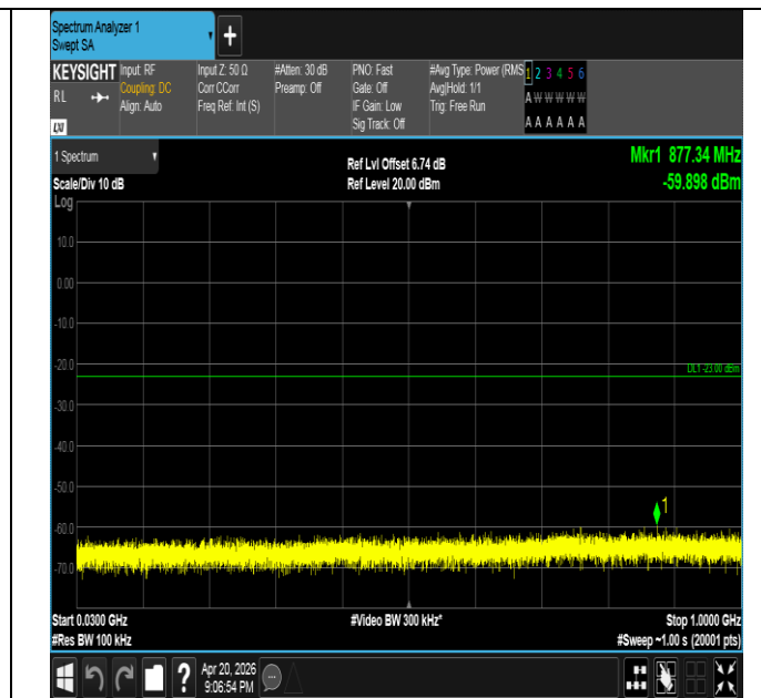
Band25-15MHz-16QAM-26365-75RB#0-30~1000-PASS
