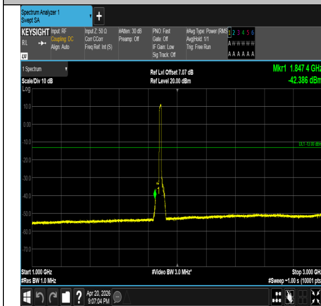
Band25-15MHz-16QAM-26365-75RB#0-1000~3000-PASS
