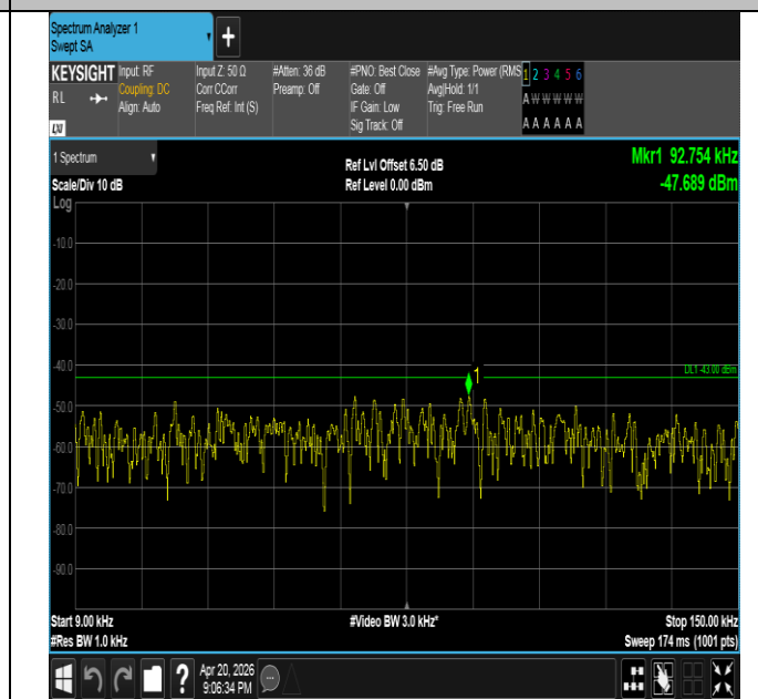
Band25-15MHz-16QAM-26365-75RB#0-0.009~0.15-PASS
