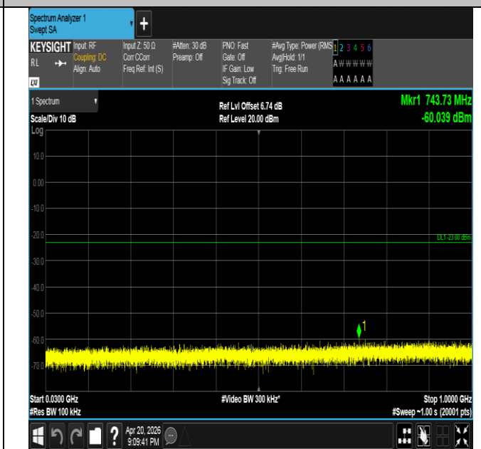
Band25-15MHz-QPSK-26615-1RB#74-30~1000-PASS
