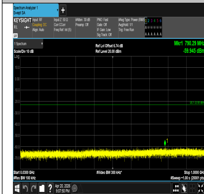
Band25-15MHz-QPSK-26615-1RB#0-30~1000-PASS
