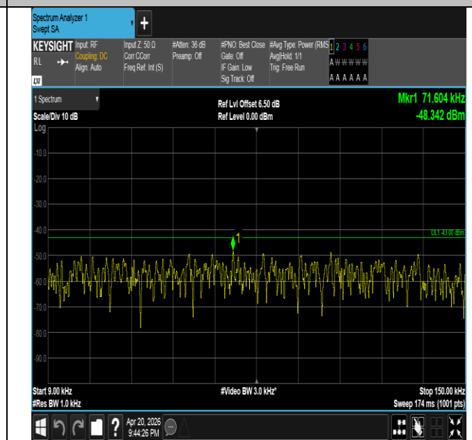
Band25-20MHz-QPSK-26140-1RB#99-0.009~0.15-PASS
