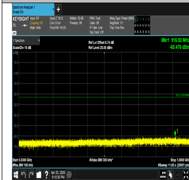
Band25-15MHz-16QAM-26615-1RB#74-30~1000-PASS
