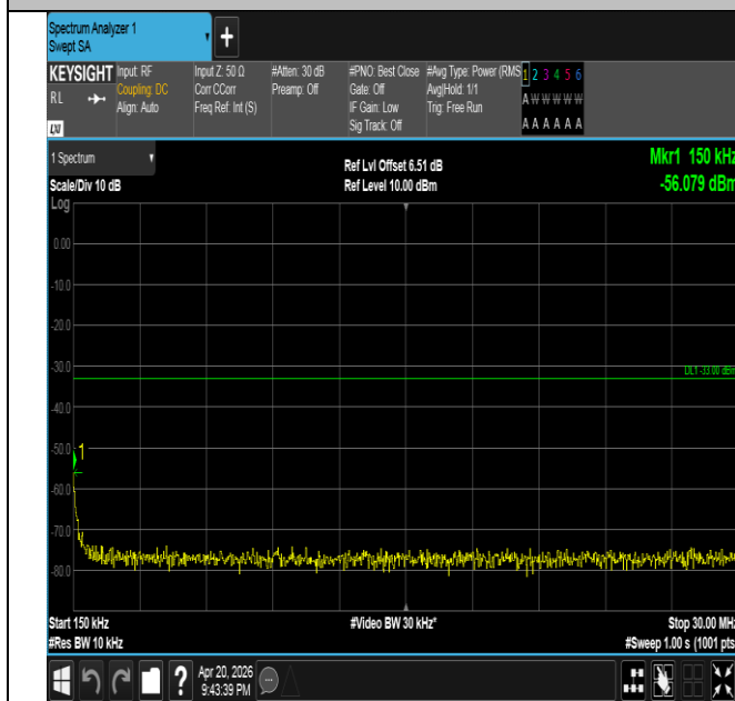
Band25-20MHz-16QAM-26140-1RB#0-0.15~30-PASS
