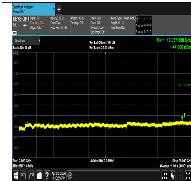
Band25-15MHz-16QAM-26615-1RB#74-3000~20000-PASS
