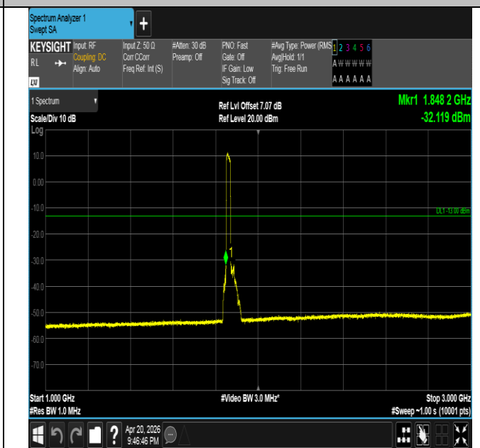
Band25-20MHz-QPSK-26140-100RB#0-1000~3000-PASS
