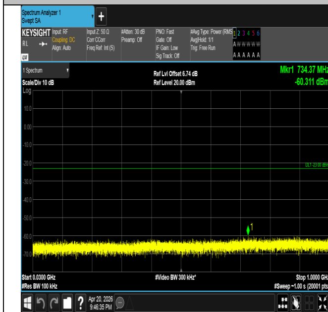
Band25-20MHz-QPSK-26140-100RB#0-30~1000-PASS
