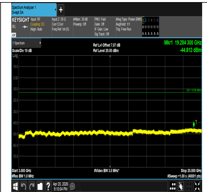
Band25-15MHz-QPSK-26615-1RB#74-3000~20000-PASS
