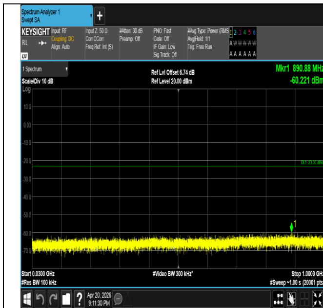
Band25-15MHz-QPSK-26615-75RB#0-30~1000-PASS
