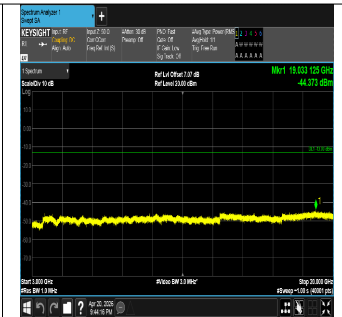
Band25-20MHz-16QAM-26140-1RB#0-3000~20000-PASS
