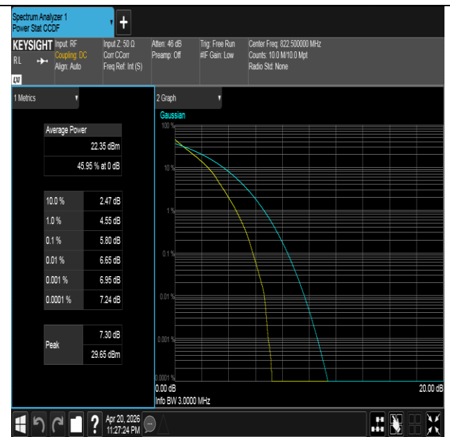
Band26(814-824)-3MHz-QPSK-26775-15RB#0-PASS
