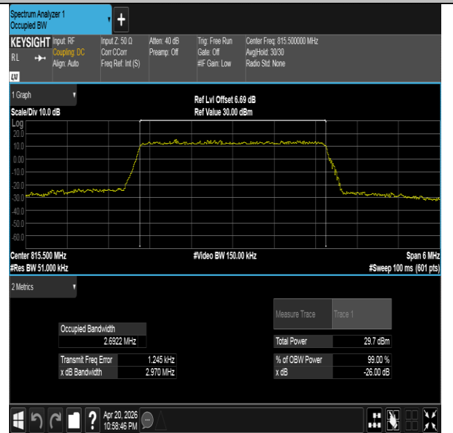
Band26(814-824)-3MHz-16QAM-26705-15RB#0-PASS
