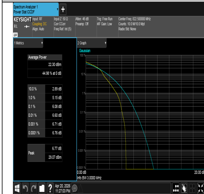
Band26(814-824)-3MHz-16QAM-26775-1RB#0-PASS
