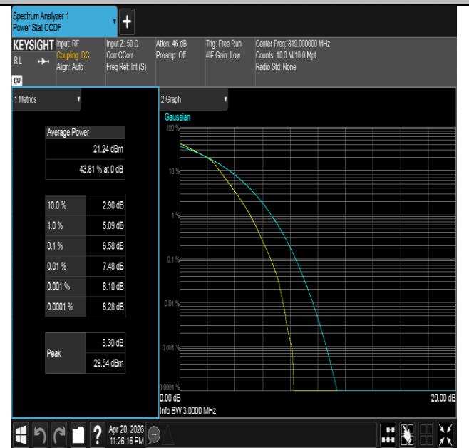
Band26(814-824)-3MHz-16QAM-26740-15RB#0-PASS
