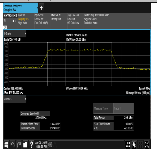
Band26(814-824)-3MHz-16QAM-26775-15RB#0-PASS
