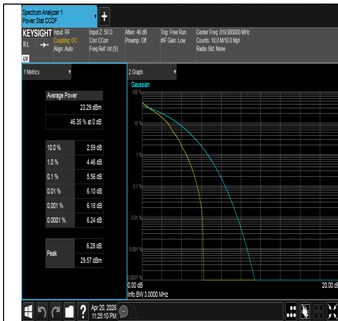
Band26(814-824)-3MHz-QPSK-26740-1RB#0-PASS
