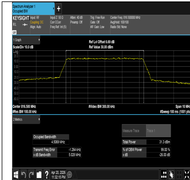
Band26(814-824)-5MHz-QPSK-26715-25RB#0-PASS
