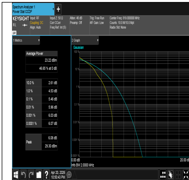
Band26(814-824)-1.4MHz-QPSK-26740-1RB#0-PASS
