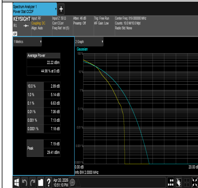
Band26(814-824)-1.4MHz-16QAM-26740-1RB#0-PASS
