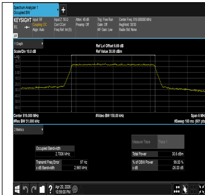
Band26(814-824)-3MHz-QPSK-26740-15RB#0-PASS
