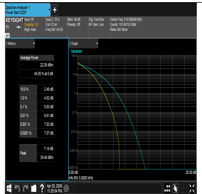
Band26(814-824)-3MHz-QPSK-26740-15RB#0-PASS
