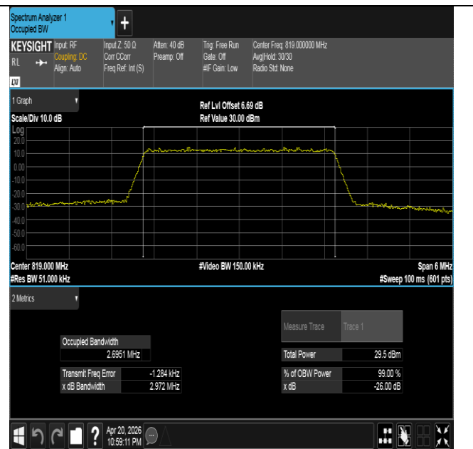
Band26(814-824)-3MHz-16QAM-26740-15RB#0-PASS
