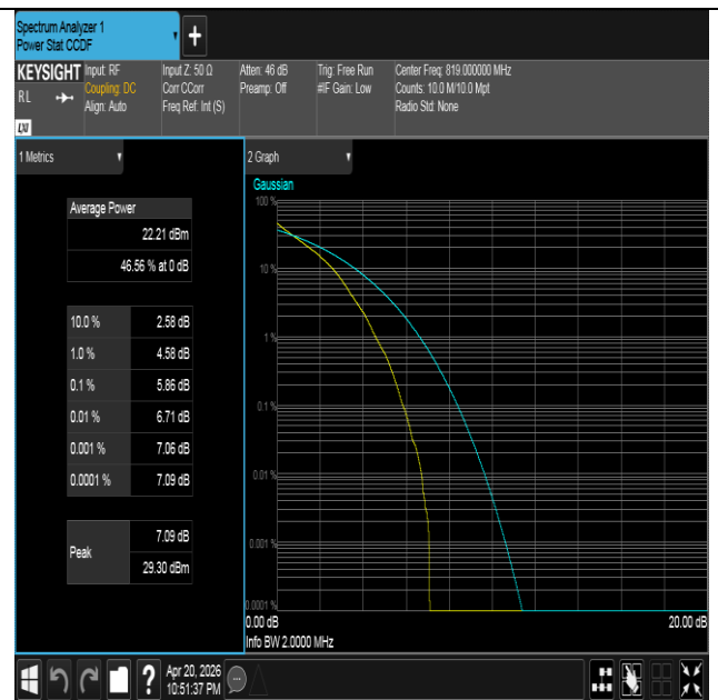
Band26(814-824)-1.4MHz-QPSK-26740-6RB#0-PASS
