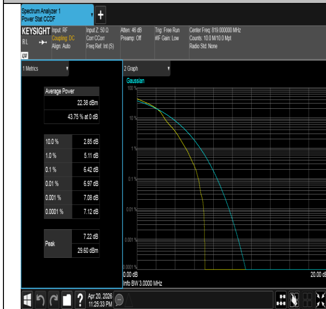
Band26(814-824)-3MHz-16QAM-26740-1RB#0-PASS
