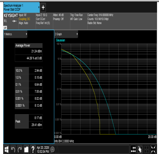
Band26(814-824)-1.4MHz-16QAM-26740-6RB#0-PASS
