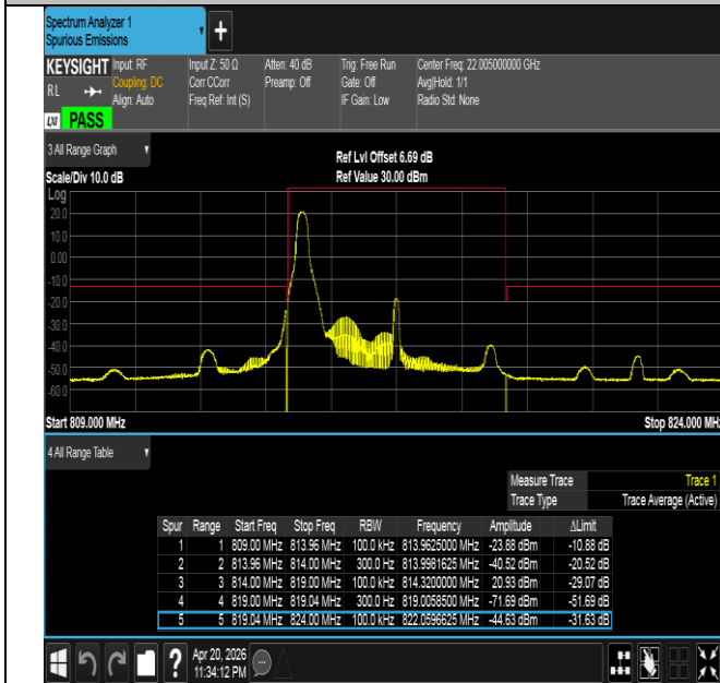
Band26(814-824)-5MHz-QPSK-26715-1RB#0-PASS
