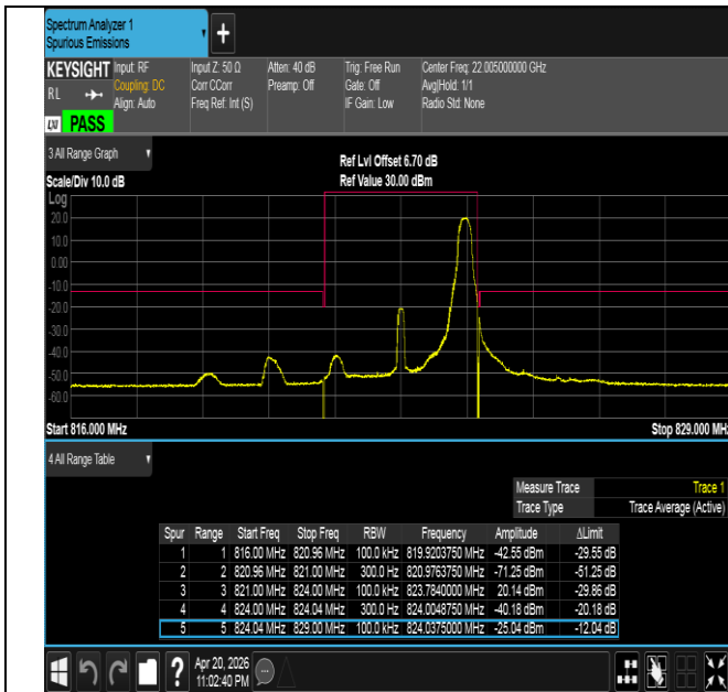
Band26(814-824)-3MHz-16QAM-26775-1RB#14-PASS
