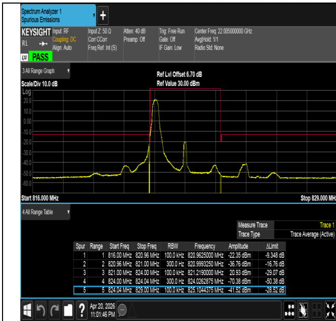
Band26(814-824)-3MHz-QPSK-26775-1RB#0-PASS
