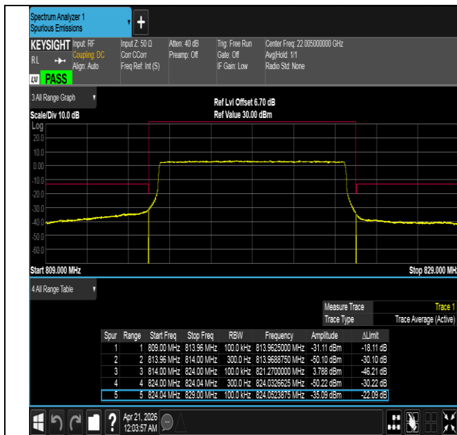
Band26(814-824)-10MHz-QPSK-26740-50RB#0-PASS
