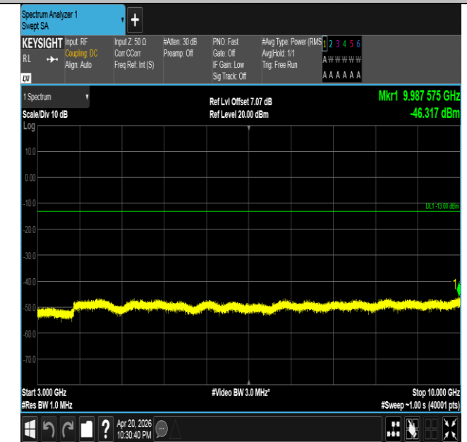
Band26(814-824)-1.4MHz-16QAM-26697-1RB#0-3000~10000
