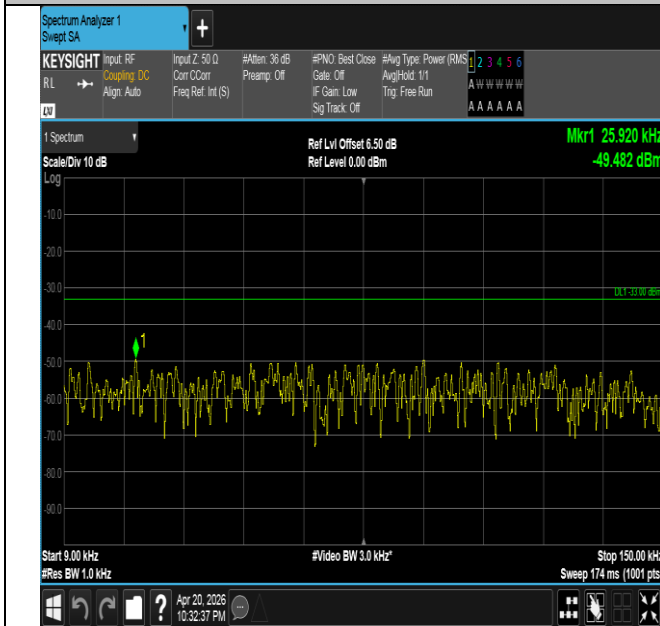
Band26(814-824)-1.4MHz-QPSK-26697-6RB#0-0.009~0.15-P ASS
