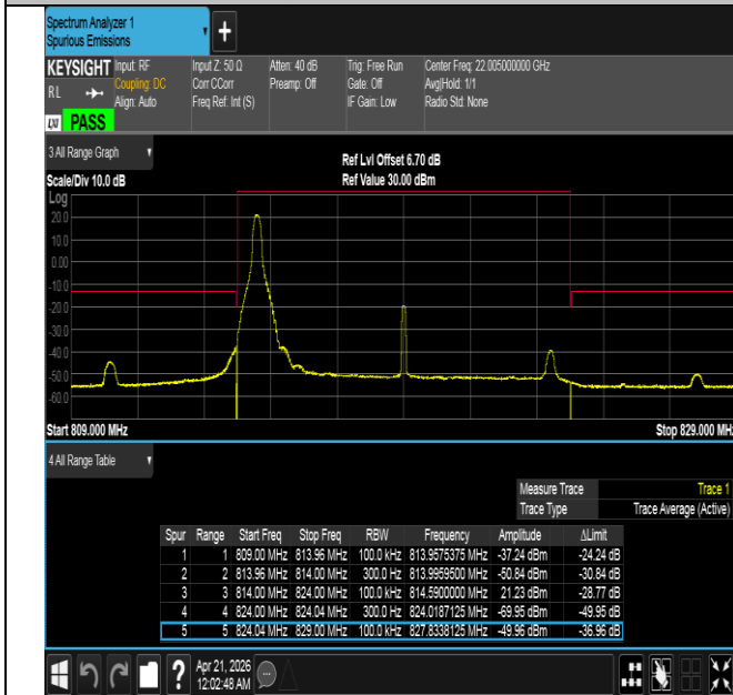
Band26(814-824)-10MHz-QPSK-26740-1RB#0-PASS
