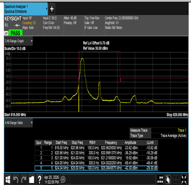
Band26(814-824)-3MHz-16QAM-26775-1RB#0-PASS
