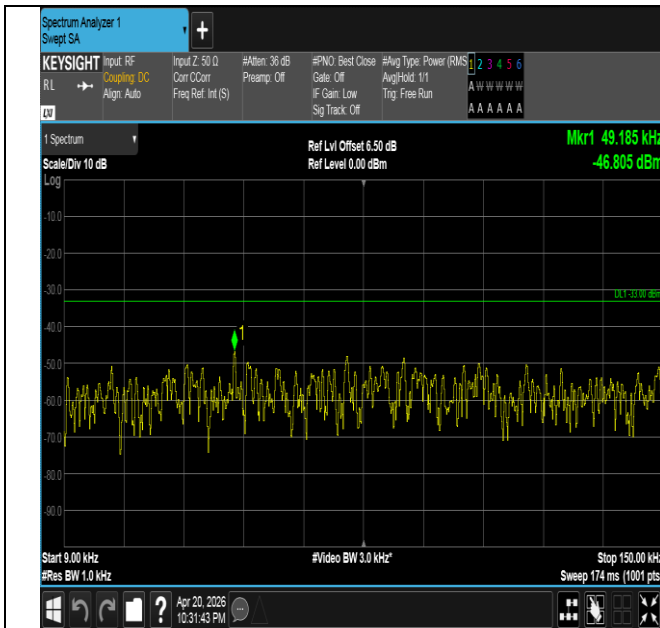
Band26(814-824)-1.4MHz-16QAM-26697-1RB#5-0.009~0.15- PASS
