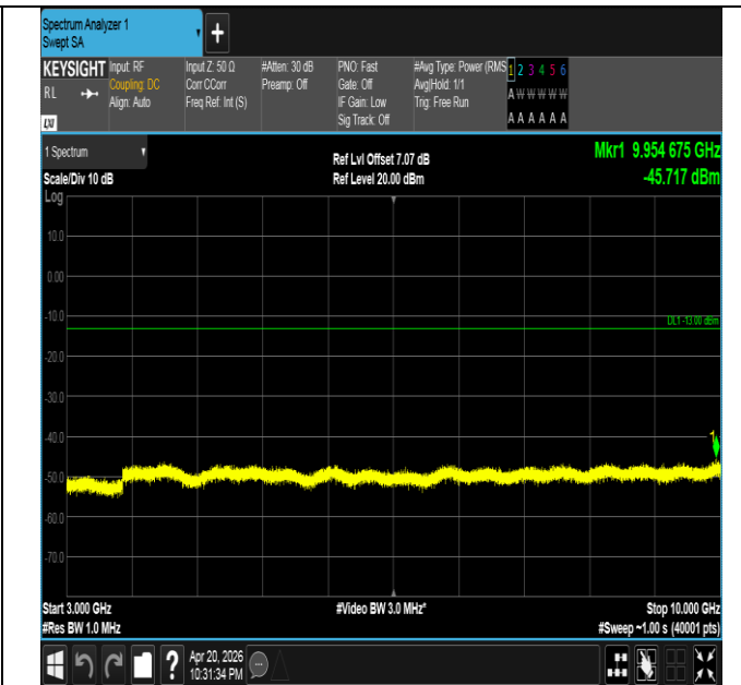
Band26(814-824)-1.4MHz-QPSK-26697-1RB#5-3000~10000- PASS
