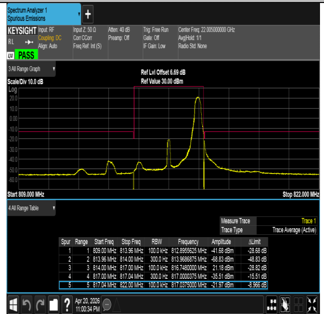
Band26(814-824)-3MHz-QPSK-26705-1RB#14-PASS
