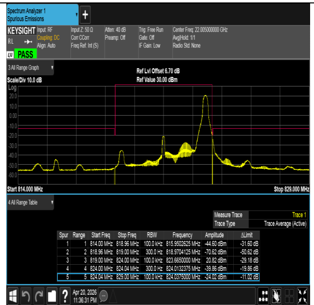
Band26(814-824)-5MHz-QPSK-26765-1RB#24-PASS
