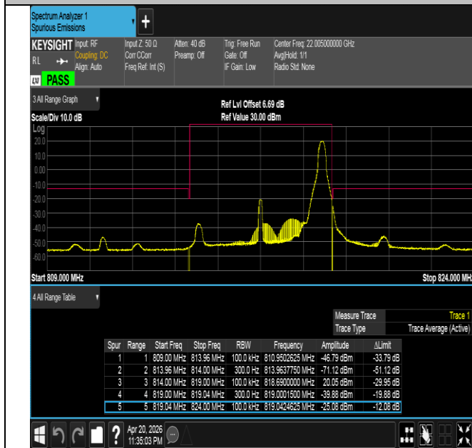
Band26(814-824)-5MHz-16QAM-26715-1RB#24-PASS
