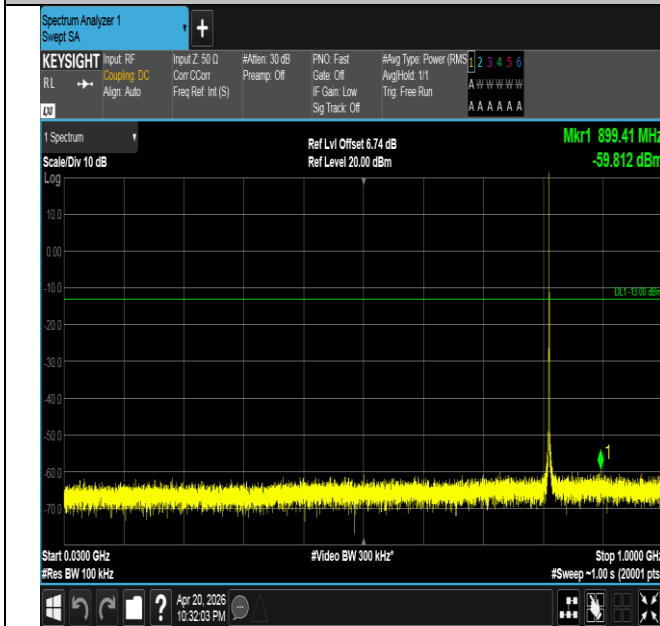
Band26(814-824)-1.4MHz-16QAM-26697-1RB#5-30~1000-PA SS
