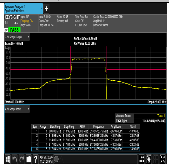
Band26(814-824)-3MHz-16QAM-26705-15RB#0-PASS
