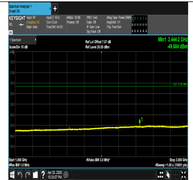
Band26(814-824)-1.4MHz-QPSK-26697-6RB#0-1000~3000-P ASS
