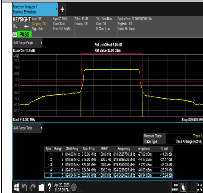
Band26(814-824)-5MHz-QPSK-26765-25RB#0-PASS
