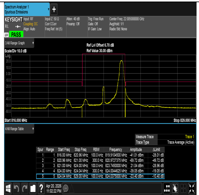
Band26(814-824)-3MHz-QPSK-26775-1RB#14-PASS
