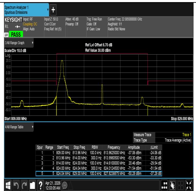
Band26(814-824)-10MHz-16QAM-26740-1RB#0-PASS
