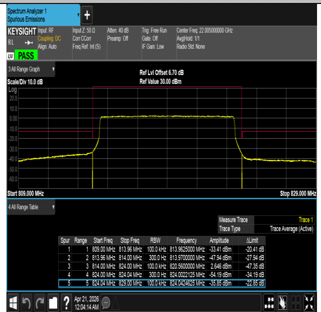
Band26(814-824)-10MHz-16QAM-26740-50RB#0-PASS
