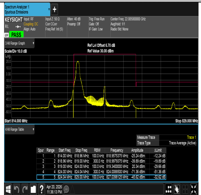
Band26(814-824)-5MHz-16QAM-26765-1RB#0-PASS
