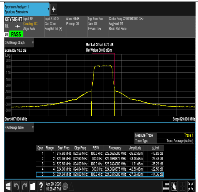
Band26(814-824)-1.4MHz-16QAM-26783-6RB#0-PASS
