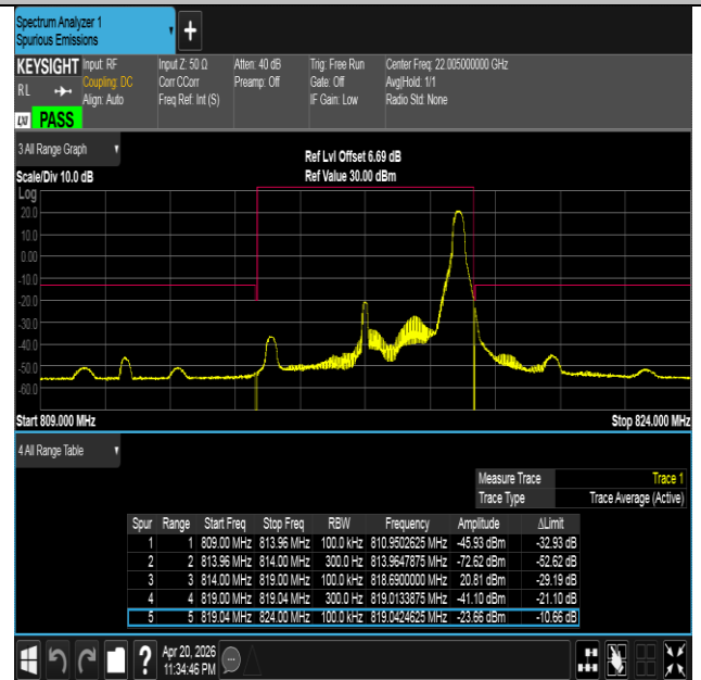
Band26(814-824)-5MHz-QPSK-26715-1RB#24-PASS
