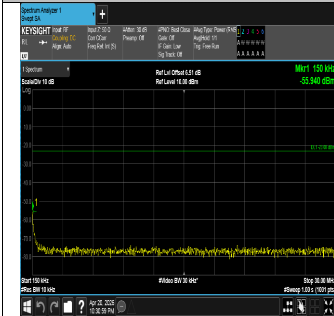
Band26(814-824)-1.4MHz-QPSK-26697-1RB#5-0.15~30-PAS S
