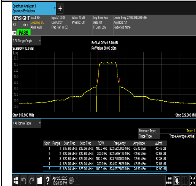
Band26(814-824)-1.4MHz-QPSK-26783-6RB#0-PASS
