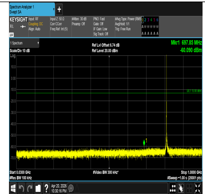
Band26(814-824)-1.4MHz-16QAM-26697-1RB#0-30~1000-PA
