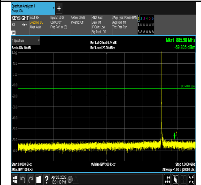
Band26(814-824)-1.4MHz-QPSK-26697-1RB#5-30~1000-PAS S
