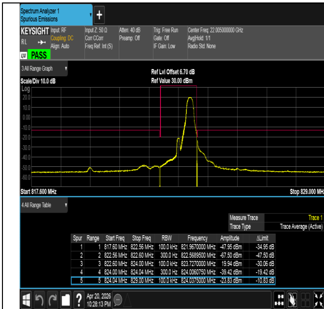
Band26(814-824)-1.4MHz-16QAM-26783-1RB#5-PASS
