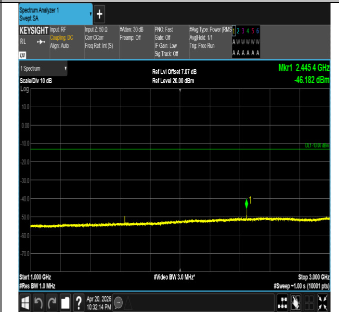
Band26(814-824)-1.4MHz-16QAM-26697-1RB#5-1000~3000- PASS
