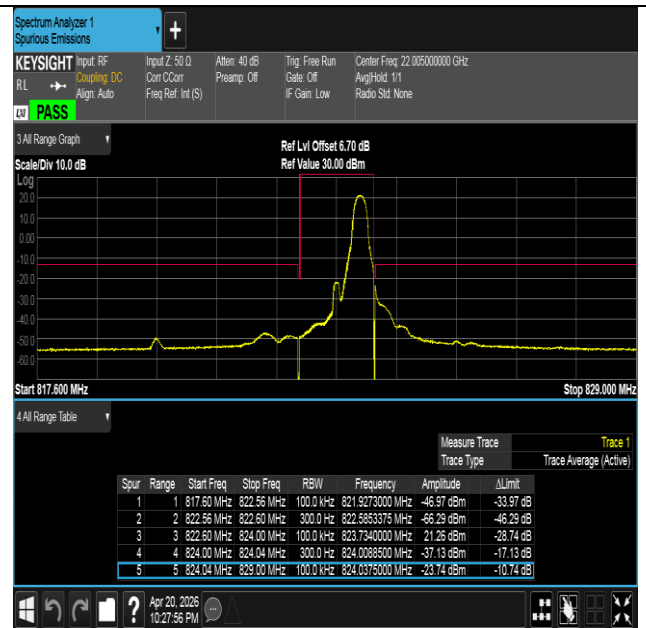
Band26(814-824)-1.4MHz-QPSK-26783-1RB#5-PASS
