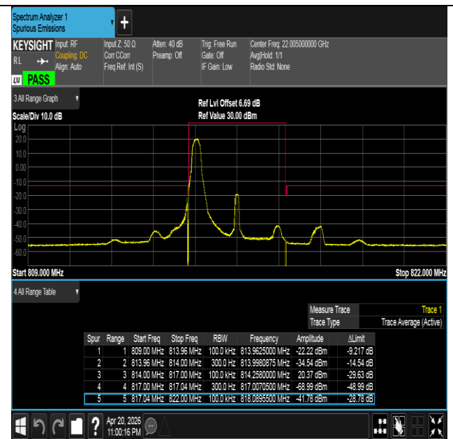
Band26(814-824)-3MHz-16QAM-26705-1RB#0-PASS
