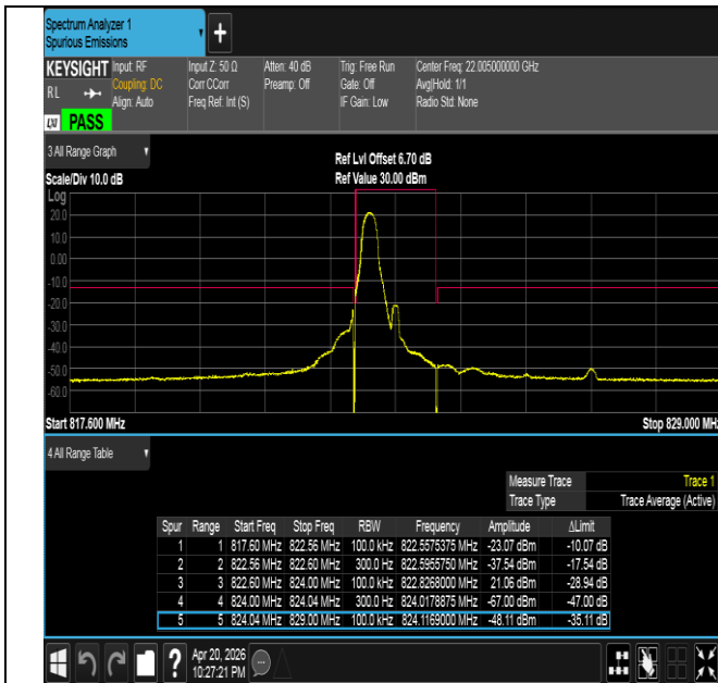
Band26(814-824)-1.4MHz-QPSK-26783-1RB#0-PASS
