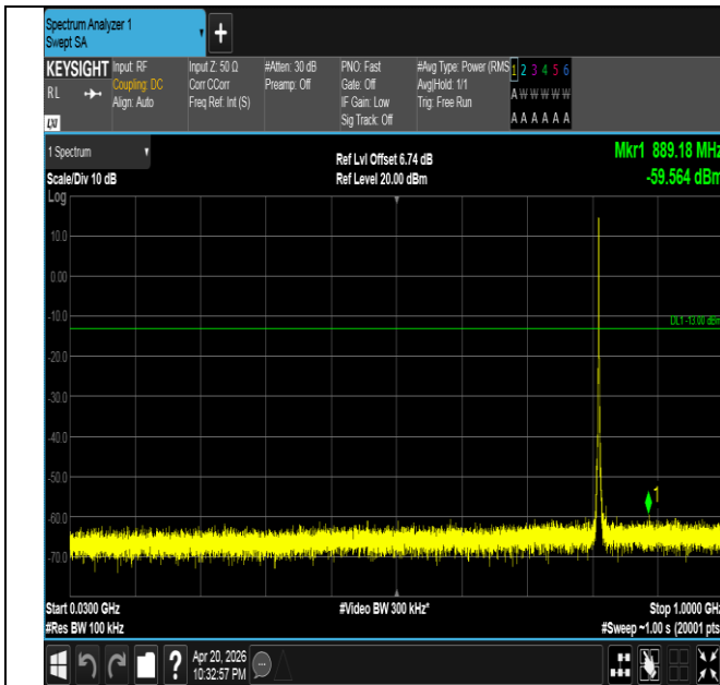
Band26(814-824)-1.4MHz-QPSK-26697-6RB#0-30~1000-PAS S
