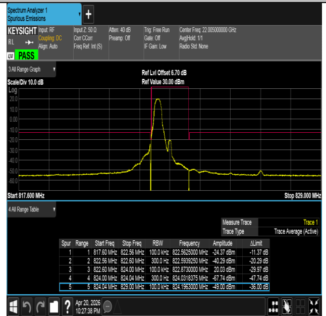
Band26(814-824)-1.4MHz-16QAM-26783-1RB#0-PASS
