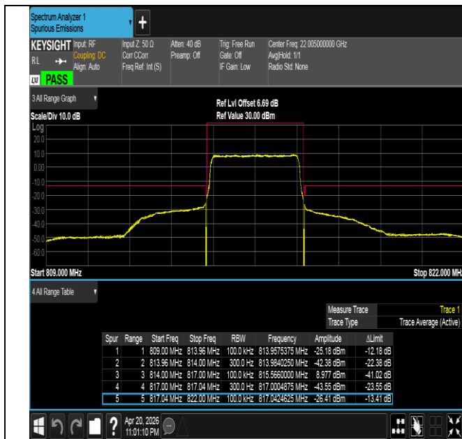
Band26(814-824)-3MHz-QPSK-26705-15RB#0-PASS
