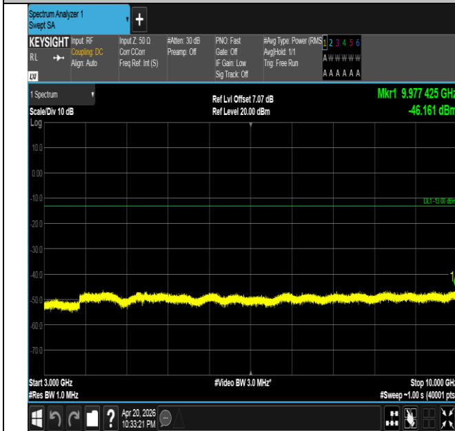
Band26(814-824)-1.4MHz-QPSK-26697-6RB#0-3000~10000- PASS
