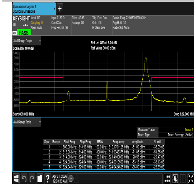
Band26(814-824)-10MHz-16QAM-26740-1RB#49-PASS
