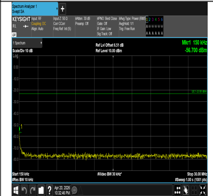
Band26(814-824)-1.4MHz-QPSK-26697-6RB#0-0.15~30-PAS S
