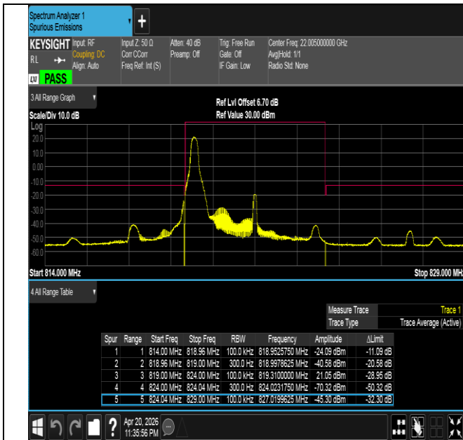
Band26(814-824)-5MHz-QPSK-26765-1RB#0-PASS
