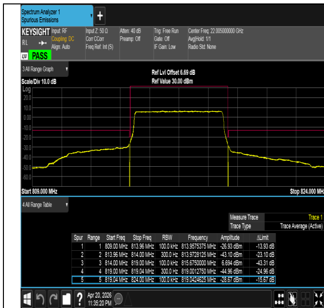
Band26(814-824)-5MHz-QPSK-26715-25RB#0-PASS
