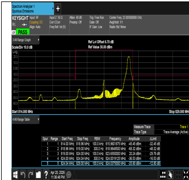
Band26(814-824)-5MHz-16QAM-26765-1RB#24-PASS
