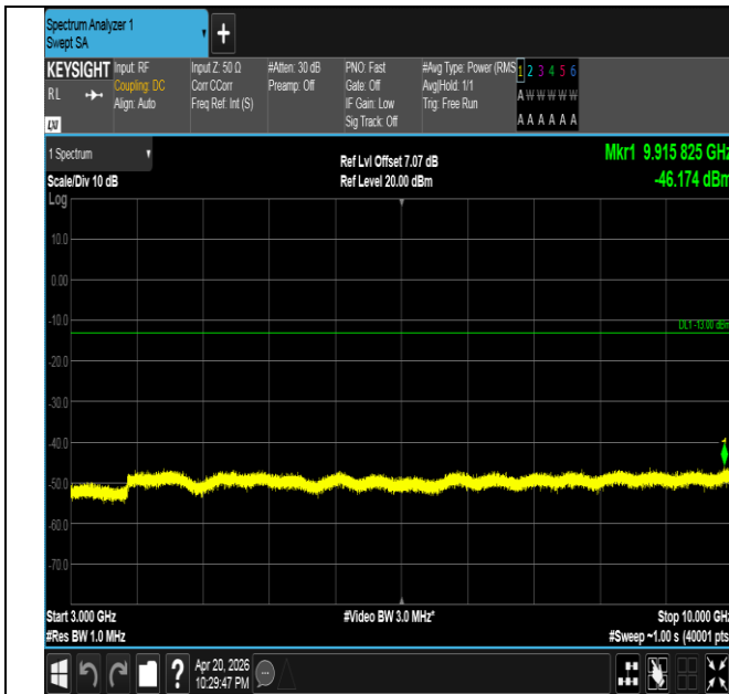
Band26(814-824)-1.4MHz-QPSK-26697-1RB#0-3000~10000- PASS
