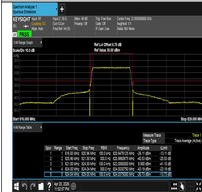
Band26(814-824)-3MHz-QPSK-26775-15RB#0-PASS
