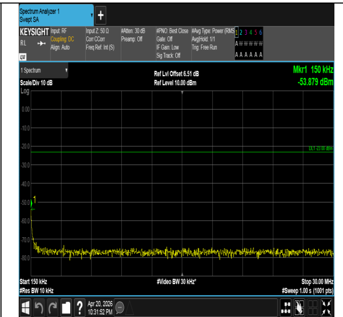
Band26(814-824)-1.4MHz-16QAM-26697-1RB#5-0.15~30-PA SS
