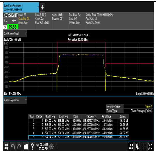
Band26(814-824)-5MHz-16QAM-26765-25RB#0-PASS
