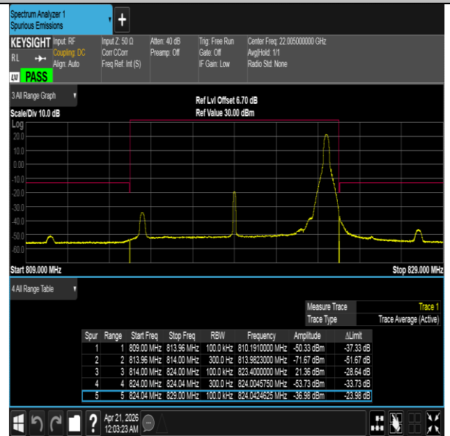
Band26(814-824)-10MHz-QPSK-26740-1RB#49-PASS
