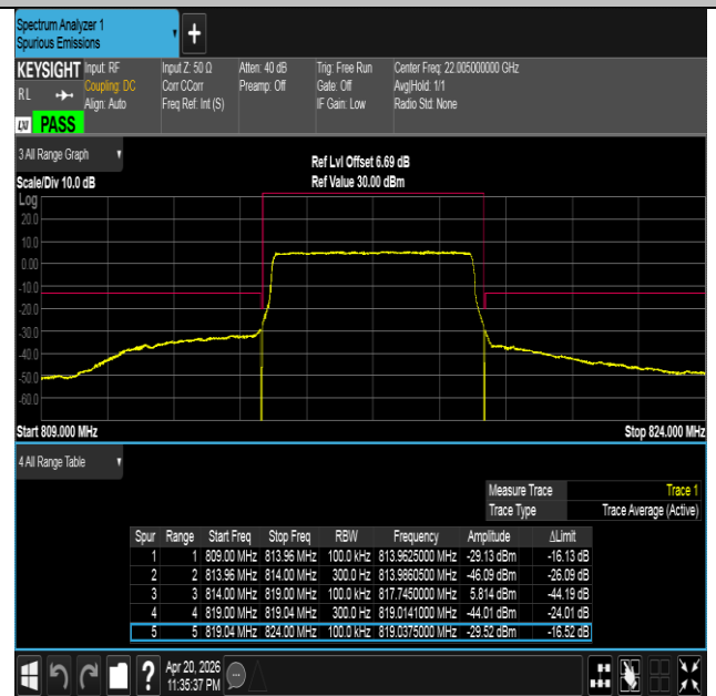
Band26(814-824)-5MHz-16QAM-26715-25RB#0-PASS
