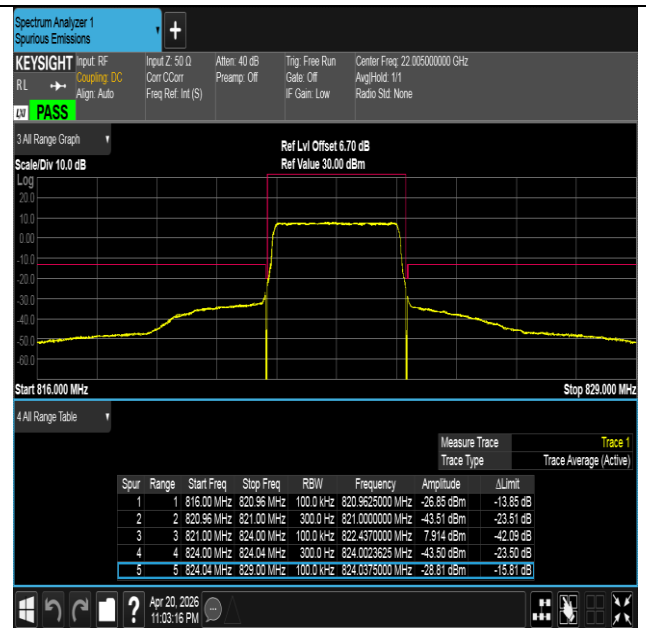
Band26(814-824)-3MHz-16QAM-26775-15RB#0-PASS
