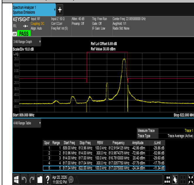
Band26(814-824)-3MHz-16QAM-26705-1RB#14-PASS
