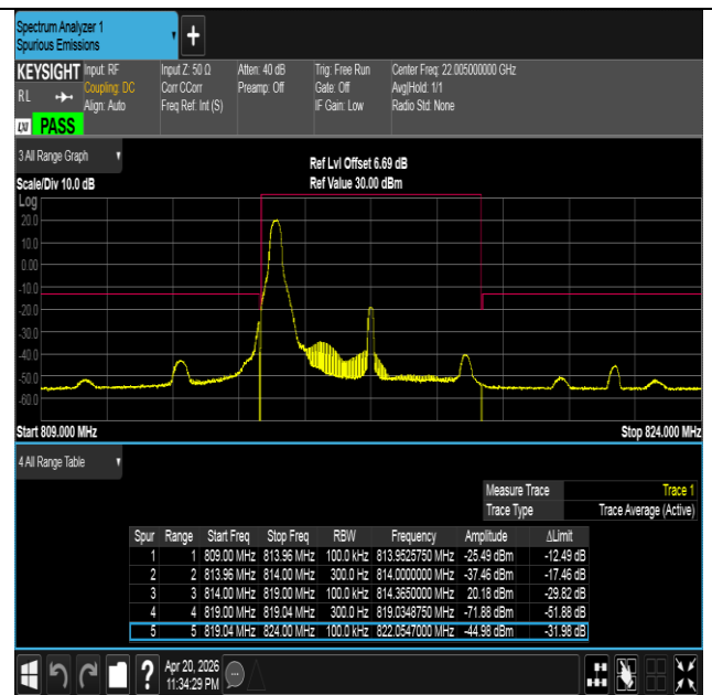
Band26(814-824)-5MHz-16QAM-26715-1RB#0-PASS
