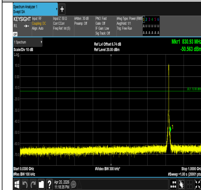
Band26(814-824)-3MHz-QPSK-26775-15RB#0-30~1000-PAS
