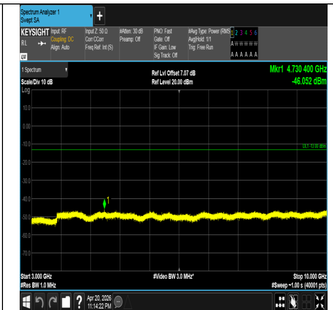
Band26(814-824)-3MHz-16QAM-26740-15RB#0-3000~10000 -PASS
