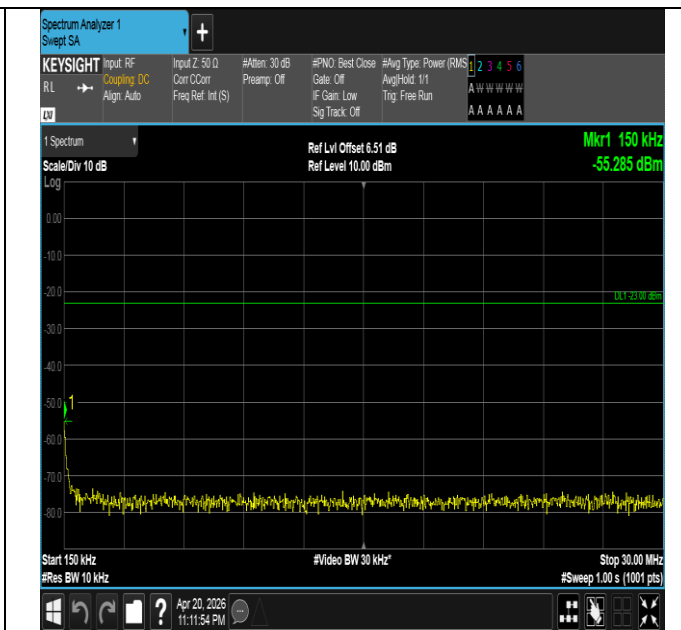
Band26(814-824)-3MHz-16QAM-26740-1RB#14-0.15~30-PAS S
