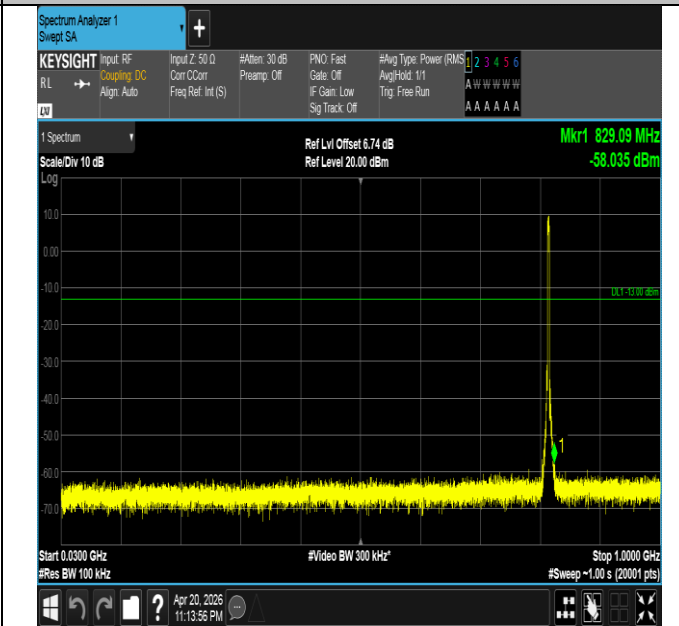
Band26(814-824)-3MHz-16QAM-26740-15RB#0-30~1000-PA SS
