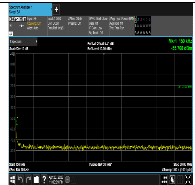
Band26(814-824)-3MHz-QPSK-26740-1RB#0-0.15~30-PASS
