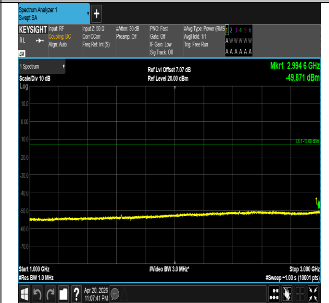
Band26(814-824)-3MHz-QPSK-26705-15RB#0-1000~3000-P ASS
