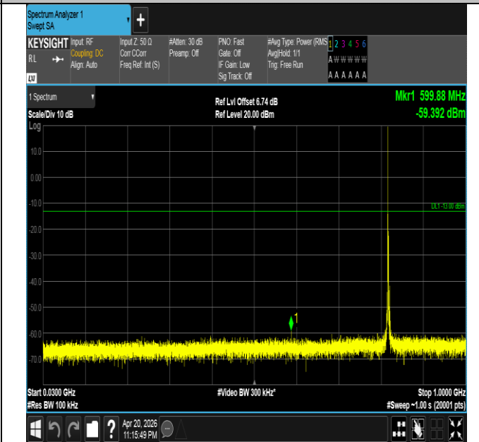
Band26(814-824)-3MHz-16QAM-26775-1RB#0-30~1000-PAS S
