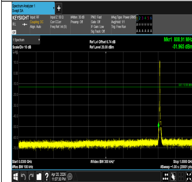
Band26(814-824)-3MHz-QPSK-26705-15RB#0-30~1000-PAS S
