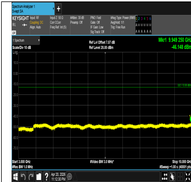
Band26(814-824)-3MHz-16QAM-26740-1RB#14-3000~10000 -PASS
