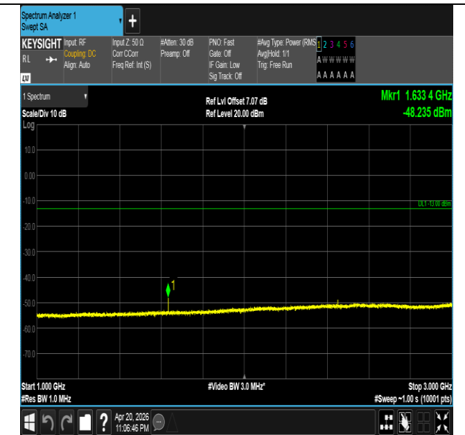
Band26(814-824)-3MHz-16QAM-26705-1RB#14-1000~3000- PASS
