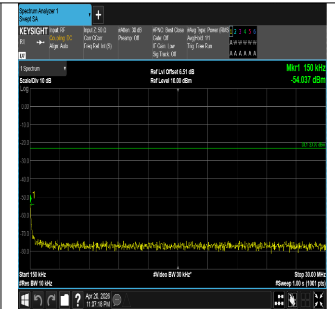
Band26(814-824)-3MHz-QPSK-26705-15RB#0-0.15~30-PAS S
