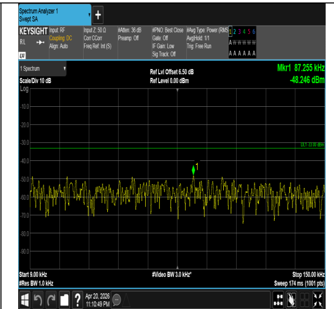
Band26(814-824)-3MHz-QPSK-26740-1RB#14-0.009~0.15-P ASS
