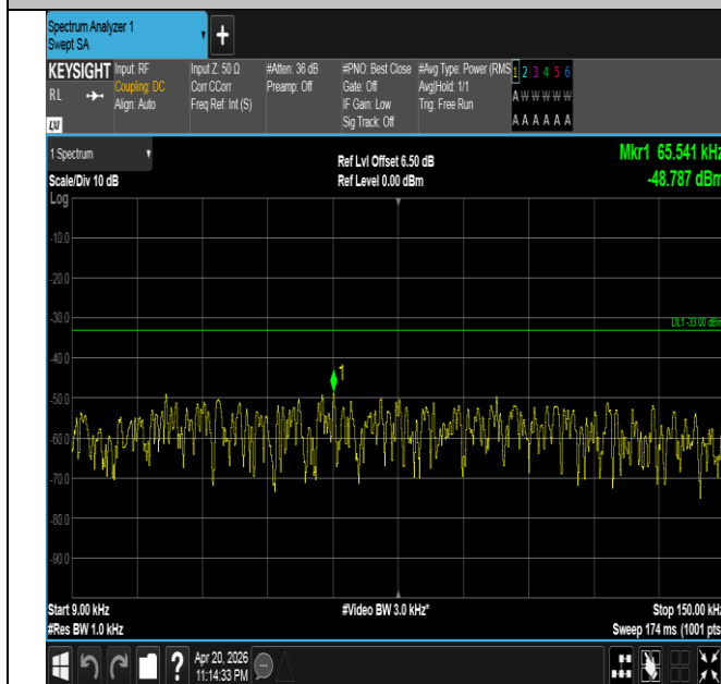
Band26(814-824)-3MHz-QPSK-26775-1RB#0-0.009~0.15-PA SS
