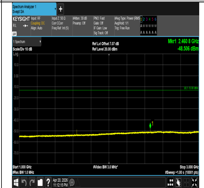
Band26(814-824)-3MHz-16QAM-26740-1RB#14-1000~3000- PASS
