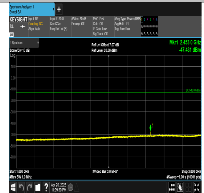
Band26(814-824)-3MHz-QPSK-26740-1RB#0-1000~3000-PA SS
