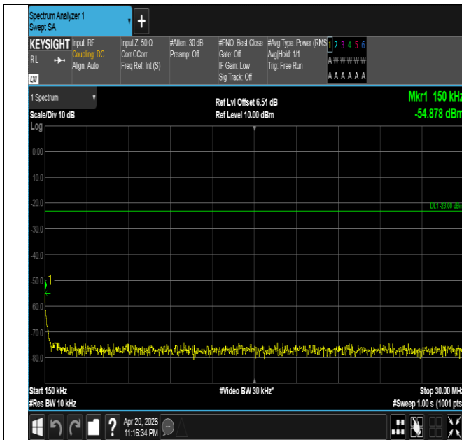
Band26(814-824)-3MHz-QPSK-26775-1RB#14-0.15~30-PAS
