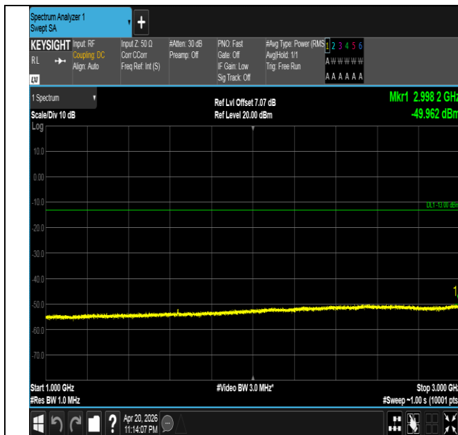
Band26(814-824)-3MHz-16QAM-26740-15RB#0-1000~3000- PASS
