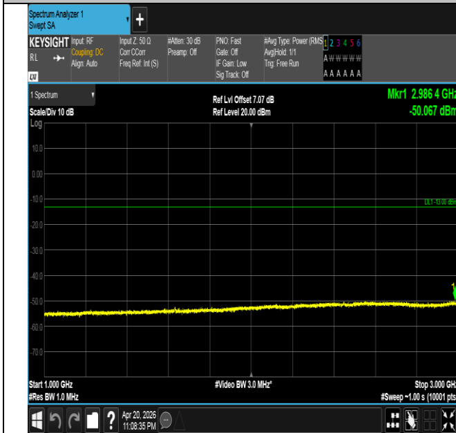
Band26(814-824)-3MHz-16QAM-26705-15RB#0-1000~3000-
