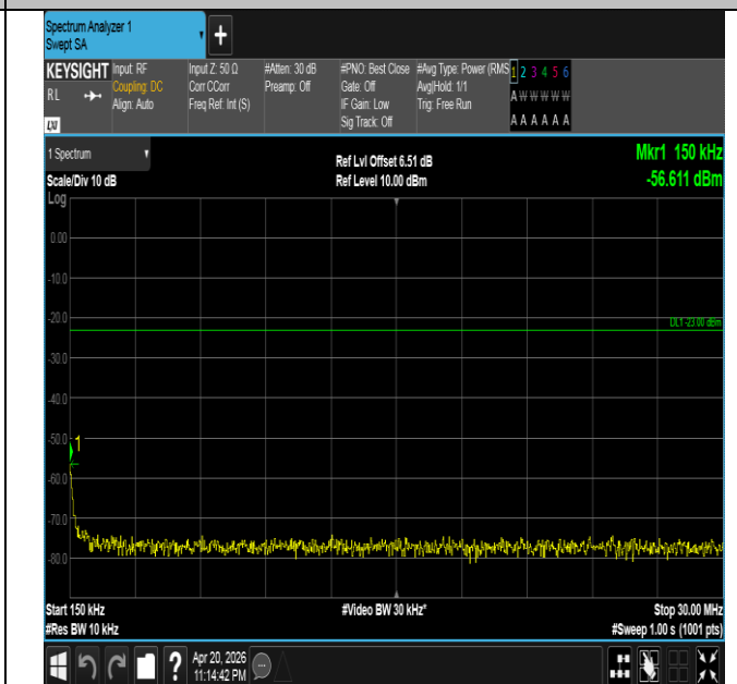
Band26(814-824)-3MHz-QPSK-26775-1RB#0-0.15~30-PASS
