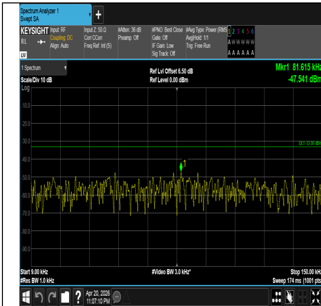
Band26(814-824)-3MHz-QPSK-26705-15RB#0-0.009~0.15-P ASS
