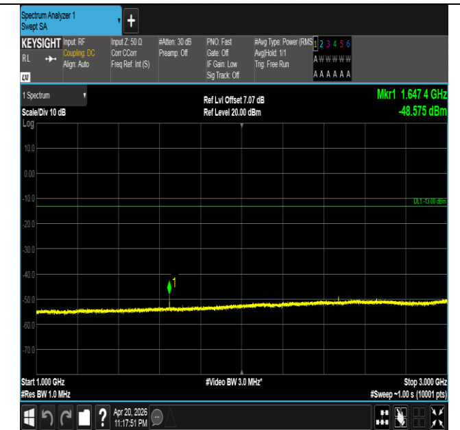
Band26(814-824)-3MHz-16QAM-26775-1RB#14-1000~3000- PASS
