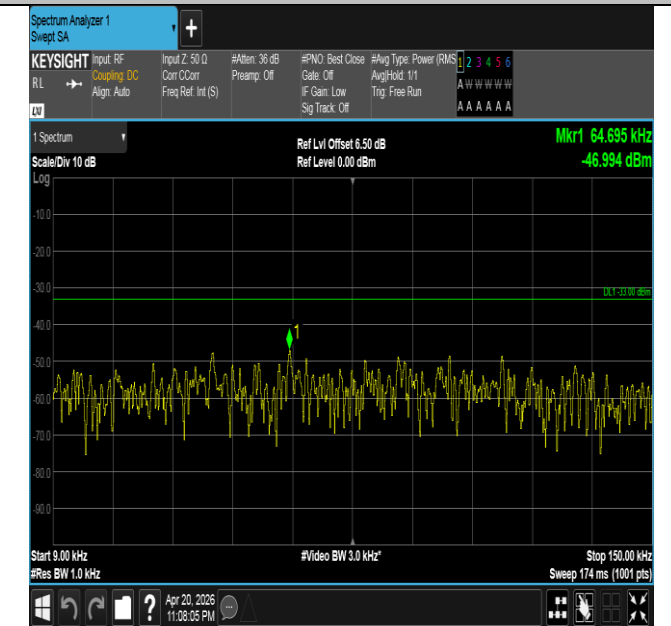
Band26(814-824)-3MHz-16QAM-26705-15RB#0-0.009~0.15- PASS
