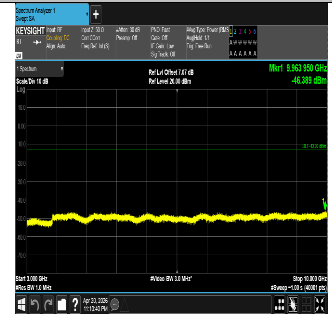
Band26(814-824)-3MHz-16QAM-26740-1RB#0-3000~10000-
