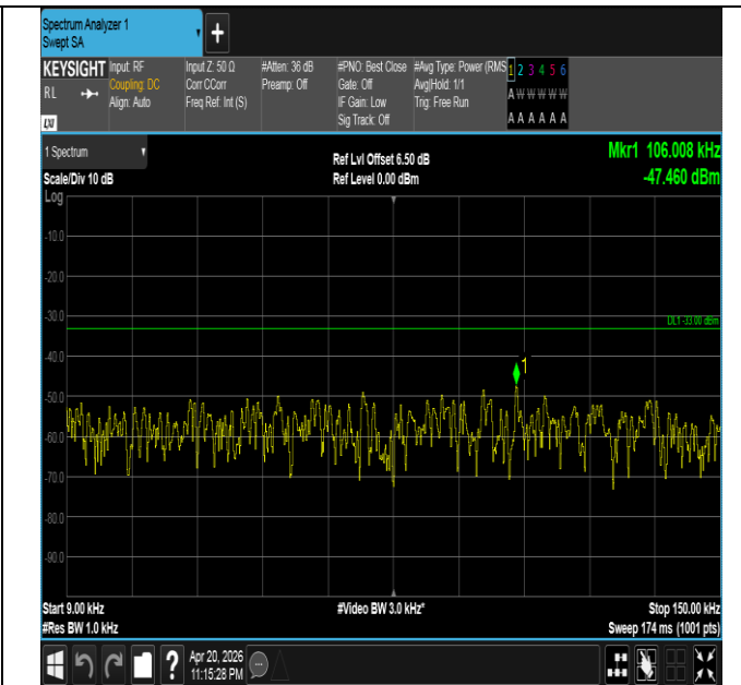
Band26(814-824)-3MHz-16QAM-26775-1RB#0-0.009~0.15-P ASS
