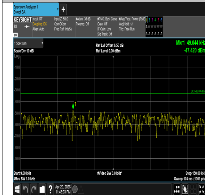
Band26(814-824)-5MHz-QPSK-26740-1RB#0-0.009~0.15-PA SS
