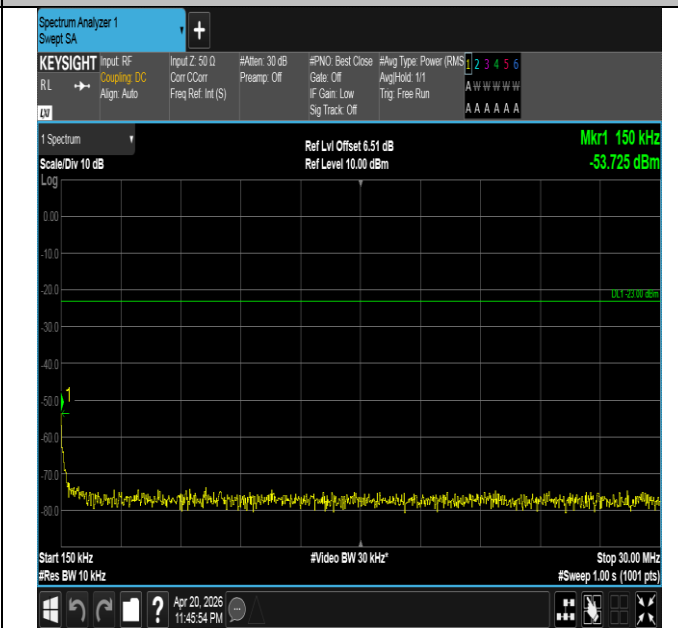
Band26(814-824)-5MHz-16QAM-26740-1RB#24-0.15~30-PAS S
