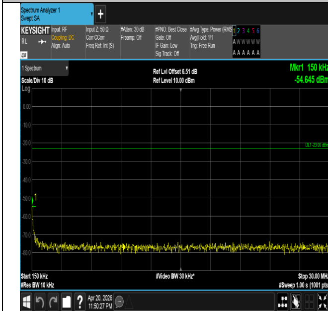
Band26(814-824)-5MHz-QPSK-26765-1RB#24-0.15~30-PAS S
