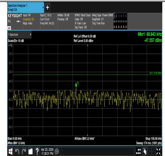
Band26(814-824)-5MHz-16QAM-26715-1RB#0-0.009~0.15-P
