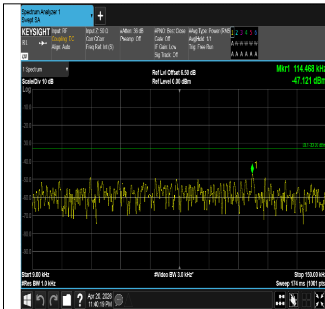
Band26(814-824)-5MHz-16QAM-26715-1RB#24-0.009~0.15- PASS
