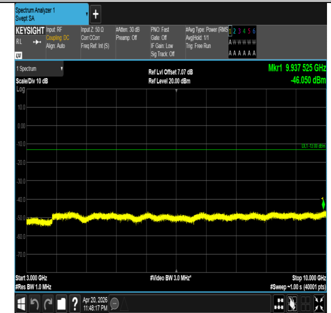
Band26(814-824)-5MHz-16QAM-26740-25RB#0-3000~10000
