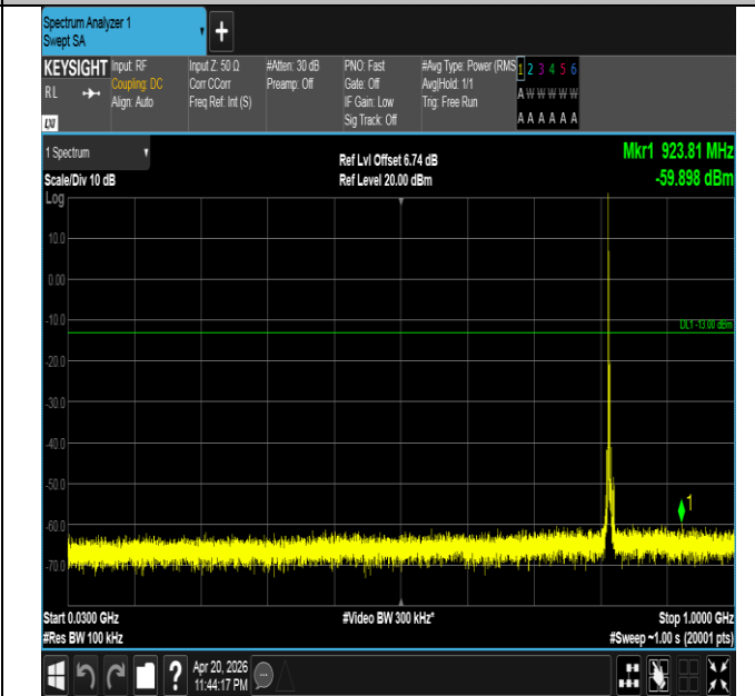
Band26(814-824)-5MHz-16QAM-26740-1RB#0-30~1000-PAS S
