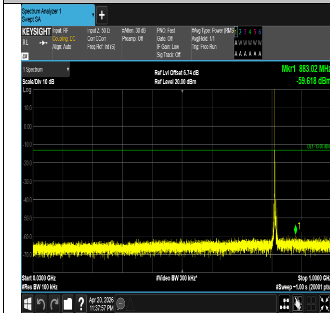
Band26(814-824)-5MHz-QPSK-26715-1RB#0-30~1000-PASS
