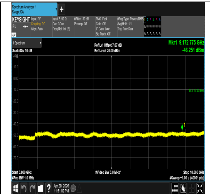
Band26(814-824)-5MHz-QPSK-26765-1RB#24-3000~10000-P ASS
