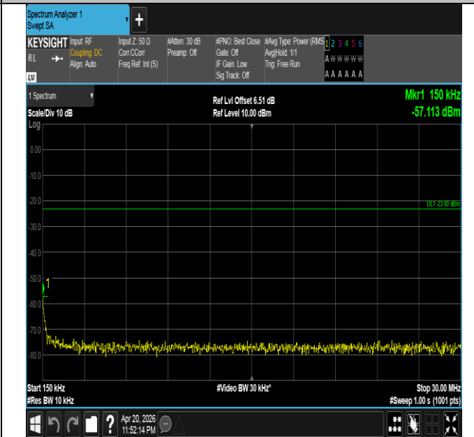
Band26(814-824)-5MHz-QPSK-26765-25RB#0-0.15~30-PAS S
