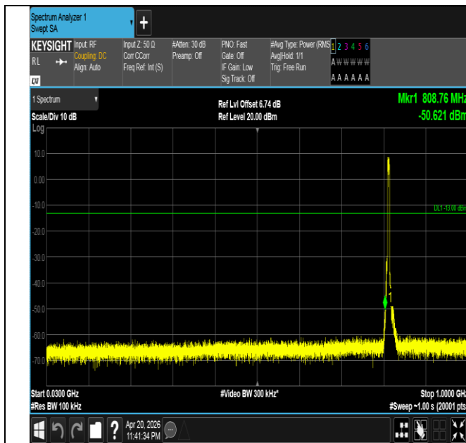
Band26(814-824)-5MHz-QPSK-26715-25RB#0-30~1000-PAS
