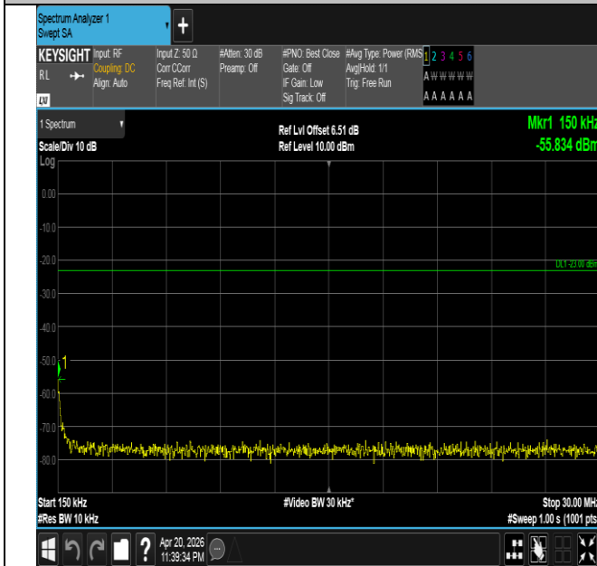
Band26(814-824)-5MHz-QPSK-26715-1RB#24-0.15~30-PAS S
