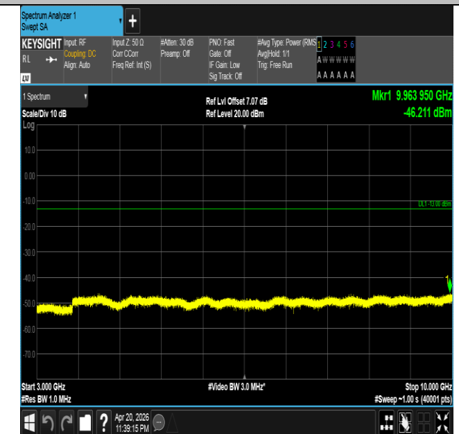
Band26(814-824)-5MHz-16QAM-26715-1RB#0-3000~10000-
