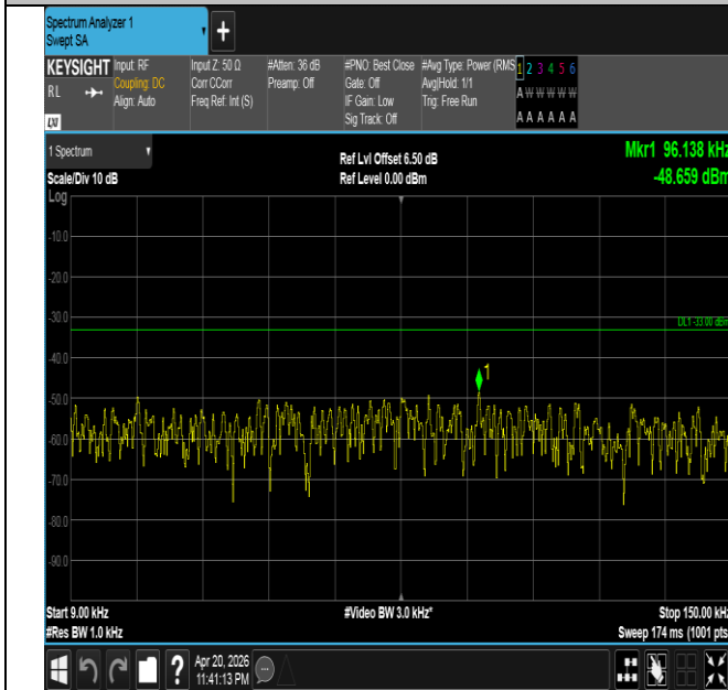
Band26(814-824)-5MHz-QPSK-26715-25RB#0-0.009~0.15-P ASS
