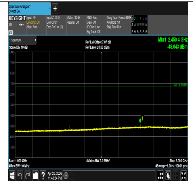
Band26(814-824)-5MHz-QPSK-26740-1RB#0-1000~3000-PA SS
