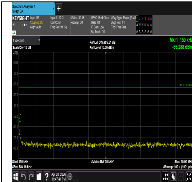
Band26(814-824)-5MHz-16QAM-26740-25RB#0-0.15~30-PA
