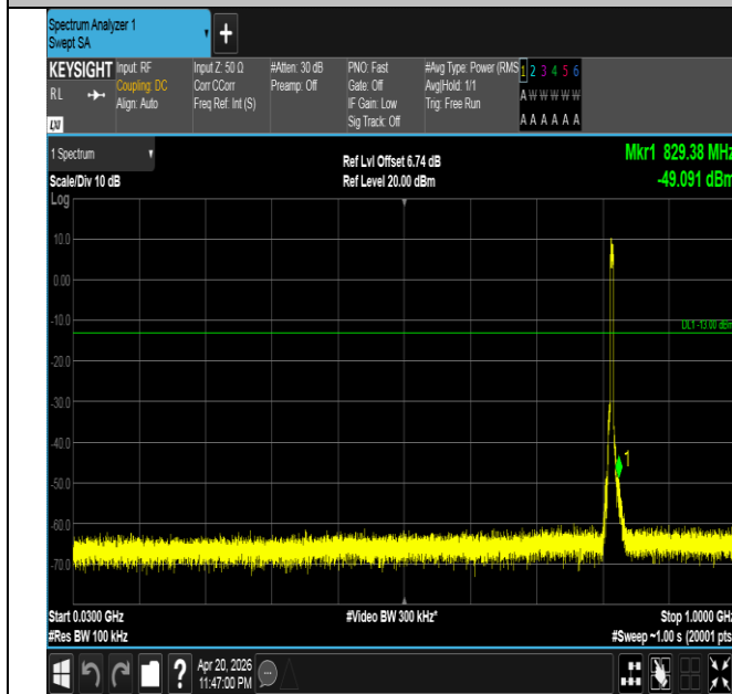
Band26(814-824)-5MHz-QPSK-26740-25RB#0-30~1000-PAS
