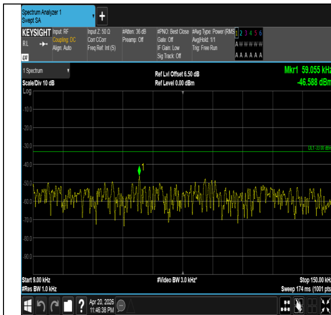
Band26(814-824)-5MHz-QPSK-26740-25RB#0-0.009~0.15-P
