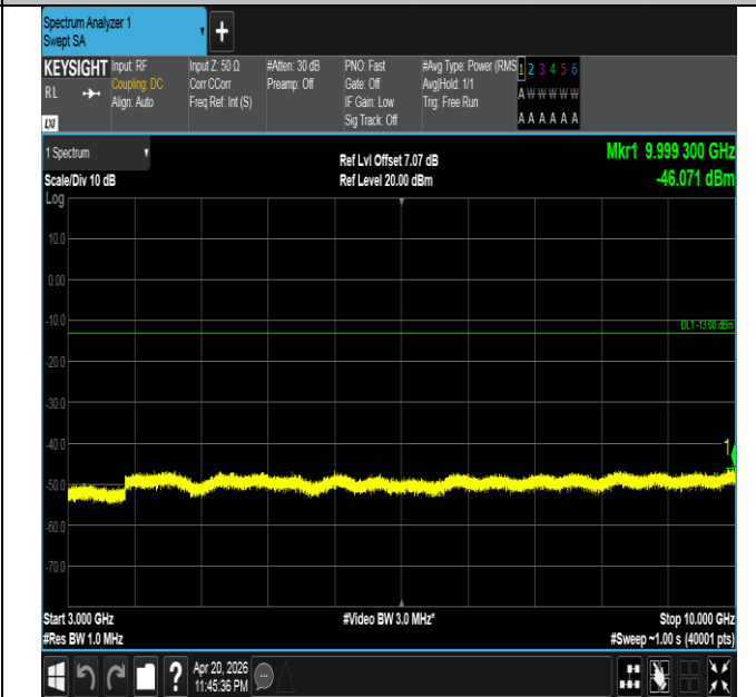
Band26(814-824)-5MHz-QPSK-26740-1RB#24-3000~10000-P
