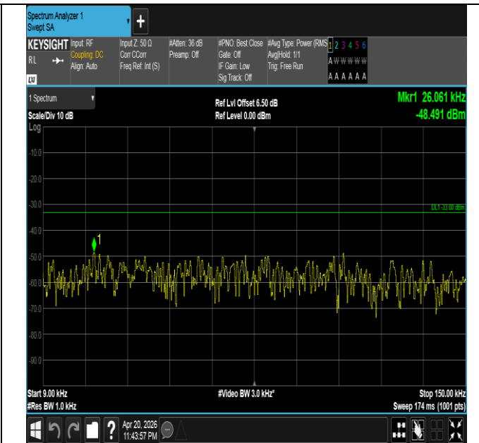
Band26(814-824)-5MHz-16QAM-26740-1RB#0-0.009~0.15-P ASS
