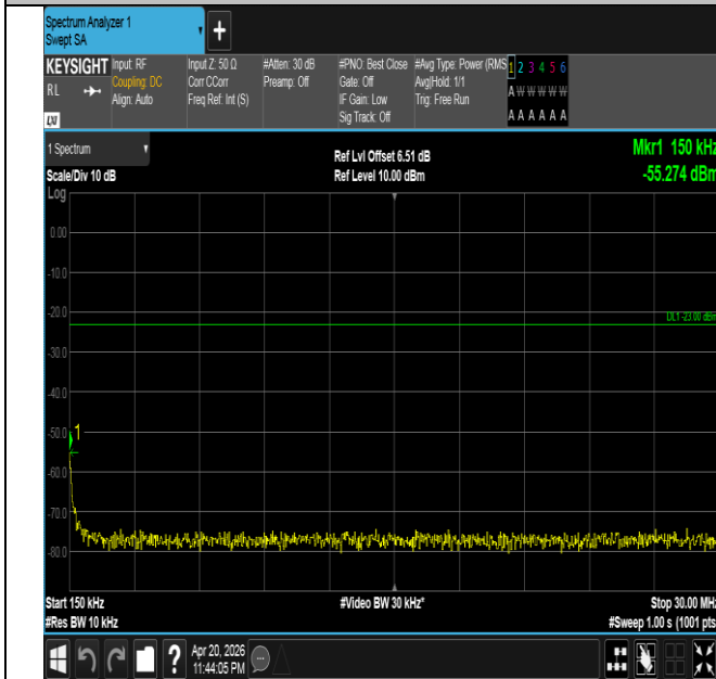
Band26(814-824)-5MHz-16QAM-26740-1RB#0-0.15~30-PAS S
