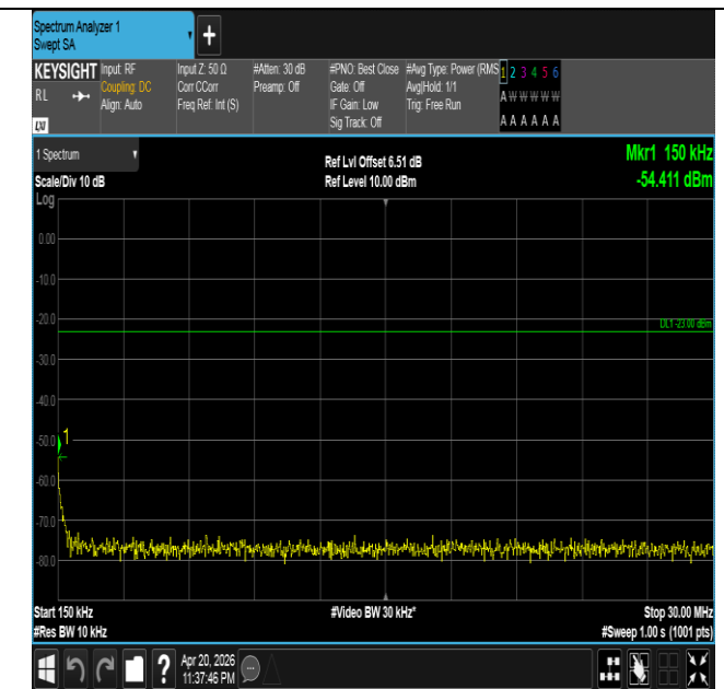
Band26(814-824)-5MHz-QPSK-26715-1RB#0-0.15~30-PASS
