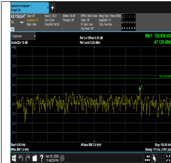
Band26(814-824)-5MHz-QPSK-26765-1RB#0-0.009~0.15-PA SS
