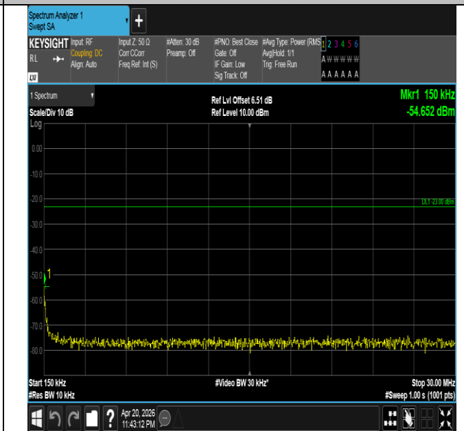
Band26(814-824)-5MHz-QPSK-26740-1RB#0-0.15~30-PASS
