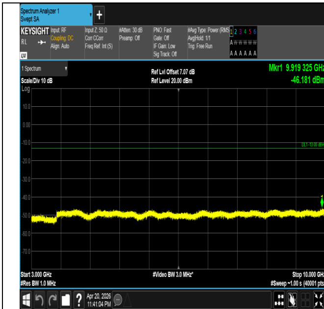
Band26(814-824)-5MHz-16QAM-26715-1RB#24-3000~10000 -PASS
