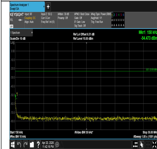
Band26(814-824)-5MHz-16QAM-26715-25RB#0-0.15~30-PA SS
