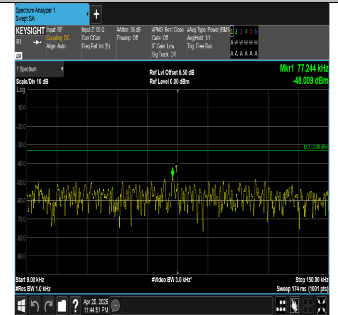
Band26(814-824)-5MHz-QPSK-26740-1RB#24-0.009~0.15-P ASS
