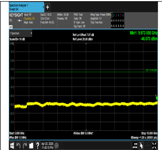
Band26(814-824)-5MHz-QPSK-26715-1RB#24-3000~10000-P ASS
