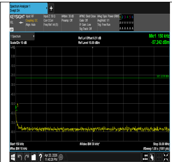
Band26(814-824)-5MHz-16QAM-26715-1RB#24-0.15~30-PAS S
