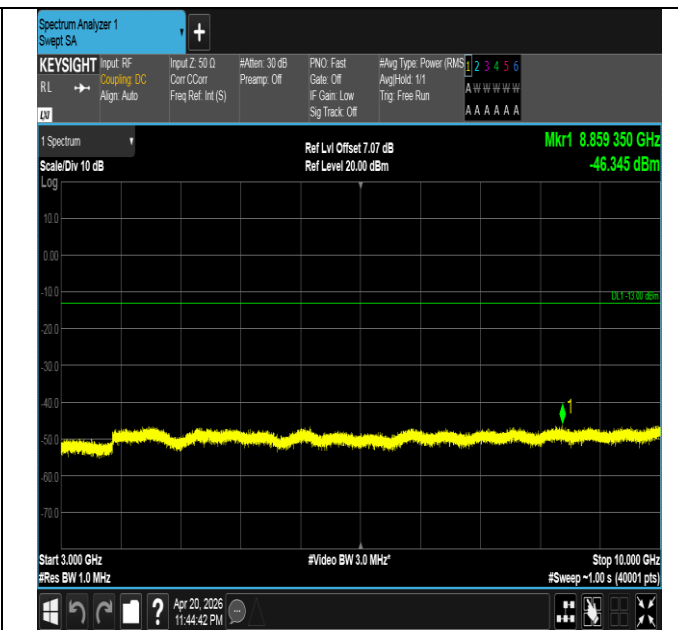
Band26(814-824)-5MHz-16QAM-26740-1RB#0-3000~10000- PASS
