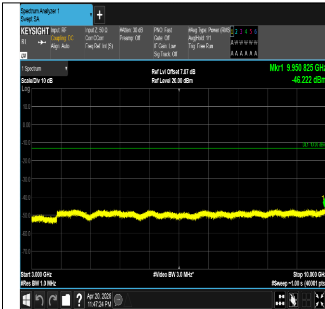
Band26(814-824)-5MHz-QPSK-26740-25RB#0-3000~10000- PASS
