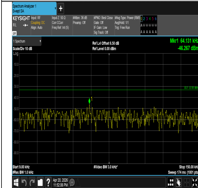
Band26(814-824)-5MHz-QPSK-26765-25RB#0-0.009~0.15-P ASS
