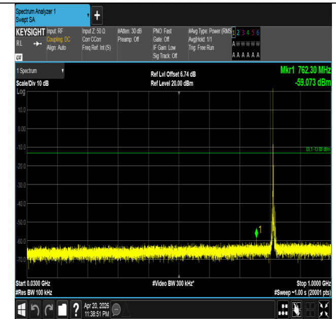
Band26(814-824)-5MHz-16QAM-26715-1RB#0-30~1000-PAS
