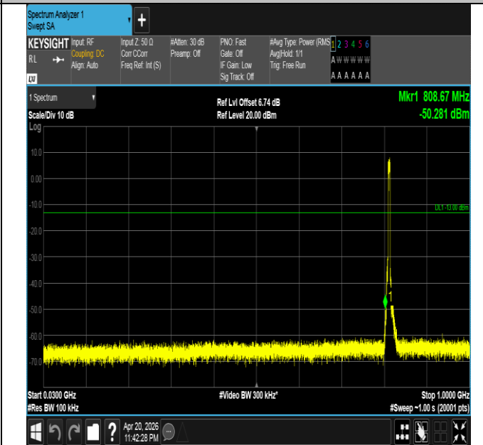
Band26(814-824)-5MHz-16QAM-26715-25RB#0-30~1000-PA SS
