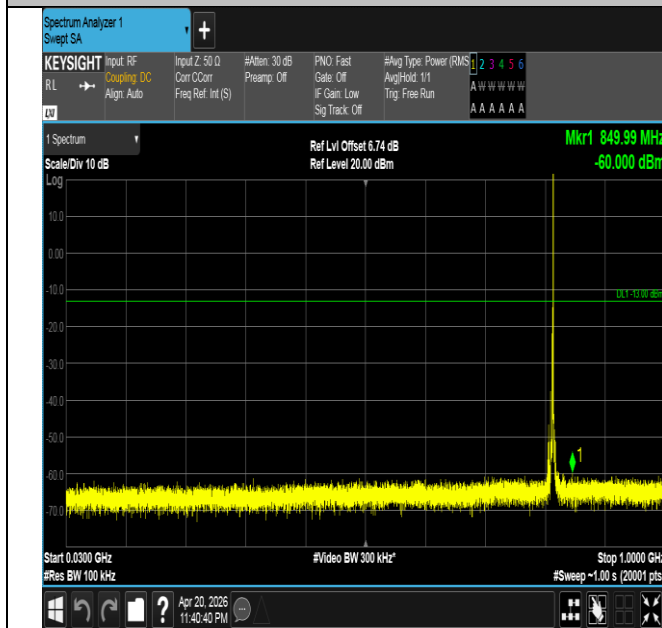
Band26(814-824)-5MHz-16QAM-26715-1RB#24-30~1000-PA SS
