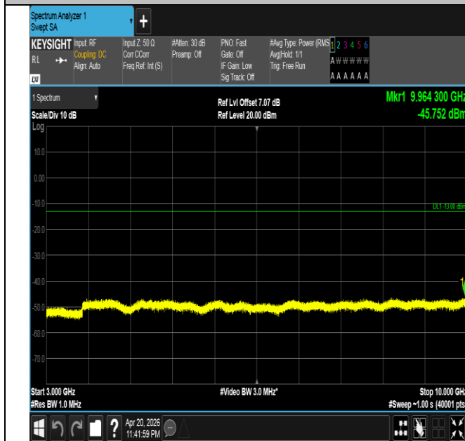
Band26(814-824)-5MHz-QPSK-26715-25RB#0-3000~10000-
