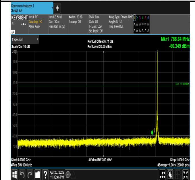
Band26(814-824)-5MHz-QPSK-26715-1RB#24-30~1000-PAS S
