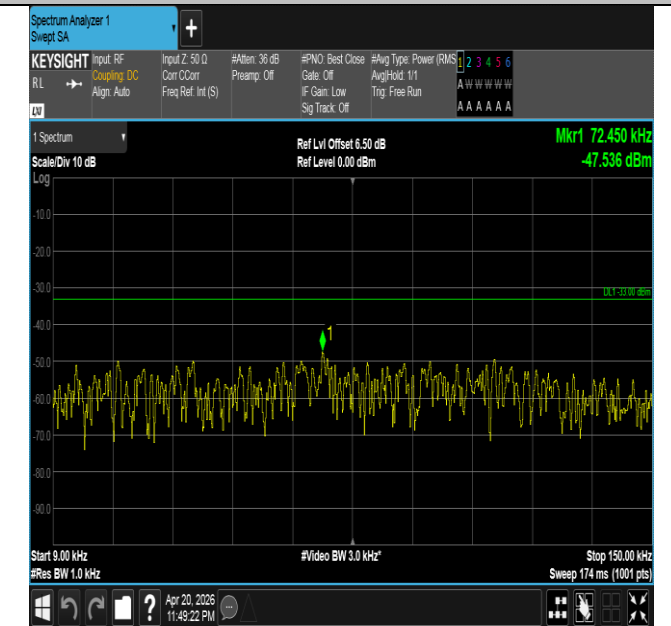
Band26(814-824)-5MHz-16QAM-26765-1RB#0-0.009~0.15-P
