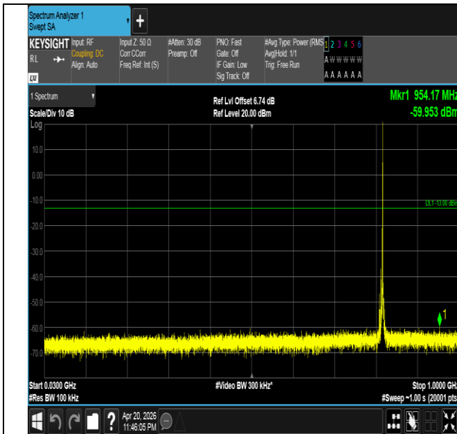
Band26(814-824)-5MHz-16QAM-26740-1RB#24-30~1000-PA SS
