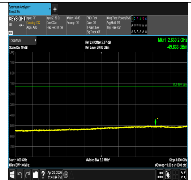
Band26(814-824)-5MHz-QPSK-26715-25RB#0-1000~3000-P
