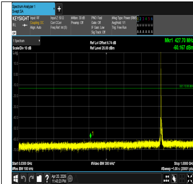
Band26(814-824)-5MHz-QPSK-26740-1RB#0-30~1000-PASS
