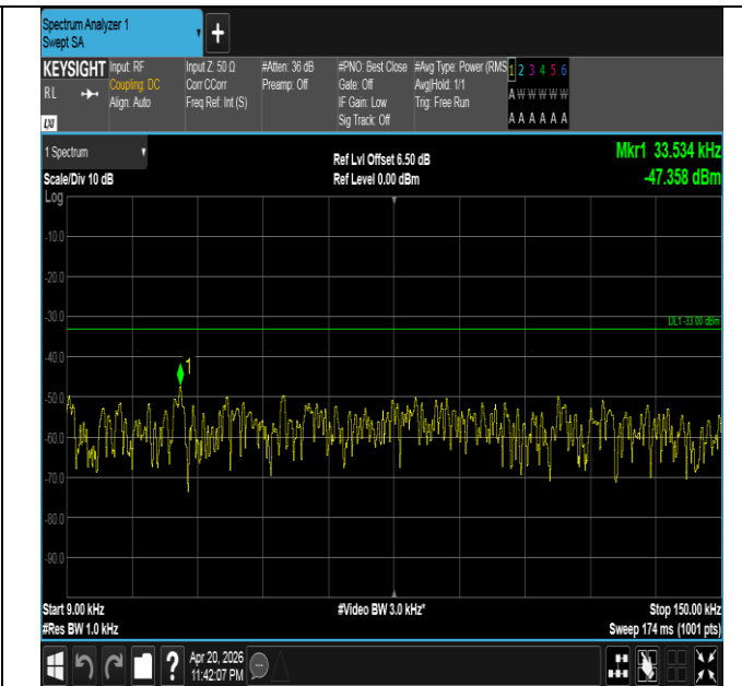
Band26(814-824)-5MHz-16QAM-26715-25RB#0-0.009~0.15- PASS
