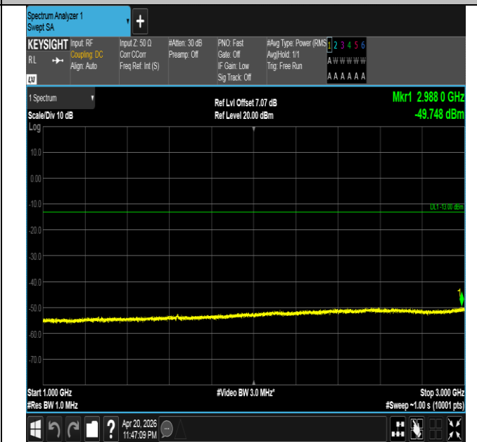
Band26(814-824)-5MHz-QPSK-26740-25RB#0-1000~3000-P
