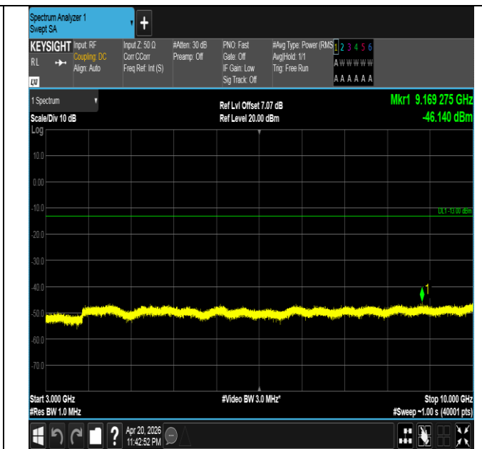
Band26(814-824)-5MHz-16QAM-26715-25RB#0-3000~10000 -PASS
