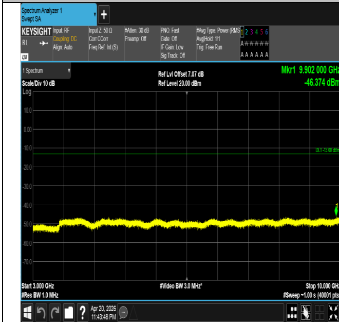
Band26(814-824)-5MHz-QPSK-26740-1RB#0-3000~10000-P ASS
