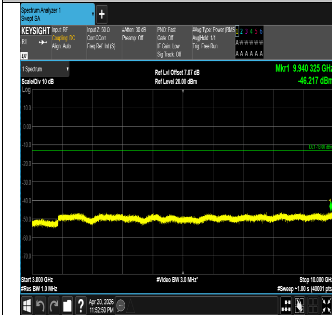
Band26(814-824)-5MHz-QPSK-26765-25RB#0-3000~10000-
