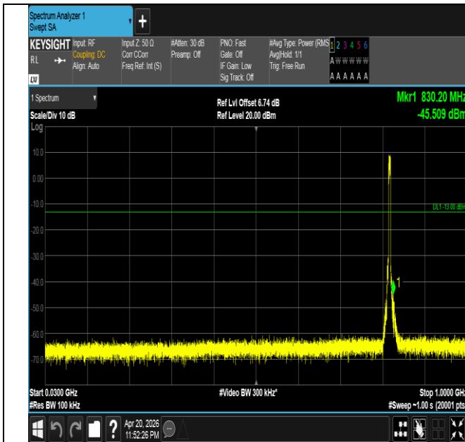
Band26(814-824)-5MHz-QPSK-26765-25RB#0-30~1000-PAS
