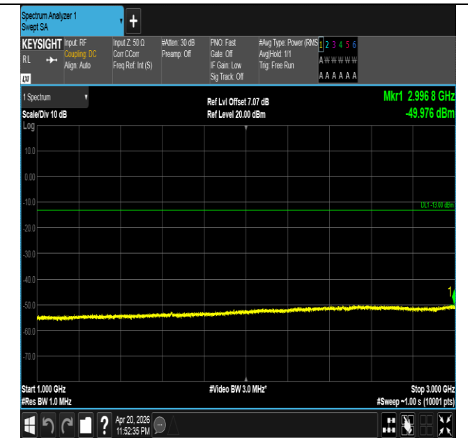
Band26(814-824)-5MHz-QPSK-26765-25RB#0-1000~3000-P
