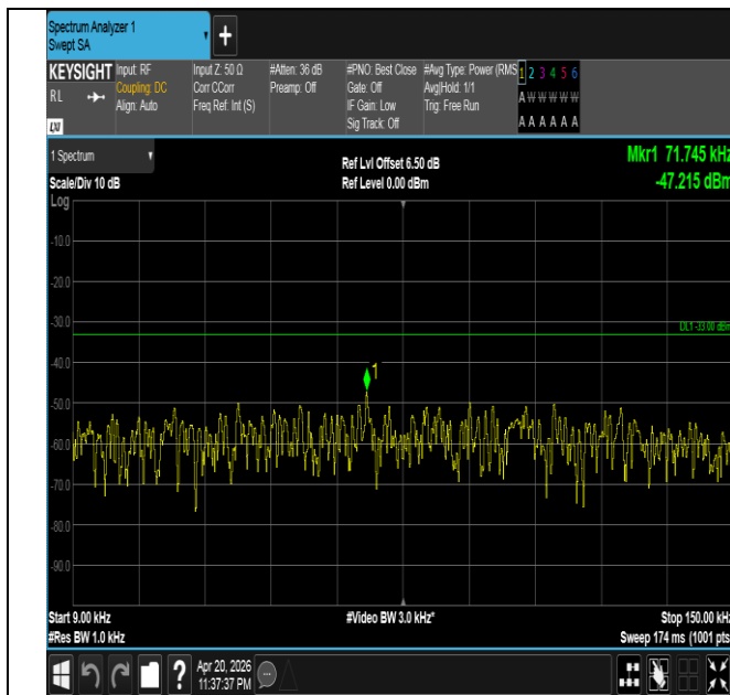
Band26(814-824)-5MHz-QPSK-26715-1RB#0-0.009~0.15-PA SS
