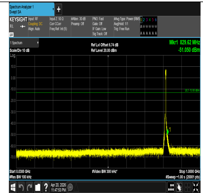
Band26(814-824)-5MHz-16QAM-26740-25RB#0-30~1000-PA
