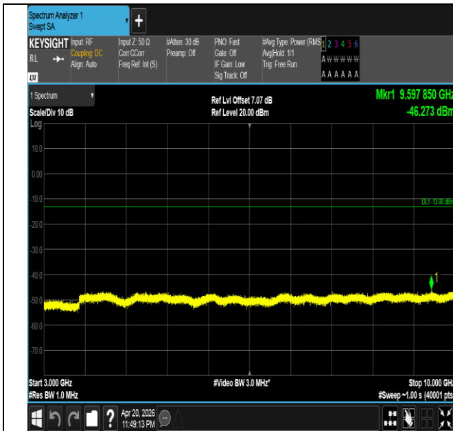
Band26(814-824)-5MHz-QPSK-26765-1RB#0-3000~10000-P ASS
