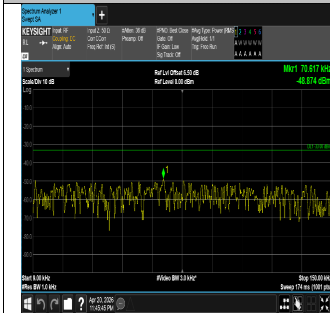
Band26(814-824)-5MHz-16QAM-26740-1RB#24-0.009~0.15- PASS
