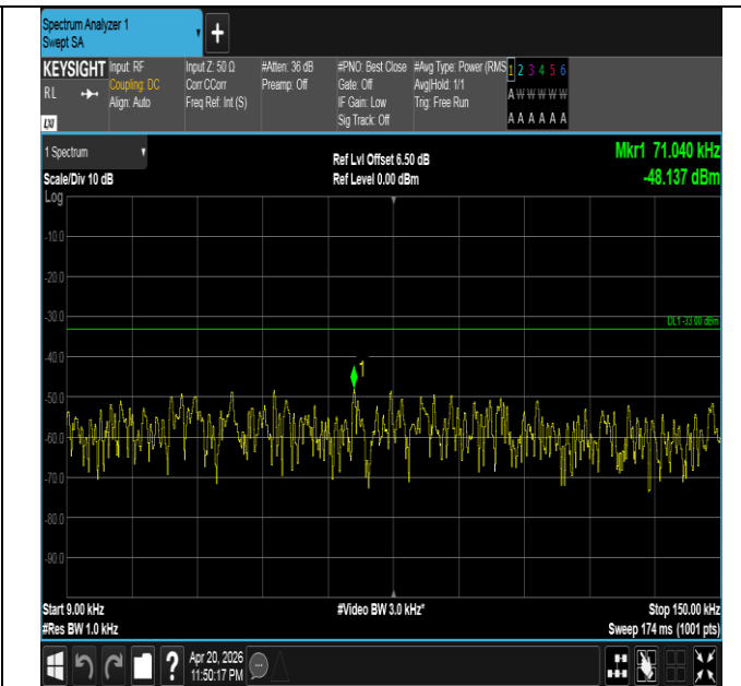
Band26(814-824)-5MHz-QPSK-26765-1RB#24-0.009~0.15-P ASS
