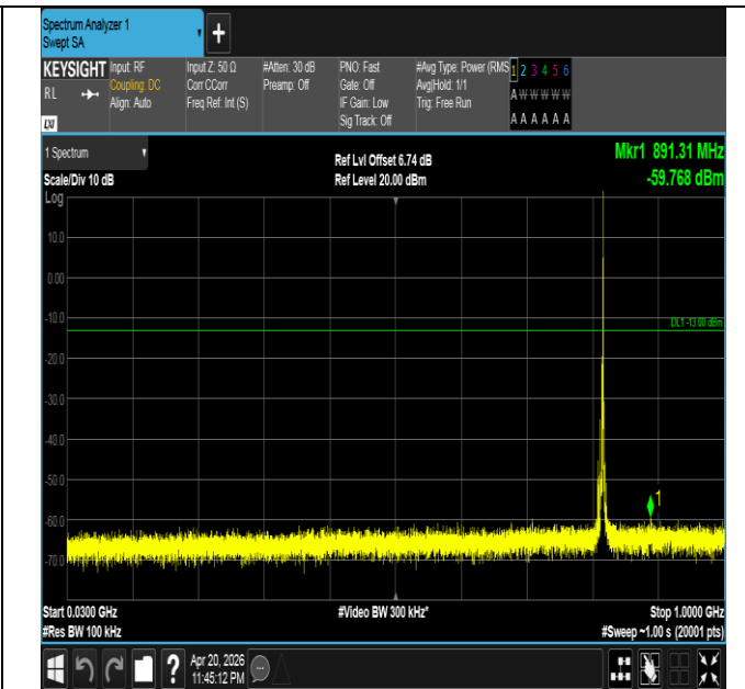
Band26(814-824)-5MHz-QPSK-26740-1RB#24-30~1000-PAS
