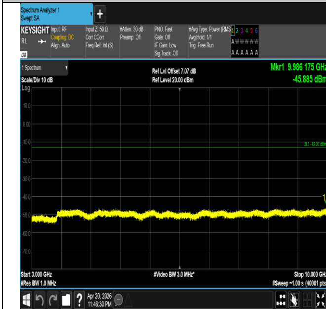
Band26(814-824)-5MHz-16QAM-26740-1RB#24-3000~10000 -PASS
