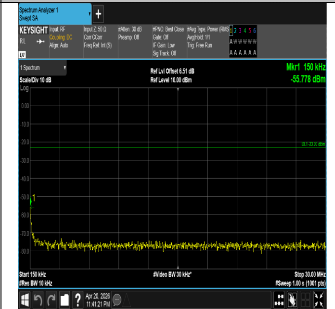
Band26(814-824)-5MHz-QPSK-26715-25RB#0-0.15~30-PAS S
