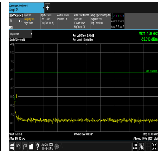
Band26(814-824)-5MHz-QPSK-26740-25RB#0-0.15~30-PAS
