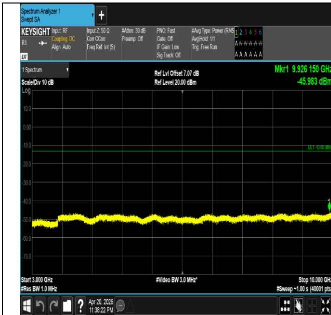
Band26(814-824)-5MHz-QPSK-26715-1RB#0-3000~10000-P ASS
