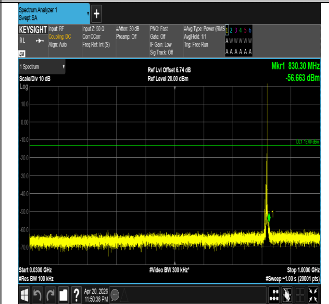
Band26(814-824)-5MHz-QPSK-26765-1RB#24-30~1000-PAS S
