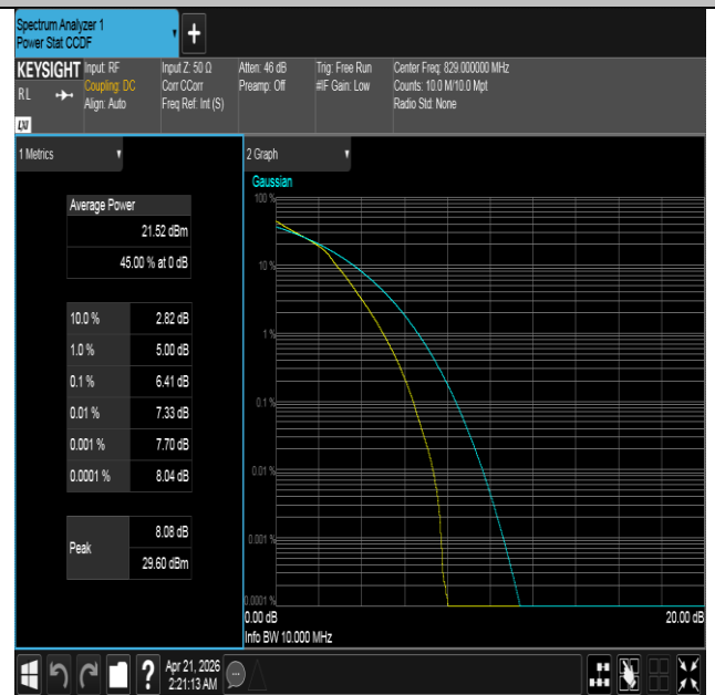
Band26(824-849)-10MHz-16QAM-26840-50RB#0-PASS
