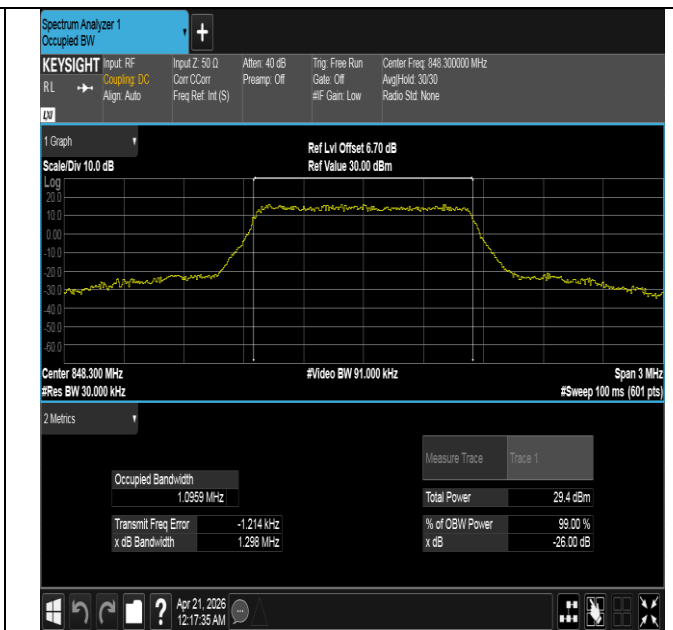
Band26(824-849)-1.4MHz-16QAM-27033-6RB#0-PASS
