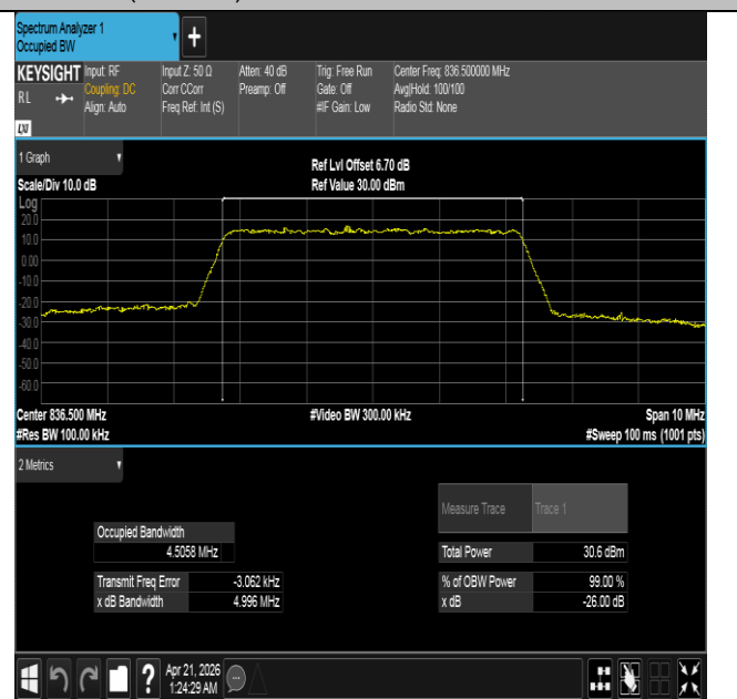
Band26(824-849)-5MHz-16QAM-26915-25RB#0-PASS
