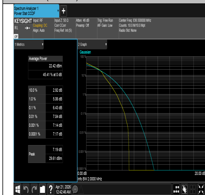
Band26(824-849)-1.4MHz-16QAM-26915-1RB#0-PASS
