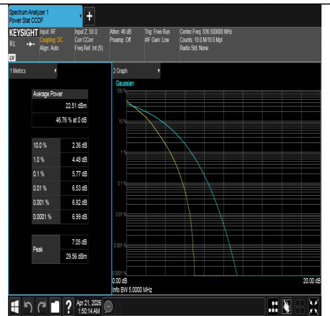
Band26(824-849)-5MHz-QPSK-26915-25RB#0-PASS
