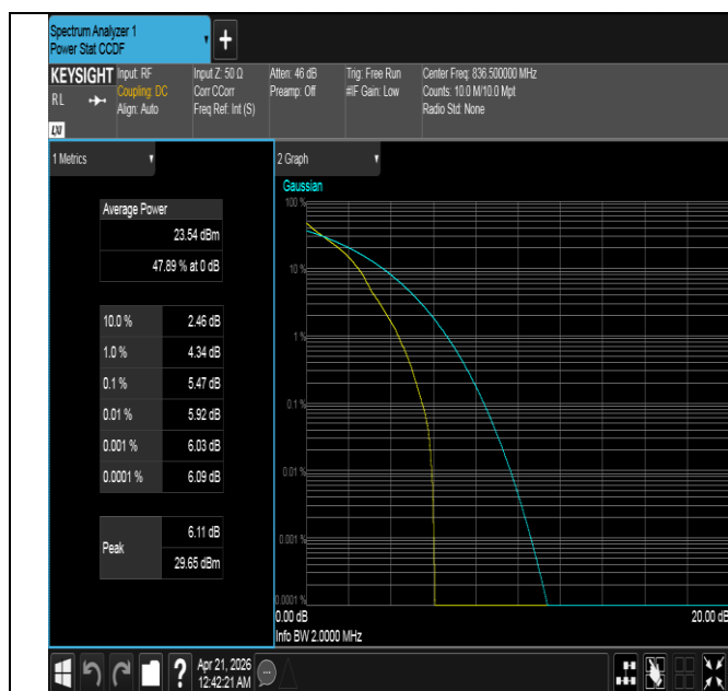
Band26(824-849)-1.4MHz-QPSK-26915-1RB#0-PASS
