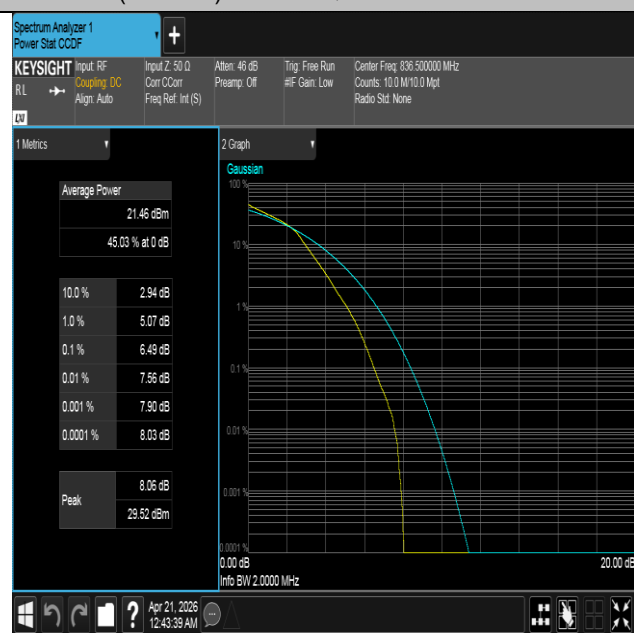
Band26(824-849)-1.4MHz-16QAM-26915-6RB#0-PASS
