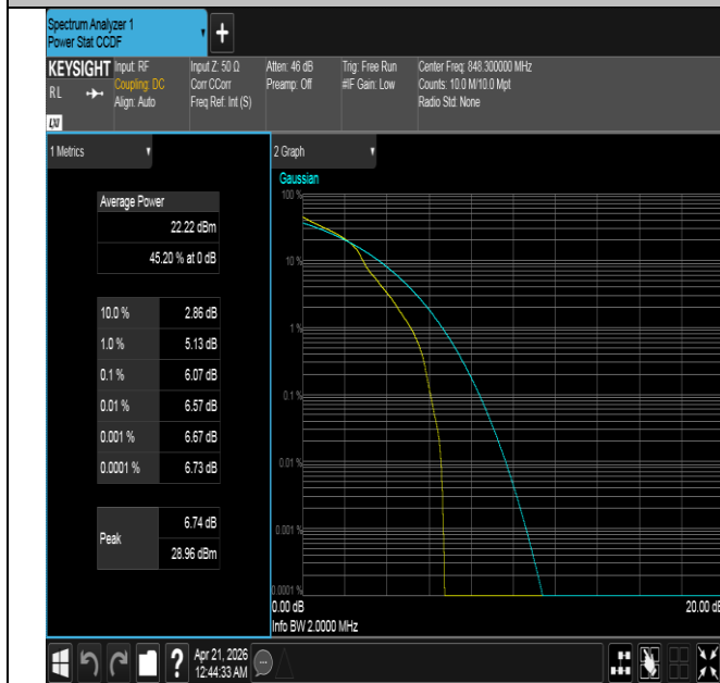
Band26(824-849)-1.4MHz-16QAM-27033-1RB#0-PASS
