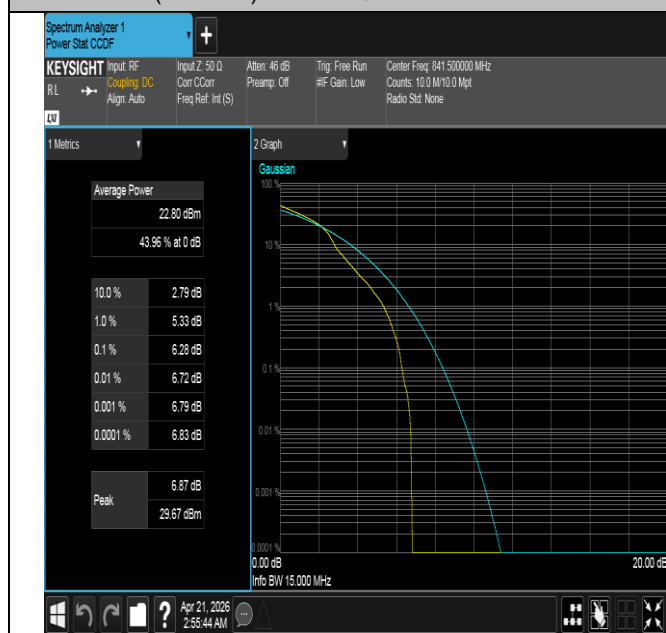
Band26(824-849)-15MHz-16QAM-26965-1RB#0-PASS
