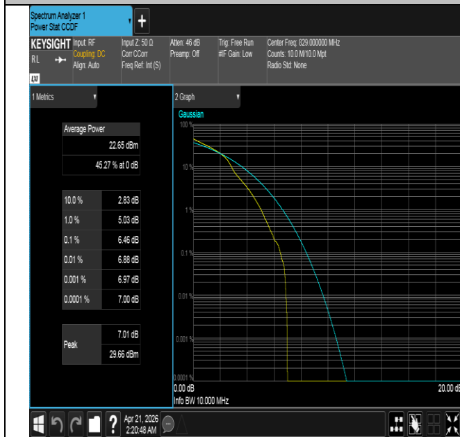
Band26(824-849)-10MHz-16QAM-26840-1RB#0-PASS
