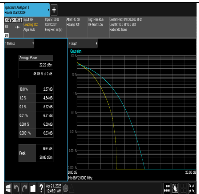
Band26(824-849)-1.4MHz-QPSK-27033-6RB#0-PASS
