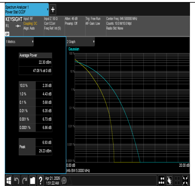
Band26(824-849)-5MHz-QPSK-27015-25RB#0-PASS
