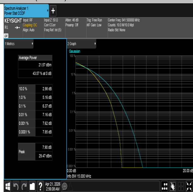
Band26(824-849)-15MHz-16QAM-26965-75RB#0-PASS
