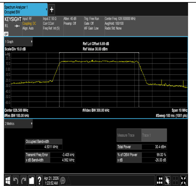
Band26(824-849)-5MHz-16QAM-26815-25RB#0-PASS
