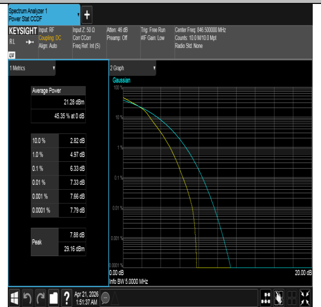
Band26(824-849)-5MHz-16QAM-27015-25RB#0-PASS
