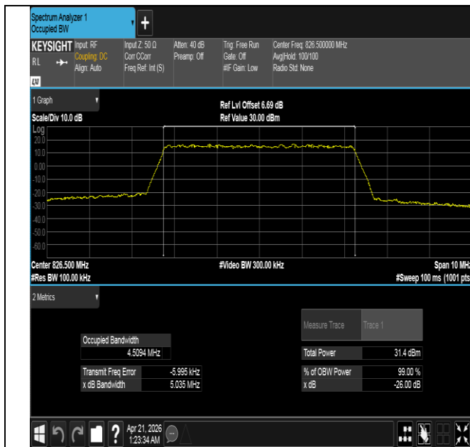
Band26(824-849)-5MHz-QPSK-26815-25RB#0-PASS
