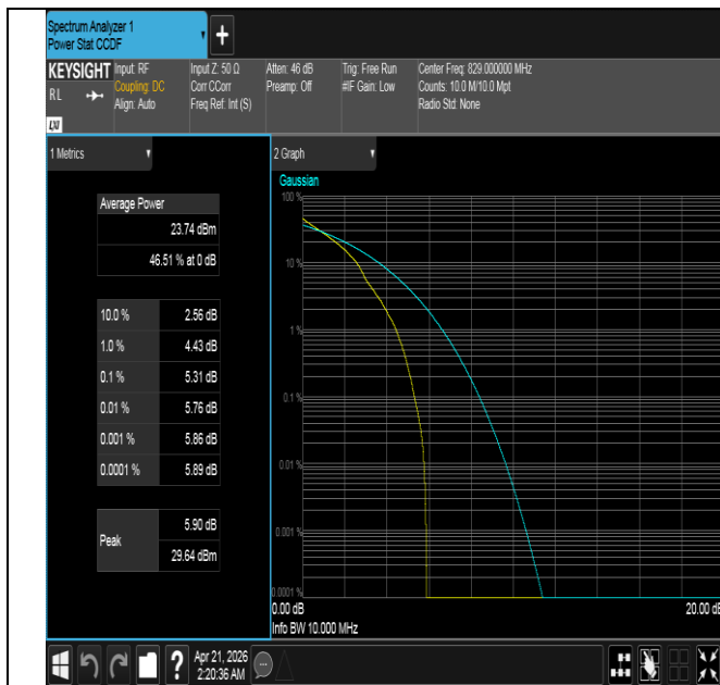
Band26(824-849)-10MHz-QPSK-26840-1RB#0-PASS
