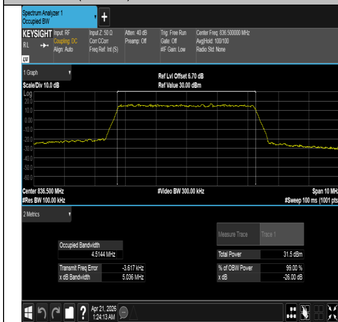
Band26(824-849)-5MHz-QPSK-26915-25RB#0-PASS
