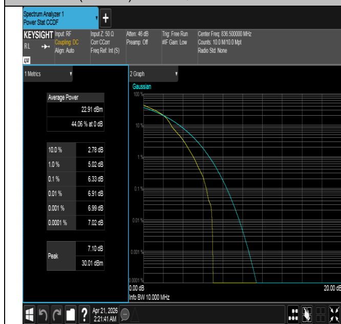
Band26(824-849)-10MHz-16QAM-26915-1RB#0-PASS
