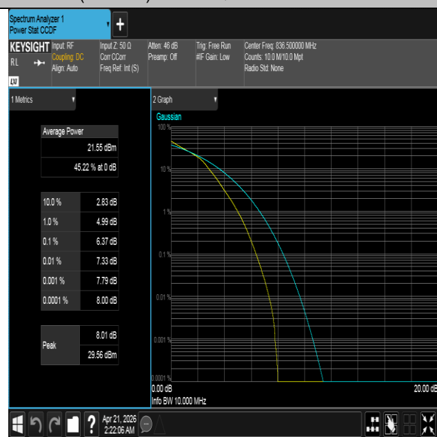
Band26(824-849)-10MHz-16QAM-26915-50RB#0-PASS
