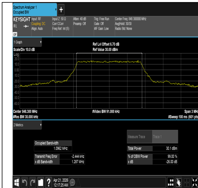
Band26(824-849)-1.4MHz-QPSK-27033-6RB#0-PASS
