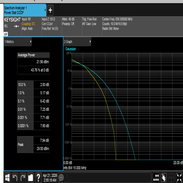
Band26(824-849)-15MHz-16QAM-26915-75RB#0-PASS
