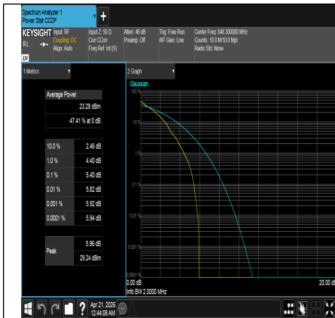
Band26(824-849)-1.4MHz-QPSK-27033-1RB#0-PASS
