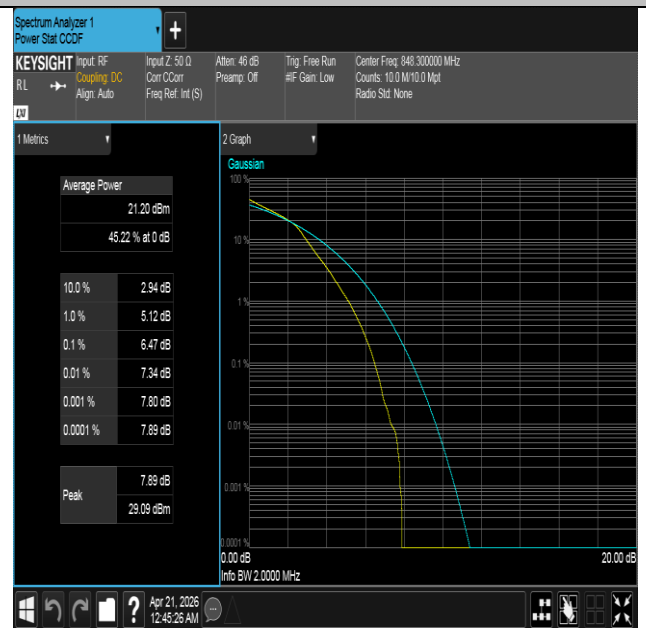
Band26(824-849)-1.4MHz-16QAM-27033-6RB#0-PASS
