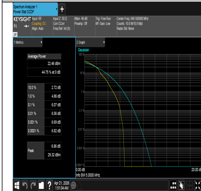
Band26(824-849)-5MHz-16QAM-27015-1RB#0-PASS
