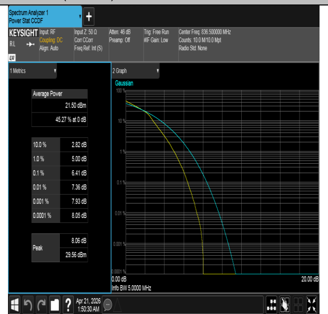
Band26(824-849)-5MHz-16QAM-26915-25RB#0-PASS
