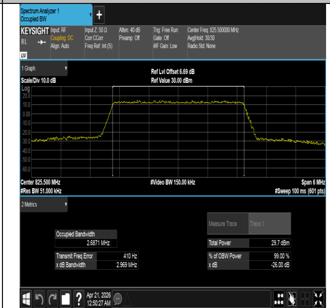
Band26(824-849)-3MHz-16QAM-26805-15RB#0-PASS
