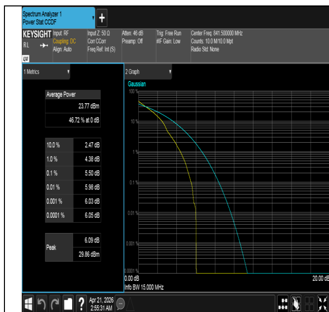
Band26(824-849)-15MHz-QPSK-26965-1RB#0-PASS
