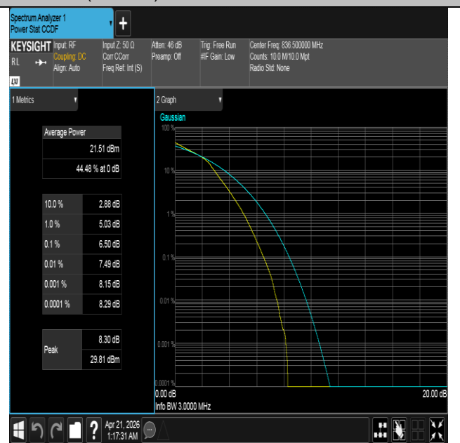
Band26(824-849)-3MHz-16QAM-26915-15RB#0-PASS
