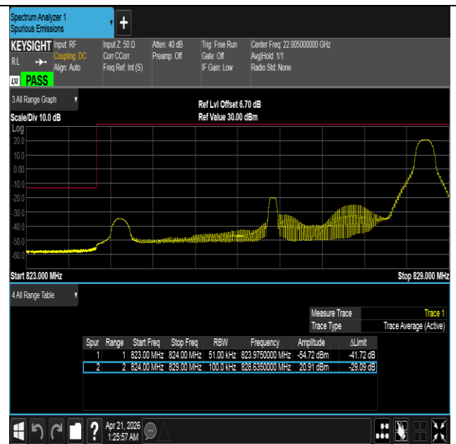
Band26(824-849)-5MHz-QPSK-26815-1RB#24-PASS
