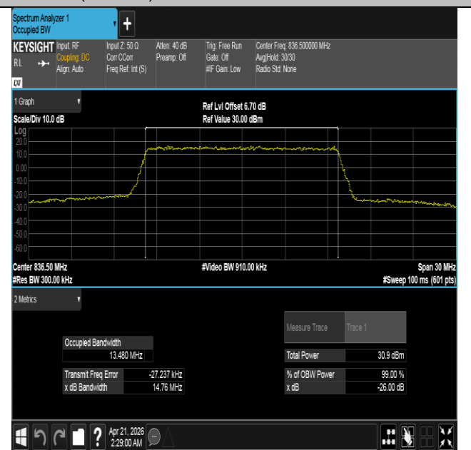
Band26(824-849)-15MHz-16QAM-26915-75RB#0-PASS
