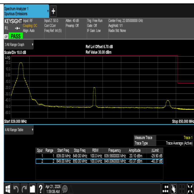
Band26(824-849)-10MHz-16QAM-26990-1RB#0-PASS
