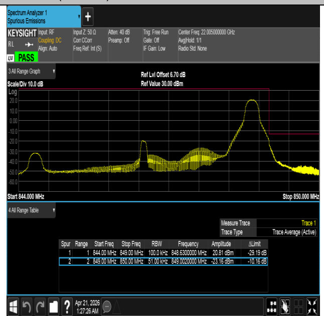
Band26(824-849)-5MHz-QPSK-27015-1RB#24-PASS
