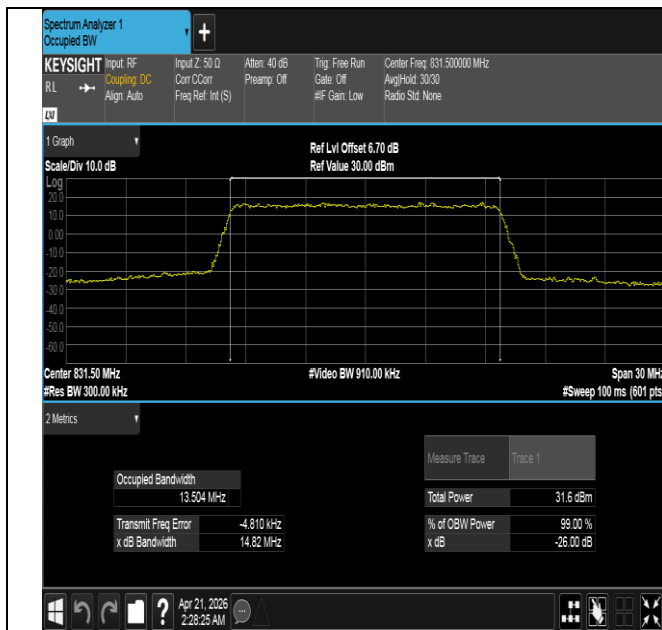
Band26(824-849)-15MHz-QPSK-26865-75RB#0-PASS
