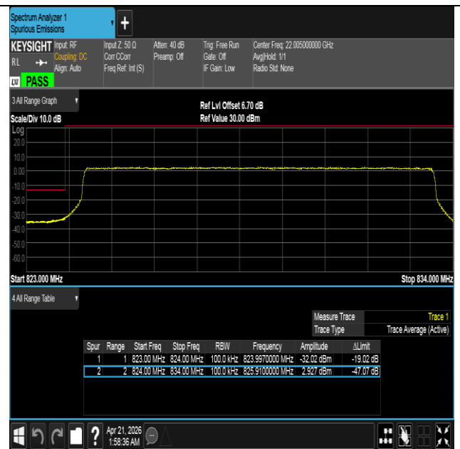
Band26(824-849)-10MHz-16QAM-26840-50RB#0-PASS
