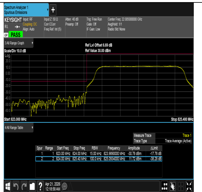
Band26(824-849)-1.4MHz-16QAM-26797-6RB#0-PASS
