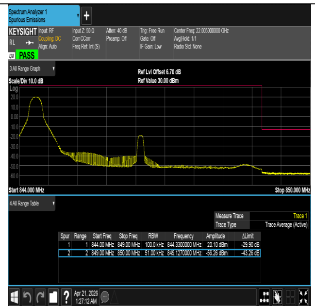
Band26(824-849)-5MHz-16QAM-27015-1RB#0-PASS
