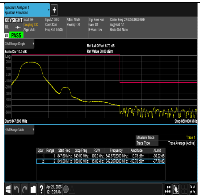
Band26(824-849)-1.4MHz-16QAM-27033-1RB#0-PASS
