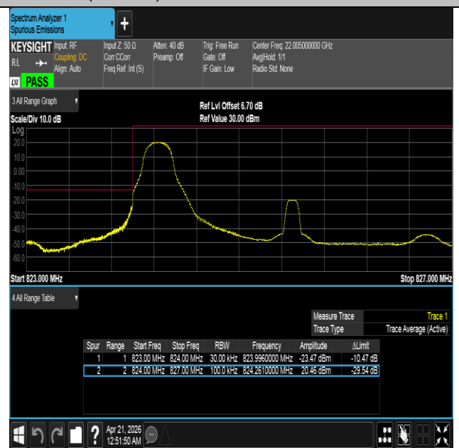
Band26(824-849)-3MHz-QPSK-26805-16QAM-26805-1RB#0-PASS
