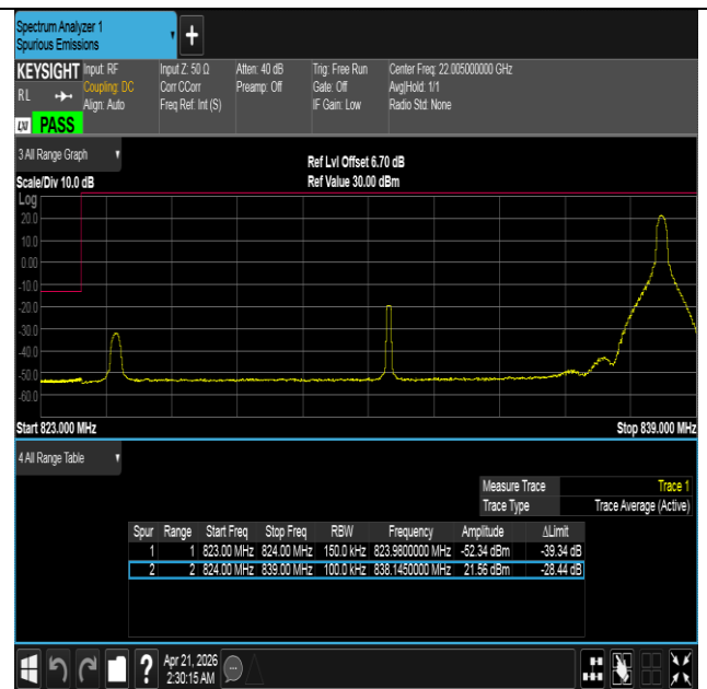
Band26(824-849)-15MHz-QPSK-26865-1RB#74-PASS
