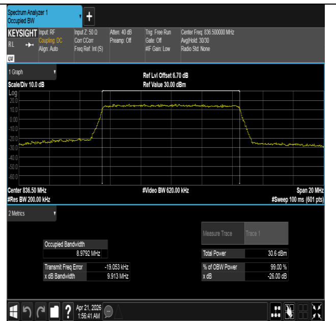
Band26(824-849)-10MHz-16QAM-26915-50RB#0-PASS
