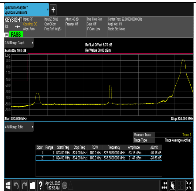
Band26(824-849)-10MHz-QPSK-26840-1RB#49-PASS
