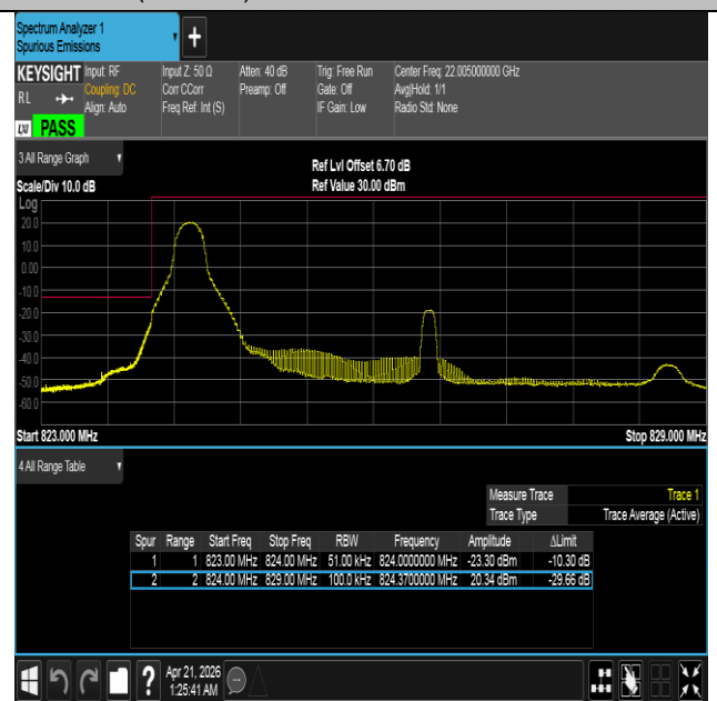
Band26(824-849)-5MHz-16QAM-26815-1RB#0-PASS
