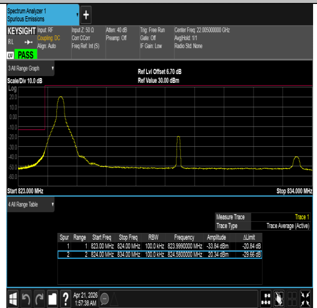
Band26(824-849)-10MHz-16QAM-26840-1RB#0-PASS
