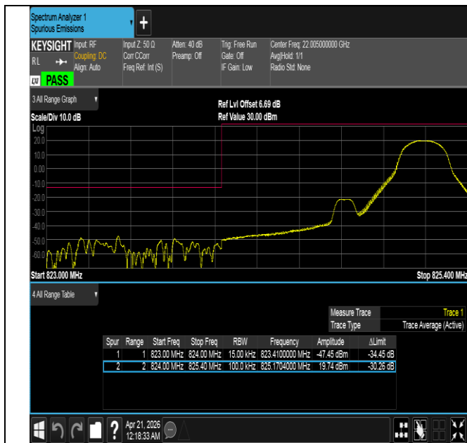
Band26(824-849)-1.4MHz-16QAM-26797-1RB#5-PASS
