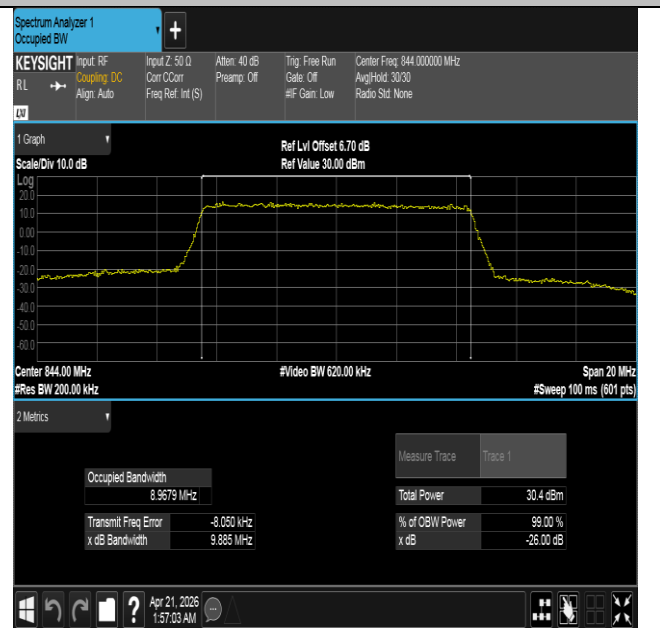
Band26(824-849)-10MHz-16QAM-26990-50RB#0-PASS
