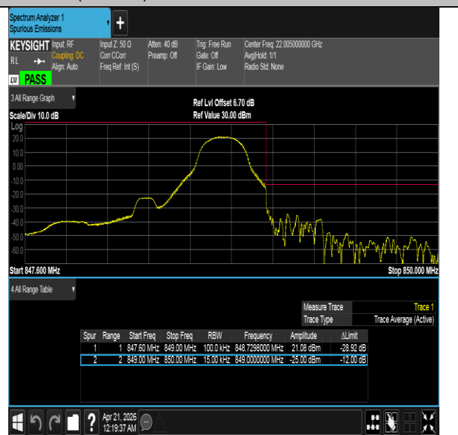
Band26(824-849)-1.4MHz-QPSK-27033-1RB#5-PASS
