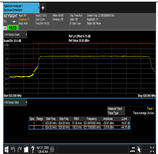
Band26(824-849)-5MHz-16QAM-26815-25RB#0-PASS
