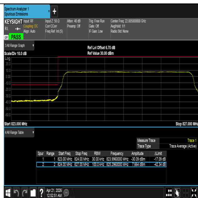
Band26(824-849)-3MHz-16QAM-26805-15RB#0-PASS
