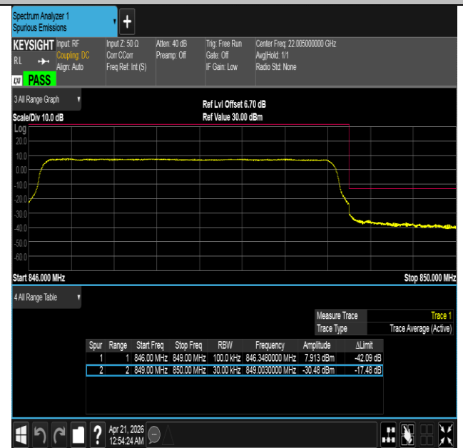
Band26(824-849)-3MHz-16QAM-27025-15RB#0-PASS
