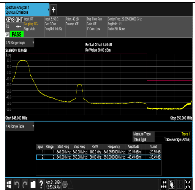
Band26(824-849)-3MHz-16QAM-27025-1RB#0-PASS
