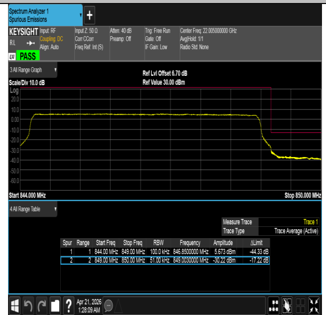
Band26(824-849)-5MHz-16QAM-27015-25RB#0-PASS
