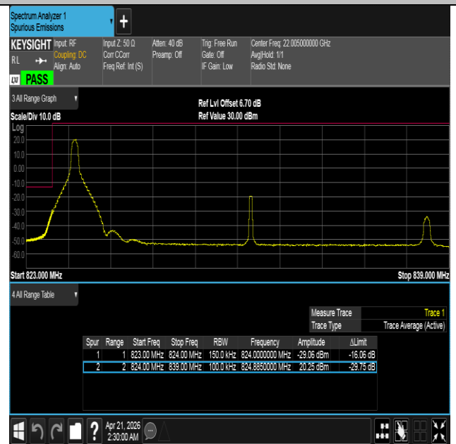
Band26(824-849)-15MHz-16QAM-26865-1RB#0-PASS
