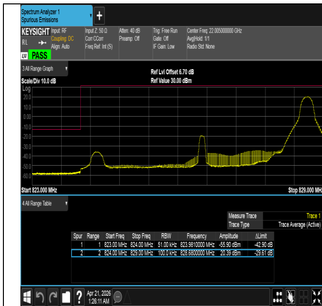
Band26(824-849)-5MHz-16QAM-26815-1RB#24-PASS
