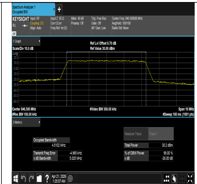
Band26(824-849)-5MHz-16QAM-27015-25RB#0-PASS
