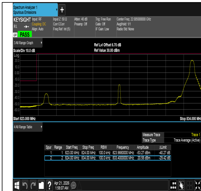
Band26(824-849)-10MHz-16QAM-26840-1RB#49-PASS
