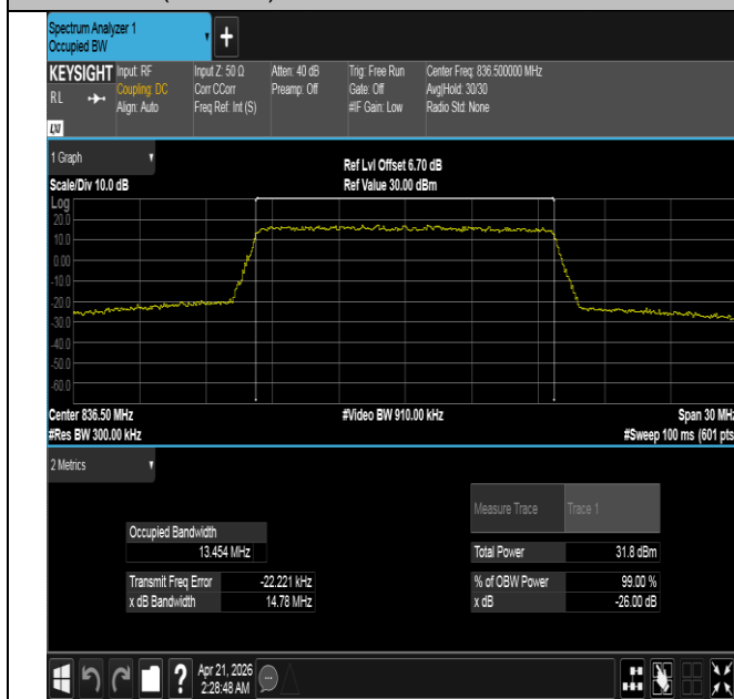
Band26(824-849)-15MHz-QPSK-26915-75RB#0-PASS
