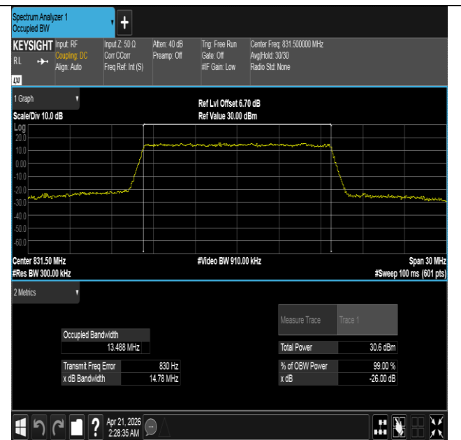
Band26(824-849)-15MHz-16QAM-26865-75RB#0-PASS
