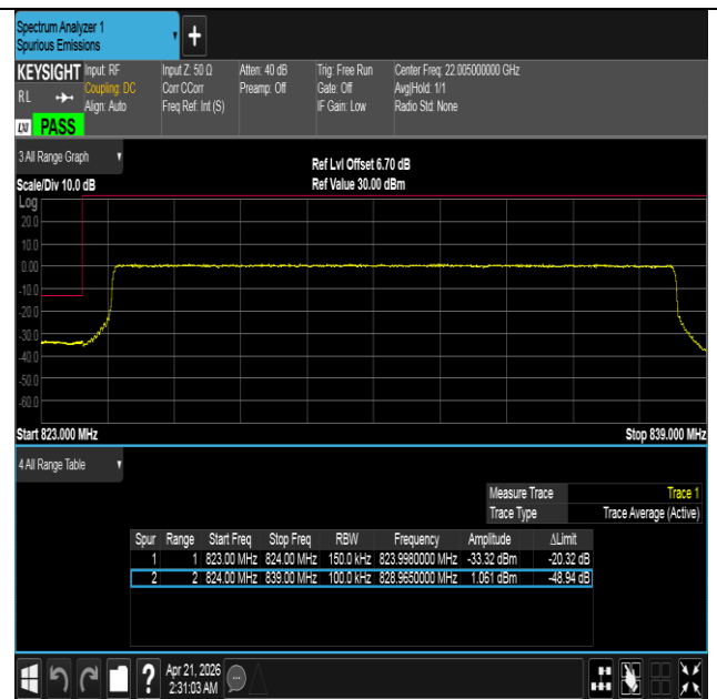
Band26(824-849)-15MHz-16QAM-26865-75RB#0-PASS
