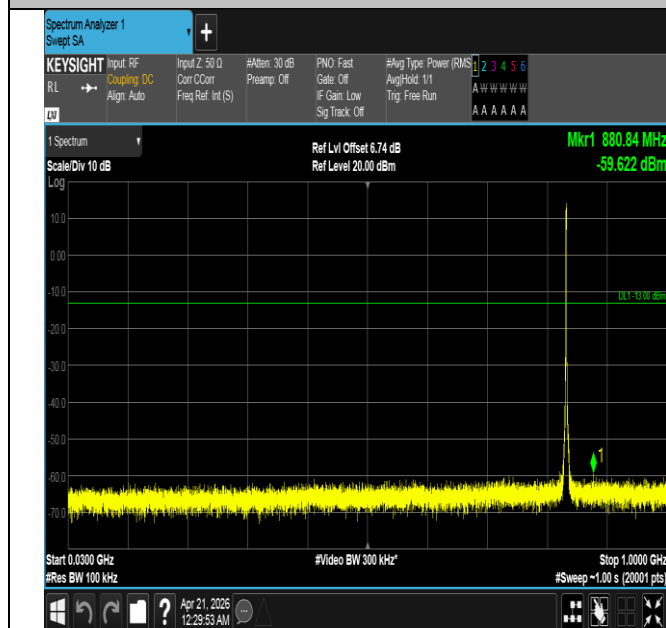
Band26(824-849)-1.4MHz-QPSK-26915-6RB#0-30~1000-PAS
