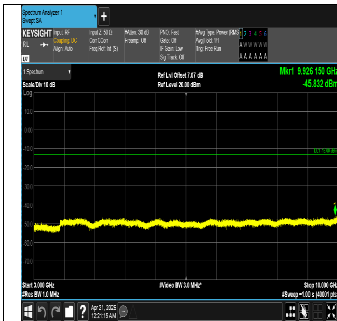
Band26(824-849)-1.4MHz-QPSK-26797-1RB#0-3000~10000- PASS
