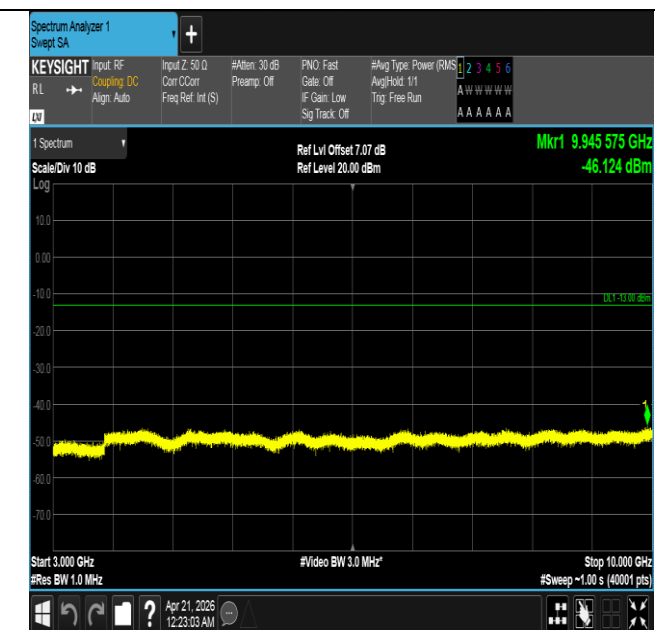
Band26(824-849)-1.4MHz-QPSK-26797-1RB#5-3000~10000- PASS
