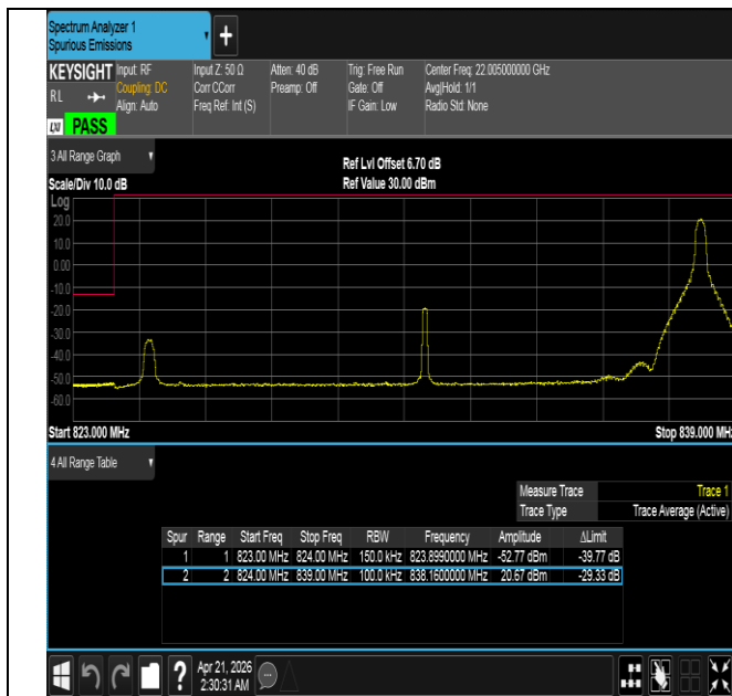
Band26(824-849)-15MHz-16QAM-26865-1RB#74-PASS
