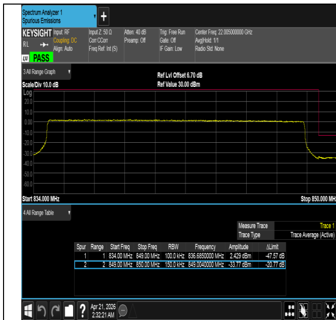
Band26(824-849)-15MHz-QPSK-26965-75RB#0-PASS
