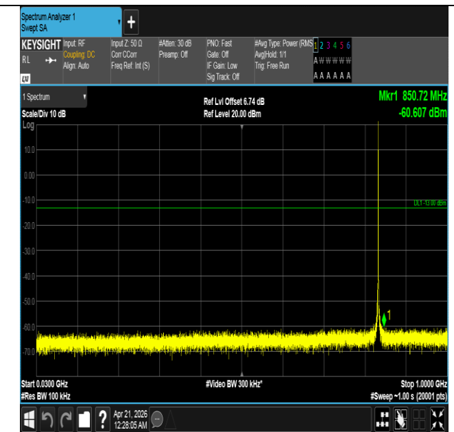
Band26(824-849)-1.4MHz-QPSK-26915-1RB#5-30~1000-PAS
