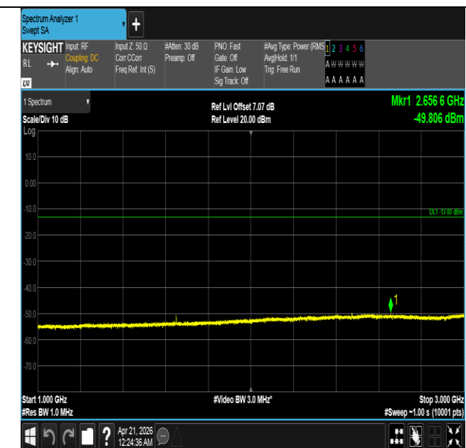
Band26(824-849)-1.4MHz-QPSK-26797-6RB#0-1000~3000-P
