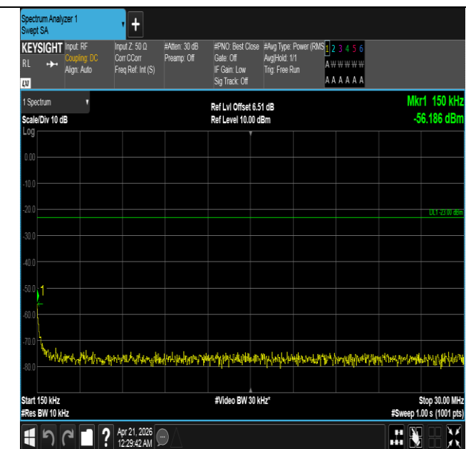
Band26(824-849)-1.4MHz-QPSK-26915-6RB#0-0.15~30-PAS
