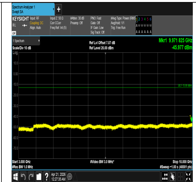
Band26(824-849)-1.4MHz-16QAM-26915-1RB#0-3000~10000 -PASS
