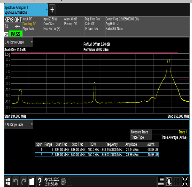
Band26(824-849)-15MHz-QPSK-26965-1RB#74-PASS
