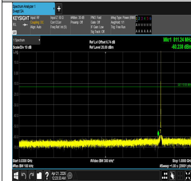
Band26(824-849)-1.4MHz-16QAM-26797-1RB#5-30~1000-PA SS
