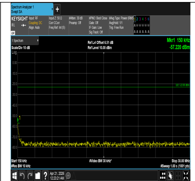
Band26(824-849)-1.4MHz-16QAM-26797-1RB#5-0.15~30-PA SS
