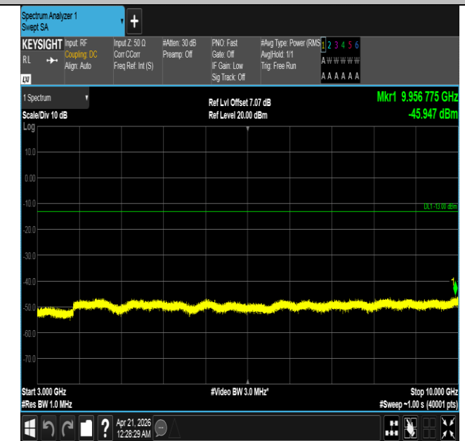
Band26(824-849)-1.4MHz-QPSK-26915-1RB#5-3000~10000-PASS
