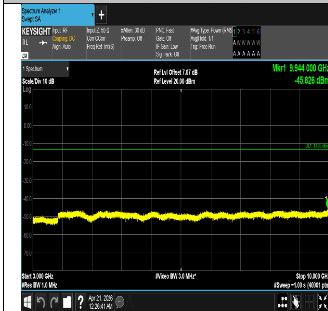
Band26(824-849)-1.4MHz-QPSK-26915-1RB#0-3000~10000- PASS
