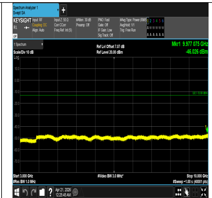
Band26(824-849)-1.4MHz-16QAM-26797-6RB#0-3000~10000 -PASS
