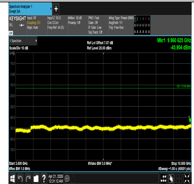
Band26(824-849)-1.4MHz-16QAM-26915-6RB#0-3000~10000
