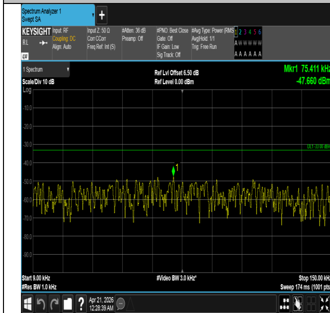
Band26(824-849)-1.4MHz-16QAM-26915-1RB#5-0.009~0.15- PASS
