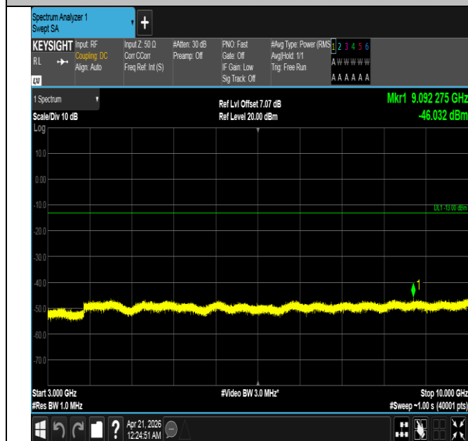
Band26(824-849)-1.4MHz-QPSK-26797-6RB#0-3000~10000-
