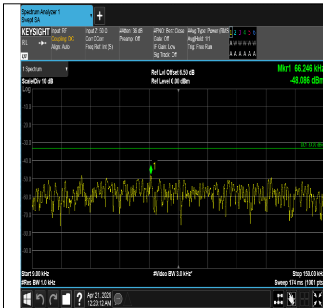
Band26(824-849)-1.4MHz-16QAM-26797-1RB#5-0.009~0.15- PASS
