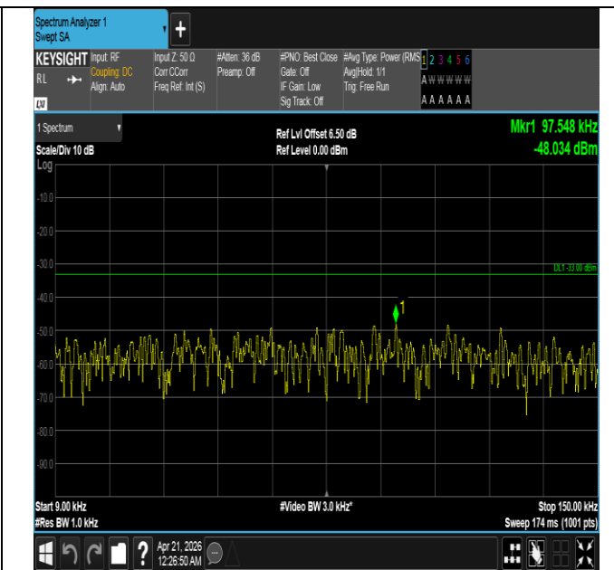
Band26(824-849)-1.4MHz-16QAM-26915-1RB#0-0.009~0.15- PASS
