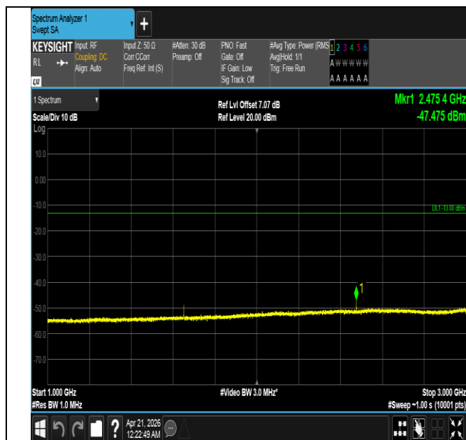
Band26(824-849)-1.4MHz-QPSK-26797-1RB#5-1000~3000-P ASS
