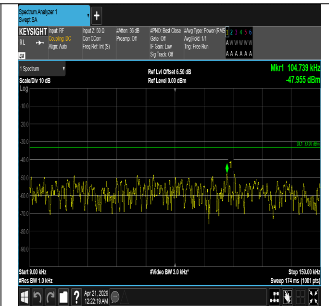
Band26(824-849)-1.4MHz-QPSK-26797-1RB#5-0.009~0.15-P ASS
