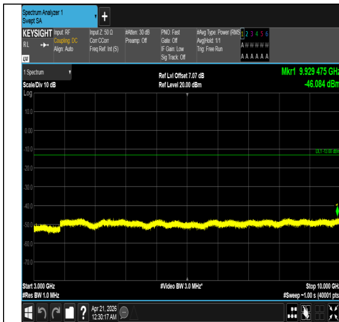
Band26(824-849)-1.4MHz-QPSK-26915-6RB#0-3000~10000- PASS
