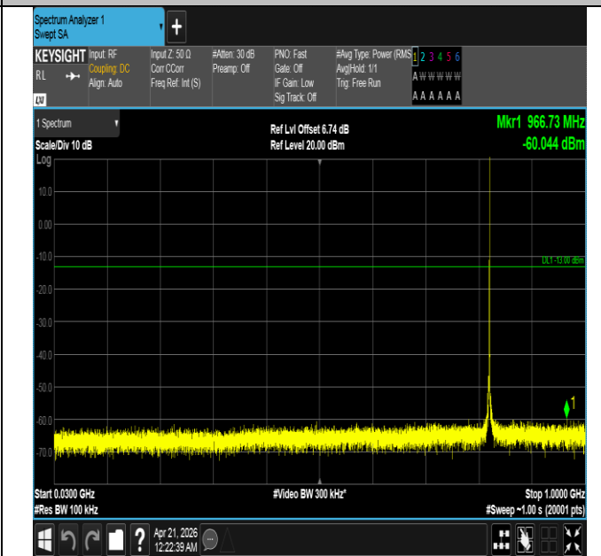
Band26(824-849)-1.4MHz-QPSK-26797-1RB#5-30~1000-PAS S
