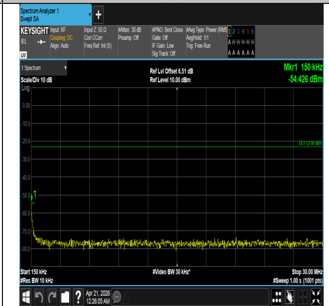
Band26(824-849)-1.4MHz-QPSK-26915-1RB#0-0.15~30-PAS S
