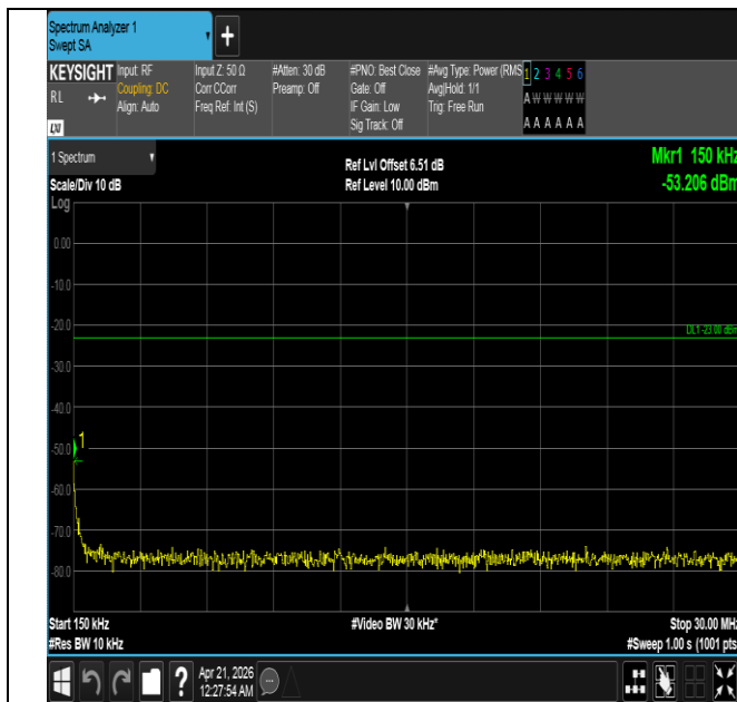
Band26(824-849)-1.4MHz-QPSK-26915-1RB#5-0.15~30-PAS
