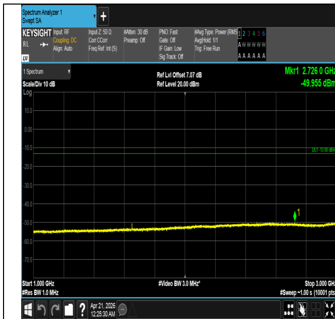
Band26(824-849)-1.4MHz-16QAM-26797-6RB#0-1000~3000- PASS
