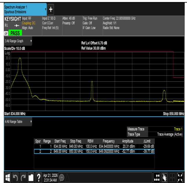
Band26(824-849)-15MHz-16QAM-26965-1RB#0-PASS
