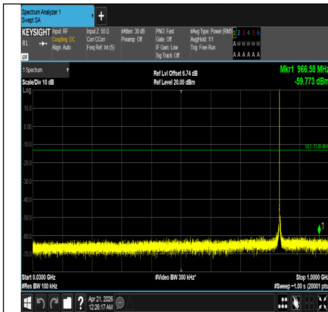
Band26(824-849)-1.4MHz-QPSK-26915-1RB#0-30~1000-PAS S
