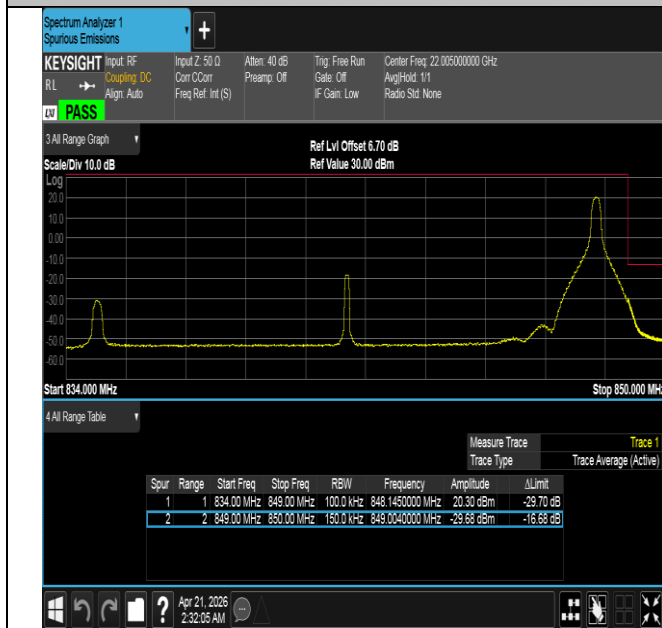
Band26(824-849)-15MHz-16QAM-26965-1RB#74-PASS
