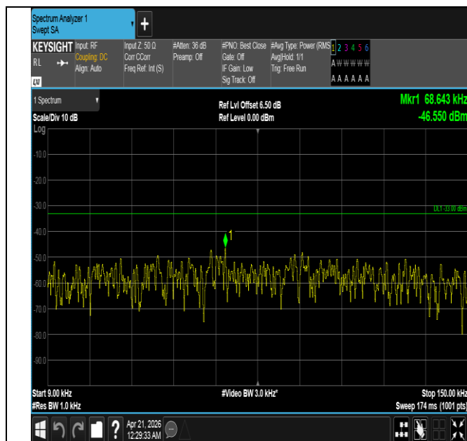
Band26(824-849)-1.4MHz-QPSK-26915-6RB#0-0.009~0.15-P
