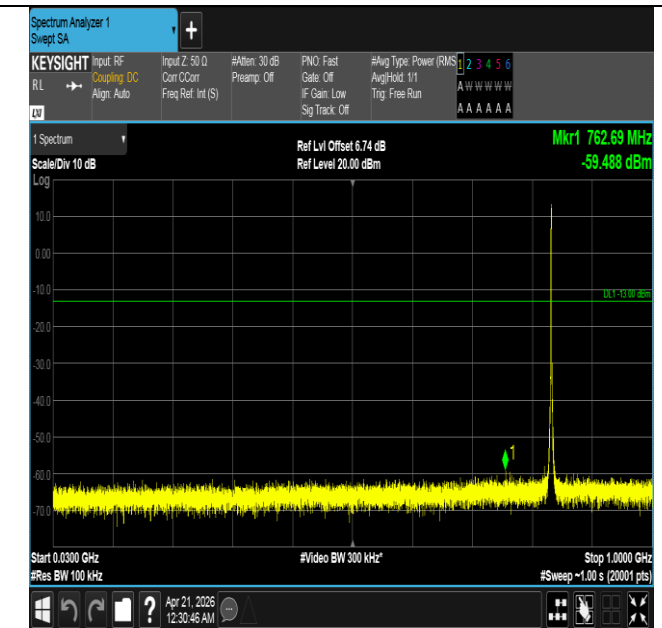
Band26(824-849)-1.4MHz-16QAM-26915-6RB#0-30~1000-PA
