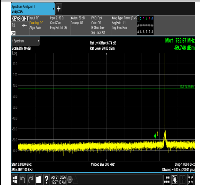
Band26(824-849)-1.4MHz-16QAM-26915-1RB#0-30~1000-PA SS
