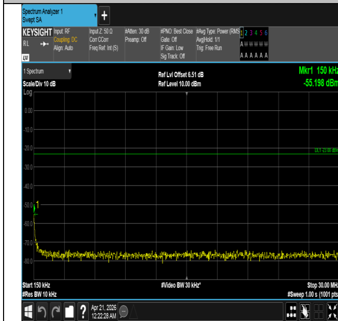
Band26(824-849)-1.4MHz-QPSK-26797-1RB#5-0.15~30-PAS S
