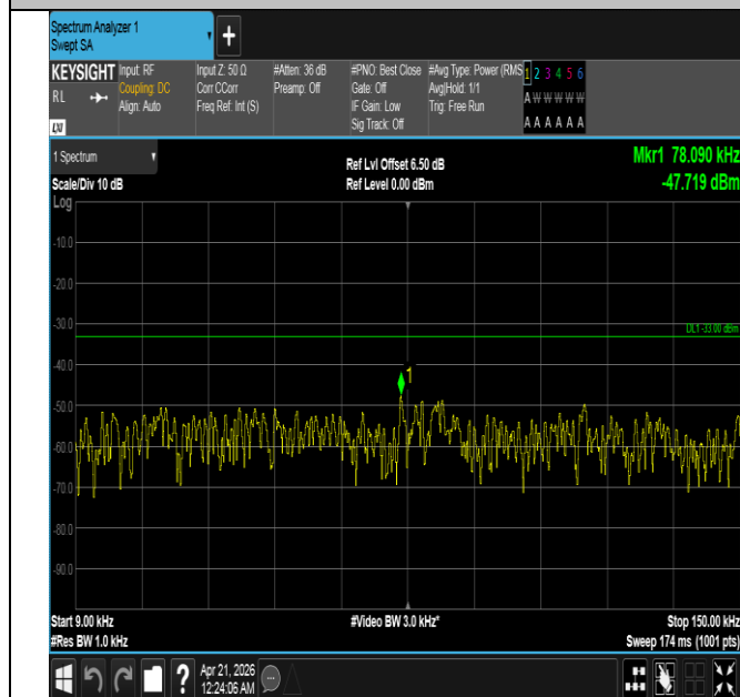
Band26(824-849)-1.4MHz-QPSK-26797-6RB#0-0.009~0.15-P ASS
