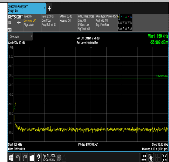
Band26(824-849)-1.4MHz-QPSK-26797-6RB#0-0.15~30-PAS S
