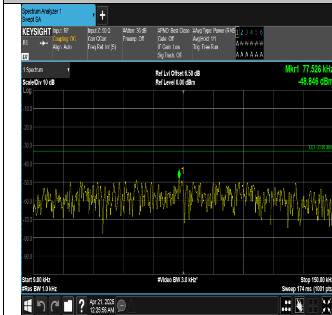
Band26(824-849)-1.4MHz-QPSK-26915-1RB#0-0.009~0.15-P ASS
