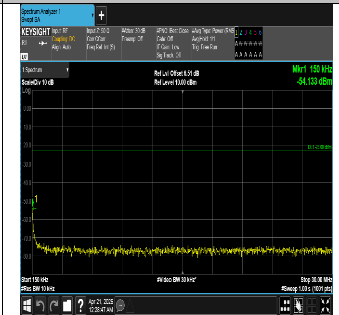
Band26(824-849)-1.4MHz-16QAM-26915-1RB#5-0.15~30-PA SS
