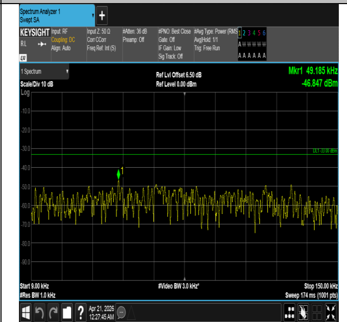
Band26(824-849)-1.4MHz-QPSK-26915-1RB#5-0.009~0.15-P ASS
