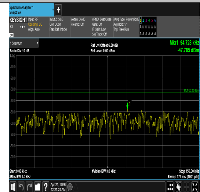
Band26(824-849)-1.4MHz-16QAM-26797-1RB#0-0.009~0.15-
