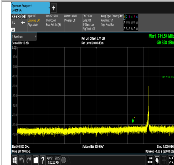
Band26(824-849)-3MHz-QPSK-26915-1RB#0-30~1000-PASS
