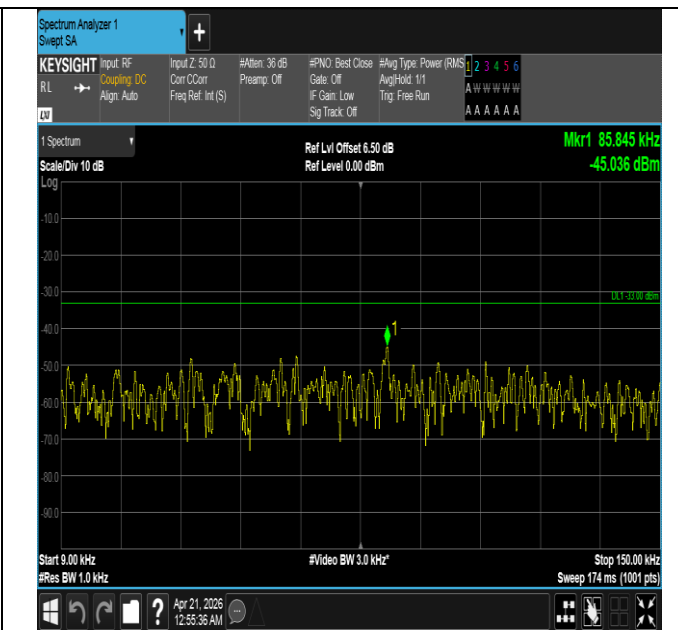
Band26(824-849)-3MHz-16QAM-26805-1RB#0-0.009~0.15-P ASS
