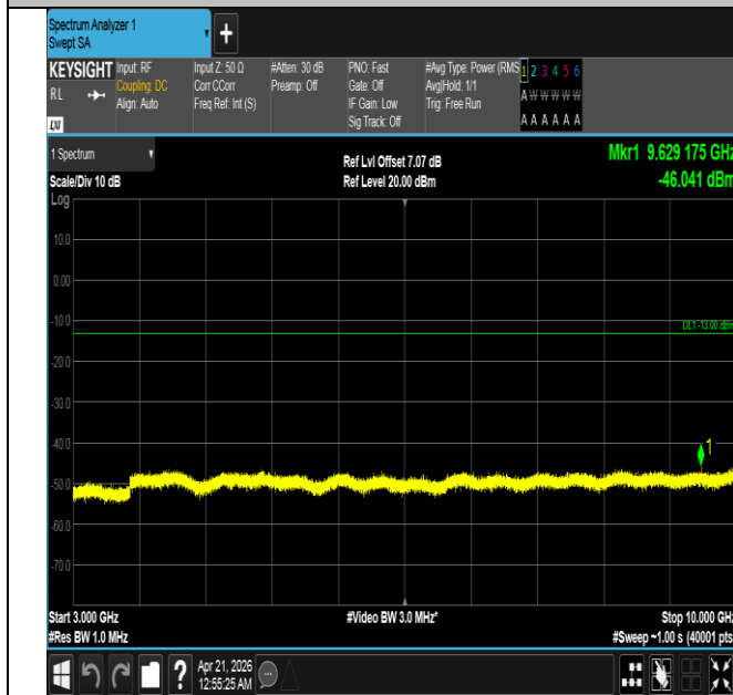
Band26(824-849)-3MHz-QPSK-26805-1RB#0-3000~10000-P ASS
