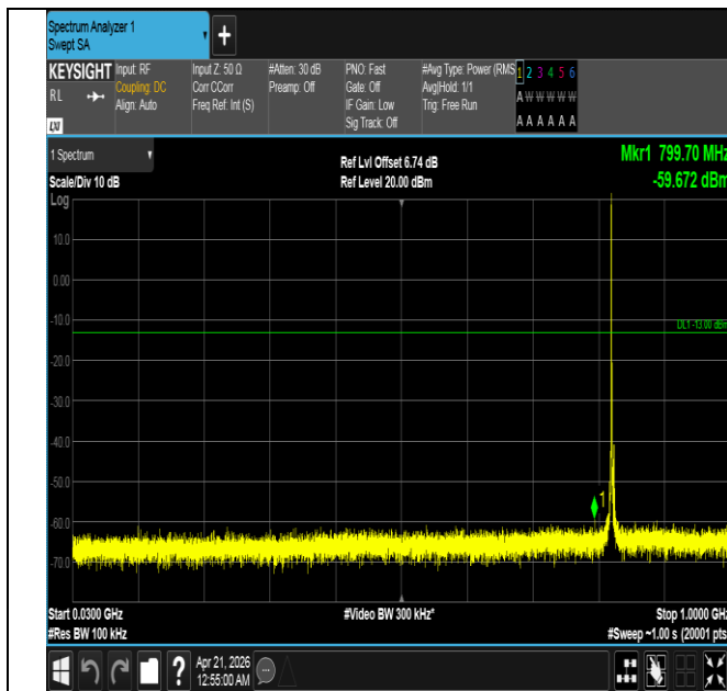
Band26(824-849)-3MHz-QPSK-26805-1RB#0-30~1000-PASS
