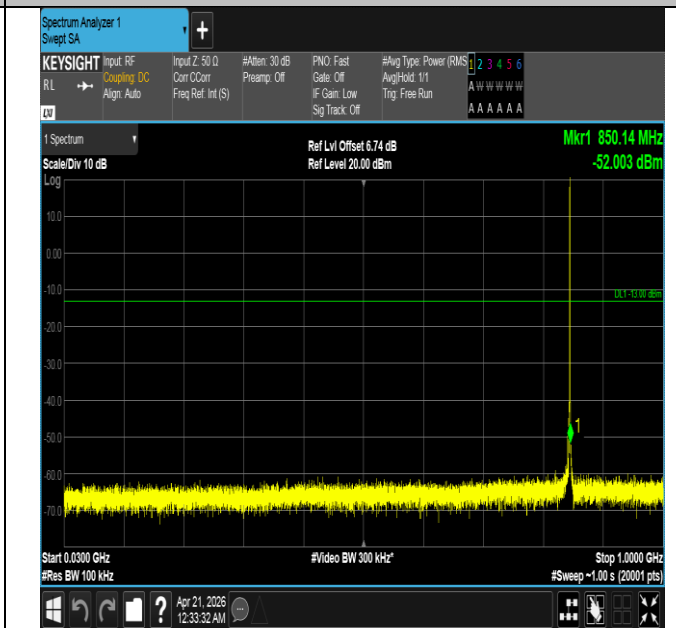
Band26(824-849)-1.4MHz-QPSK-27033-1RB#5-30~1000-PAS S
