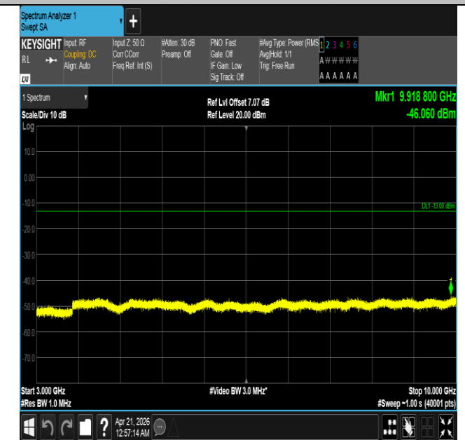
Band26(824-849)-3MHz-QPSK-26805-1RB#14-3000~10000-P
