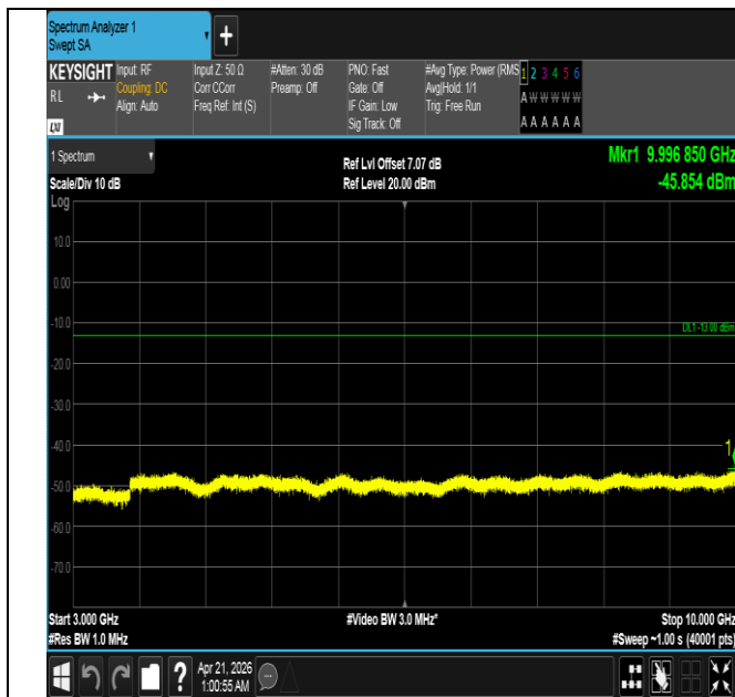
Band26(824-849)-3MHz-QPSK-26915-1RB#0-3000~10000-P ASS
