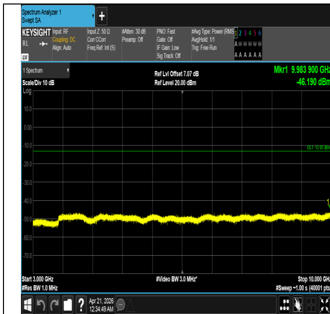
Band26(824-849)-1.4MHz-16QAM-27033-1RB#5-3000~10000 -PASS
