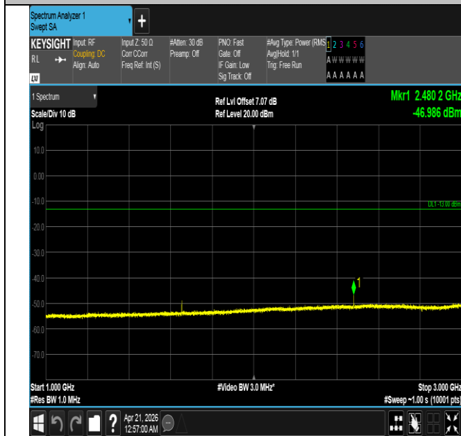
Band26(824-849)-3MHz-QPSK-26805-1RB#14-1000~3000-P
