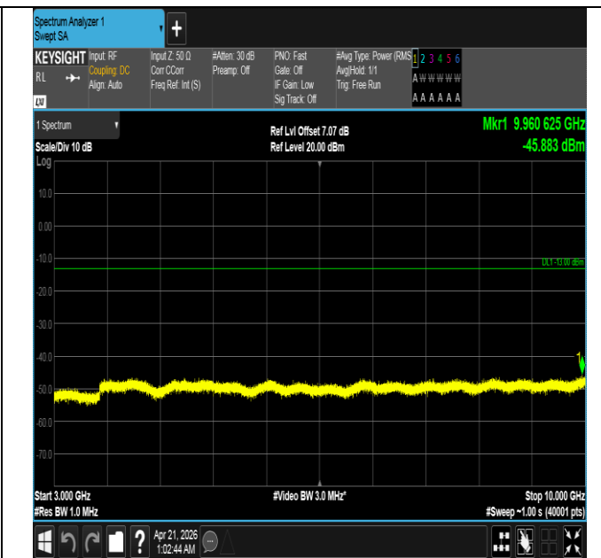
Band26(824-849)-3MHz-QPSK-26915-1RB#14-3000~10000-P
