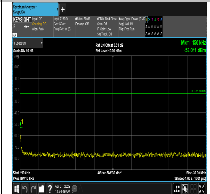
Band26(824-849)-3MHz-QPSK-26805-1RB#0-0.15~30-PASS
