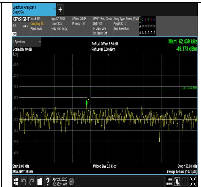
Band26(824-849)-1.4MHz-QPSK-27033-1RB#5-0.009~0.15-P ASS
