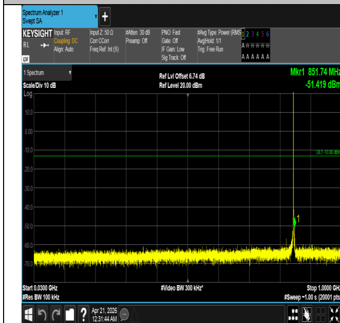
Band26(824-849)-1.4MHz-QPSK-27033-1RB#0-30~1000-PAS
