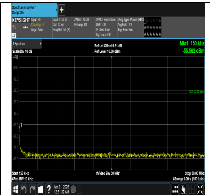
Band26(824-849)-1.4MHz-QPSK-27033-1RB#0-0.15~30-PAS
