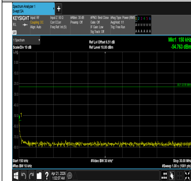
Band26(824-849)-3MHz-QPSK-26915-1RB#14-0.15~30-PAS S
