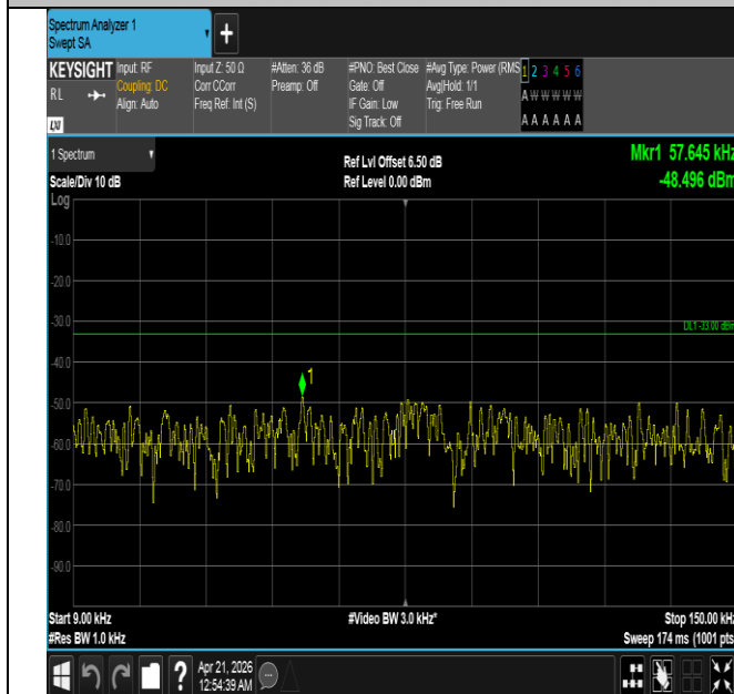
Band26(824-849)-3MHz-QPSK-26805-1RB#0-0.009~0.15-PA SS
