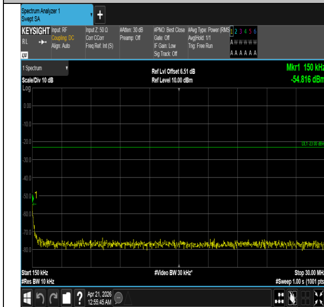
Band26(824-849)-3MHz-16QAM-26805-1RB#0-0.15~30-PAS S
