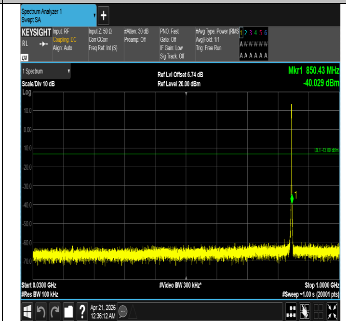
Band26(824-849)-1.4MHz-16QAM-27033-6RB#0-30~1000-PA SS
