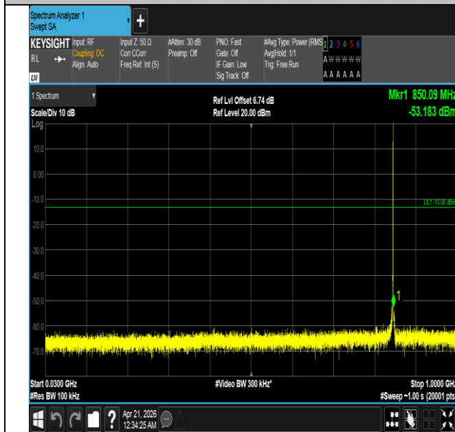
Band26(824-849)-1.4MHz-16QAM-27033-1RB#5-30~1000-PA SS
