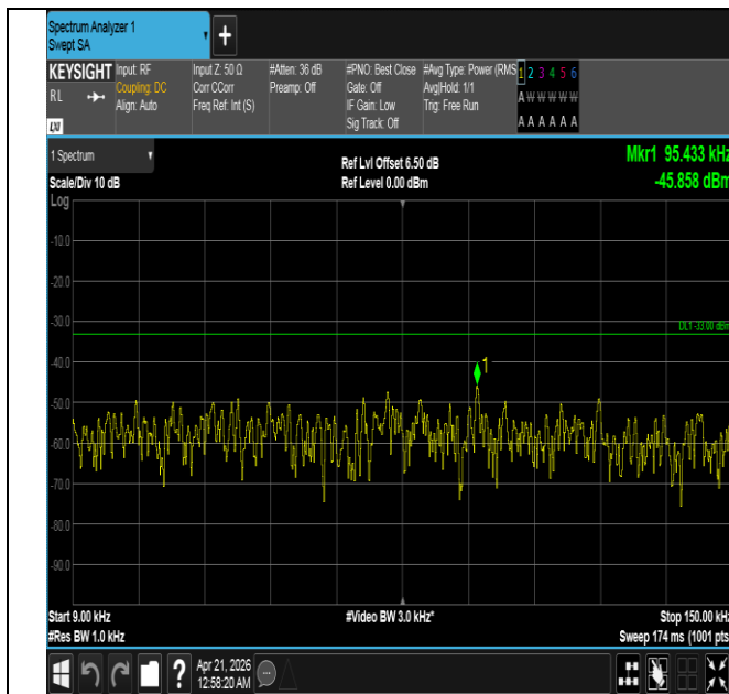
Band26(824-849)-3MHz-QPSK-26805-15RB#0-0.009~0.15-P
