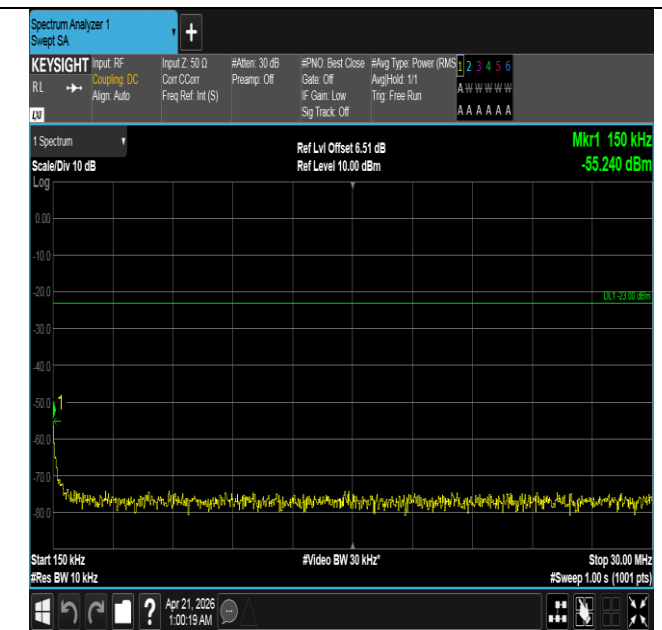
Band26(824-849)-3MHz-QPSK-26915-1RB#0-0.15~30-PASS
