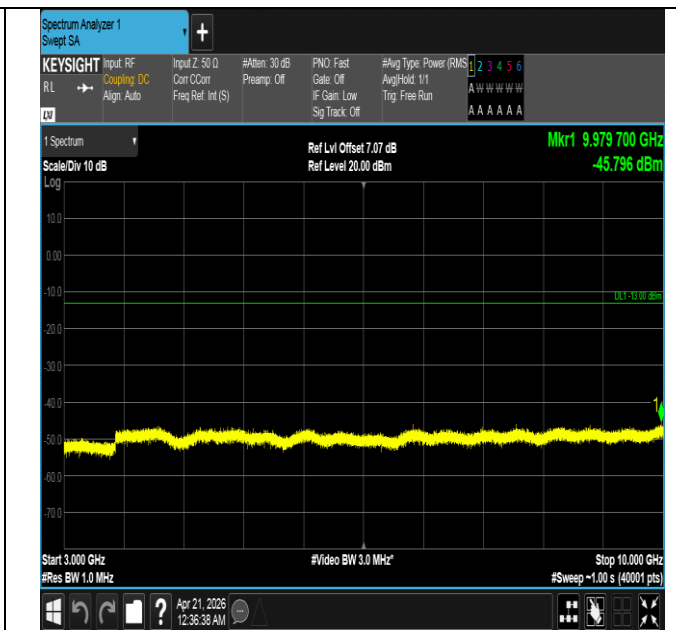
Band26(824-849)-1.4MHz-16QAM-27033-6RB#0-3000~10000 -PASS
