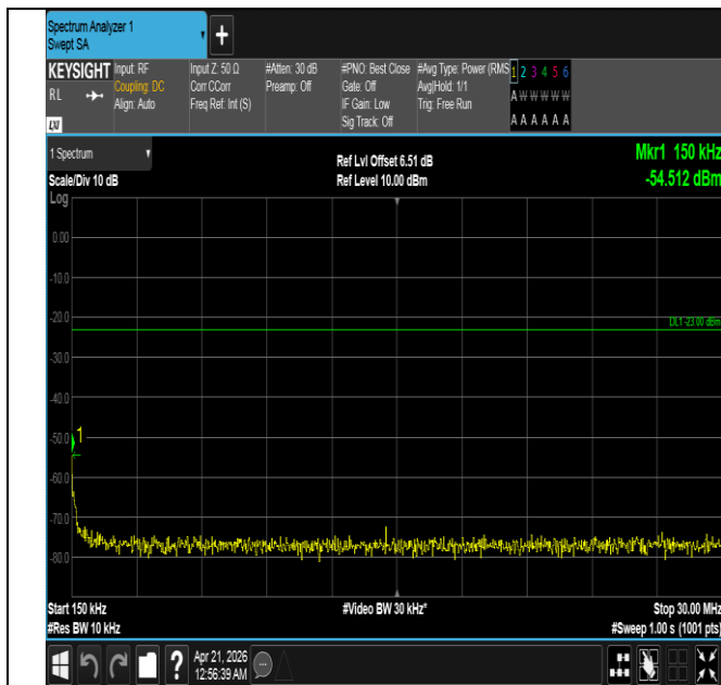
Band26(824-849)-3MHz-QPSK-26805-1RB#14-0.15~30-PAS
