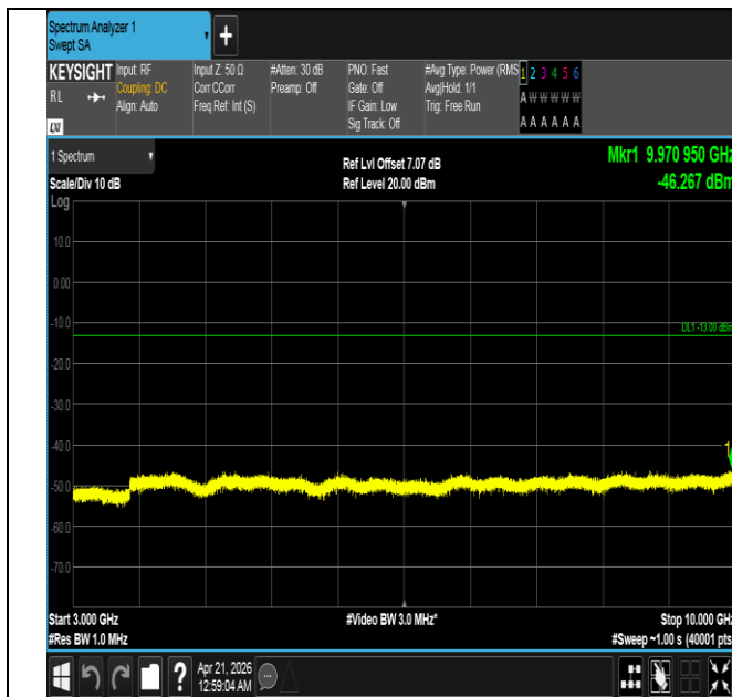
Band26(824-849)-3MHz-QPSK-26805-15RB#0-3000~10000- PASS
