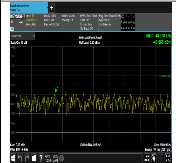
Band26(824-849)-3MHz-16QAM-26805-15RB#0-0.009~0.15- PASS
