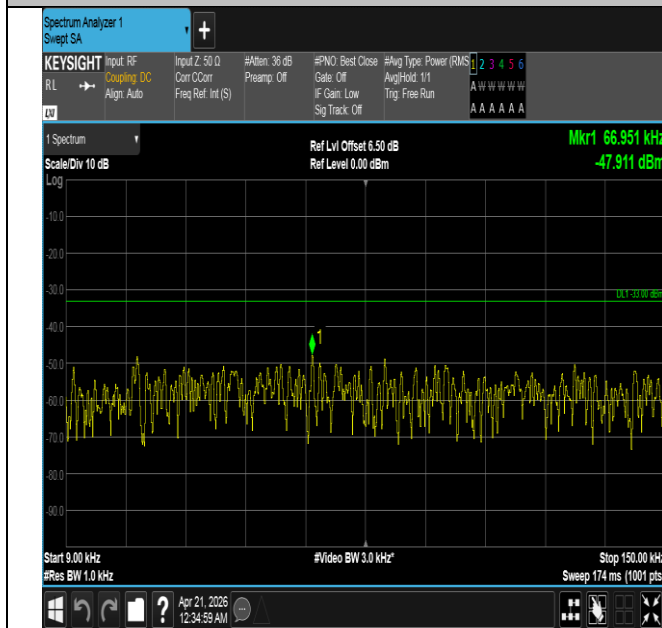
Band26(824-849)-1.4MHz-QPSK-27033-6RB#0-0.009~0.15-P ASS
