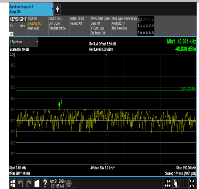
Band26(824-849)-3MHz-16QAM-26915-1RB#0-0.009~0.15-P
