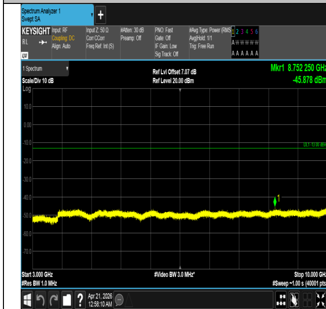
Band26(824-849)-3MHz-16QAM-26805-1RB#14-3000~10000 -PASS
