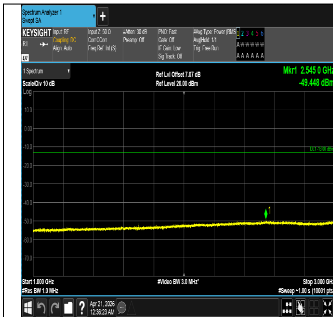
Band26(824-849)-1.4MHz-16QAM-27033-6RB#0-1000~3000- PASS
