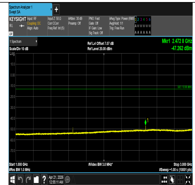
Band26(824-849)-3MHz-QPSK-26805-1RB#0-1000~3000-PA SS
