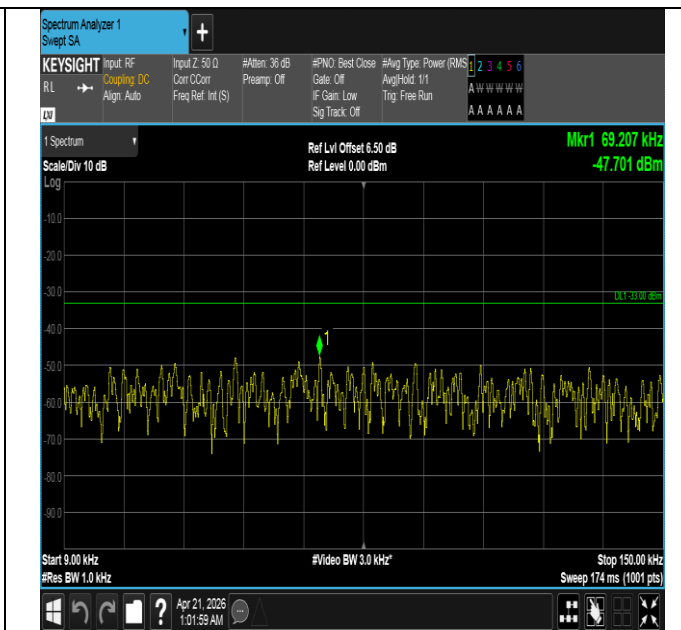
Band26(824-849)-3MHz-QPSK-26915-1RB#14-0.009~0.15-P ASS
