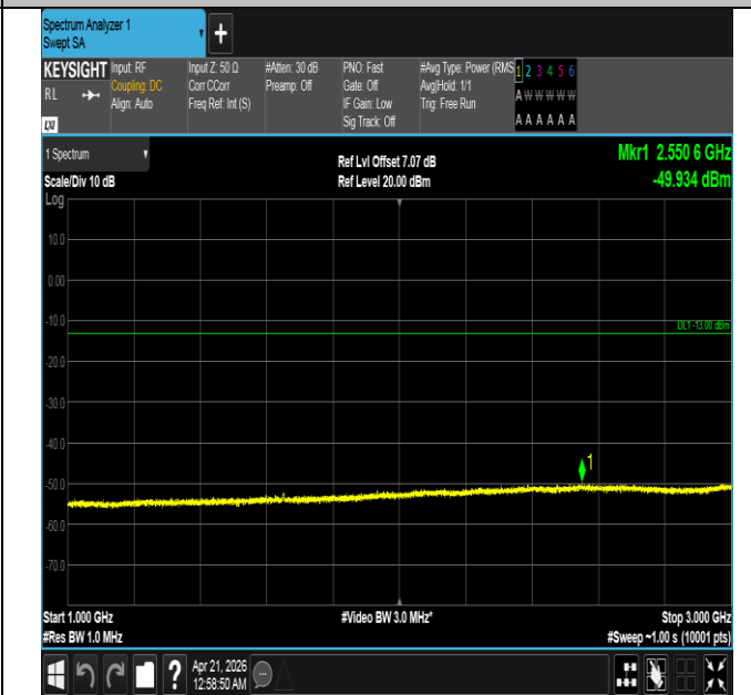
Band26(824-849)-3MHz-QPSK-26805-15RB#0-1000~3000-P
