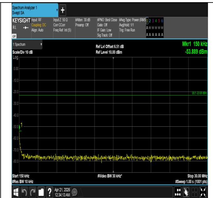
Band26(824-849)-1.4MHz-16QAM-27033-1RB#5-0.15~30-PA SS
