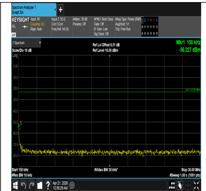
Band26(824-849)-3MHz-QPSK-26805-15RB#0-0.15~30-PAS
