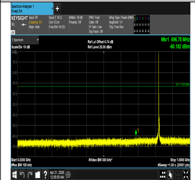
Band26(824-849)-3MHz-16QAM-26805-1RB#0-30~1000-PAS S
