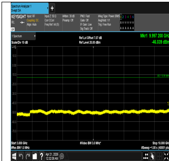
Band26(824-849)-1.4MHz-QPSK-27033-1RB#0-3000~10000- PASS
