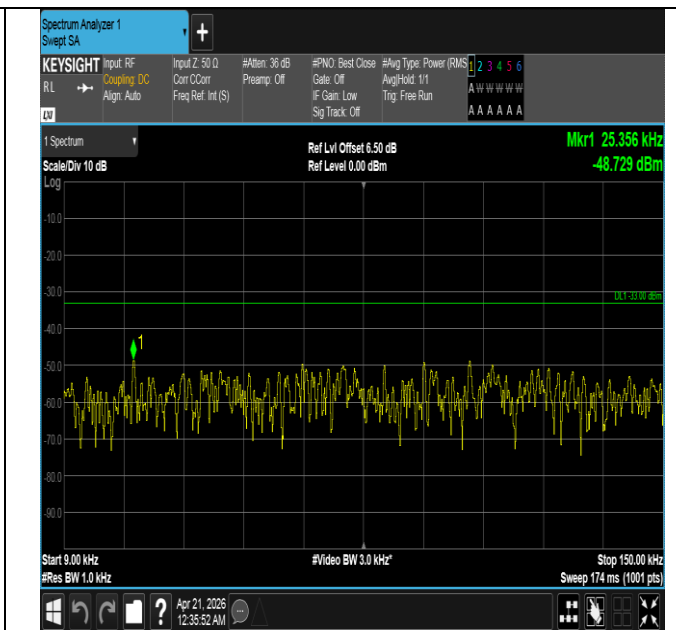
Band26(824-849)-1.4MHz-16QAM-27033-6RB#0-0.009~0.15- PASS
