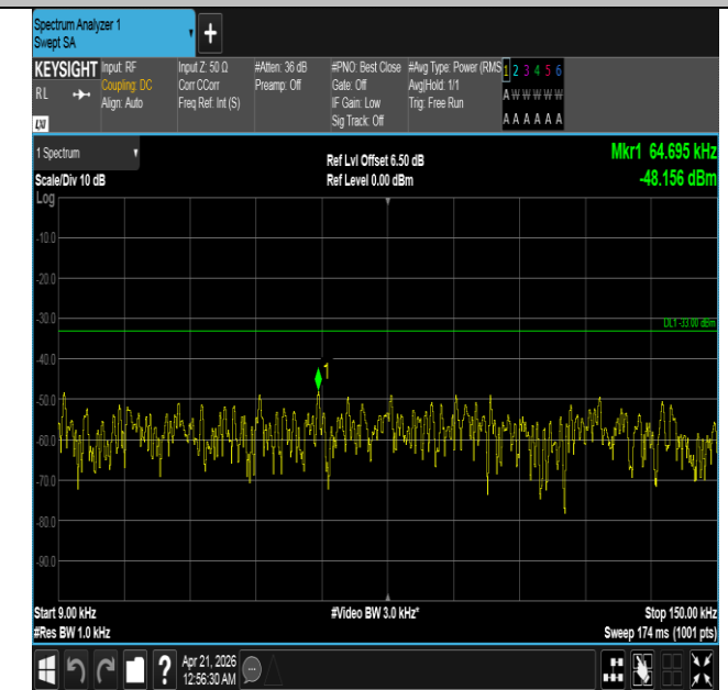
Band26(824-849)-3MHz-QPSK-26805-1RB#14-0.009~0.15-P ASS
