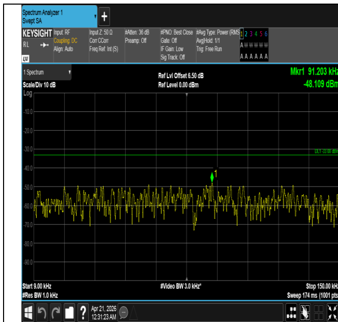
Band26(824-849)-1.4MHz-QPSK-27033-1RB#0-0.009~0.15-P
