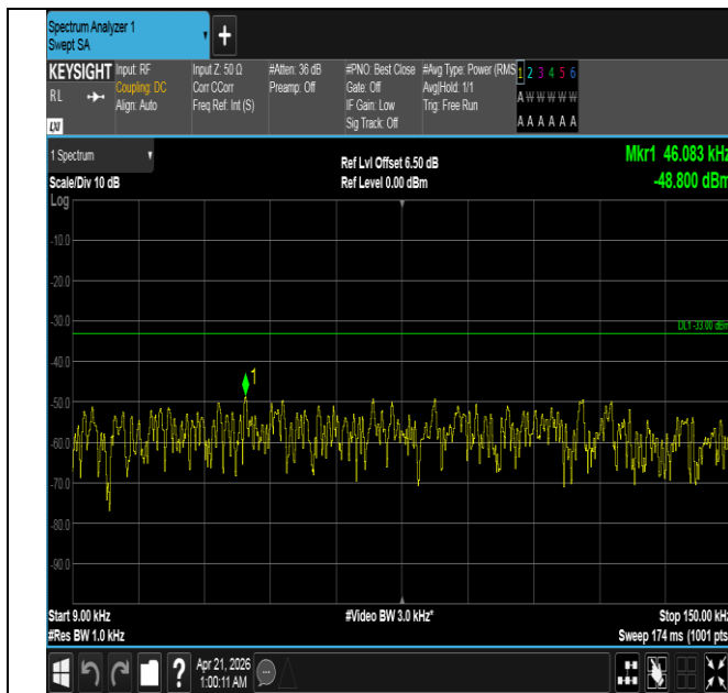
Band26(824-849)-3MHz-QPSK-26915-1RB#0-0.009~0.15-PA SS
