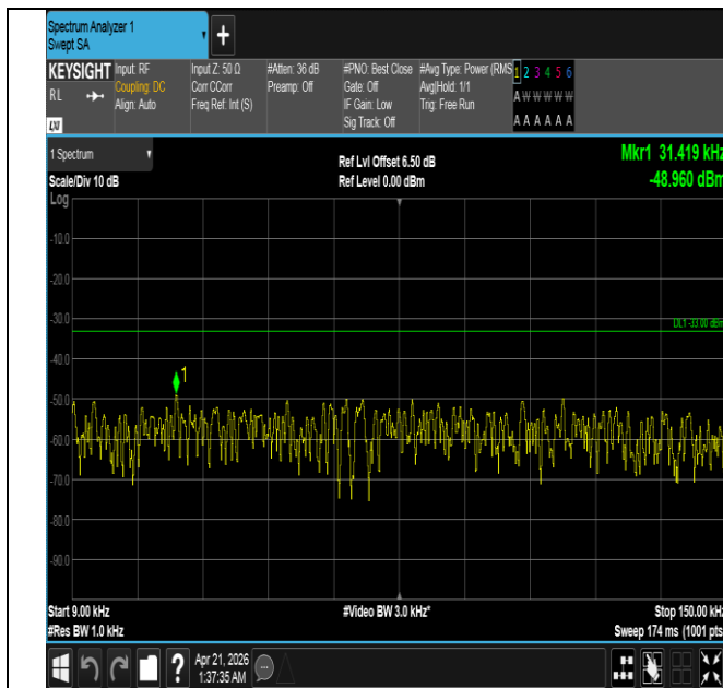
Band26(824-849)-5MHz-QPSK-26915-25RB#0-0.009~0.15-P
