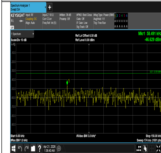
Band26(824-849)-5MHz-16QAM-26915-1RB#24-0.009~0.15- PASS
