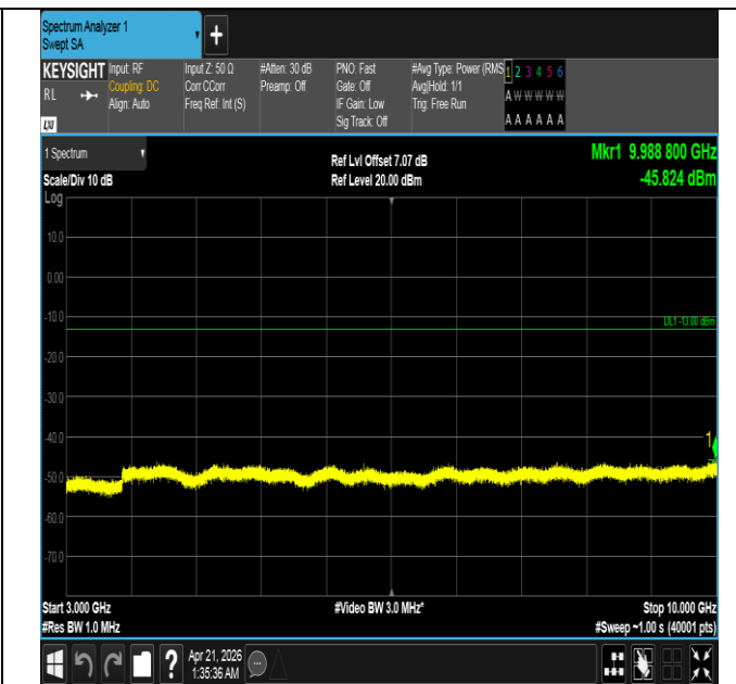
Band26(824-849)-5MHz-16QAM-26915-1RB#0-3000~10000- PASS
