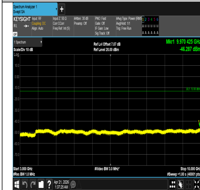
Band26(824-849)-5MHz-16QAM-26915-1RB#24-3000~10000 -PASS
