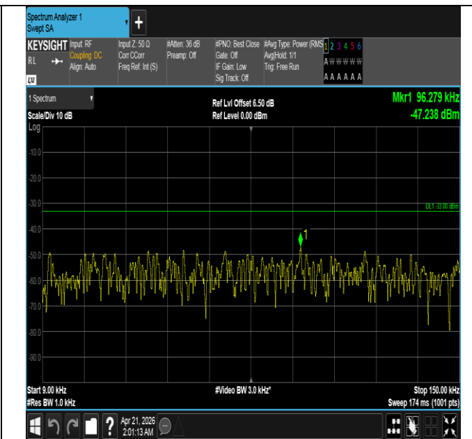
Band26(824-849)-10MHz-16QAM-26840-1RB#0-0.009~0.15- PASS
