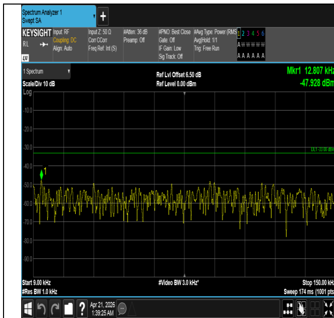
Band26(824-849)-5MHz-QPSK-27015-1RB#0-0.009~0.15-PA SS
