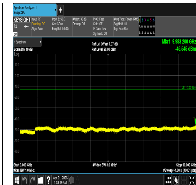
Band26(824-849)-5MHz-QPSK-26915-25RB#0-3000~10000- PASS
