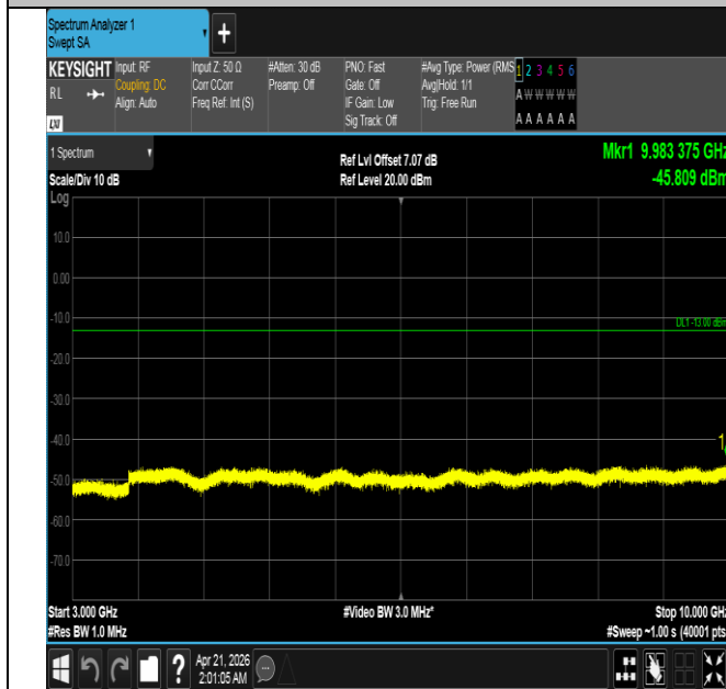
Band26(824-849)-10MHz-QPSK-26840-1RB#0-3000~10000-
