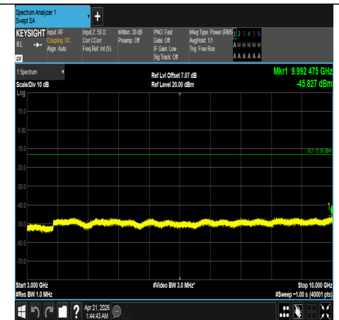
Band26(824-849)-5MHz-16QAM-27015-25RB#0-3000~10000
