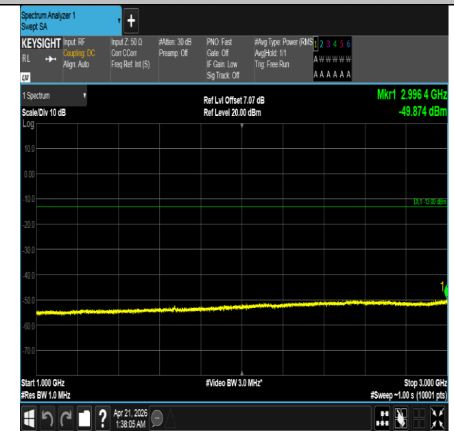
Band26(824-849)-5MHz-QPSK-26915-25RB#0-1000~3000-P
