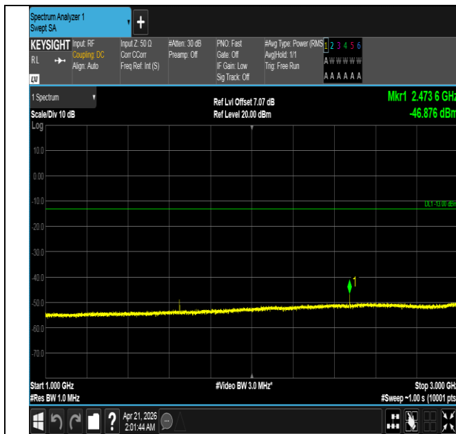
Band26(824-849)-10MHz-16QAM-26840-1RB#0-1000~3000- PASS
