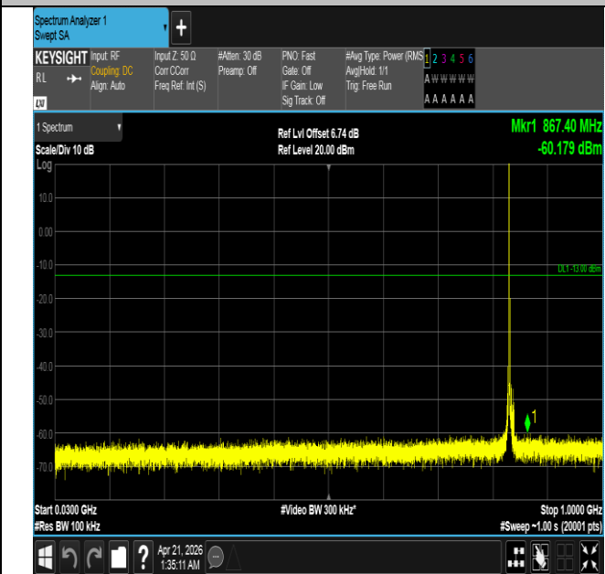
Band26(824-849)-5MHz-16QAM-26915-1RB#0-30~1000-PAS S
