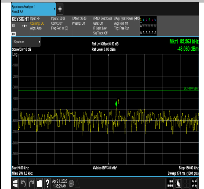
Band26(824-849)-5MHz-16QAM-26915-25RB#0-0.009~0.15- PASS
