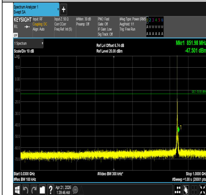
Band26(824-849)-5MHz-QPSK-27015-1RB#0-30~1000-PASS
