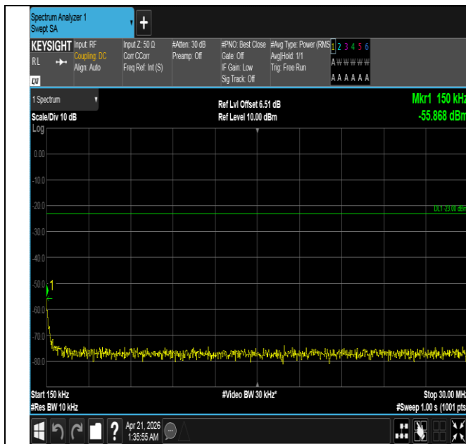
Band26(824-849)-5MHz-QPSK-26915-1RB#24-0.15~30-PAS
