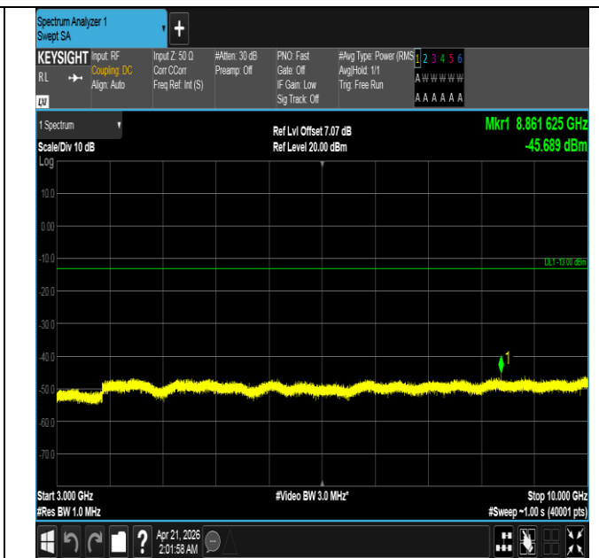
Band26(824-849)-10MHz-16QAM-26840-1RB#0-3000~10000 -PASS
