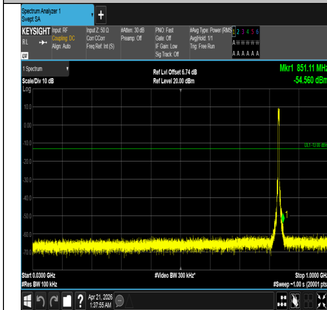
Band26(824-849)-5MHz-QPSK-26915-25RB#0-30~1000-PAS
