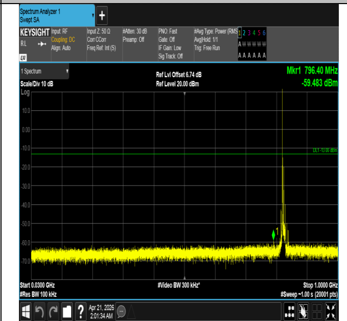
Band26(824-849)-10MHz-16QAM-26840-1RB#0-30~1000-PA SS
