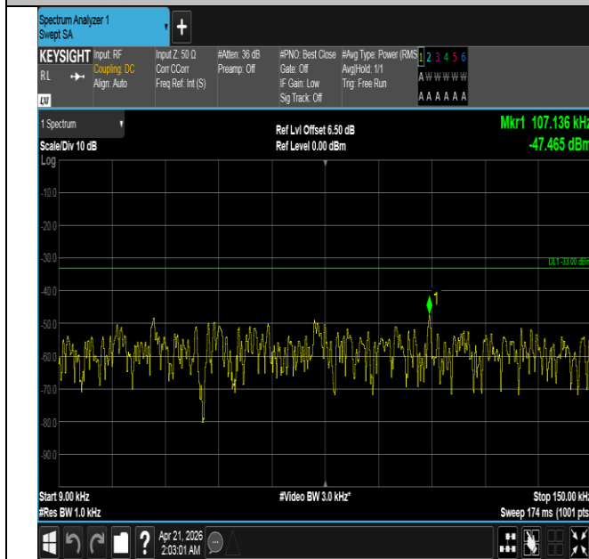
Band26(824-849)-10MHz-16QAM-26840-1RB#49-0.009~0.15 -PASS
