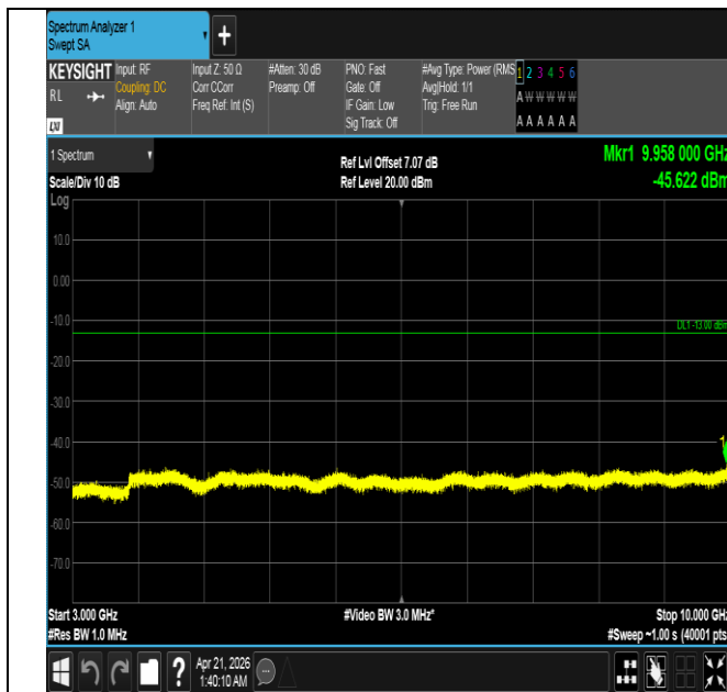
Band26(824-849)-5MHz-QPSK-27015-1RB#0-3000~10000-P ASS
