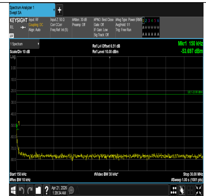
Band26(824-849)-5MHz-QPSK-27015-1RB#0-0.15~30-PASS
