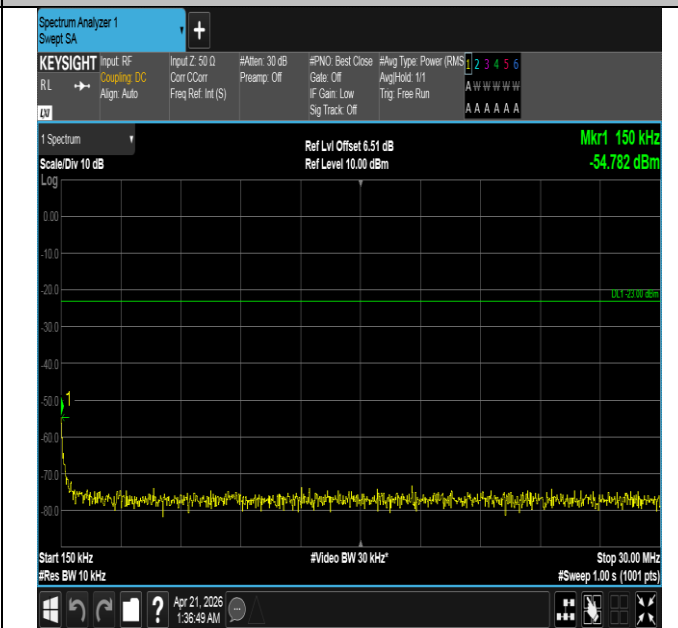
Band26(824-849)-5MHz-16QAM-26915-1RB#24-0.15~30-PAS S
