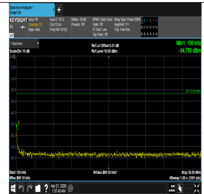
Band26(824-849)-5MHz-QPSK-26915-25RB#0-0.15~30-PAS
