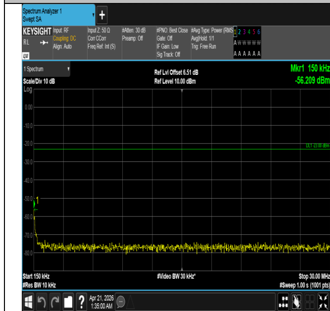
Band26(824-849)-5MHz-16QAM-26915-1RB#0-0.15~30-PAS S
