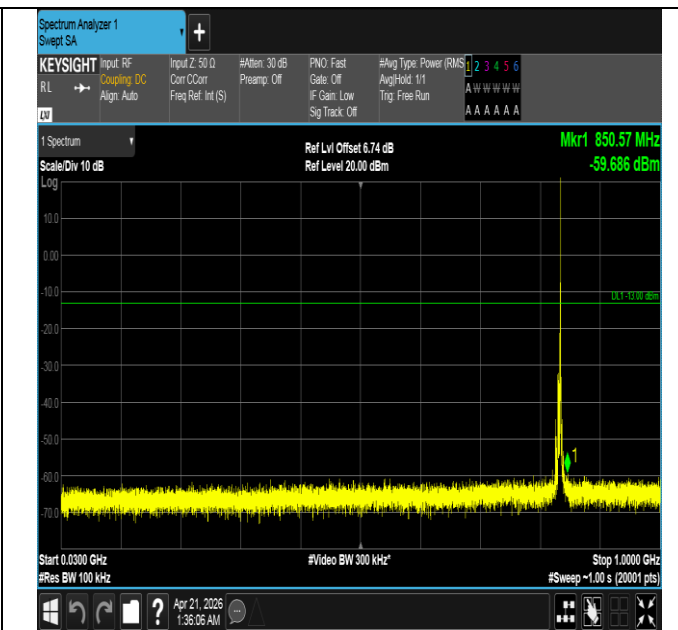
Band26(824-849)-5MHz-QPSK-26915-1RB#24-30~1000-PAS
