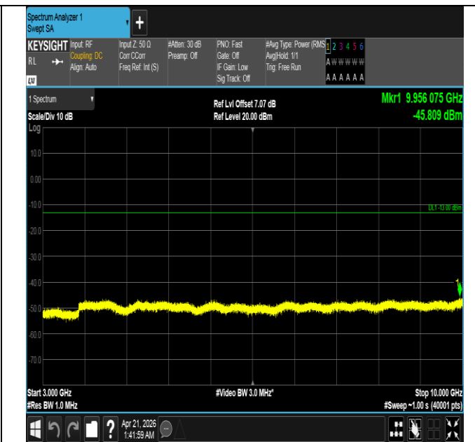
Band26(824-849)-5MHz-QPSK-27015-1RB#24-3000~10000-P
