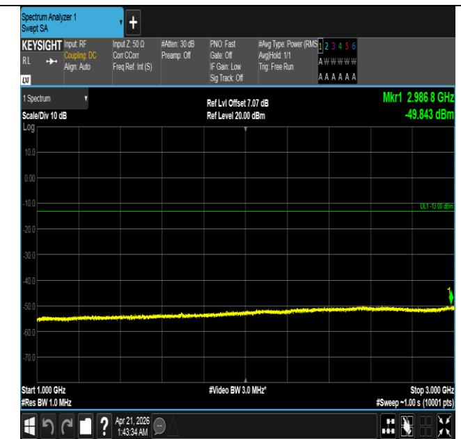
Band26(824-849)-5MHz-QPSK-27015-25RB#0-1000~3000-P
