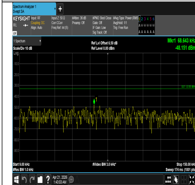
Band26(824-849)-5MHz-QPSK-27015-25RB#0-0.009~0.15-P
