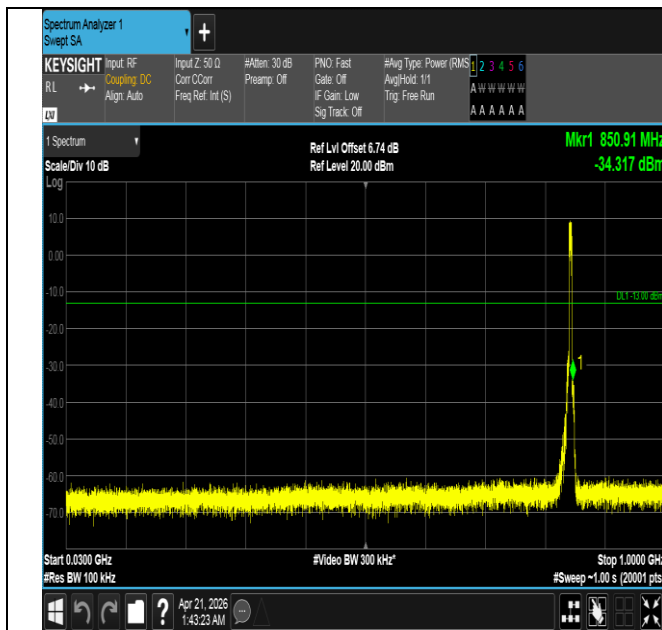
Band26(824-849)-5MHz-QPSK-27015-25RB#0-30~1000-PAS
