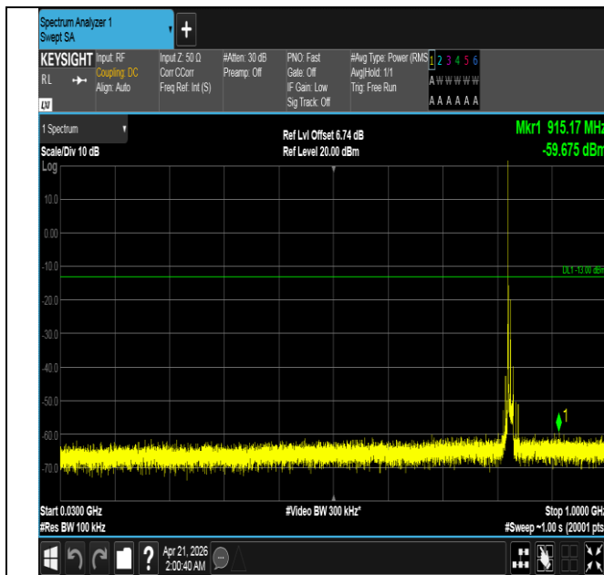
Band26(824-849)-10MHz-QPSK-26840-1RB#0-30~1000-PAS
