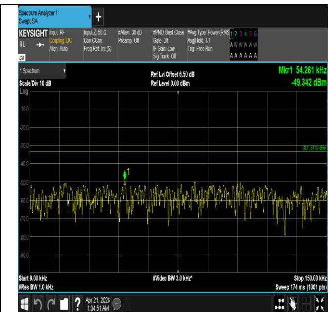
Band26(824-849)-5MHz-16QAM-26915-1RB#0-0.009~0.15-P ASS
