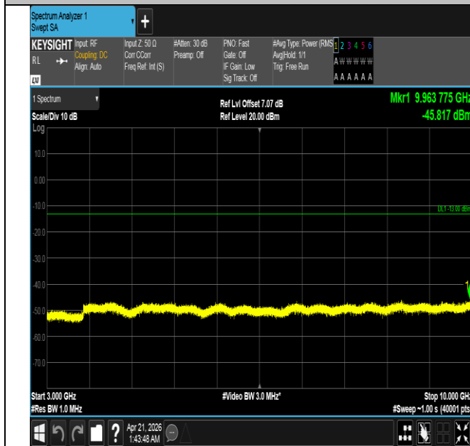
Band26(824-849)-5MHz-QPSK-27015-25RB#0-3000~10000-
