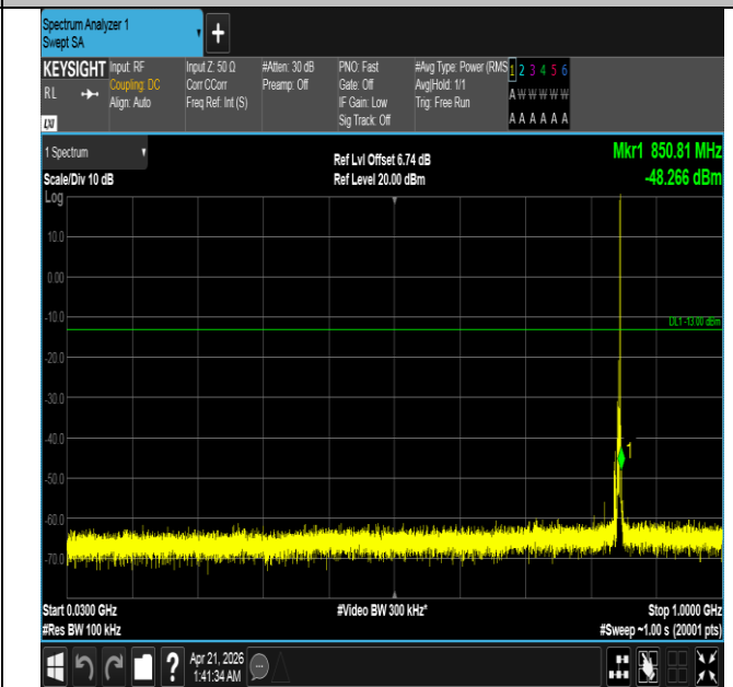
Band26(824-849)-5MHz-QPSK-27015-1RB#24-30~1000-PAS S
