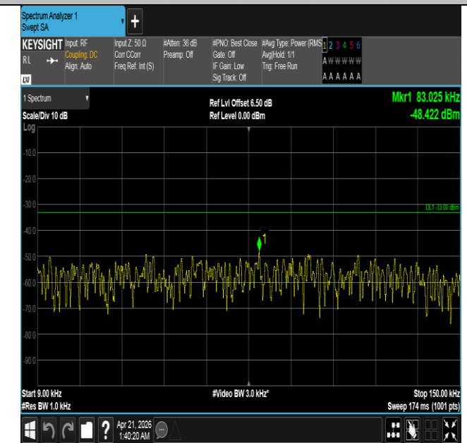
Band26(824-849)-5MHz-16QAM-27015-1RB#0-0.009~0.15-P
