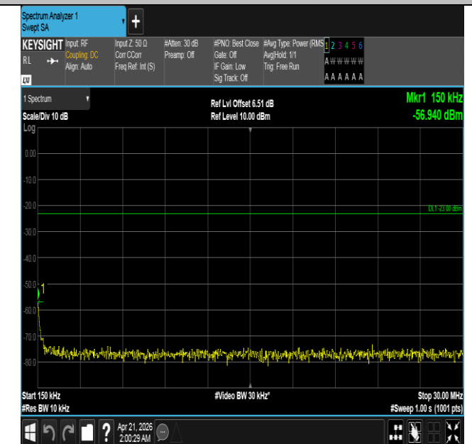
Band26(824-849)-10MHz-QPSK-26840-1RB#0-0.15~30-PAS
