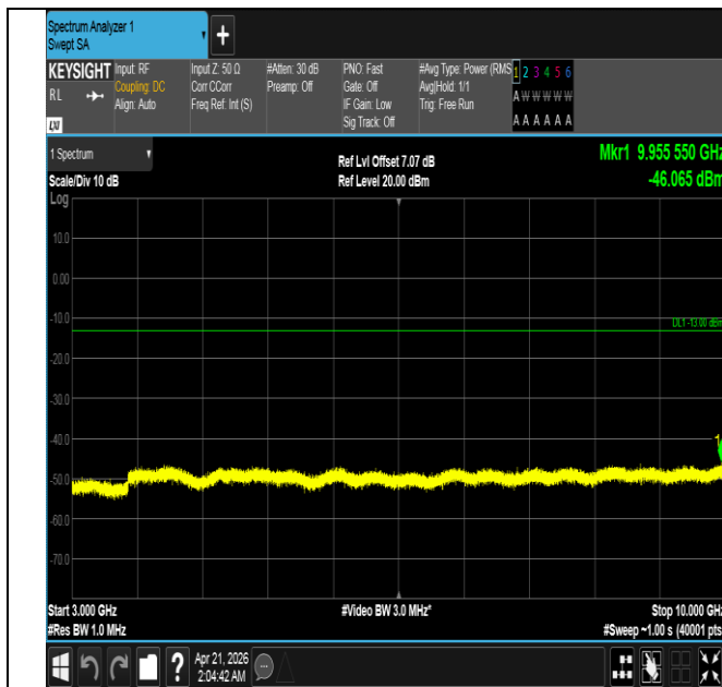
Band26(824-849)-10MHz-QPSK-26840-50RB#0-3000~10000- PASS
