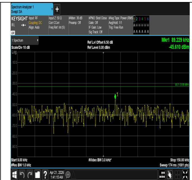
Band26(824-849)-5MHz-QPSK-27015-1RB#24-0.009~0.15-P ASS
