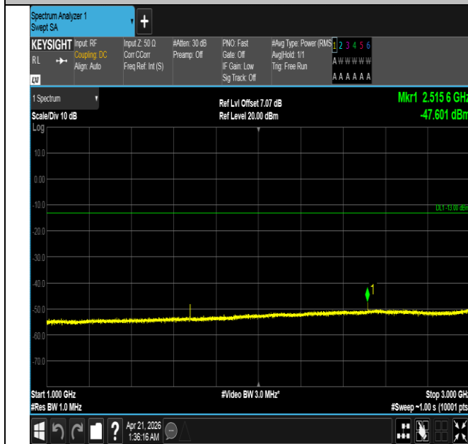
Band26(824-849)-5MHz-QPSK-26915-1RB#24-1000~3000-P
