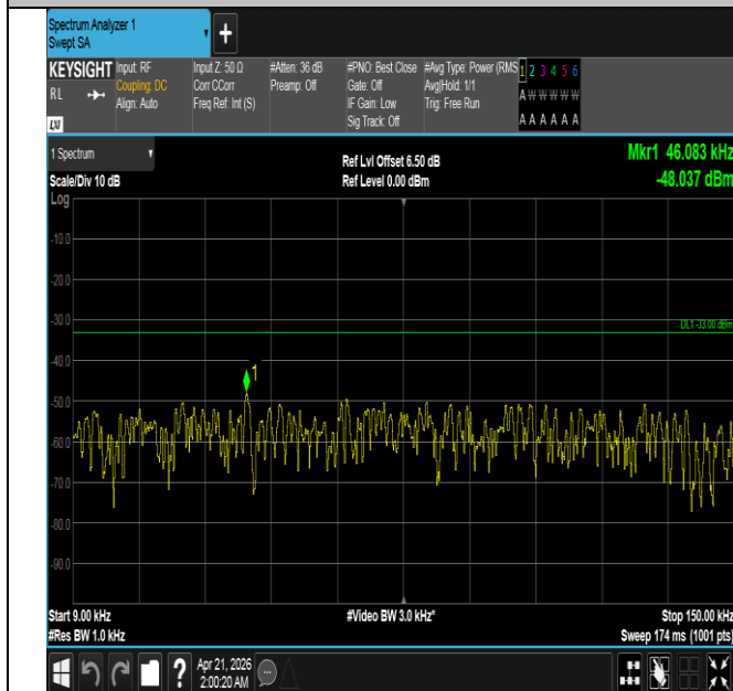
Band26(824-849)-10MHz-QPSK-26840-1RB#0-0.009~0.15-P
