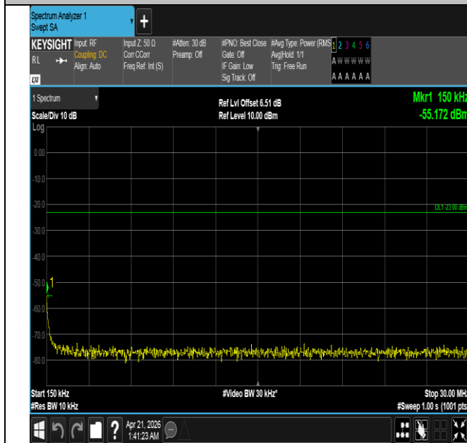
Band26(824-849)-5MHz-QPSK-27015-1RB#24-0.15~30-PAS S
