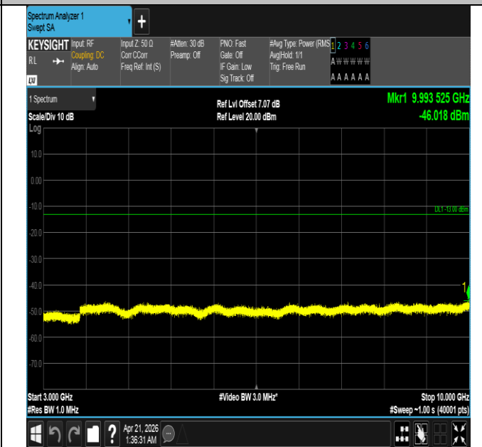
Band26(824-849)-5MHz-QPSK-26915-1RB#24-3000~10000-P
