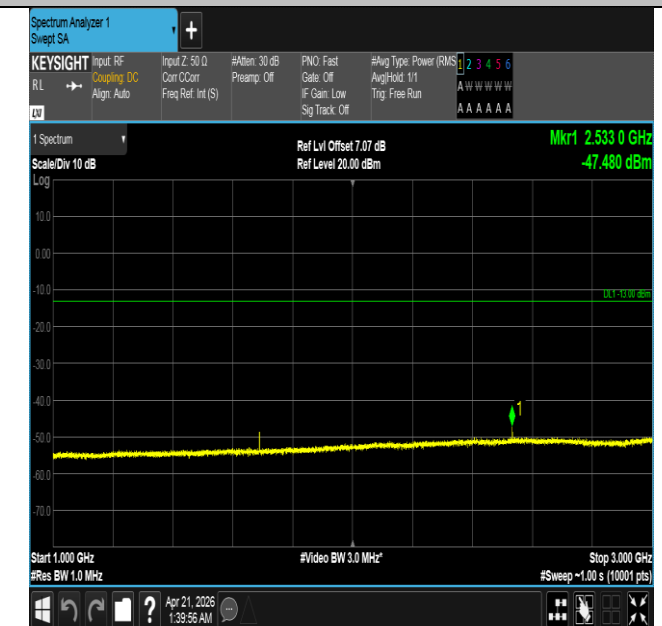
Band26(824-849)-5MHz-QPSK-27015-1RB#0-1000~3000-PA SS
