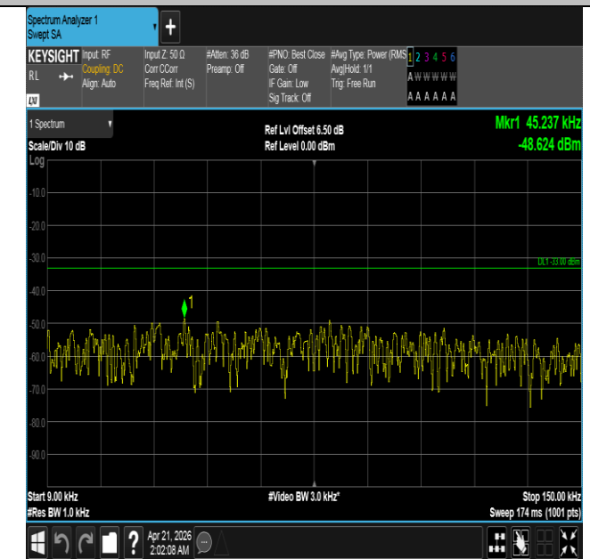
Band26(824-849)-10MHz-QPSK-26840-1RB#49-0.009~0.15-P
