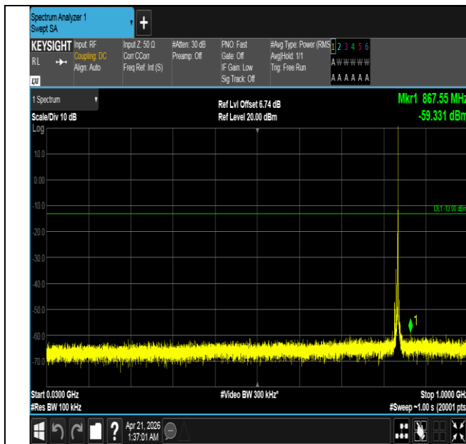
Band26(824-849)-5MHz-16QAM-26915-1RB#24-30~1000-PA SS
