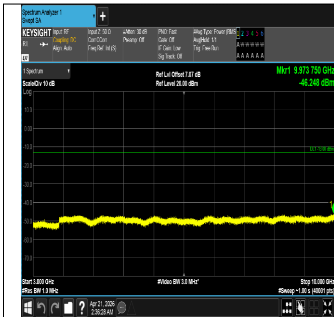
Band26(824-849)-15MHz-16QAM-26865-1RB#74-3000~1000 0-PASS
