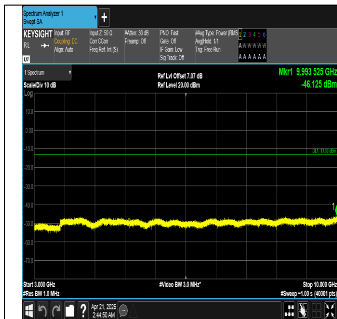
Band26(824-849)-15MHz-QPSK-26965-1RB#0-3000~10000- PASS
