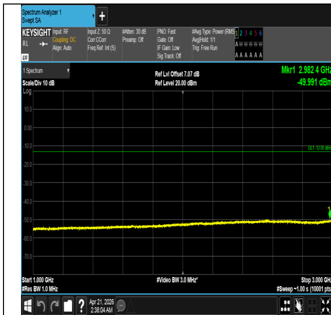
Band26(824-849)-15MHz-16QAM-26865-75RB#0-1000~3000 -PASS
