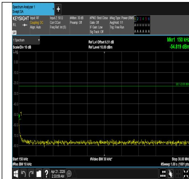
Band26(824-849)-15MHz-16QAM-26865-1RB#0-0.15~30-PA
