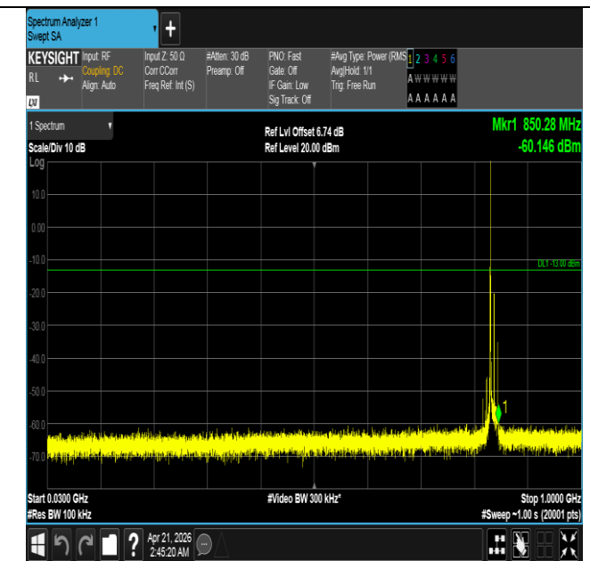
Band26(824-849)-15MHz-16QAM-26965-1RB#0-30~1000-PA
