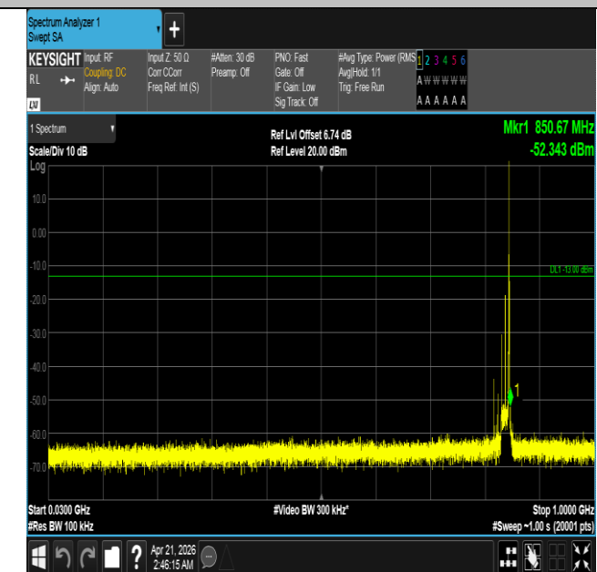
Band26(824-849)-15MHz-QPSK-26965-1RB#74-30~1000-PA SS
