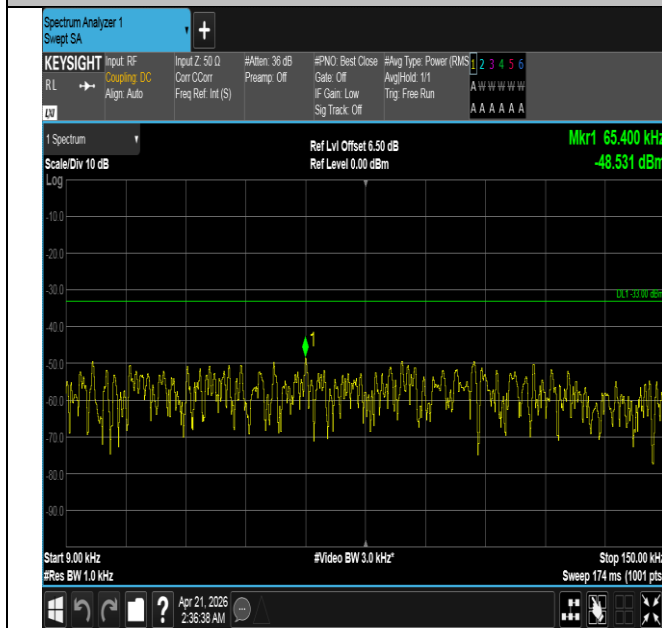
Band26(824-849)-15MHz-QPSK-26865-75RB#0-0.009~0.15- PASS
