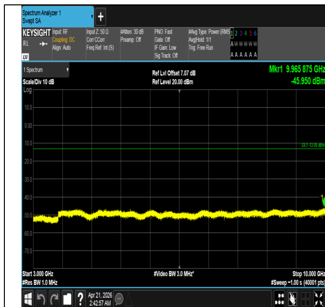
Band26(824-849)-15MHz-QPSK-26915-75RB#0-3000~10000- PASS
