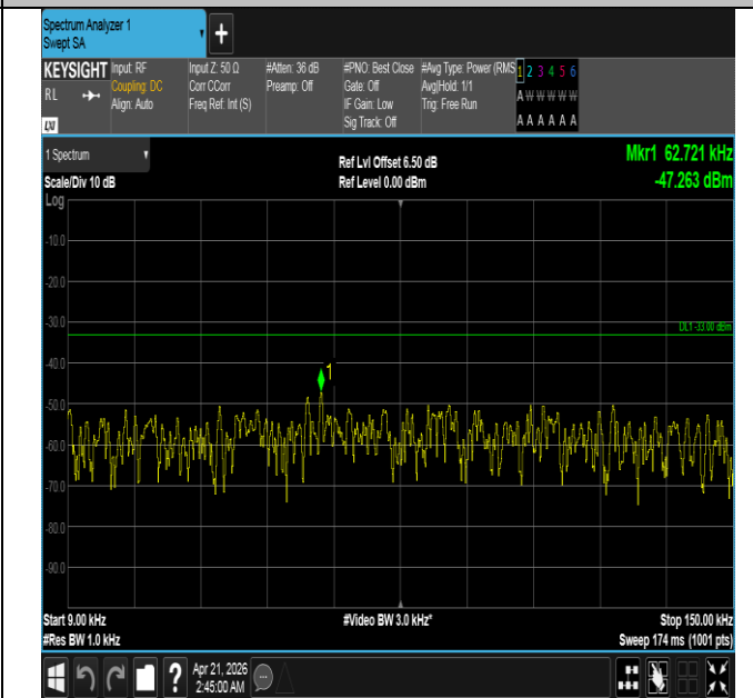
Band26(824-849)-15MHz-16QAM-26965-1RB#0-0.009~0.15- PASS
