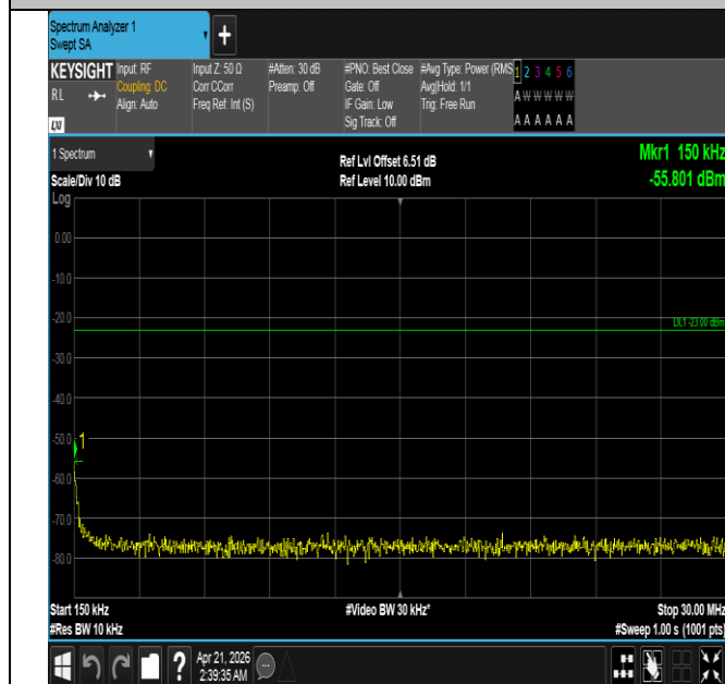
Band26(824-849)-15MHz-16QAM-26915-1RB#0-0.15~30-PA SS
