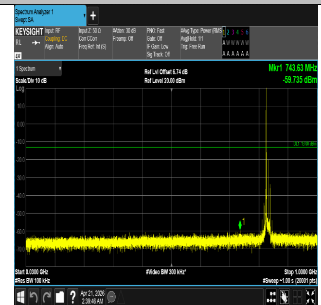
Band26(824-849)-15MHz-16QAM-26915-1RB#0-30~1000-PA SS
