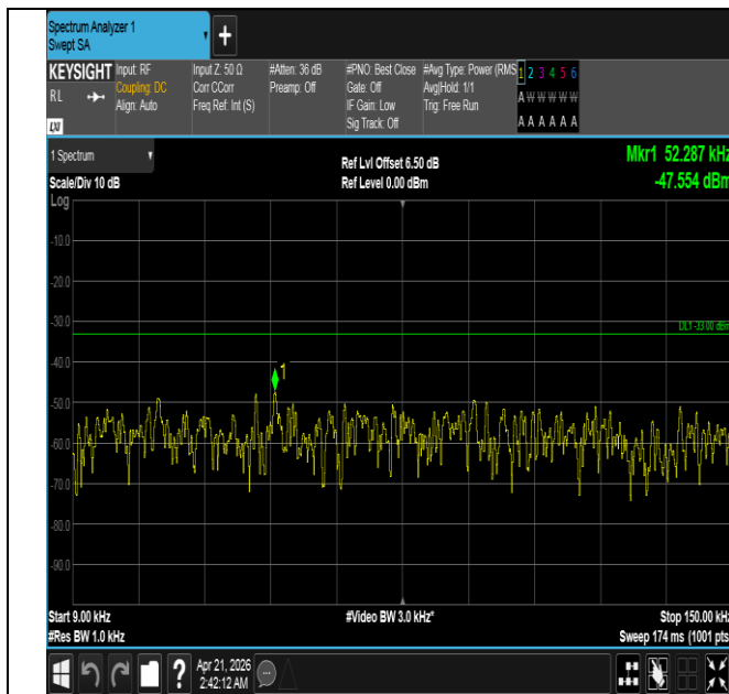
Band26(824-849)-15MHz-QPSK-26915-75RB#0-0.009~0.15- PASS
