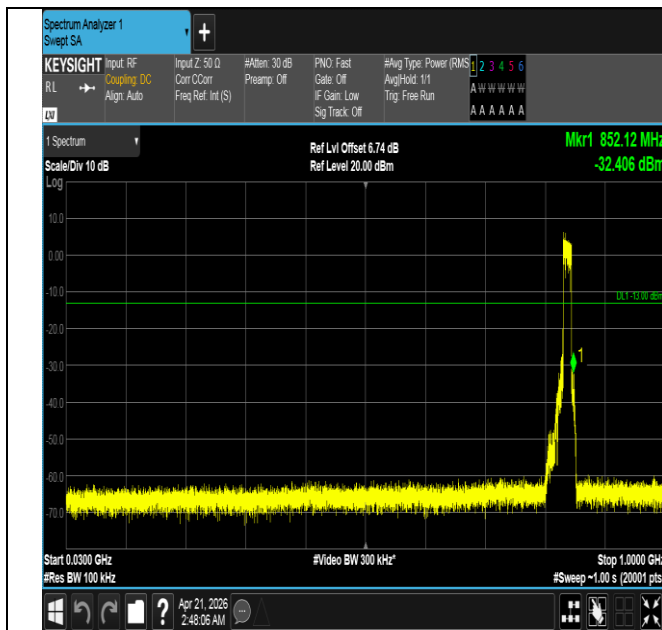
Band26(824-849)-15MHz-QPSK-26965-75RB#0-30~1000-PA SS
