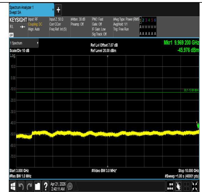
Band26(824-849)-15MHz-16QAM-26915-1RB#0-3000~10000 -PASS
