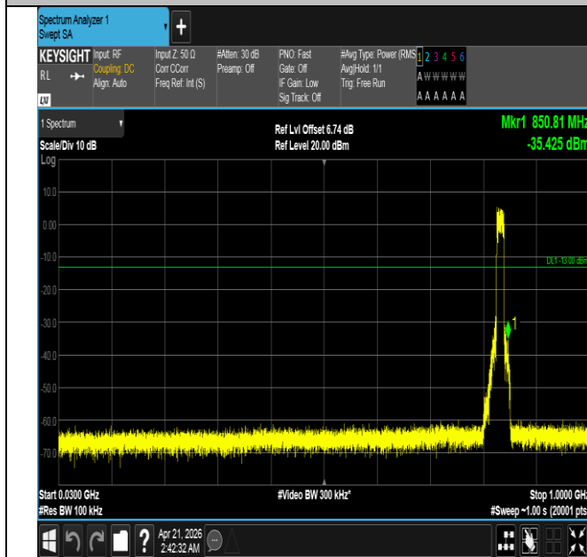
Band26(824-849)-15MHz-QPSK-26915-75RB#0-30~1000-PA SS
