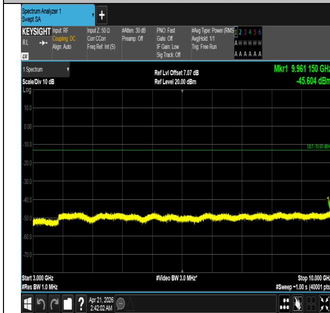
Band26(824-849)-15MHz-16QAM-26915-1RB#74-3000~1000 0-PASS
