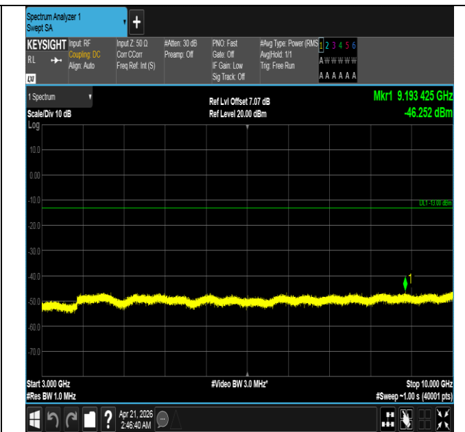
Band26(824-849)-15MHz-QPSK-26965-1RB#74-3000~10000- PASS
