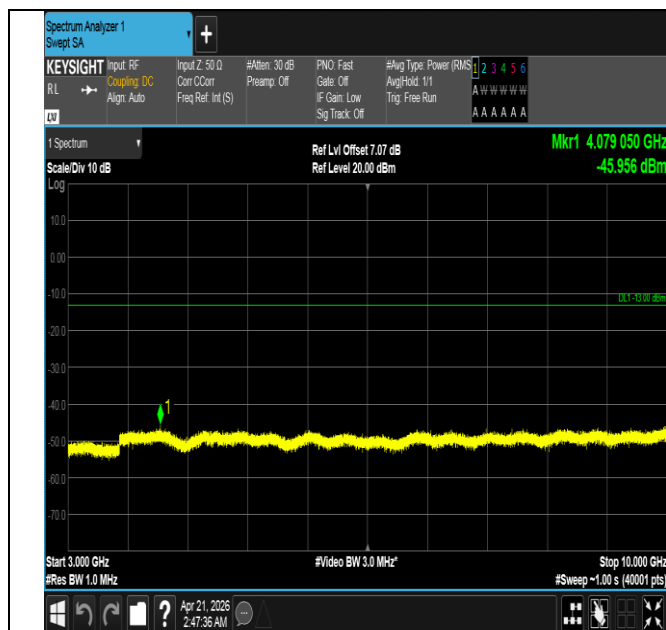
Band26(824-849)-15MHz-16QAM-26965-1RB#74-3000~1000 0-PASS
