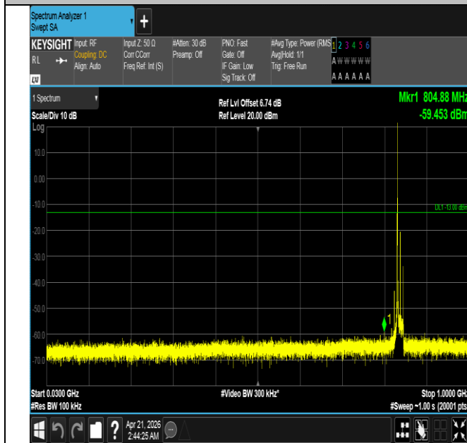
Band26(824-849)-15MHz-QPSK-26965-1RB#0-30~1000-PAS S
