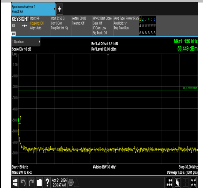
Band26(824-849)-15MHz-QPSK-26865-75RB#0-0.15~30-PAS S
