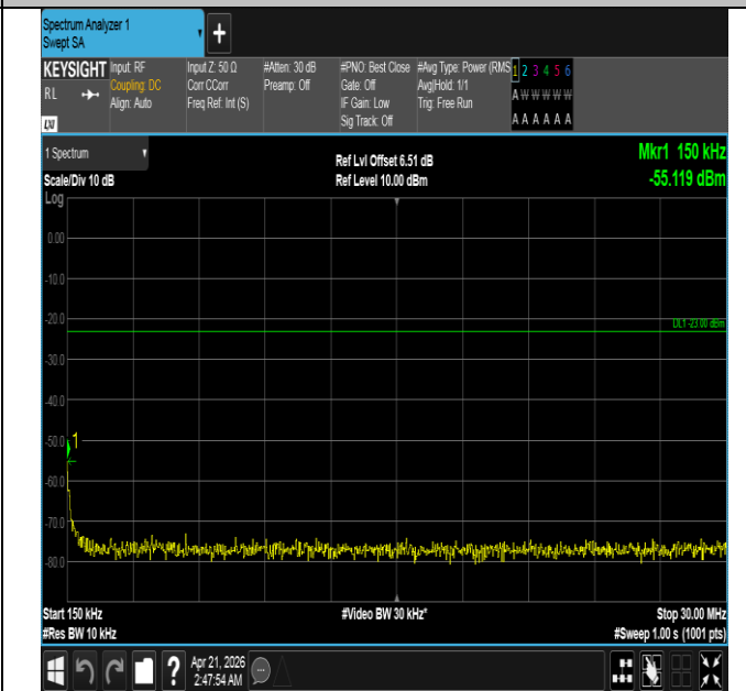
Band26(824-849)-15MHz-QPSK-26965-75RB#0-0.15~30-PAS S
