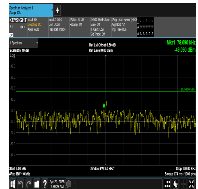
Band26(824-849)-15MHz-16QAM-26915-1RB#0-0.009~0.15- PASS
