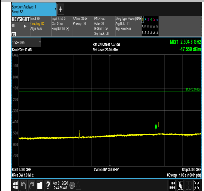
Band26(824-849)-15MHz-QPSK-26965-1RB#0-1000~3000-P ASS
