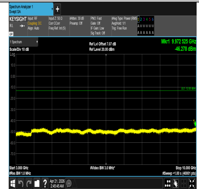
Band26(824-849)-15MHz-16QAM-26965-1RB#0-3000~10000
