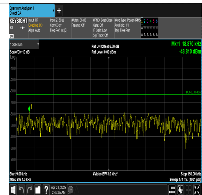
Band26(824-849)-15MHz-QPSK-26965-1RB#74-0.009~0.15-P ASS
