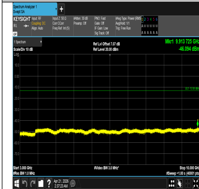
Band26(824-849)-15MHz-QPSK-26865-75RB#0-3000~10000- PASS
