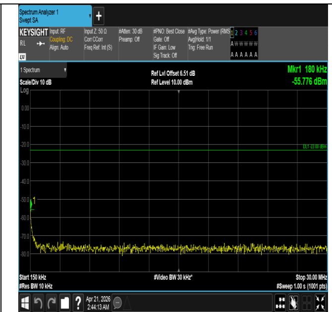
Band26(824-849)-15MHz-QPSK-26965-1RB#0-0.15~30-PAS S
