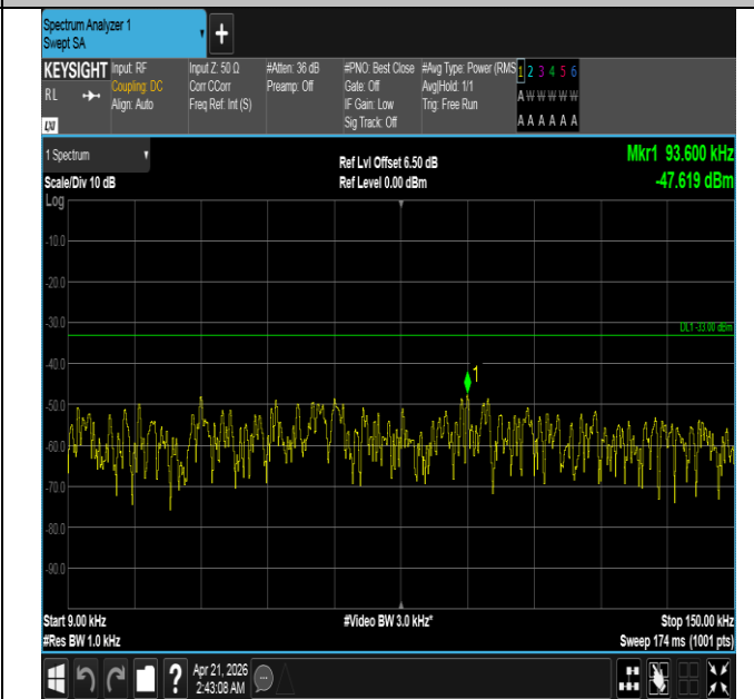
Band26(824-849)-15MHz-16QAM-26915-75RB#0-0.009~0.15 -PASS
