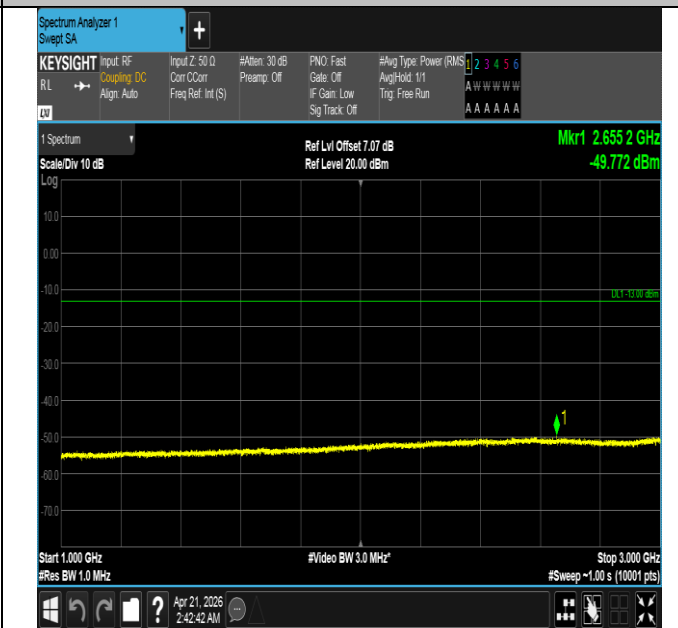
Band26(824-849)-15MHz-QPSK-26915-75RB#0-1000~3000-P ASS
