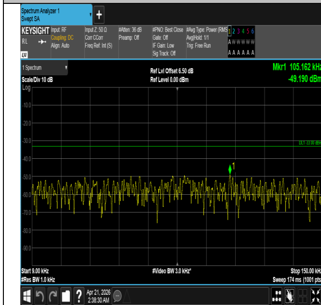
Band26(824-849)-15MHz-QPSK-26915-1RB#0-0.009~0.15-P ASS
