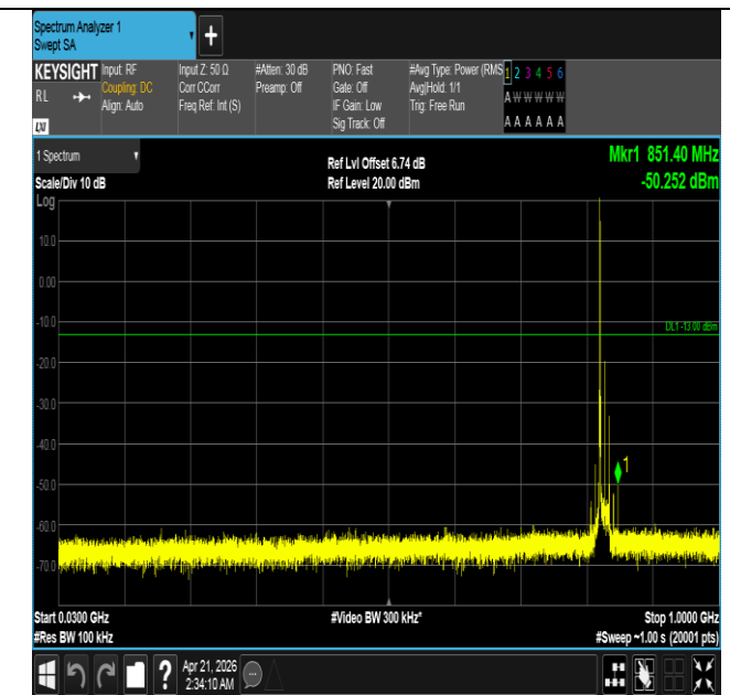
Band26(824-849)-15MHz-16QAM-26865-1RB#0-30~1000-PA
