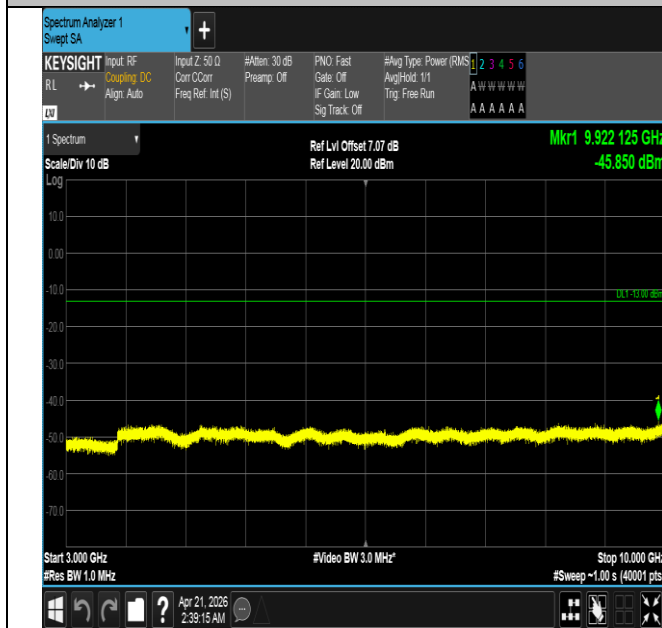
Band26(824-849)-15MHz-QPSK-26915-1RB#0-3000~10000-
