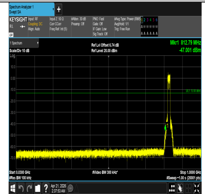
Band26(824-849)-15MHz-16QAM-26865-75RB#0-30~1000-P ASS
