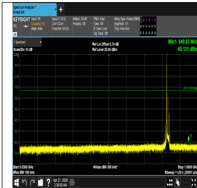
Band26(824-849)-15MHz-QPSK-26915-1RB#0-30~1000-PAS
