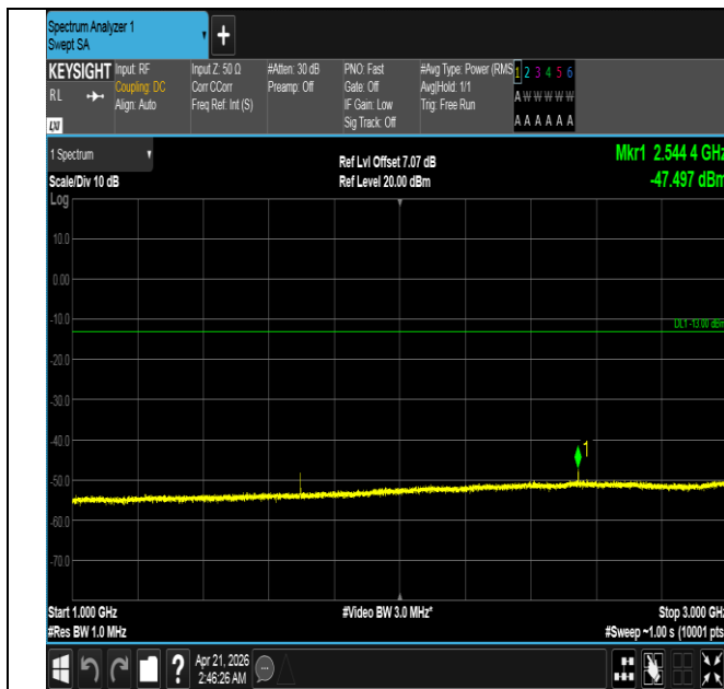
Band26(824-849)-15MHz-QPSK-26965-1RB#74-1000~3000- PASS
