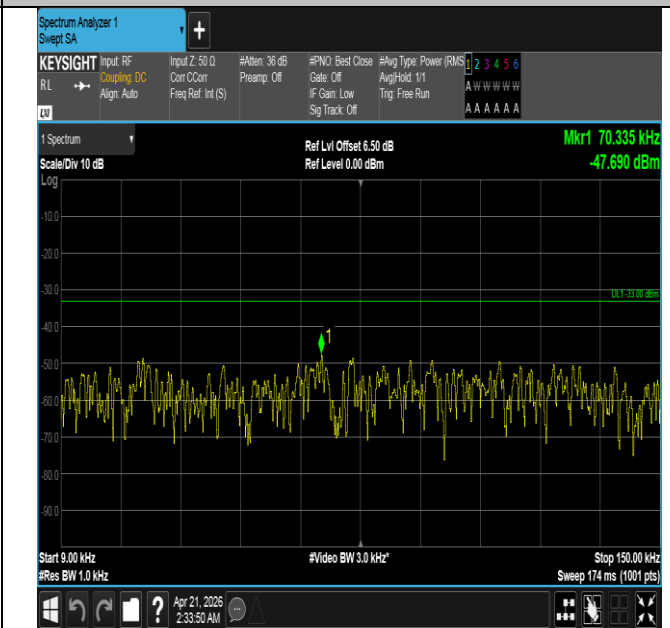
Band26(824-849)-15MHz-16QAM-26865-1RB#0-0.009~0.15- PASS
