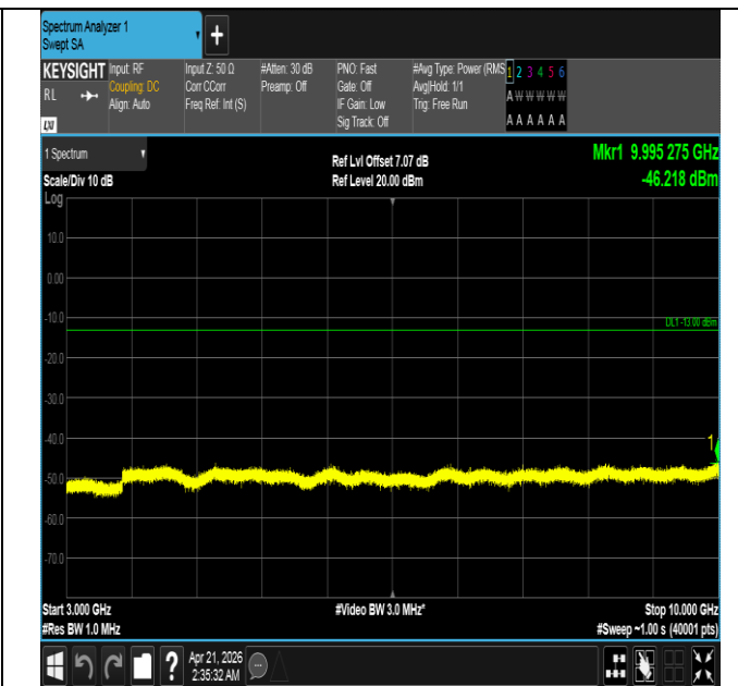
Band26(824-849)-15MHz-QPSK-26865-1RB#74-3000~10000- PASS
