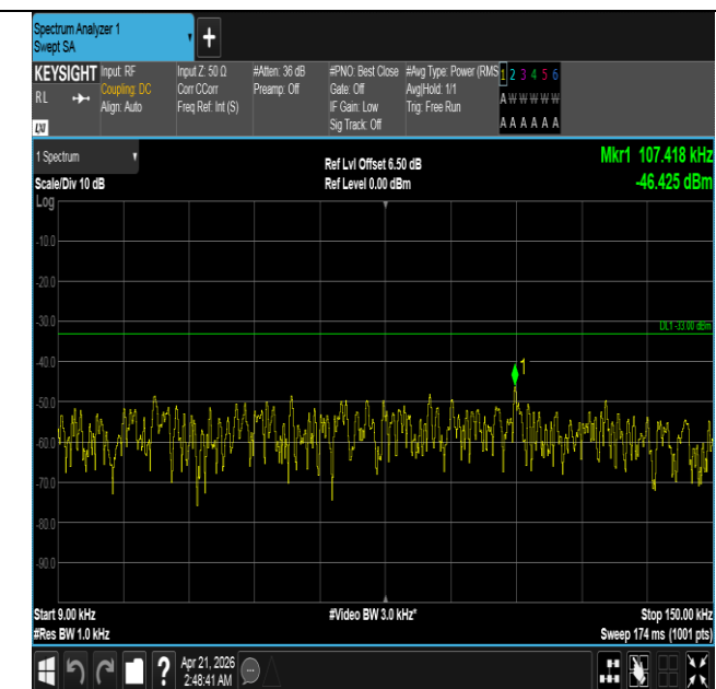
Band26(824-849)-15MHz-16QAM-26965-75RB#0-0.009~0.15 -PASS
