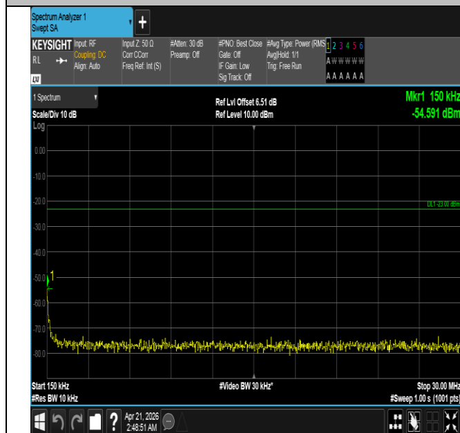
Band26(824-849)-15MHz-16QAM-26965-75RB#0-0.15~30-PA SS
