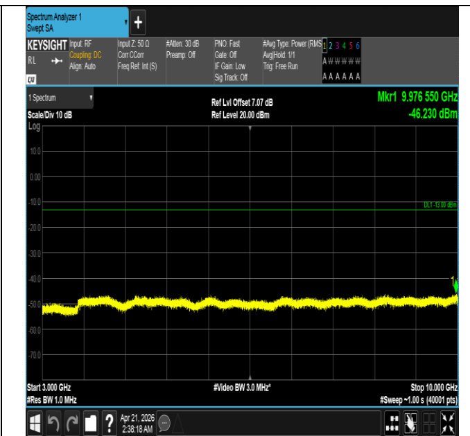
Band26(824-849)-15MHz-16QAM-26865-75RB#0-3000~1000 0-PASS
