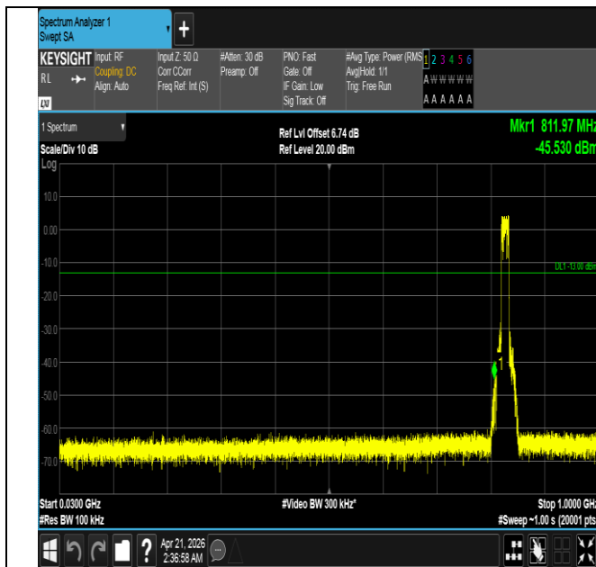
Band26(824-849)-15MHz-QPSK-26865-75RB#0-30~1000-PA SS
