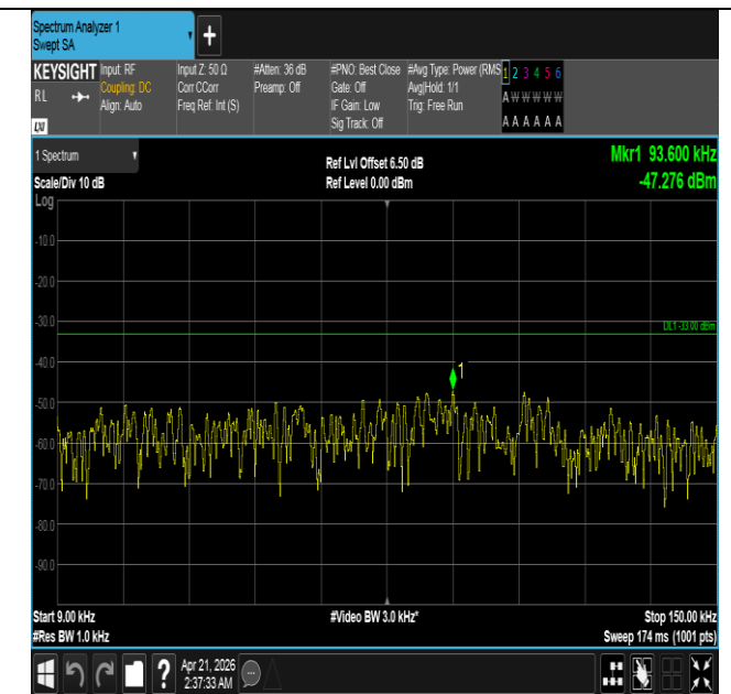
Band26(824-849)-15MHz-16QAM-26865-75RB#0-0.009~0.15 -PASS
