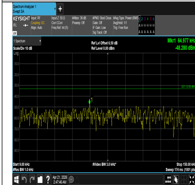
Band26(824-849)-15MHz-QPSK-26965-75RB#0-0.009~0.15- PASS
