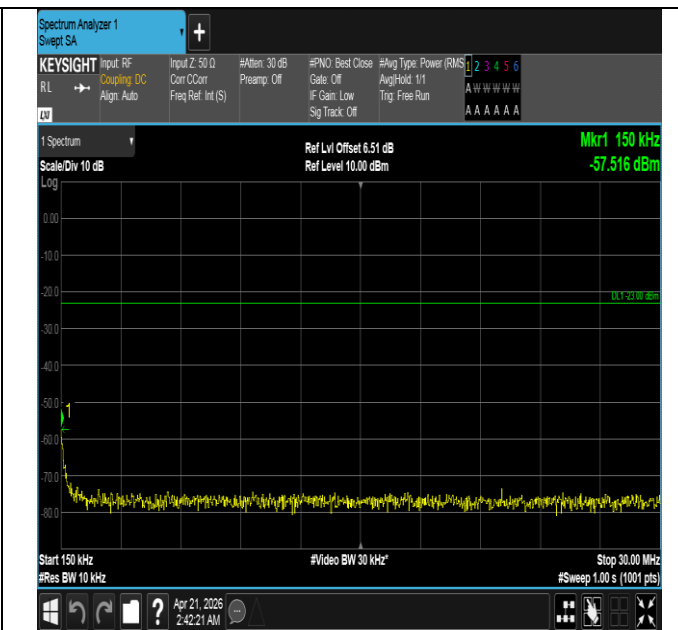
Band26(824-849)-15MHz-QPSK-26915-75RB#0-0.15~30-PAS S
