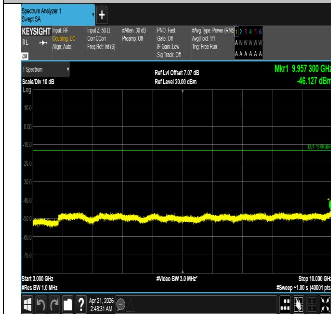
Band26(824-849)-15MHz-QPSK-26965-75RB#0-3000~10000- PASS
