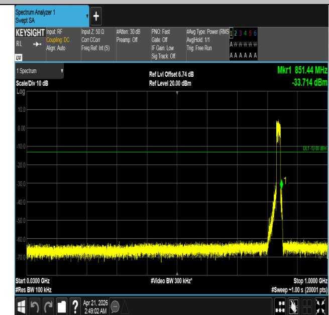
Band26(824-849)-15MHz-16QAM-26965-75RB#0-30~1000-P ASS
