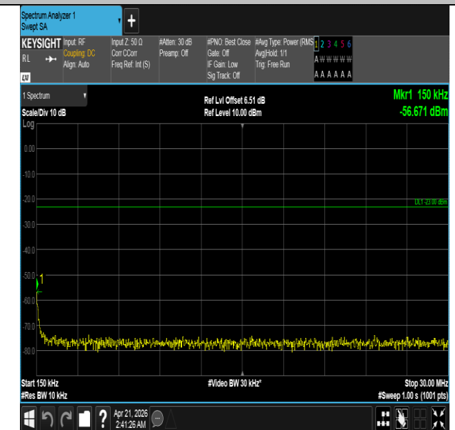
Band26(824-849)-15MHz-16QAM-26915-1RB#74-0.15~30-PA SS
