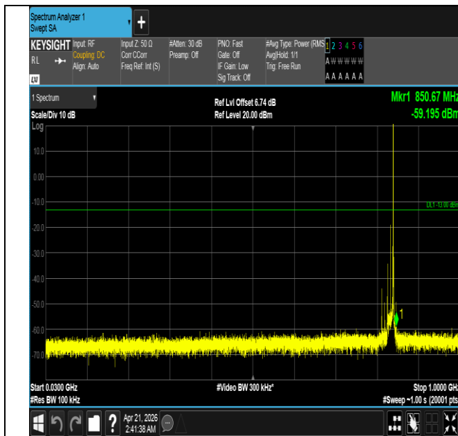
Band26(824-849)-15MHz-16QAM-26915-1RB#74-30~1000-P ASS
