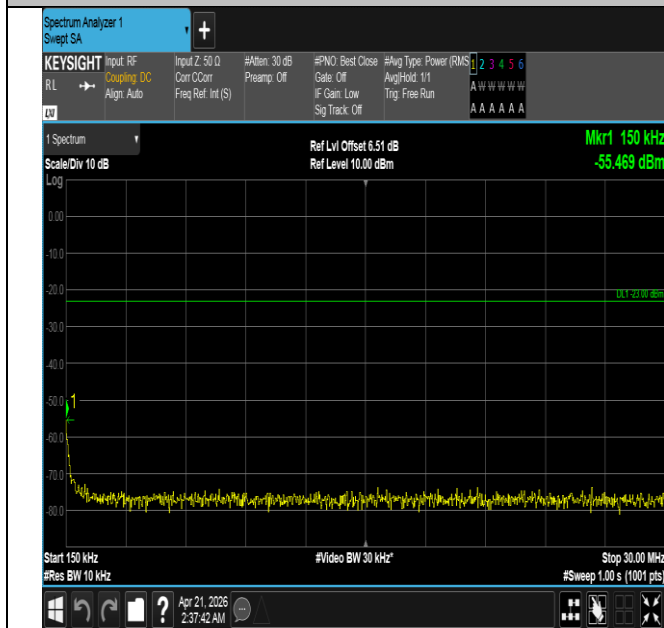
Band26(824-849)-15MHz-16QAM-26865-75RB#0-0.15~30-PA SS
