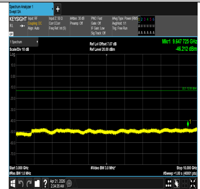
Band26(824-849)-15MHz-16QAM-26865-1RB#0-3000~10000
