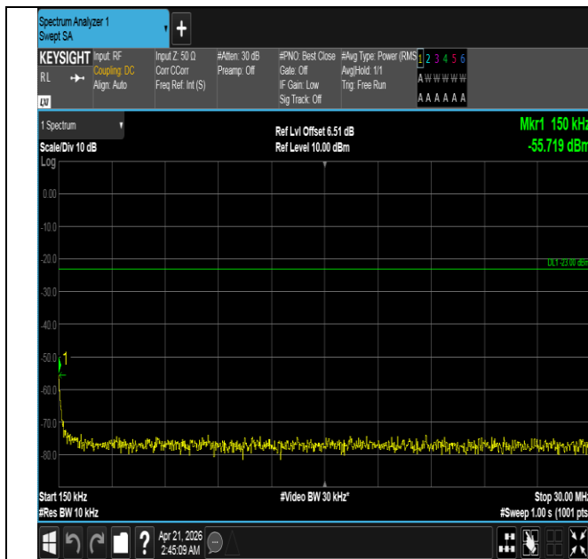
Band26(824-849)-15MHz-16QAM-26965-1RB#0-0.15~30-PA
