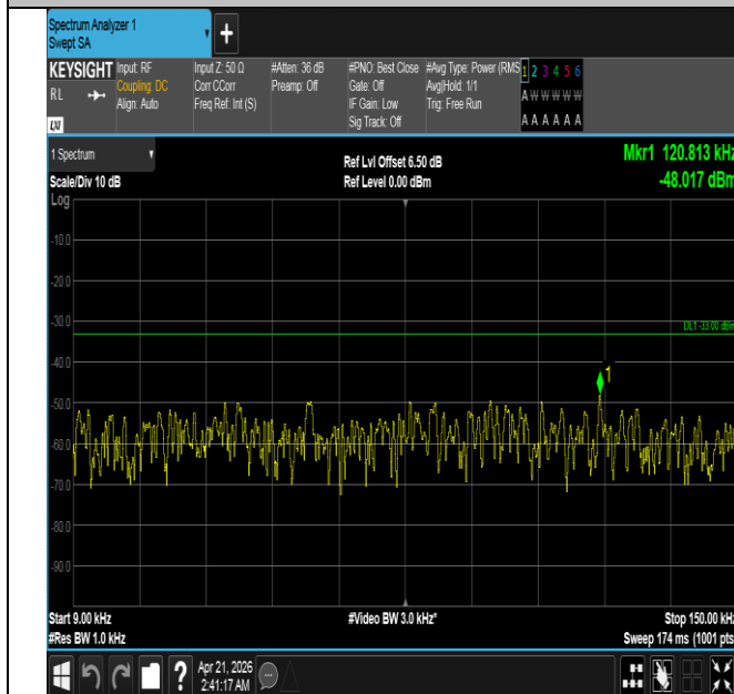
Band26(824-849)-15MHz-16QAM-26915-1RB#74-0.009~0.15 -PASS
