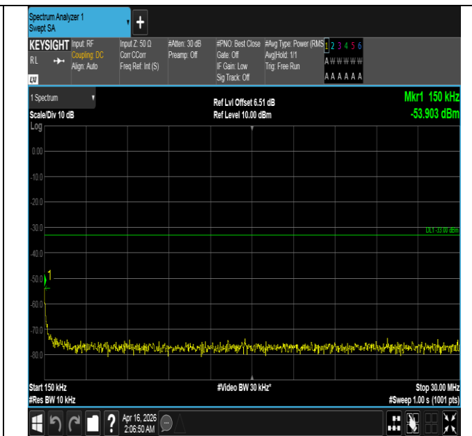
Band4-20MHz-16QAM-20175-1RB#99-0.15~30-PASS
