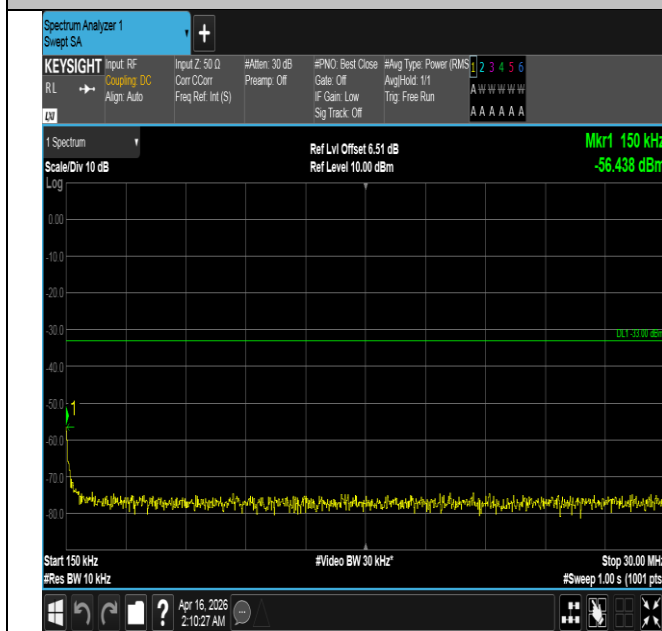
Band4-20MHz-16QAM-20300-1RB#0-0.15~30-PASS
