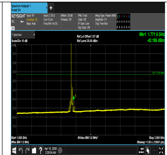
Band4-20MHz-QPSK-20300-1RB#0-1000~3000-PASS
