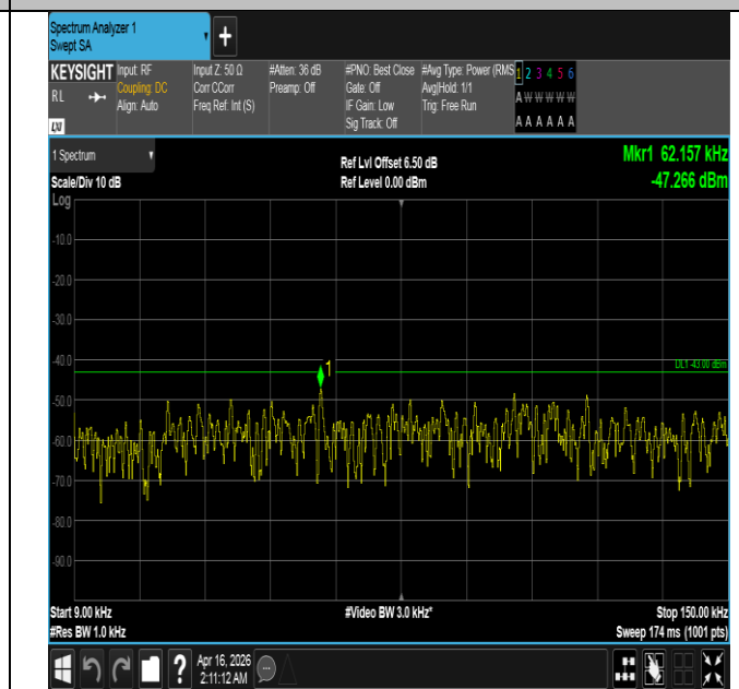
Band4-20MHz-QPSK-20300-1RB#99-0.009~0.15-PASS
