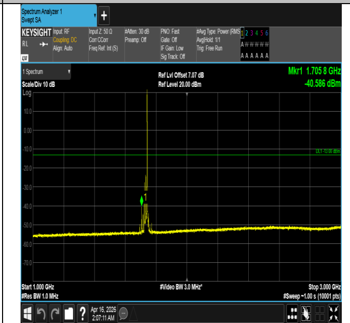
Band4-20MHz-16QAM-20175-1RB#99-1000~3000-PASS
