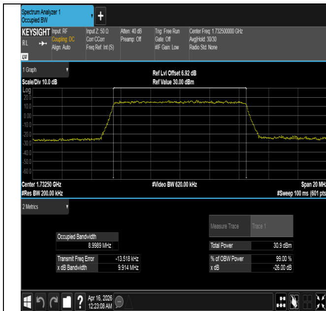
Band4-10MHz-QPSK-20175-50RB#0-PASS
