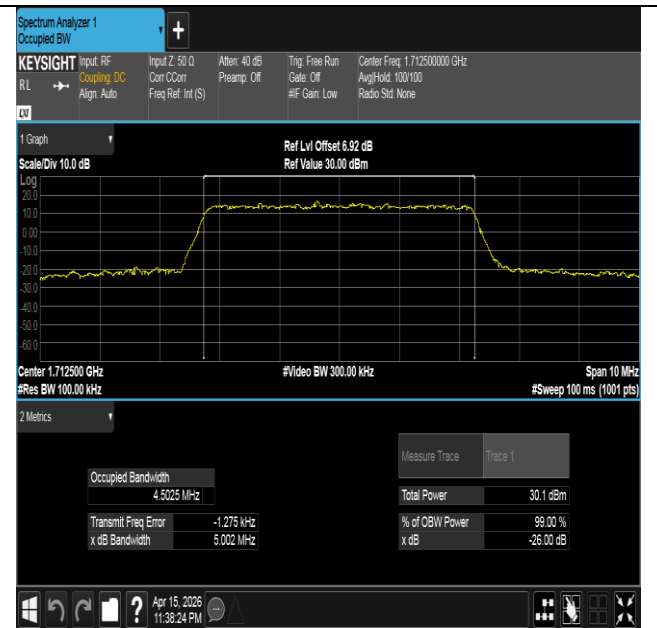
Band4-5MHz-16QAM-19975-25RB#0-PASS
