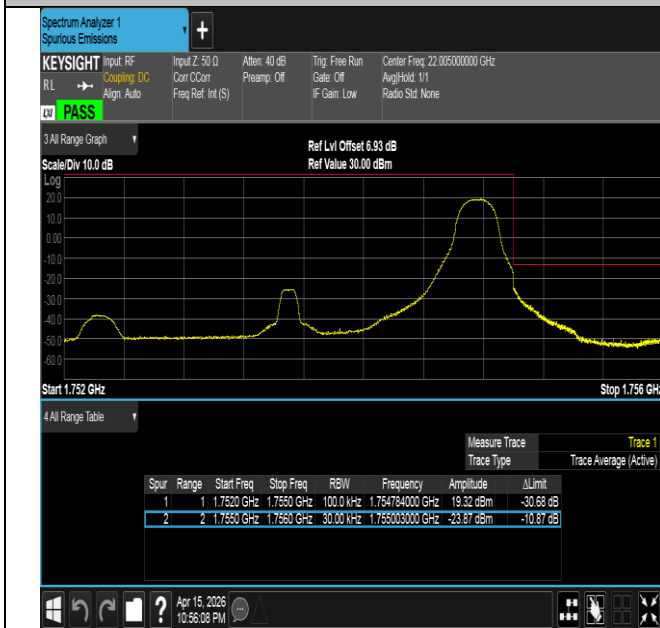
Band4-3MHz-16QAM-20385-1RB#14-PASS
