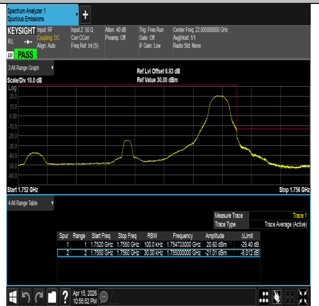
Band4-3MHz-QPSK-20385-1RB#14-PASS
