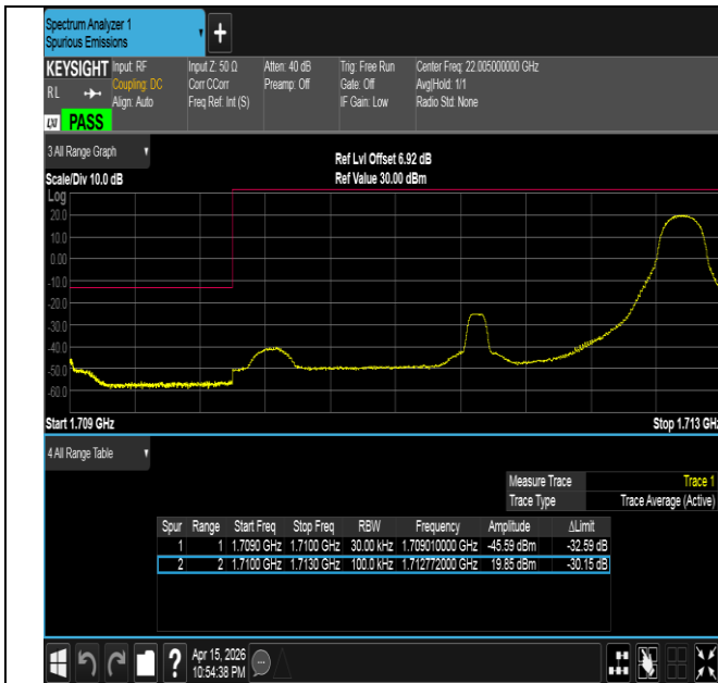
Band4-3MHz-16QAM-19965-1RB#14-PASS
