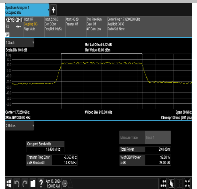
Band4-15MHz-16QAM-20175-75RB#0-PASS
