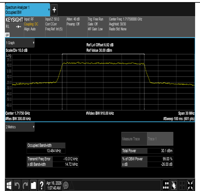
Band4-15MHz-16QAM-20025-75RB#0-PASS
