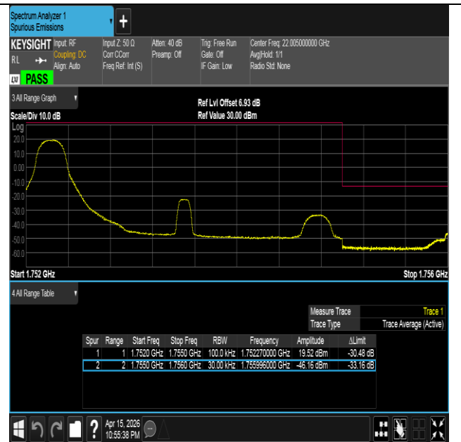
Band4-3MHz-16QAM-20385-1RB#0-PASS
