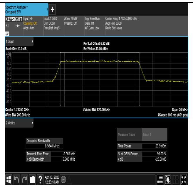
Band4-10MHz-16QAM-20175-50RB#0-PASS
