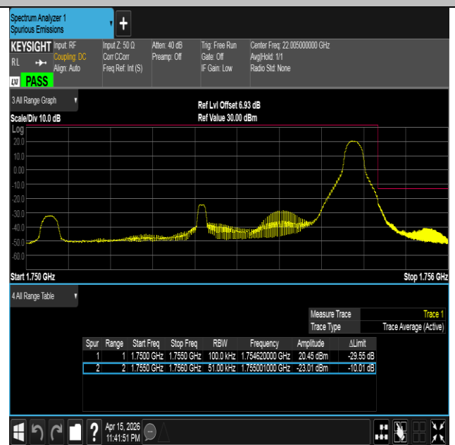
Band4-5MHz-QPSK-20375-1RB#24-PASS
