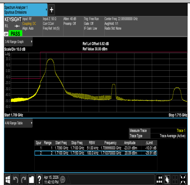
Band4-5MHz-16QAM-19975-1RB#0-PASS
