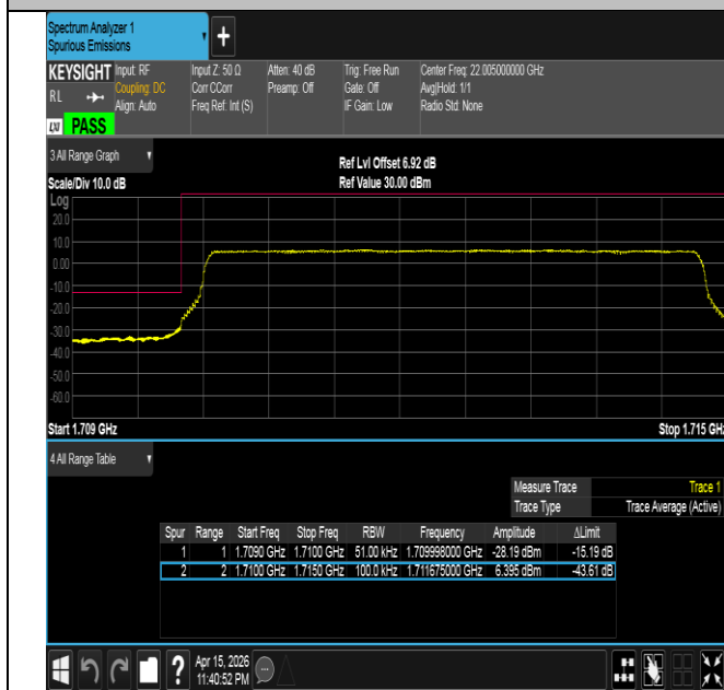
Band4-5MHz-QPSK-19975-25RB#0-PASS
