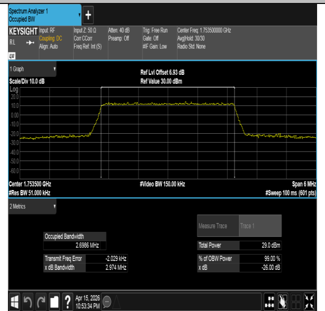
Band4-3MHz-16QAM-20385-15RB#0-PASS
