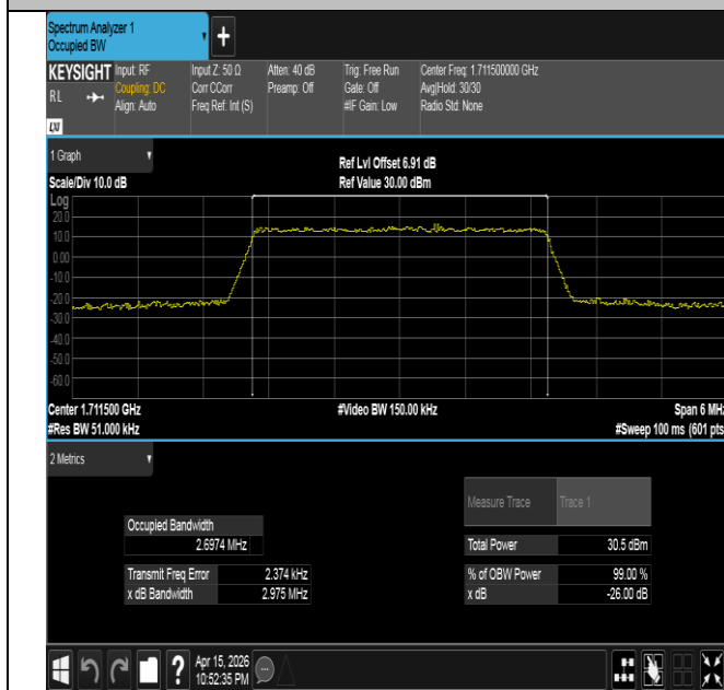
Band4-3MHz-QPSK-19965-15RB#0-PASS
