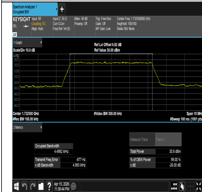
Band4-5MHz-QPSK-20175-25RB#0-PASS
