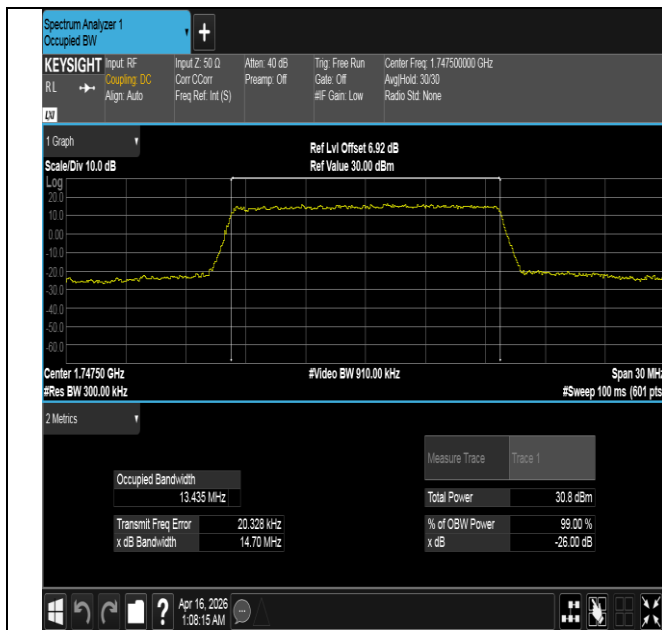
Band4-15MHz-QPSK-20325-75RB#0-PASS
