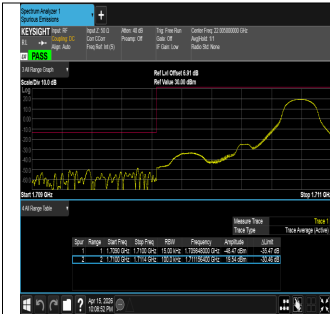
Band4-1.4MHz-16QAM-19957-1RB#5-PASS
