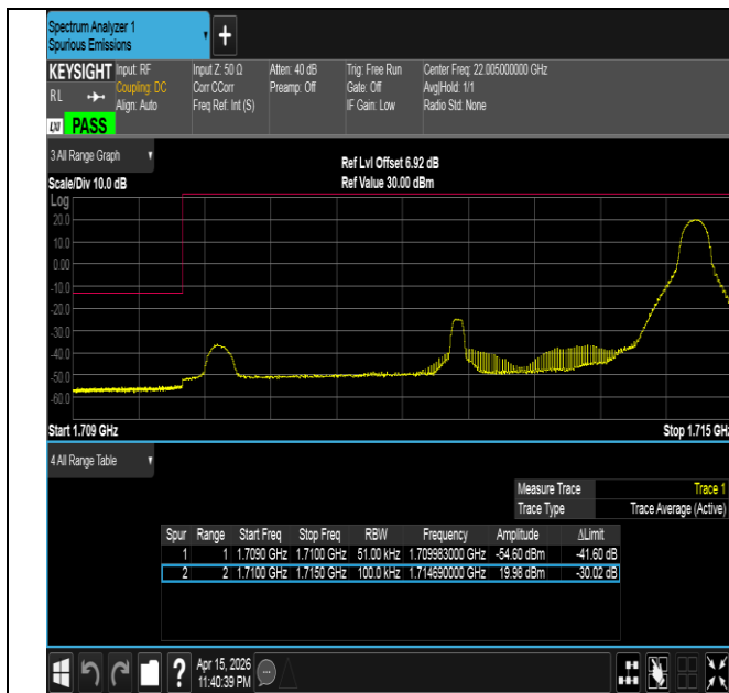
Band4-5MHz-16QAM-19975-1RB#24-PASS
