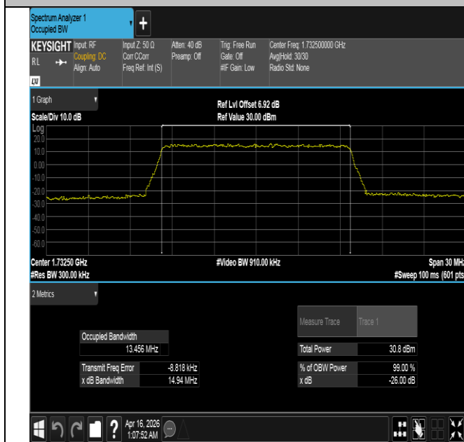
Band4-15MHz-QPSK-20175-75RB#0-PASS
