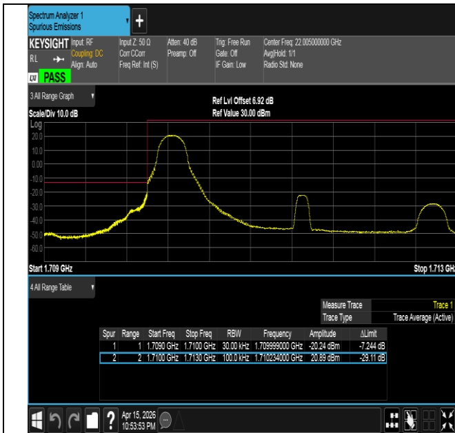
Band4-3MHz-QPSK-19965-1RB#0-PASS
