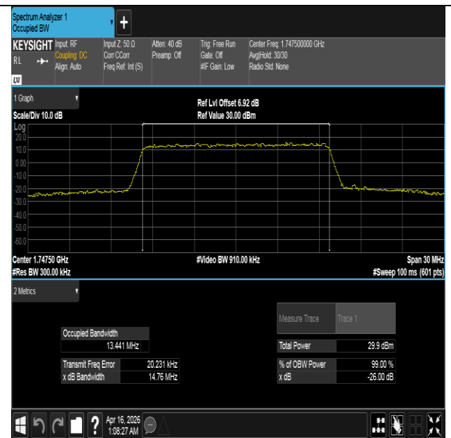
Band4-15MHz-16QAM-20325-75RB#0-PASS
