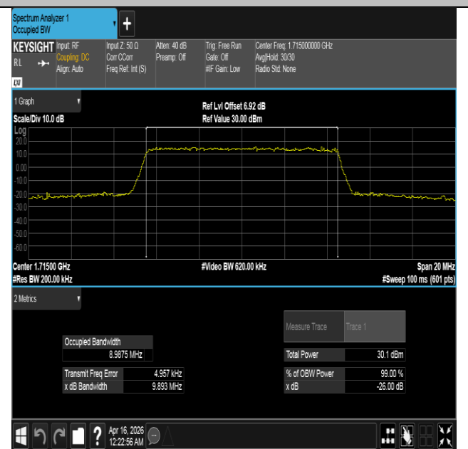
Band4-10MHz-16QAM-20000-50RB#0-PASS
