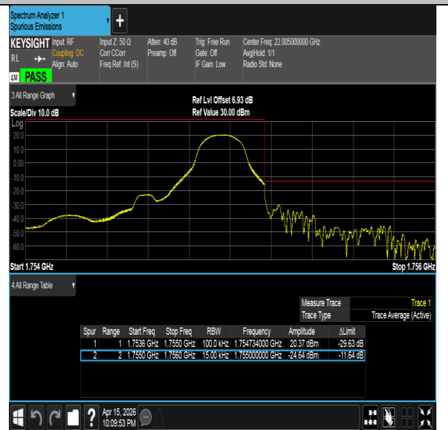
Band4-1.4MHz-QPSK-20393-1RB#5-PASS
