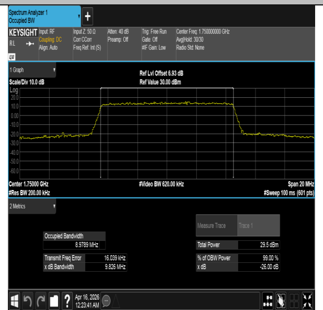
Band4-10MHz-16QAM-20350-50RB#0-PASS
