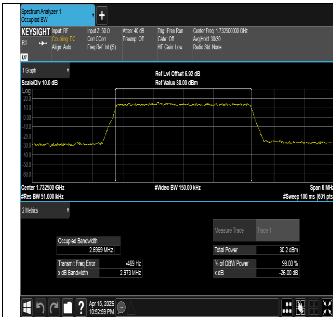
Band4-3MHz-QPSK-20175-15RB#0-PASS
