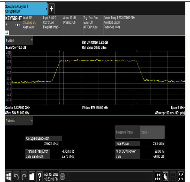
Band4-3MHz-16QAM-20175-15RB#0-PASS
