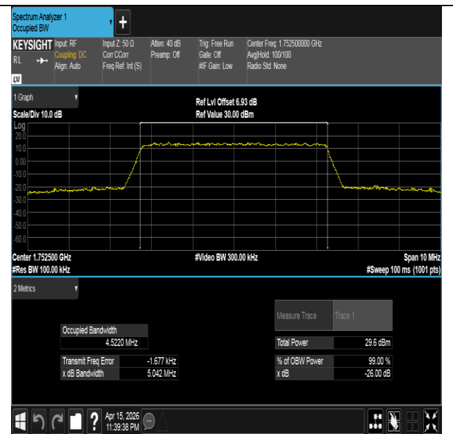
Band4-5MHz-16QAM-20375-25RB#0-PASS
