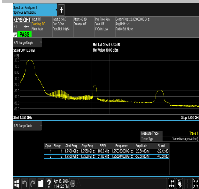
Band4-5MHz-QPSK-20375-1RB#0-PASS
