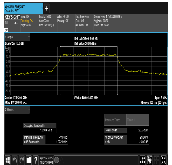
Band4-1.4MHz-16QAM-20393-6RB#0-PASS
