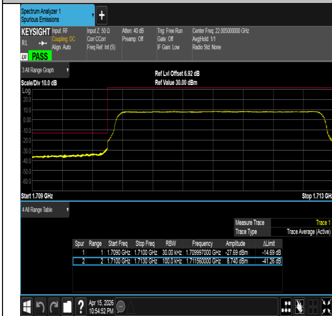
Band4-3MHz-QPSK-19965-15RB#0-PASS
