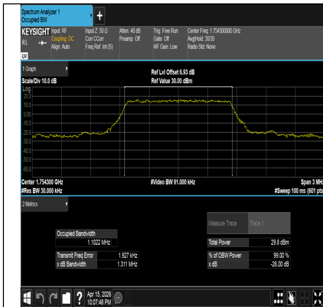
Band4-1.4MHz-QPSK-20393-6RB#0-PASS
