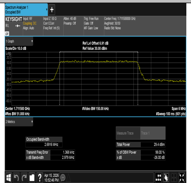
Band4-3MHz-16QAM-19965-15RB#0-PASS
