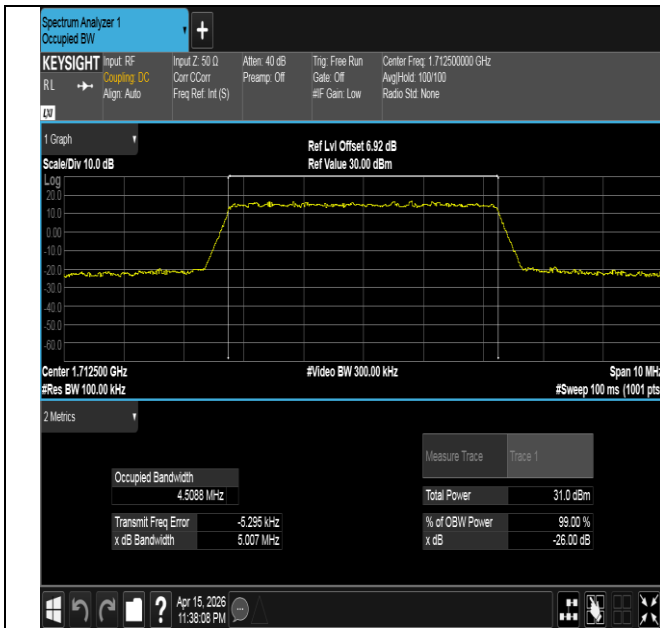
Band4-5MHz-QPSK-19975-25RB#0-PASS
