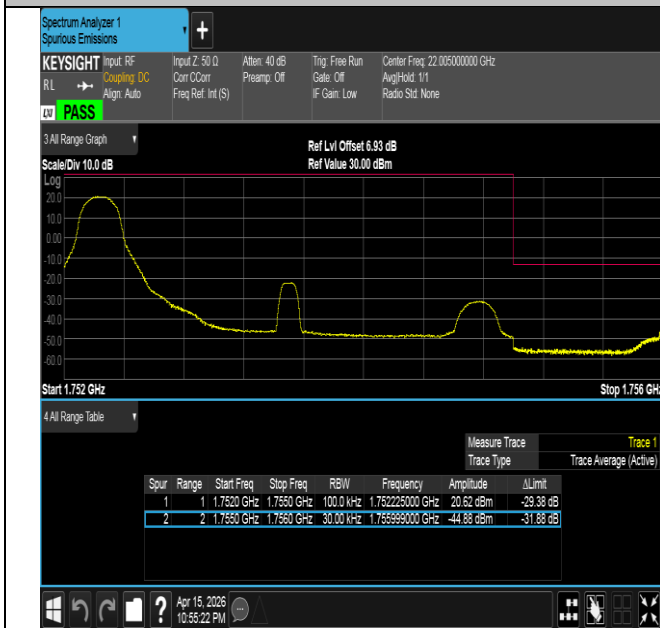
Band4-3MHz-QPSK-20385-1RB#0-PASS
