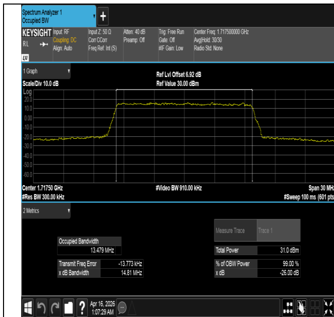
Band4-15MHz-QPSK-20025-75RB#0-PASS
