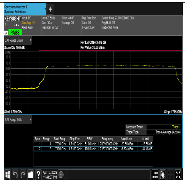
Band4-5MHz-16QAM-19975-25RB#0-PASS
