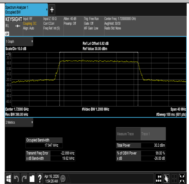
Band4-20MHz-16QAM-20050-100RB#0-PASS
