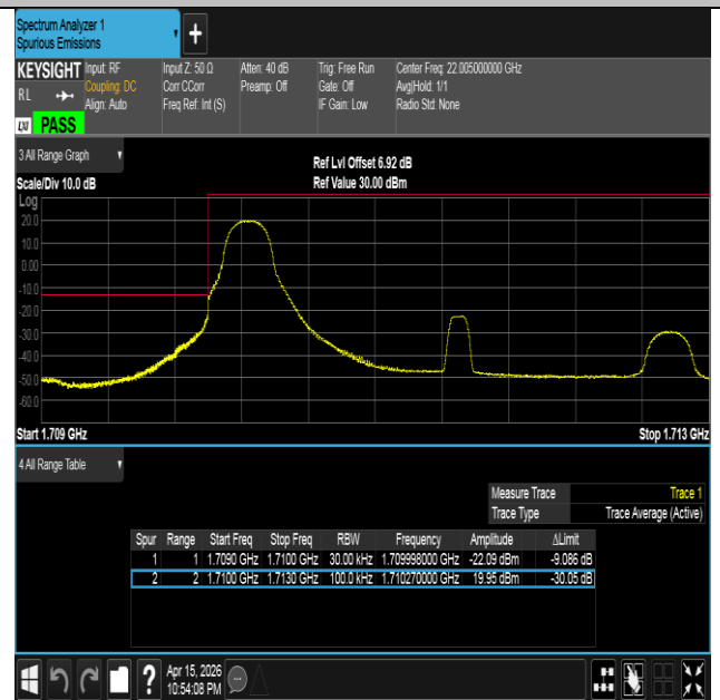
Band4-3MHz-16QAM-19965-1RB#0-PASS
