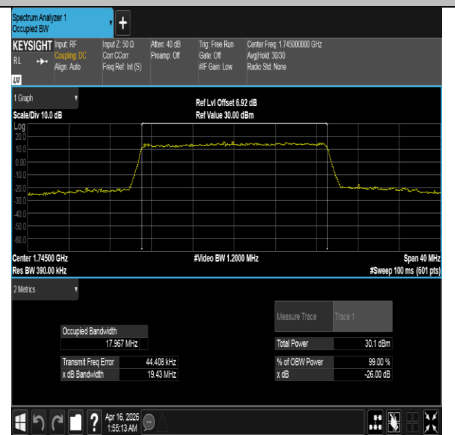
Band4-20MHz-16QAM-20300-100RB#0-PASS
