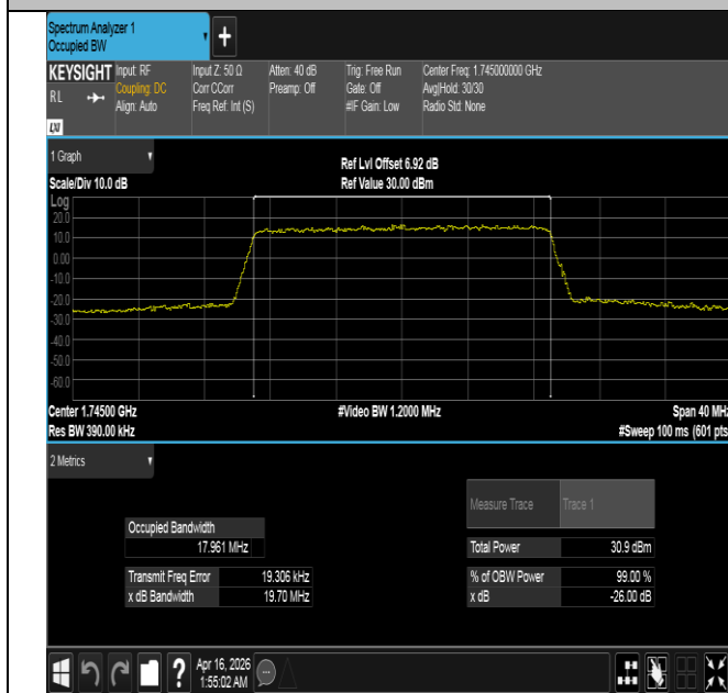
Band4-20MHz-QPSK-20300-100RB#0-PASS
