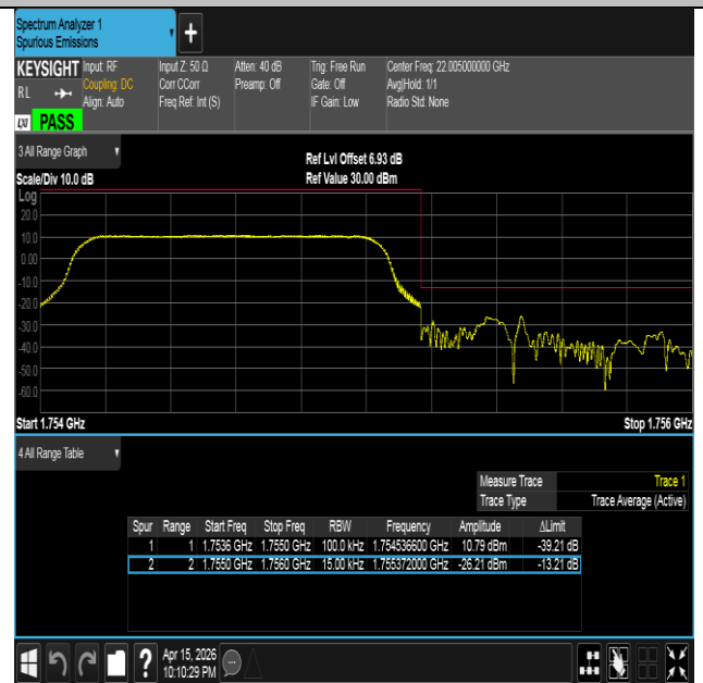
Band4-1.4MHz-16QAM-20393-6RB#0-PASS
