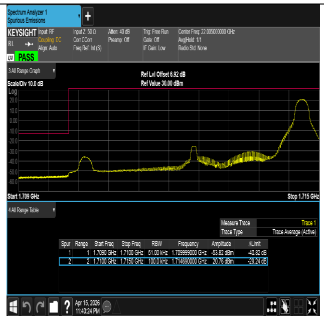
Band4-5MHz-QPSK-19975-1RB#24-PASS
