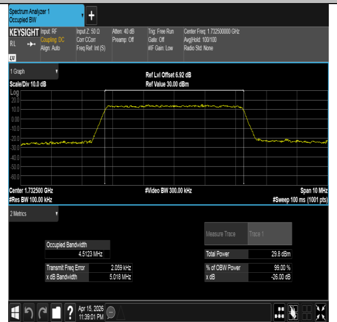
Band4-5MHz-16QAM-20175-25RB#0-PASS
