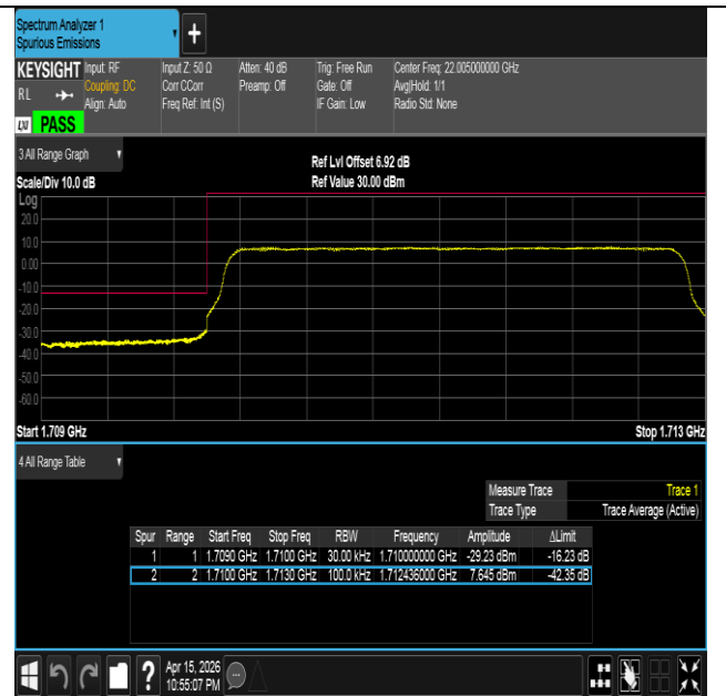
Band4-3MHz-16QAM-19965-15RB#0-PASS
