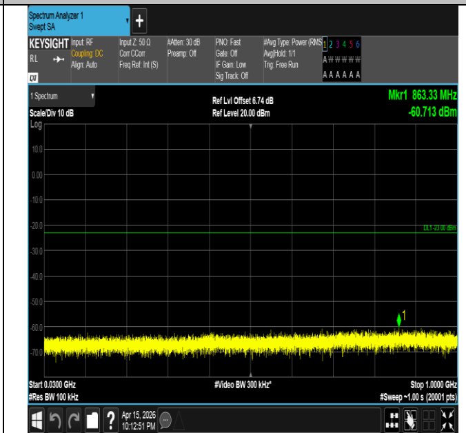
Band4-1.4MHz-QPSK-19957-1RB#5-30~1000-PASS
