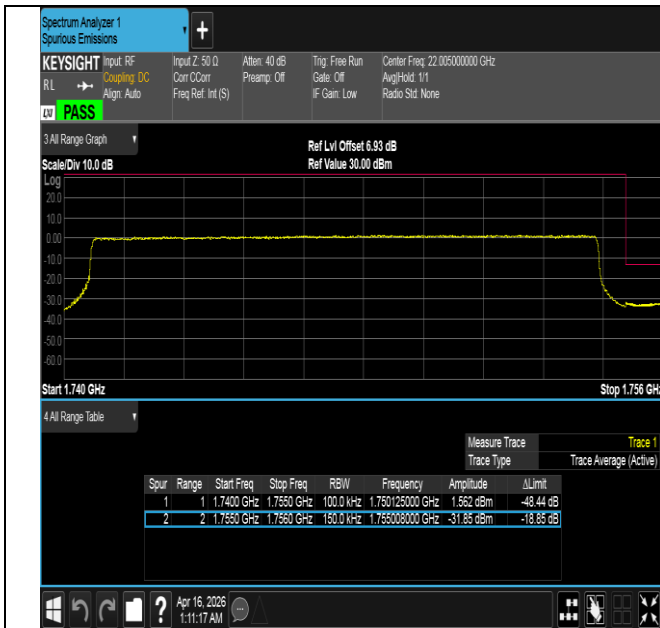
Band4-15MHz-QPSK-20325-75RB#0-PASS
