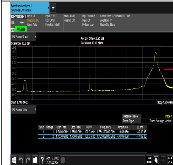
Band4-15MHz-16QAM-20325-1RB#74-PASS
