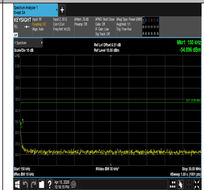
Band4-1.4MHz-QPSK-20175-1RB#0-0.15~30-PASS
