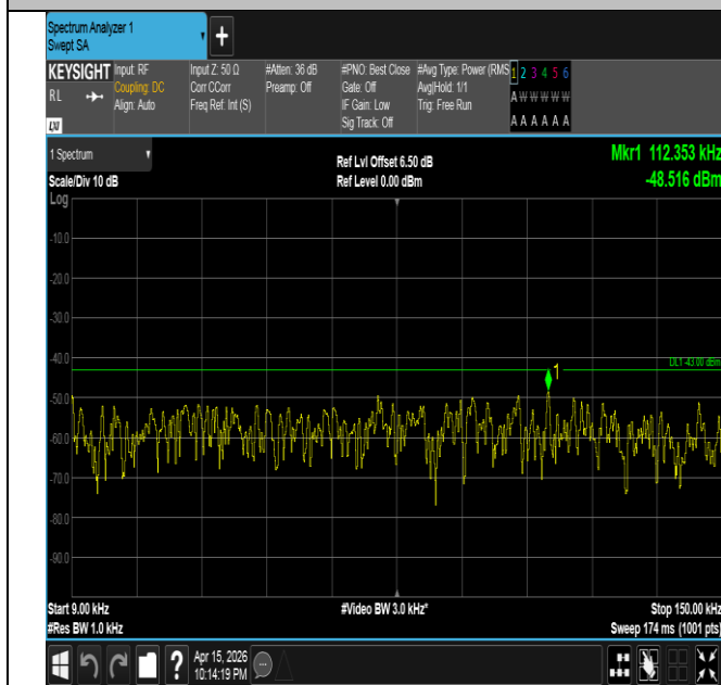
Band4-1.4MHz-QPSK-19957-6RB#0-0.009~0.15-PASS
