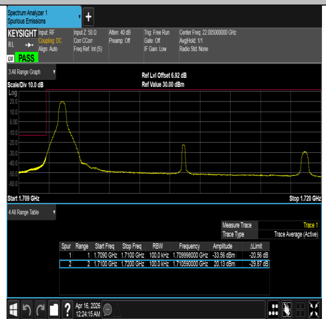
Band4-10MHz-16QAM-20000-1RB#0-PASS
