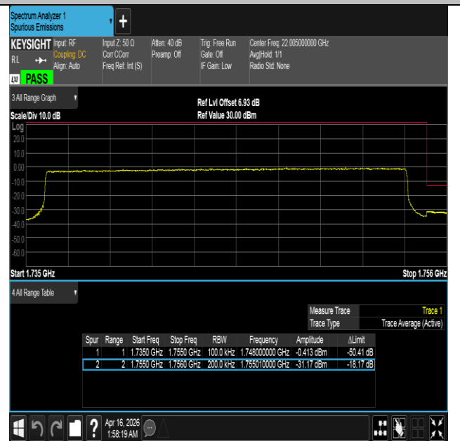
Band4-20MHz-16QAM-20300-100RB#0-PASS
