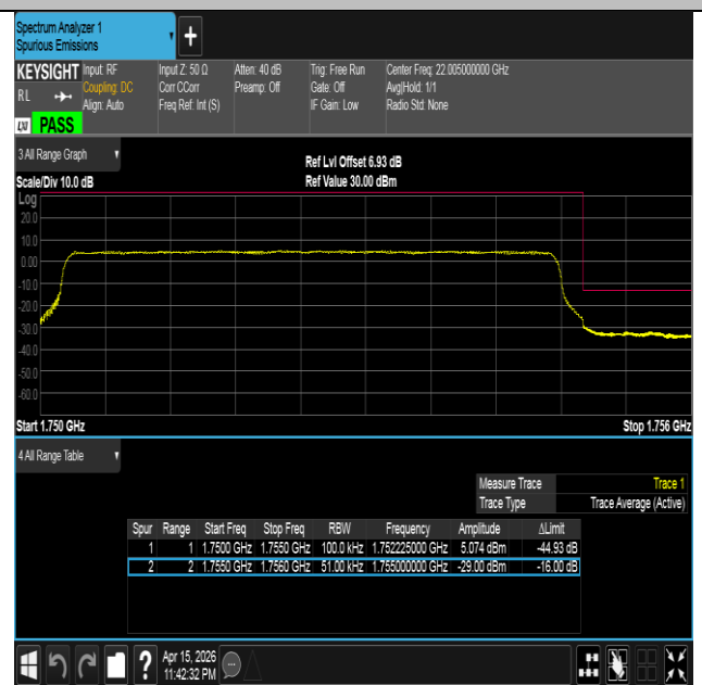
Band4-5MHz-16QAM-20375-25RB#0-PASS
