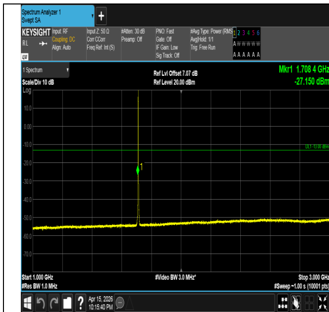
Band4-1.4MHz-16QAM-19957-6RB#0-1000~3000-PASS
