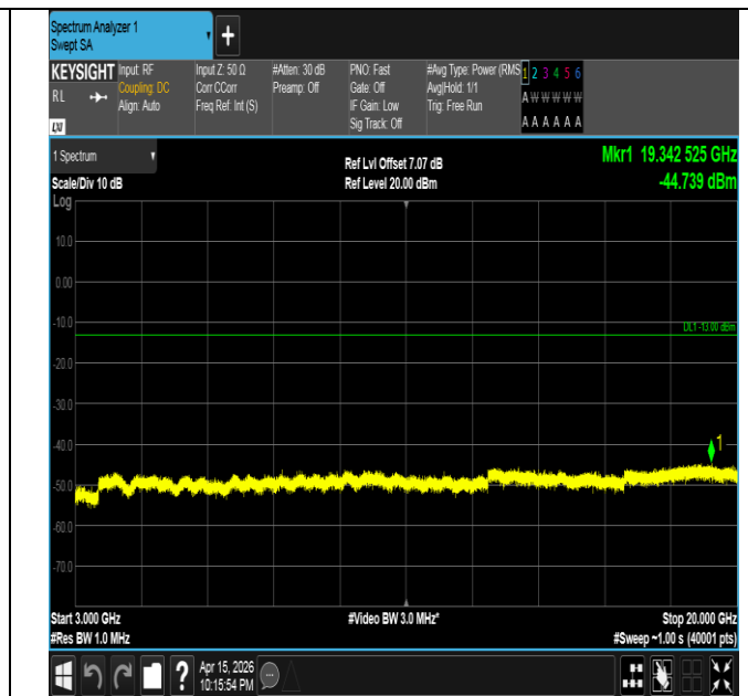
Band4-1.4MHz-16QAM-19957-6RB#0-3000~20000-PASS
