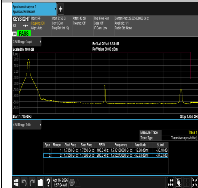
Band4-20MHz-QPSK-20300-1RB#0-PASS
