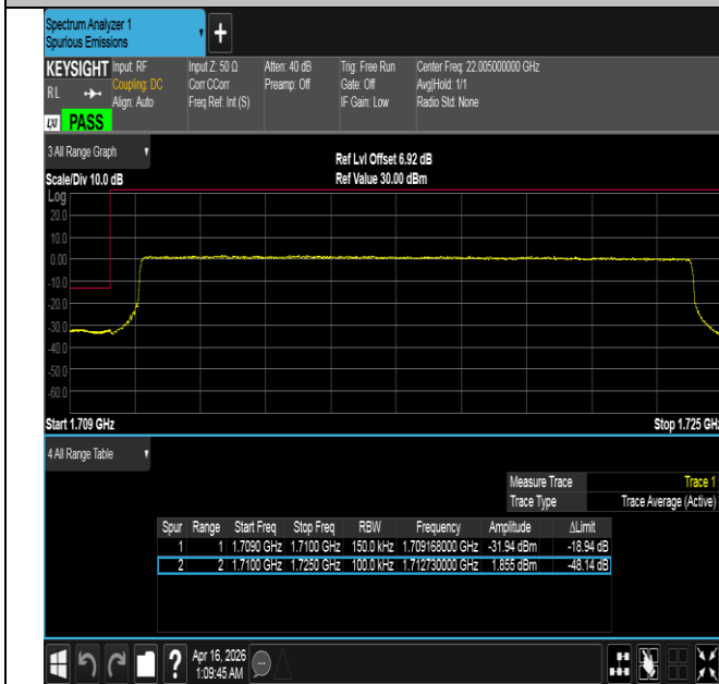
Band4-15MHz-QPSK-20025-75RB#0-PASS
