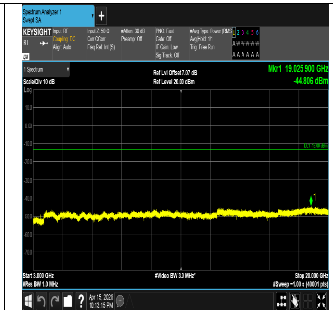
Band4-1.4MHz-QPSK-19957-1RB#5-3000~20000-PASS
