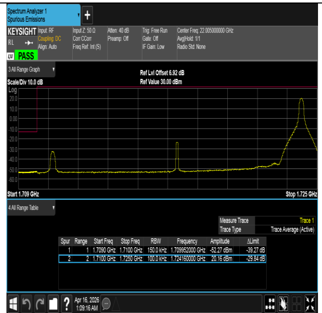
Band4-15MHz-QPSK-20025-1RB#74-PASS
