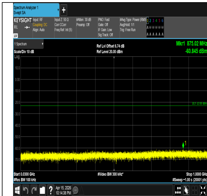
Band4-1.4MHz-QPSK-19957-6RB#0-30~1000-PASS
