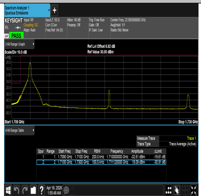
Band4-20MHz-16QAM-20050-1RB#0-PASS
