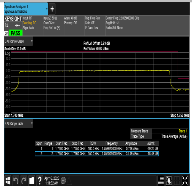
Band4-15MHz-16QAM-20325-75RB#0-PASS
