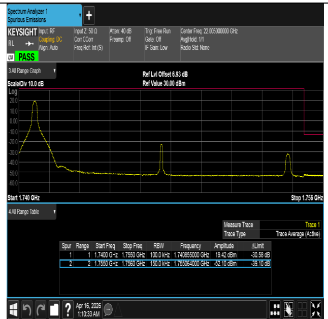
Band4-15MHz-16QAM-20325-1RB#0-PASS
