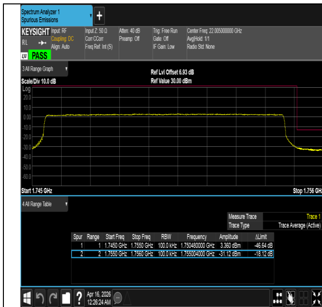
Band4-10MHz-QPSK-20350-50RB#0-PASS
