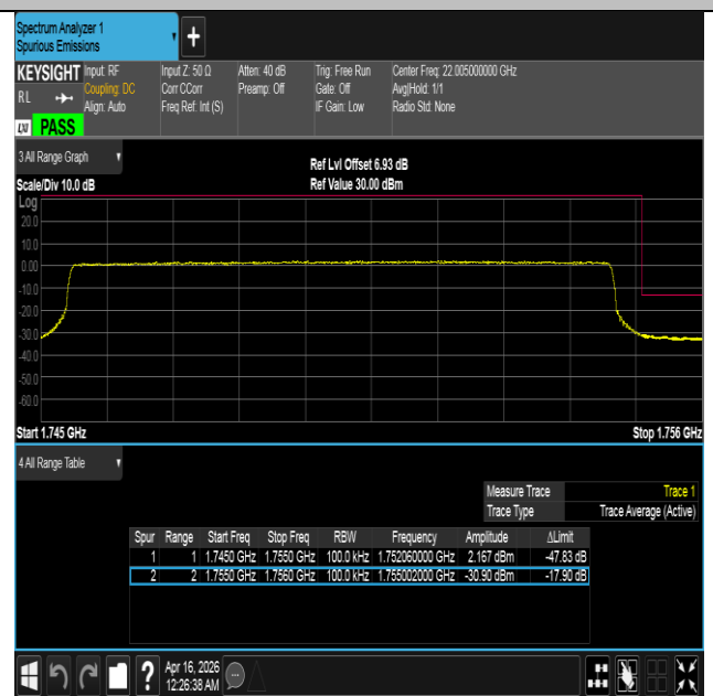
Band4-10MHz-16QAM-20350-50RB#0-PASS
