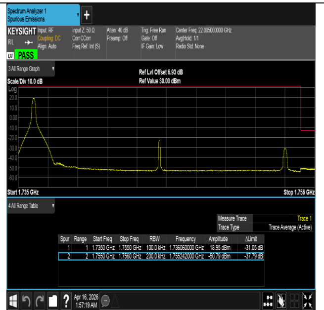
Band4-20MHz-16QAM-20300-1RB#0-PASS
