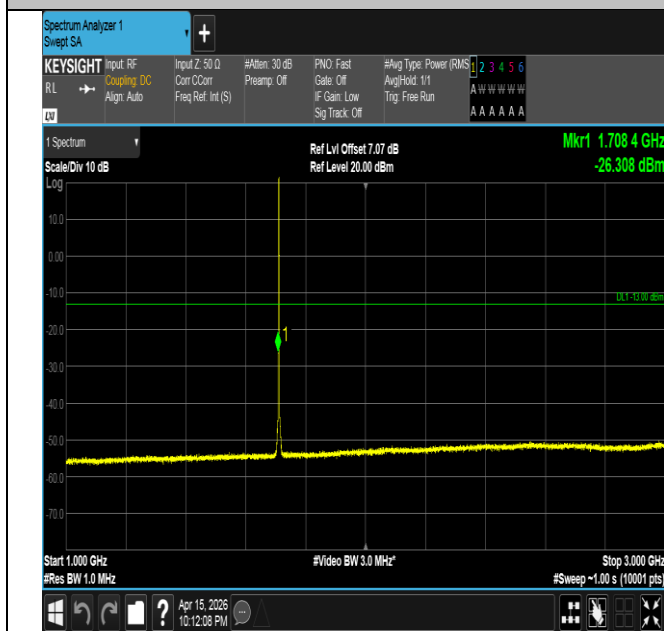
Band4-1.4MHz-16QAM-19957-1RB#0-1000~3000-PASS
