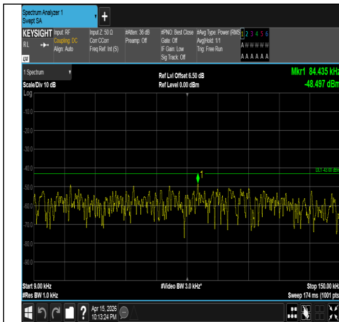
Band4-1.4MHz-16QAM-19957-1RB#5-0.009~0.15-PASS
