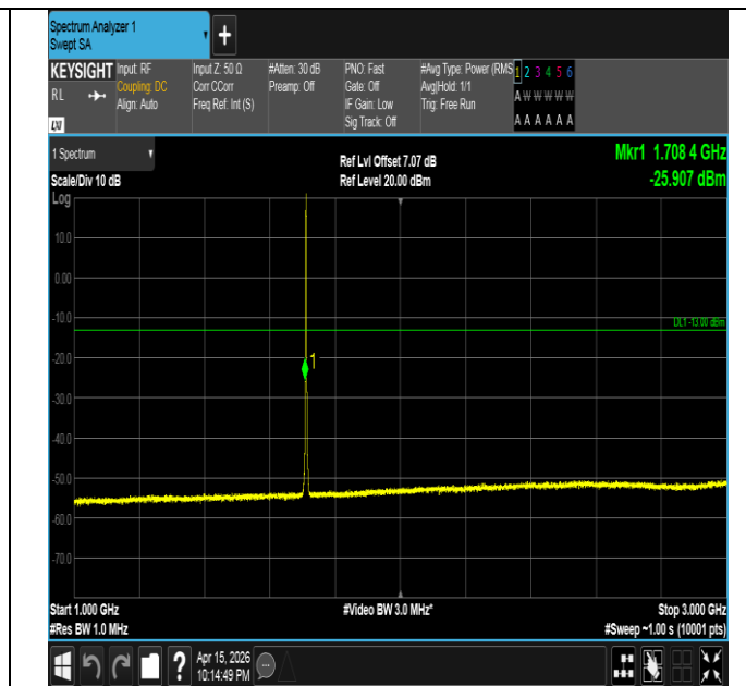
Band4-1.4MHz-QPSK-19957-6RB#0-1000~3000-PASS
