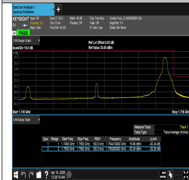
Band4-10MHz-16QAM-20350-1RB#49-PASS
