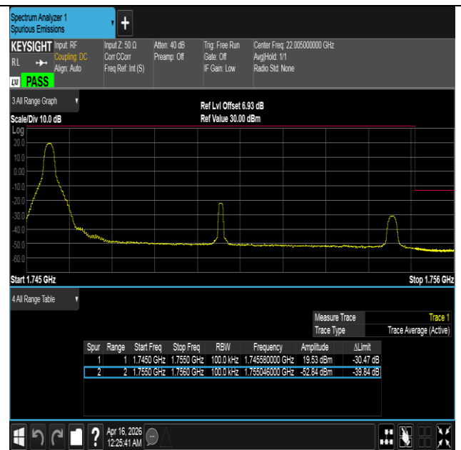
Band4-10MHz-16QAM-20350-1RB#0-PASS
