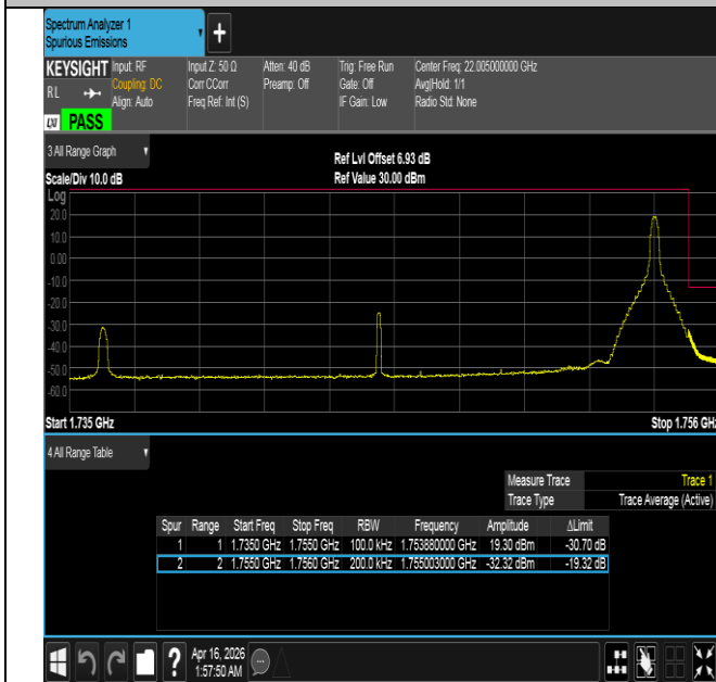
Band4-20MHz-16QAM-20300-1RB#99-PASS
