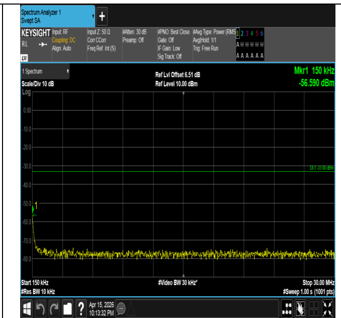
Band4-1.4MHz-16QAM-19957-1RB#5-0.15~30-PASS
