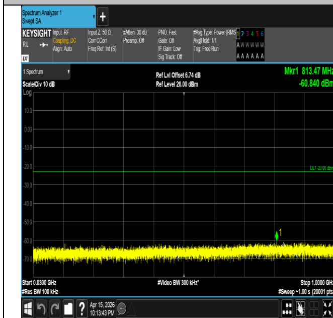
Band4-1.4MHz-16QAM-19957-1RB#5-30~1000-PASS
