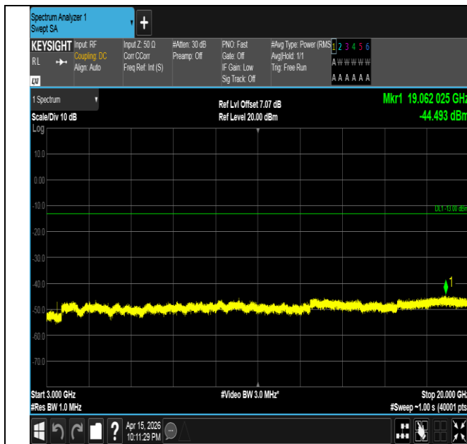
Band4-1.4MHz-QPSK-19957-1RB#0-3000~20000-PASS
