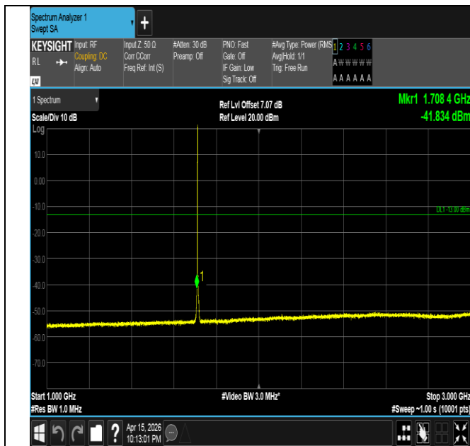
Band4-1.4MHz-QPSK-19957-1RB#5-1000~3000-PASS
