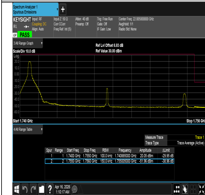
Band4-15MHz-QPSK-20325-1RB#0-PASS
