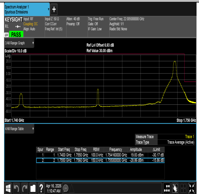
Band4-15MHz-QPSK-20325-1RB#74-PASS
