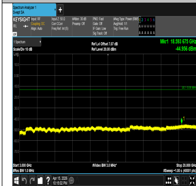
Band4-1.4MHz-QPSK-19957-6RB#0-3000~20000-PASS
