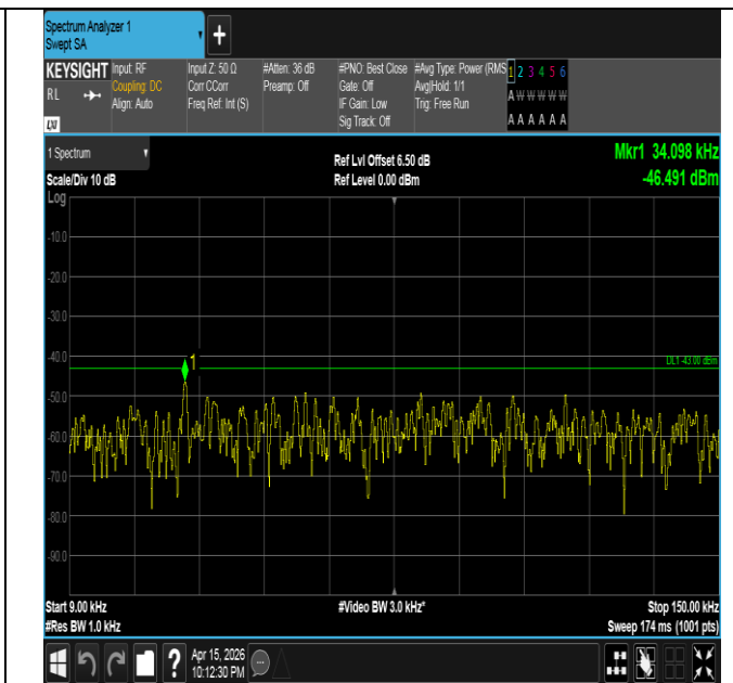
Band4-1.4MHz-QPSK-19957-1RB#5-0.009~0.15-PASS
