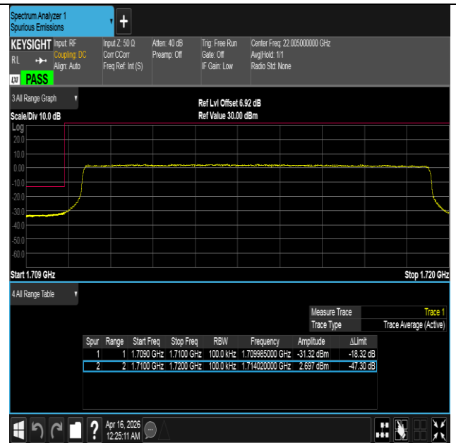
Band4-10MHz-16QAM-20000-50RB#0-PASS
