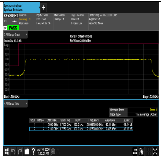
Band4-15MHz-16QAM-20025-75RB#0-PASS
