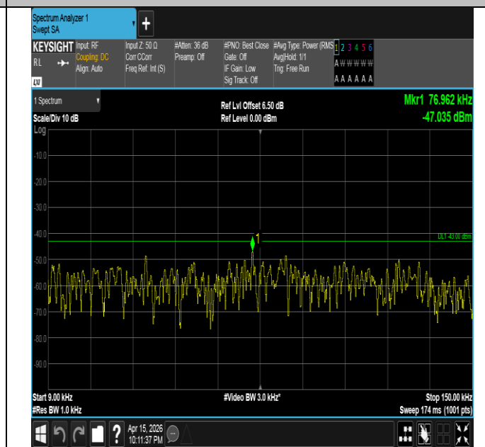
Band4-1.4MHz-16QAM-19957-1RB#0-0.009~0.15-PASS
