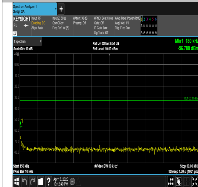
Band4-1.4MHz-QPSK-19957-1RB#5-0.15~30-PASS
