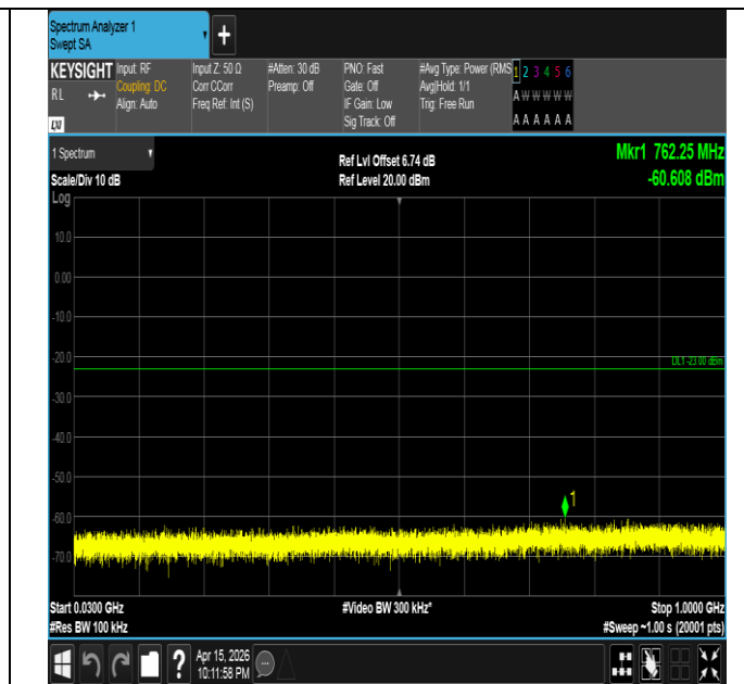
Band4-1.4MHz-16QAM-19957-1RB#0-30~1000-PASS
