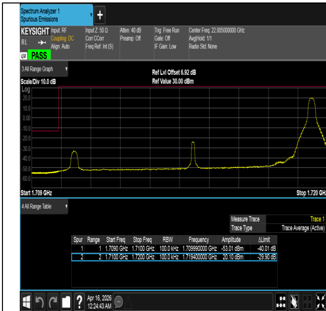
Band4-10MHz-16QAM-20000-1RB#49-PASS
