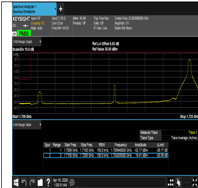
Band4-15MHz-16QAM-20025-1RB#74-PASS
