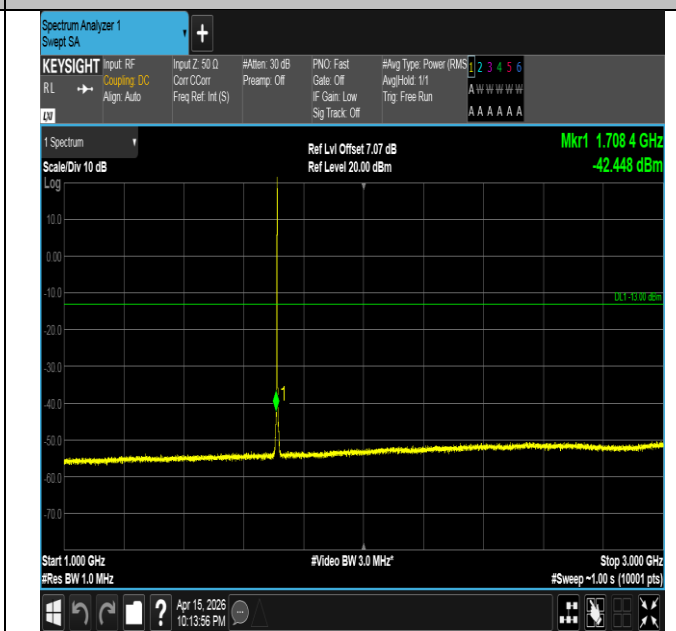
Band4-1.4MHz-16QAM-19957-1RB#5-1000~3000-PASS
