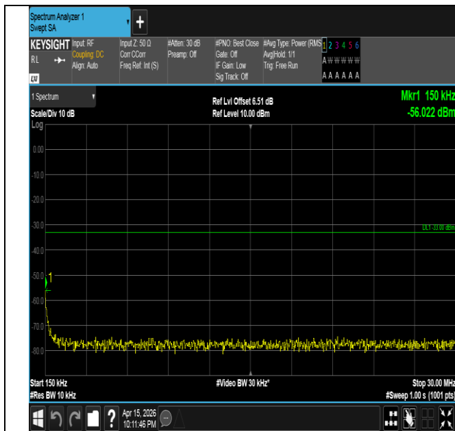
Band4-1.4MHz-16QAM-19957-1RB#0-0.15~30-PASS
