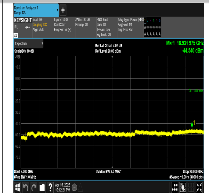
Band4-1.4MHz-16QAM-19957-1RB#0-3000~20000-PASS
