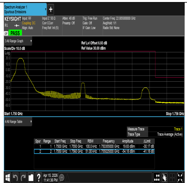
Band4-5MHz-16QAM-20375-1RB#0-PASS
