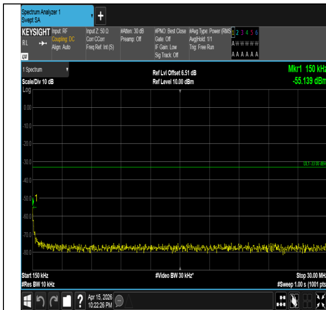
Band4-1.4MHz-16QAM-20393-1RB#0-0.15~30-PASS
