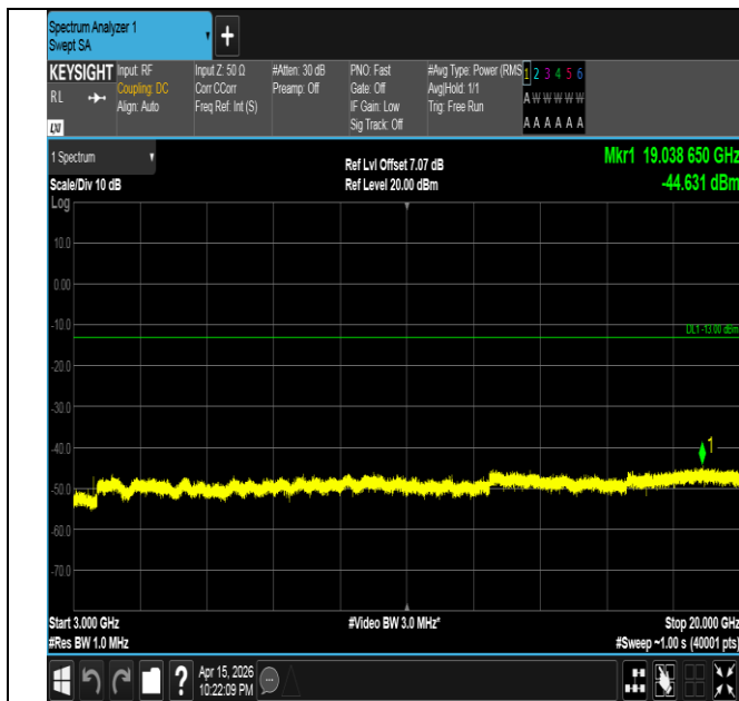
Band4-1.4MHz-QPSK-20393-1RB#0-3000~20000-PASS
