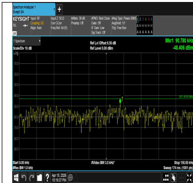
Band4-1.4MHz-QPSK-20175-6RB#0-0.009~0.15-PASS
