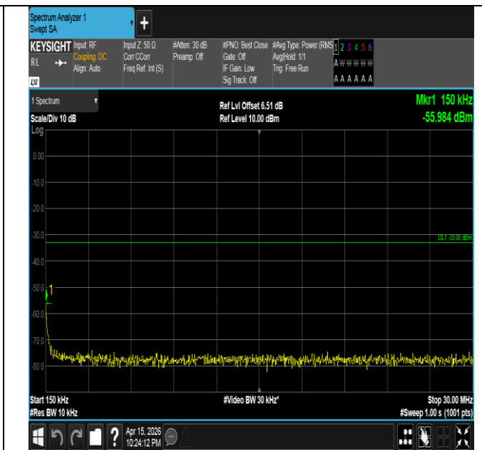
Band4-1.4MHz-16QAM-20393-1RB#5-0.15~30-PASS
