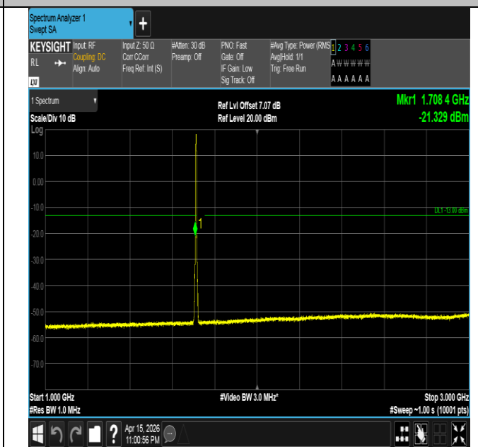
Band4-3MHz-QPSK-19965-15RB#0-1000~3000-PASS
