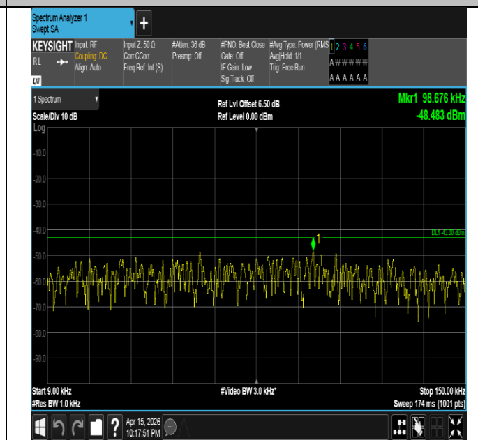
Band4-1.4MHz-QPSK-20175-1RB#5-0.009~0.15-PASS
