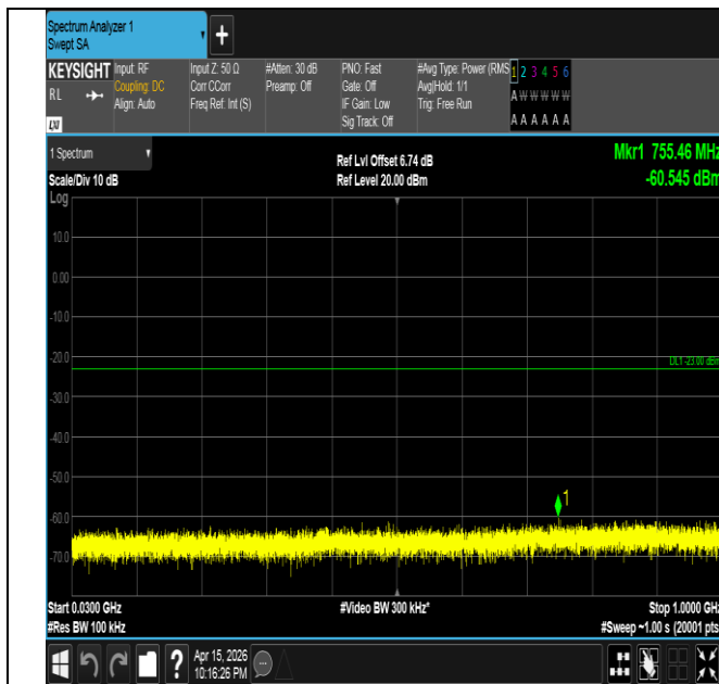
Band4-1.4MHz-QPSK-20175-1RB#0-30~1000-PASS
