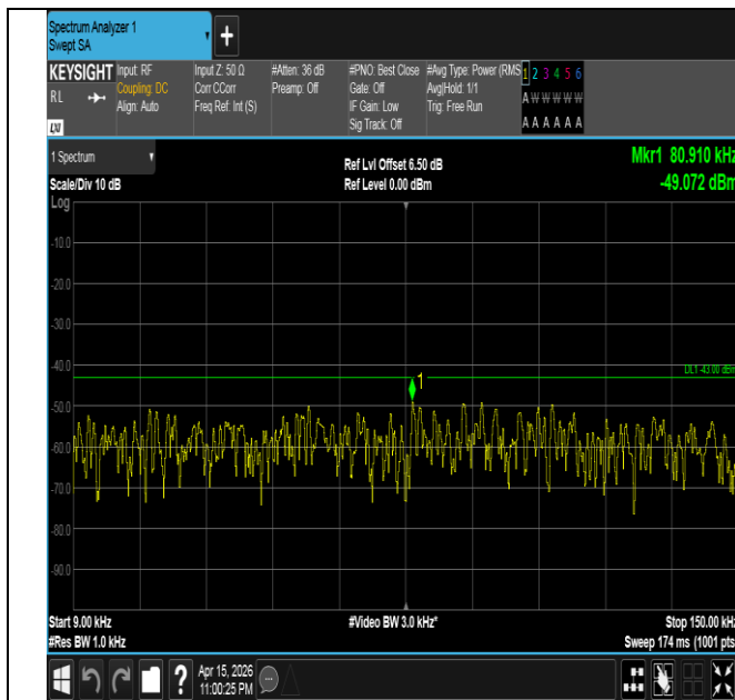
Band4-3MHz-QPSK-19965-15RB#0-0.009~0.15-PASS
