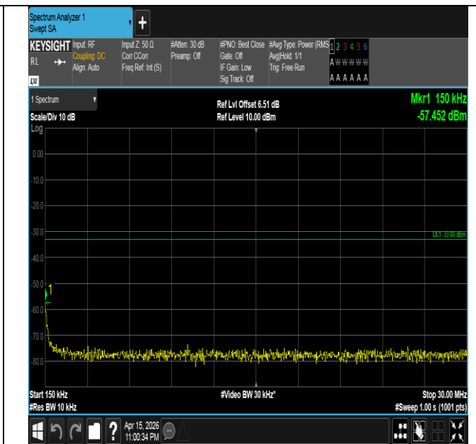
Band4-3MHz-QPSK-19965-15RB#0-0.15~30-PASS
