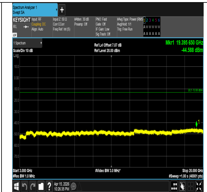
Band4-1.4MHz-16QAM-20393-6RB#0-3000~20000-PASS
