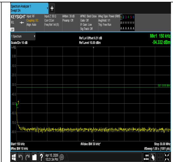
Band4-1.4MHz-QPSK-20393-1RB#0-0.15~30-PASS
