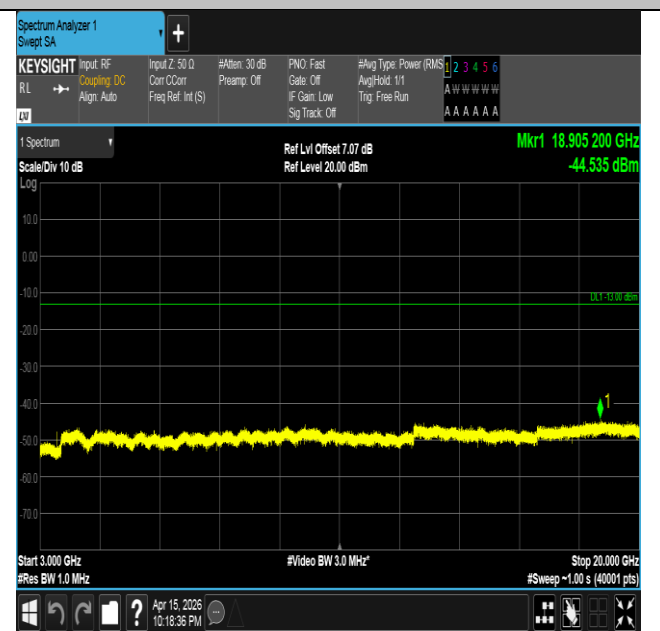
Band4-1.4MHz-QPSK-20175-1RB#5-3000~20000-PASS
