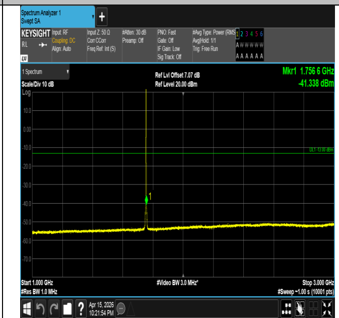
Band4-1.4MHz-QPSK-20393-1RB#0-1000~3000-PASS
