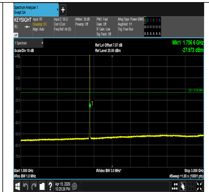
Band4-1.4MHz-QPSK-20393-6RB#0-1000~3000-PASS
