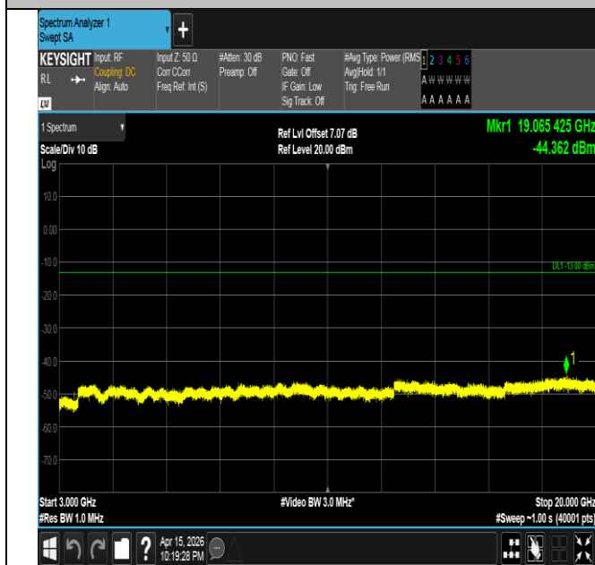
Band4-1.4MHz-16QAM-20175-1RB#5-3000~20000-PASS
