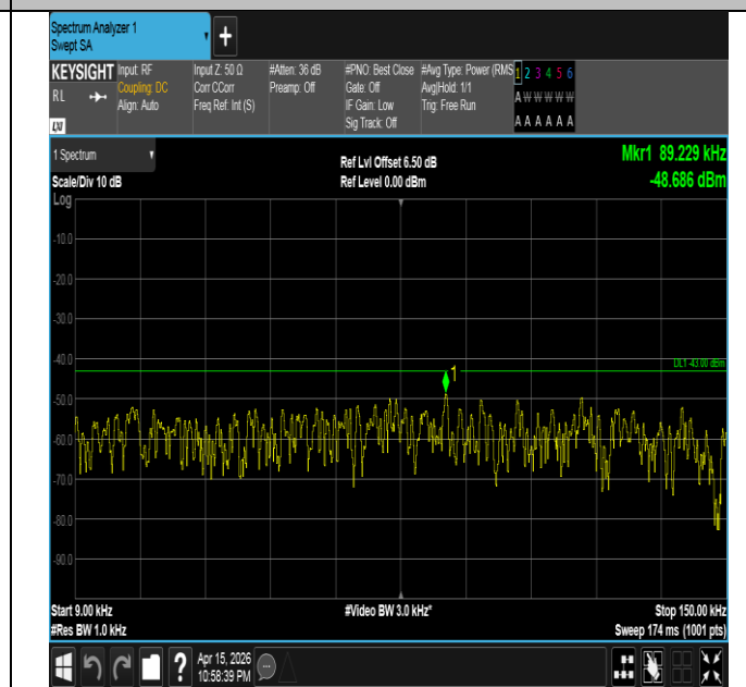
Band4-3MHz-QPSK-19965-1RB#14-0.009~0.15-PASS
