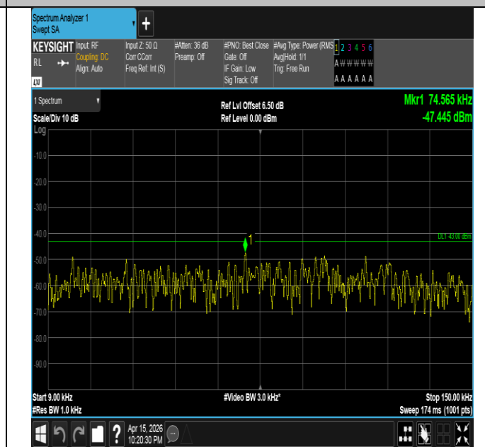
Band4-1.4MHz-16QAM-20175-6RB#0-0.009~0.15-PASS
