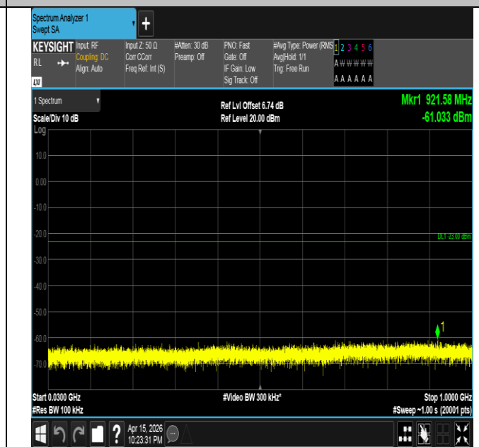
Band4-1.4MHz-QPSK-20393-1RB#5-30~1000-PASS
