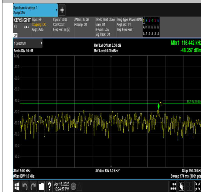
Band4-1.4MHz-QPSK-20393-6RB#0-0.009~0.15-PASS
