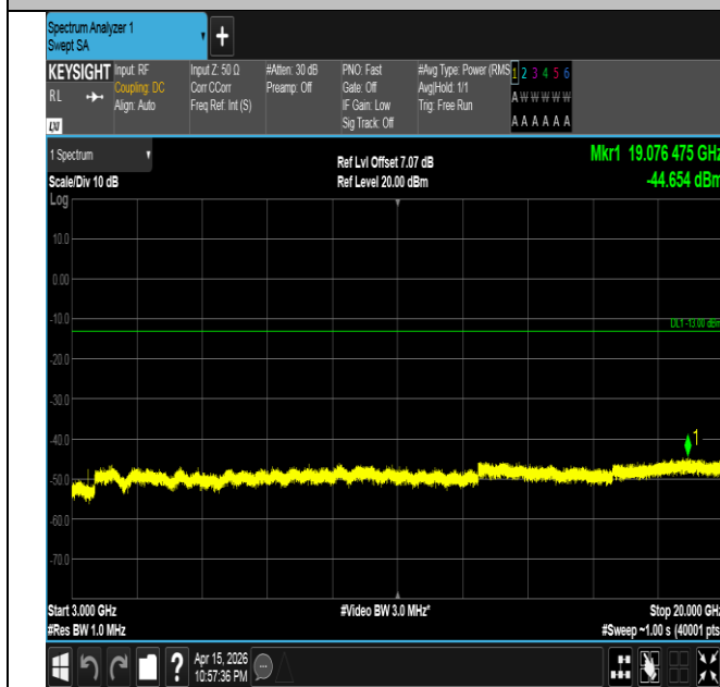
Band4-3MHz-QPSK-19965-1RB#0-3000~20000-PASS
