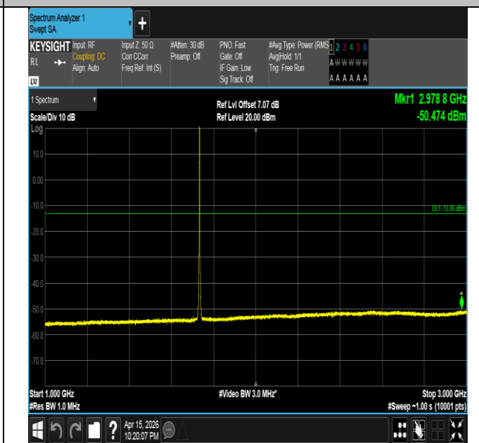
Band4-1.4MHz-QPSK-20175-6RB#0-1000~3000-PASS
