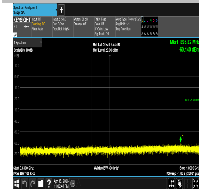
Band4-3MHz-QPSK-19965-15RB#0-30~1000-PASS
