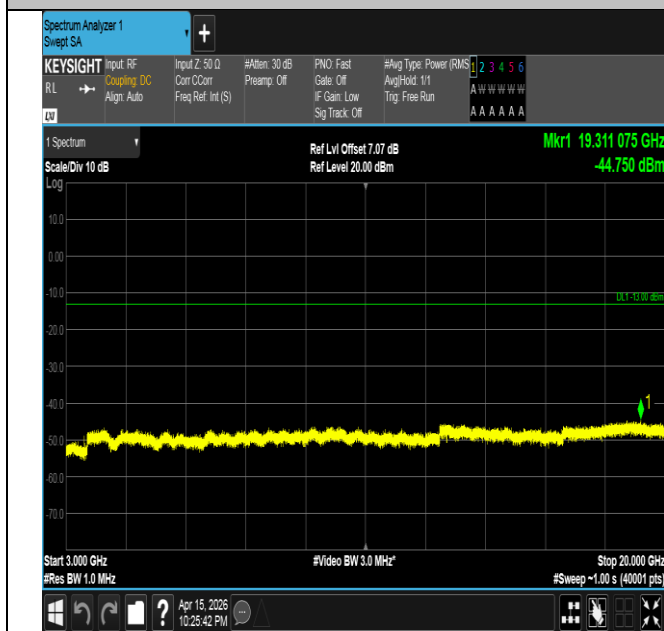
Band4-1.4MHz-QPSK-20393-6RB#0-3000~20000-PASS
