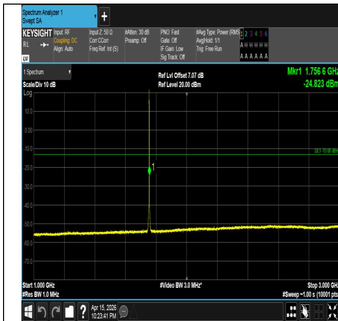
Band4-1.4MHz-QPSK-20393-1RB#5-1000~3000-PASS
