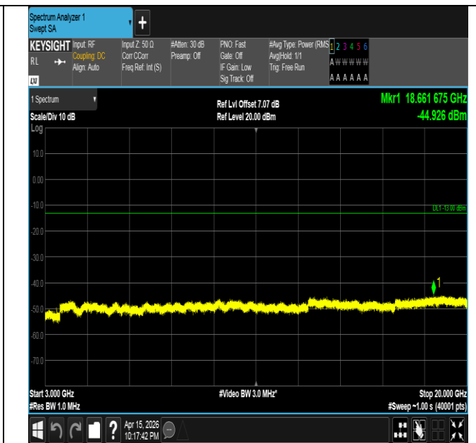
Band4-1.4MHz-16QAM-20175-1RB#0-3000~20000-PASS
