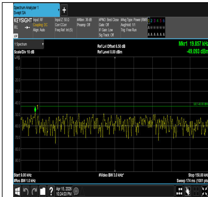
Band4-1.4MHz-16QAM-20393-1RB#5-0.009~0.15-PASS
