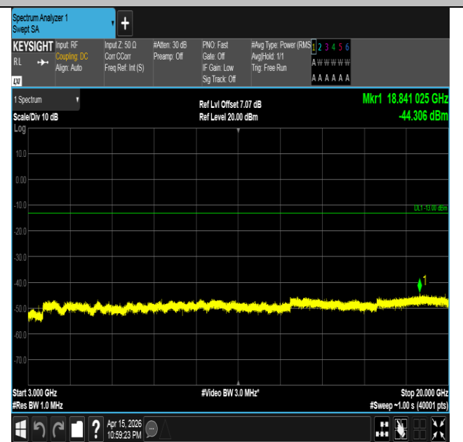
Band4-3MHz-QPSK-19965-1RB#14-3000~20000-PASS
