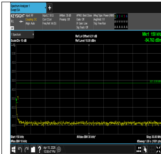
Band4-3MHz-QPSK-19965-1RB#14-0.15~30-PASS
