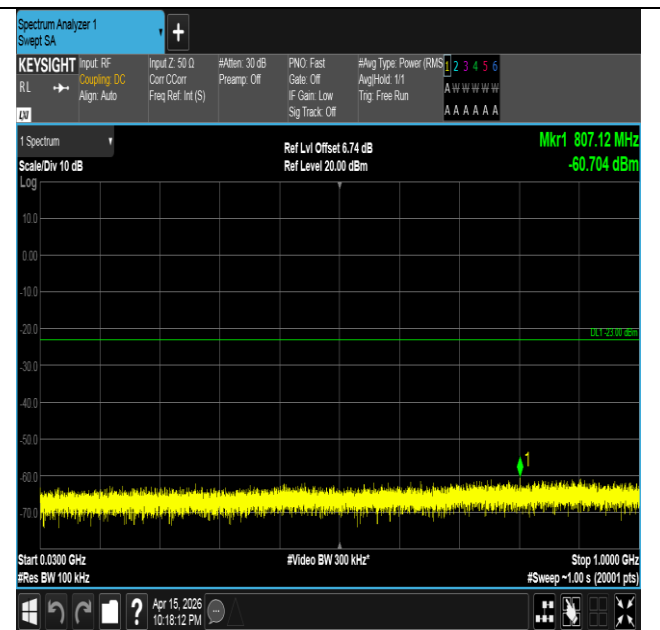
Band4-1.4MHz-QPSK-20175-1RB#5-30~1000-PASS
