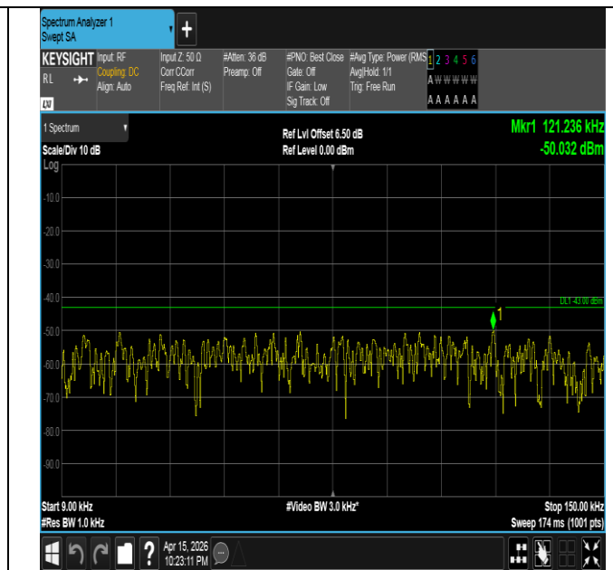
Band4-1.4MHz-QPSK-20393-1RB#5-0.009~0.15-PASS
