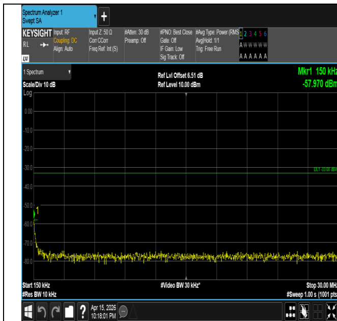
Band4-1.4MHz-QPSK-20175-1RB#5-0.15~30-PASS
