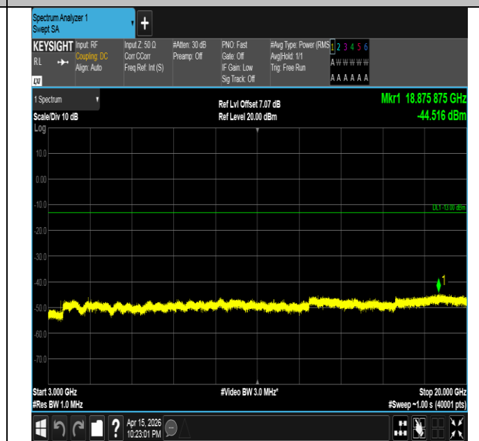
Band4-1.4MHz-16QAM-20393-1RB#0-3000~20000-PASS
