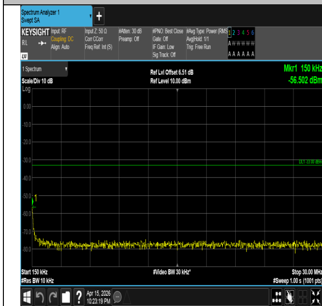
Band4-1.4MHz-QPSK-20393-1RB#5-0.15~30-PASS
