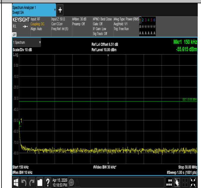
Band4-1.4MHz-16QAM-20175-1RB#5-0.15~30-PASS
