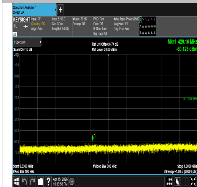
Band4-1.4MHz-QPSK-20175-6RB#0-30~1000-PASS
