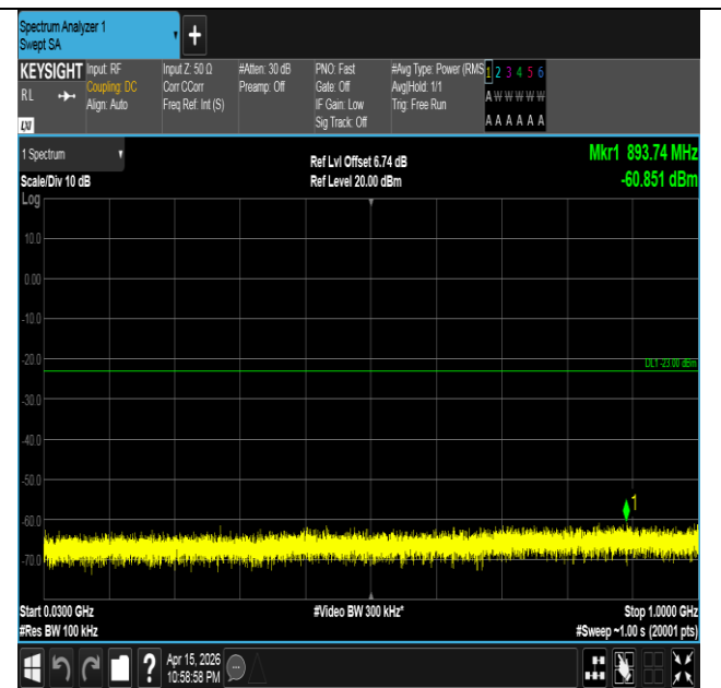
Band4-3MHz-QPSK-19965-1RB#14-30~1000-PASS
