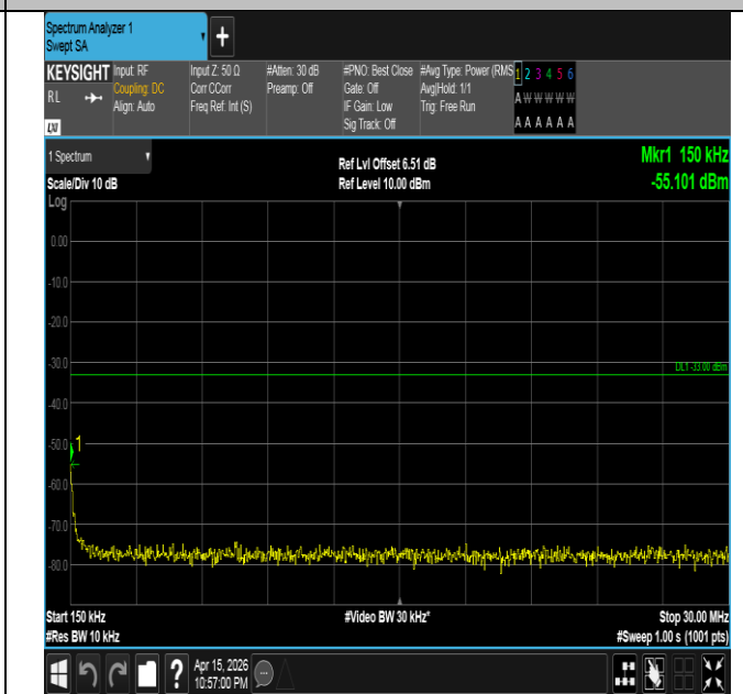
Band4-3MHz-QPSK-19965-1RB#0-0.15~30-PASS
