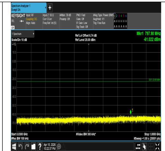
Band4-1.4MHz-16QAM-20393-1RB#0-30~1000-PASS
