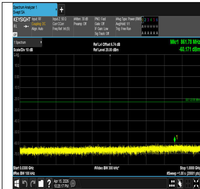
Band4-1.4MHz-QPSK-20393-6RB#0-30~1000-PASS
