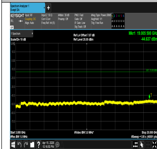
Band4-1.4MHz-QPSK-20175-1RB#0-3000~20000-PASS
