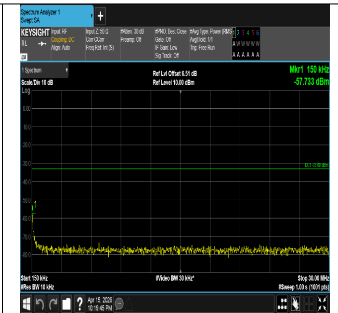
Band4-1.4MHz-QPSK-20175-6RB#0-0.15~30-PASS
