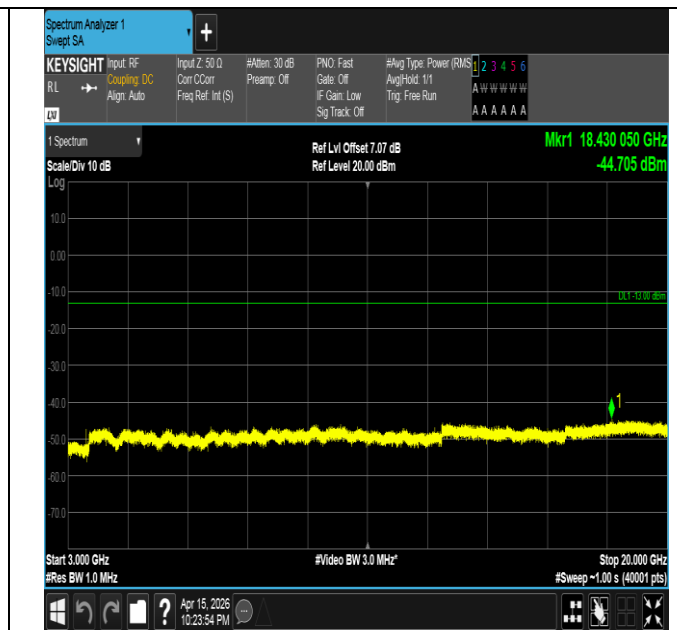
Band4-1.4MHz-QPSK-20393-1RB#5-3000~20000-PASS
