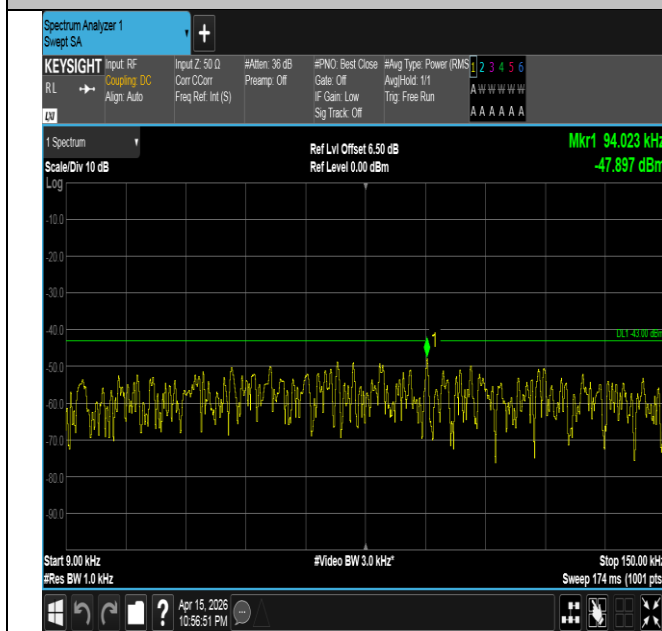
Band4-3MHz-QPSK-19965-1RB#0-0.009~0.15-PASS
