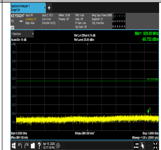
Band4-1.4MHz-16QAM-20175-1RB#0-30~1000-PASS
