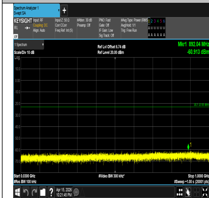
Band4-1.4MHz-QPSK-20393-1RB#0-30~1000-PASS
