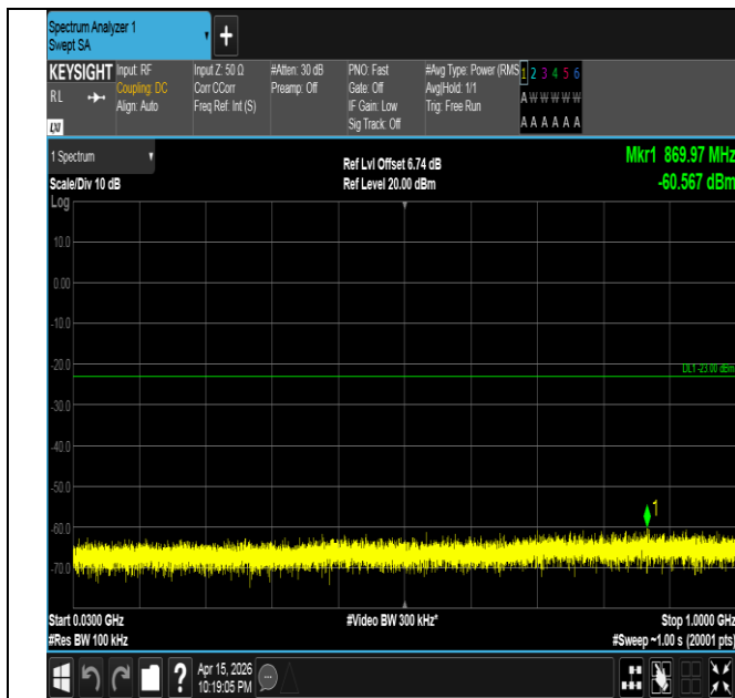
Band4-1.4MHz-16QAM-20175-1RB#5-30~1000-PASS
