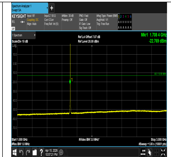
Band4-3MHz-QPSK-19965-1RB#0-1000~3000-PASS
