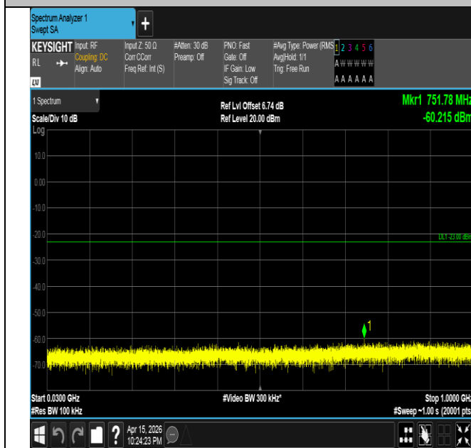
Band4-1.4MHz-16QAM-20393-1RB#5-30~1000-PASS
