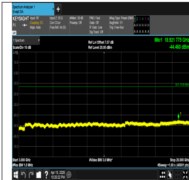
Band4-1.4MHz-QPSK-20175-6RB#0-3000~20000-PASS
