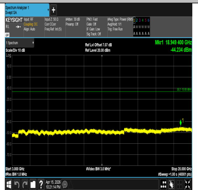
Band4-1.4MHz-16QAM-20175-6RB#0-3000~20000-PASS
