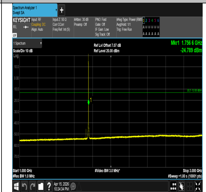
Band4-1.4MHz-16QAM-20393-1RB#5-1000~3000-PASS
