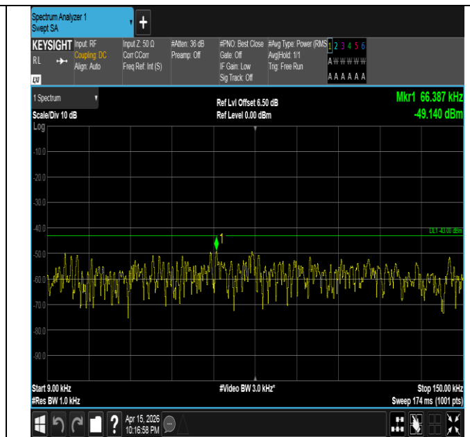
Band4-1.4MHz-16QAM-20175-1RB#0-0.009~0.15-PASS
