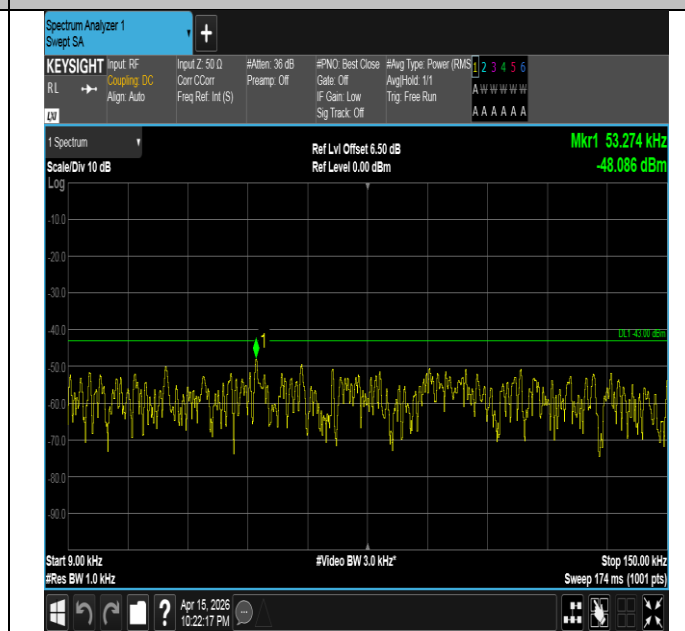
Band4-1.4MHz-16QAM-20393-1RB#0-0.009~0.15-PASS
