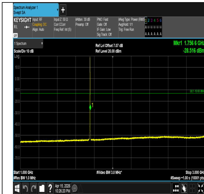
Band4-1.4MHz-16QAM-20393-6RB#0-1000~3000-PASS
