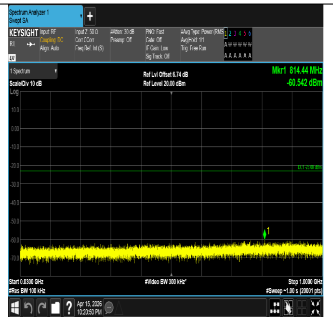
Band4-1.4MHz-16QAM-20175-6RB#0-30~1000-PASS
