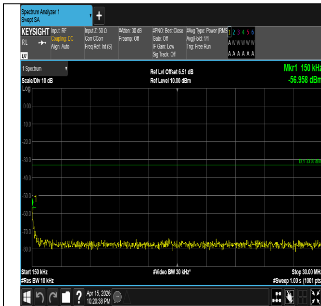
Band4-1.4MHz-16QAM-20175-6RB#0-0.15~30-PASS
