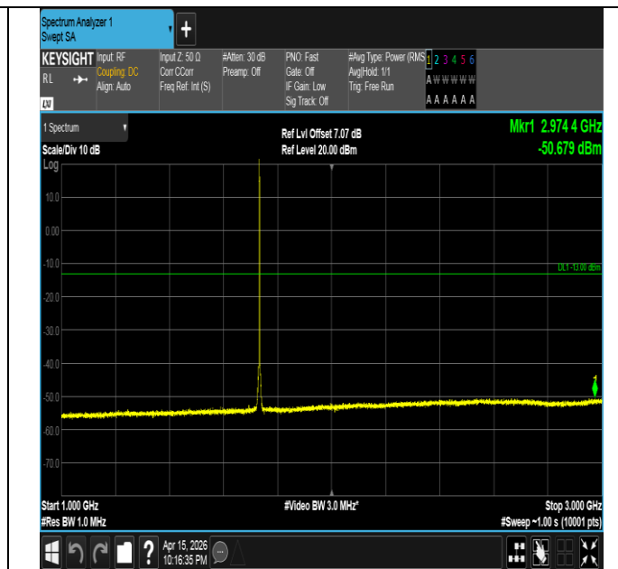
Band4-1.4MHz-QPSK-20175-1RB#0-1000~3000-PASS
