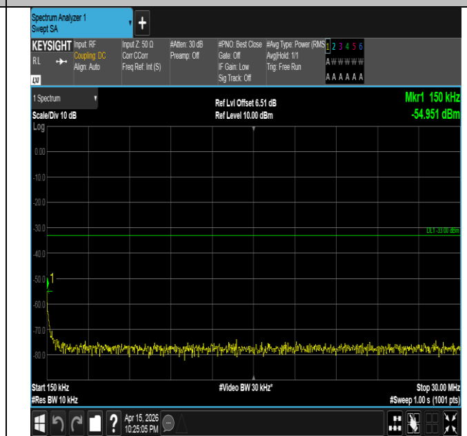
Band4-1.4MHz-QPSK-20393-6RB#0-0.15~30-PASS
