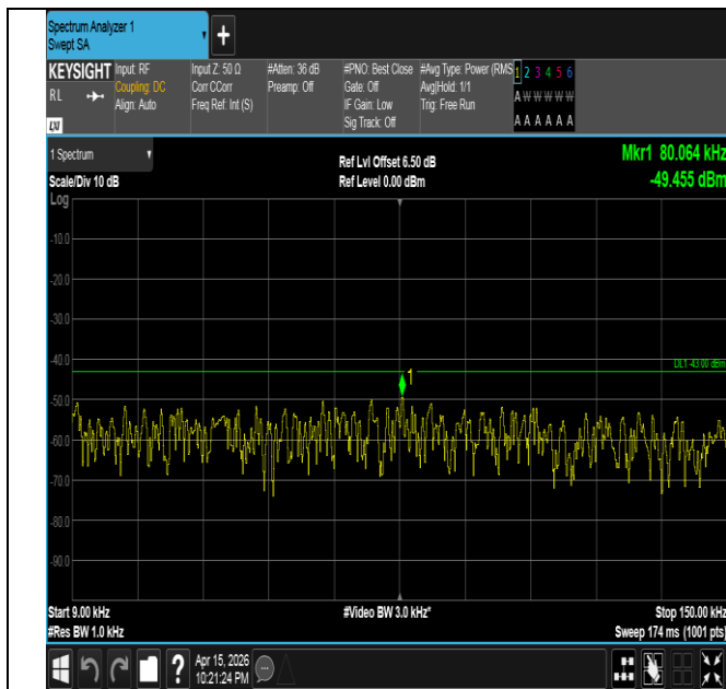
Band4-1.4MHz-QPSK-20393-1RB#0-0.009~0.15-PASS
