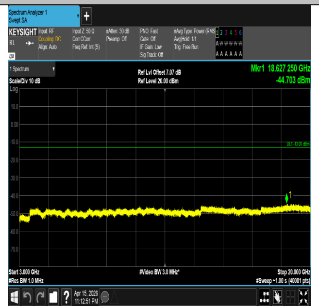
Band4-3MHz-16QAM-20385-15RB#0-3000~20000-PASS
