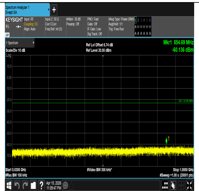
Band4-3MHz-QPSK-20385-1RB#14-30~1000-PASS
