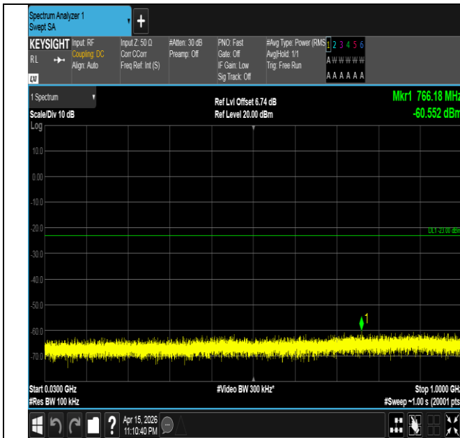
Band4-3MHz-16QAM-20385-1RB#14-30~1000-PASS
