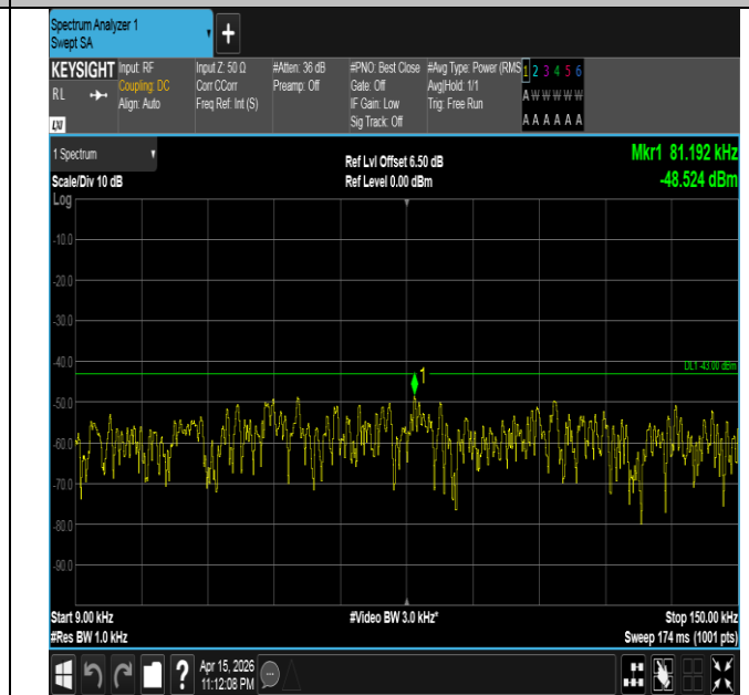
Band4-3MHz-16QAM-20385-15RB#0-0.009~0.15-PASS
