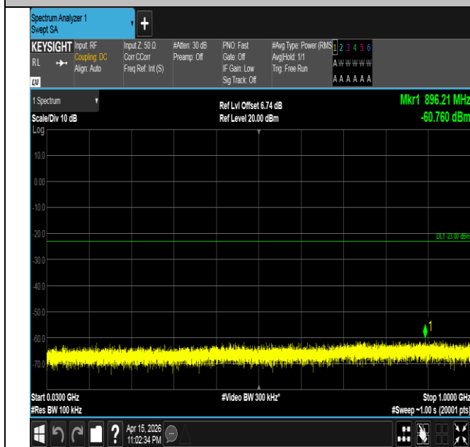
Band4-3MHz-QPSK-20175-1RB#0-30~1000-PASS
