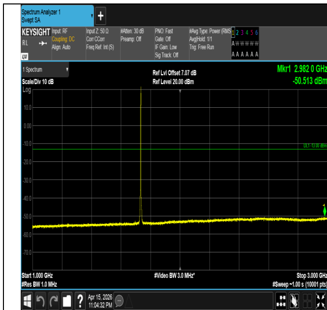
Band4-3MHz-QPSK-20175-1RB#14-1000~3000-PASS
