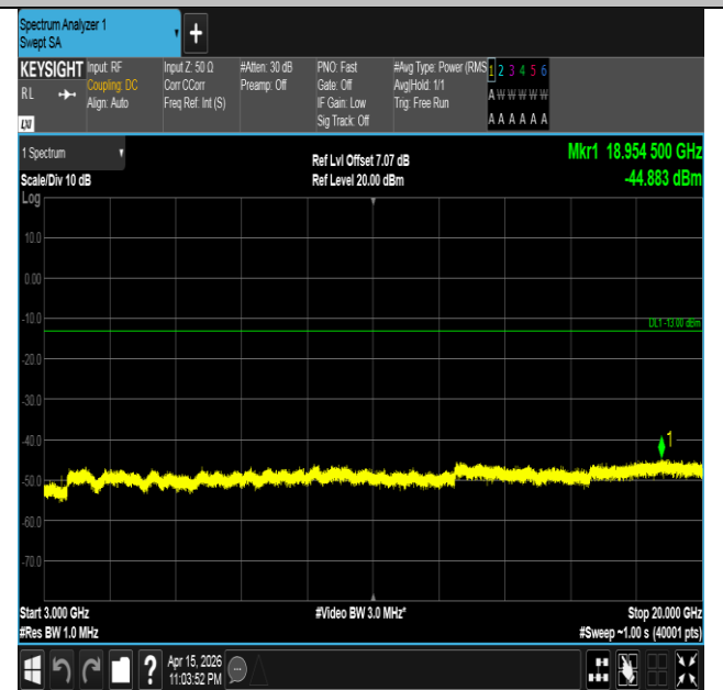
Band4-3MHz-16QAM-20175-1RB#0-3000~20000-PASS
