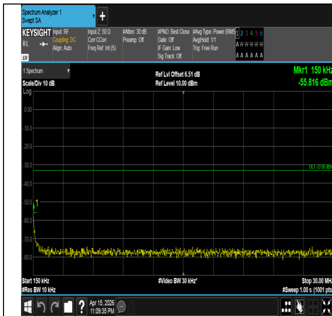
Band4-3MHz-QPSK-20385-1RB#14-0.15~30-PASS
