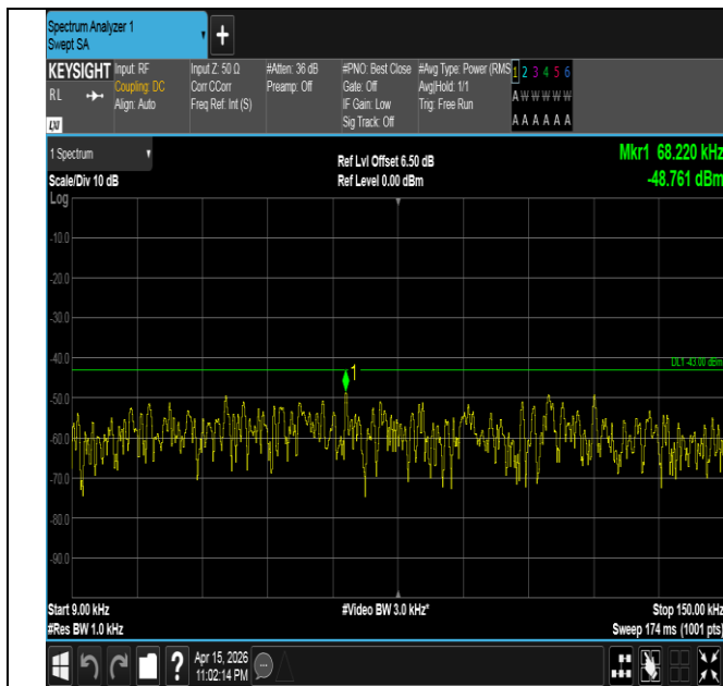
Band4-3MHz-QPSK-20175-1RB#0-0.009~0.15-PASS
