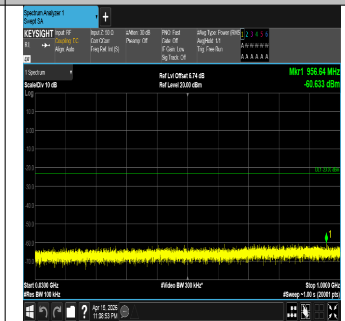
Band4-3MHz-16QAM-20385-1RB#0-30~1000-PASS
