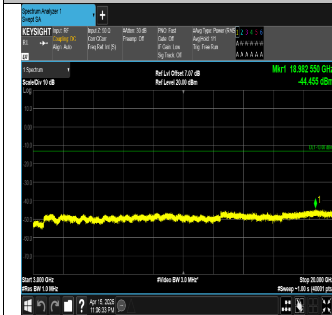
Band4-3MHz-QPSK-20175-15RB#0-3000~20000-PASS
