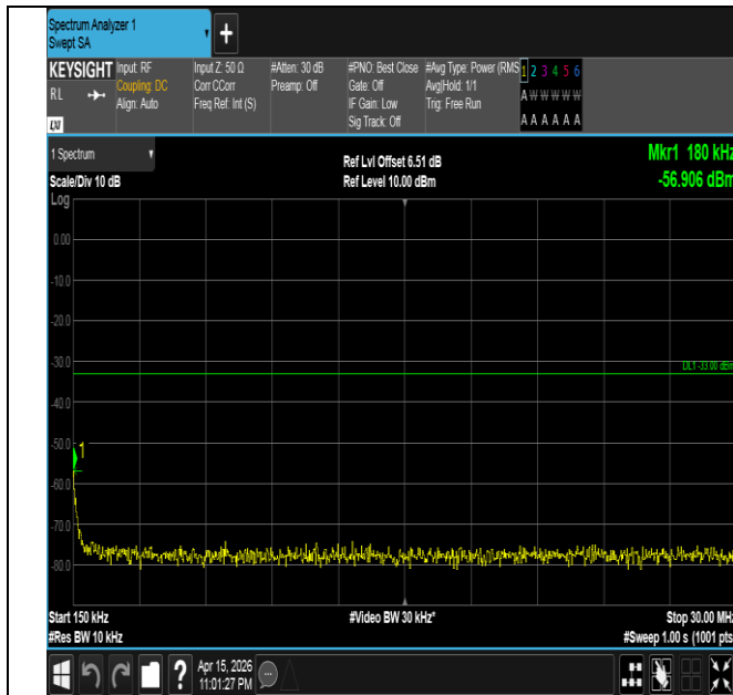
Band4-3MHz-16QAM-19965-15RB#0-0.15~30-PASS
