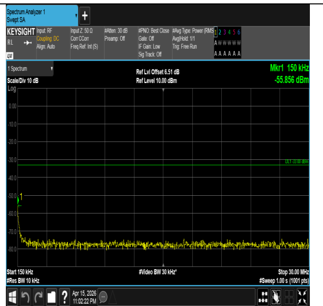
Band4-3MHz-QPSK-20175-1RB#0-0.15~30-PASS
