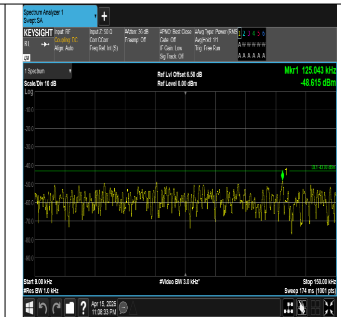
Band4-3MHz-16QAM-20385-1RB#0-0.009~0.15-PASS
