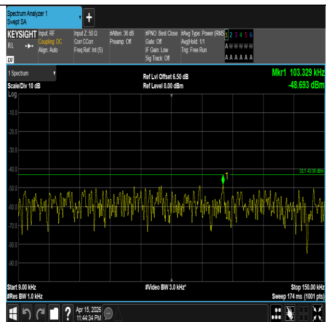
Band4-5MHz-QPSK-19975-1RB#24-0.009~0.15-PASS
