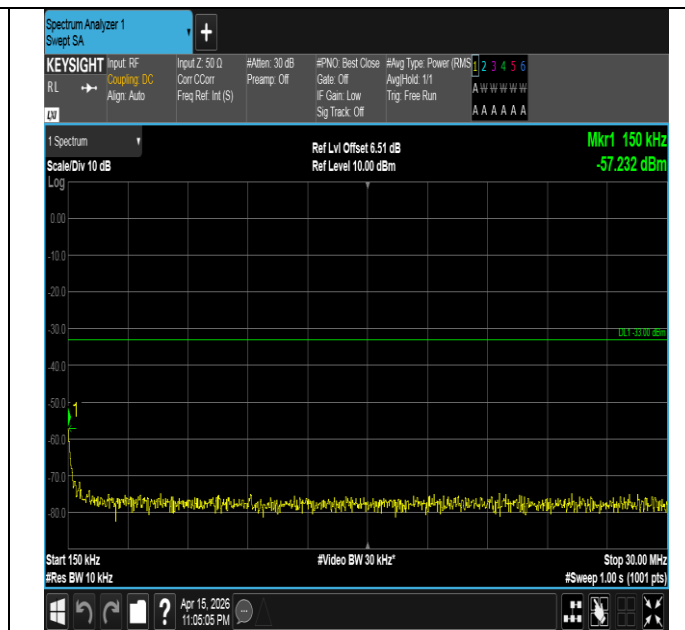
Band4-3MHz-16QAM-20175-1RB#14-0.15~30-PASS
