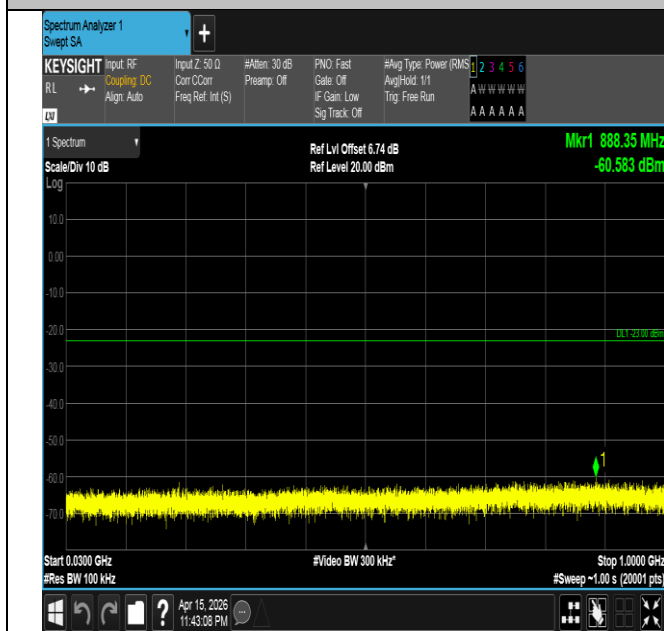
Band4-5MHz-QPSK-19975-1RB#0-30~1000-PASS
