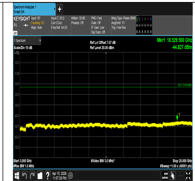
Band4-3MHz-16QAM-20175-15RB#0-3000~20000-PASS
