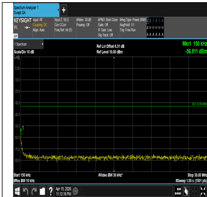
Band4-3MHz-16QAM-20385-15RB#0-0.15~30-PASS
