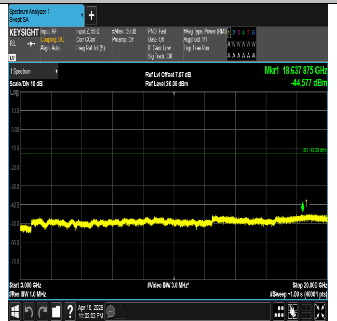
Band4-3MHz-16QAM-19965-15RB#0-3000~20000-PASS
