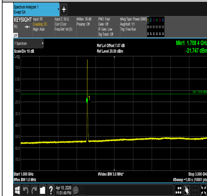
Band4-3MHz-16QAM-19965-15RB#0-1000~3000-PASS
