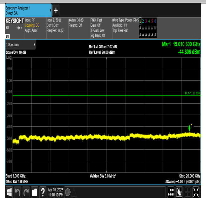
Band4-3MHz-QPSK-20385-1RB#14-3000~20000-PASS
