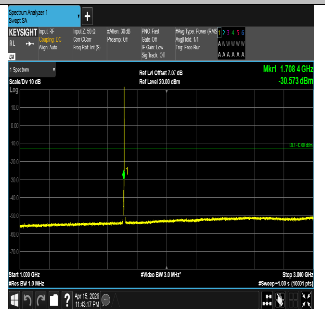
Band4-5MHz-QPSK-19975-1RB#0-1000~3000-PASS
