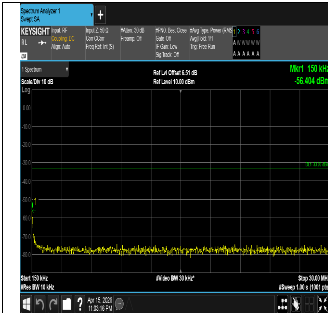
Band4-3MHz-16QAM-20175-1RB#0-0.15~30-PASS
