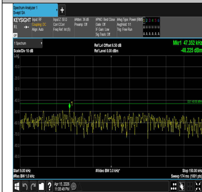
Band4-3MHz-QPSK-20175-15RB#0-0.009~0.15-PASS
