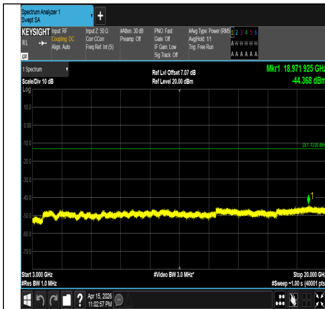
Band4-3MHz-QPSK-20175-1RB#0-3000~20000-PASS
