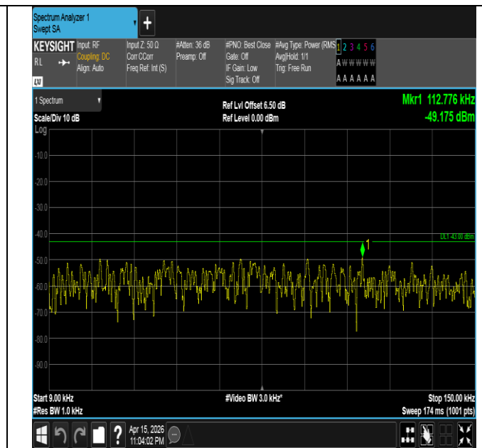
Band4-3MHz-QPSK-20175-1RB#14-0.009~0.15-PASS
