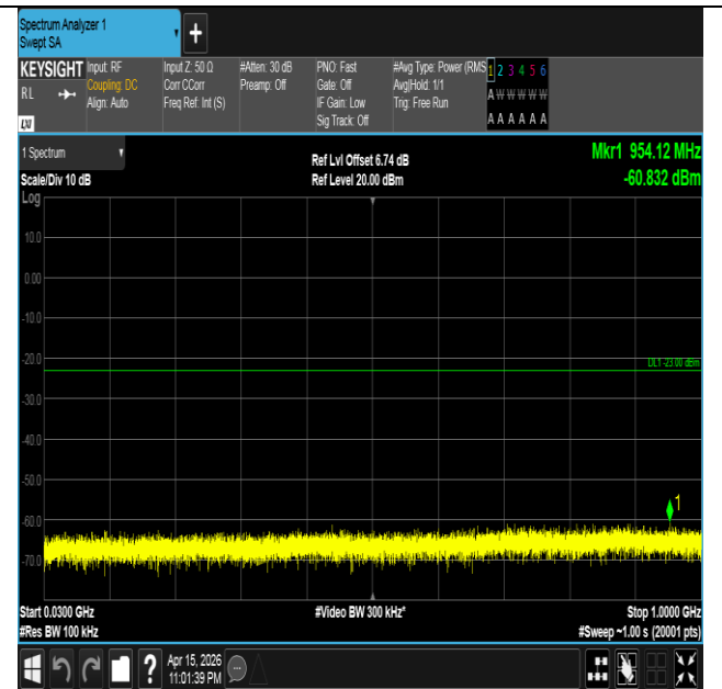
Band4-3MHz-16QAM-19965-15RB#0-30~1000-PASS
