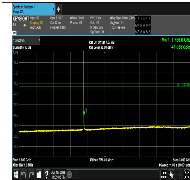
Band4-3MHz-16QAM-20385-1RB#0-1000~3000-PASS
