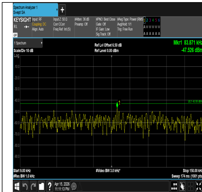
Band4-3MHz-QPSK-20385-15RB#0-0.009~0.15-PASS
