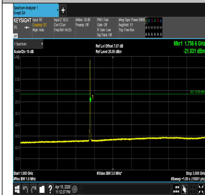
Band4-3MHz-16QAM-20385-15RB#0-1000~3000-PASS
