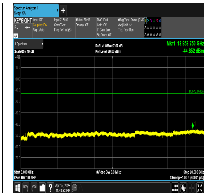
Band4-5MHz-QPSK-19975-1RB#0-3000~20000-PASS
