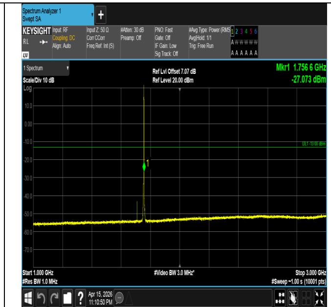
Band4-3MHz-16QAM-20385-1RB#14-1000~3000-PASS
