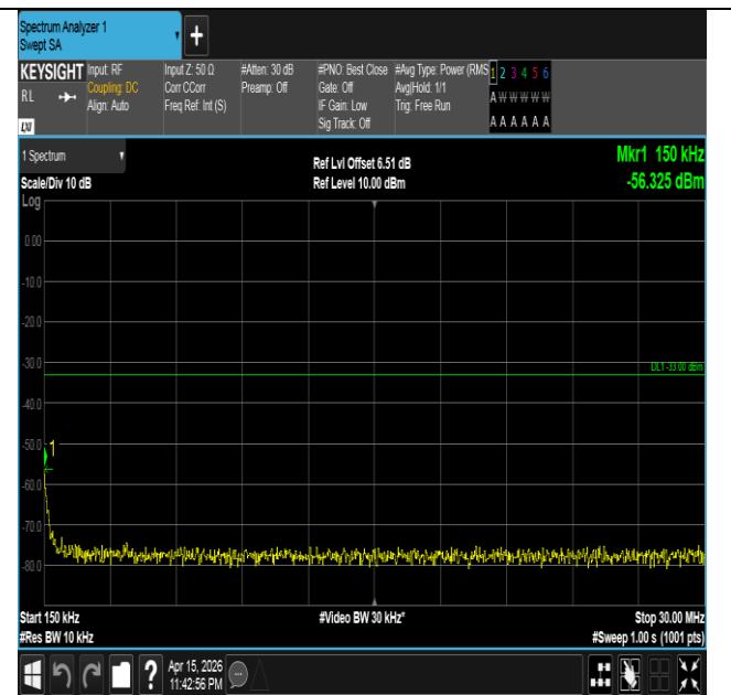
Band4-5MHz-QPSK-19975-1RB#0-0.15~30-PASS
