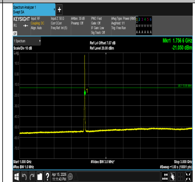
Band4-3MHz-QPSK-20385-15RB#0-1000~3000-PASS
