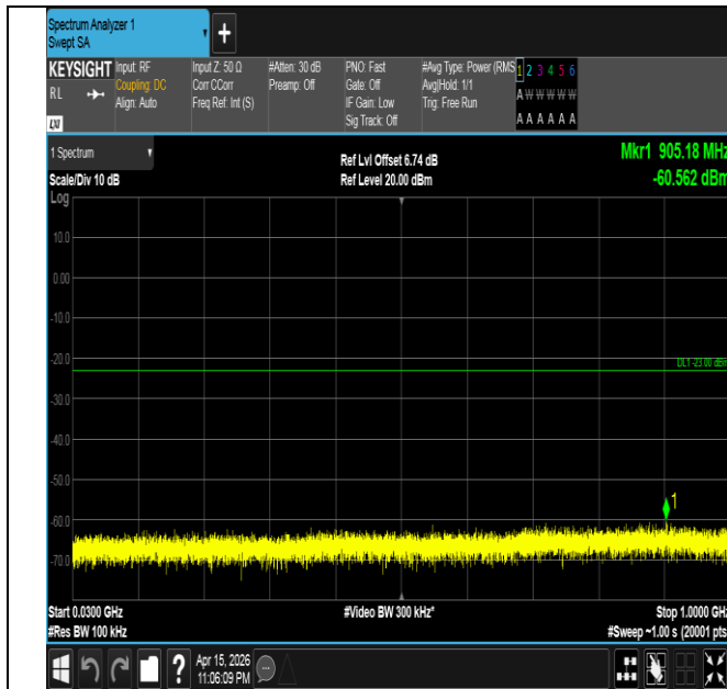
Band4-3MHz-QPSK-20175-15RB#0-30~1000-PASS
