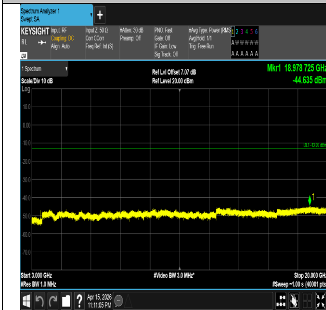
Band4-3MHz-16QAM-20385-1RB#14-3000~20000-PASS
