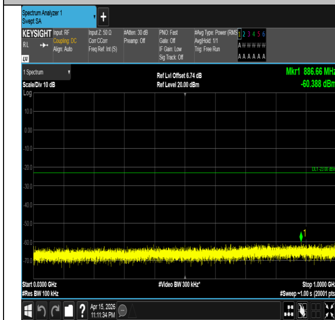
Band4-3MHz-QPSK-20385-15RB#0-30~1000-PASS
