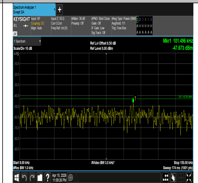
Band4-3MHz-QPSK-20385-1RB#14-0.009~0.15-PASS
