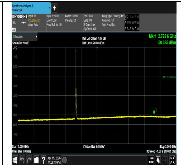
Band4-3MHz-QPSK-20175-15RB#0-1000~3000-PASS
