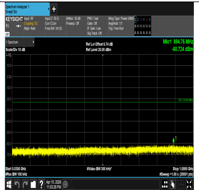
Band4-3MHz-16QAM-20175-1RB#0-30~1000-PASS
