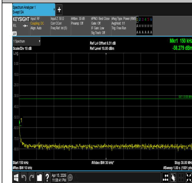
Band4-3MHz-16QAM-20385-1RB#0-0.15~30-PASS
