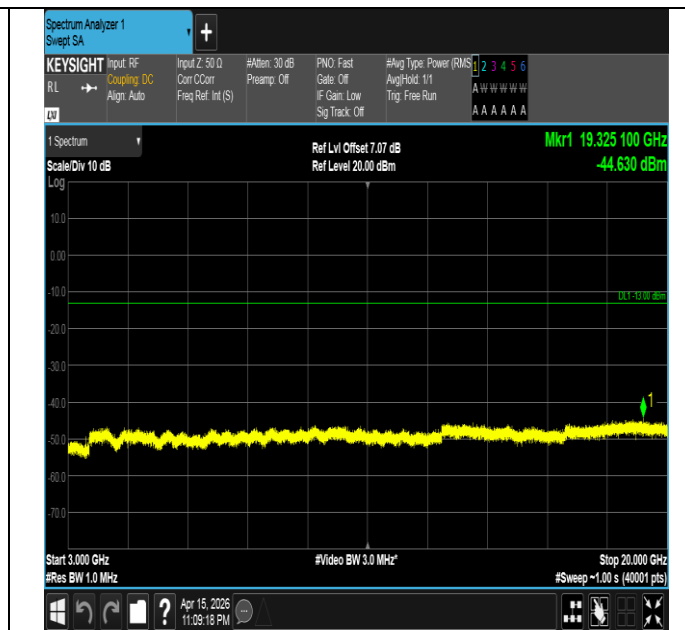
Band4-3MHz-16QAM-20385-1RB#0-3000~20000-PASS
