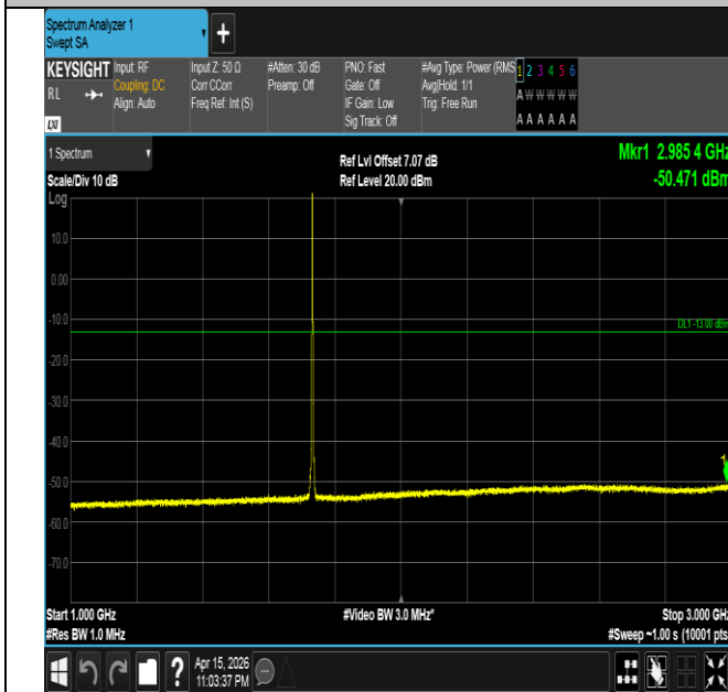
Band4-3MHz-16QAM-20175-1RB#0-1000~3000-PASS
