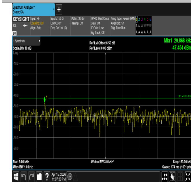
Band4-3MHz-QPSK-20385-1RB#0-0.009~0.15-PASS
