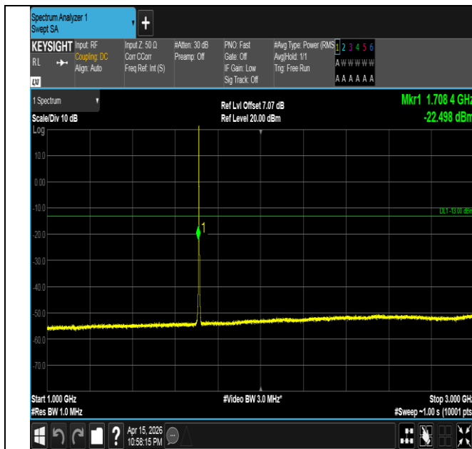
Band4-3MHz-16QAM-19965-1RB#0-1000~3000-PASS
