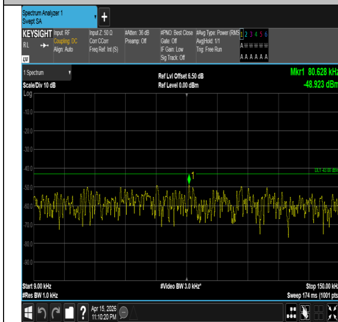
Band4-3MHz-16QAM-20385-1RB#14-0.009~0.15-PASS
