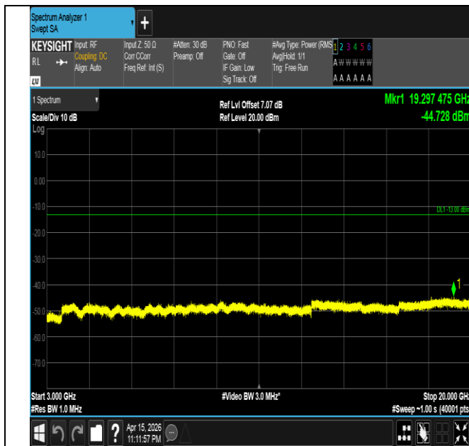
Band4-3MHz-QPSK-20385-15RB#0-3000~20000-PASS
