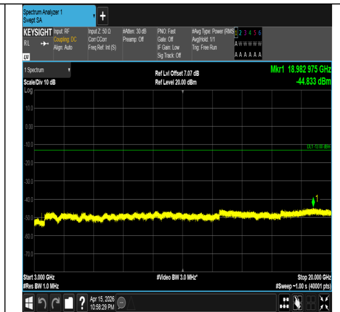
Band4-3MHz-16QAM-19965-1RB#0-3000~20000-PASS
