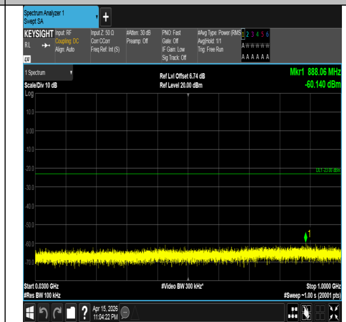
Band4-3MHz-QPSK-20175-1RB#14-30~1000-PASS
