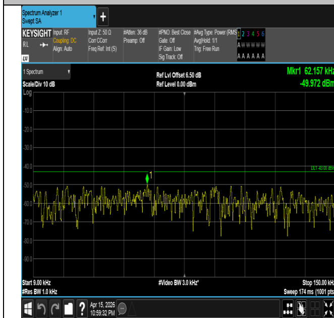
Band4-3MHz-16QAM-19965-1RB#14-0.009~0.15-PASS
