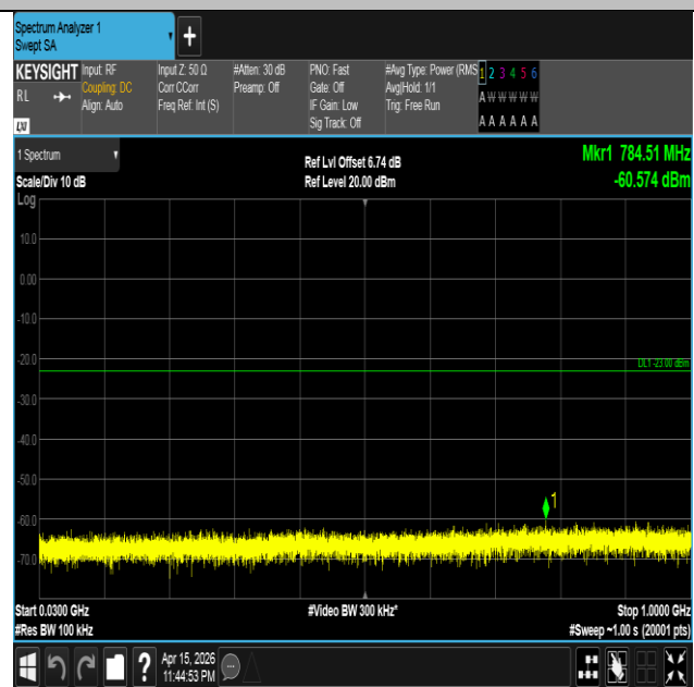
Band4-5MHz-QPSK-19975-1RB#24-30~1000-PASS
