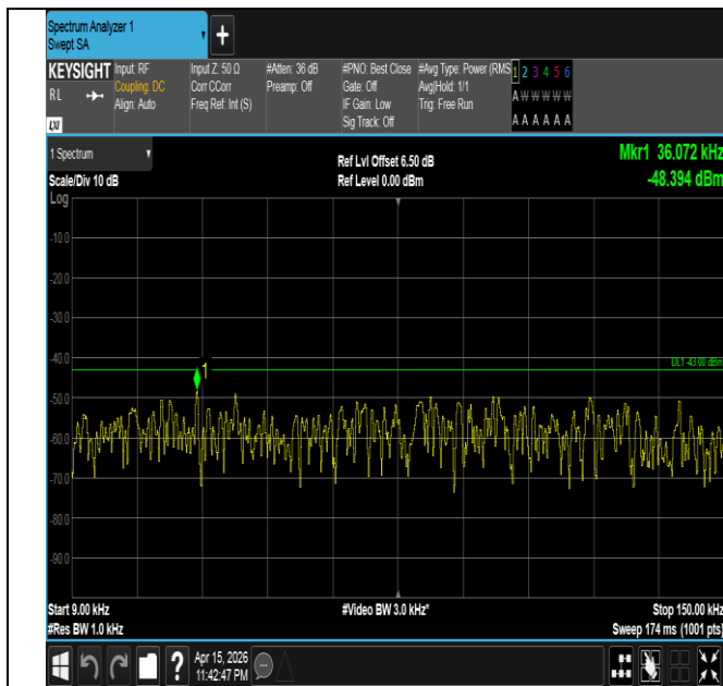
Band4-5MHz-QPSK-19975-1RB#0-0.009~0.15-PASS
