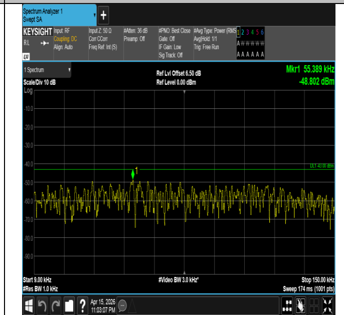
Band4-3MHz-16QAM-20175-1RB#0-0.009~0.15-PASS
