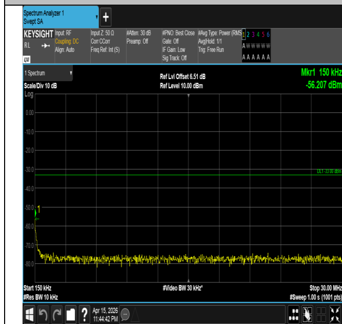
Band4-5MHz-QPSK-19975-1RB#24-0.15~30-PASS
