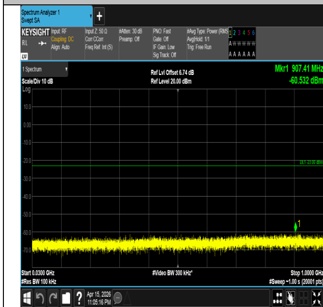
Band4-3MHz-16QAM-20175-1RB#14-30~1000-PASS
