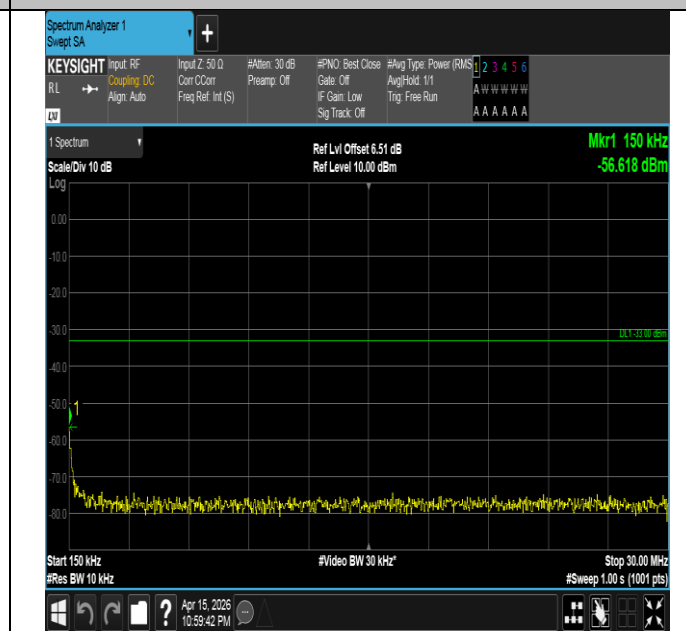
Band4-3MHz-16QAM-19965-1RB#14-0.15~30-PASS
