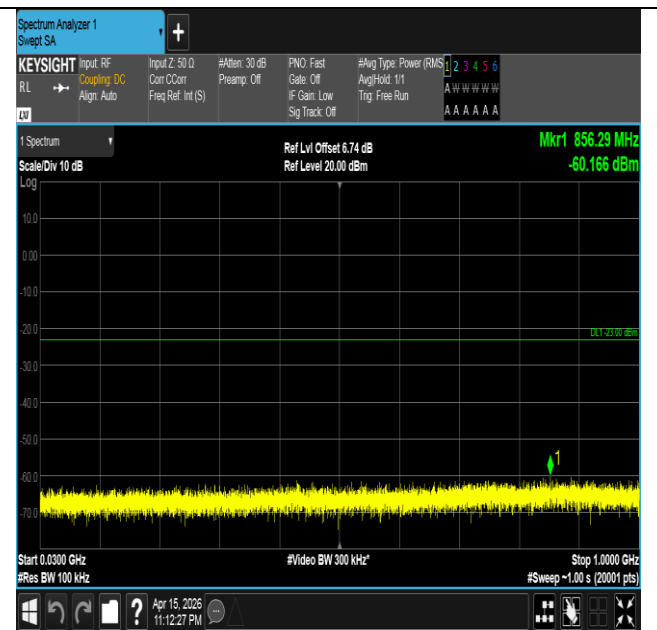
Band4-3MHz-16QAM-20385-15RB#0-30~1000-PASS
