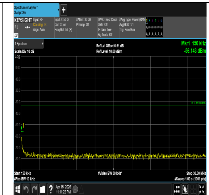
Band4-3MHz-QPSK-20385-15RB#0-0.15~30-PASS
