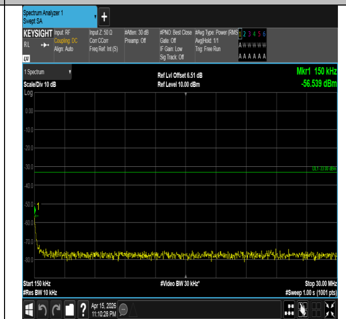
Band4-3MHz-16QAM-20385-1RB#14-0.15~30-PASS
