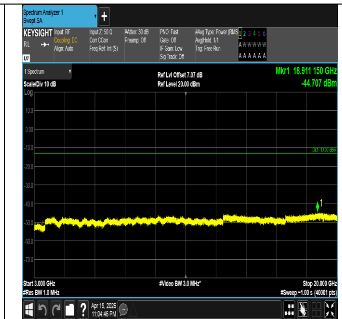
Band4-3MHz-QPSK-20175-1RB#14-3000~20000-PASS
