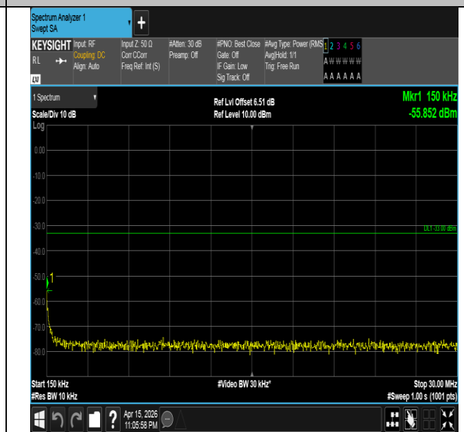
Band4-3MHz-QPSK-20175-15RB#0-0.15~30-PASS
