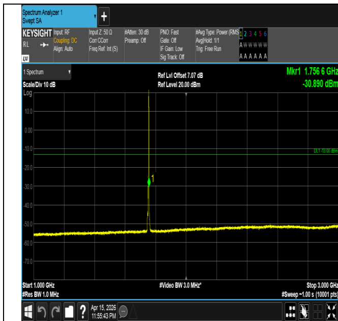
Band4-5MHz-QPSK-20375-1RB#24-1000~3000-PASS
