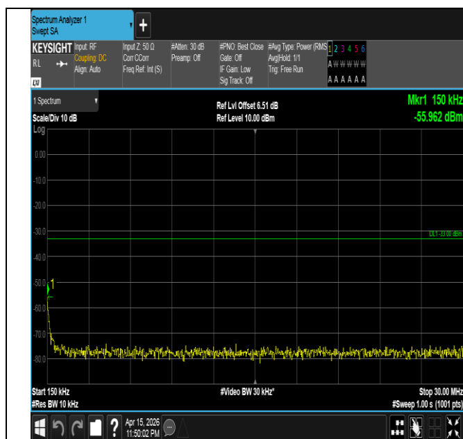
Band4-5MHz-QPSK-20175-1RB#24-0.15~30-PASS
