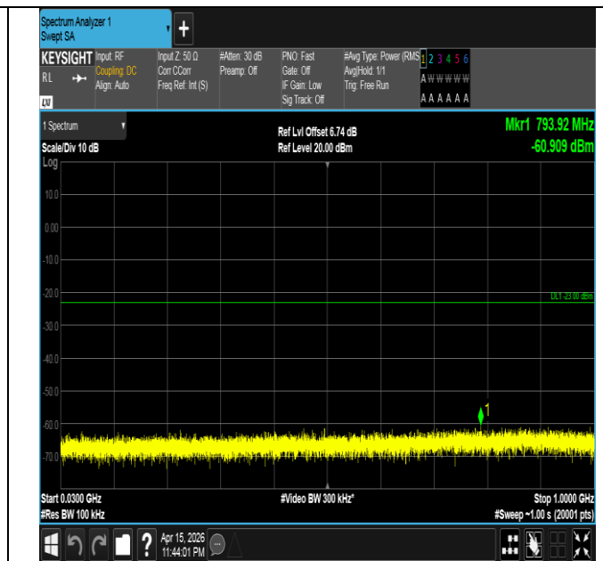
Band4-5MHz-16QAM-19975-1RB#0-30~1000-PASS
