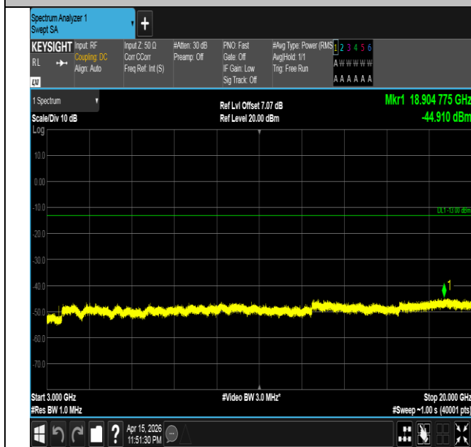
Band4-5MHz-16QAM-20175-1RB#24-3000~20000-PASS
