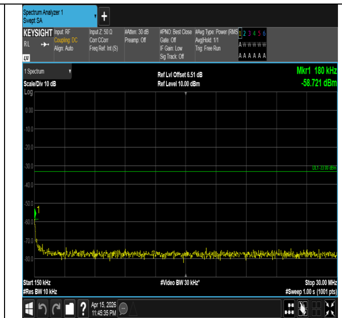
Band4-5MHz-16QAM-19975-1RB#24-0.15~30-PASS
