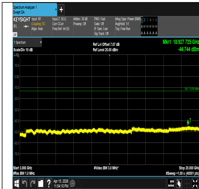
Band4-5MHz-QPSK-20375-1RB#0-3000~20000-PASS
