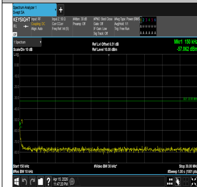
Band4-5MHz-16QAM-19975-25RB#0-0.15~30-PASS
