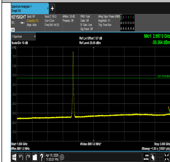
Band4-5MHz-16QAM-20175-25RB#0-1000~3000-PASS
