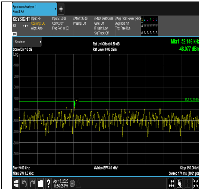
Band4-5MHz-16QAM-20375-1RB#24-0.009~0.15-PASS
