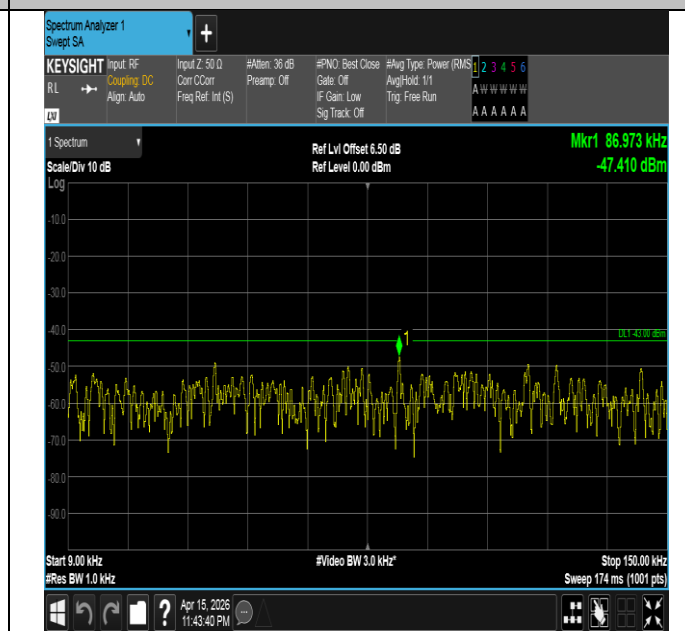
Band4-5MHz-16QAM-19975-1RB#0-0.009~0.15-PASS
