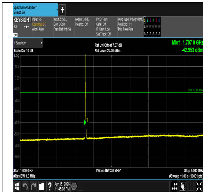
Band4-5MHz-QPSK-19975-1RB#24-1000~3000-PASS
