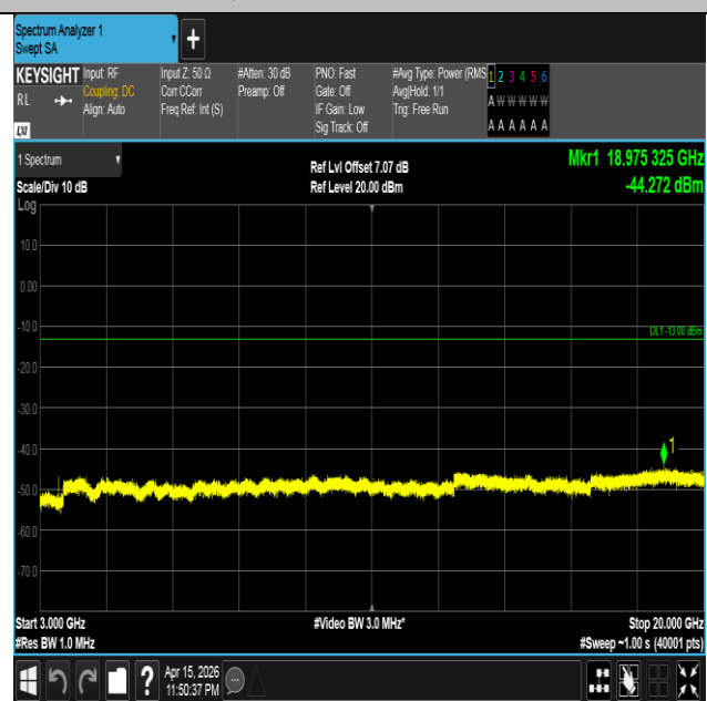
Band4-5MHz-QPSK-20175-1RB#24-3000~20000-PASS
