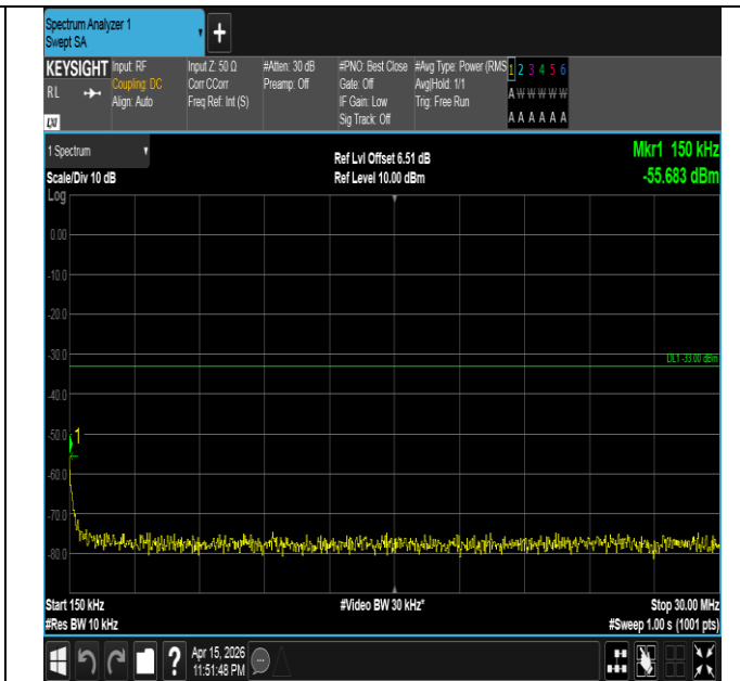
Band4-5MHz-QPSK-20175-25RB#0-0.15~30-PASS
