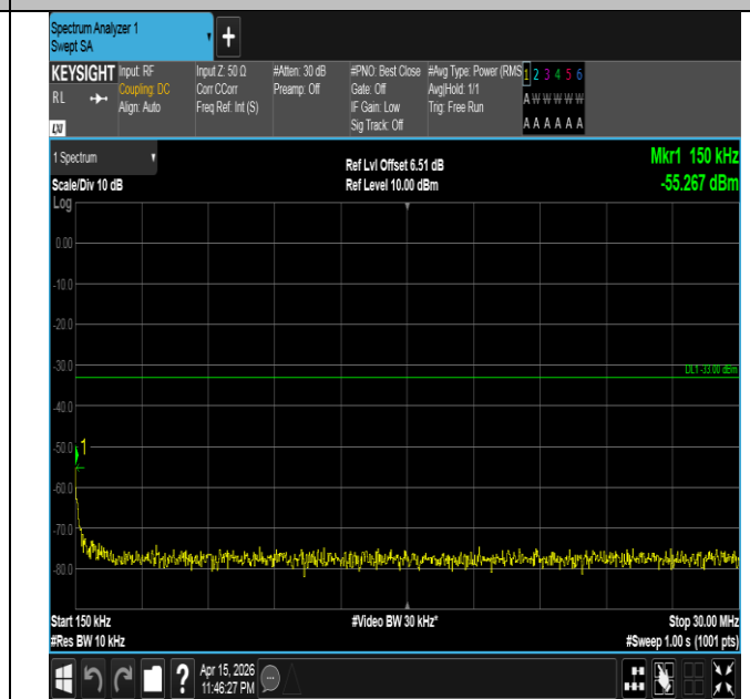
Band4-5MHz-QPSK-19975-25RB#0-0.15~30-PASS
