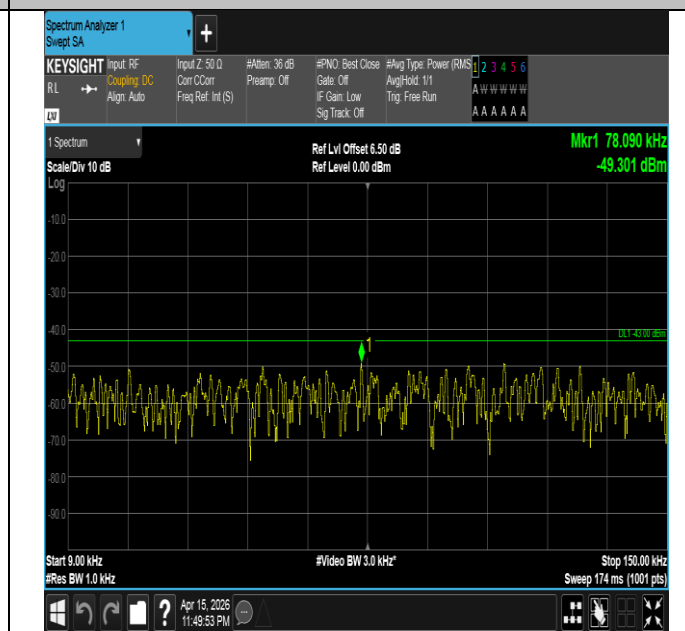
Band4-5MHz-QPSK-20175-1RB#24-0.009~0.15-PASS
