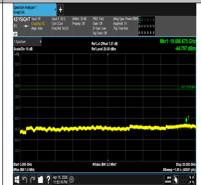
Band4-5MHz-16QAM-20175-25RB#0-3000~20000-PASS
