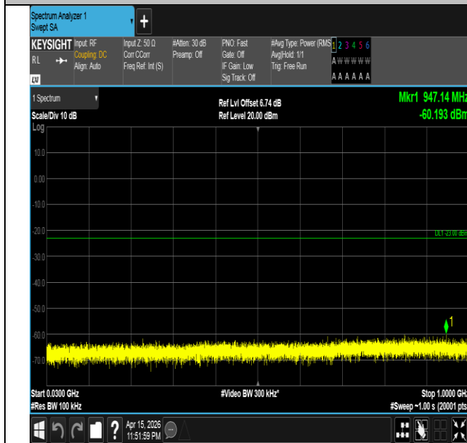
Band4-5MHz-QPSK-20175-25RB#0-30~1000-PASS
