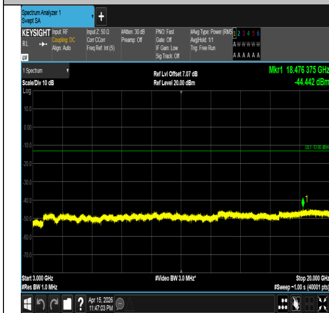
Band4-5MHz-QPSK-19975-25RB#0-3000~20000-PASS
