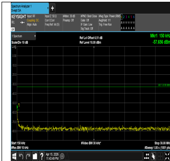
Band4-5MHz-16QAM-19975-1RB#0-0.15~30-PASS
