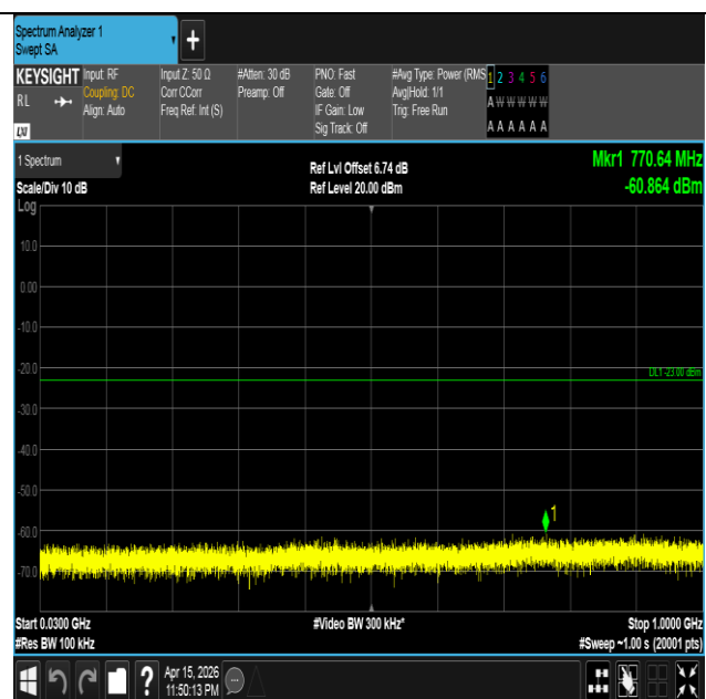
Band4-5MHz-QPSK-20175-1RB#24-30~1000-PASS
