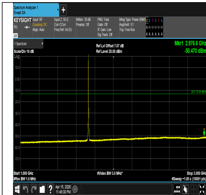
Band4-5MHz-16QAM-20175-1RB#0-1000~3000-PASS
