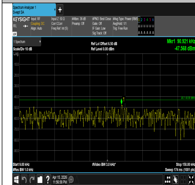
Band4-5MHz-QPSK-20375-25RB#0-0.009~0.15-PASS
