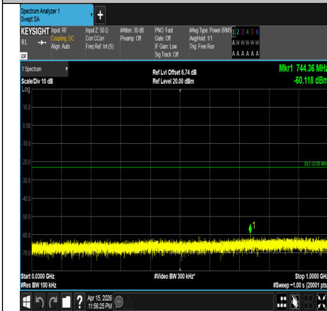
Band4-5MHz-16QAM-20375-1RB#24-30~1000-PASS
