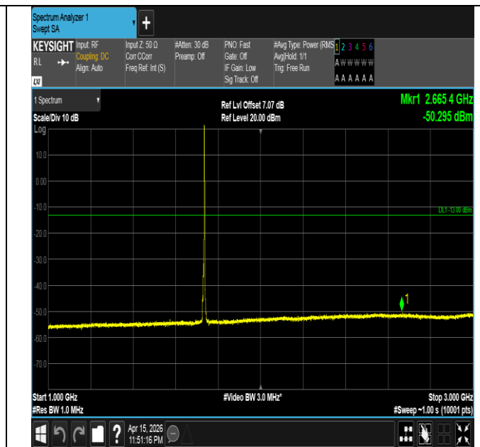
Band4-5MHz-16QAM-20175-1RB#24-1000~3000-PASS
