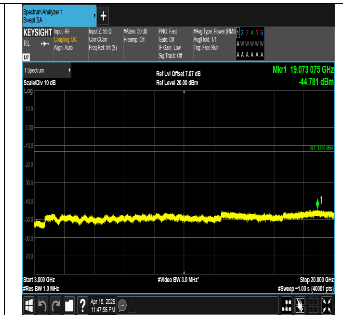
Band4-5MHz-16QAM-19975-25RB#0-3000~20000-PASS
