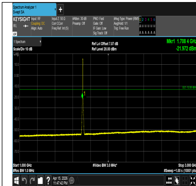
Band4-5MHz-16QAM-19975-25RB#0-1000~3000-PASS
