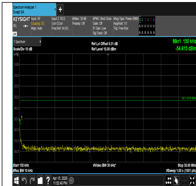
Band4-5MHz-16QAM-20175-25RB#0-0.15~30-PASS
