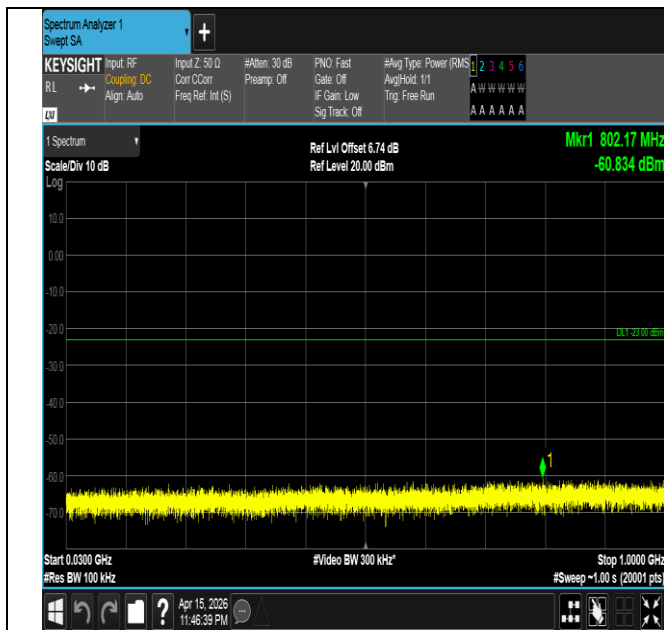
Band4-5MHz-QPSK-19975-25RB#0-30~1000-PASS
