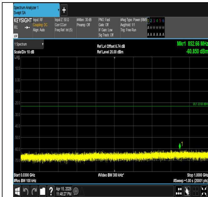
Band4-5MHz-QPSK-20175-1RB#0-30~1000-PASS
