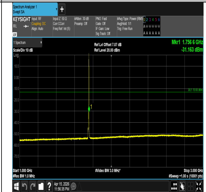
Band4-5MHz-16QAM-20375-1RB#24-1000~3000-PASS
