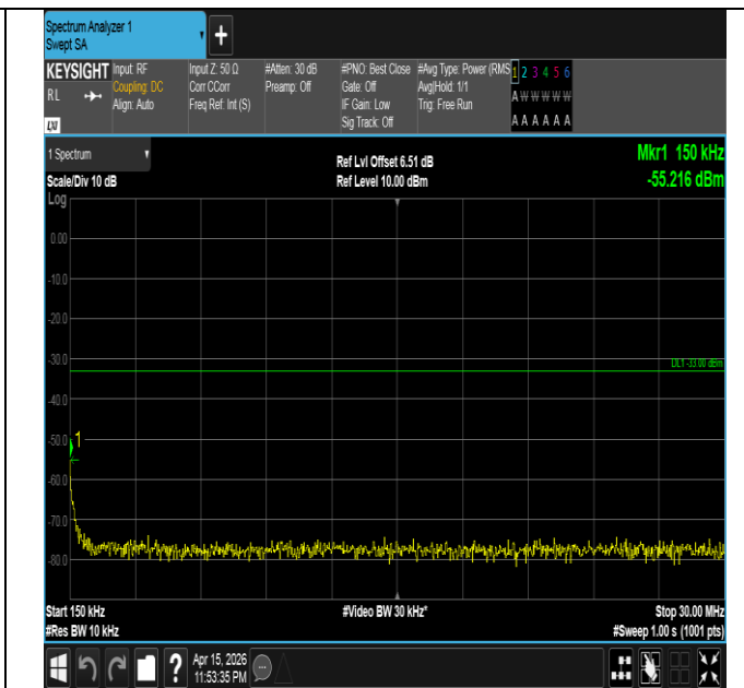
Band4-5MHz-QPSK-20375-1RB#0-0.15~30-PASS
