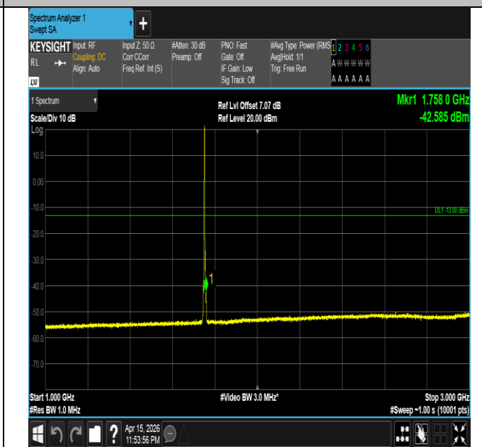
Band4-5MHz-QPSK-20375-1RB#0-1000~3000-PASS
