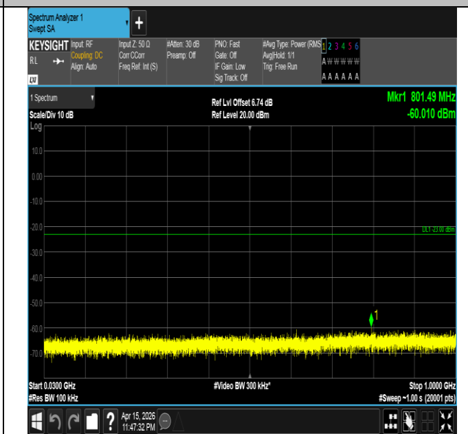
Band4-5MHz-16QAM-19975-25RB#0-30~1000-PASS
