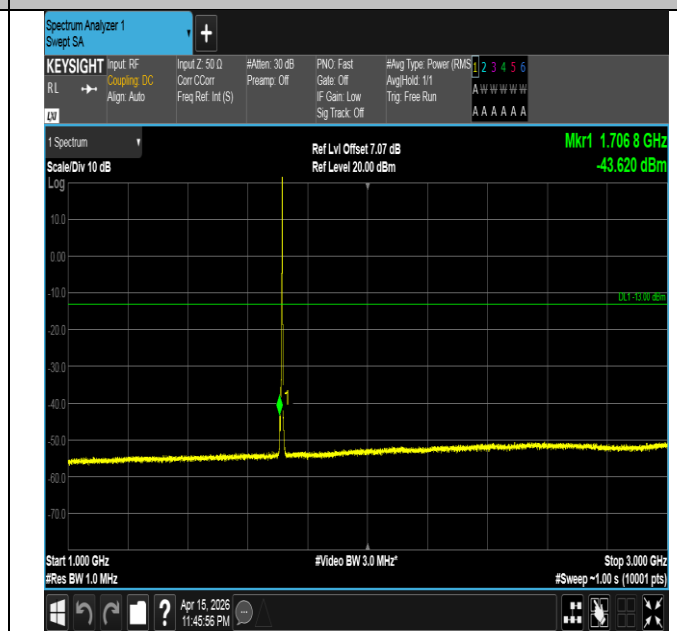
Band4-5MHz-16QAM-19975-1RB#24-1000~3000-PASS
