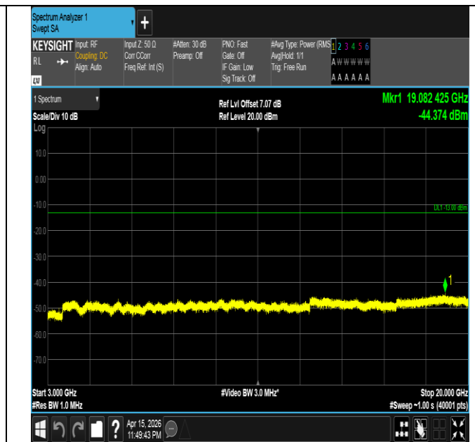
Band4-5MHz-16QAM-20175-1RB#0-3000~20000-PASS
