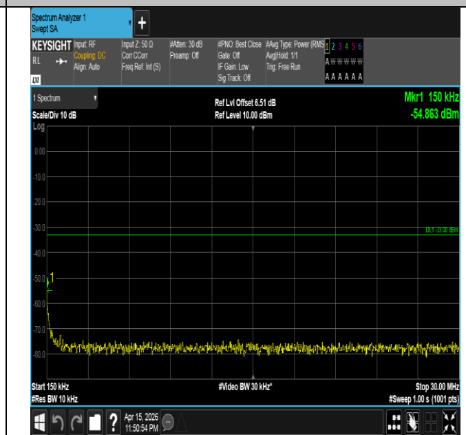
Band4-5MHz-16QAM-20175-1RB#24-0.15~30-PASS
