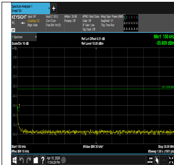
Band4-5MHz-16QAM-20375-1RB#0-0.15~30-PASS
