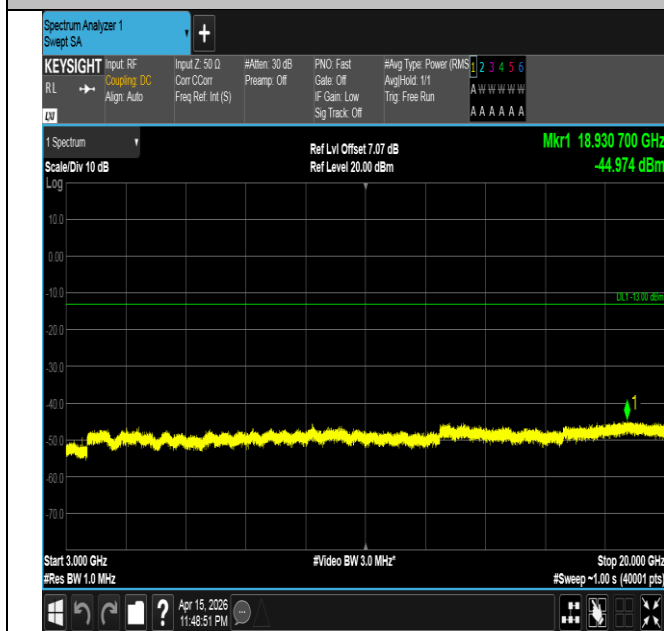
Band4-5MHz-QPSK-20175-1RB#0-3000~20000-PASS
