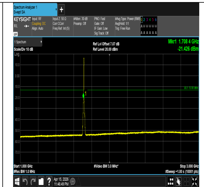
Band4-5MHz-QPSK-19975-25RB#0-1000~3000-PASS
