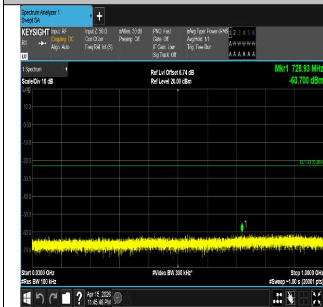
Band4-5MHz-16QAM-19975-1RB#24-30~1000-PASS
