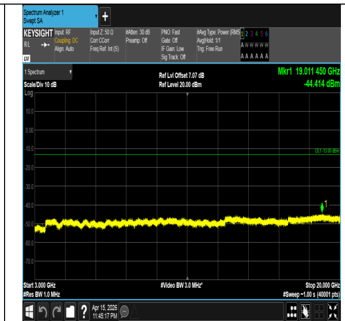
Band4-5MHz-QPSK-19975-1RB#24-3000~20000-PASS
