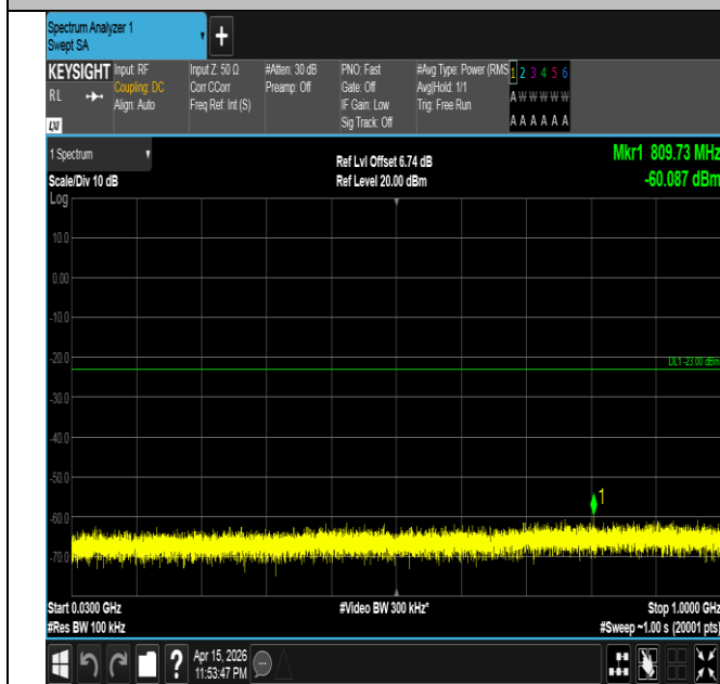
Band4-5MHz-QPSK-20375-1RB#0-30~1000-PASS
