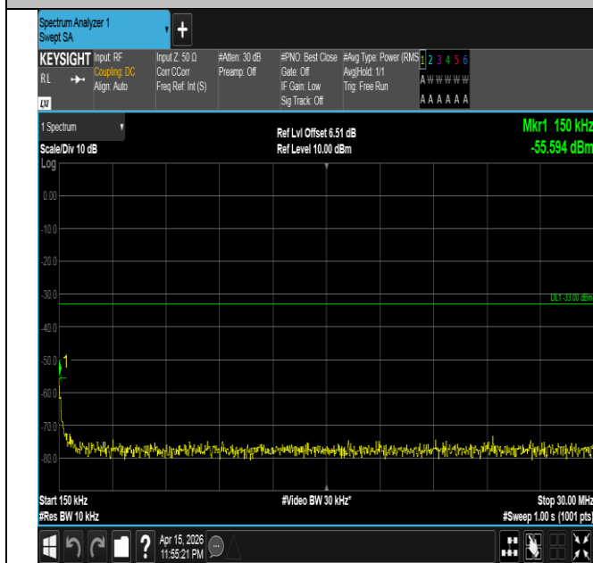
Band4-5MHz-QPSK-20375-1RB#24-0.15~30-PASS
