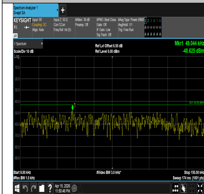
Band4-5MHz-16QAM-20175-1RB#24-0.009~0.15-PASS
