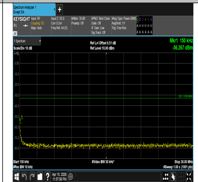
Band4-5MHz-QPSK-20375-25RB#0-0.15~30-PASS
