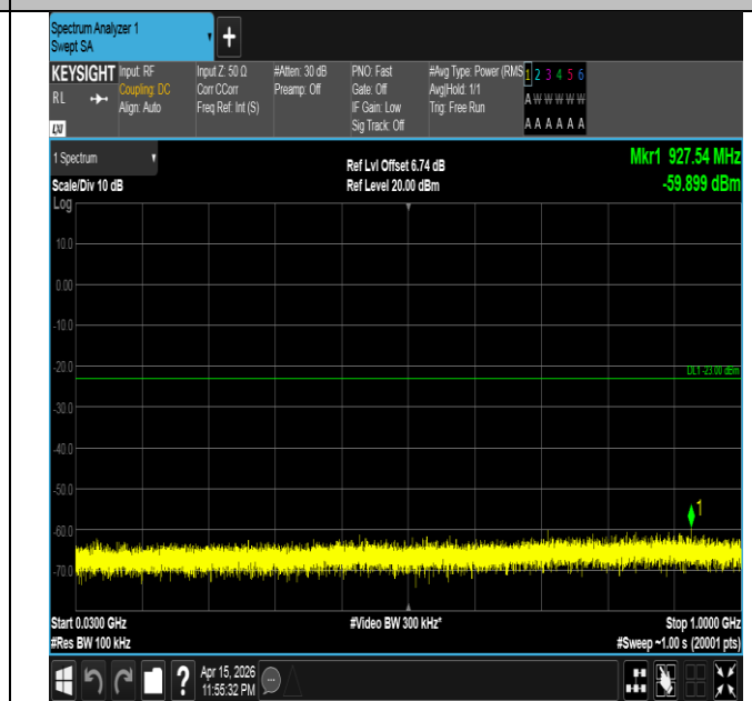
Band4-5MHz-QPSK-20375-1RB#24-30~1000-PASS
