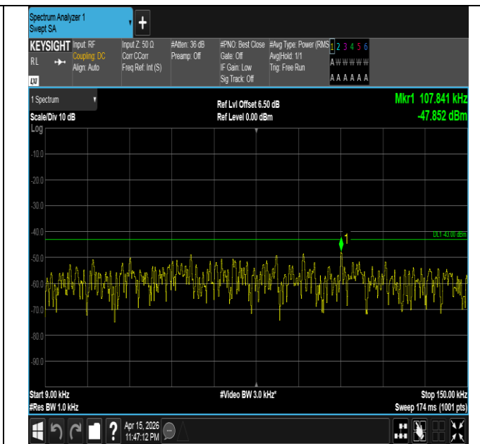
Band4-5MHz-16QAM-19975-25RB#0-0.009~0.15-PASS
