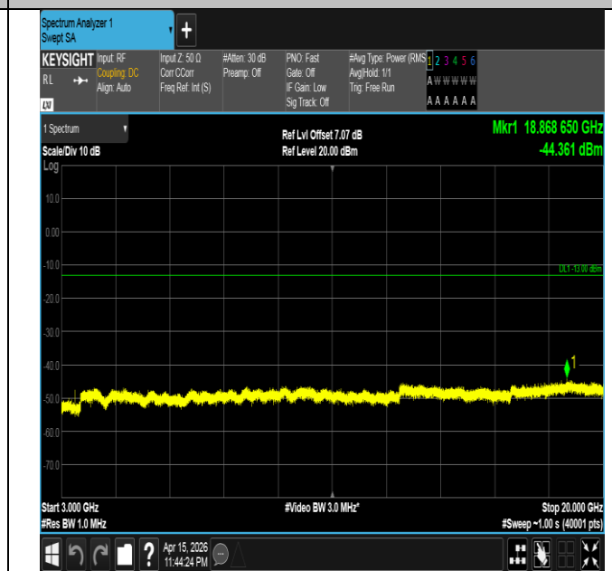
Band4-5MHz-16QAM-19975-1RB#0-3000~20000-PASS
