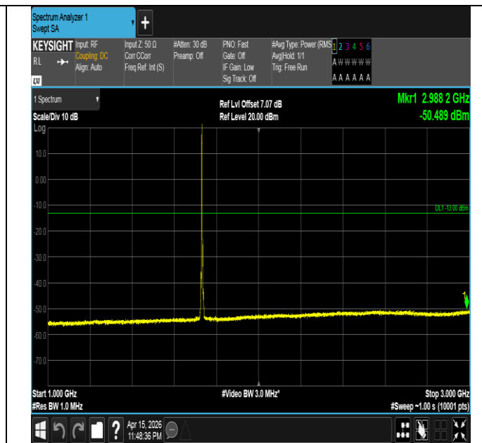
Band4-5MHz-QPSK-20175-1RB#0-1000~3000-PASS
