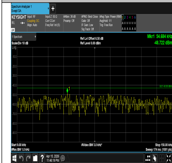
Band4-5MHz-QPSK-19975-25RB#0-0.009~0.15-PASS
