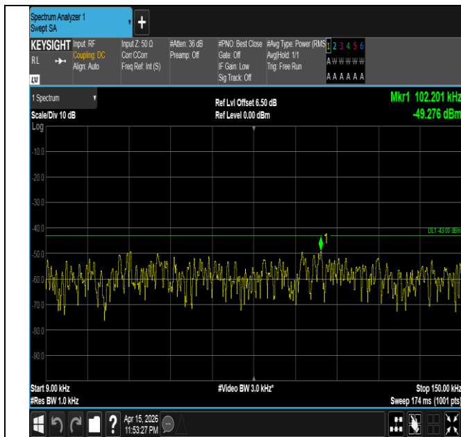
Band4-5MHz-QPSK-20375-1RB#0-0.009~0.15-PASS
