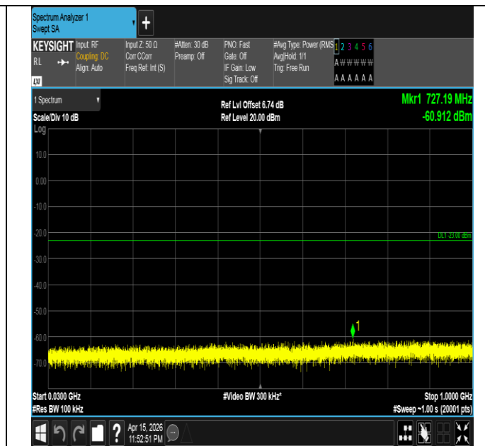
Band4-5MHz-16QAM-20175-25RB#0-30~1000-PASS
