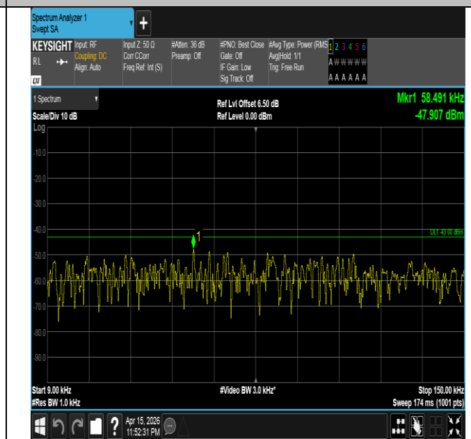
Band4-5MHz-16QAM-20175-25RB#0-0.009~0.15-PASS
