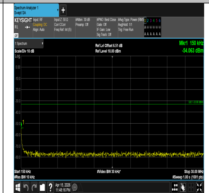
Band4-5MHz-QPSK-20175-1RB#0-0.15~30-PASS
