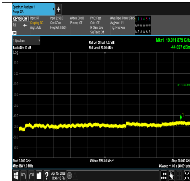
Band4-5MHz-16QAM-19975-1RB#24-3000~20000-PASS
