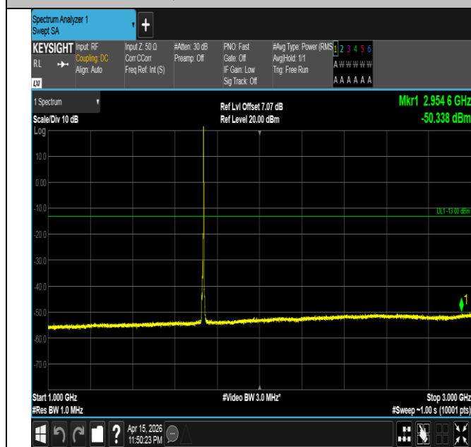
Band4-5MHz-QPSK-20175-1RB#24-1000~3000-PASS
