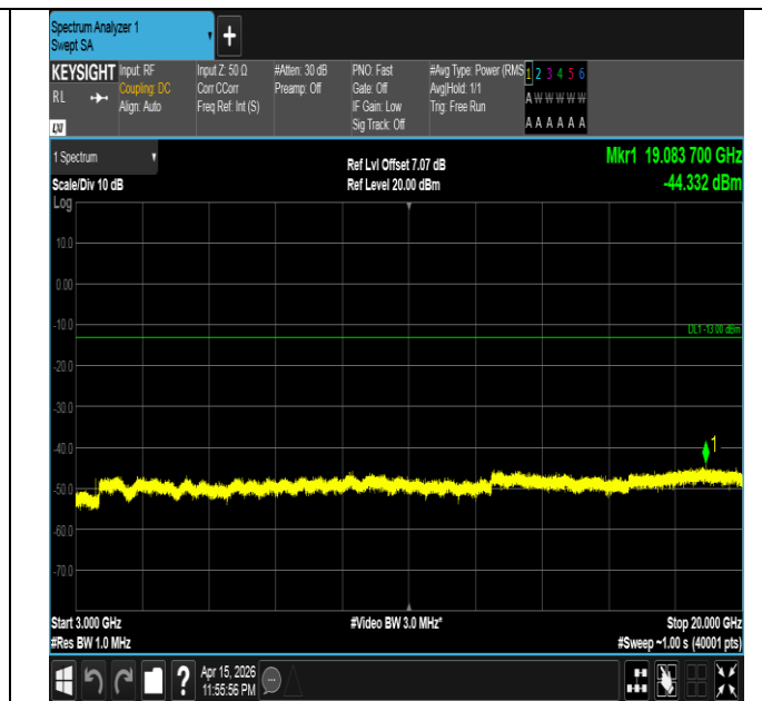
Band4-5MHz-QPSK-20375-1RB#24-3000~20000-PASS
