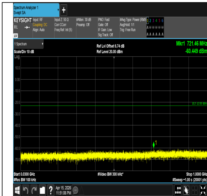
Band4-5MHz-16QAM-20175-1RB#24-30~1000-PASS
