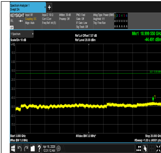
Band4-10MHz-QPSK-20000-50RB#0-3000~20000-PASS
