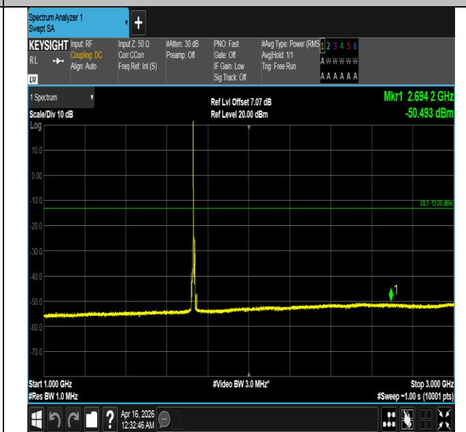
Band4-10MHz-QPSK-20175-1RB#0-1000~3000-PASS
