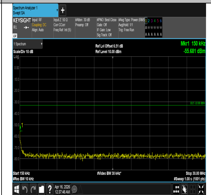
Band4-10MHz-QPSK-20350-1RB#0-0.15~30-PASS
