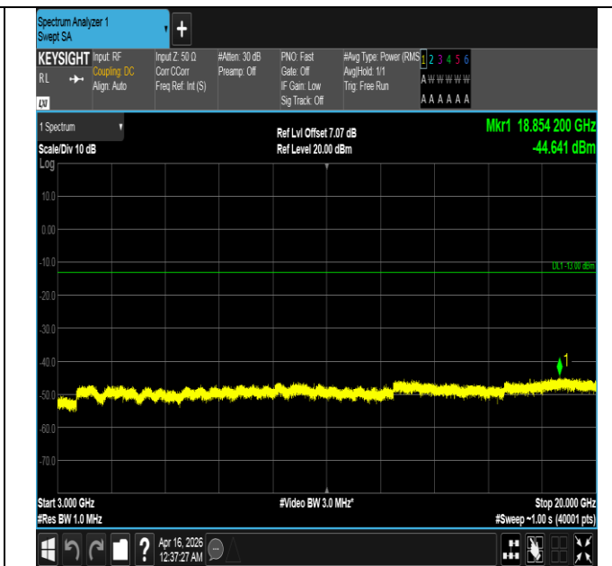
Band4-10MHz-16QAM-20175-50RB#0-3000~20000-PASS
