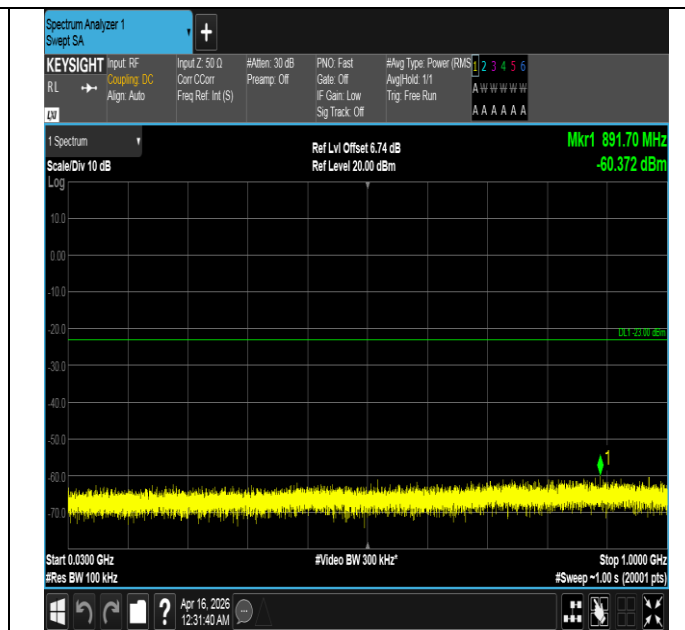
Band4-10MHz-16QAM-20000-50RB#0-30~1000-PASS
