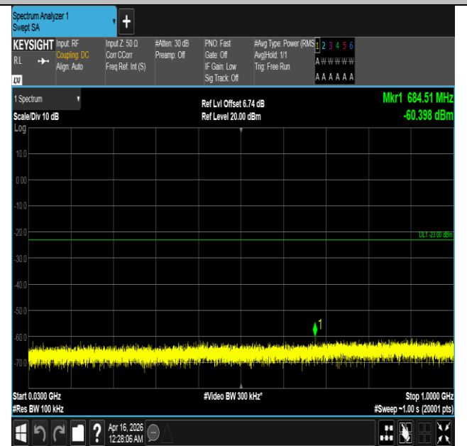
Band4-10MHz-16QAM-20000-1RB#0-30~1000-PASS
