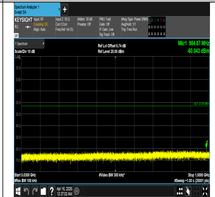
Band4-10MHz-16QAM-20175-50RB#0-30~1000-PASS
