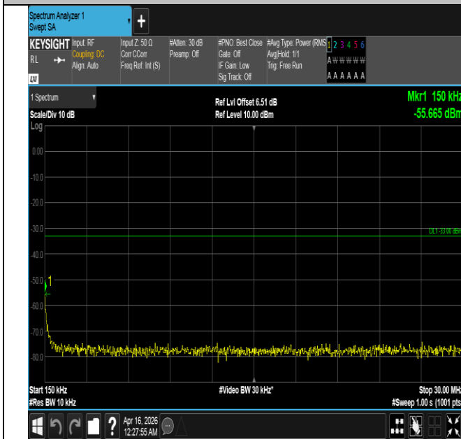
Band4-10MHz-16QAM-20000-1RB#0-0.15~30-PASS
