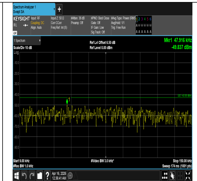
Band4-10MHz-16QAM-20175-50RB#0-0.009~0.15-PASS
