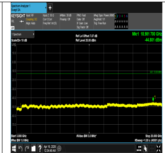
Band4-10MHz-QPSK-20175-1RB#49-3000~20000-PASS
