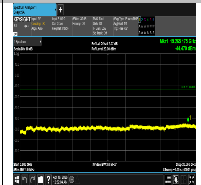
Band4-10MHz-16QAM-20000-50RB#0-3000~20000-PASS
