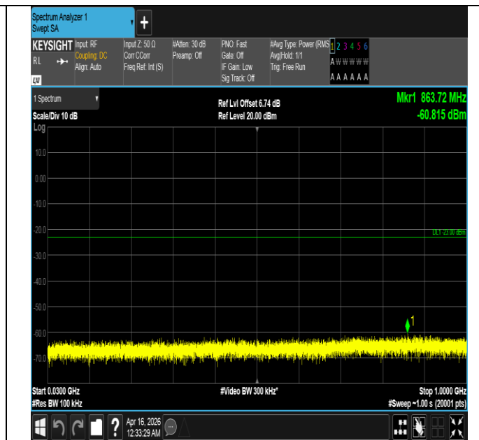
Band4-10MHz-16QAM-20175-1RB#0-30~1000-PASS
