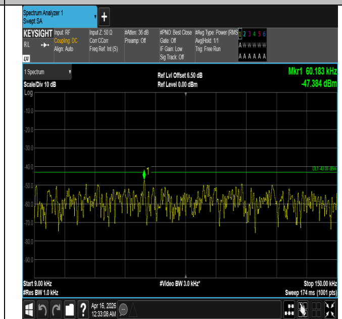
Band4-10MHz-16QAM-20175-1RB#0-0.009~0.15-PASS
