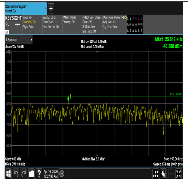
Band4-10MHz-16QAM-20000-1RB#0-0.009~0.15-PASS
