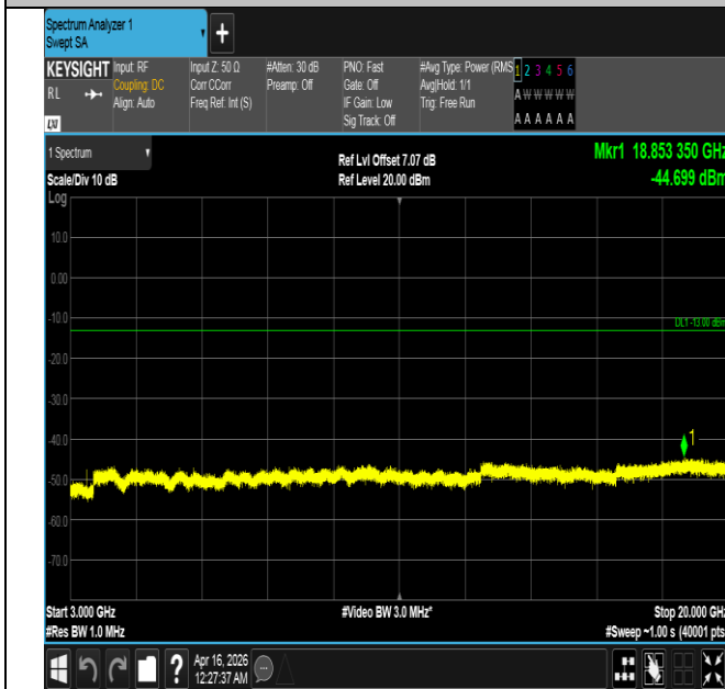
Band4-10MHz-QPSK-20000-1RB#0-3000~20000-PASS
