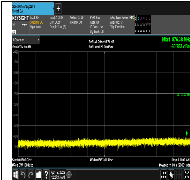
Band4-10MHz-QPSK-20000-1RB#0-30~1000-PASS
