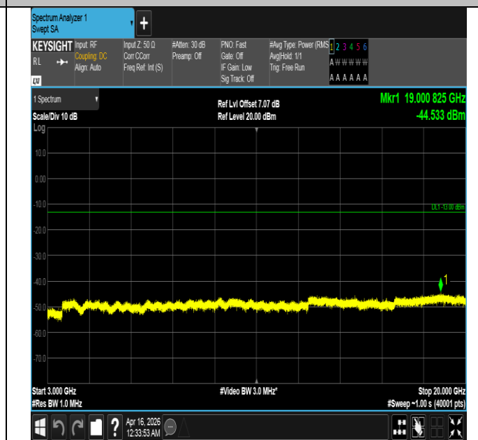
Band4-10MHz-16QAM-20175-1RB#0-3000~20000-PASS
