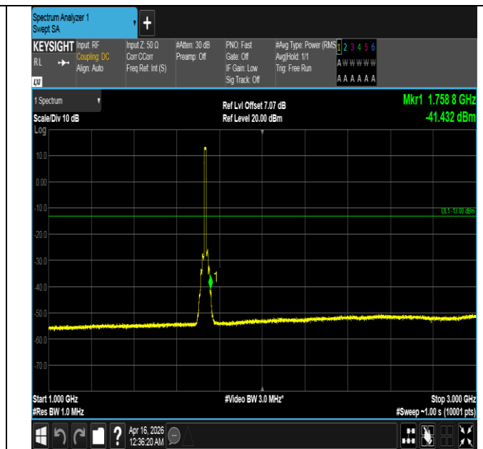
Band4-10MHz-QPSK-20175-50RB#0-1000~3000-PASS
