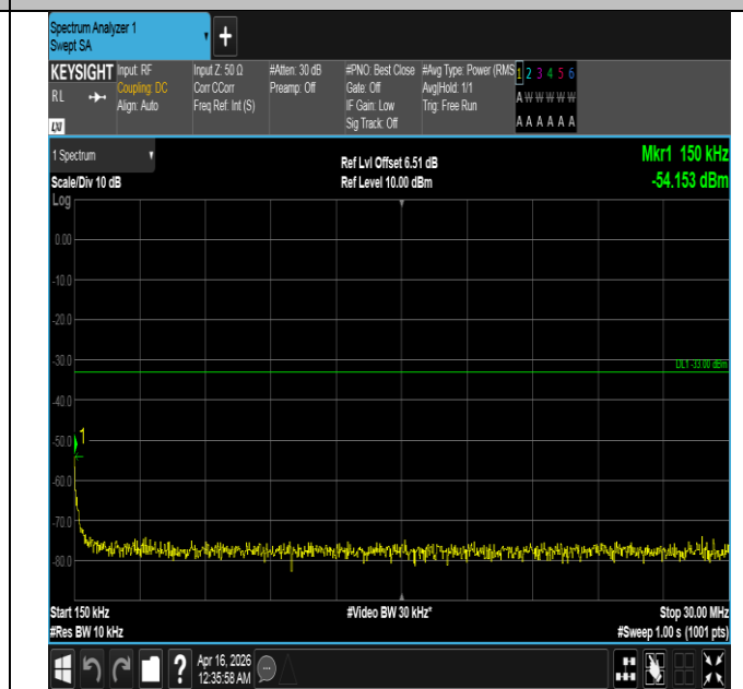
Band4-10MHz-QPSK-20175-50RB#0-0.15~30-PASS
