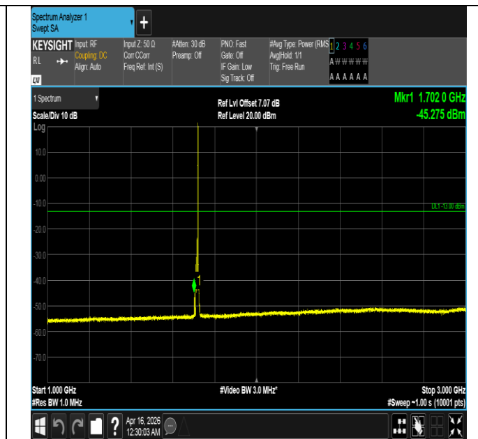
Band4-10MHz-16QAM-20000-1RB#49-1000~3000-PASS
