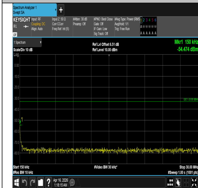
Band4-15MHz-16QAM-20175-1RB#0-0.15~30-PASS
