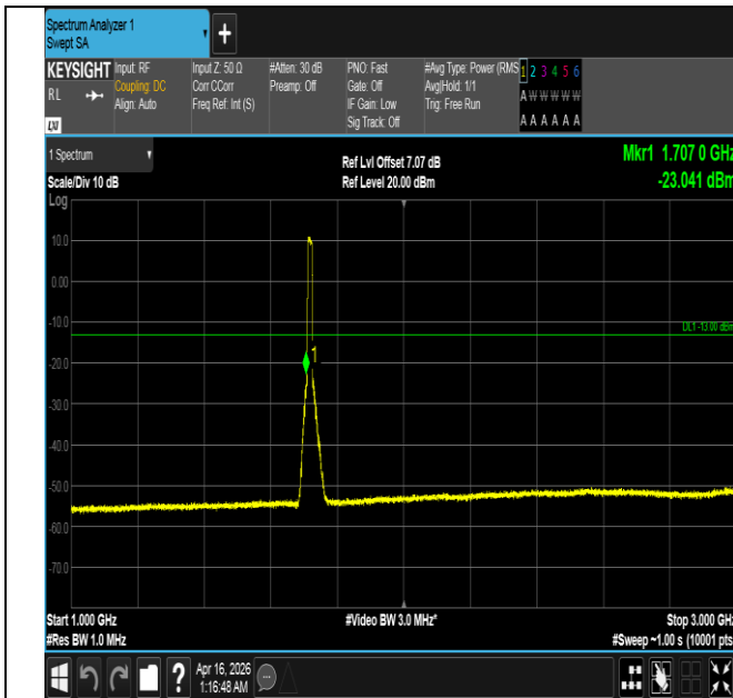
Band4-15MHz-16QAM-20025-75RB#0-1000~3000-PASS
