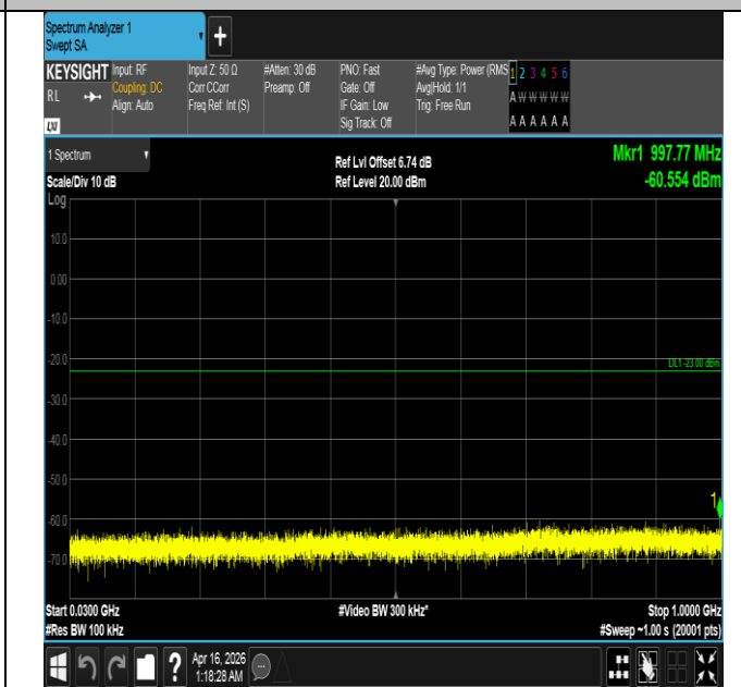
Band4-15MHz-16QAM-20175-1RB#0-30~1000-PASS
