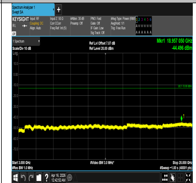
Band4-10MHz-16QAM-20350-50RB#0-3000~20000-PASS
