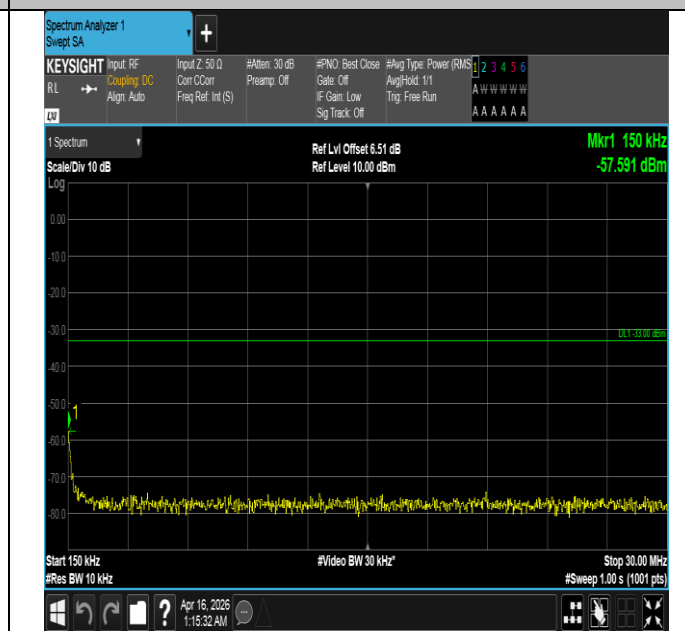
Band4-15MHz-QPSK-20025-75RB#0-0.15~30-PASS
