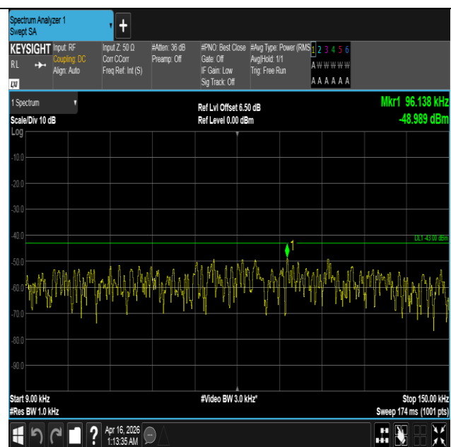
Band4-15MHz-QPSK-20025-1RB#74-0.009~0.15-PASS
