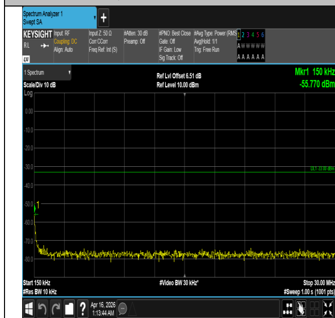
Band4-15MHz-QPSK-20025-1RB#74-0.15~30-PASS
