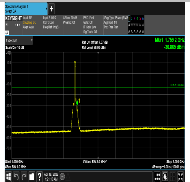
Band4-15MHz-QPSK-20175-75RB#0-1000~3000-PASS
