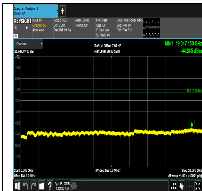
Band4-15MHz-QPSK-20025-1RB#0-3000~20000-PASS
