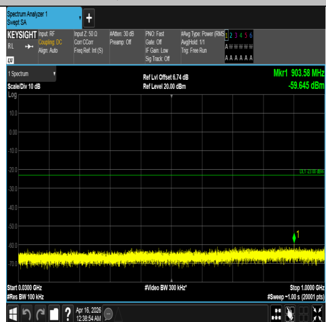
Band4-10MHz-16QAM-20350-1RB#0-30~1000-PASS
