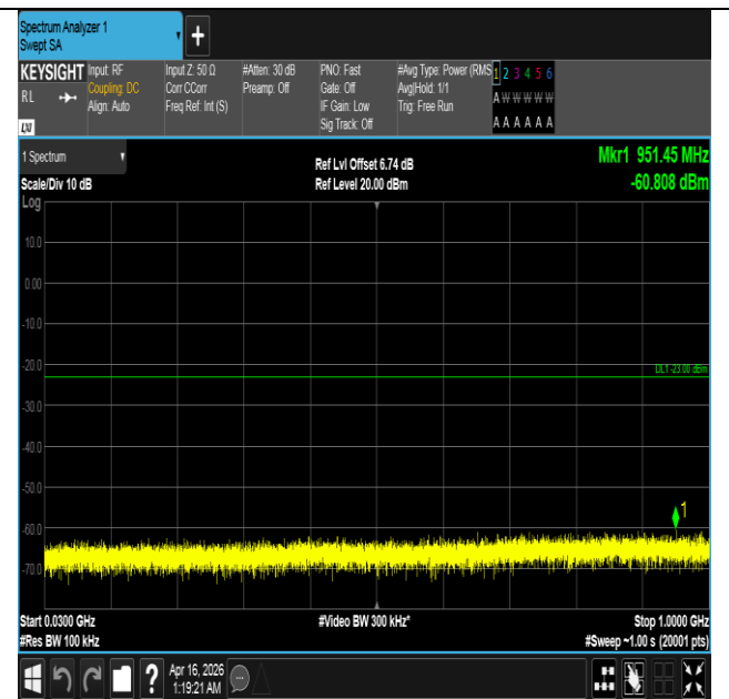
Band4-15MHz-QPSK-20175-1RB#74-30~1000-PASS
