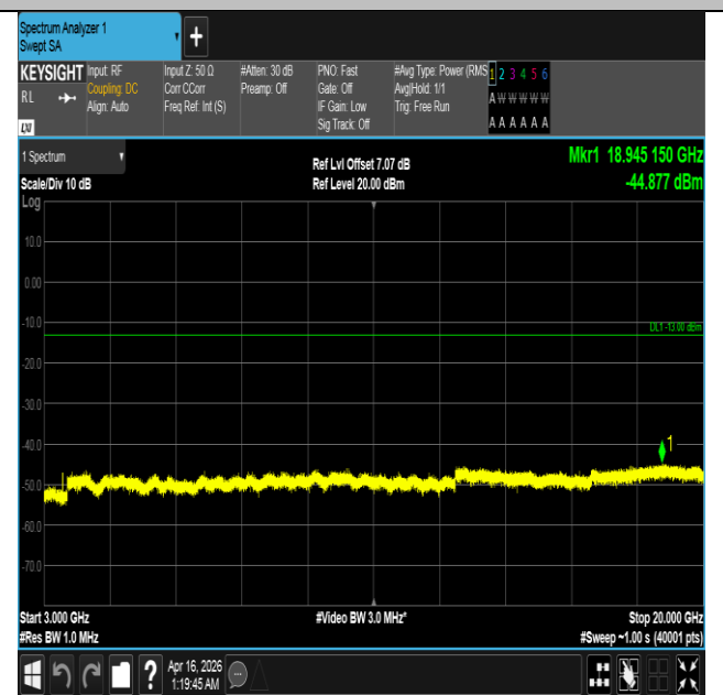
Band4-15MHz-QPSK-20175-1RB#74-3000~20000-PASS
