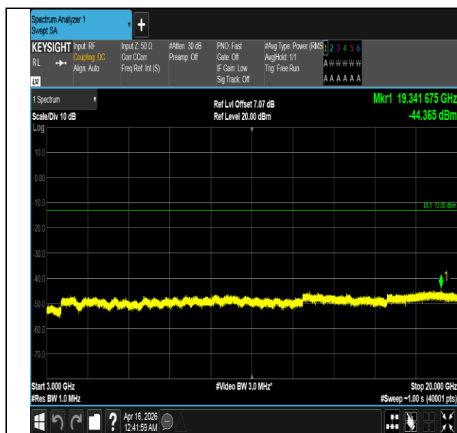
Band4-10MHz-QPSK-20350-50RB#0-3000~20000-PASS
