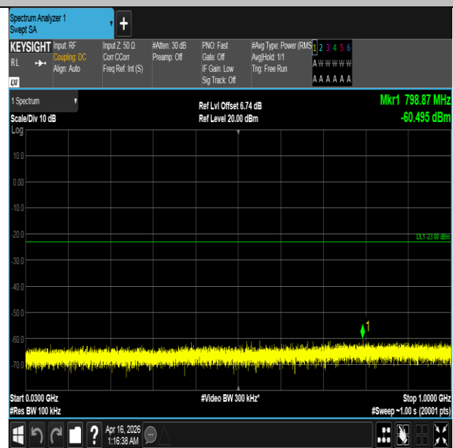
Band4-15MHz-16QAM-20025-75RB#0-30~1000-PASS
