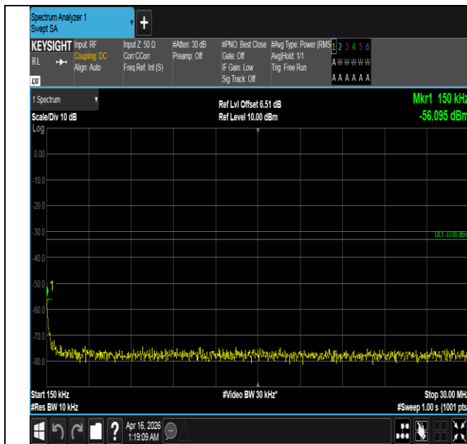
Band4-15MHz-QPSK-20175-1RB#74-0.15~30-PASS
