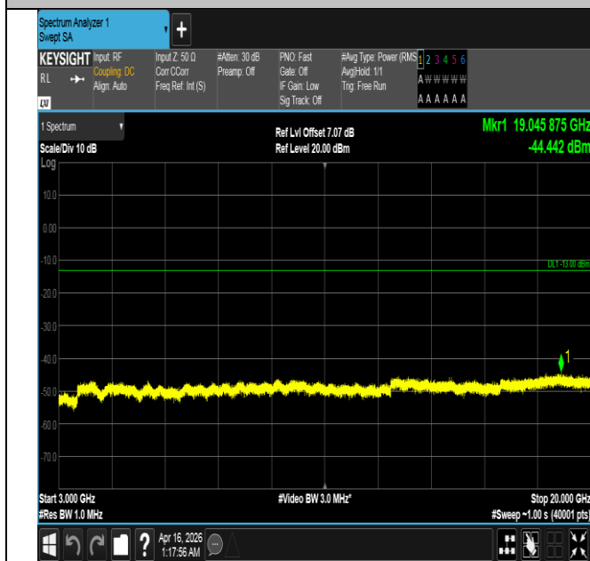
Band4-15MHz-QPSK-20175-1RB#0-3000~20000-PASS
