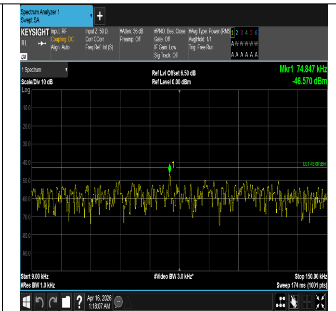
Band4-15MHz-16QAM-20175-1RB#0-0.009~0.15-PASS
