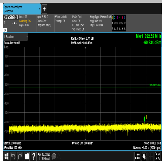
Band4-15MHz-QPSK-20025-1RB#74-30~1000-PASS
