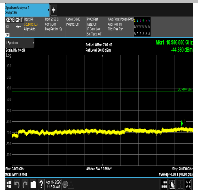
Band4-15MHz-16QAM-20025-1RB#0-3000~20000-PASS
