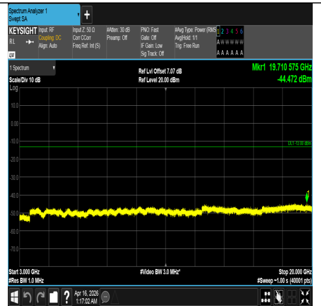
Band4-15MHz-16QAM-20025-75RB#0-3000~20000-PASS
