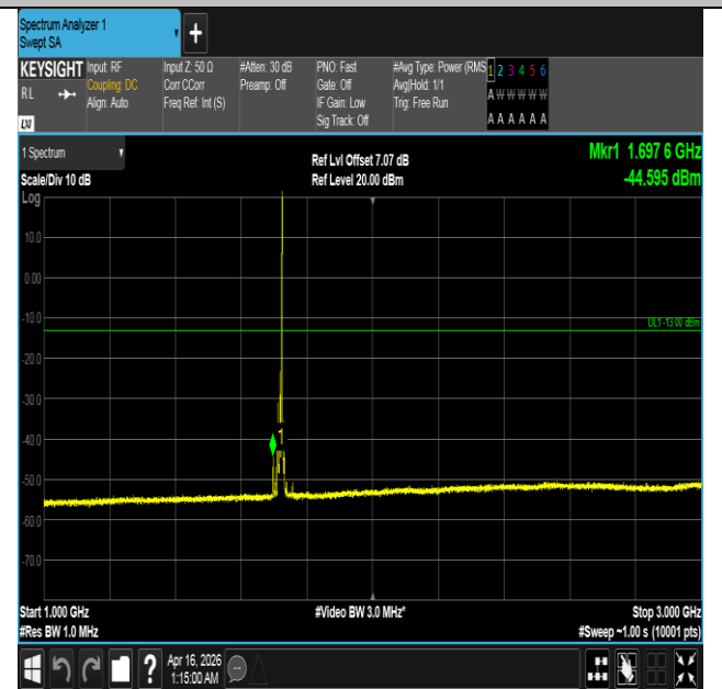
Band4-15MHz-16QAM-20025-1RB#74-1000~3000-PASS
