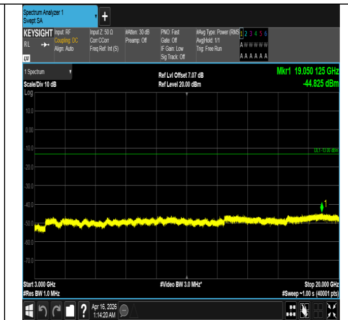
Band4-15MHz-QPSK-20025-1RB#74-3000~20000-PASS
