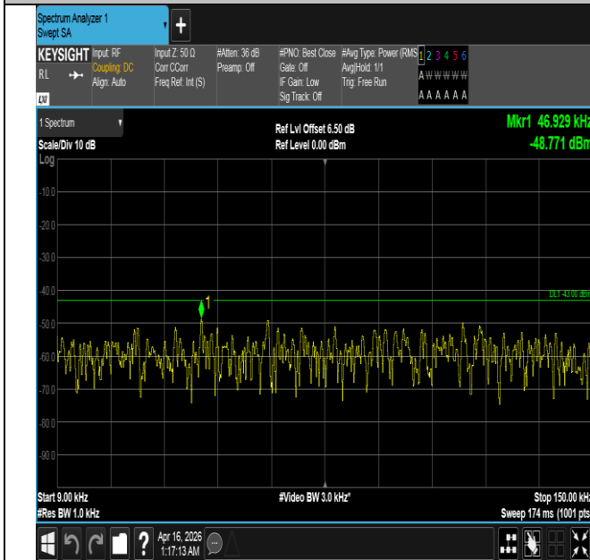
Band4-15MHz-QPSK-20175-1RB#0-0.009~0.15-PASS
