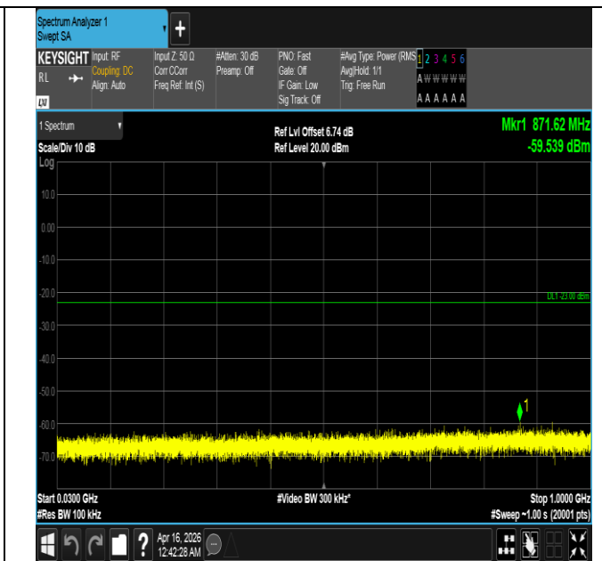
Band4-10MHz-16QAM-20350-50RB#0-30~1000-PASS
