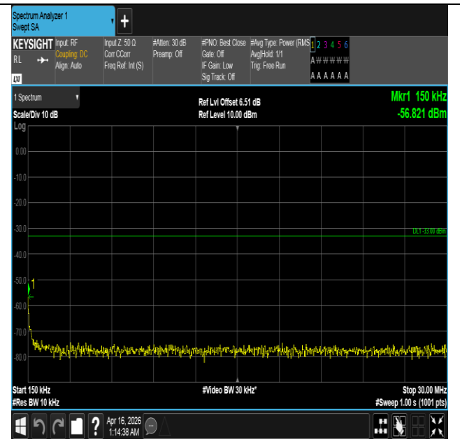
Band4-15MHz-16QAM-20025-1RB#74-0.15~30-PASS
