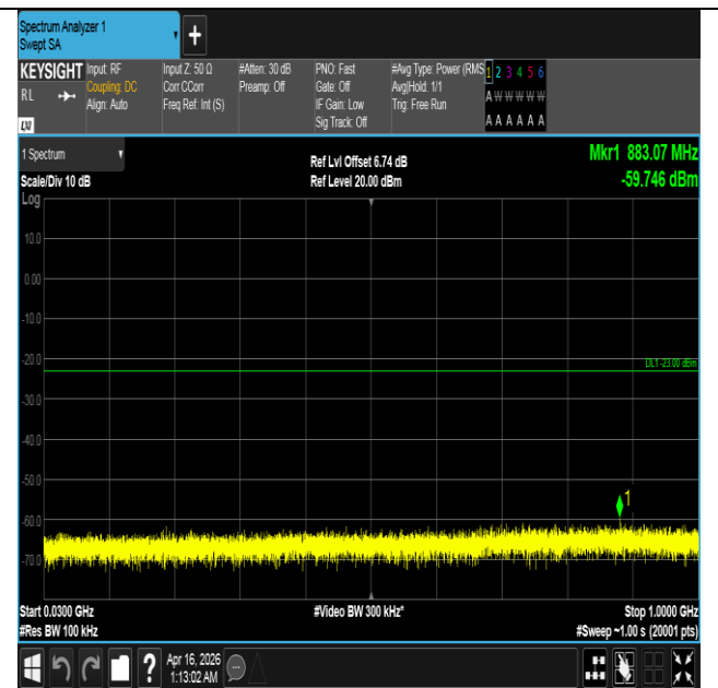
Band4-15MHz-16QAM-20025-1RB#0-30~1000-PASS
