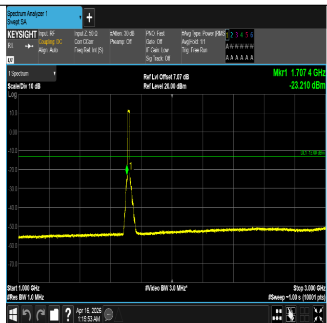
Band4-15MHz-QPSK-20025-75RB#0-1000~3000-PASS
