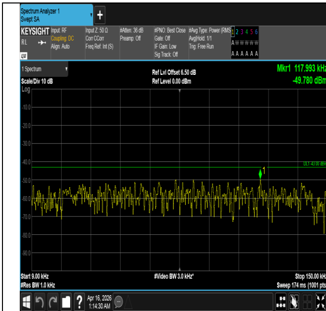
Band4-15MHz-16QAM-20025-1RB#74-0.009~0.15-PASS
