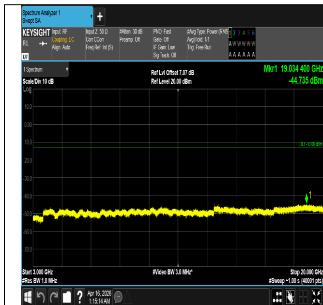
Band4-15MHz-16QAM-20025-1RB#74-3000~20000-PASS
