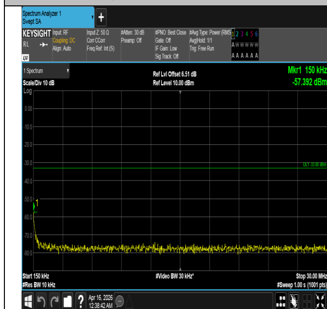
Band4-10MHz-16QAM-20350-1RB#0-0.15~30-PASS
