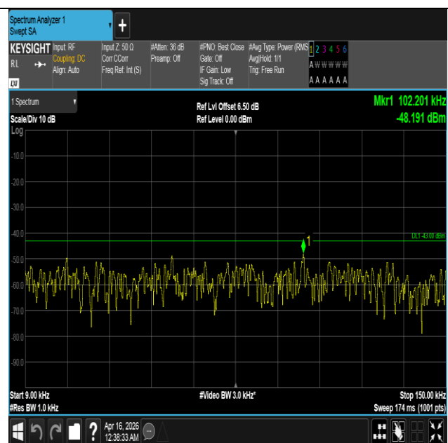
Band4-10MHz-16QAM-20350-1RB#0-0.009~0.15-PASS
