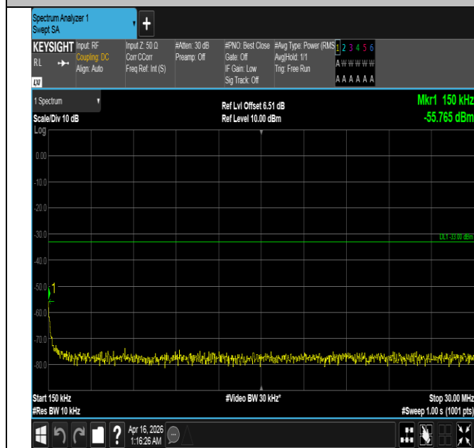
Band4-15MHz-16QAM-20025-75RB#0-0.15~30-PASS
