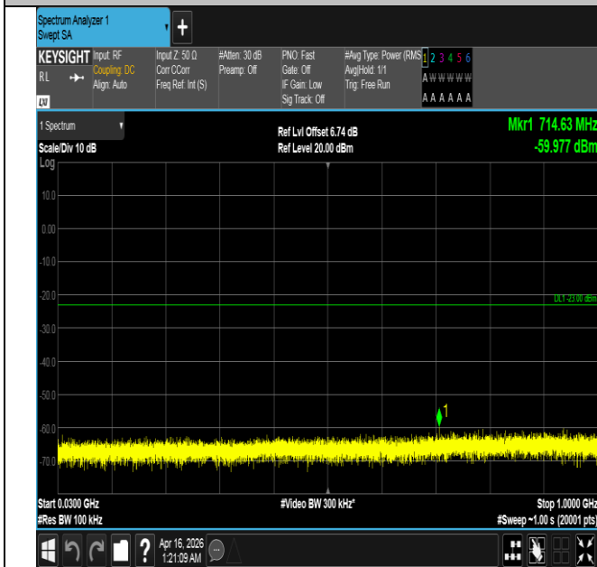
Band4-15MHz-QPSK-20175-75RB#0-30~1000-PASS
