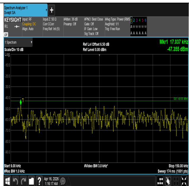
Band4-15MHz-16QAM-20025-75RB#0-0.009~0.15-PASS
