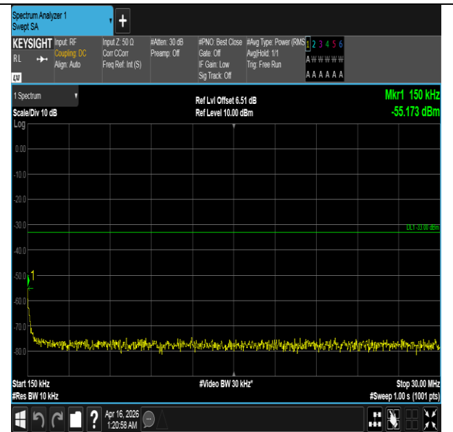
Band4-15MHz-QPSK-20175-75RB#0-0.15~30-PASS
