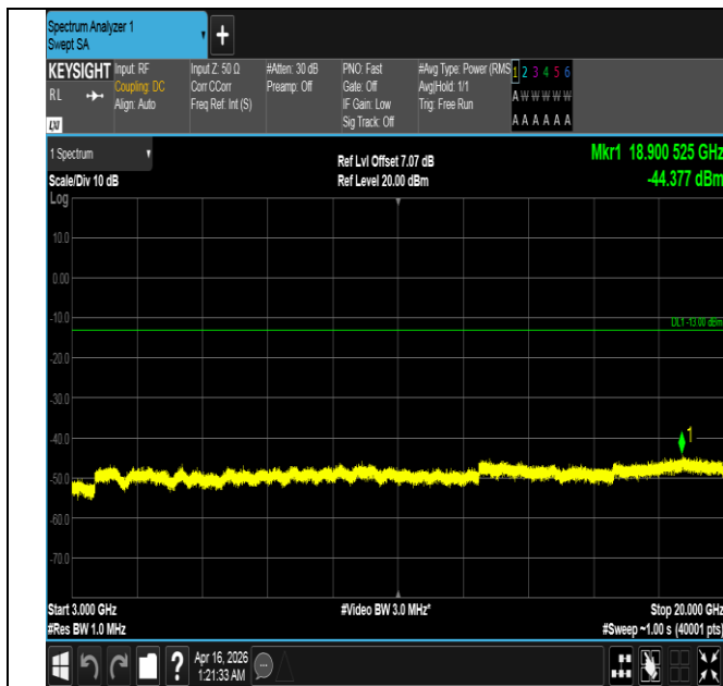
Band4-15MHz-QPSK-20175-75RB#0-3000~20000-PASS
