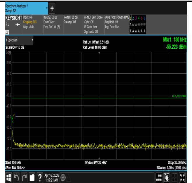
Band4-15MHz-QPSK-20175-1RB#0-0.15~30-PASS
