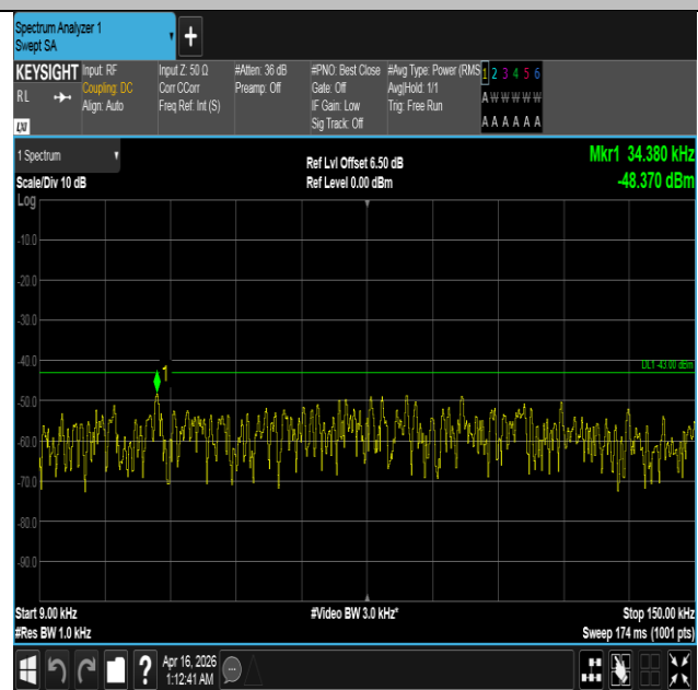
Band4-15MHz-16QAM-20025-1RB#0-0.009~0.15-PASS
