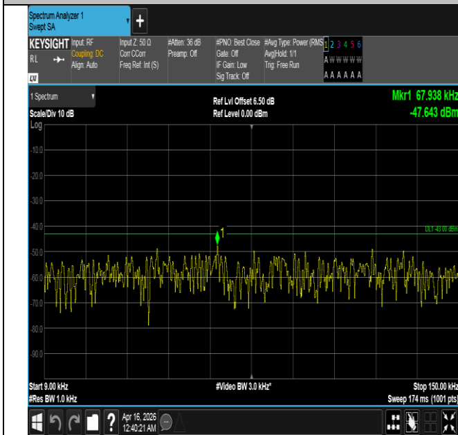
Band4-10MHz-16QAM-20350-1RB#49-0.009~0.15-PASS
