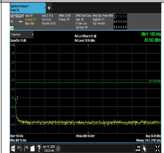
Band4-15MHz-QPSK-20325-75RB#0-0.15~30-PASS
