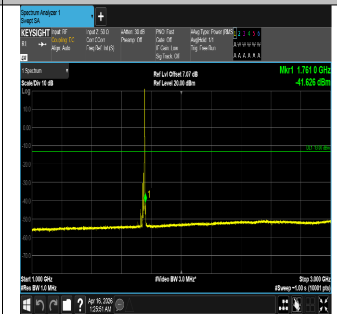
Band4-15MHz-16QAM-20325-1RB#74-1000~3000-PASS
