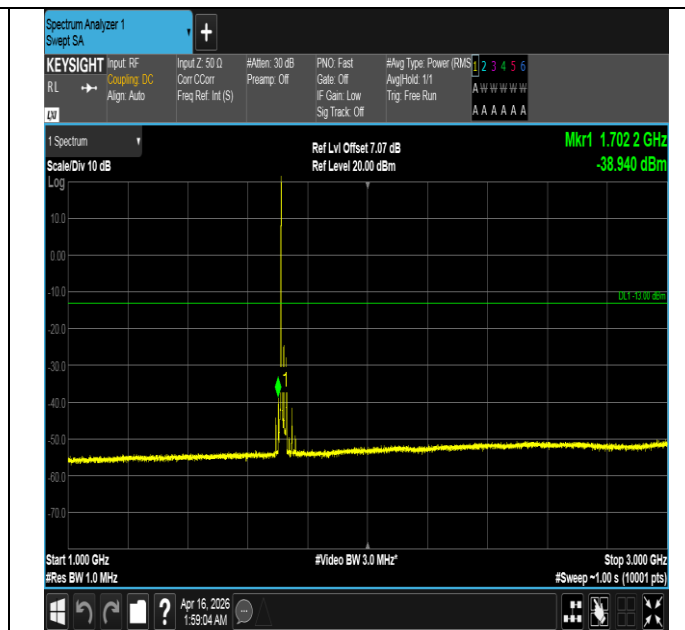
Band4-20MHz-QPSK-20050-1RB#0-1000~3000-PASS
