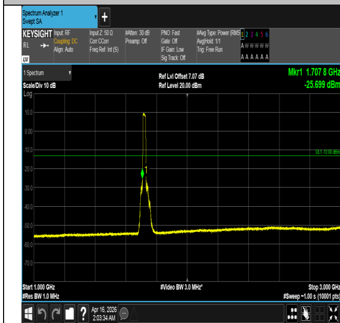
Band4-20MHz-16QAM-20050-100RB#0-1000~3000-PASS
