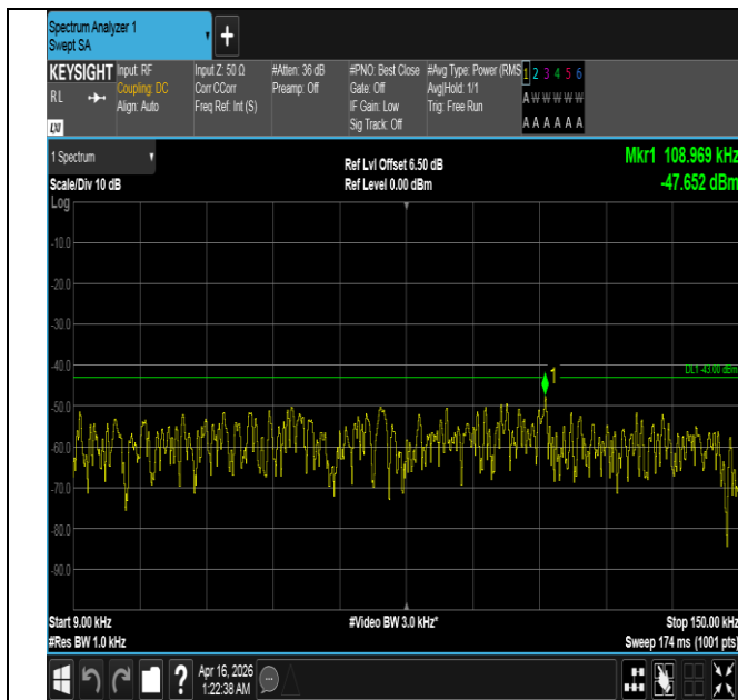
Band4-15MHz-QPSK-20325-1RB#0-0.009~0.15-PASS
