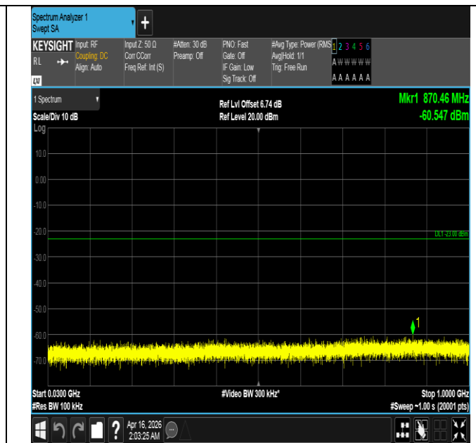
Band4-20MHz-16QAM-20050-100RB#0-30~1000-PASS
