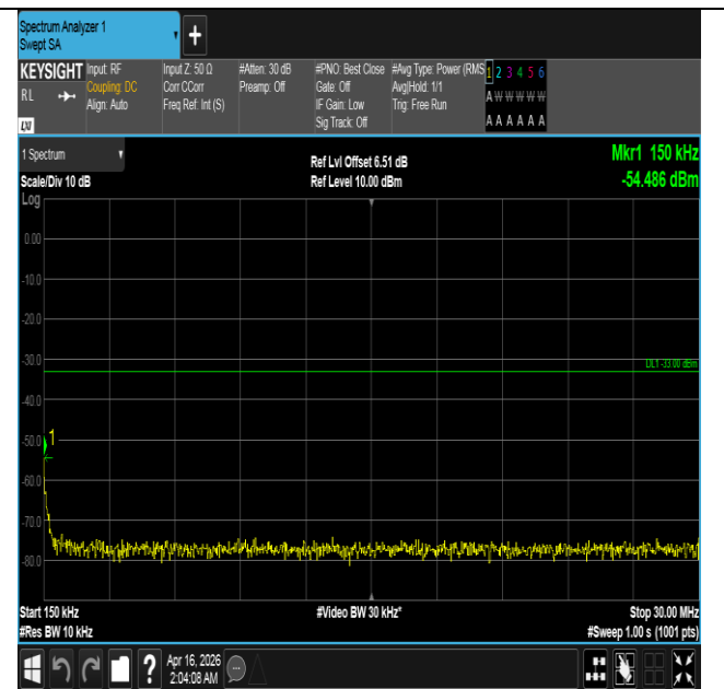
Band4-20MHz-QPSK-20175-1RB#0-0.15~30-PASS
