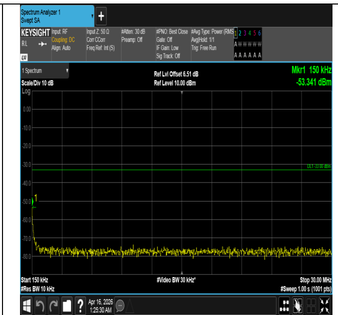
Band4-15MHz-16QAM-20325-1RB#74-0.15~30-PASS
