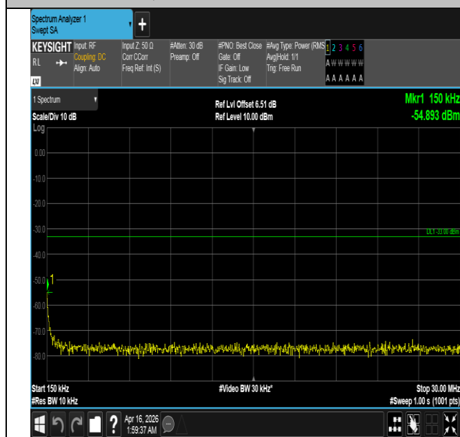
Band4-20MHz-16QAM-20050-1RB#0-0.15~30-PASS
