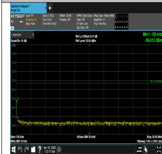
Band4-15MHz-16QAM-20325-75RB#0-0.15~30-PASS
