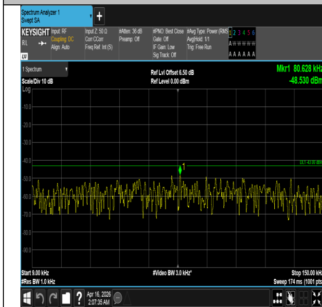
Band4-20MHz-QPSK-20175-100RB#0-0.009~0.15-PASS
