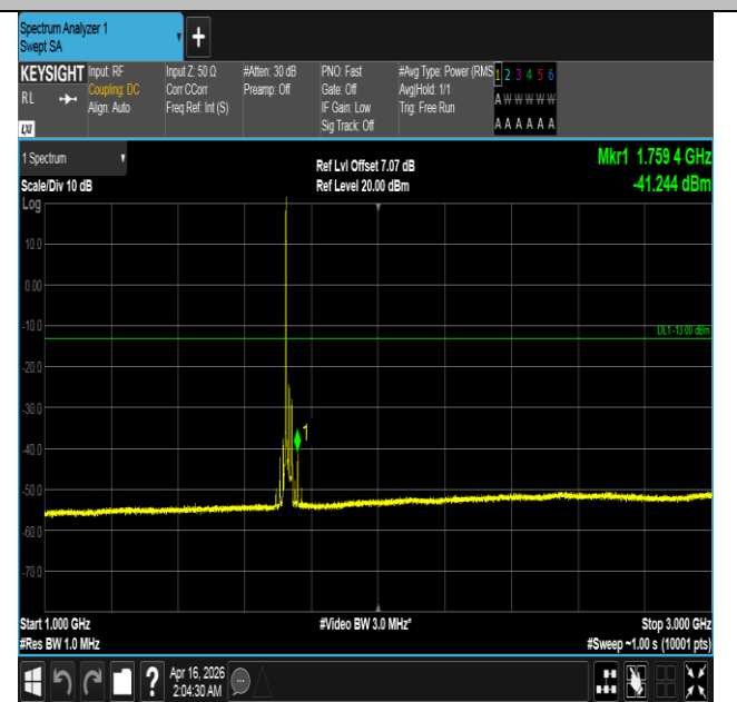
Band4-20MHz-QPSK-20175-1RB#0-1000~3000-PASS
