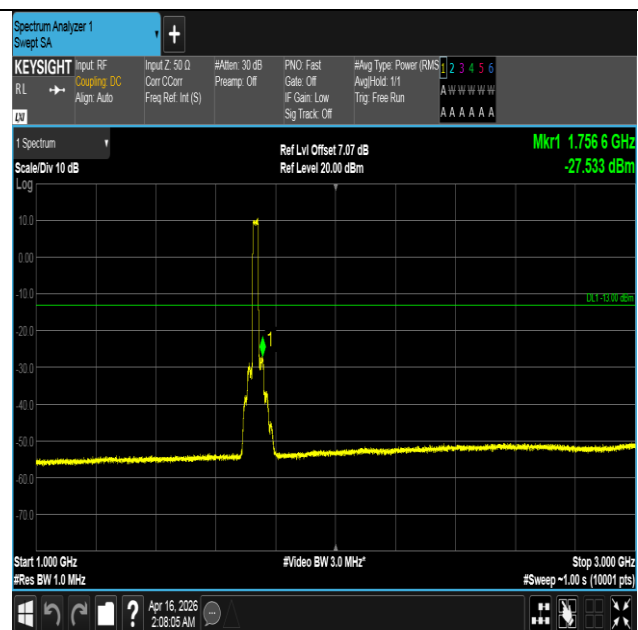
Band4-20MHz-QPSK-20175-100RB#0-1000~3000-PASS
