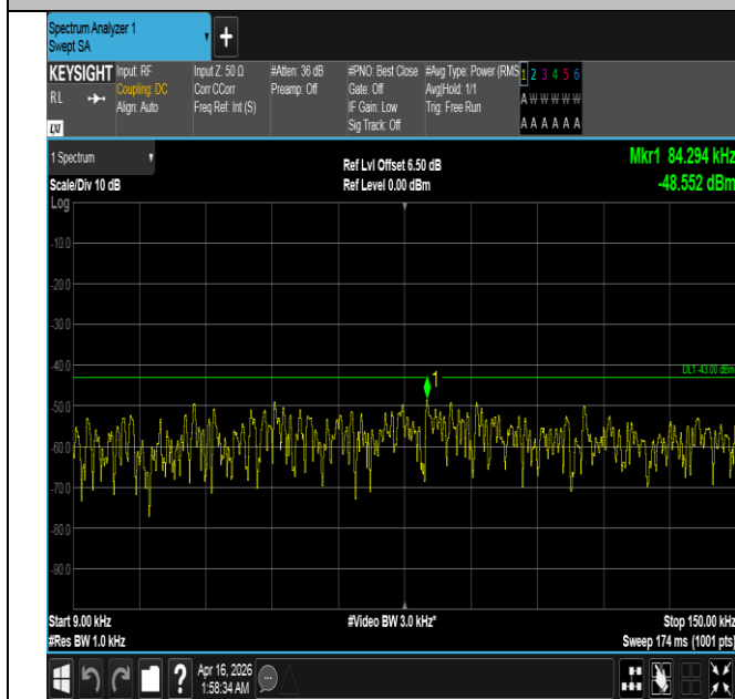
Band4-20MHz-QPSK-20050-1RB#0-0.009~0.15-PASS
