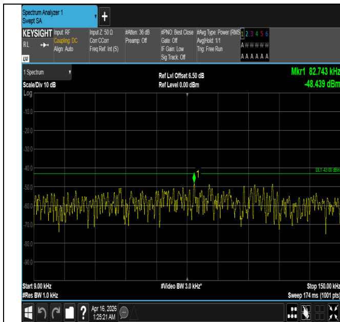
Band4-15MHz-16QAM-20325-1RB#74-0.009~0.15-PASS
