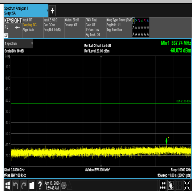
Band4-20MHz-16QAM-20050-1RB#0-30~1000-PASS
