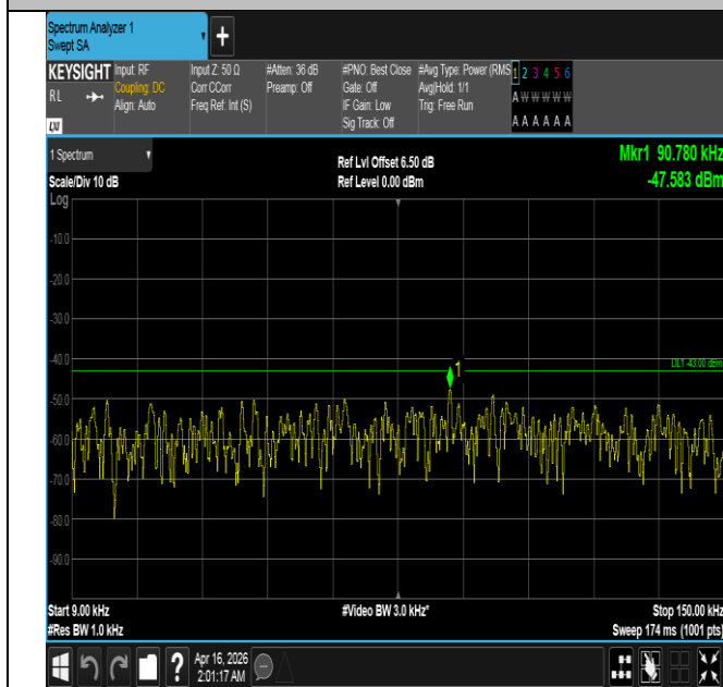
Band4-20MHz-16QAM-20050-1RB#99-0.009~0.15-PASS
