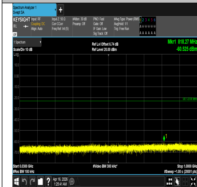
Band4-15MHz-16QAM-20325-1RB#74-30~1000-PASS
