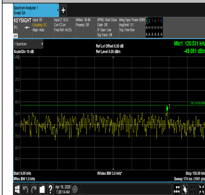
Band4-15MHz-QPSK-20325-75RB#0-0.009~0.15-PASS
