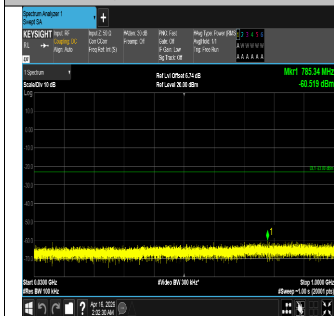
Band4-20MHz-QPSK-20050-100RB#0-30~1000-PASS
