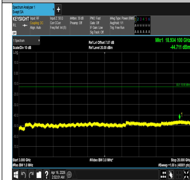
Band4-20MHz-16QAM-20050-1RB#99-3000~20000-PASS
