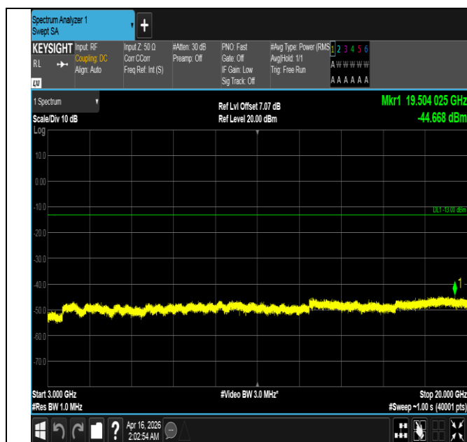
Band4-20MHz-QPSK-20050-100RB#0-3000~20000-PASS
