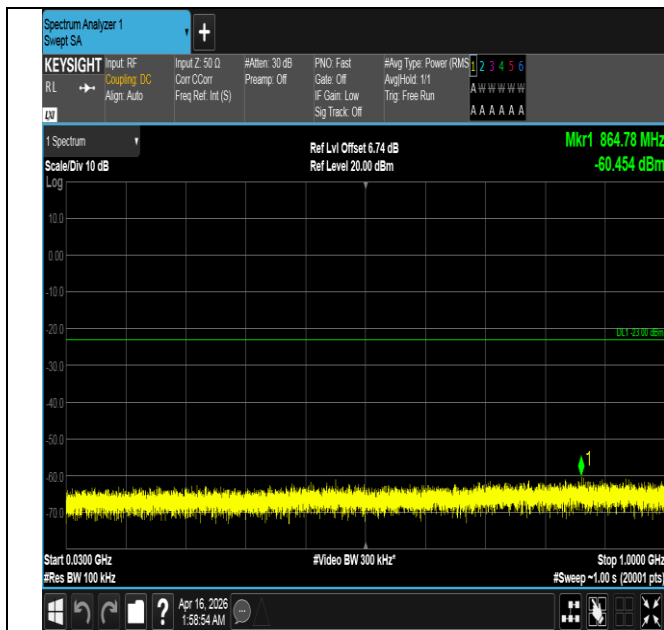
Band4-20MHz-QPSK-20050-1RB#0-30~1000-PASS
