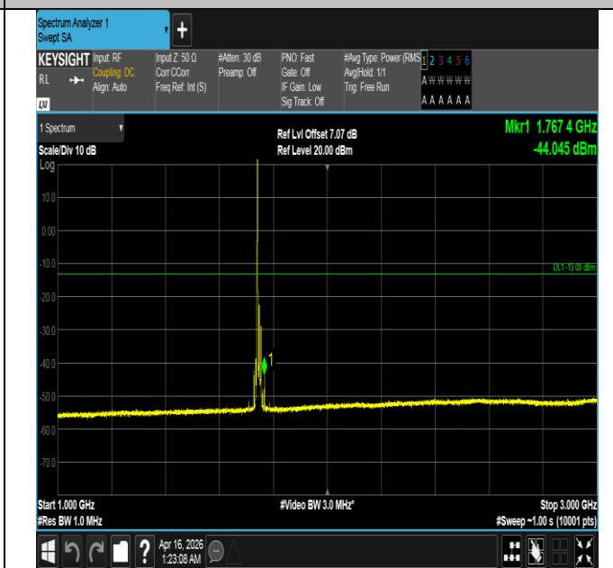
Band4-15MHz-QPSK-20325-1RB#0-1000~3000-PASS
