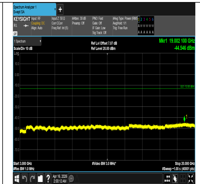
Band4-20MHz-16QAM-20050-1RB#0-3000~20000-PASS
