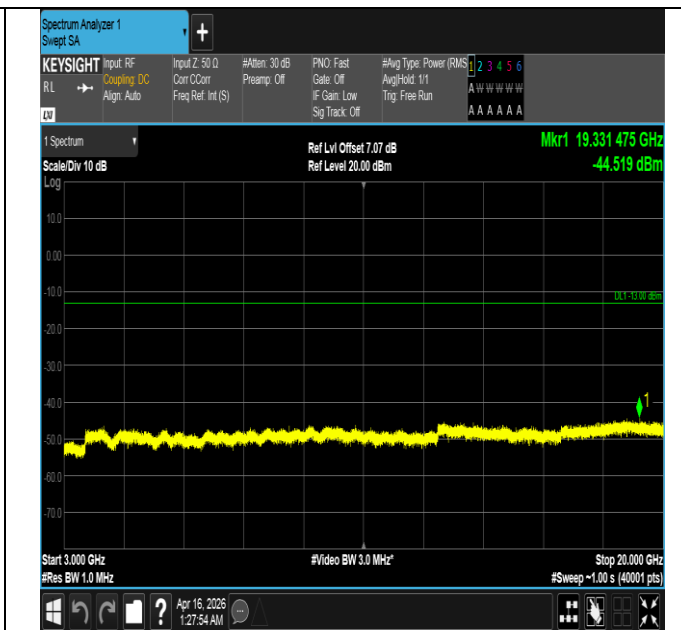
Band4-15MHz-16QAM-20325-75RB#0-3000~20000-PASS
