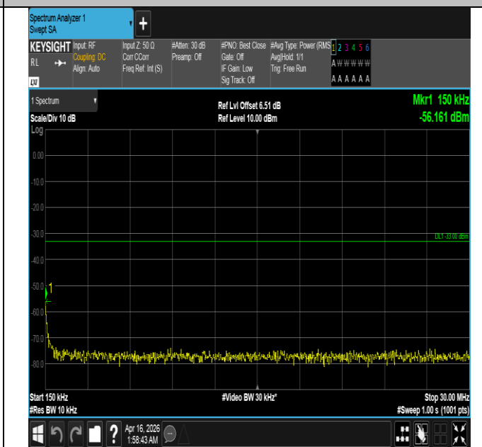
Band4-20MHz-QPSK-20050-1RB#0-0.15~30-PASS
