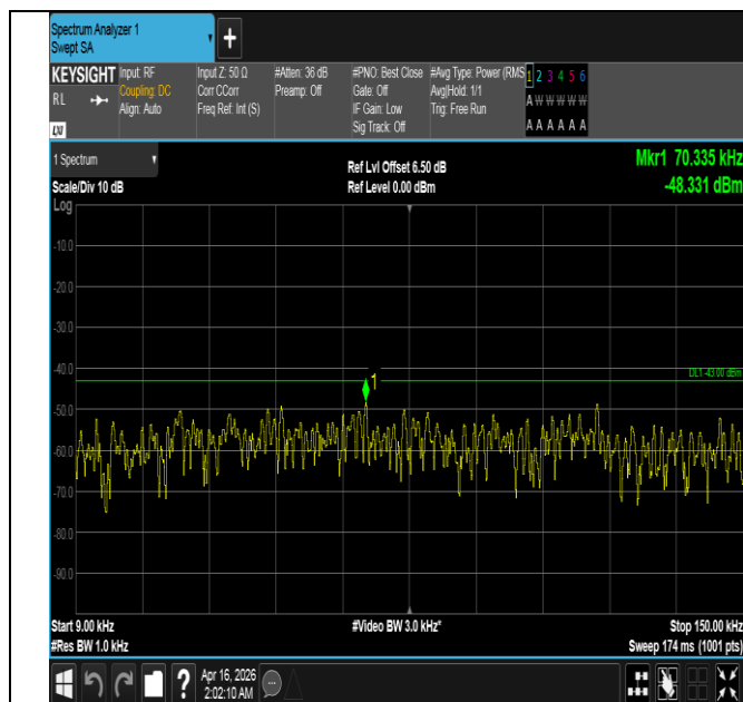
Band4-20MHz-QPSK-20050-100RB#0-0.009~0.15-PASS
