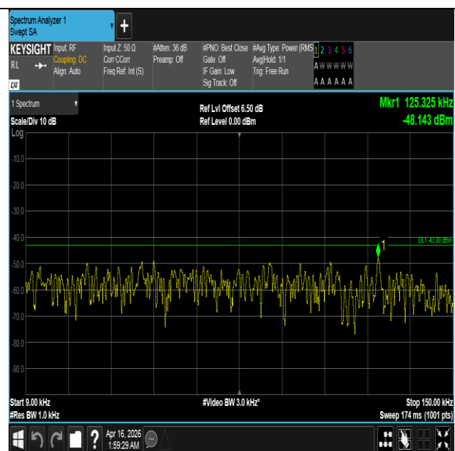
Band4-20MHz-16QAM-20050-1RB#0-0.009~0.15-PASS
