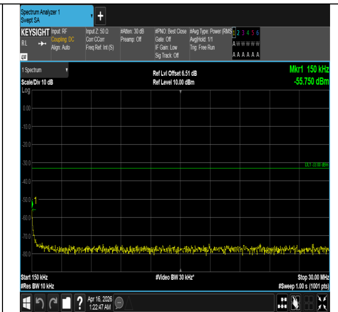
Band4-15MHz-QPSK-20325-1RB#0-0.15~30-PASS
