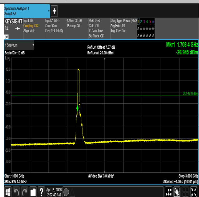
Band4-20MHz-QPSK-20050-100RB#0-1000~3000-PASS
