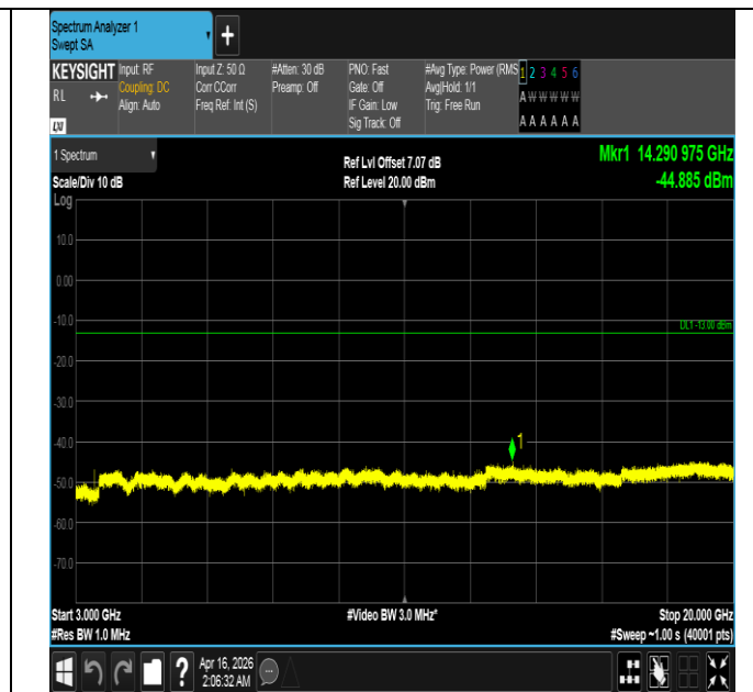
Band4-20MHz-QPSK-20175-1RB#99-3000~20000-PASS
