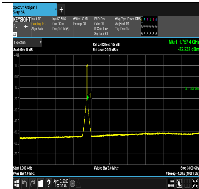
Band4-15MHz-16QAM-20325-75RB#0-1000~3000-PASS
