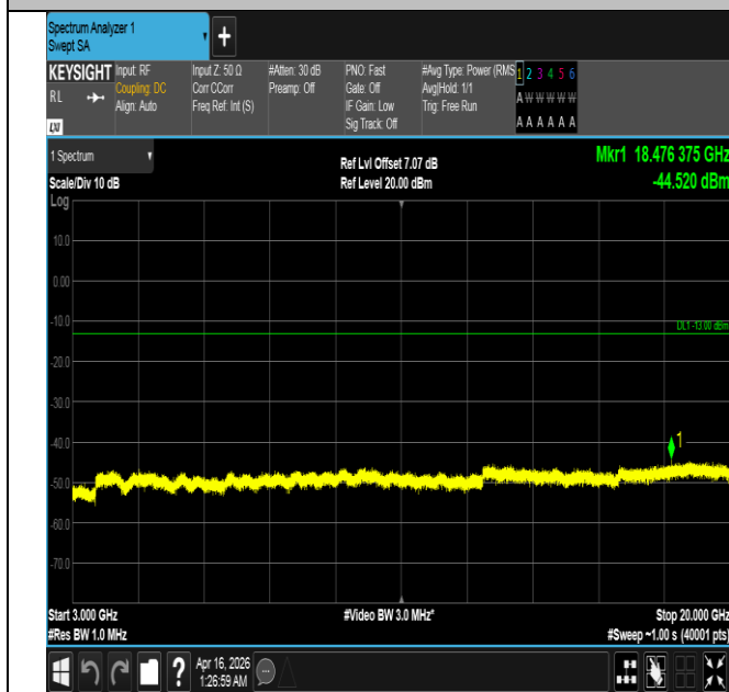
Band4-15MHz-QPSK-20325-75RB#0-3000~20000-PASS
