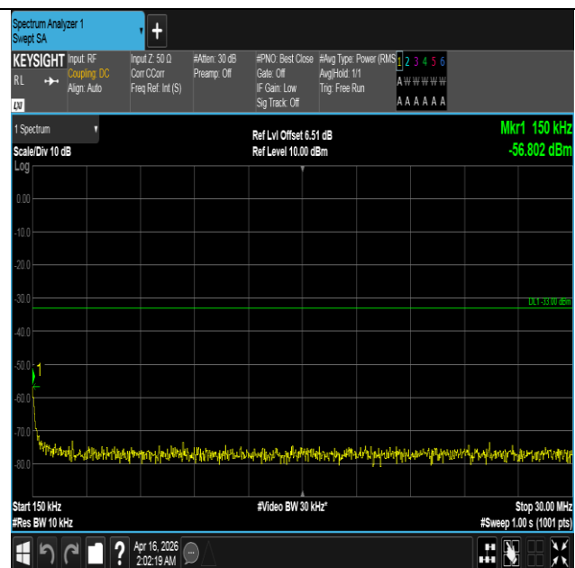
Band4-20MHz-QPSK-20050-100RB#0-0.15~30-PASS
