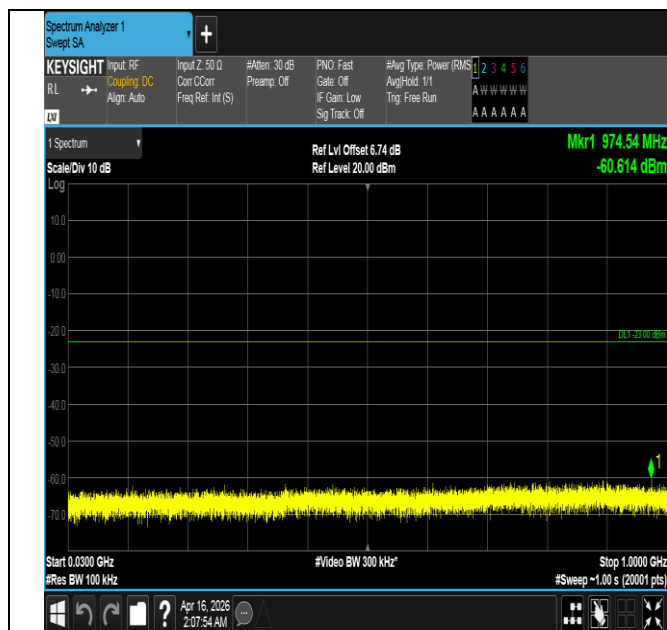
Band4-20MHz-QPSK-20175-100RB#0-30~1000-PASS
