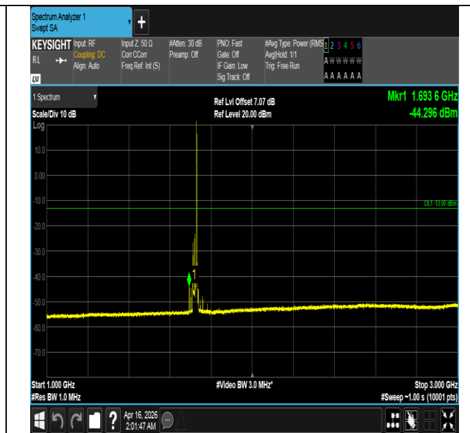
Band4-20MHz-16QAM-20050-1RB#99-1000~3000-PASS
