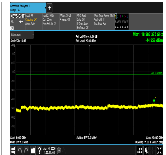
Band4-15MHz-QPSK-20325-1RB#74-3000~20000-PASS
