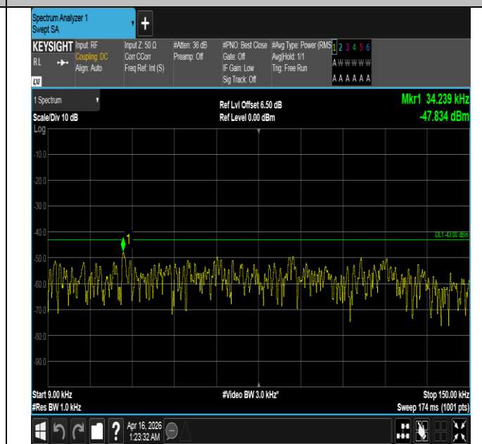
Band4-15MHz-16QAM-20325-1RB#0-0.009~0.15-PASS
