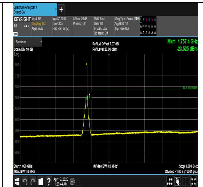
Band4-15MHz-QPSK-20325-75RB#0-1000~3000-PASS
