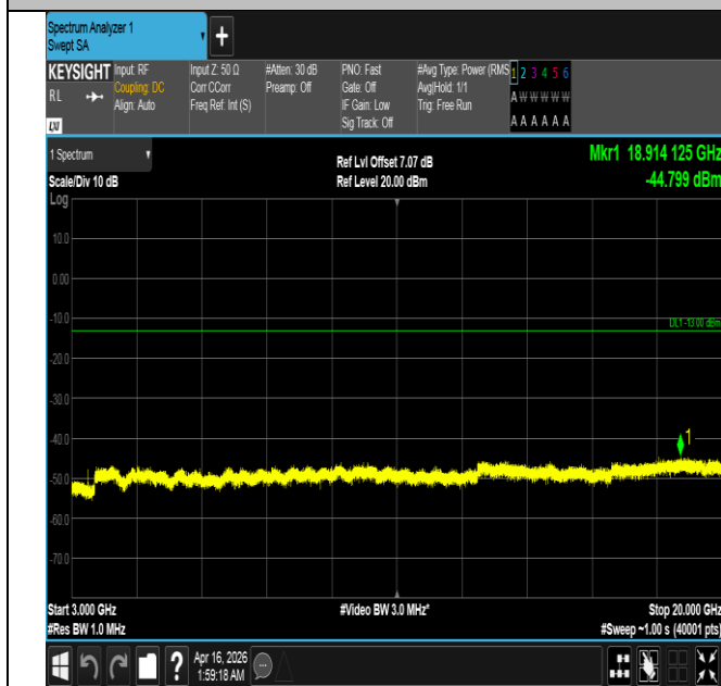
Band4-20MHz-QPSK-20050-1RB#0-3000~20000-PASS
