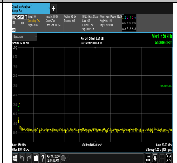
Band4-20MHz-QPSK-20175-100RB#0-0.15~30-PASS
