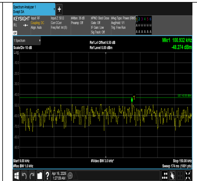
Band4-15MHz-16QAM-20325-75RB#0-0.009~0.15-PASS
