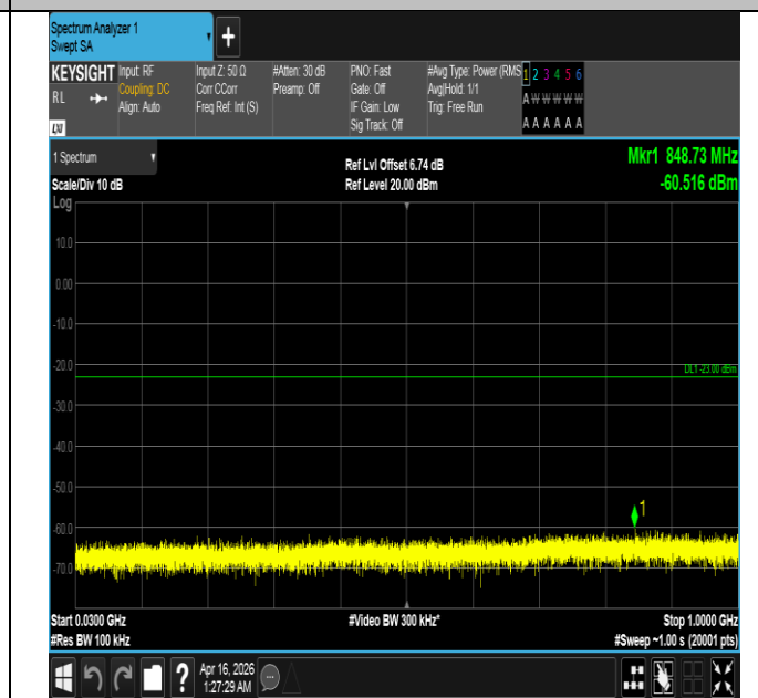
Band4-15MHz-16QAM-20325-75RB#0-30~1000-PASS
