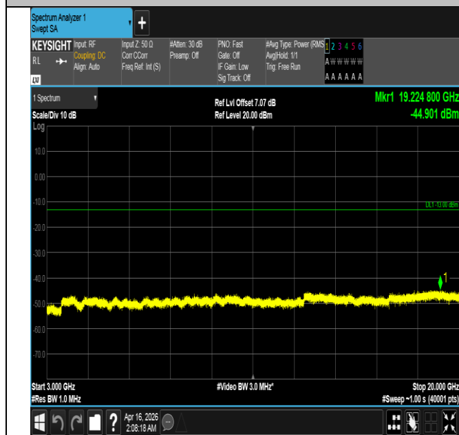
Band4-20MHz-QPSK-20175-100RB#0-3000~20000-PASS
