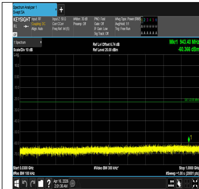
Band4-20MHz-16QAM-20050-1RB#99-30~1000-PASS
