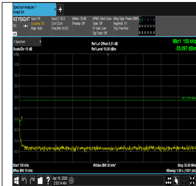
Band4-20MHz-16QAM-20050-100RB#0-0.15~30-PASS
