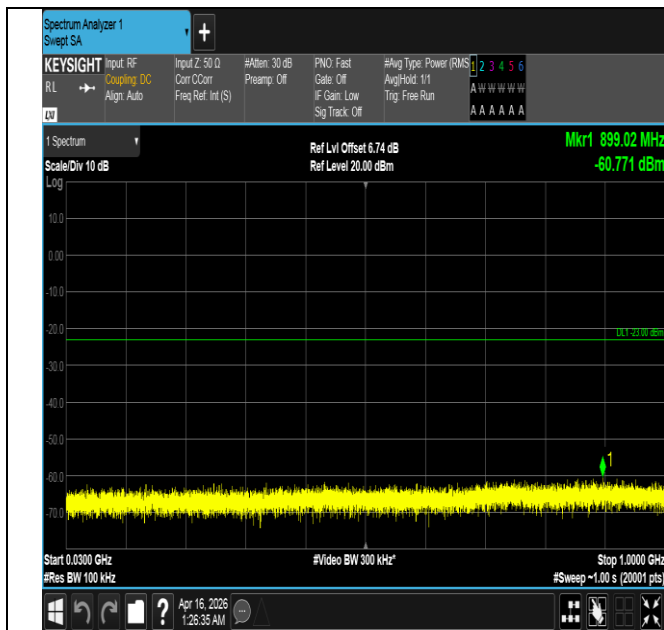
Band4-15MHz-QPSK-20325-75RB#0-30~1000-PASS
