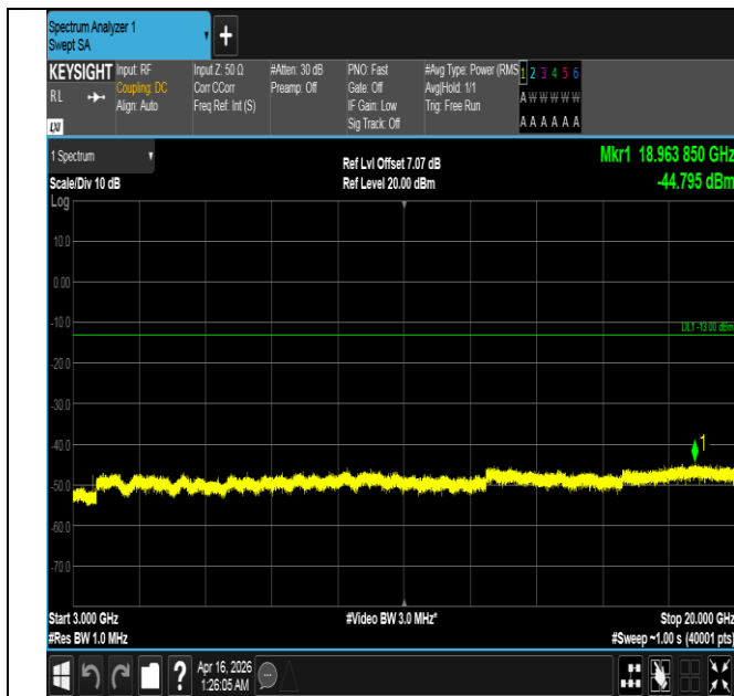
Band4-15MHz-16QAM-20325-1RB#74-3000~20000-PASS
