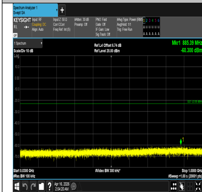
Band4-20MHz-QPSK-20175-1RB#0-30~1000-PASS
