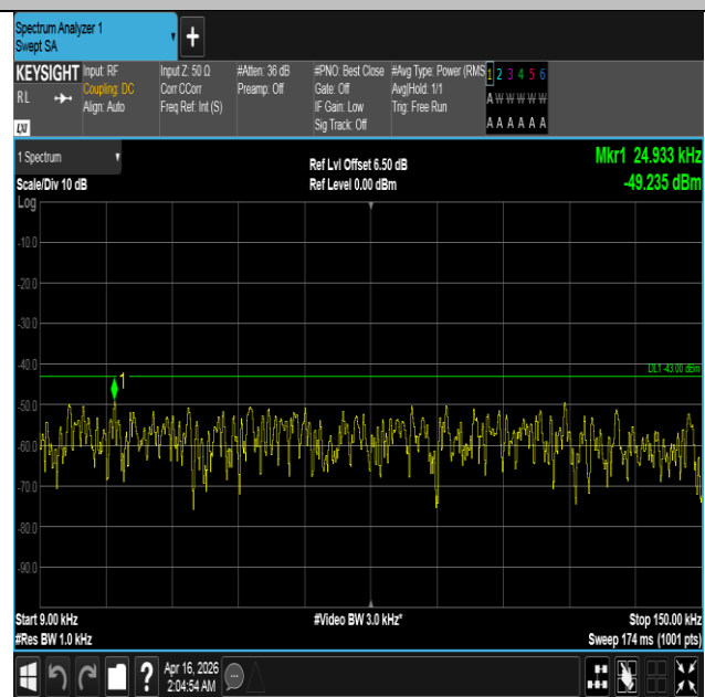
Band4-20MHz-16QAM-20175-1RB#0-0.009~0.15-PASS
