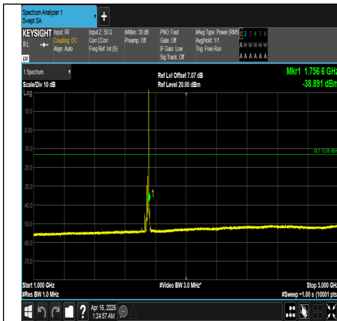
Band4-15MHz-QPSK-20325-1RB#74-1000~3000-PASS
