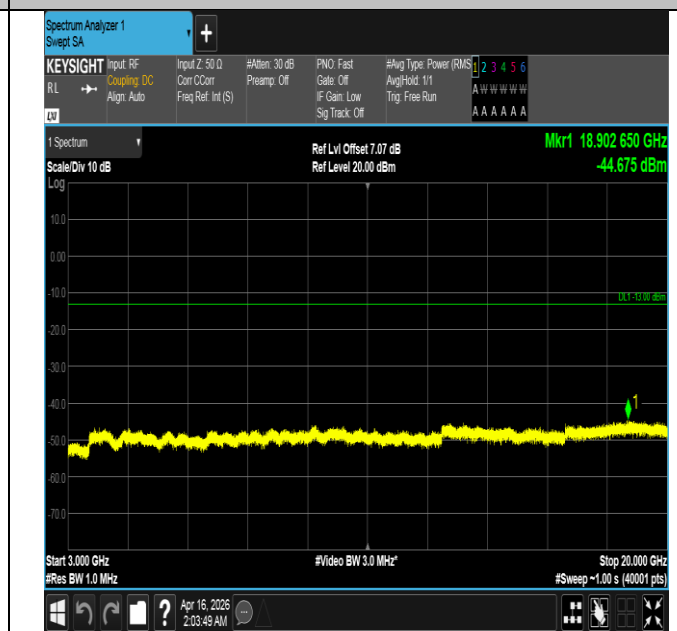
Band4-20MHz-16QAM-20050-100RB#0-3000~20000-PASS
