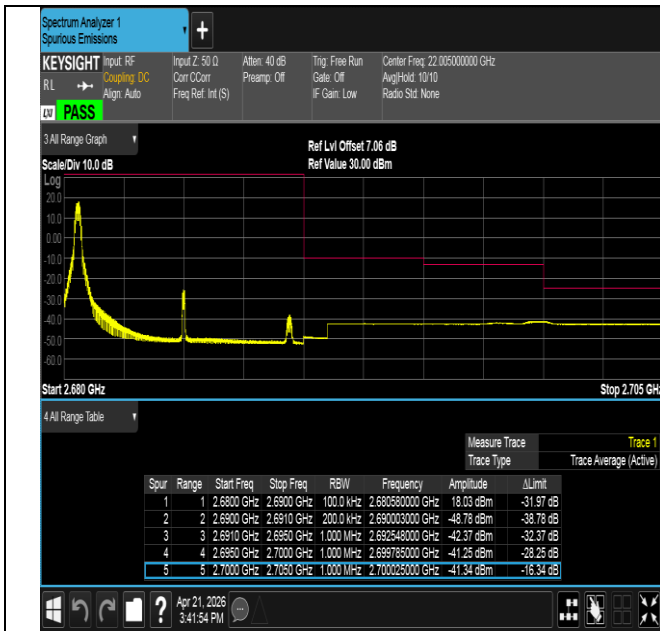
Band41-10MHz-QPSK-41540-1RB#0-PASS
