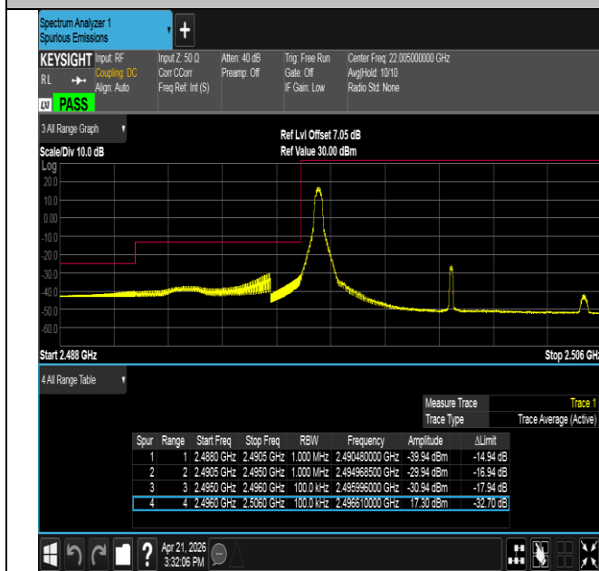
Band41-10MHz-QPSK-39700-1RB#0-PASS
