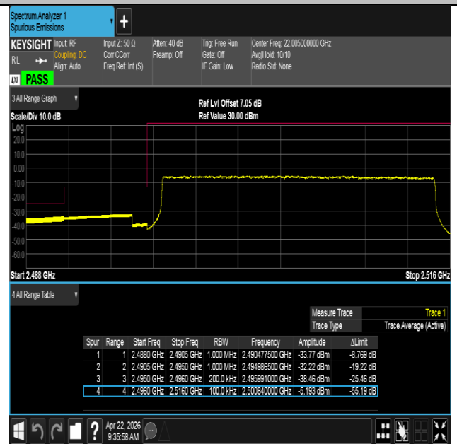
Band41-20MHz-16QAM-39750-100RB#0-PASS
