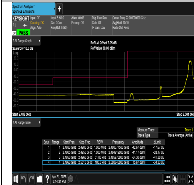
Band41-5MHz-16QAM-39675-1RB#24-PASS
