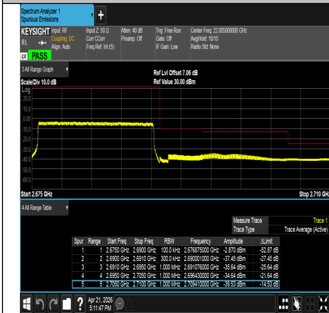
Band41-15MHz-QPSK-41515-75RB#0-PASS
