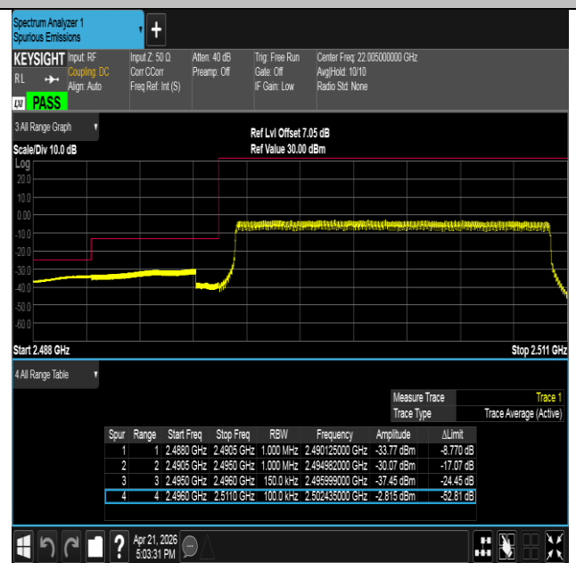
Band41-15MHz-16QAM-39725-75RB#0-PASS
