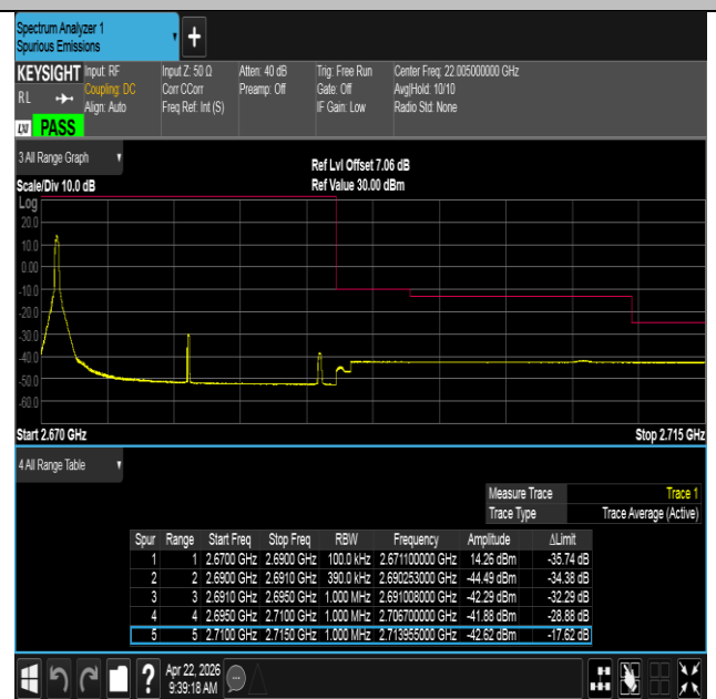
Band41-20MHz-16QAM-41490-1RB#0-PASS
