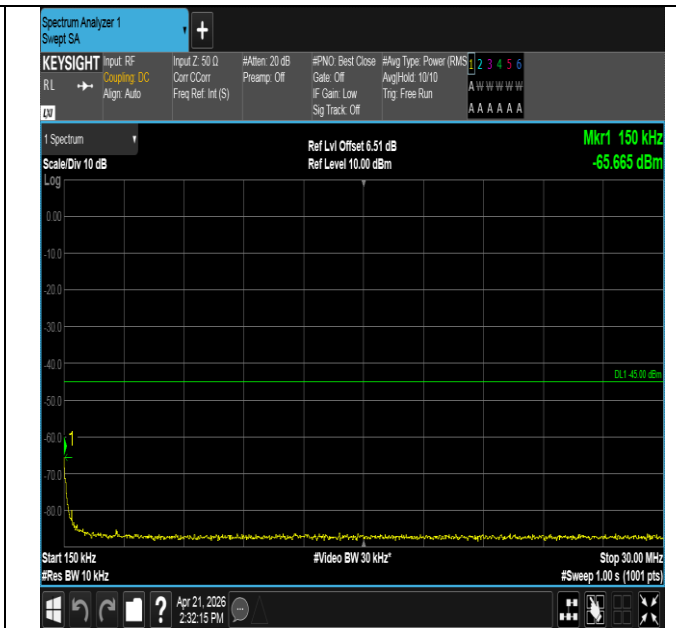
Band41-5MHz-QPSK-39675-1RB#24-0.15~30-PASS
