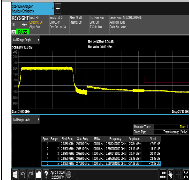
Band41-5MHz-QPSK-41565-25RB#0-PASS
