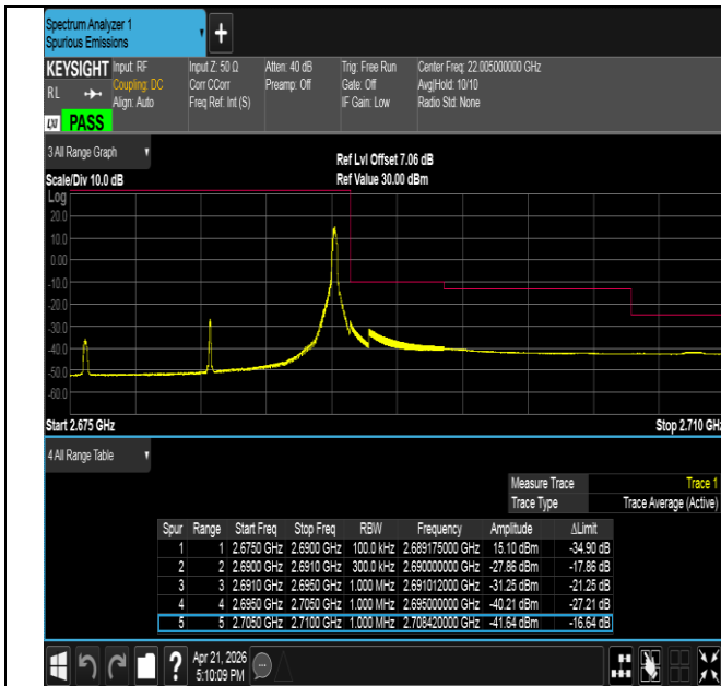
Band41-15MHz-16QAM-41515-1RB#74-PASS
