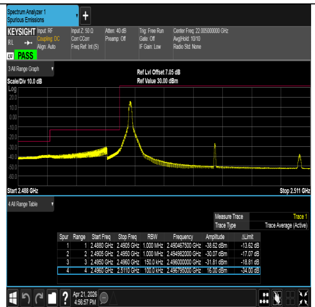
Band41-15MHz-16QAM-39725-1RB#0-PASS
