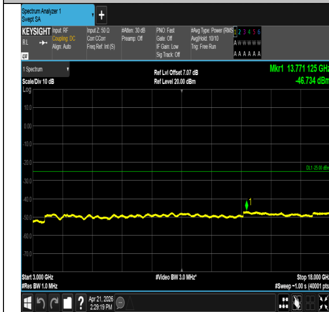
Band41-5MHz-QPSK-39675-1RB#0-3000~18000-PASS
