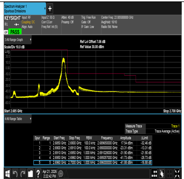
Band41-5MHz-QPSK-41565-1RB#24-PASS
