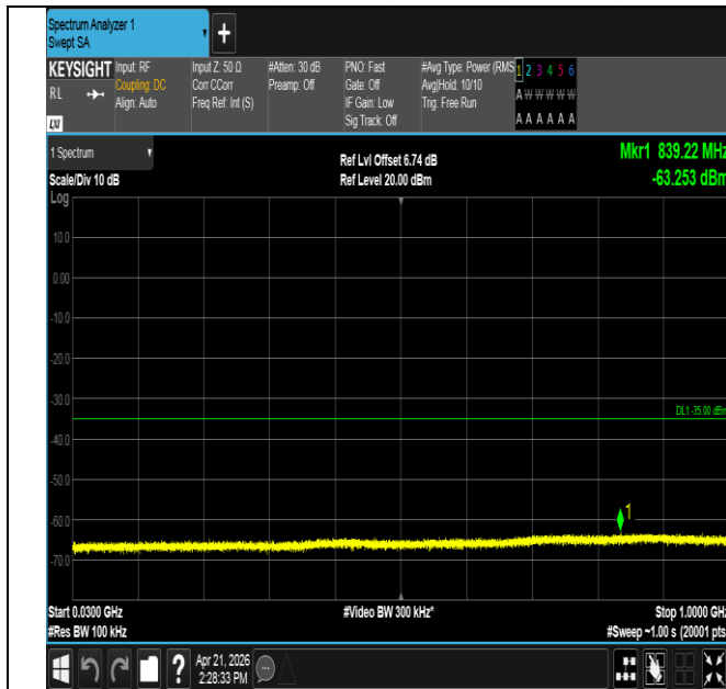
Band41-5MHz-QPSK-39675-1RB#0-30~1000-PASS
