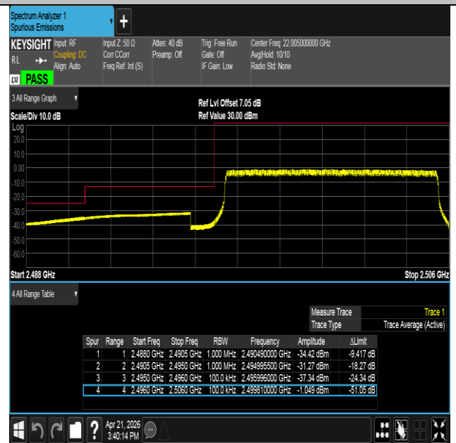
Band41-10MHz-16QAM-39700-50RB#0-PASS
