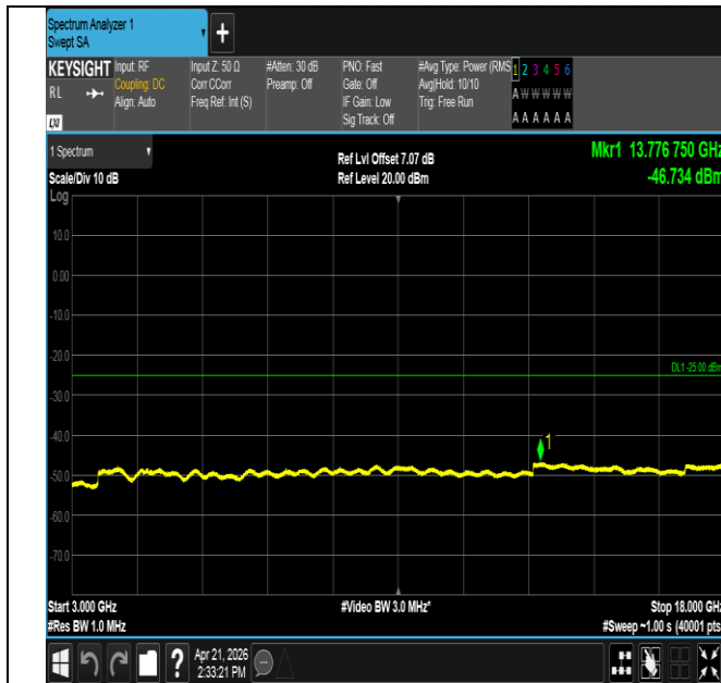
Band41-5MHz-QPSK-39675-1RB#24-3000~18000-PASS
