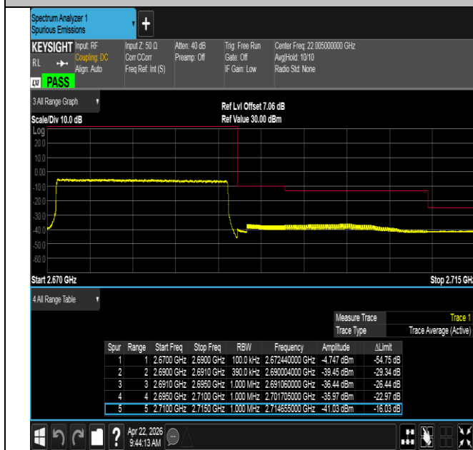
Band41-20MHz-QPSK-41490-100RB#0-PASS
