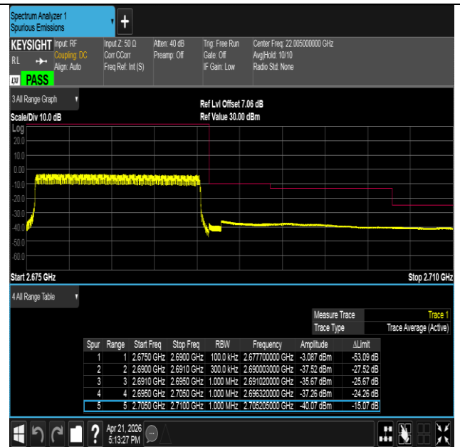
Band41-15MHz-16QAM-41515-75RB#0-PASS
