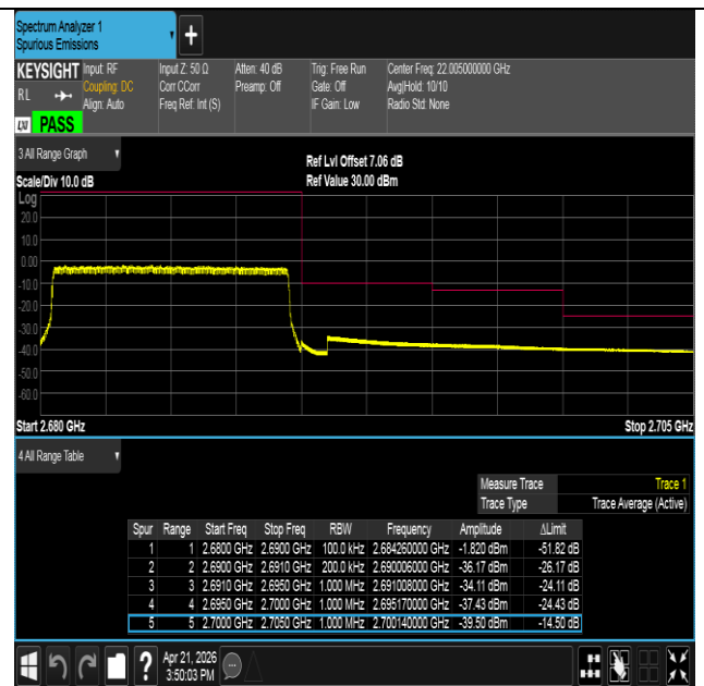
Band41-10MHz-16QAM-41540-50RB#0-PASS
