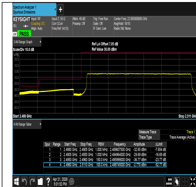
Band41-15MHz-QPSK-39725-75RB#0-PASS
