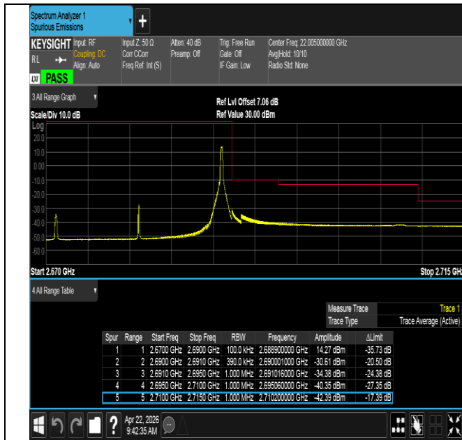
Band41-20MHz-16QAM-41490-1RB#99-PASS
