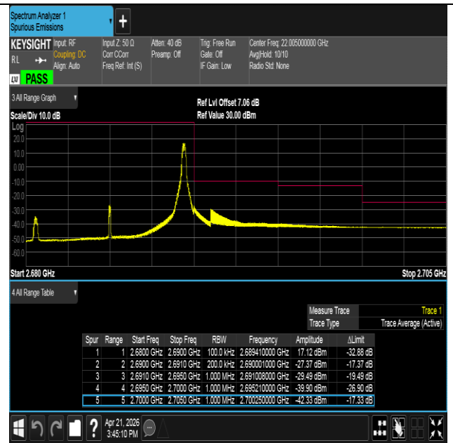
Band41-10MHz-QPSK-41540-1RB#49-PASS
