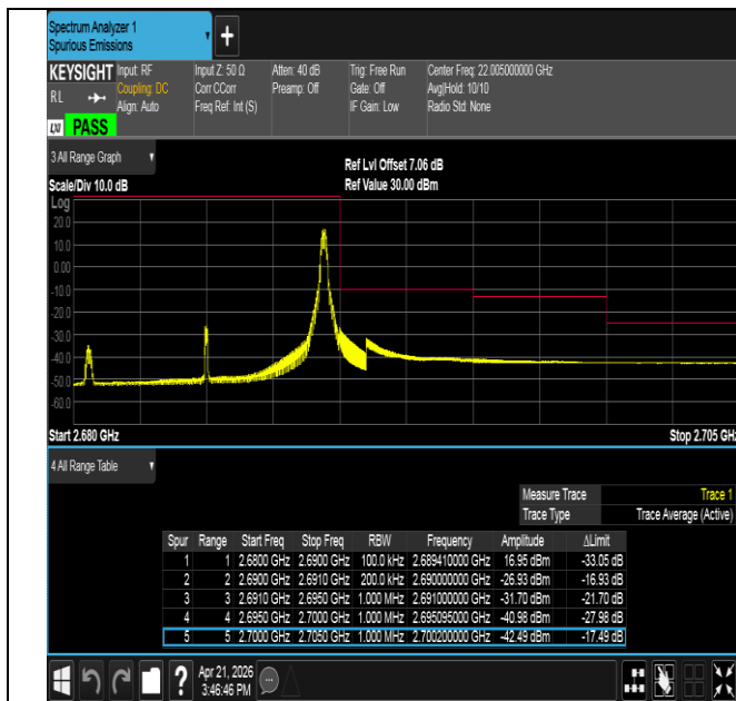
Band41-10MHz-16QAM-41540-1RB#49-PASS
