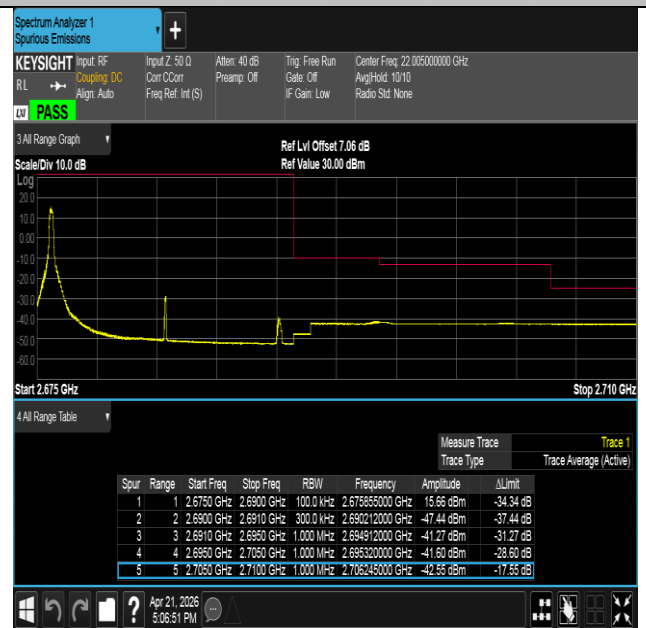
Band41-15MHz-16QAM-41515-1RB#0-PASS
