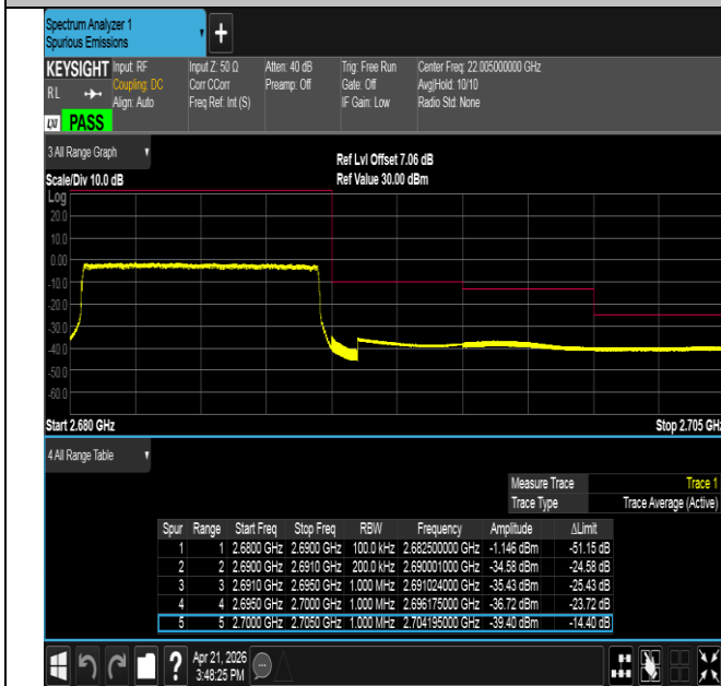
Band41-10MHz-QPSK-41540-50RB#0-PASS
