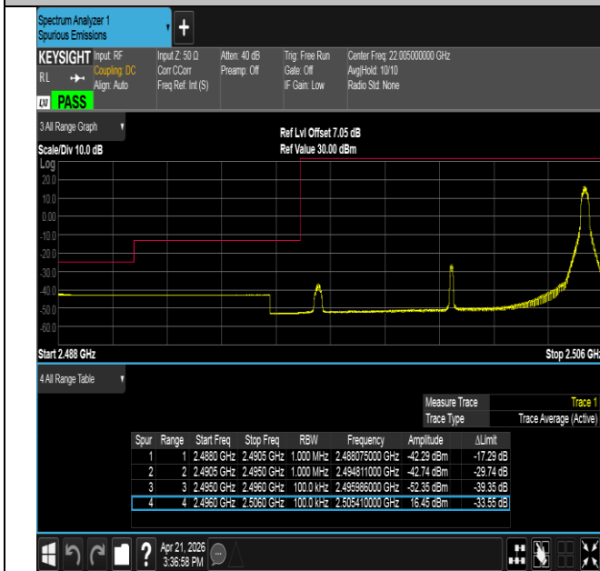
Band41-10MHz-16QAM-39700-1RB#49-PASS
