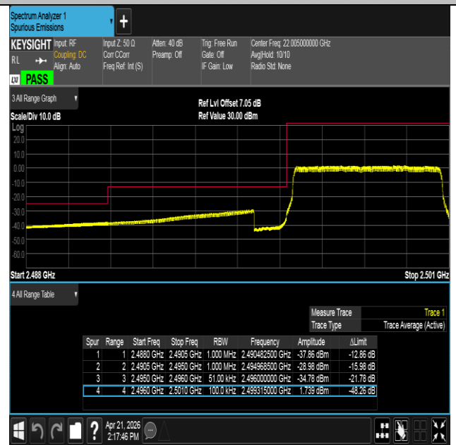
Band41-5MHz-16QAM-39675-25RB#0-PASS
