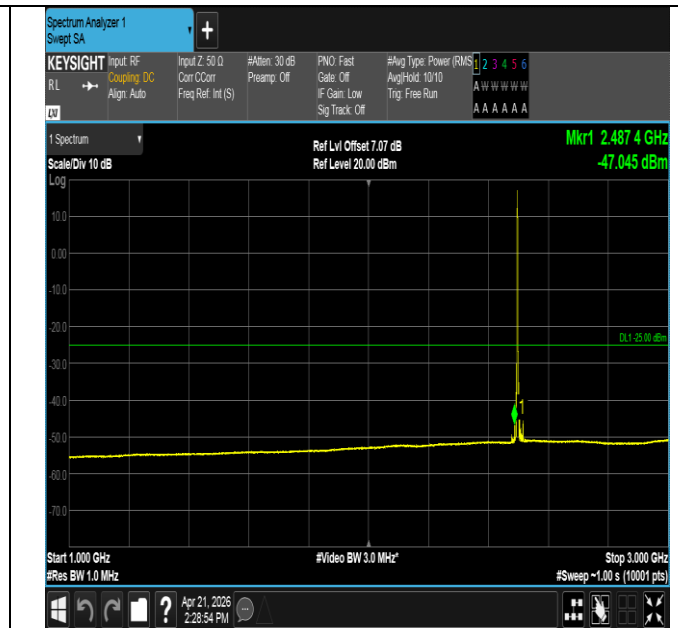
Band41-5MHz-QPSK-39675-1RB#0-1000~3000-PASS
