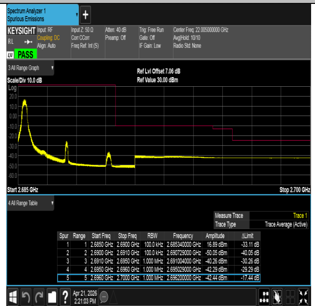
Band41-5MHz-16QAM-41565-1RB#0-PASS
