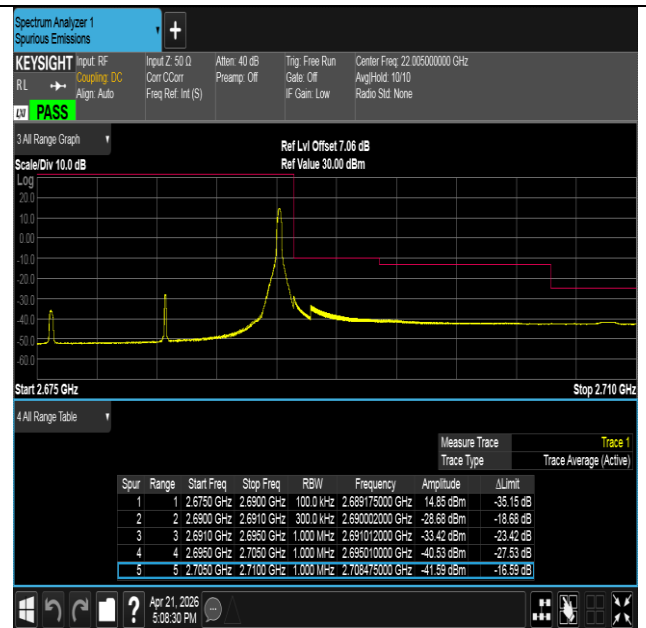
Band41-15MHz-QPSK-41515-1RB#74-PASS
