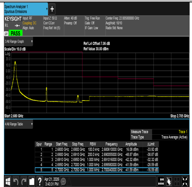
Band41-10MHz-16QAM-41540-1RB#0-PASS
