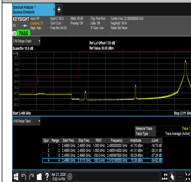
Band41-15MHz-16QAM-39725-1RB#74-PASS
