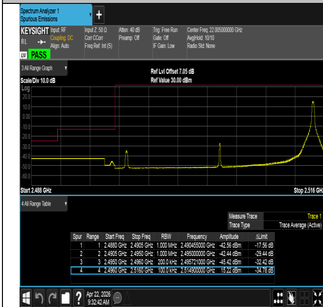
Band41-20MHz-16QAM-39750-1RB#99-PASS
