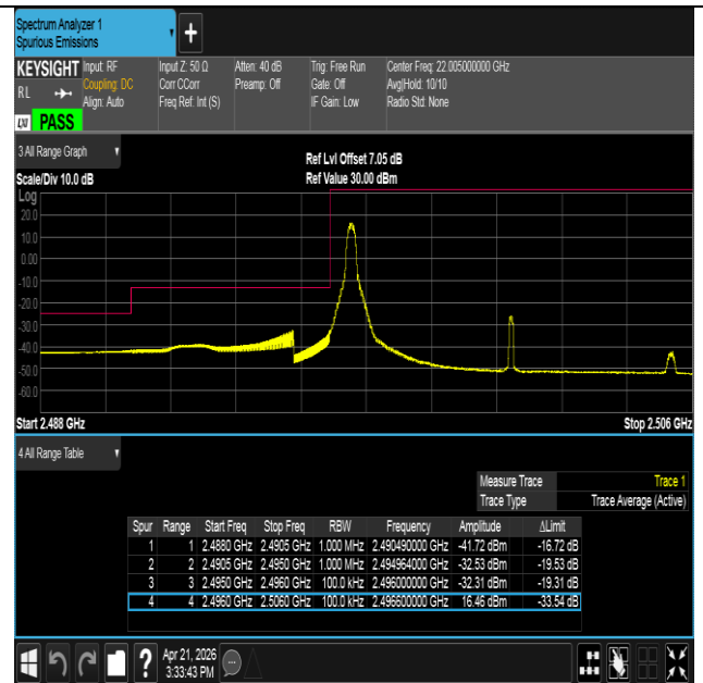
Band41-10MHz-16QAM-39700-1RB#0-PASS
