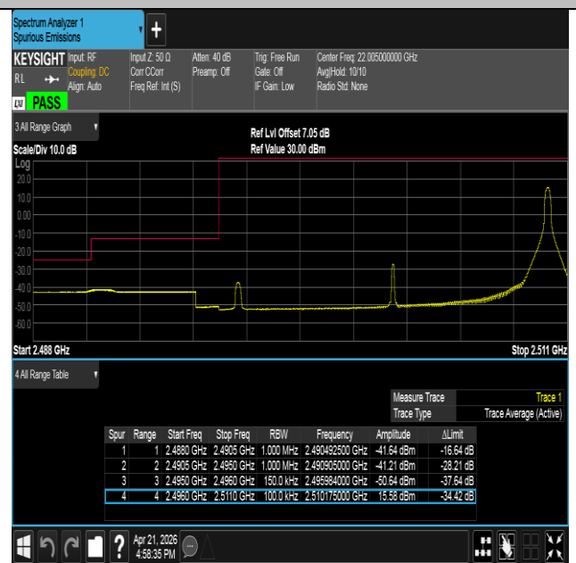
Band41-15MHz-QPSK-39725-1RB#74-PASS
