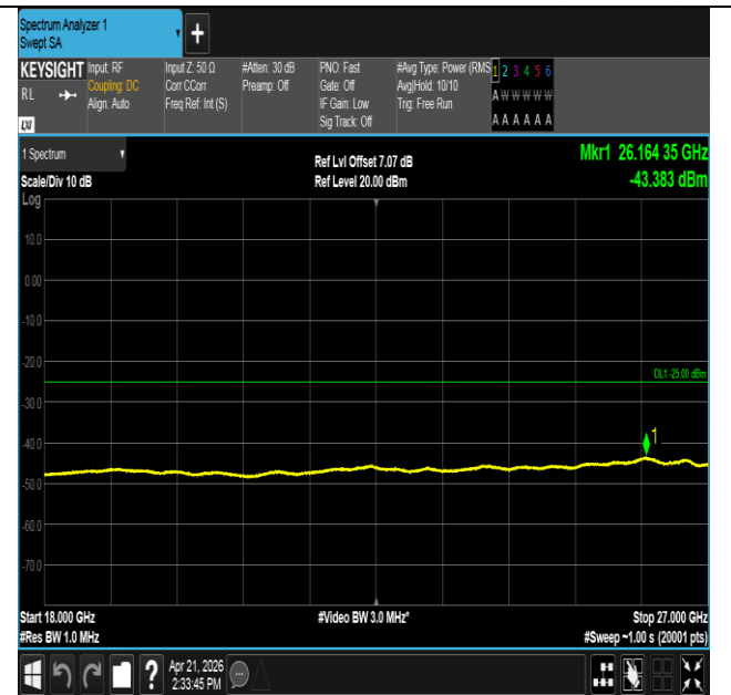
Band41-5MHz-QPSK-39675-1RB#24-18000~27000-PASS
