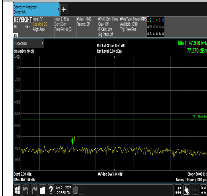
Band41-5MHz-QPSK-39675-25RB#0-0.009~0.15-PASS
