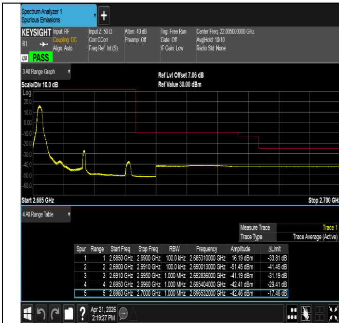
Band41-5MHz-QPSK-41565-1RB#0-PASS
