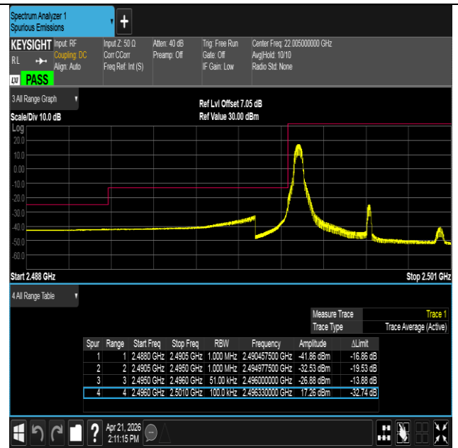
Band41-5MHz-16QAM-39675-1RB#0-PASS
