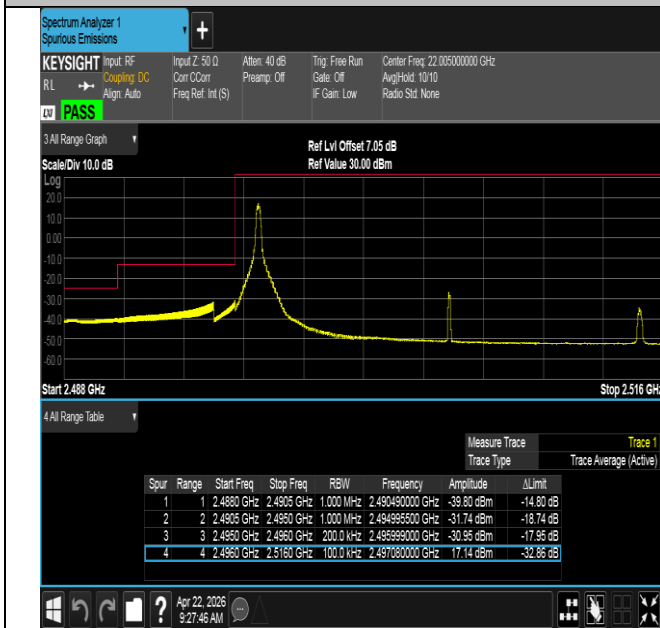
Band41-20MHz-QPSK-39750-1RB#0-PASS
