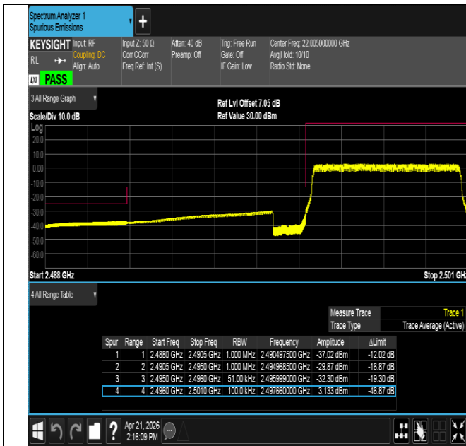
Band41-5MHz-QPSK-39675-25RB#0-PASS
