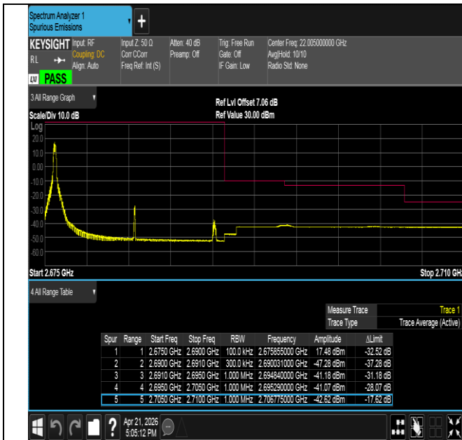
Band41-15MHz-QPSK-41515-1RB#0-PASS
