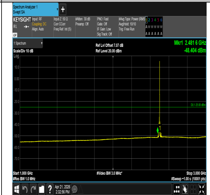
Band41-5MHz-QPSK-39675-1RB#24-1000~3000-PASS
