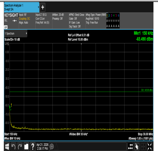
Band41-5MHz-QPSK-39675-25RB#0-0.15~30-PASS
