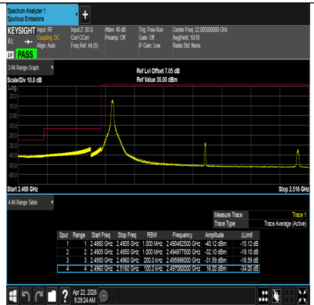
Band41-20MHz-16QAM-39750-1RB#0-PASS
