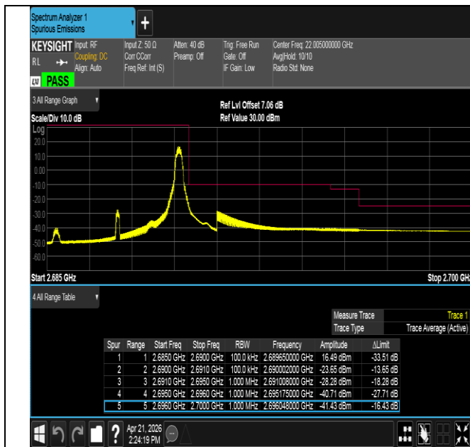
Band41-5MHz-16QAM-41565-1RB#24-PASS
