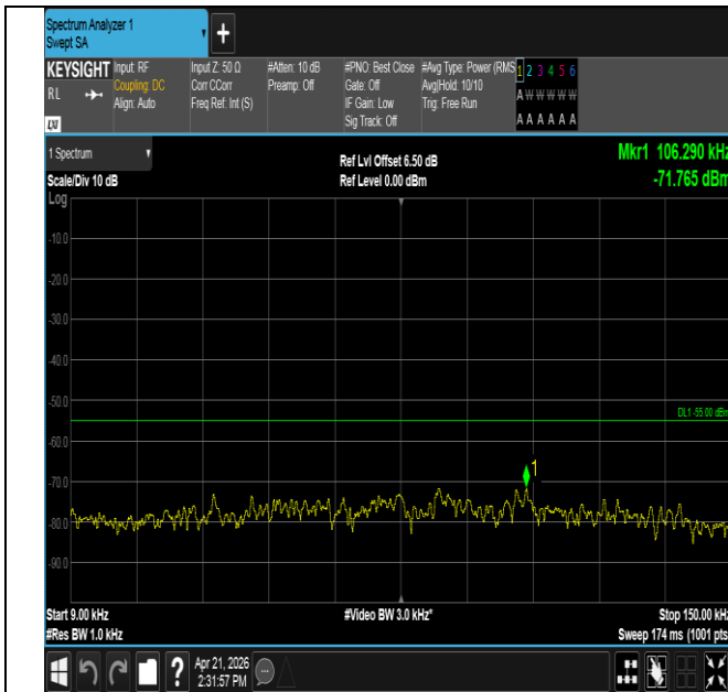
Band41-5MHz-QPSK-39675-1RB#24-0.009~0.15-PASS
