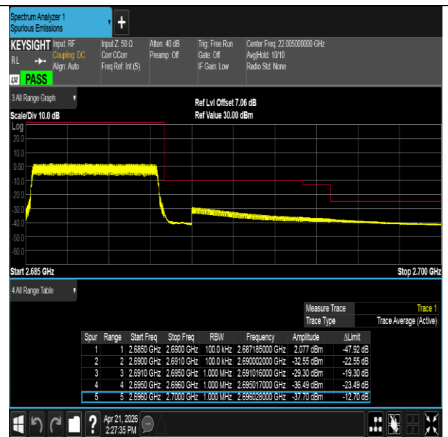
Band41-5MHz-16QAM-41565-25RB#0-PASS
