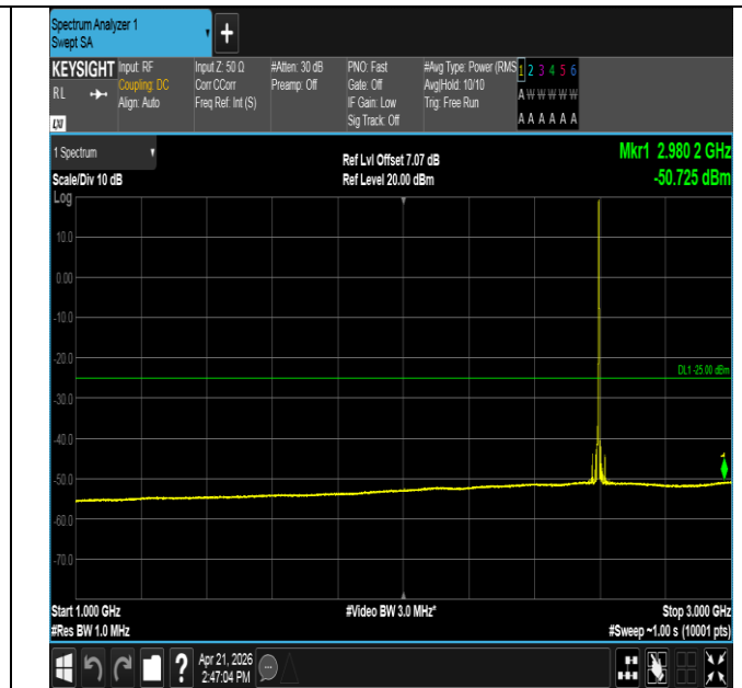
Band41-5MHz-16QAM-40620-1RB#24-1000~3000-PASS
