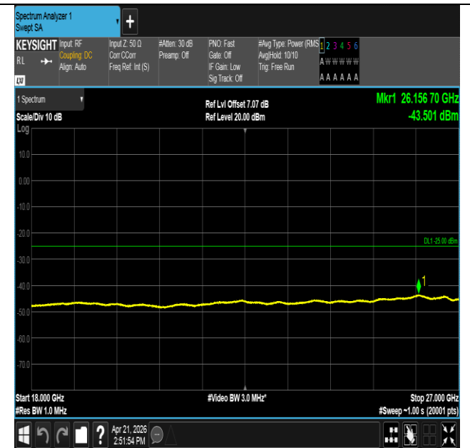
Band41-5MHz-16QAM-40620-25RB#0-18000~27000-PASS
