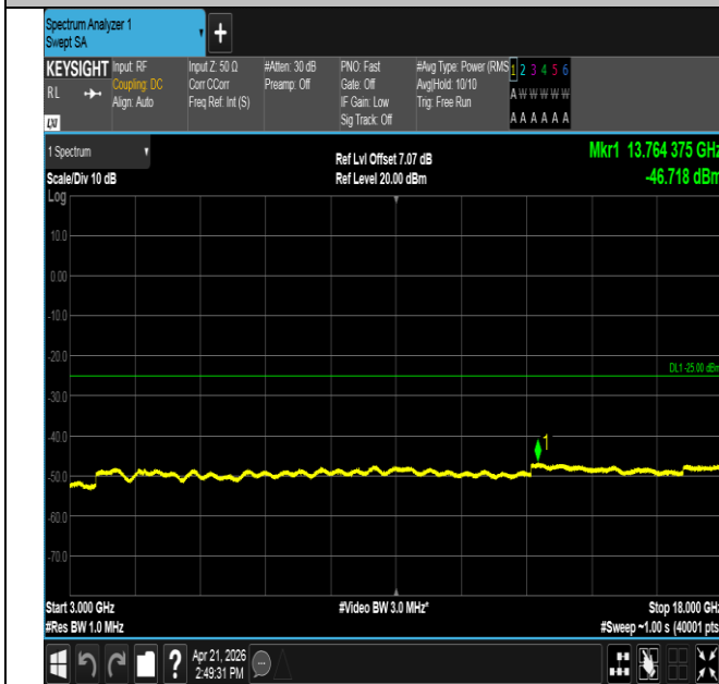
Band41-5MHz-QPSK-40620-25RB#0-3000~18000-PASS
