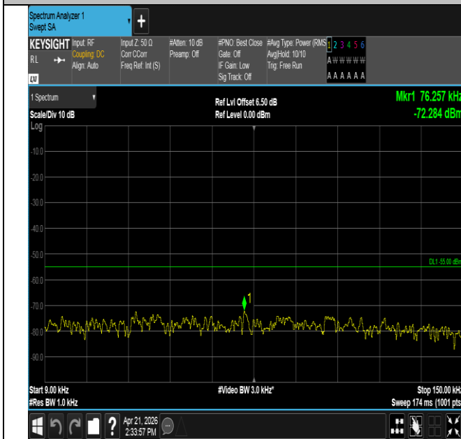
Band41-5MHz-16QAM-39675-1RB#24-0.009~0.15-PASS
