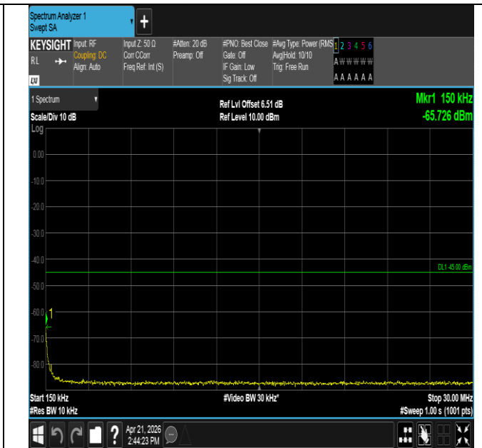
Band41-5MHz-QPSK-40620-1RB#24-0.15~30-PASS
