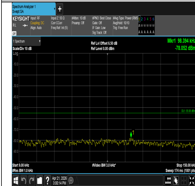
Band41-5MHz-QPSK-41565-25RB#0-0.009~0.15-PASS
