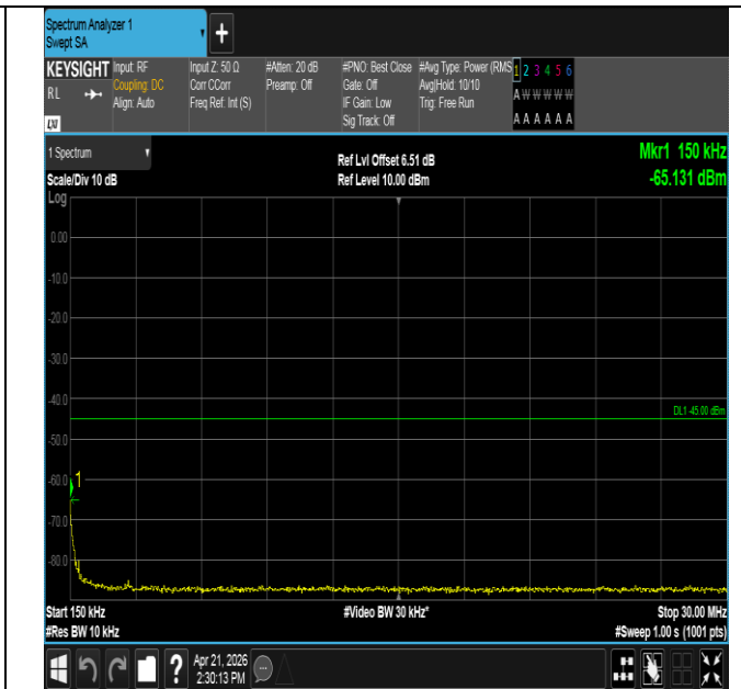
Band41-5MHz-16QAM-39675-1RB#0-0.15~30-PASS
