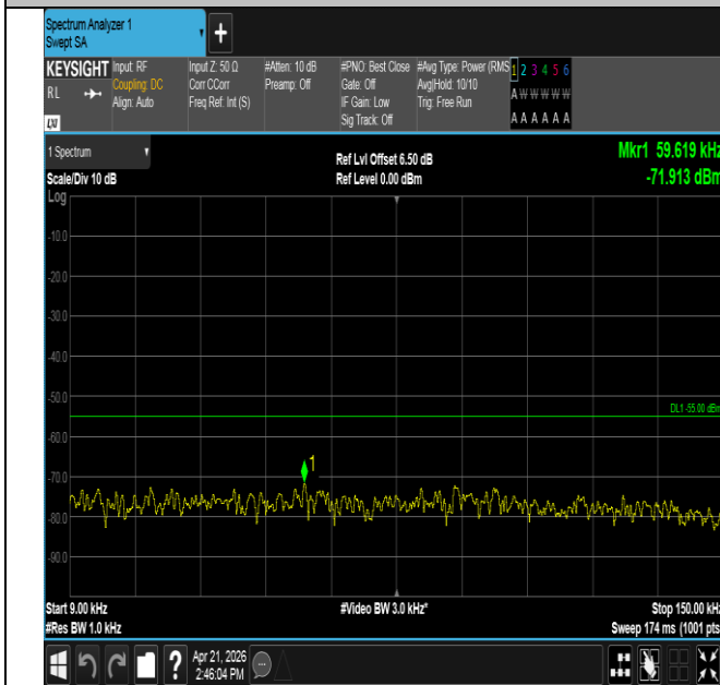
Band41-5MHz-16QAM-40620-1RB#24-0.009~0.15-PASS
