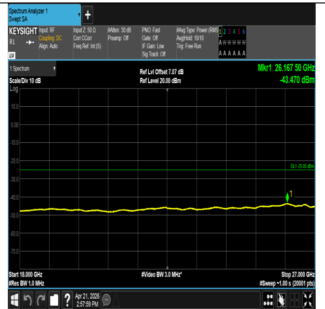
Band41-5MHz-QPSK-41565-1RB#24-18000~27000-PASS
