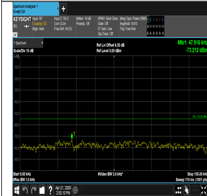
Band41-5MHz-QPSK-41565-1RB#0-0.009~0.15-PASS
