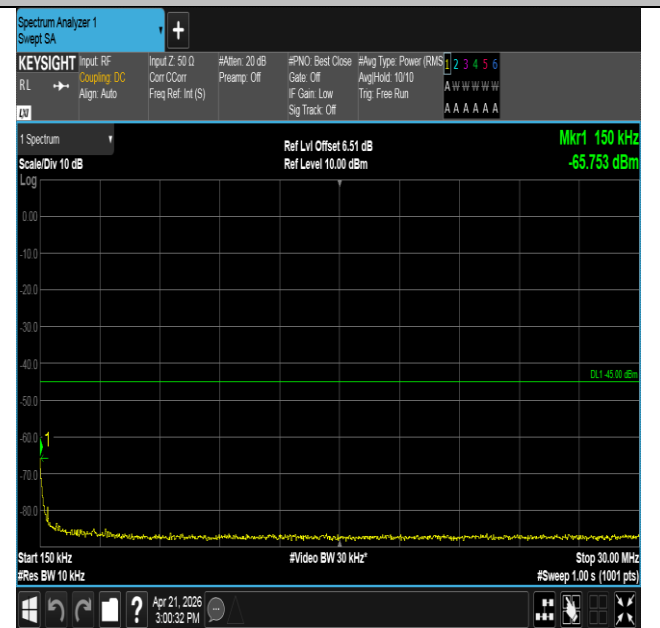
Band41-5MHz-QPSK-41565-25RB#0-0.15~30-PASS
