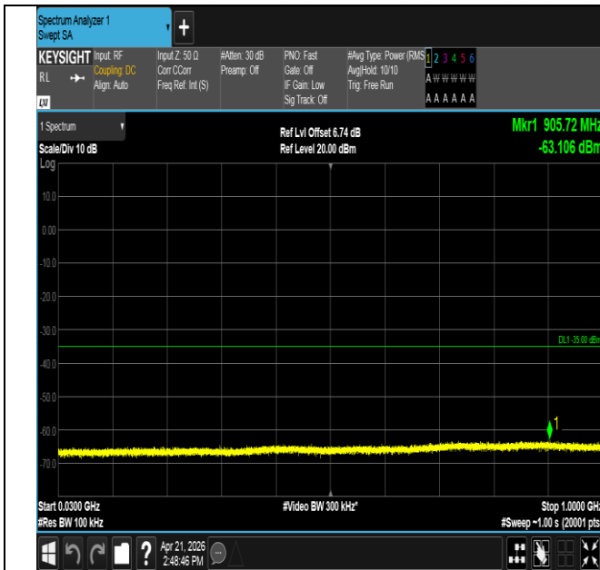
Band41-5MHz-QPSK-40620-25RB#0-30~1000-PASS
