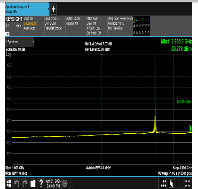
Band41-5MHz-16QAM-40620-1RB#0-1000~3000-PASS
