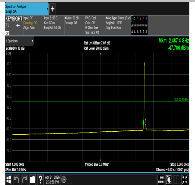
Band41-5MHz-16QAM-39675-25RB#0-1000~3000-PASS
