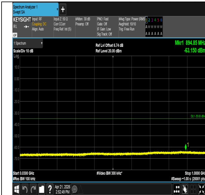
Band41-5MHz-QPSK-41565-1RB#0-30~1000-PASS
