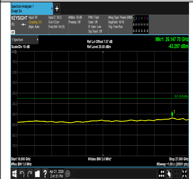
Band41-5MHz-QPSK-40620-1RB#0-18000~27000-PASS
