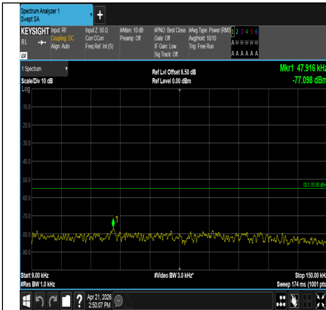
Band41-5MHz-16QAM-40620-25RB#0-0.009~0.15-PASS
