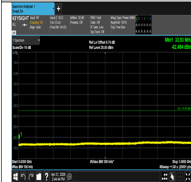
Band41-5MHz-QPSK-40620-1RB#24-30~1000-PASS
