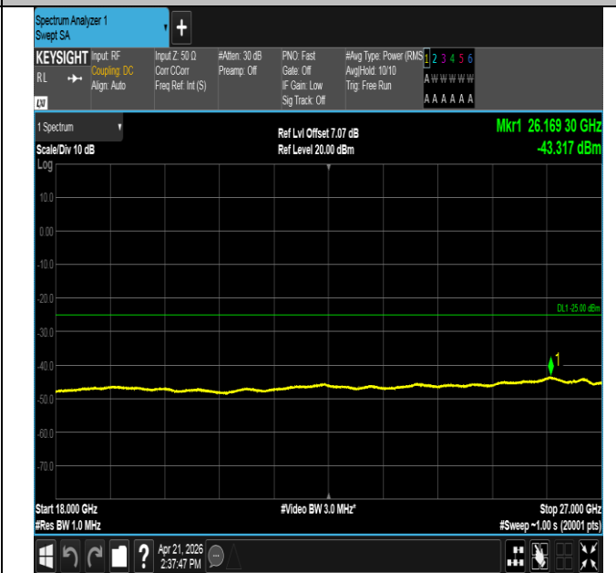
Band41-5MHz-QPSK-39675-25RB#0-18000~27000-PASS
