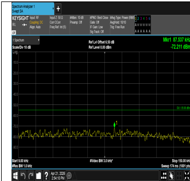
Band41-5MHz-16QAM-41565-1RB#0-0.009~0.15-PASS
