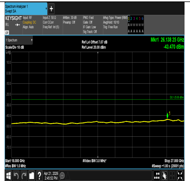
Band41-5MHz-QPSK-40620-1RB#24-18000~27000-PASS
