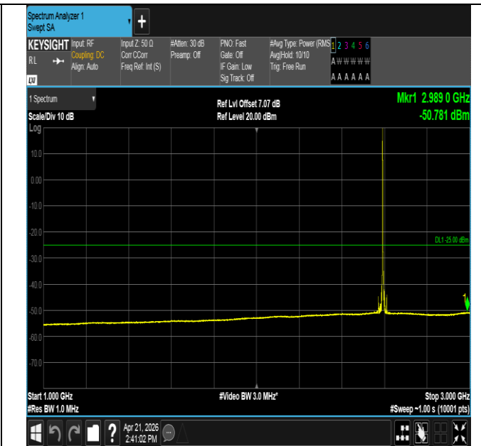
Band41-5MHz-QPSK-40620-1RB#0-1000~3000-PASS
