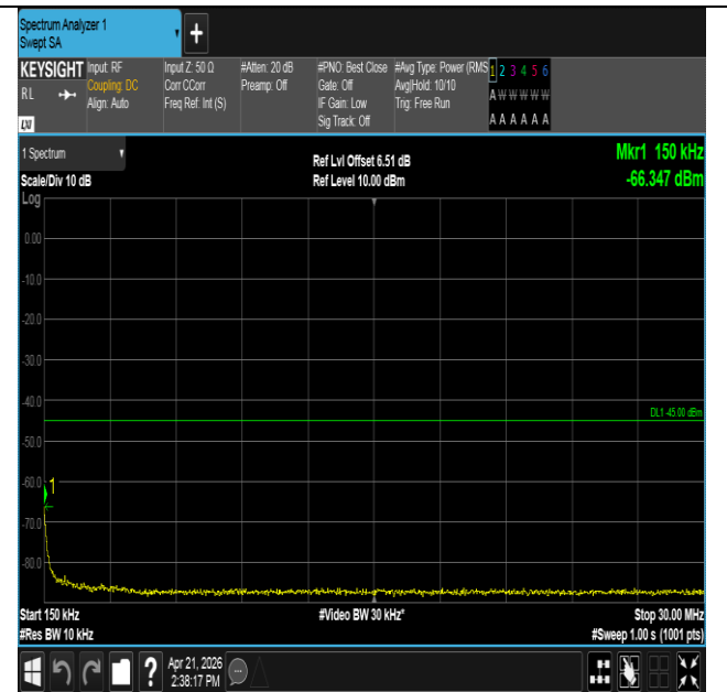
Band41-5MHz-16QAM-39675-25RB#0-0.15~30-PASS
