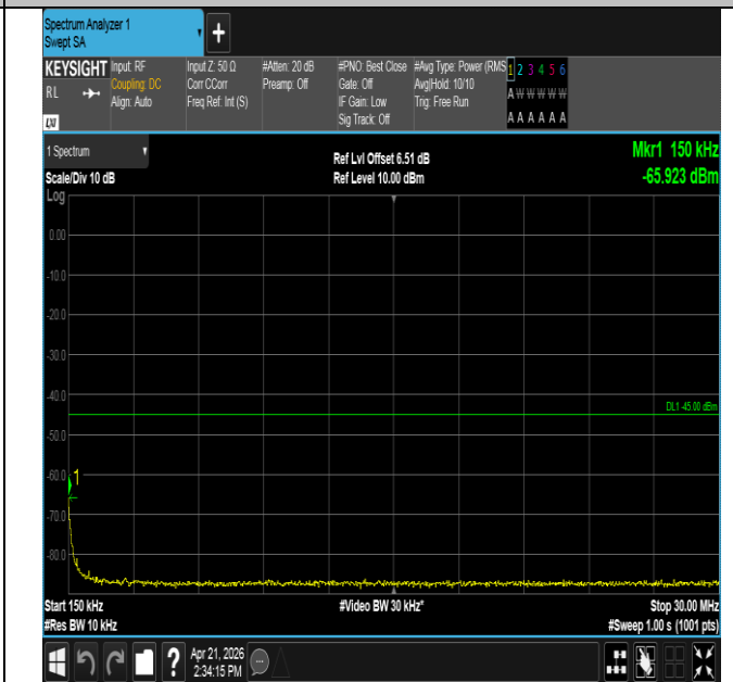
Band41-5MHz-16QAM-39675-1RB#24-0.15~30-PASS
