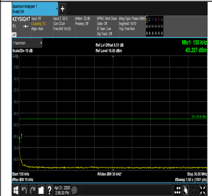
Band41-5MHz-16QAM-41565-1RB#24-0.15~30-PASS
