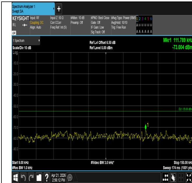
Band41-5MHz-QPSK-41565-1RB#24-0.009~0.15-PASS
