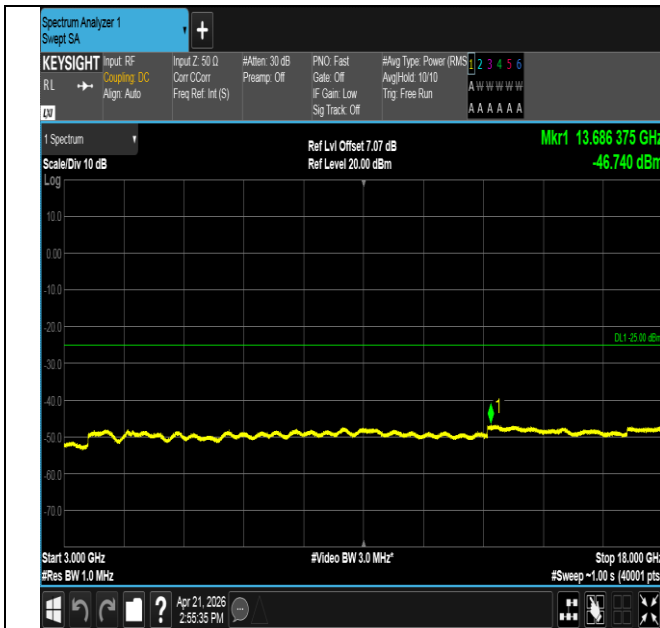
Band41-5MHz-16QAM-41565-1RB#0-3000~18000-PASS
