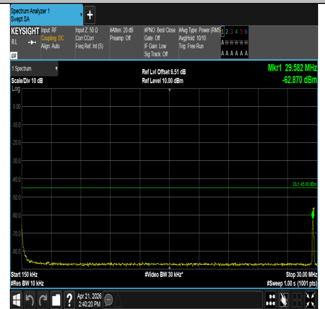
Band41-5MHz-QPSK-40620-1RB#0-0.15~30-PASS
