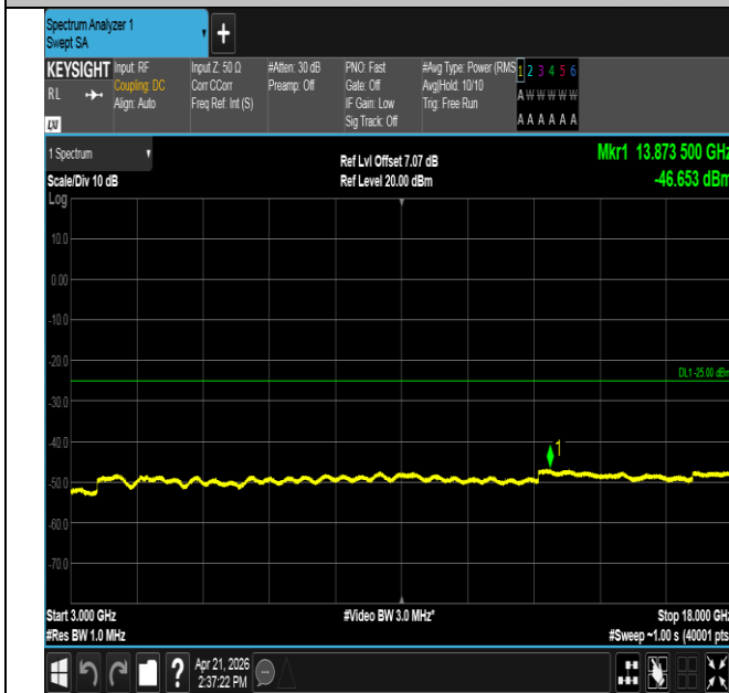
Band41-5MHz-QPSK-39675-25RB#0-3000~18000-PASS
