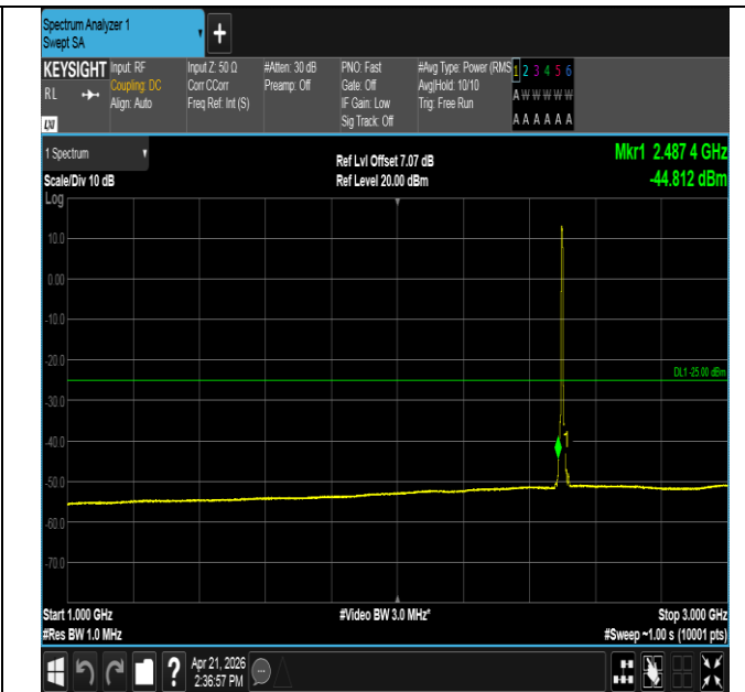
Band41-5MHz-QPSK-39675-25RB#0-1000~3000-PASS
