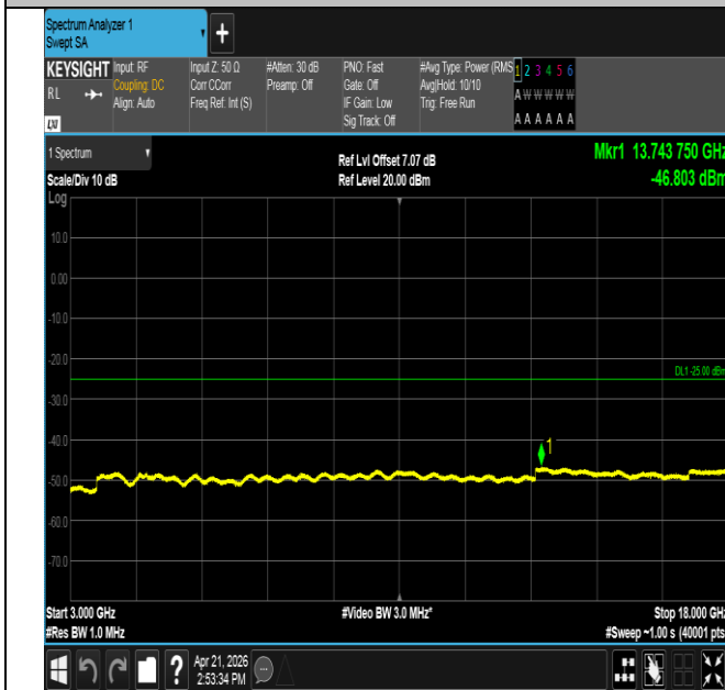
Band41-5MHz-QPSK-41565-1RB#0-3000~18000-PASS
