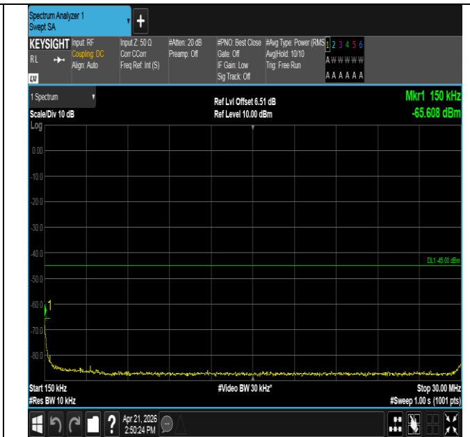
Band41-5MHz-16QAM-40620-25RB#0-0.15~30-PASS
