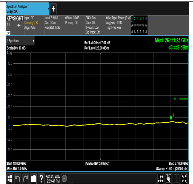
Band41-5MHz-16QAM-39675-25RB#0-18000~27000-PASS
