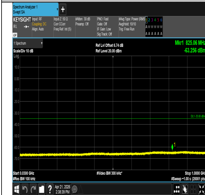
Band41-5MHz-16QAM-39675-25RB#0-30~1000-PASS
