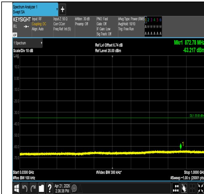
Band41-5MHz-QPSK-39675-25RB#0-30~1000-PASS
