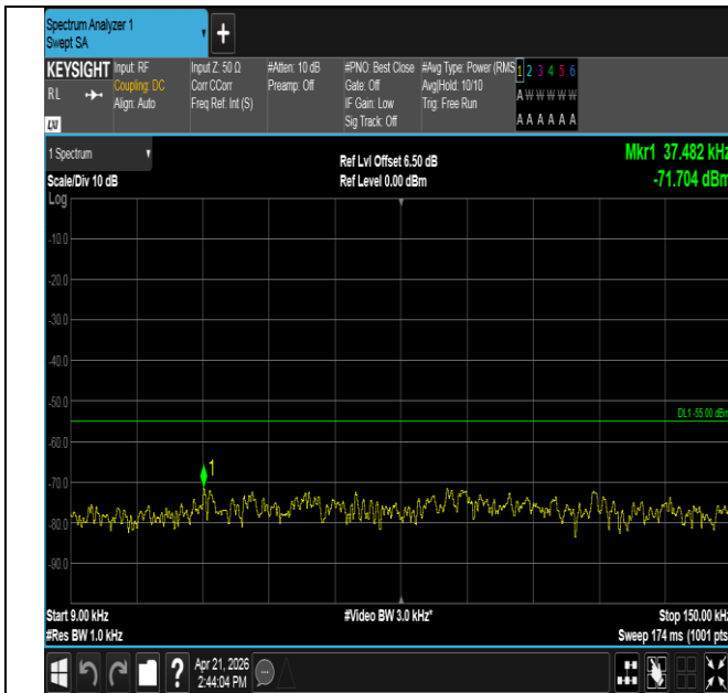
Band41-5MHz-QPSK-40620-1RB#24-0.009~0.15-PASS
