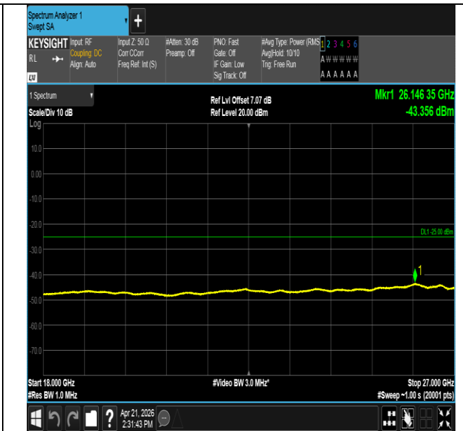
Band41-5MHz-16QAM-39675-1RB#0-18000~27000-PASS
