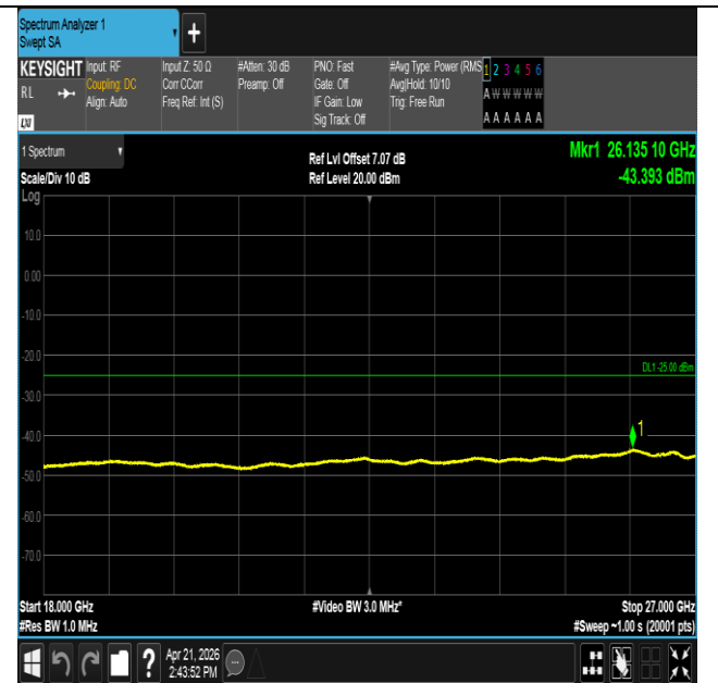
Band41-5MHz-16QAM-40620-1RB#0-18000~27000-PASS
