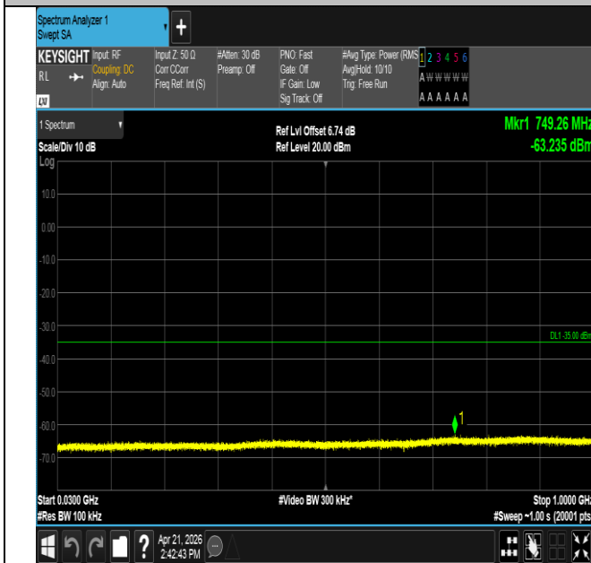
Band41-5MHz-16QAM-40620-1RB#0-30~1000-PASS
