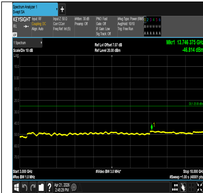
Band41-5MHz-QPSK-40620-1RB#24-3000~18000-PASS
