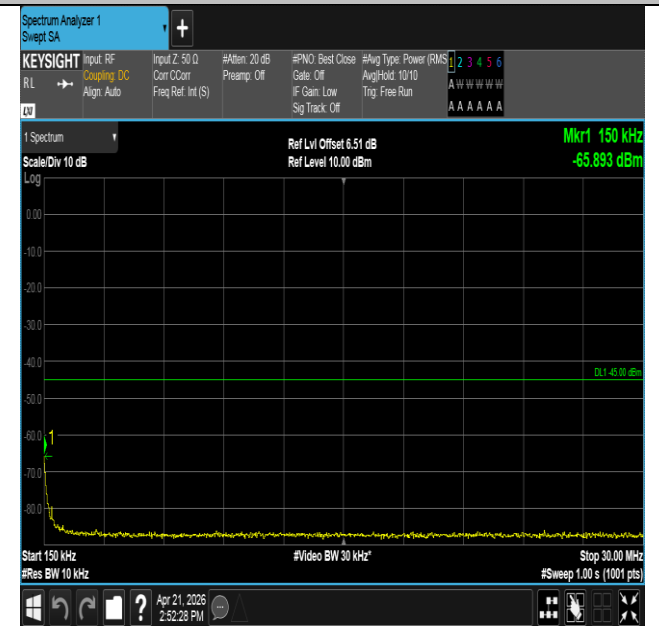
Band41-5MHz-QPSK-41565-1RB#0-0.15~30-PASS
