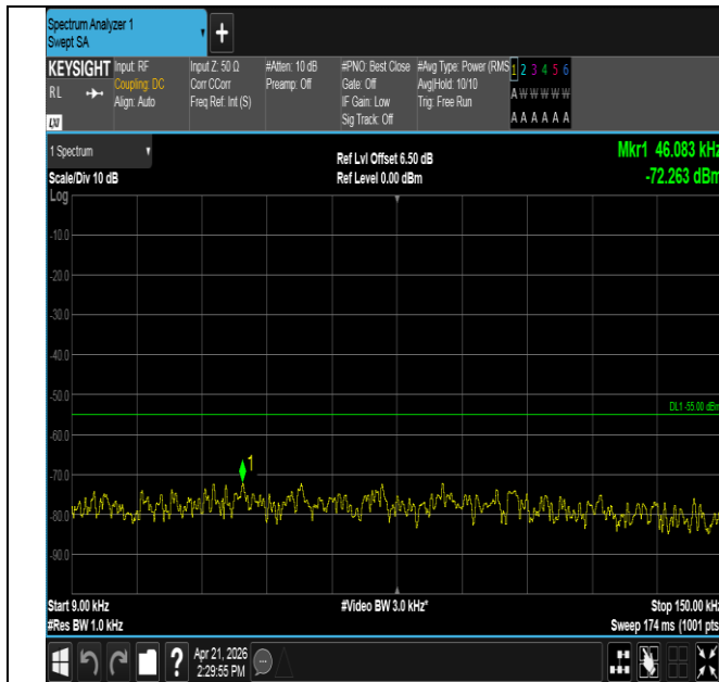
Band41-5MHz-16QAM-39675-1RB#0-0.009~0.15-PASS
