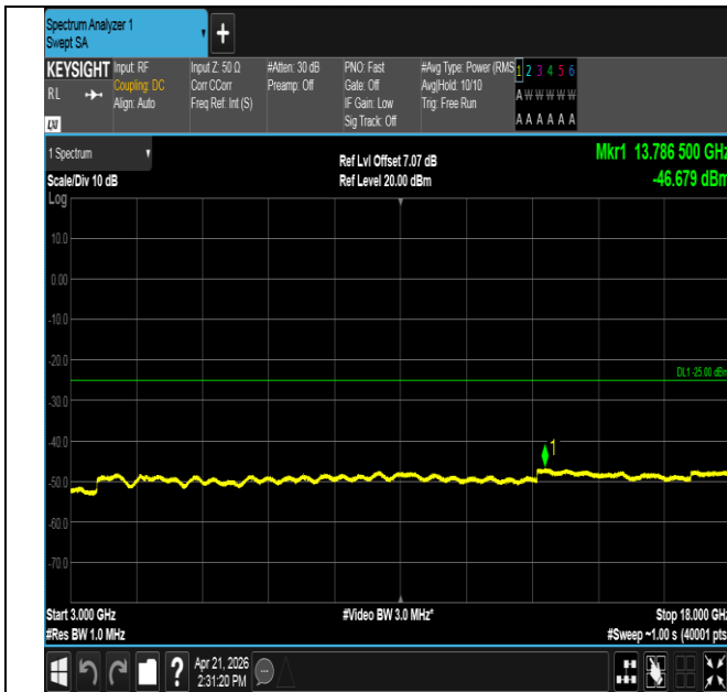
Band41-5MHz-16QAM-39675-1RB#0-3000~18000-PASS
