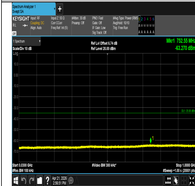
Band41-5MHz-QPSK-41565-1RB#24-30~1000-PASS
