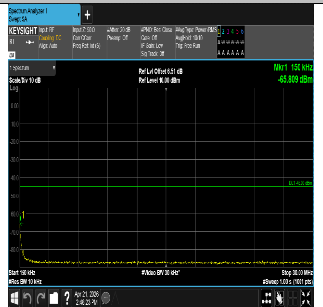
Band41-5MHz-16QAM-40620-1RB#24-0.15~30-PASS
