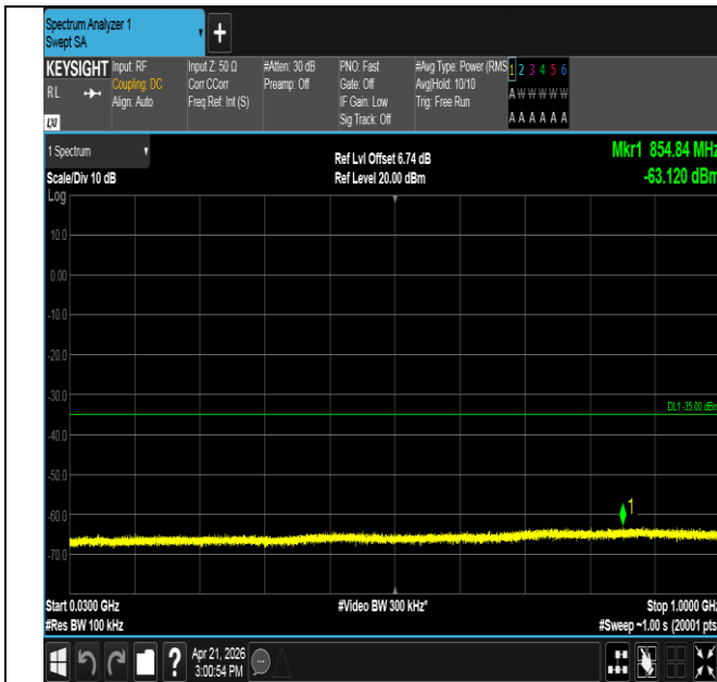
Band41-5MHz-QPSK-41565-25RB#0-30~1000-PASS
