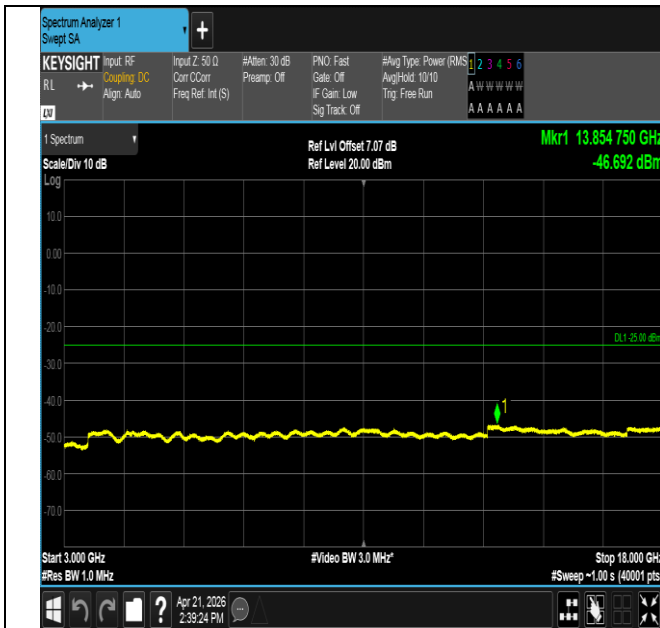
Band41-5MHz-16QAM-39675-25RB#0-3000~18000-PASS
