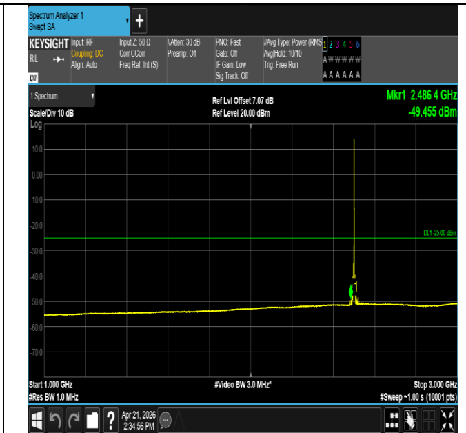
Band41-5MHz-16QAM-39675-1RB#24-1000~3000-PASS
