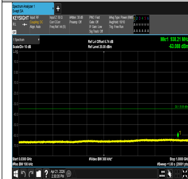
Band41-5MHz-16QAM-39675-1RB#0-30~1000-PASS
