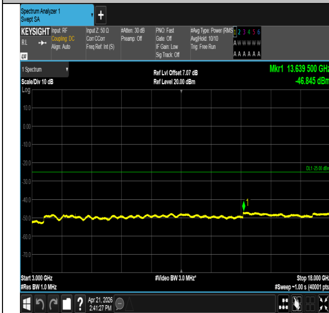
Band41-5MHz-QPSK-40620-1RB#0-3000~18000-PASS
