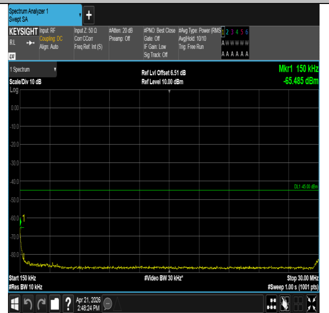
Band41-5MHz-QPSK-40620-25RB#0-0.15~30-PASS
