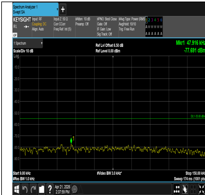
Band41-5MHz-16QAM-39675-25RB#0-0.009~0.15-PASS
