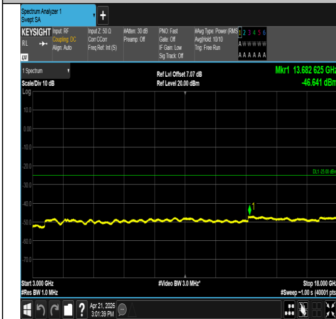
Band41-5MHz-QPSK-41565-25RB#0-3000~18000-PASS
