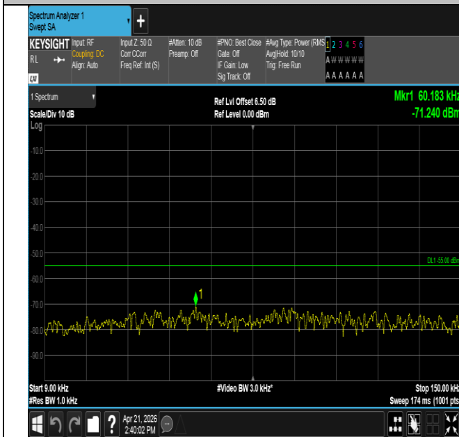
Band41-5MHz-QPSK-40620-1RB#0-0.009~0.15-PASS
