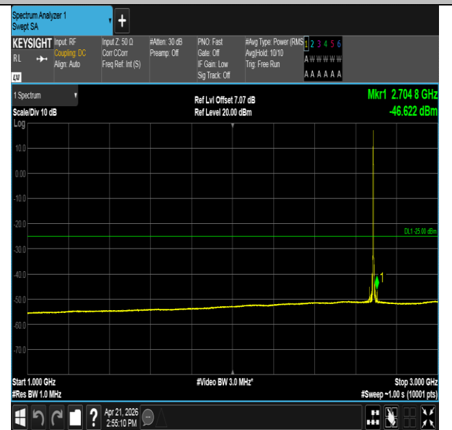
Band41-5MHz-16QAM-41565-1RB#0-1000~3000-PASS
