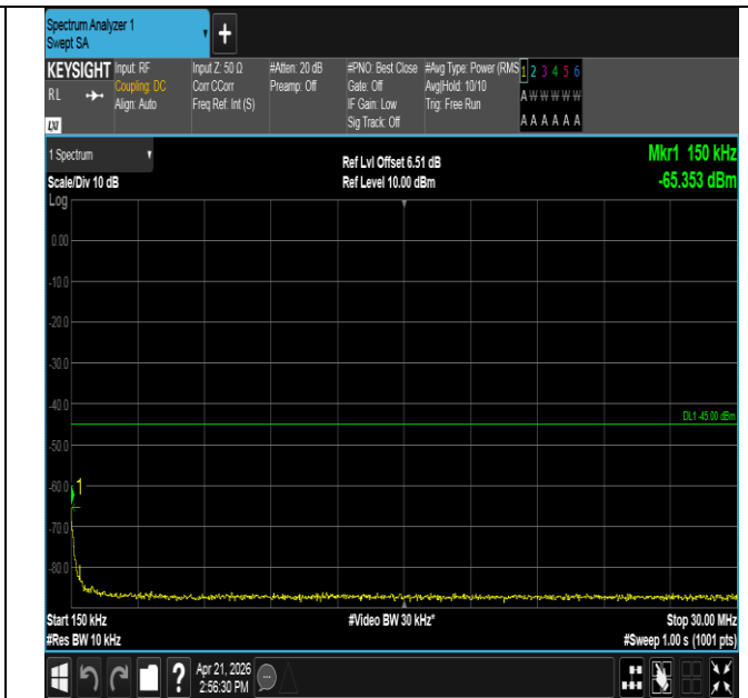
Band41-5MHz-QPSK-41565-1RB#24-0.15~30-PASS
