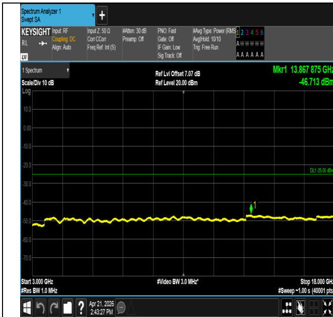
Band41-5MHz-16QAM-40620-1RB#0-3000~18000-PASS
