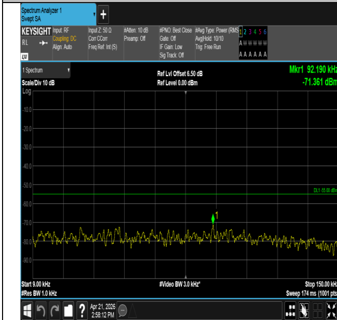
Band41-5MHz-16QAM-41565-1RB#24-0.009~0.15-PASS
