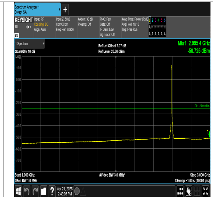
Band41-5MHz-QPSK-40620-25RB#0-1000~3000-PASS
