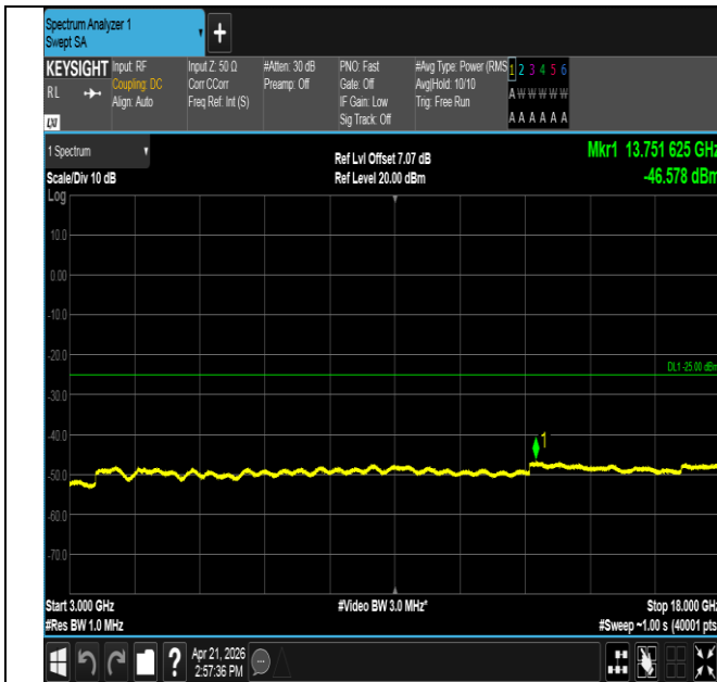
Band41-5MHz-QPSK-41565-1RB#24-3000~18000-PASS
