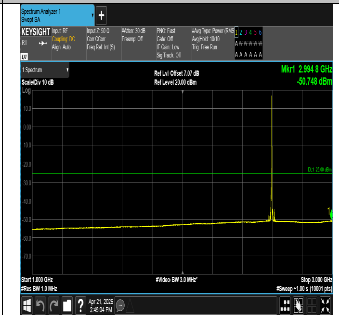
Band41-5MHz-QPSK-40620-1RB#24-1000~3000-PASS
