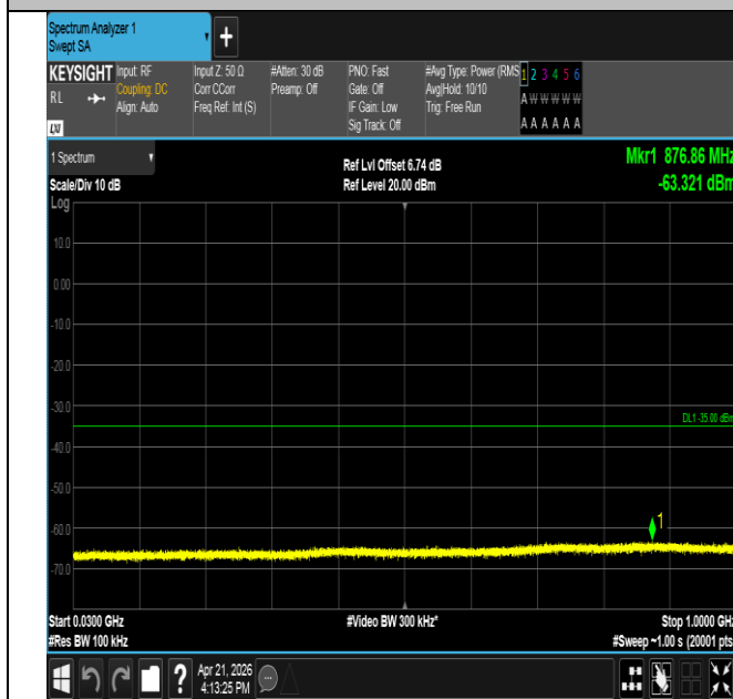
Band41-10MHz-16QAM-40620-50RB#0-30~1000-PASS
