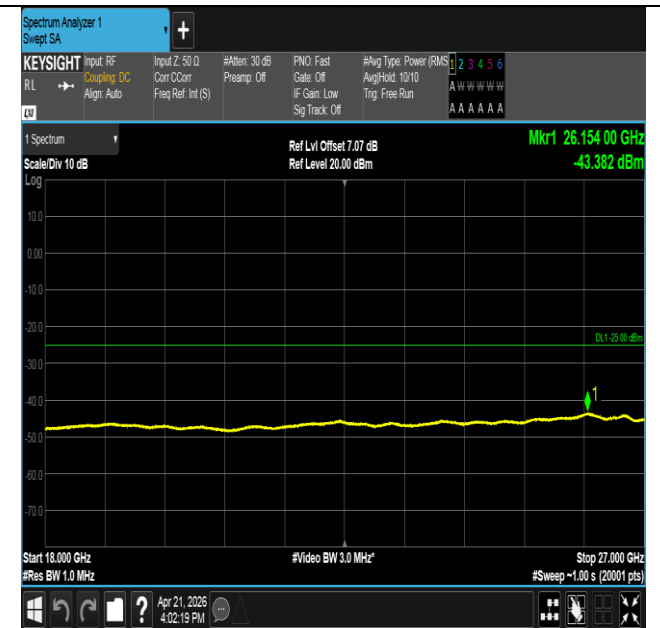
Band41-10MHz-16QAM-39700-50RB#0-18000~27000-PASS
