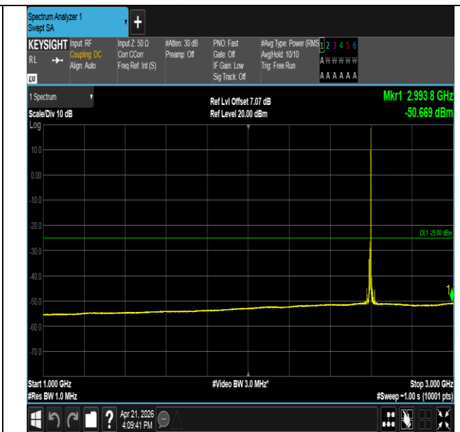
Band41-10MHz-16QAM-40620-1RB#49-1000~3000-PASS
