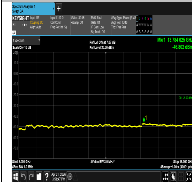
Band41-10MHz-QPSK-39700-1RB#0-3000~18000-PASS
