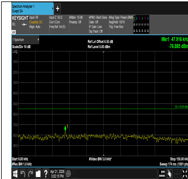
Band41-5MHz-16QAM-41565-25RB#0-0.009~0.15-PASS
