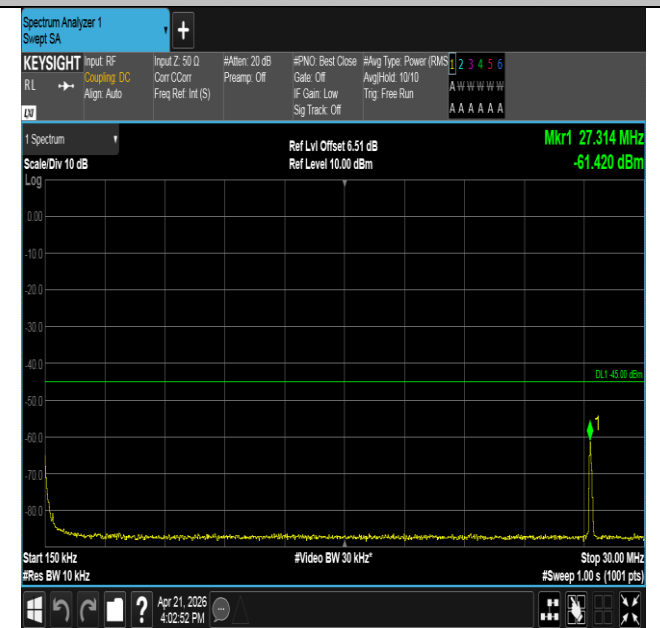
Band41-10MHz-QPSK-40620-1RB#0-0.15~30-PASS
