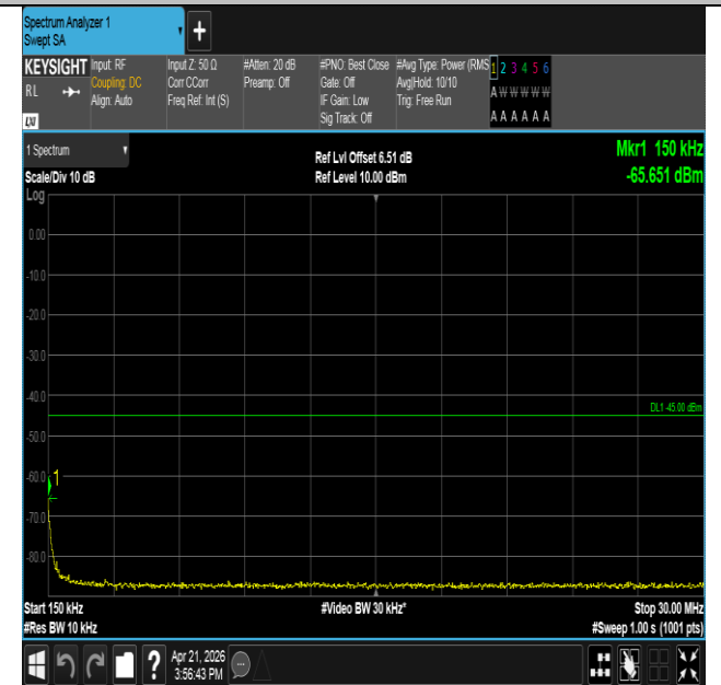
Band41-10MHz-16QAM-39700-1RB#49-0.15~30-PASS
