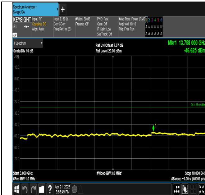
Band41-10MHz-QPSK-39700-1RB#49-3000~18000-PASS
