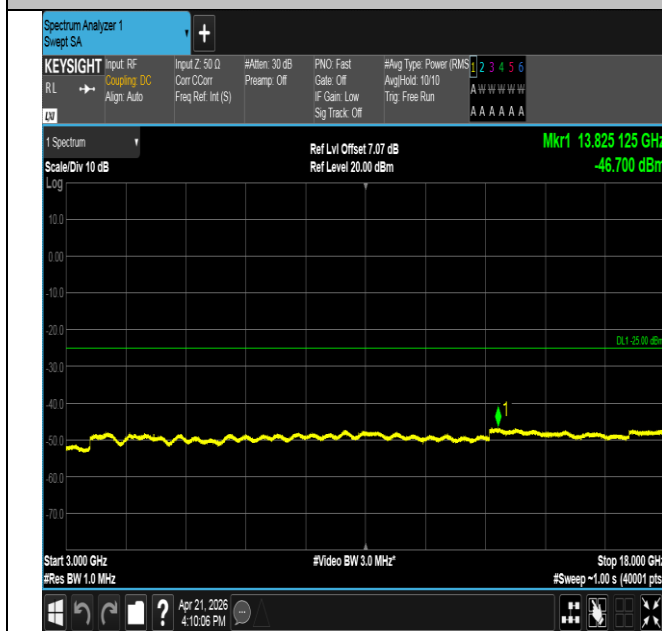
Band41-10MHz-16QAM-40620-1RB#49-3000~18000-PASS
