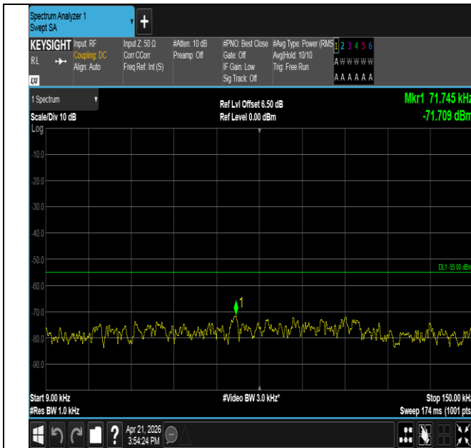
Band41-10MHz-QPSK-39700-1RB#49-0.009~0.15-PASS
