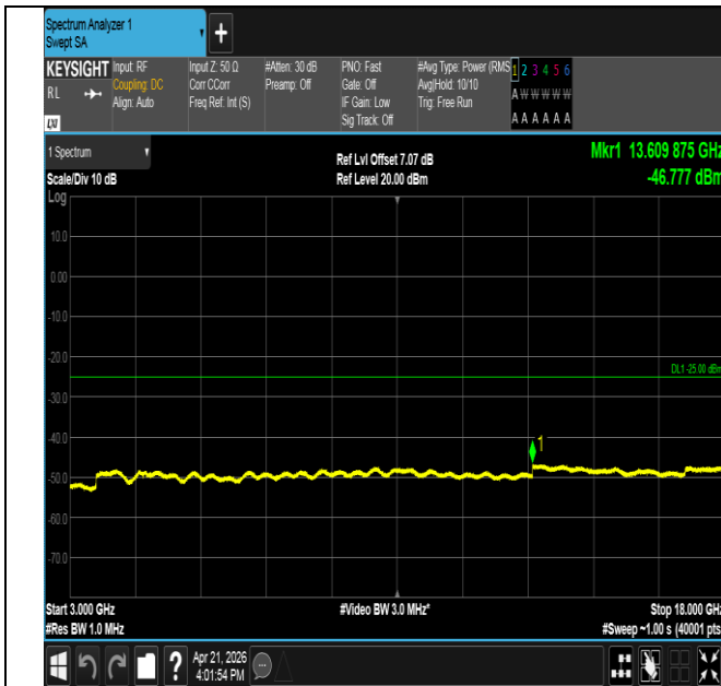
Band41-10MHz-16QAM-39700-50RB#0-3000~18000-PASS
