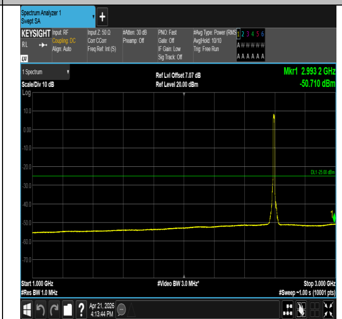
Band41-10MHz-16QAM-40620-50RB#0-1000~3000-PASS
