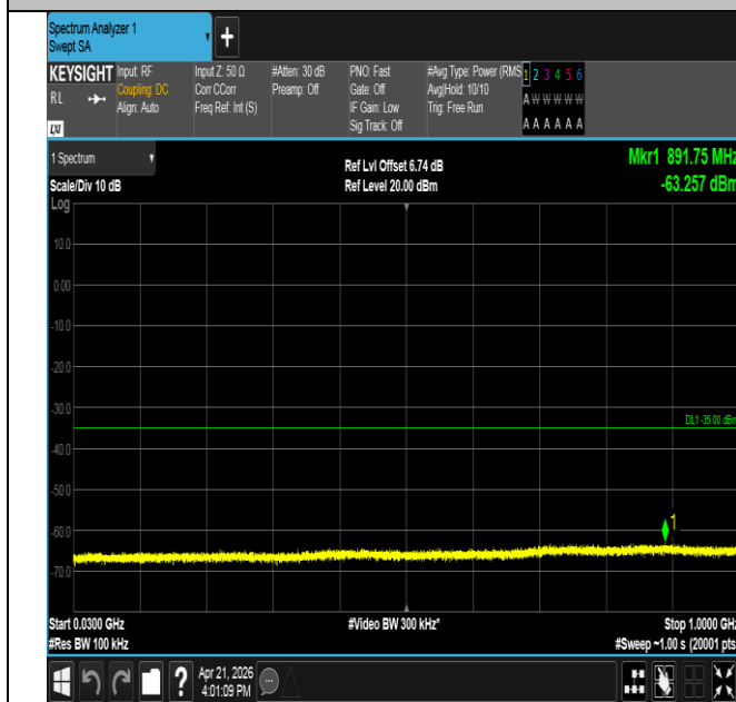
Band41-10MHz-16QAM-39700-50RB#0-30~1000-PASS
