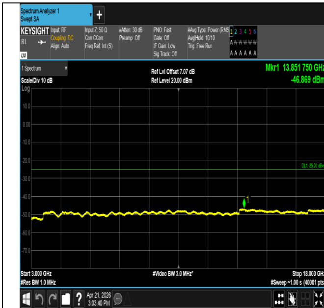
Band41-5MHz-16QAM-41565-25RB#0-3000~18000-PASS
