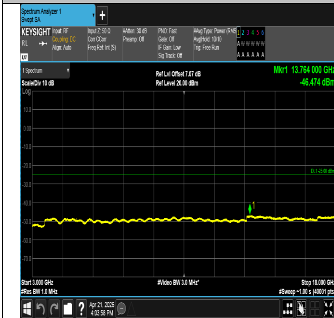
Band41-10MHz-QPSK-40620-1RB#0-3000~18000-PASS
