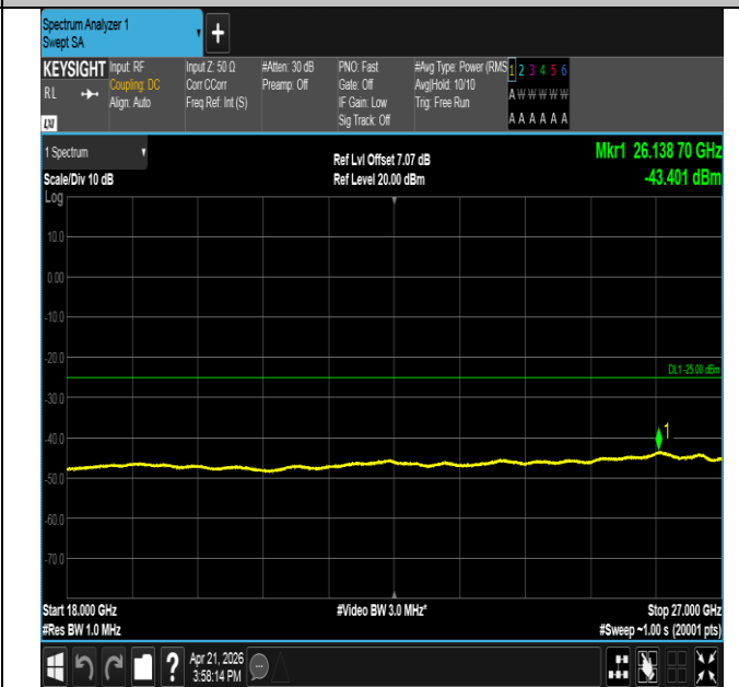
Band41-10MHz-16QAM-39700-1RB#49-18000~27000-PASS
