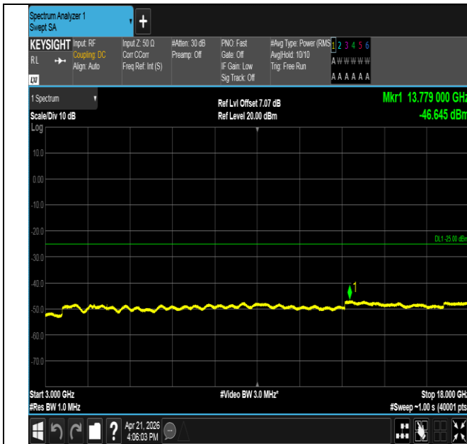
Band41-10MHz-16QAM-40620-1RB#0-3000~18000-PASS
