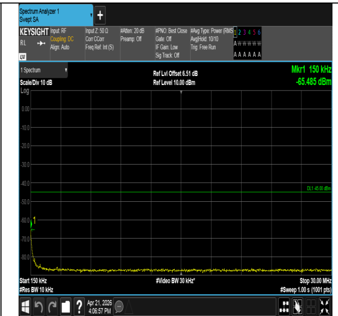
Band41-10MHz-QPSK-40620-1RB#49-0.15~30-PASS
