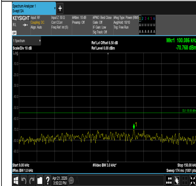
Band41-10MHz-QPSK-39700-1RB#0-0.009~0.15-PASS
