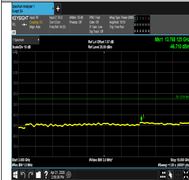
Band41-5MHz-16QAM-41565-1RB#24-3000~18000-PASS
