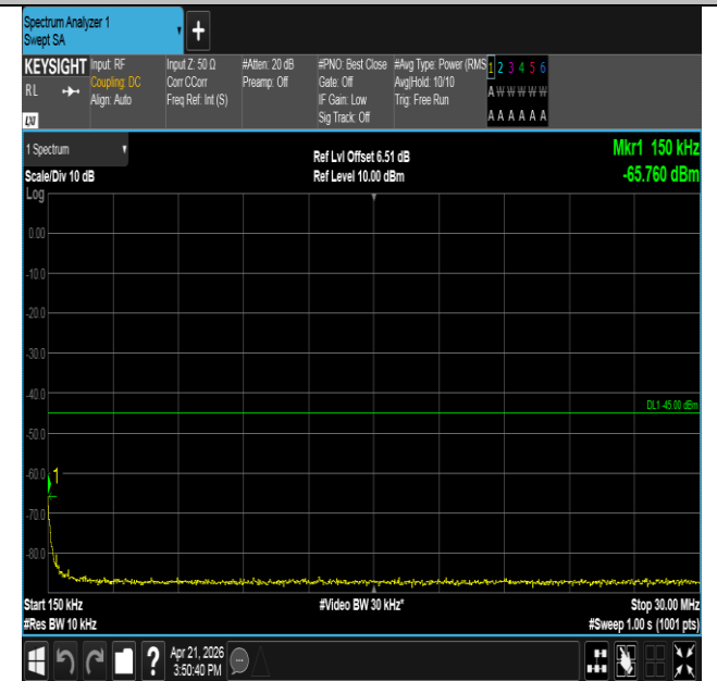
Band41-10MHz-QPSK-39700-1RB#0-0.15~30-PASS
