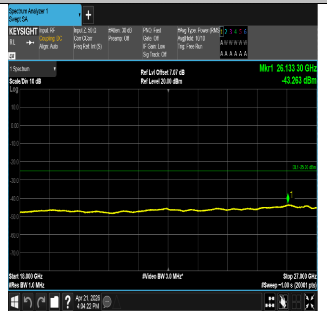
Band41-10MHz-QPSK-40620-1RB#0-18000~27000-PASS
