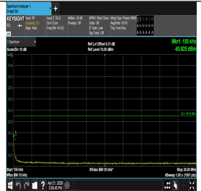
Band41-10MHz-QPSK-39700-50RB#0-0.15~30-PASS
