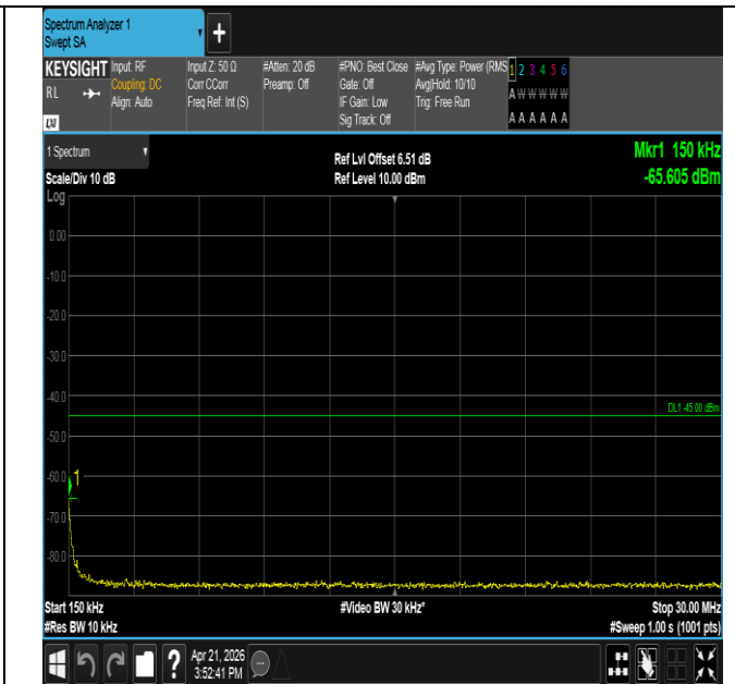
Band41-10MHz-16QAM-39700-1RB#0-0.15~30-PASS
