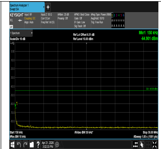
Band41-5MHz-16QAM-41565-25RB#0-0.15~30-PASS
