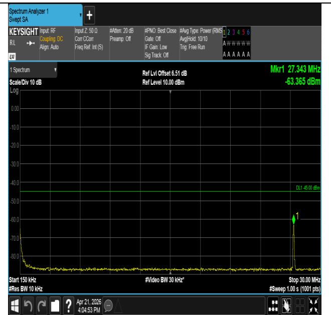
Band41-10MHz-16QAM-40620-1RB#0-0.15~30-PASS
