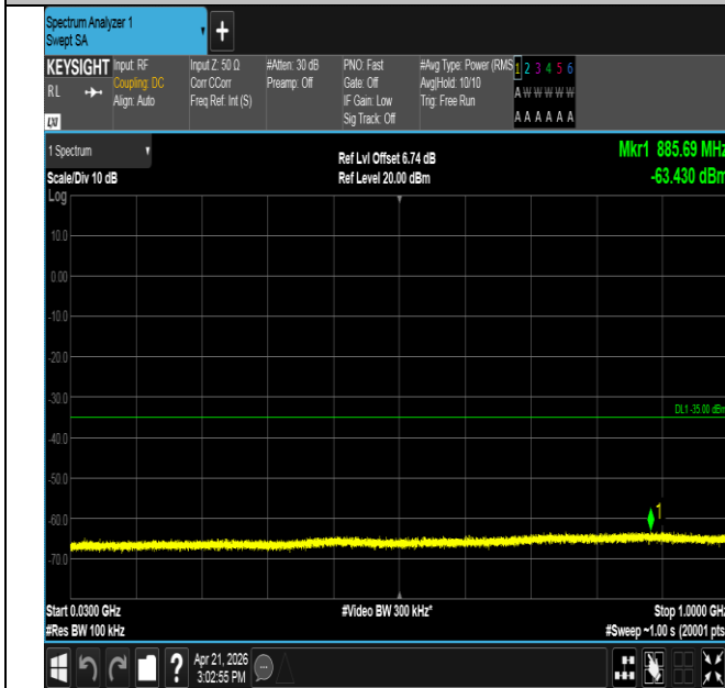
Band41-5MHz-16QAM-41565-25RB#0-30~1000-PASS
