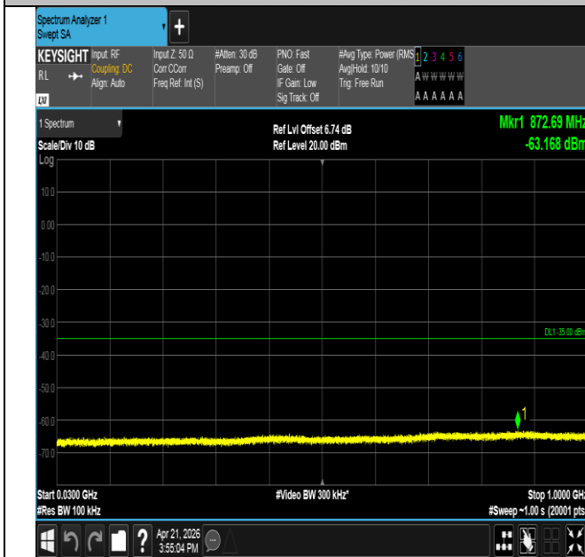
Band41-10MHz-QPSK-39700-1RB#49-30~1000-PASS
