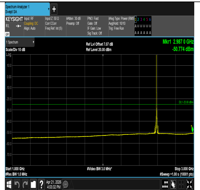
Band41-10MHz-QPSK-40620-1RB#0-1000~3000-PASS
