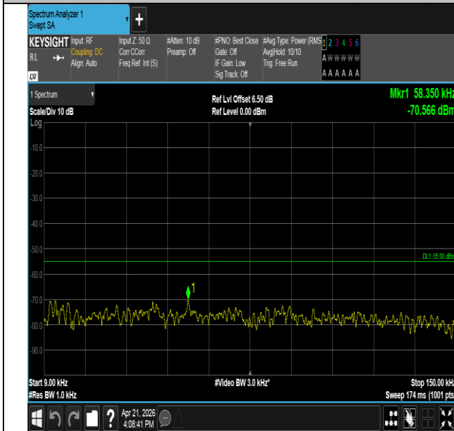
Band41-10MHz-16QAM-40620-1RB#49-0.009~0.15-PASS
