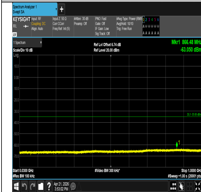
Band41-10MHz-16QAM-39700-1RB#0-30~1000-PASS
