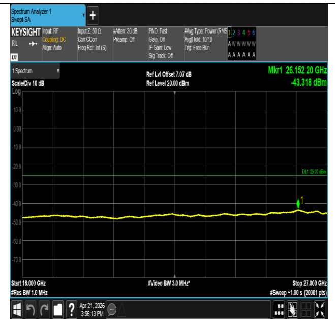
Band41-10MHz-QPSK-39700-1RB#49-18000~27000-PASS
