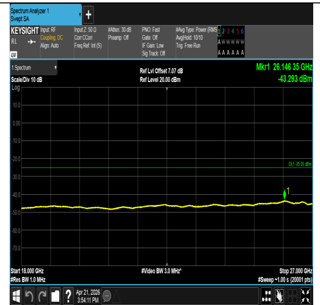
Band41-10MHz-16QAM-39700-1RB#0-18000~27000-PASS
