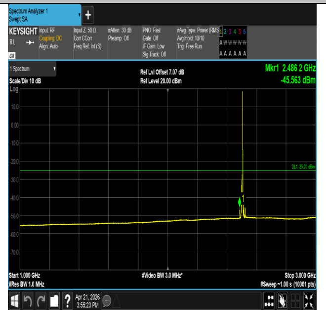
Band41-10MHz-QPSK-39700-1RB#49-1000~3000-PASS
