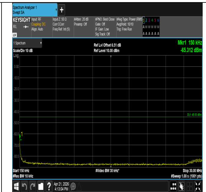
Band41-10MHz-16QAM-40620-50RB#0-0.15~30-PASS
