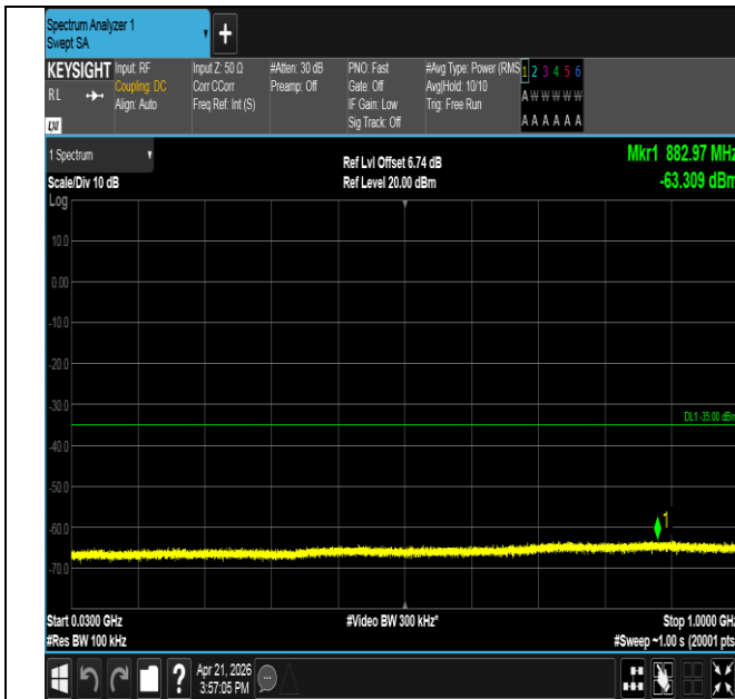
Band41-10MHz-16QAM-39700-1RB#49-30~1000-PASS
