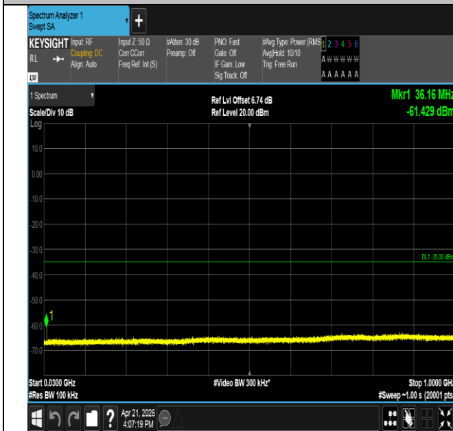
Band41-10MHz-QPSK-40620-1RB#49-30~1000-PASS
