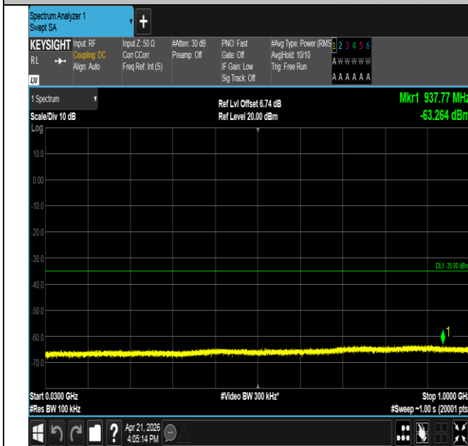
Band41-10MHz-16QAM-40620-1RB#0-30~1000-PASS
