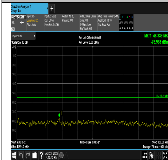
Band41-10MHz-QPSK-40620-50RB#0-0.009~0.15-PASS
