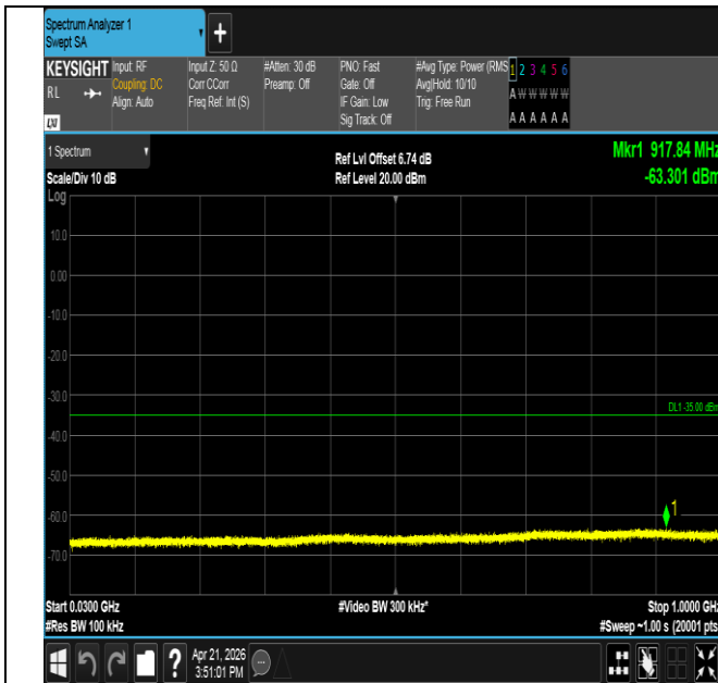
Band41-10MHz-QPSK-39700-1RB#0-30~1000-PASS
