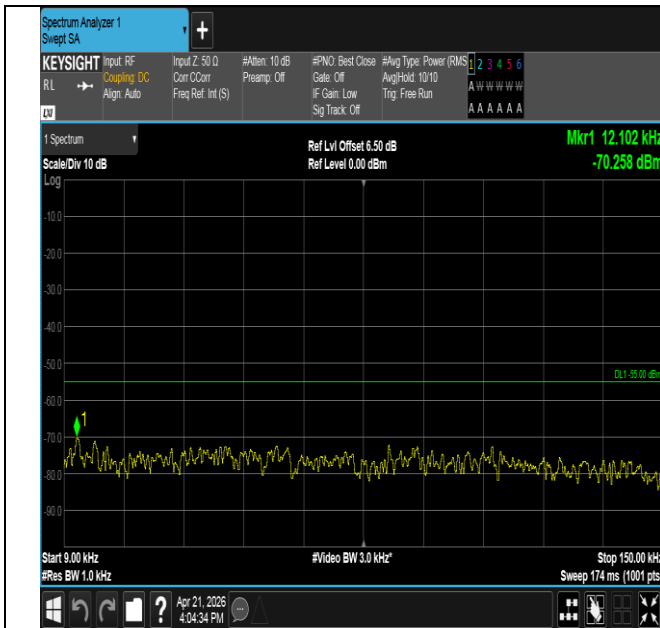
Band41-10MHz-16QAM-40620-1RB#0-0.009~0.15-PASS
