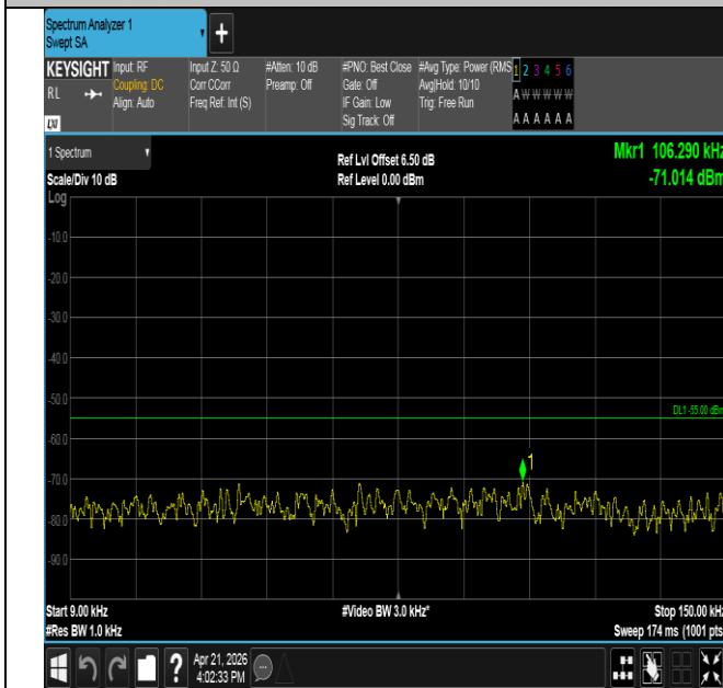
Band41-10MHz-QPSK-40620-1RB#0-0.009~0.15-PASS
