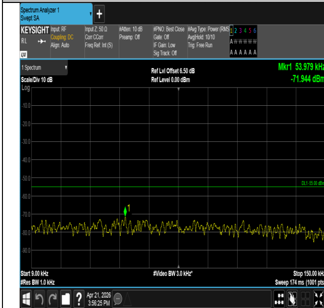
Band41-10MHz-16QAM-39700-1RB#49-0.009~0.15-PASS
