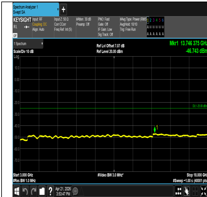
Band41-10MHz-16QAM-39700-1RB#0-3000~18000-PASS
