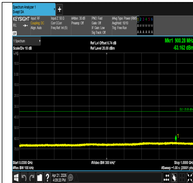
Band41-10MHz-16QAM-40620-1RB#49-30~1000-PASS
