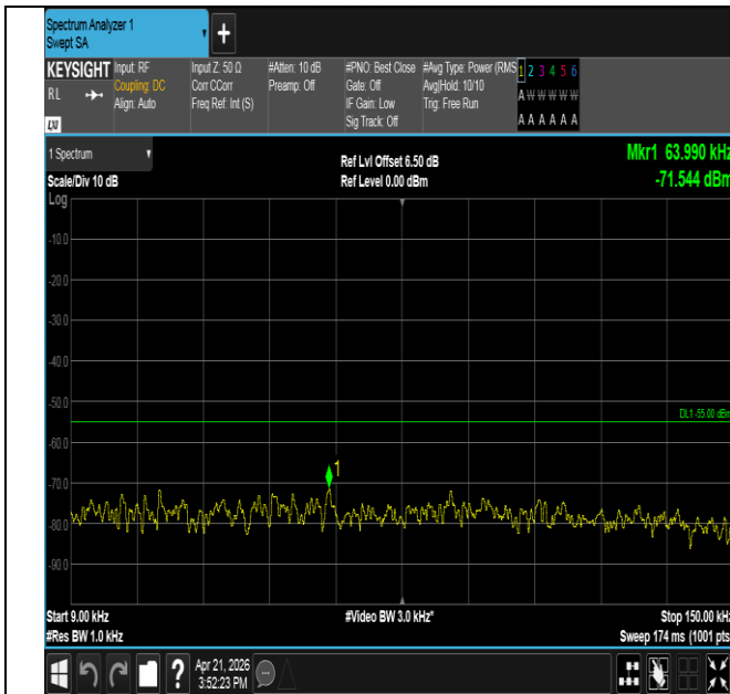
Band41-10MHz-16QAM-39700-1RB#0-0.009~0.15-PASS
