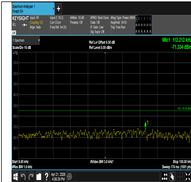
Band41-10MHz-QPSK-40620-1RB#49-0.009~0.15-PASS
