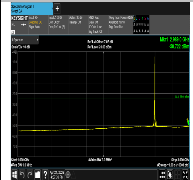
Band41-10MHz-QPSK-40620-1RB#49-1000~3000-PASS
