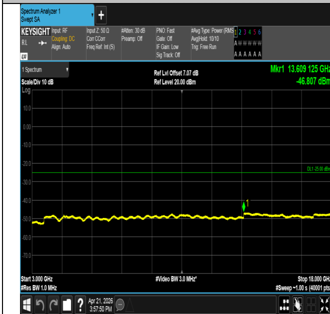
Band41-10MHz-16QAM-39700-1RB#49-3000~18000-PASS
