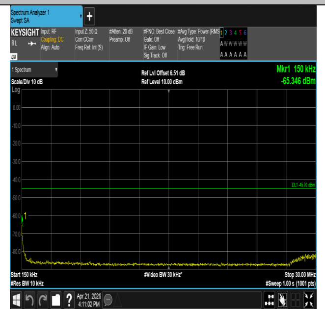
Band41-10MHz-QPSK-40620-50RB#0-0.15~30-PASS
