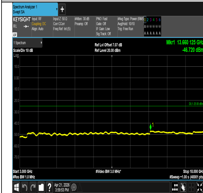
Band41-10MHz-QPSK-39700-50RB#0-3000~18000-PASS
