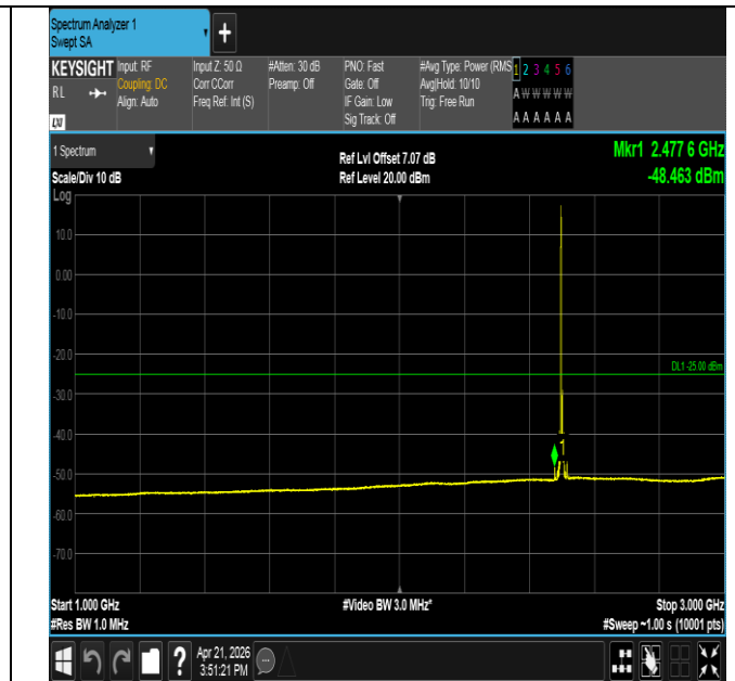
Band41-10MHz-QPSK-39700-1RB#0-1000~3000-PASS
