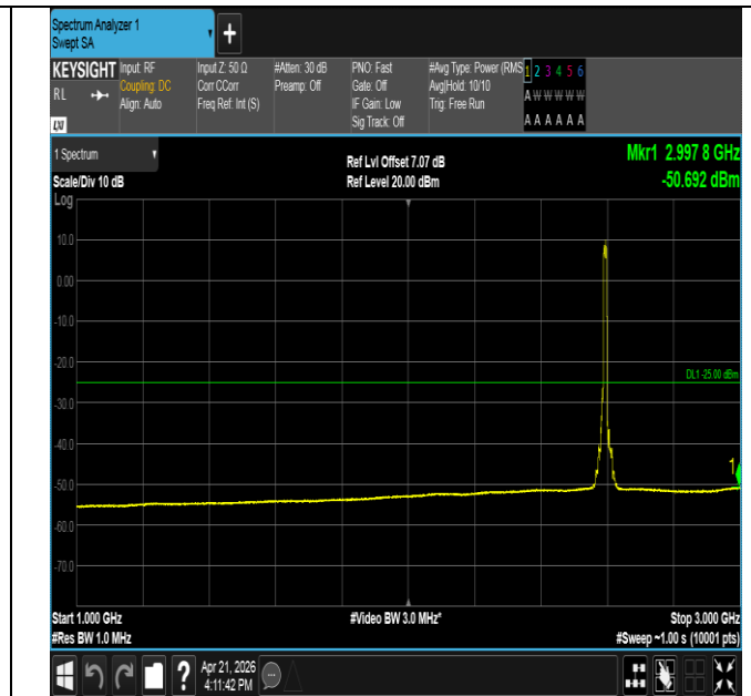
Band41-10MHz-QPSK-40620-50RB#0-1000~3000-PASS
