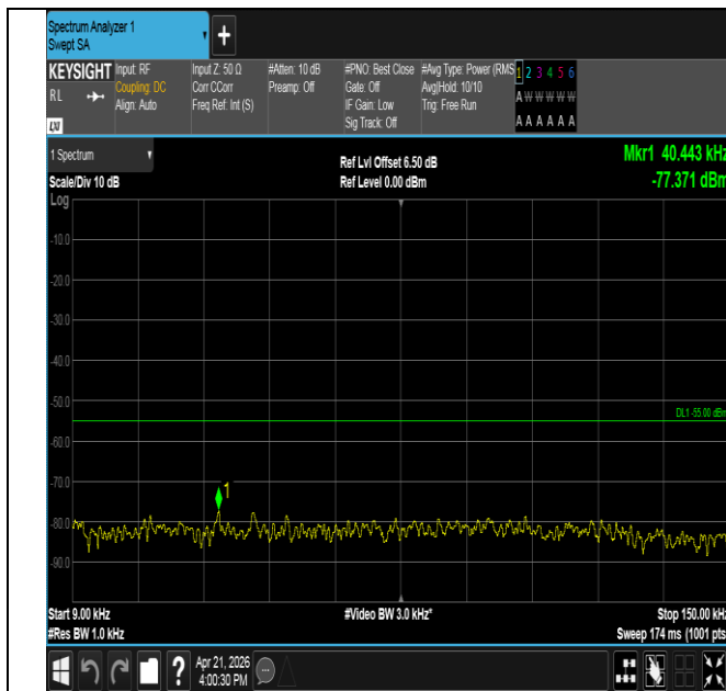
Band41-10MHz-16QAM-39700-50RB#0-0.009~0.15-PASS
