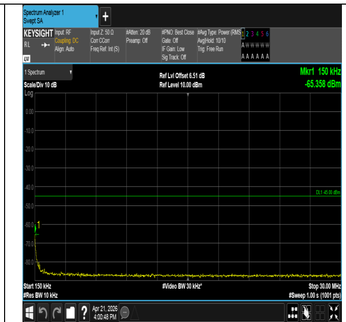
Band41-10MHz-16QAM-39700-50RB#0-0.15~30-PASS
