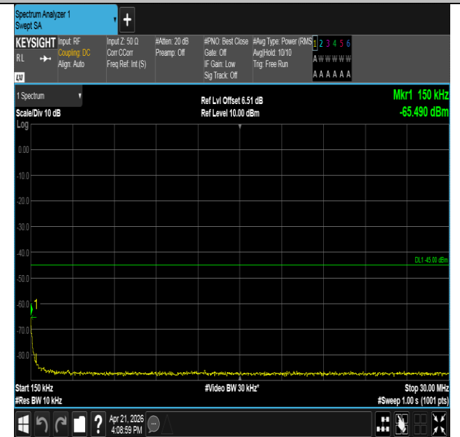
Band41-10MHz-16QAM-40620-1RB#49-0.15~30-PASS
