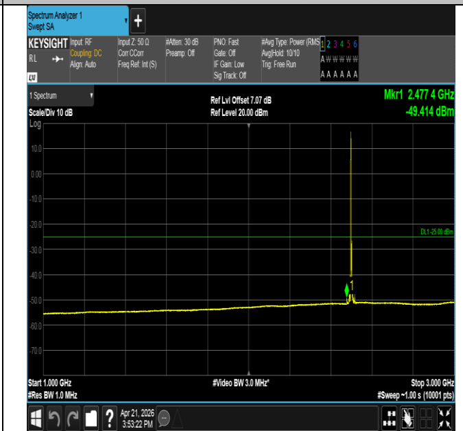
Band41-10MHz-16QAM-39700-1RB#0-1000~3000-PASS
