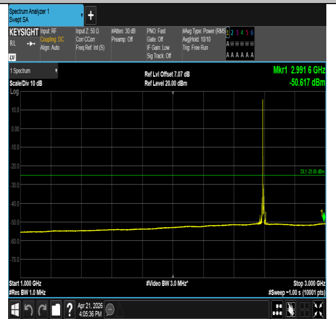
Band41-10MHz-16QAM-40620-1RB#0-1000~3000-PASS
