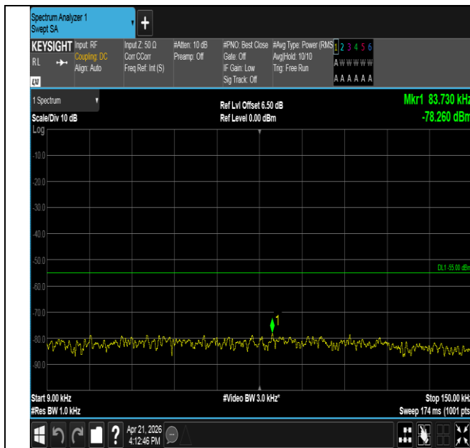
Band41-10MHz-16QAM-40620-50RB#0-0.009~0.15-PASS
