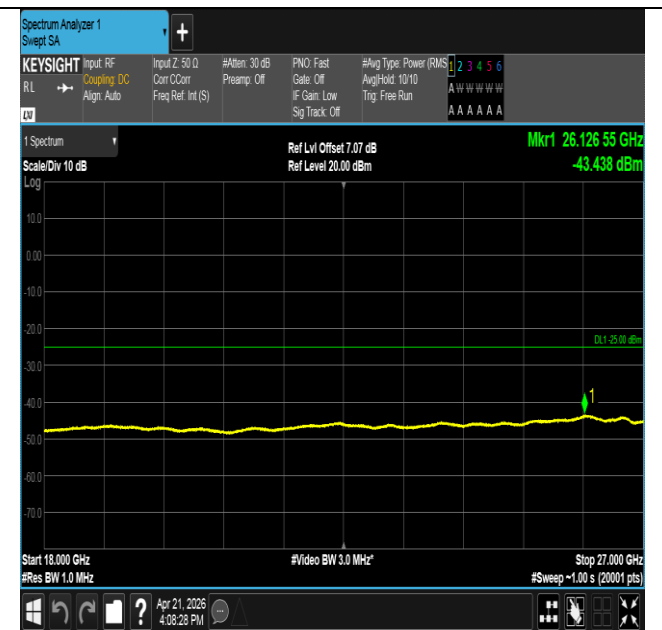
Band41-10MHz-QPSK-40620-1RB#49-18000~27000-PASS
