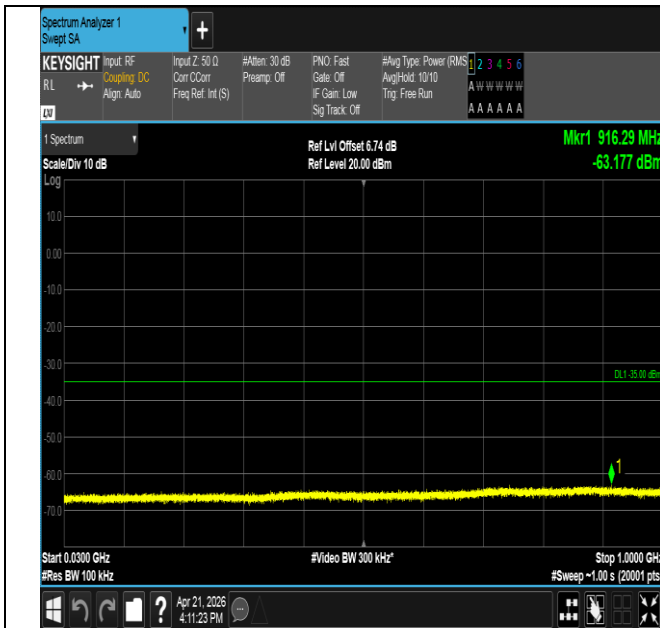
Band41-10MHz-QPSK-40620-50RB#0-30~1000-PASS
