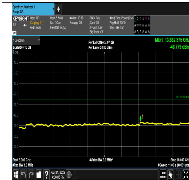
Band41-10MHz-QPSK-40620-1RB#49-3000~18000-PASS
