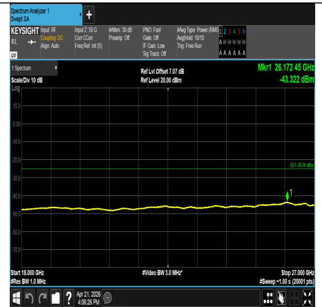
Band41-10MHz-16QAM-40620-1RB#0-18000~27000-PASS
