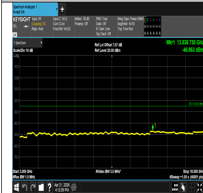
Band41-10MHz-QPSK-40620-50RB#0-3000~18000-PASS
