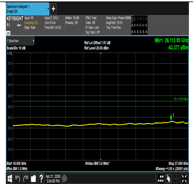
Band41-5MHz-16QAM-41565-25RB#0-18000~27000-PASS
