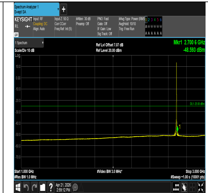
Band41-5MHz-16QAM-41565-1RB#24-1000~3000-PASS
