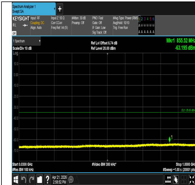
Band41-5MHz-16QAM-41565-1RB#24-30~1000-PASS
