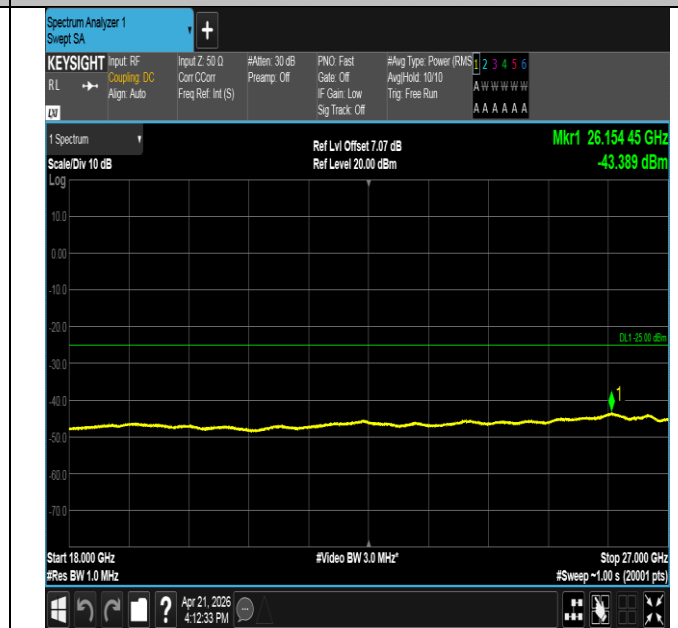
Band41-10MHz-QPSK-40620-50RB#0-18000~27000-PASS
