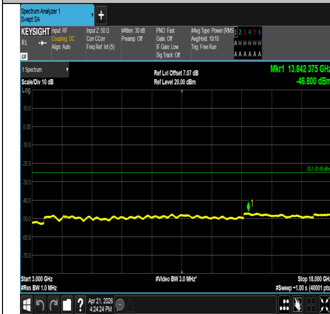
Band41-10MHz-QPSK-41540-50RB#0-3000~18000-PASS
