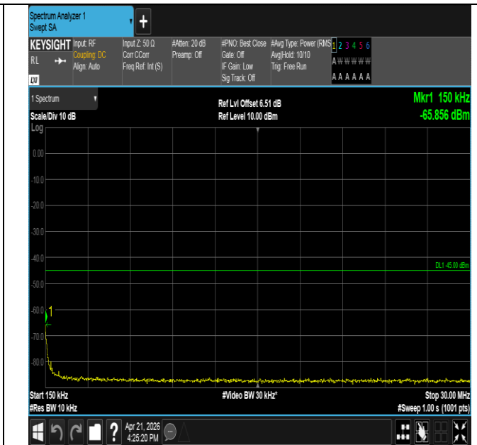
Band41-10MHz-16QAM-41540-50RB#0-0.15~30-PASS
