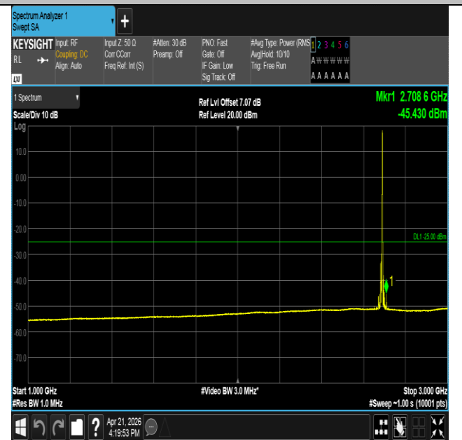
Band41-10MHz-QPSK-41540-1RB#49-1000~3000-PASS
