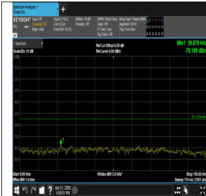
Band41-10MHz-16QAM-41540-50RB#0-0.009~0.15-PASS
