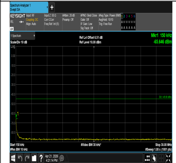
Band41-10MHz-16QAM-41540-1RB#49-0.15~30-PASS
