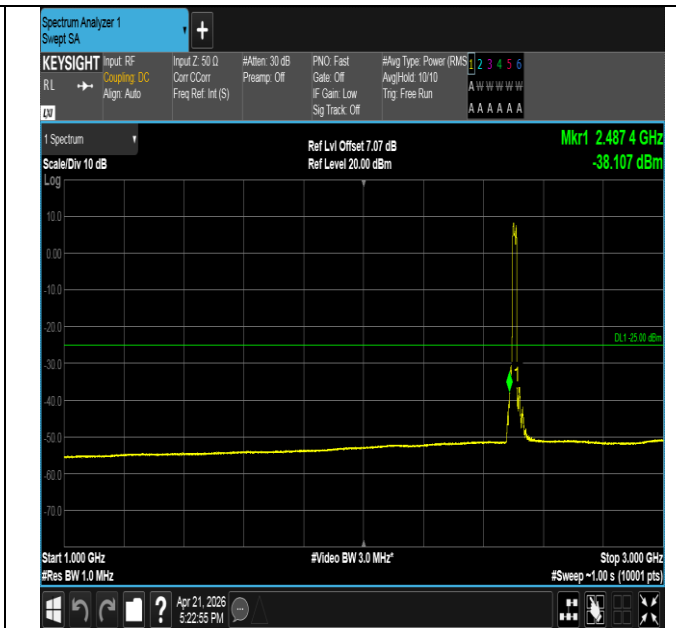
Band41-15MHz-QPSK-39725-75RB#0-1000~3000-PASS
