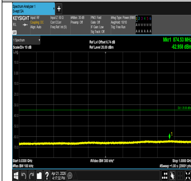
Band41-10MHz-16QAM-41540-1RB#0-30~1000-PASS
