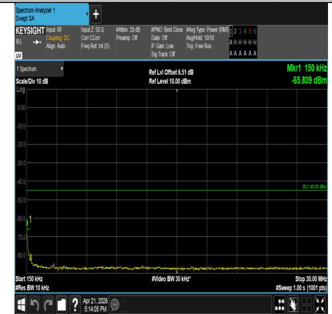
Band41-15MHz-QPSK-39725-1RB#0-0.15~30-PASS
