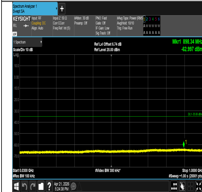
Band41-15MHz-16QAM-39725-75RB#0-30~1000-PASS
