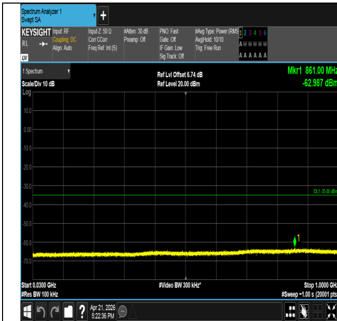
Band41-15MHz-QPSK-39725-75RB#0-30~1000-PASS
