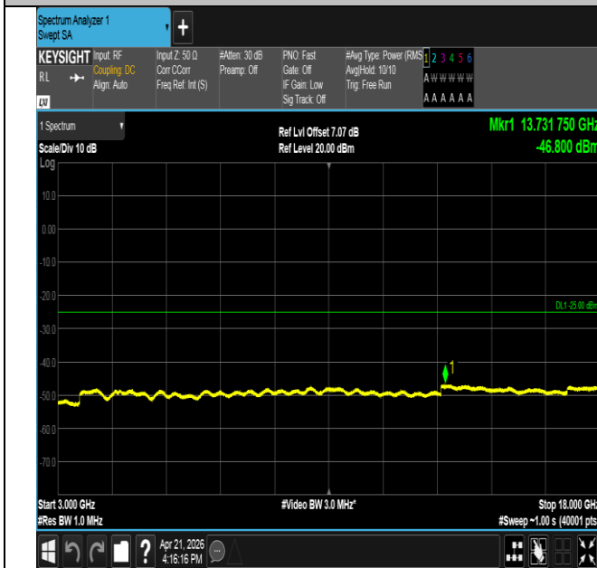
Band41-10MHz-QPSK-41540-1RB#0-3000~18000-PASS
