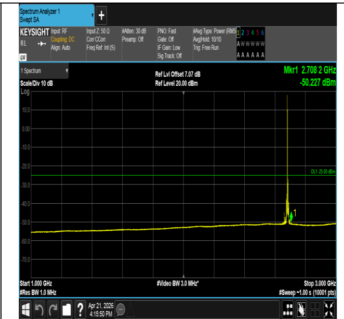
Band41-10MHz-QPSK-41540-1RB#0-1000~3000-PASS
