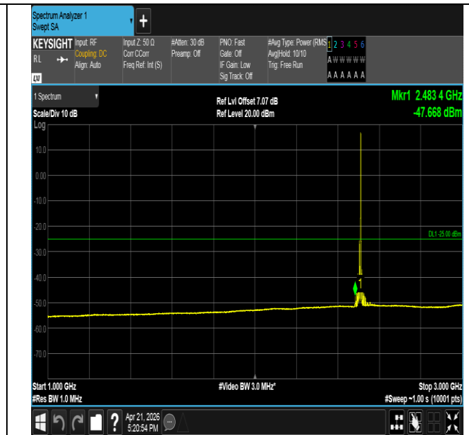
Band41-15MHz-16QAM-39725-1RB#74-1000~3000-PASS
