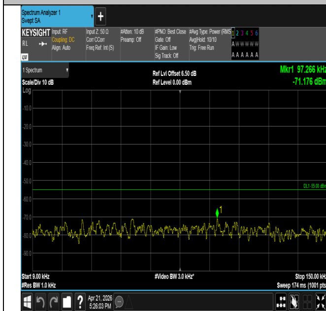
Band41-15MHz-QPSK-40620-1RB#0-0.009~0.15-PASS
