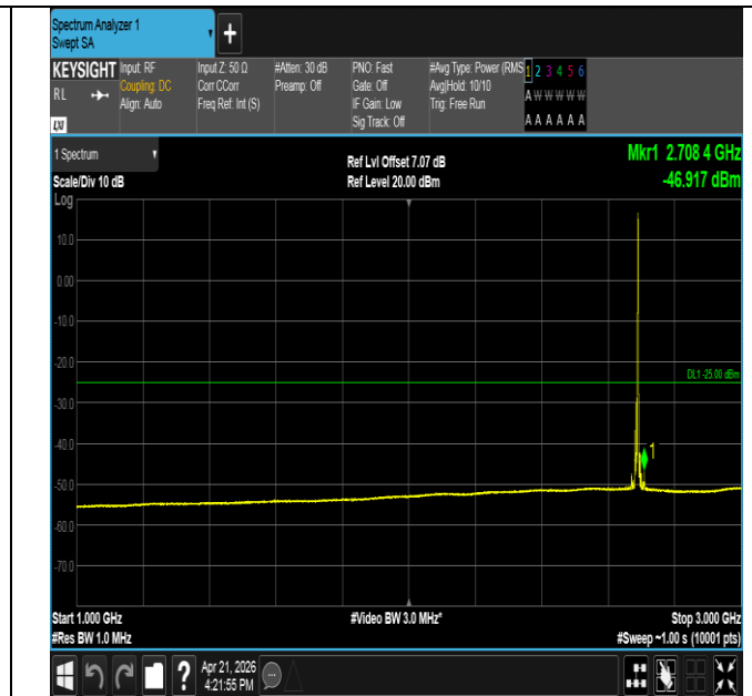
Band41-10MHz-16QAM-41540-1RB#49-1000~3000-PASS
