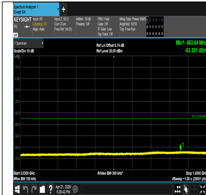
Band41-15MHz-QPSK-40620-1RB#0-30~1000-PASS
