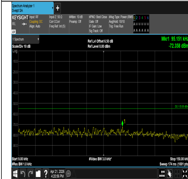
Band41-10MHz-16QAM-41540-1RB#49-0.009~0.15-PASS
