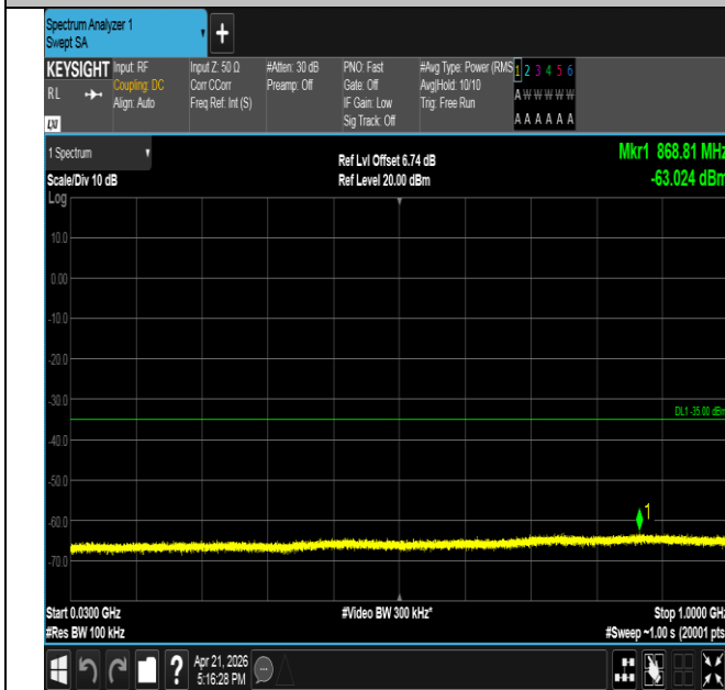
Band41-15MHz-16QAM-39725-1RB#0-30~1000-PASS
