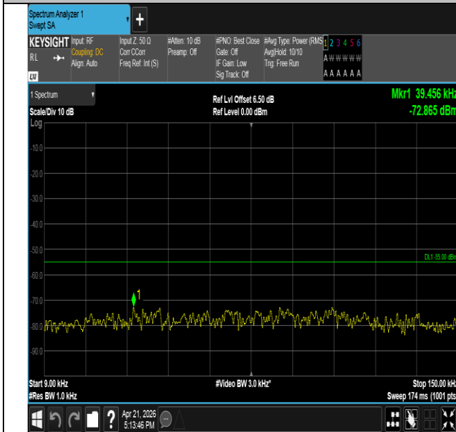
Band41-15MHz-QPSK-39725-1RB#0-0.009~0.15-PASS
