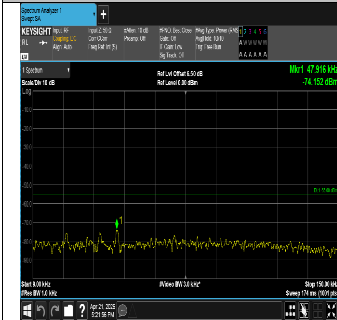
Band41-15MHz-QPSK-39725-75RB#0-0.009~0.15-PASS
