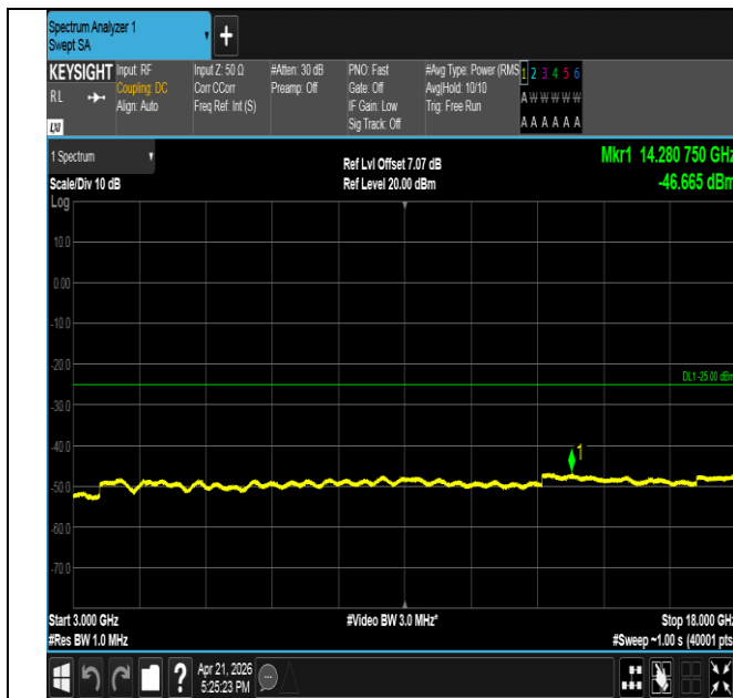
Band41-15MHz-16QAM-39725-75RB#0-3000~18000-PASS
