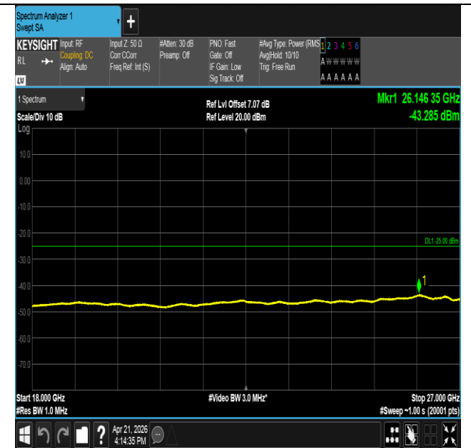
Band41-10MHz-16QAM-40620-50RB#0-18000~27000-PASS
