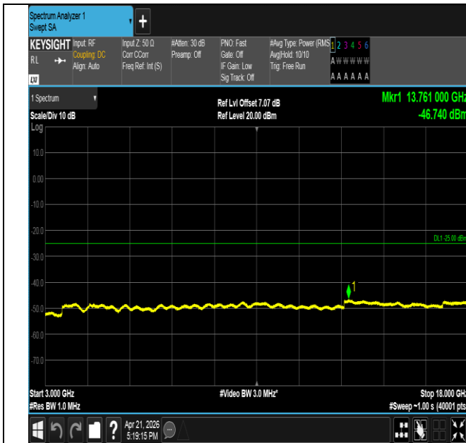
Band41-15MHz-QPSK-39725-1RB#74-3000~18000-PASS
