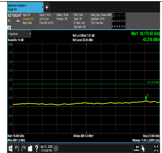
Band41-15MHz-QPSK-39725-1RB#74-18000~27000-PASS
