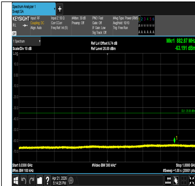
Band41-15MHz-QPSK-39725-1RB#0-30~1000-PASS
