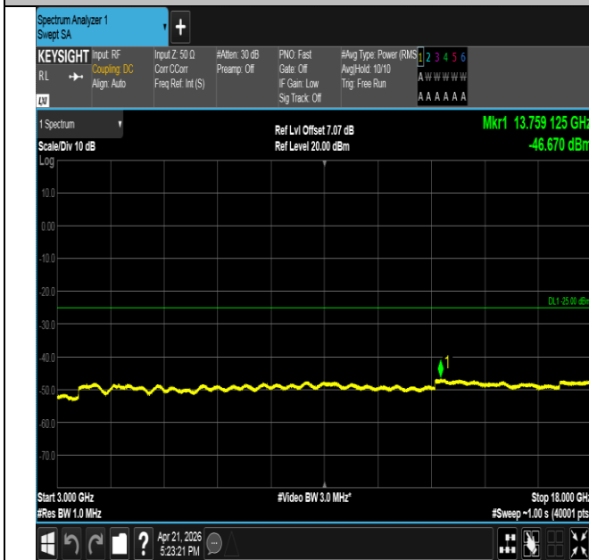
Band41-15MHz-QPSK-39725-75RB#0-3000~18000-PASS
