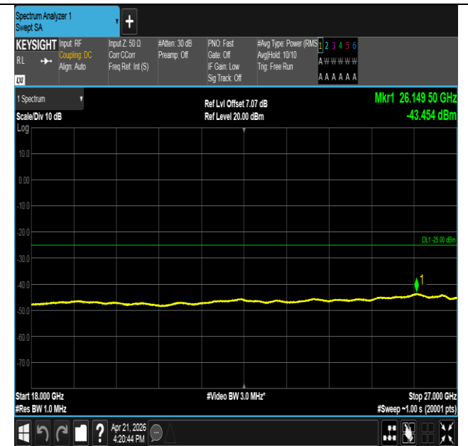
Band41-10MHz-QPSK-41540-1RB#49-18000~27000-PASS
