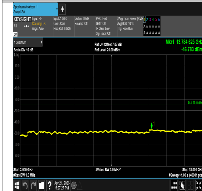
Band41-15MHz-QPSK-40620-1RB#0-3000~18000-PASS
