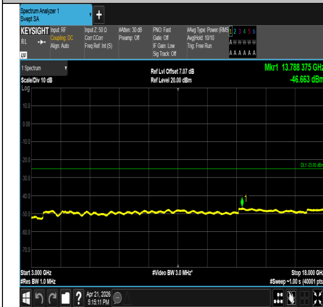
Band41-15MHz-QPSK-39725-1RB#0-3000~18000-PASS
