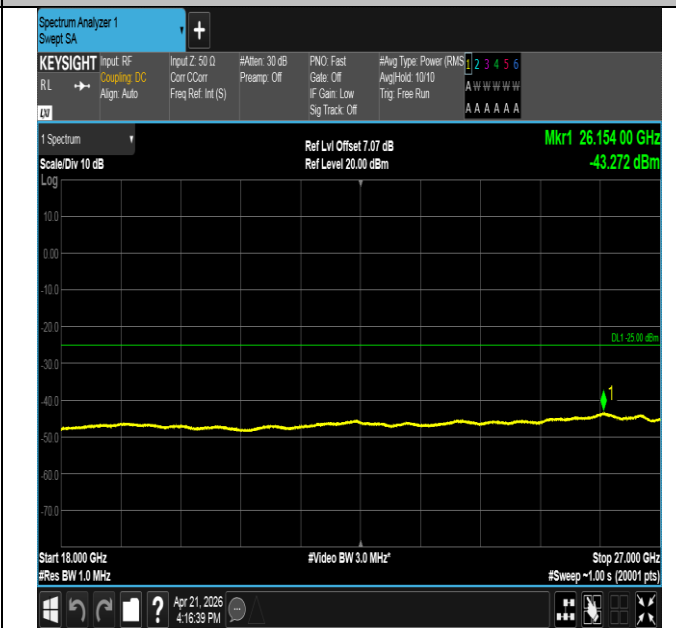
Band41-10MHz-QPSK-41540-1RB#0-18000~27000-PASS
