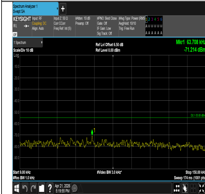
Band41-15MHz-16QAM-39725-1RB#74-0.009~0.15-PASS
