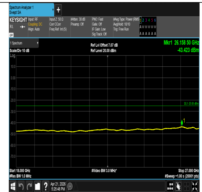
Band41-15MHz-16QAM-39725-75RB#0-18000~27000-PASS
