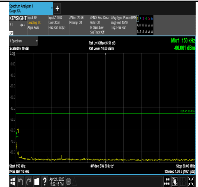
Band41-15MHz-QPSK-39725-75RB#0-0.15~30-PASS
