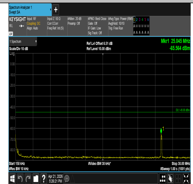
Band41-15MHz-QPSK-40620-1RB#0-0.15~30-PASS
