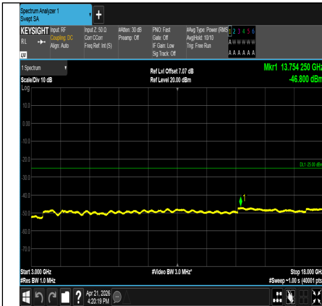
Band41-10MHz-QPSK-41540-1RB#49-3000~18000-PASS
