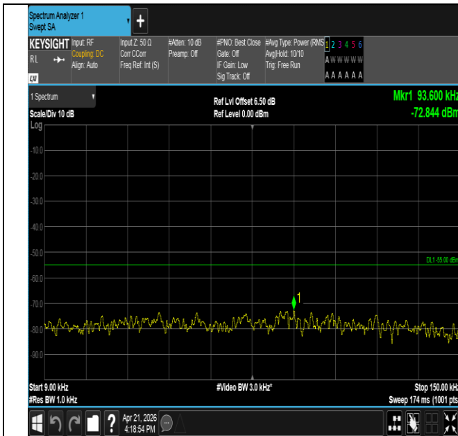
Band41-10MHz-QPSK-41540-1RB#49-0.009~0.15-PASS
