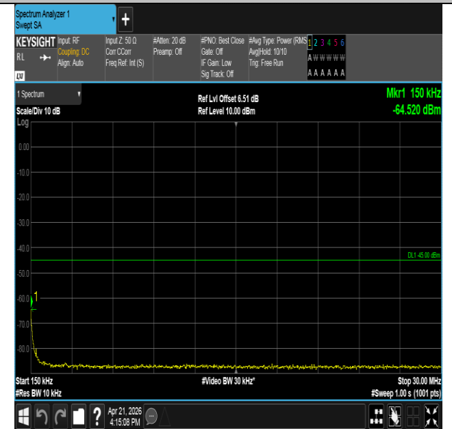
Band41-10MHz-QPSK-41540-1RB#0-0.15~30-PASS
