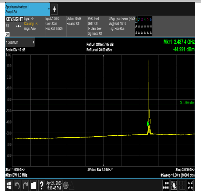
Band41-15MHz-16QAM-39725-1RB#0-1000~3000-PASS
