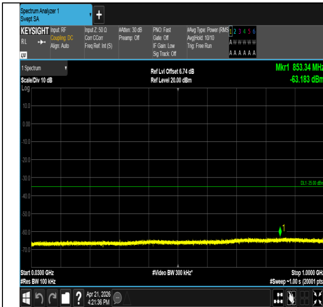
Band41-10MHz-16QAM-41540-1RB#49-30~1000-PASS
