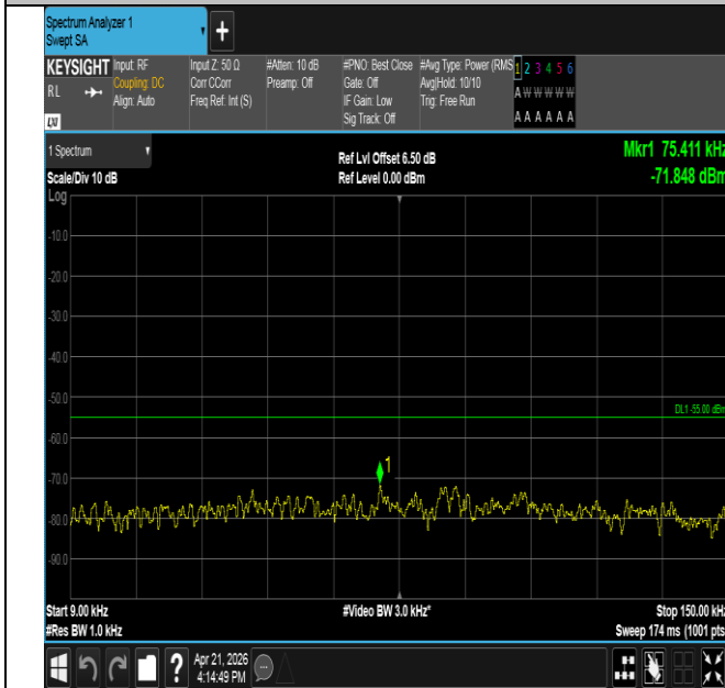
Band41-10MHz-QPSK-41540-1RB#0-0.009~0.15-PASS
