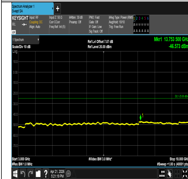
Band41-15MHz-16QAM-39725-1RB#74-3000~18000-PASS
