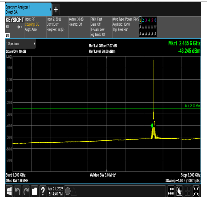
Band41-15MHz-QPSK-39725-1RB#0-1000~3000-PASS
