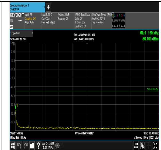
Band41-15MHz-16QAM-39725-75RB#0-0.15~30-PASS
