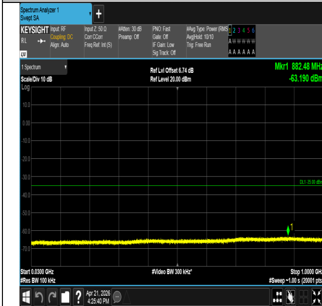
Band41-10MHz-16QAM-41540-50RB#0-30~1000-PASS
