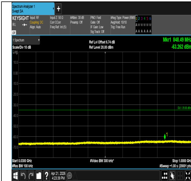
Band41-10MHz-QPSK-41540-50RB#0-30~1000-PASS
