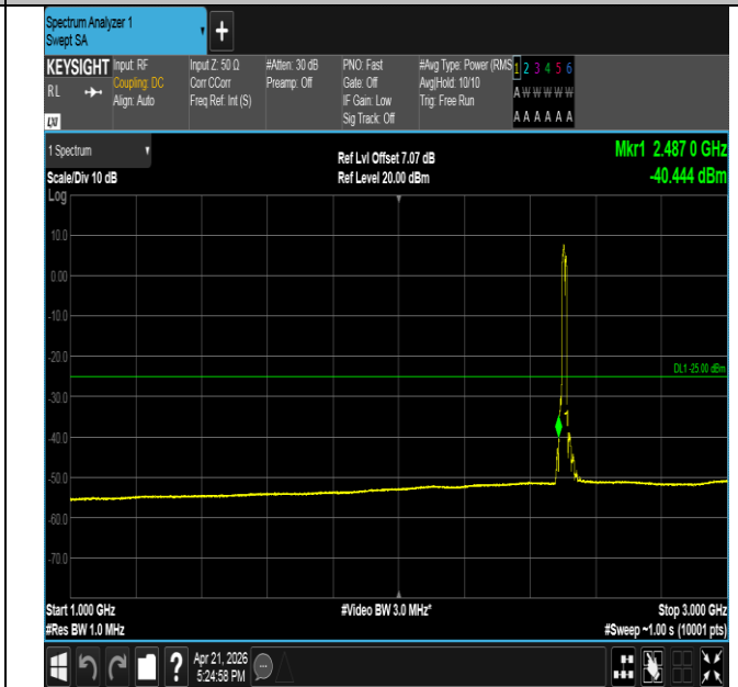
Band41-15MHz-16QAM-39725-75RB#0-1000~3000-PASS
