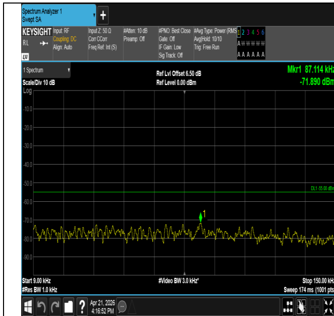
Band41-10MHz-16QAM-41540-1RB#0-0.009~0.15-PASS
