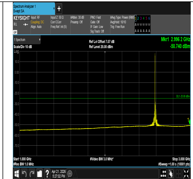
Band41-15MHz-QPSK-40620-1RB#0-1000~3000-PASS
