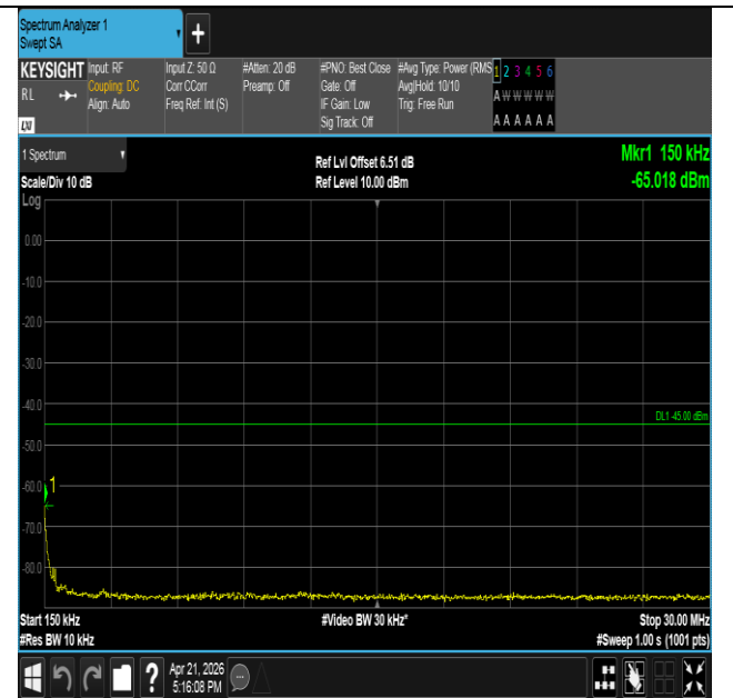
Band41-15MHz-16QAM-39725-1RB#0-0.15~30-PASS
