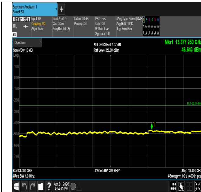
Band41-10MHz-16QAM-40620-50RB#0-3000~18000-PASS
