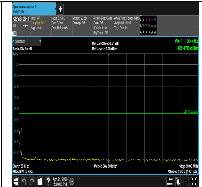
Band41-15MHz-QPSK-39725-1RB#74-0.15~30-PASS
