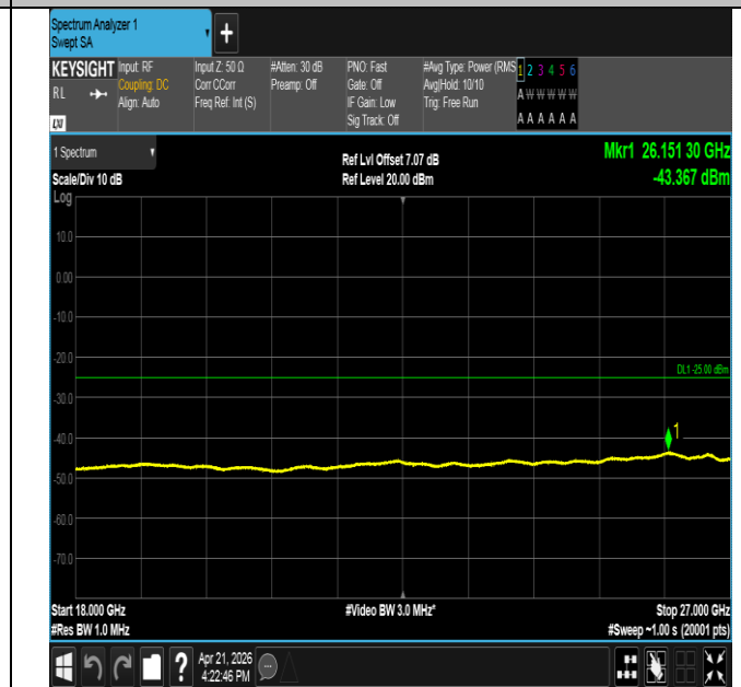
Band41-10MHz-16QAM-41540-1RB#49-18000~27000-PASS
