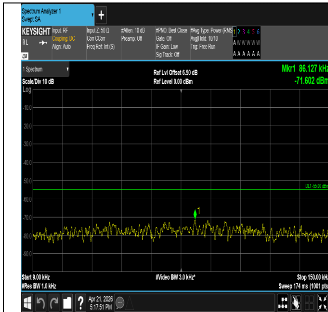
Band41-15MHz-QPSK-39725-1RB#74-0.009~0.15-PASS
