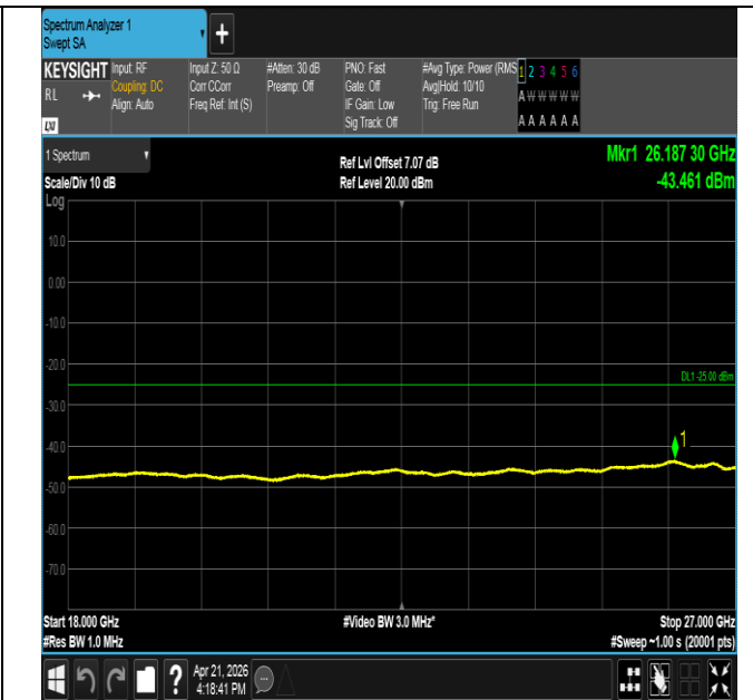
Band41-10MHz-16QAM-41540-1RB#0-18000~27000-PASS
