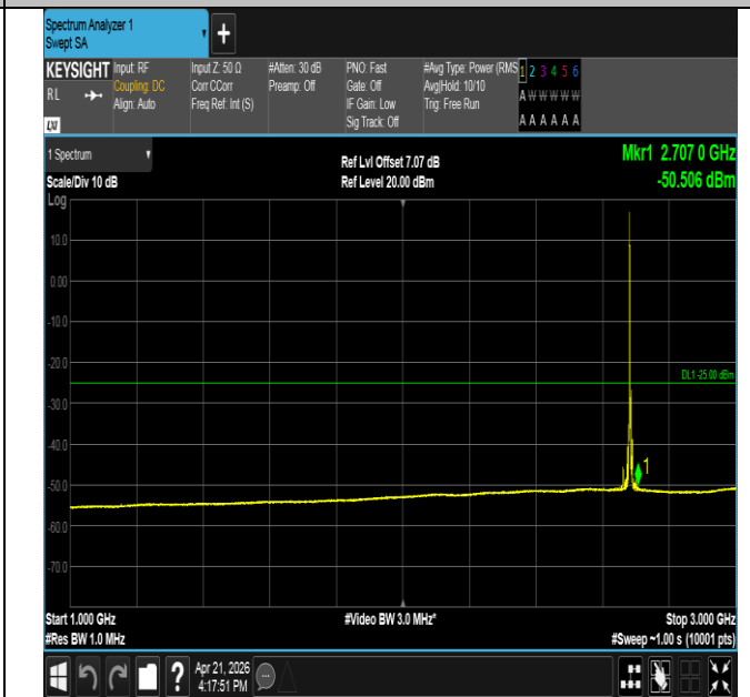
Band41-10MHz-16QAM-41540-1RB#0-1000~3000-PASS
