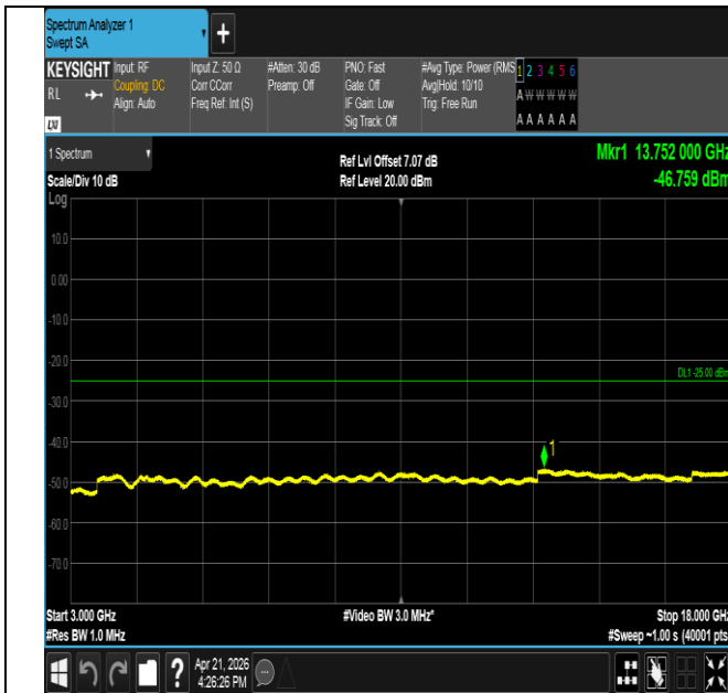
Band41-10MHz-16QAM-41540-50RB#0-3000~18000-PASS
