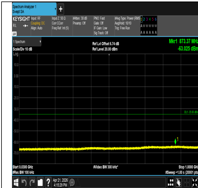
Band41-10MHz-QPSK-41540-1RB#0-30~1000-PASS
