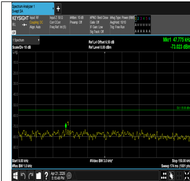
Band41-15MHz-16QAM-39725-1RB#0-0.009~0.15-PASS
