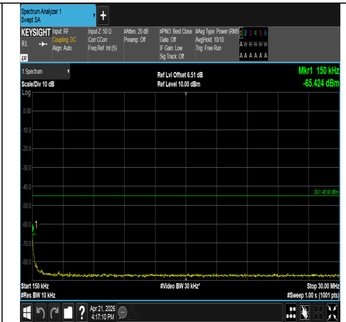
Band41-10MHz-16QAM-41540-1RB#0-0.15~30-PASS
