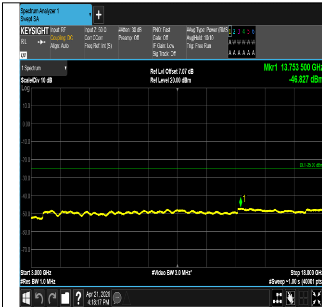
Band41-10MHz-16QAM-41540-1RB#0-3000~18000-PASS
