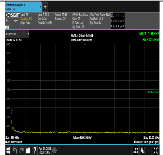
Band41-15MHz-16QAM-39725-1RB#74-0.15~30-PASS
