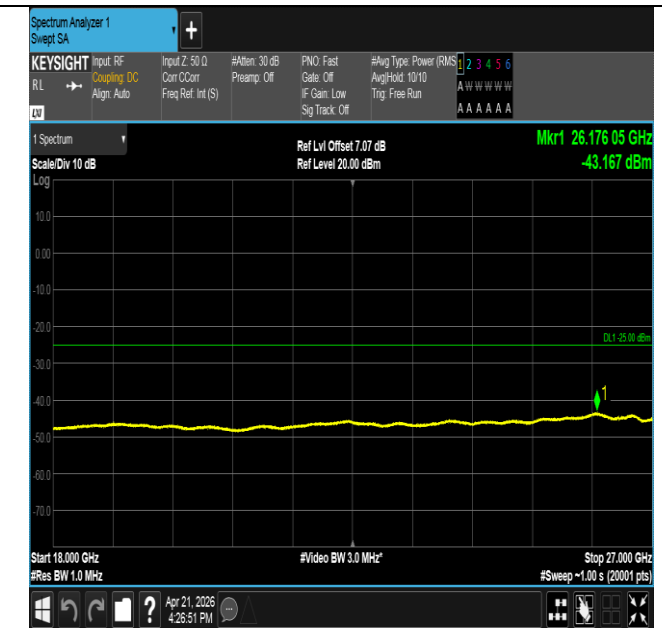
Band41-10MHz-16QAM-41540-50RB#0-18000~27000-PASS
