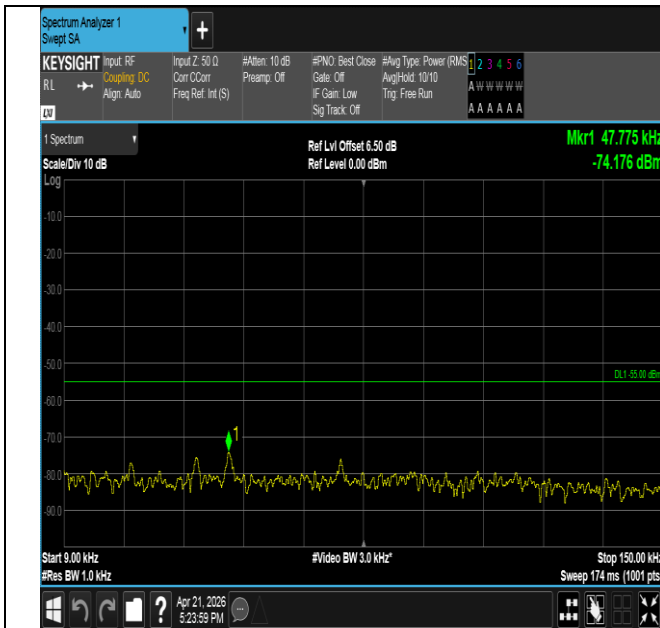
Band41-15MHz-16QAM-39725-75RB#0-0.009~0.15-PASS
