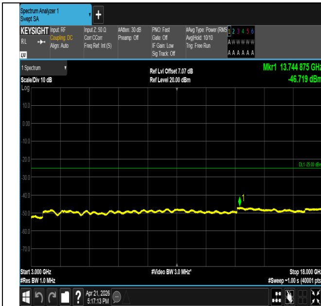
Band41-15MHz-16QAM-39725-1RB#0-3000~18000-PASS
