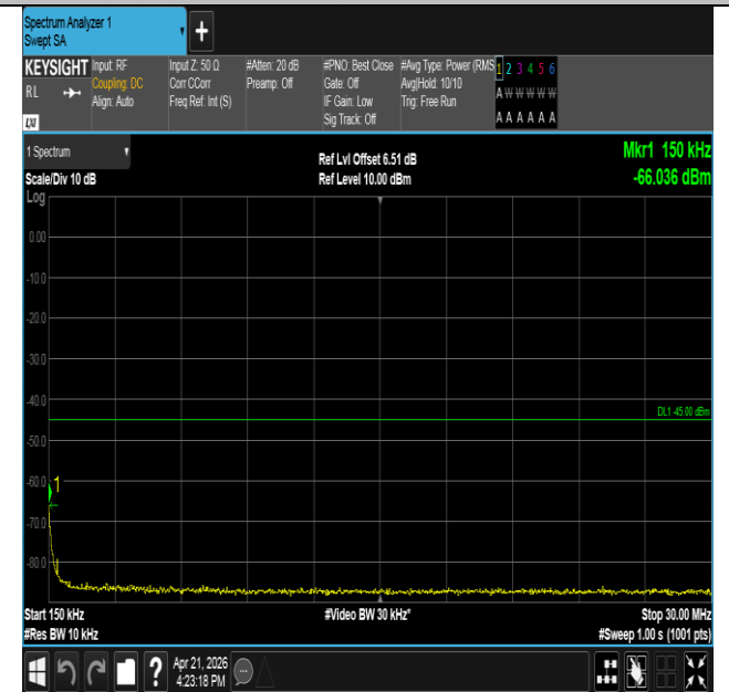
Band41-10MHz-QPSK-41540-50RB#0-0.15~30-PASS
