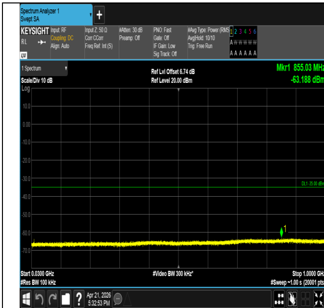
Band41-15MHz-16QAM-40620-1RB#74-30~1000-PASS
