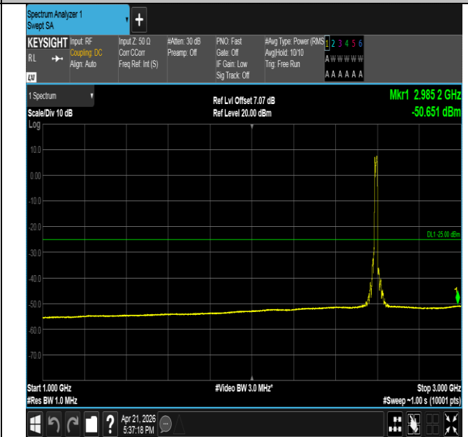
Band41-15MHz-16QAM-40620-75RB#0-1000~3000-PASS
