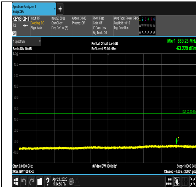
Band41-15MHz-QPSK-40620-75RB#0-30~1000-PASS
