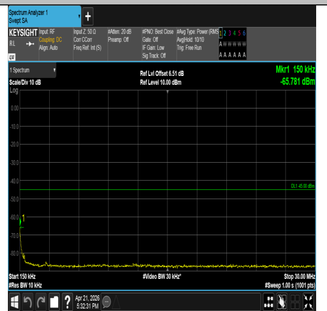
Band41-15MHz-16QAM-40620-1RB#74-0.15~30-PASS
