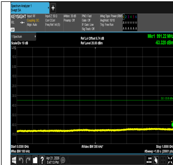
Band41-15MHz-QPSK-41515-75RB#0-30~1000-PASS
