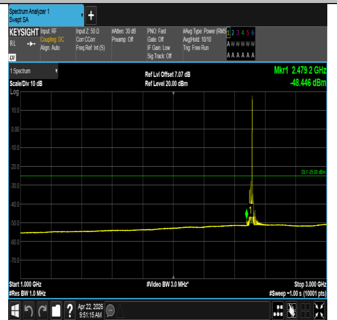
Band41-20MHz-QPSK-39750-1RB#99-1000~3000-PASS
