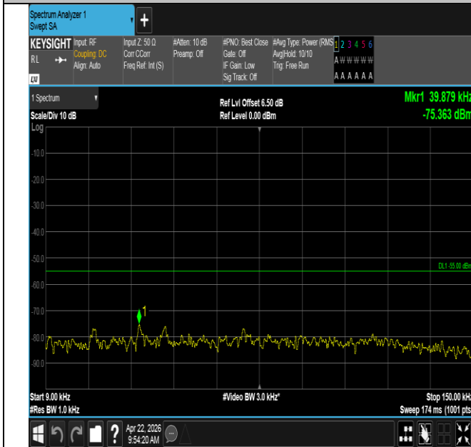
Band41-20MHz-QPSK-39750-100RB#0-0.009~0.15-PASS
