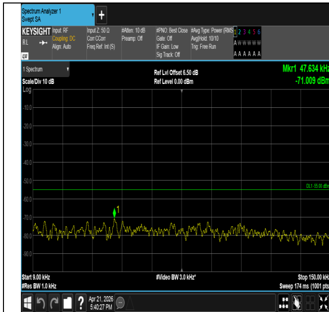
Band41-15MHz-16QAM-41515-1RB#0-0.009~0.15-PASS
