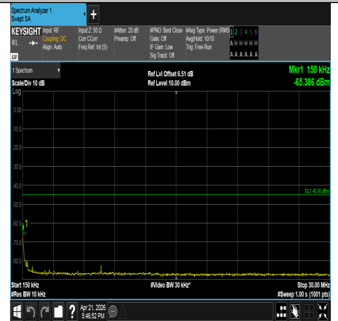
Band41-15MHz-QPSK-41515-75RB#0-0.15~30-PASS
