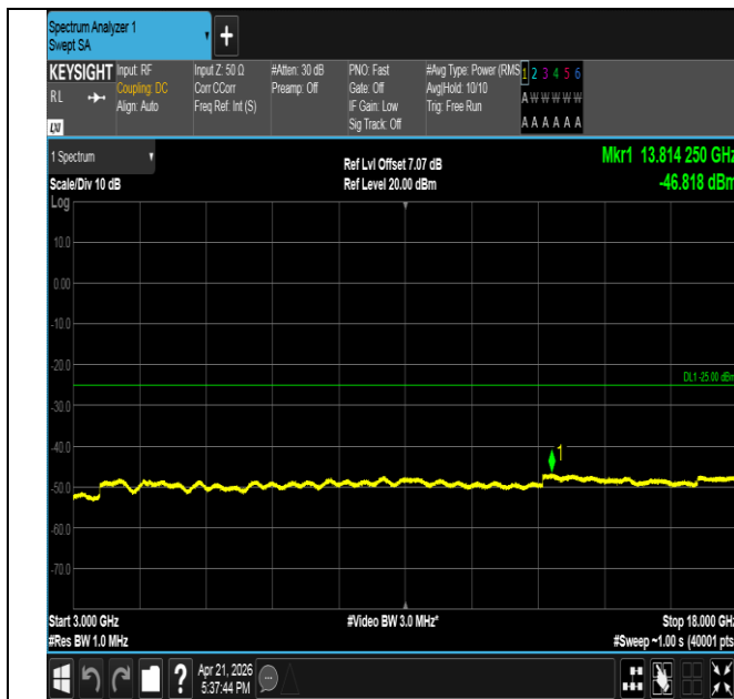
Band41-15MHz-16QAM-40620-75RB#0-3000~18000-PASS
