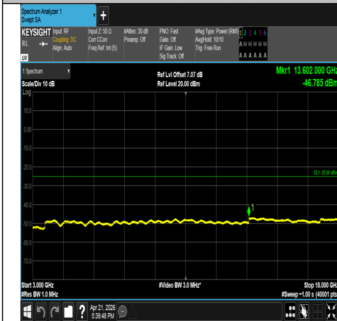
Band41-15MHz-QPSK-41515-1RB#0-3000~18000-PASS
