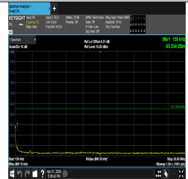
Band41-15MHz-QPSK-41515-1RB#0-0.15~30-PASS
