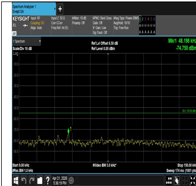
Band41-15MHz-16QAM-40620-75RB#0-0.009~0.15-PASS
