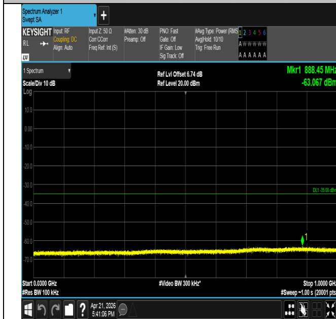
Band41-15MHz-16QAM-41515-1RB#0-30~1000-PASS
