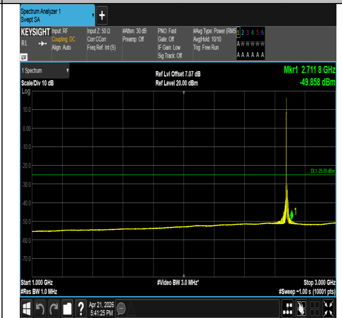
Band41-15MHz-16QAM-41515-1RB#0-1000~3000-PASS
