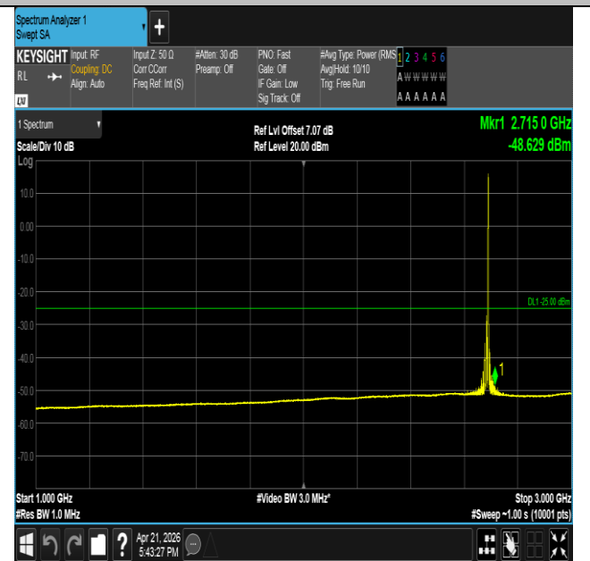
Band41-15MHz-QPSK-41515-1RB#74-1000~3000-PASS
