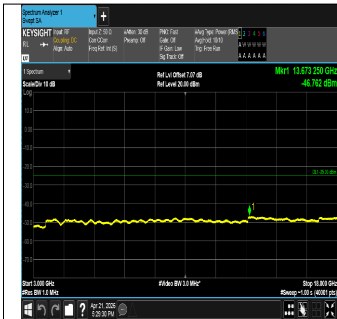
Band41-15MHz-16QAM-40620-1RB#0-3000~18000-PASS
