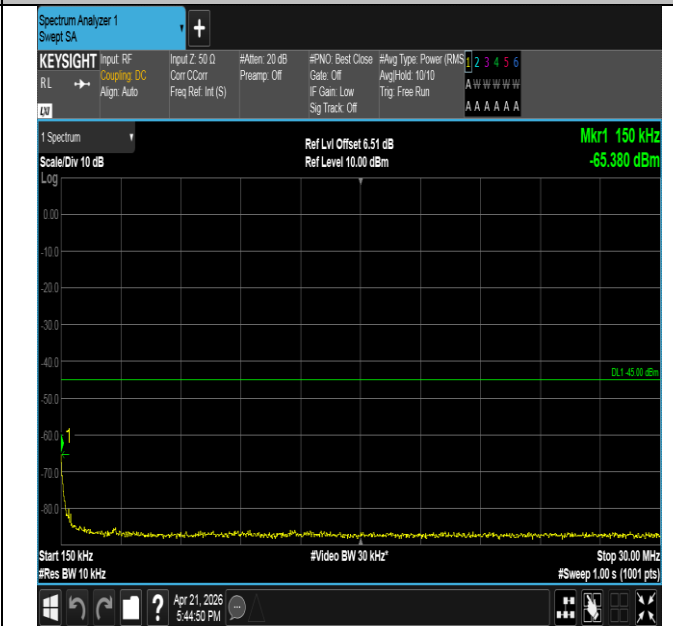
Band41-15MHz-16QAM-41515-1RB#74-0.15~30-PASS
