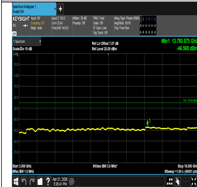
Band41-15MHz-QPSK-40620-75RB#0-3000~18000-PASS
