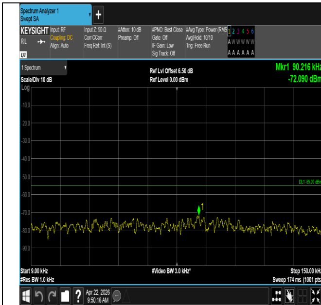
Band41-20MHz-QPSK-39750-1RB#99-0.009~0.15-PASS
