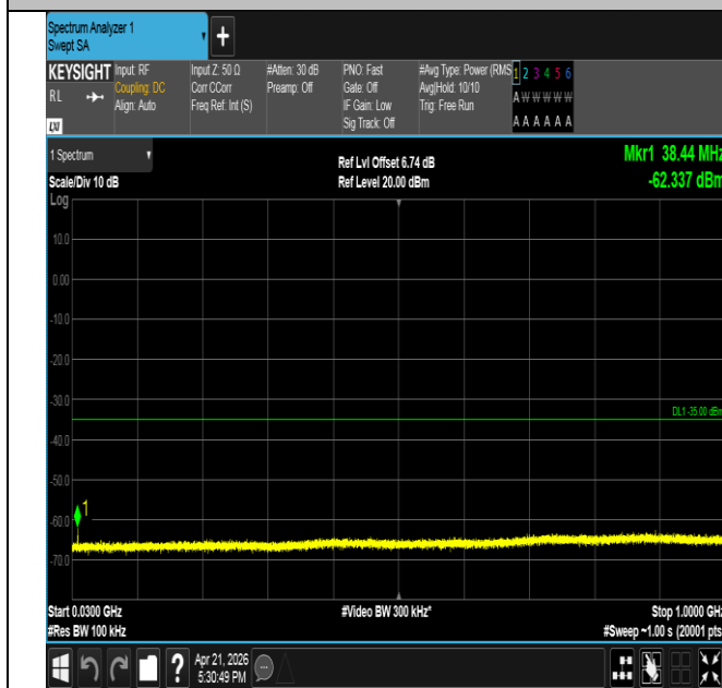
Band41-15MHz-QPSK-40620-1RB#74-30~1000-PASS
