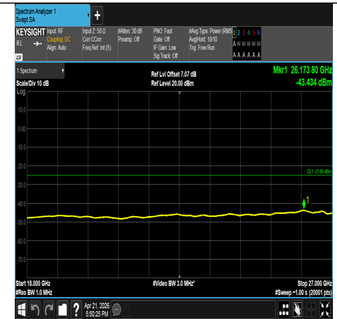
Band41-15MHz-16QAM-41515-75RB#0-18000~27000-PASS
