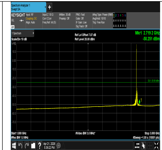
Band41-15MHz-QPSK-41515-1RB#0-1000~3000-PASS
