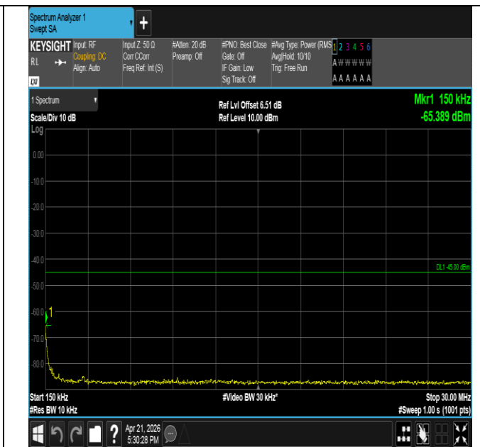
Band41-15MHz-QPSK-40620-1RB#74-0.15~30-PASS
