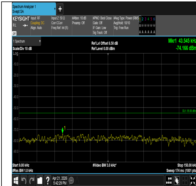
Band41-15MHz-QPSK-41515-1RB#74-0.009~0.15-PASS
