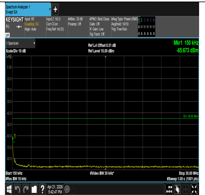
Band41-15MHz-QPSK-41515-1RB#74-0.15~30-PASS
