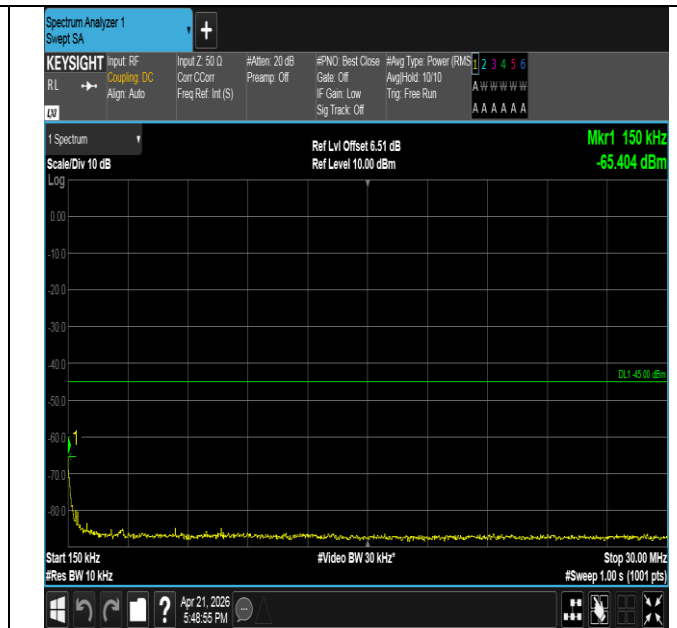
Band41-15MHz-16QAM-41515-75RB#0-0.15~30-PASS
