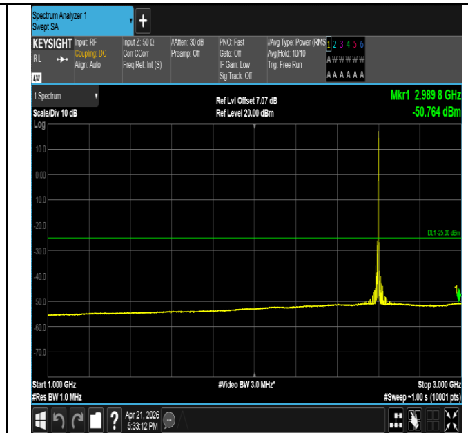
Band41-15MHz-16QAM-40620-1RB#74-1000~3000-PASS
