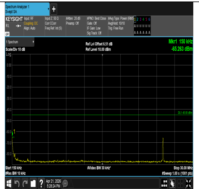
Band41-15MHz-16QAM-40620-1RB#0-0.15~30-PASS
