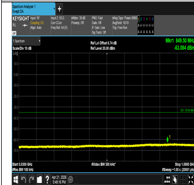
Band41-15MHz-16QAM-41515-75RB#0-30~1000-PASS
