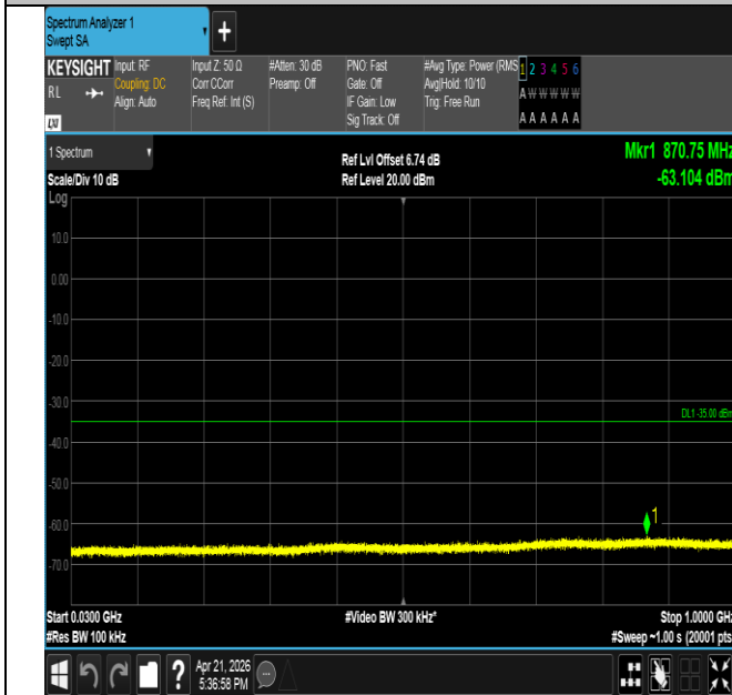
Band41-15MHz-16QAM-40620-75RB#0-30~1000-PASS
