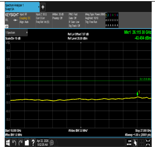
Band41-20MHz-QPSK-39750-1RB#99-18000~27000-PASS
