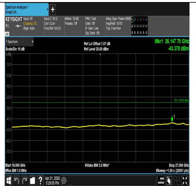
Band41-15MHz-16QAM-40620-1RB#0-18000~27000-PASS
