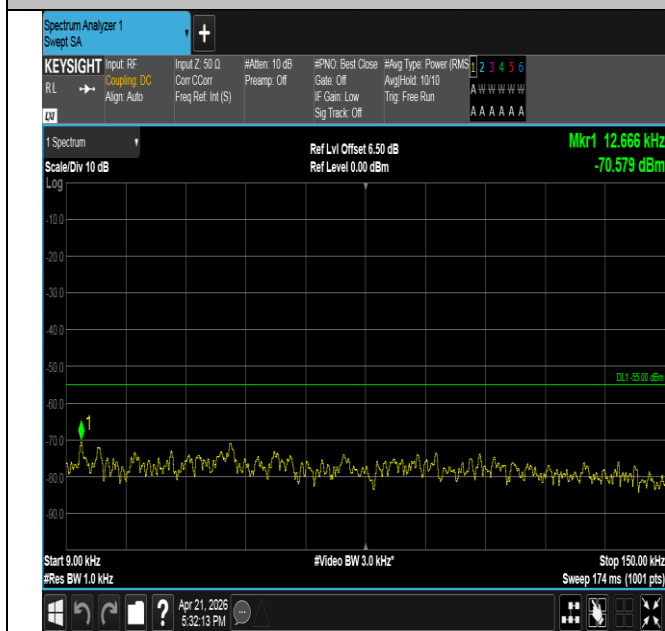
Band41-15MHz-16QAM-40620-1RB#74-0.009~0.15-PASS
