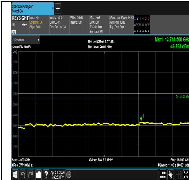
Band41-15MHz-QPSK-41515-1RB#74-3000~18000-PASS
