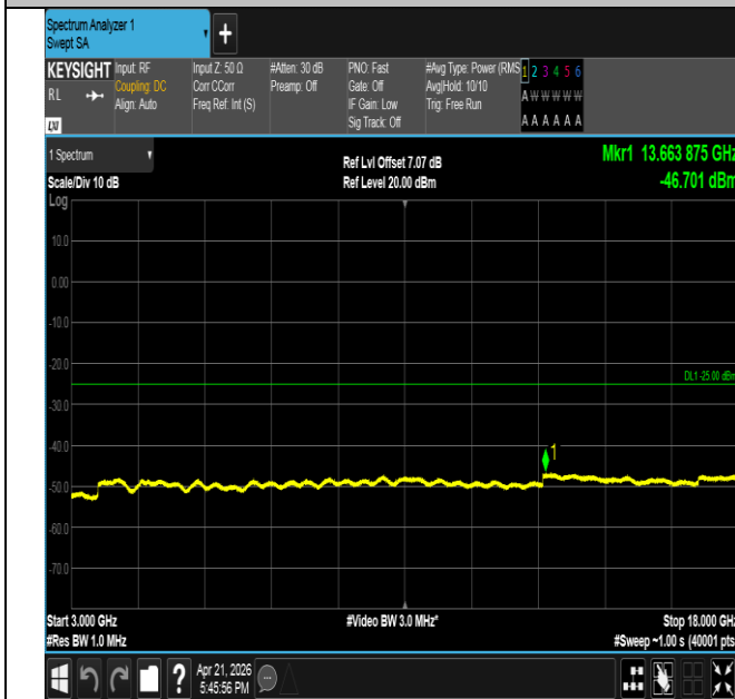
Band41-15MHz-16QAM-41515-1RB#74-3000~18000-PASS
