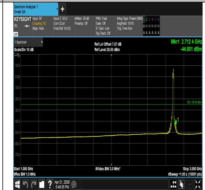
Band41-15MHz-16QAM-41515-75RB#0-1000~3000-PASS
