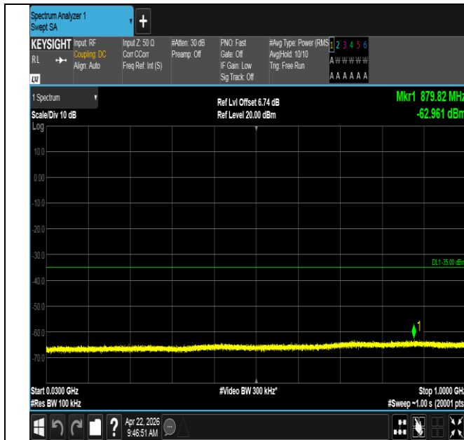
Band41-20MHz-QPSK-39750-1RB#0-30~1000-PASS
