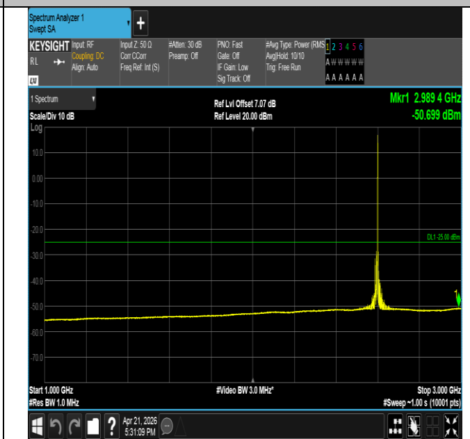
Band41-15MHz-QPSK-40620-1RB#74-1000~3000-PASS
