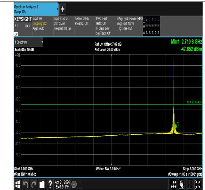
Band41-15MHz-16QAM-41515-1RB#74-1000~3000-PASS
