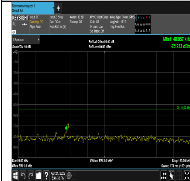
Band41-15MHz-QPSK-41515-75RB#0-0.009~0.15-PASS
