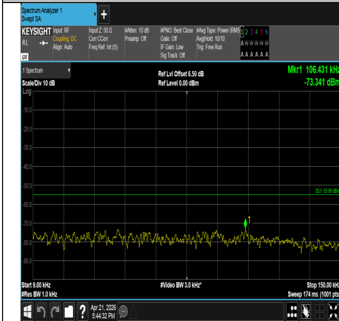
Band41-15MHz-16QAM-41515-1RB#74-0.009~0.15-PASS
