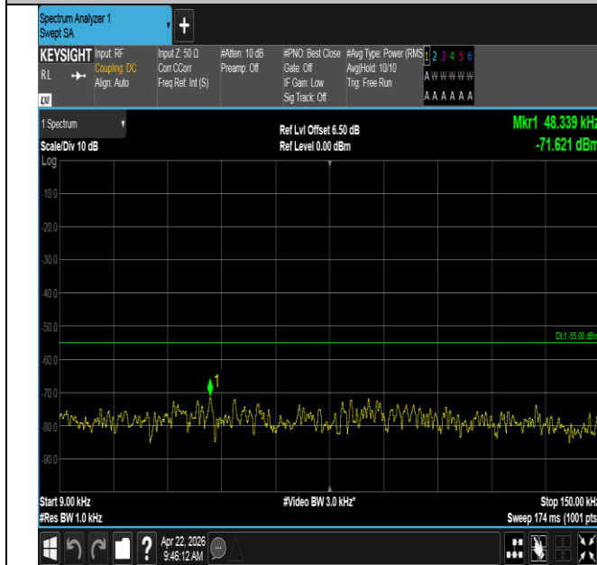
Band41-20MHz-QPSK-39750-1RB#0-0.009~0.15-PASS
