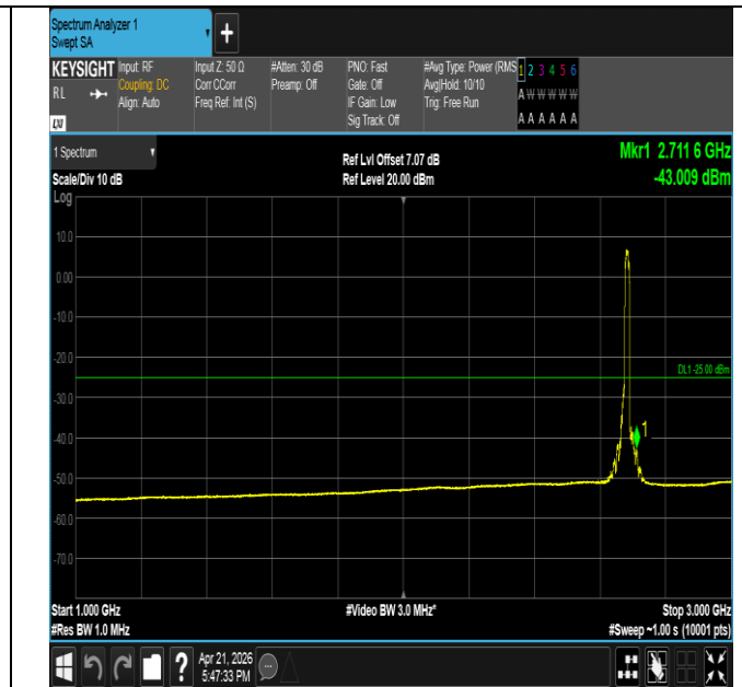
Band41-15MHz-QPSK-41515-75RB#0-1000~3000-PASS
