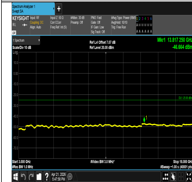
Band41-15MHz-QPSK-41515-75RB#0-3000~18000-PASS
