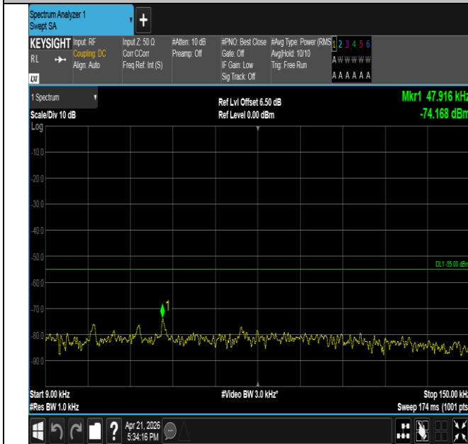
Band41-15MHz-QPSK-40620-75RB#0-0.009~0.15-PASS
