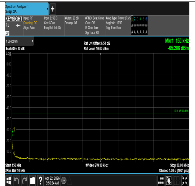
Band41-20MHz-QPSK-39750-1RB#99-0.15~30-PASS
