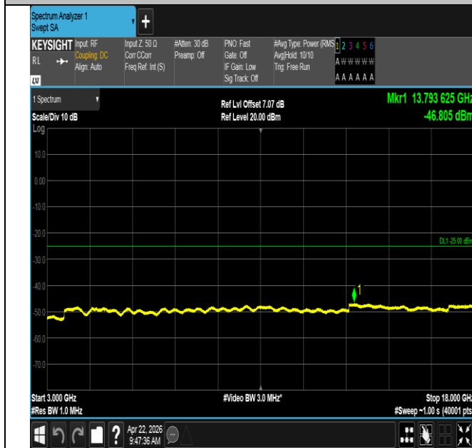
Band41-20MHz-QPSK-39750-1RB#0-3000~18000-PASS
