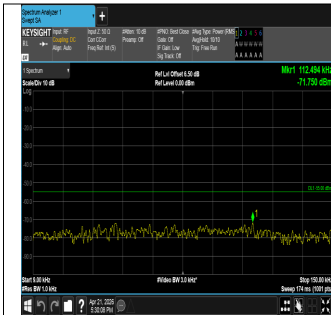
Band41-15MHz-QPSK-40620-1RB#74-0.009~0.15-PASS
