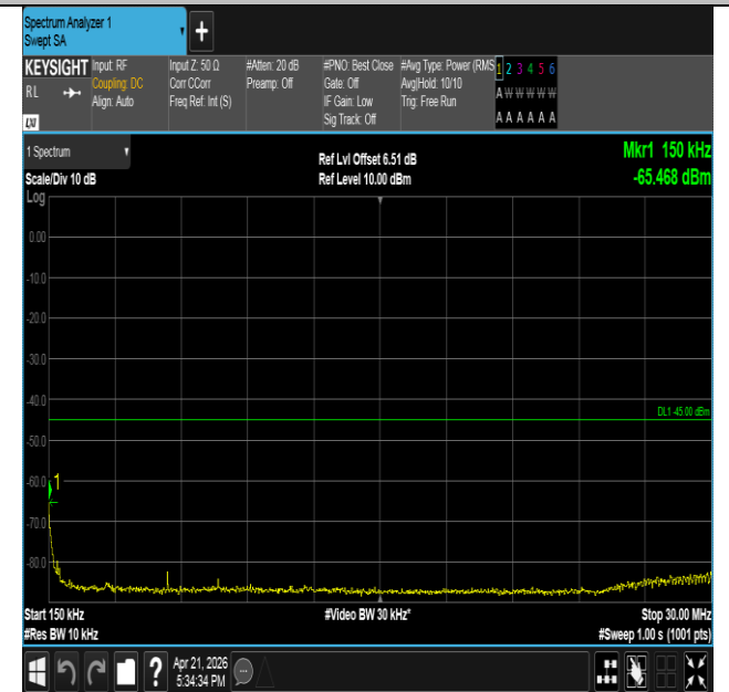
Band41-15MHz-QPSK-40620-75RB#0-0.15~30-PASS
