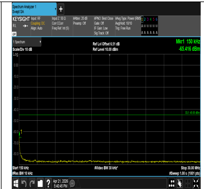
Band41-15MHz-16QAM-41515-1RB#0-0.15~30-PASS
