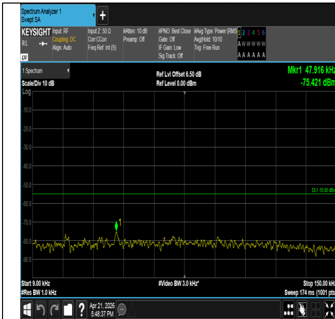
Band41-15MHz-16QAM-41515-75RB#0-0.009~0.15-PASS
