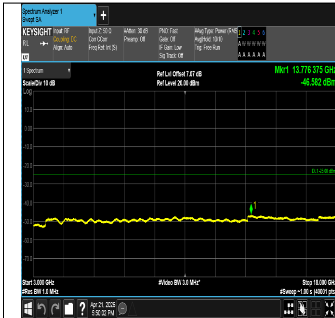
Band41-15MHz-16QAM-41515-75RB#0-3000~18000-PASS
