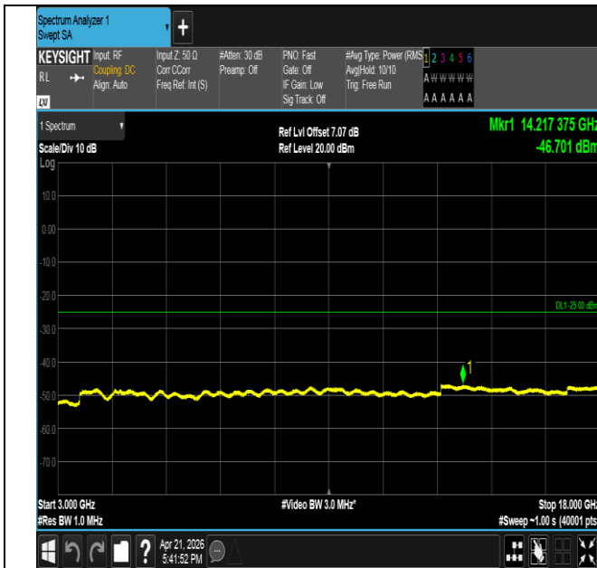
Band41-15MHz-16QAM-41515-1RB#0-3000~18000-PASS
