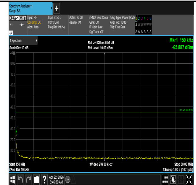
Band41-20MHz-QPSK-39750-1RB#0-0.15~30-PASS
