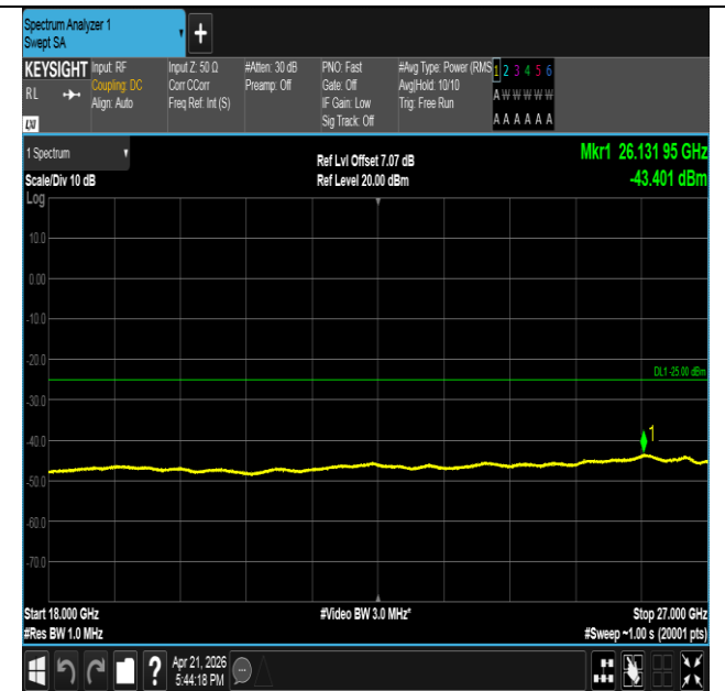
Band41-15MHz-QPSK-41515-1RB#74-18000~27000-PASS
