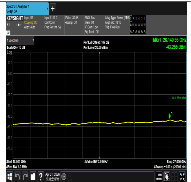
Band41-15MHz-QPSK-40620-1RB#74-18000~27000-PASS
