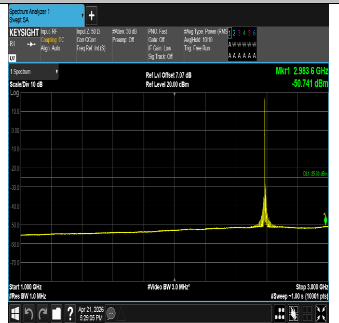
Band41-15MHz-16QAM-40620-1RB#0-1000~3000-PASS
