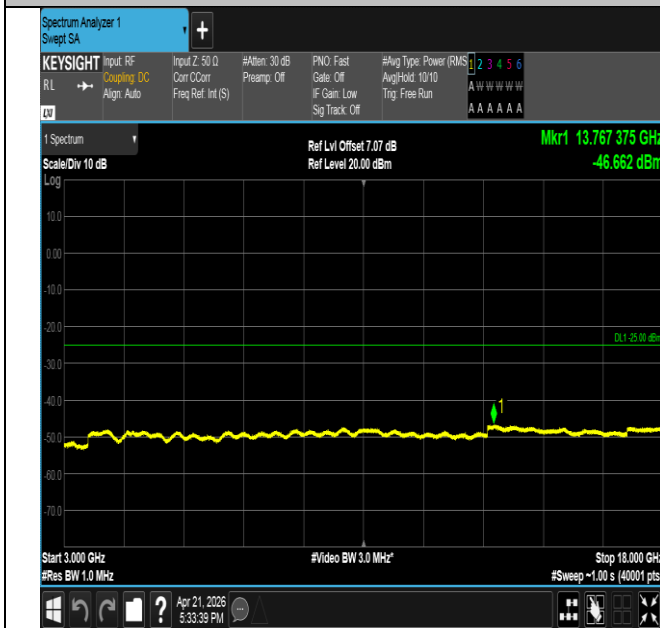
Band41-15MHz-16QAM-40620-1RB#74-3000~18000-PASS
