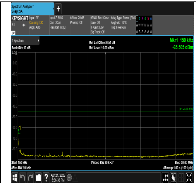
Band41-15MHz-16QAM-40620-75RB#0-0.15~30-PASS
