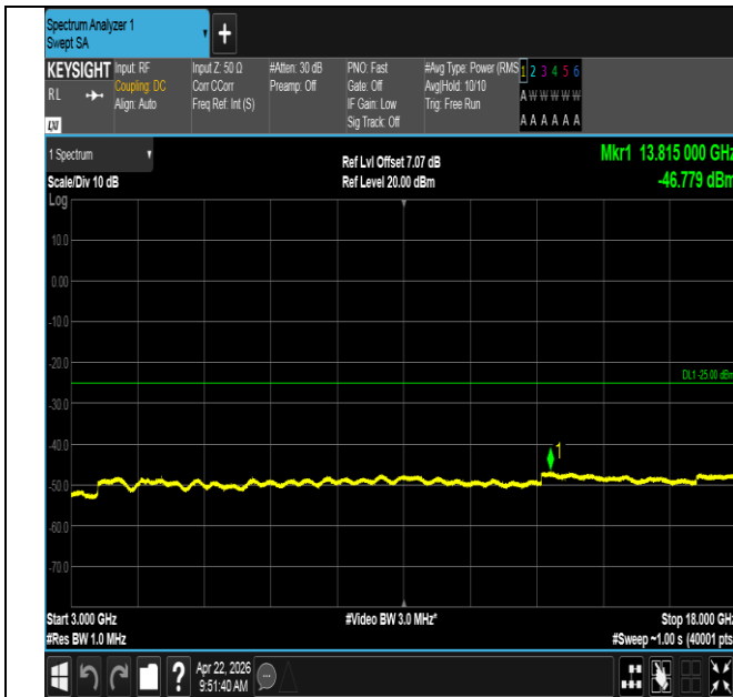
Band41-20MHz-QPSK-39750-1RB#99-3000~18000-PASS
