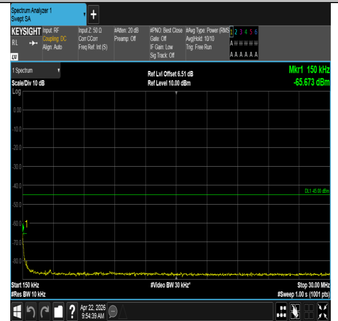
Band41-20MHz-QPSK-39750-100RB#0-0.15~30-PASS
