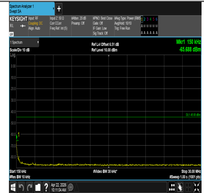
Band41-20MHz-QPSK-41490-1RB#0-0.15~30-PASS
