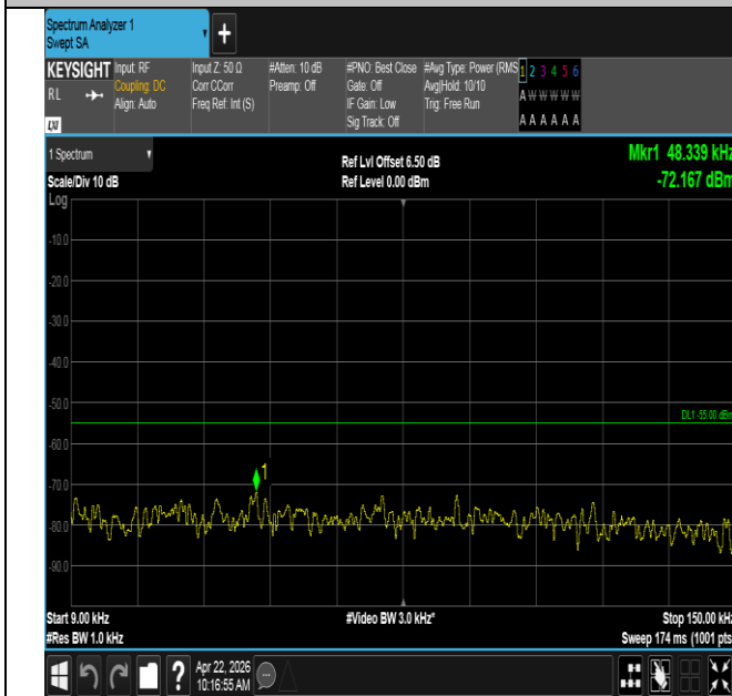
Band41-20MHz-16QAM-41490-1RB#99-0.009~0.15-PASS
