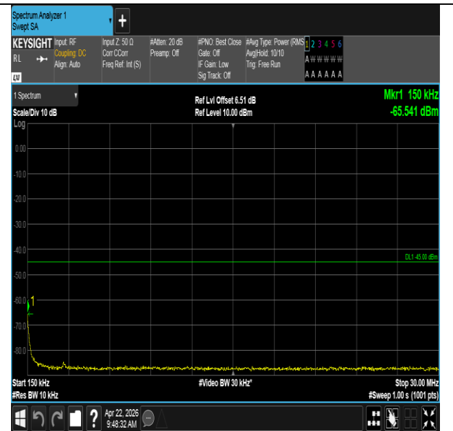
Band41-20MHz-16QAM-39750-1RB#0-0.15~30-PASS
