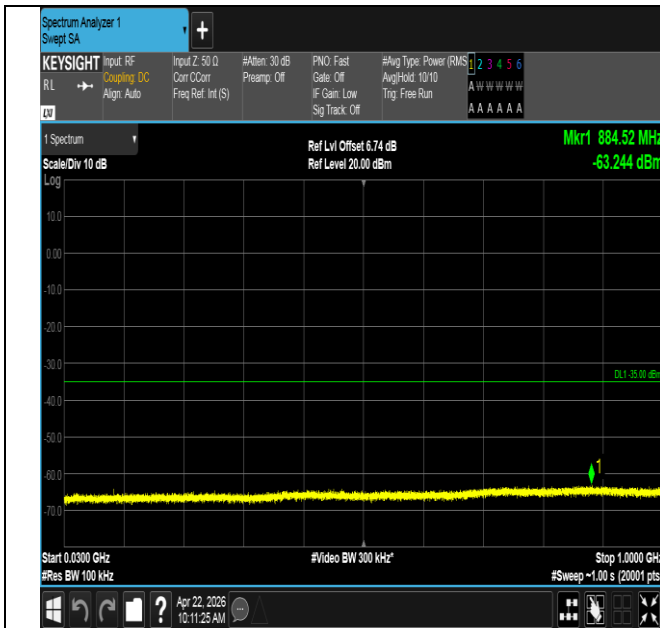
Band41-20MHz-QPSK-41490-1RB#0-30~1000-PASS
