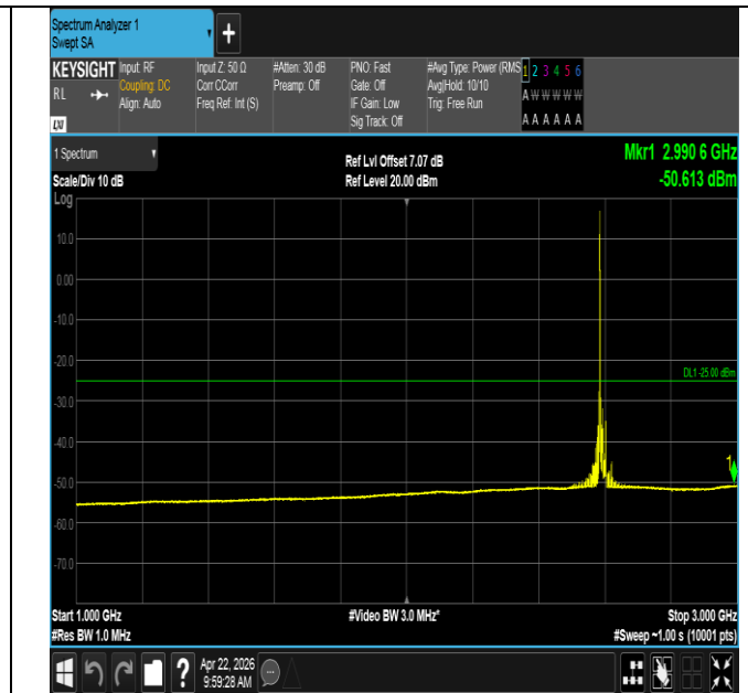
Band41-20MHz-QPSK-40620-1RB#0-1000~3000-PASS
