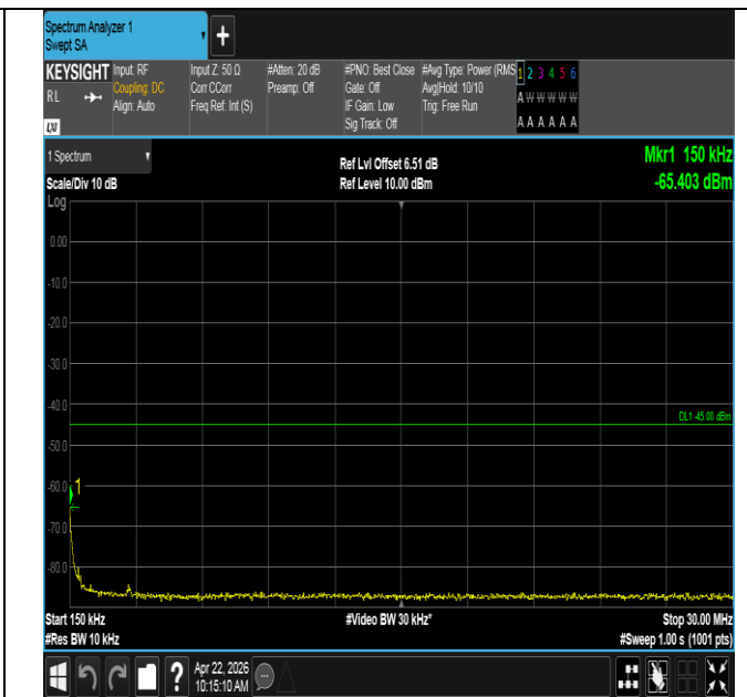
Band41-20MHz-QPSK-41490-1RB#99-0.15~30-PASS
