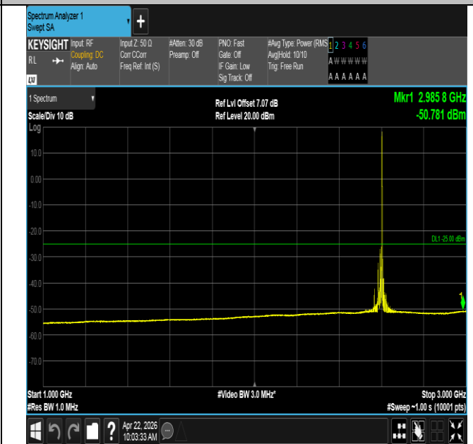
Band41-20MHz-QPSK-40620-1RB#99-1000~3000-PASS
