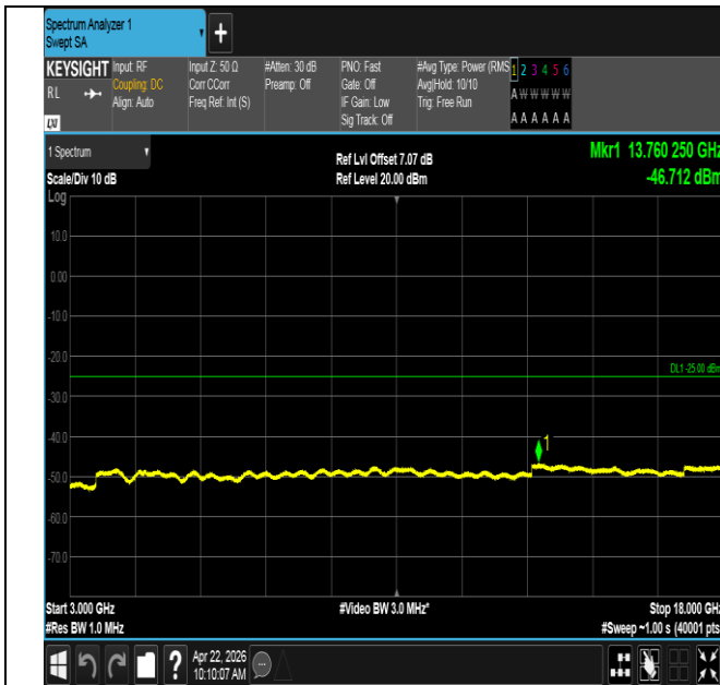
Band41-20MHz-16QAM-40620-100RB#0-3000~18000-PASS
