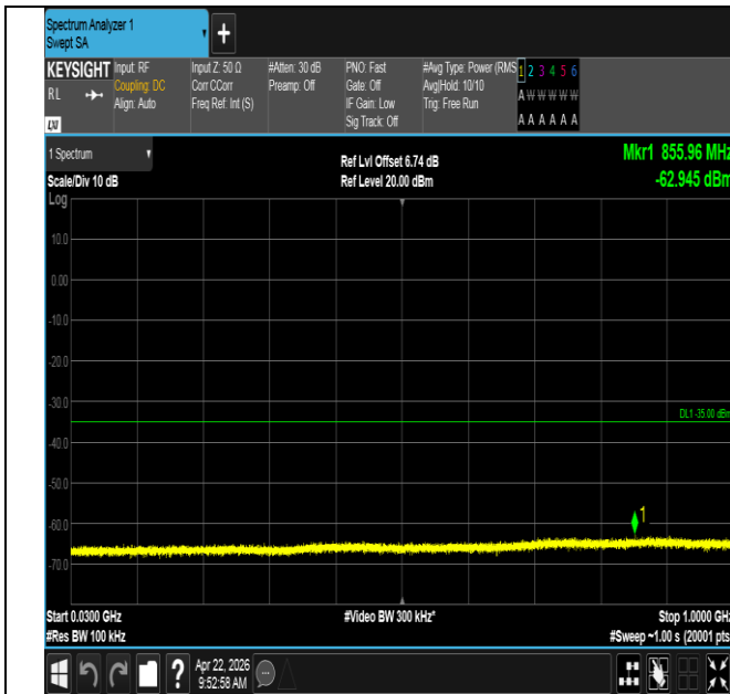
Band41-20MHz-16QAM-39750-1RB#99-30~1000-PASS
