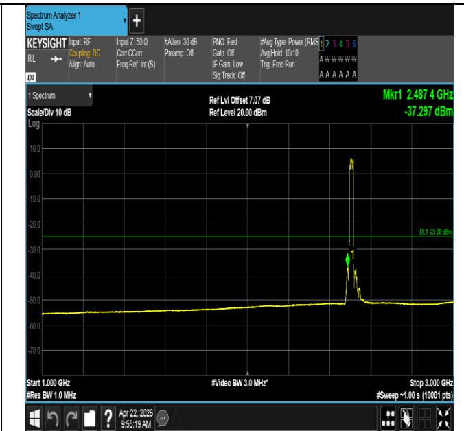
Band41-20MHz-QPSK-39750-100RB#0-1000~3000-PASS
