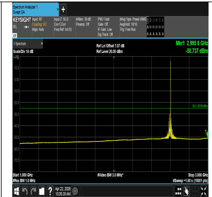
Band41-20MHz-16QAM-40620-1RB#99-1000~3000-PASS
