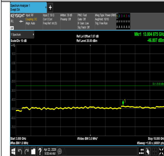
Band41-20MHz-QPSK-39750-100RB#0-3000~18000-PASS
