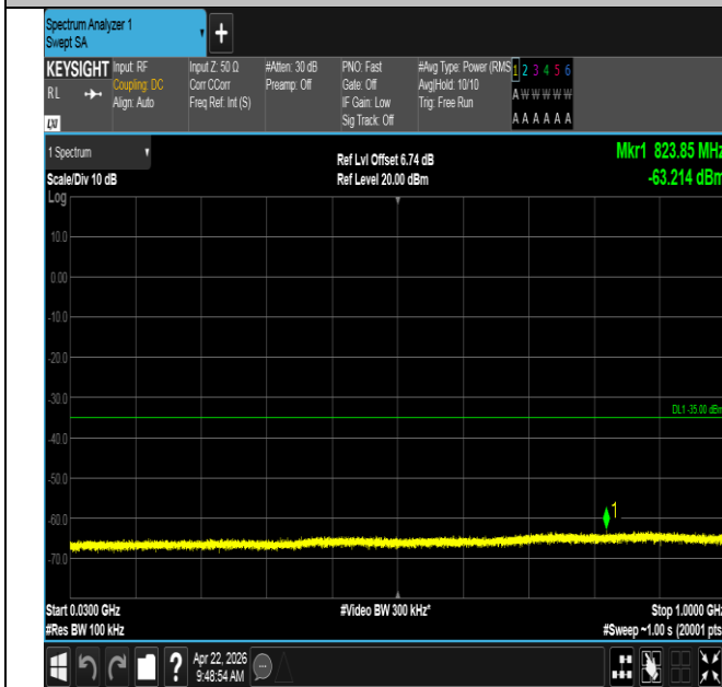
Band41-20MHz-16QAM-39750-1RB#0-30~1000-PASS
