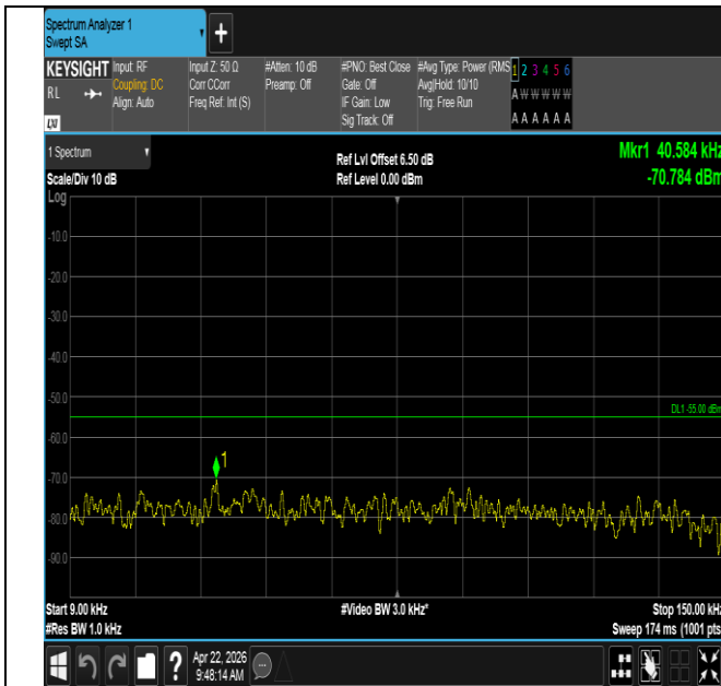
Band41-20MHz-16QAM-39750-1RB#0-0.009~0.15-PASS
