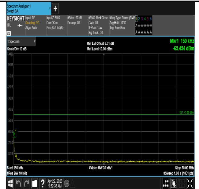
Band41-20MHz-16QAM-39750-1RB#99-0.15~30-PASS
