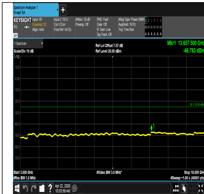
Band41-20MHz-QPSK-40620-1RB#99-3000~18000-PASS
