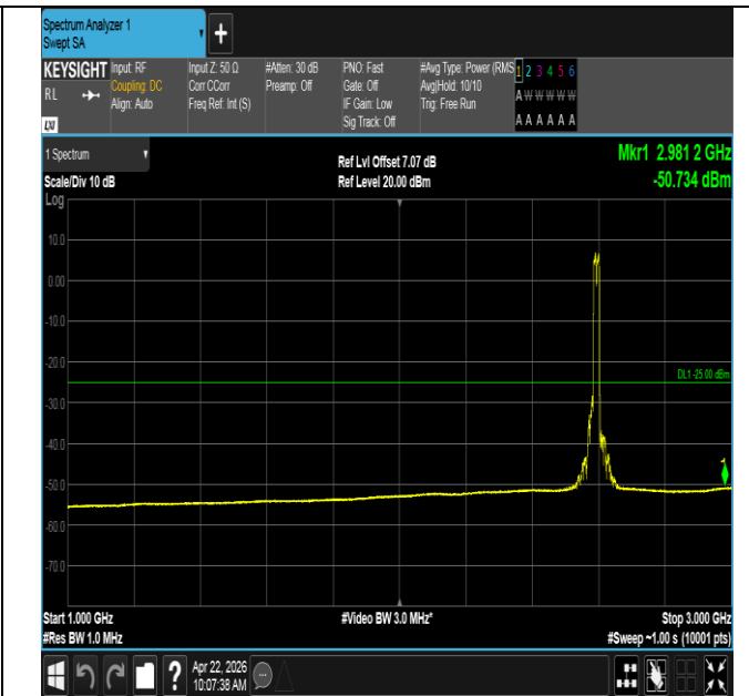
Band41-20MHz-QPSK-40620-100RB#0-1000~3000-PASS
