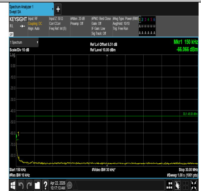
Band41-20MHz-16QAM-41490-1RB#99-0.15~30-PASS
