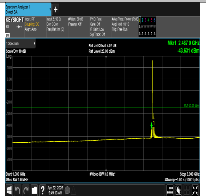
Band41-20MHz-16QAM-39750-1RB#0-1000~3000-PASS
