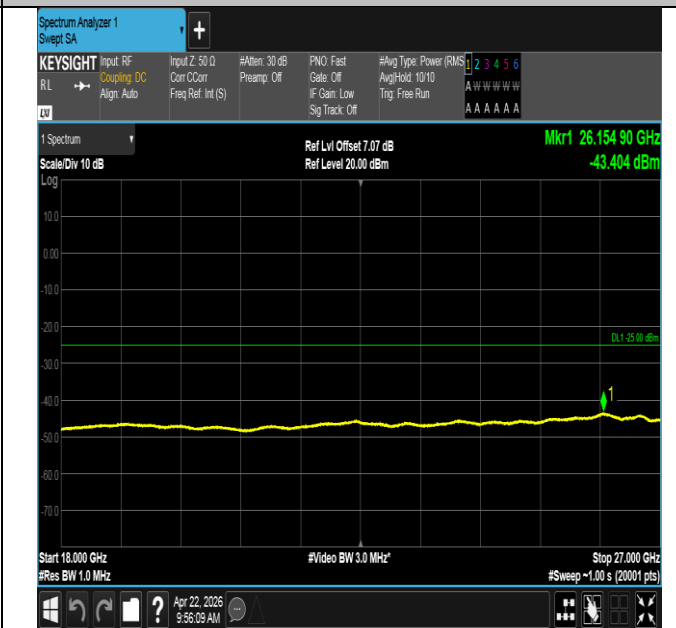
Band41-20MHz-QPSK-39750-100RB#0-18000~27000-PASS
