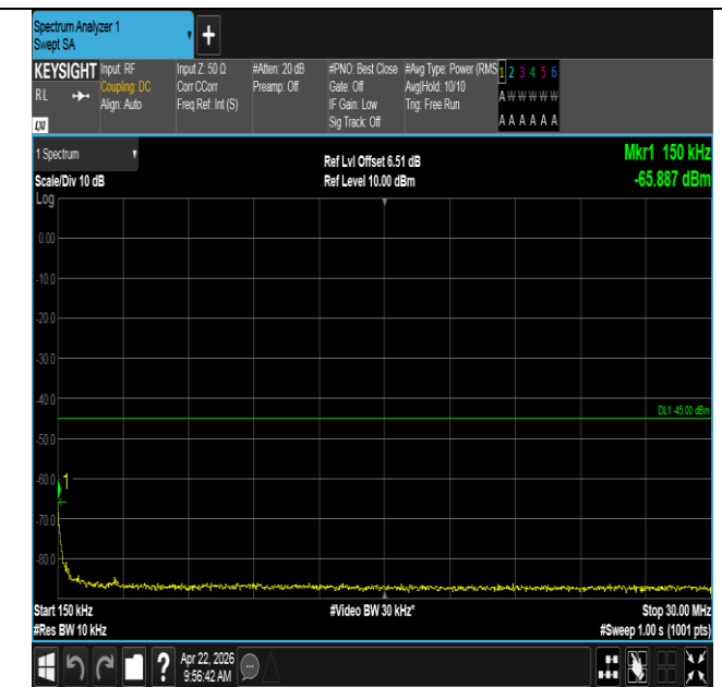
Band41-20MHz-16QAM-39750-100RB#0-0.15~30-PASS
