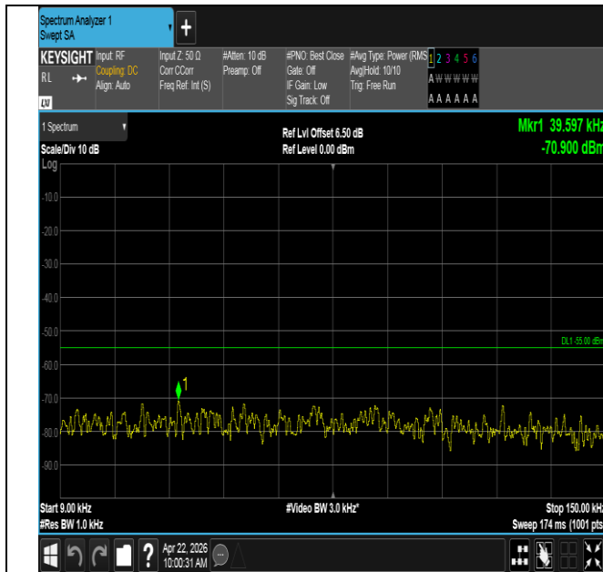
Band41-20MHz-16QAM-40620-1RB#0-0.009~0.15-PASS
