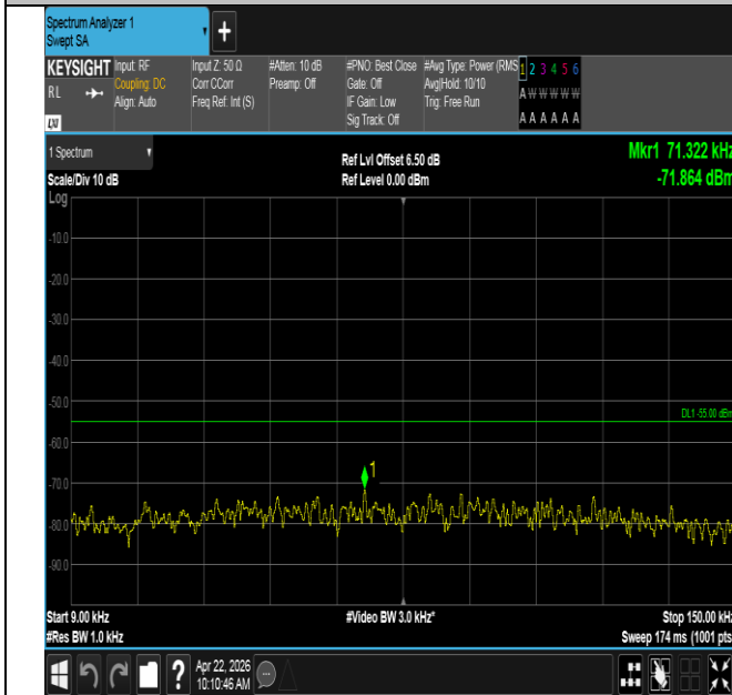
Band41-20MHz-QPSK-41490-1RB#0-0.009~0.15-PASS
