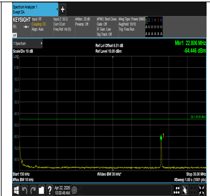
Band41-20MHz-16QAM-40620-1RB#0-0.15~30-PASS
