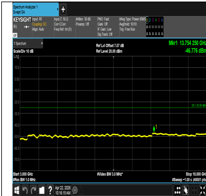
Band41-20MHz-QPSK-41490-1RB#99-3000~18000-PASS
