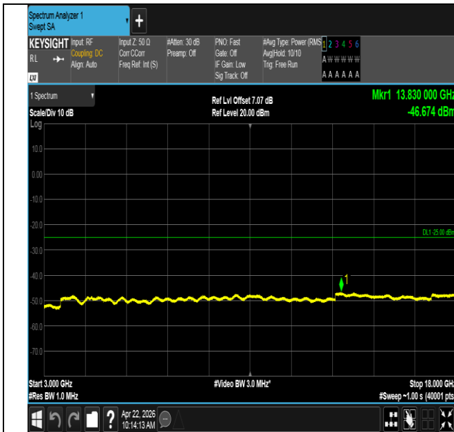
Band41-20MHz-16QAM-41490-1RB#0-3000~18000-PASS
