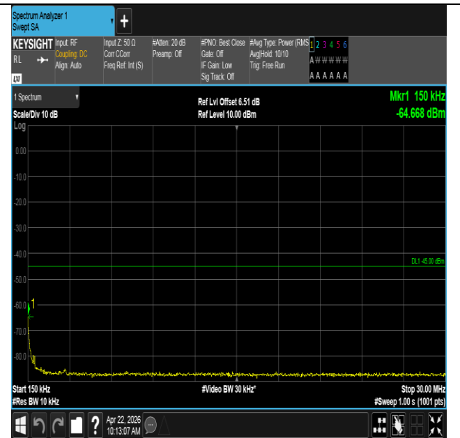
Band41-20MHz-16QAM-41490-1RB#0-0.15~30-PASS
