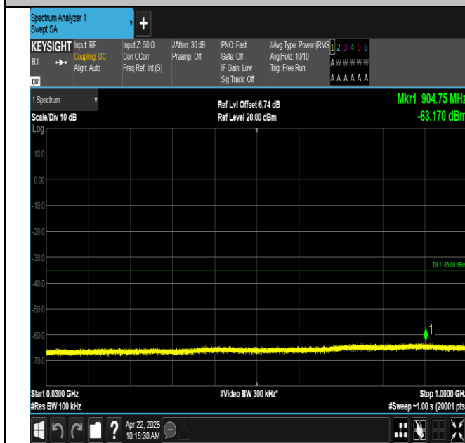
Band41-20MHz-QPSK-41490-1RB#99-30~1000-PASS
