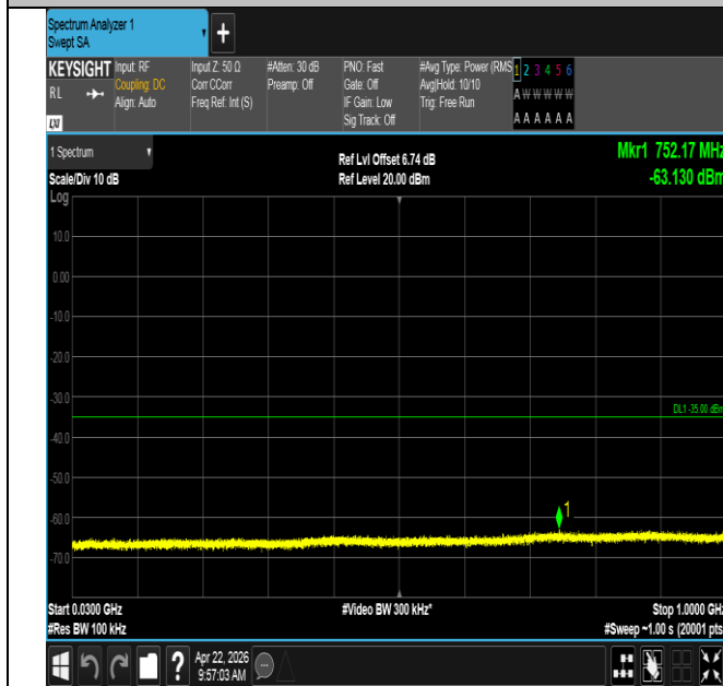
Band41-20MHz-16QAM-39750-100RB#0-30~1000-PASS
