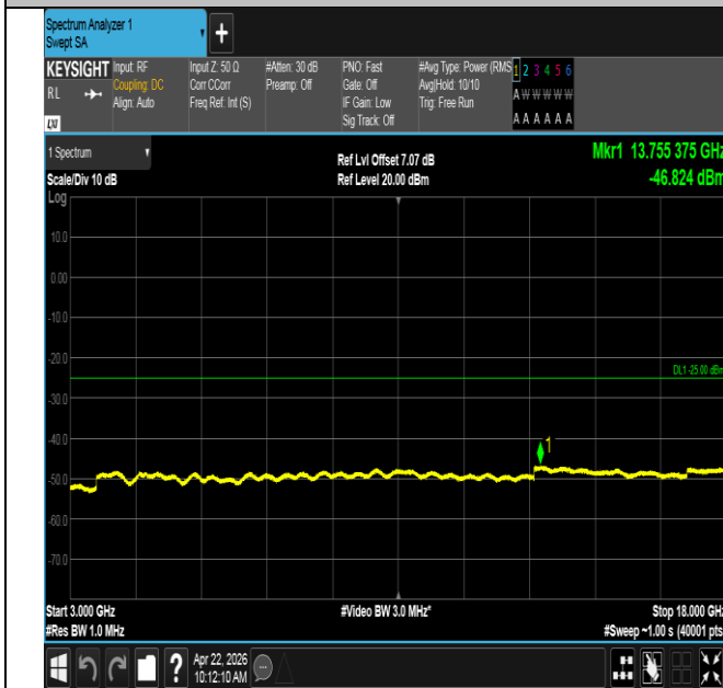
Band41-20MHz-QPSK-41490-1RB#0-3000~18000-PASS
