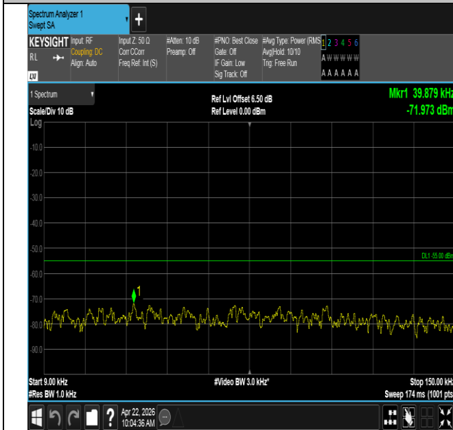
Band41-20MHz-16QAM-40620-1RB#99-0.009~0.15-PASS
