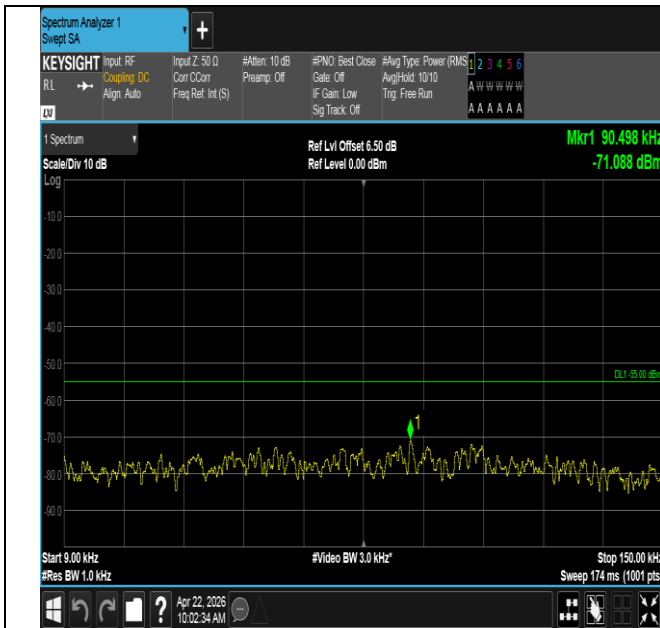
Band41-20MHz-QPSK-40620-1RB#99-0.009~0.15-PASS
