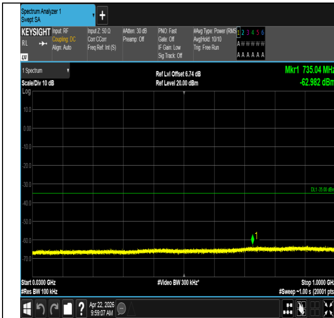
Band41-20MHz-QPSK-40620-1RB#0-30~1000-PASS
