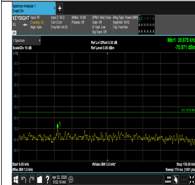
Band41-20MHz-16QAM-39750-1RB#99-0.009~0.15-PASS
