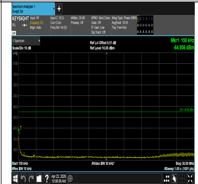
Band41-20MHz-QPSK-40620-100RB#0-0.15~30-PASS
