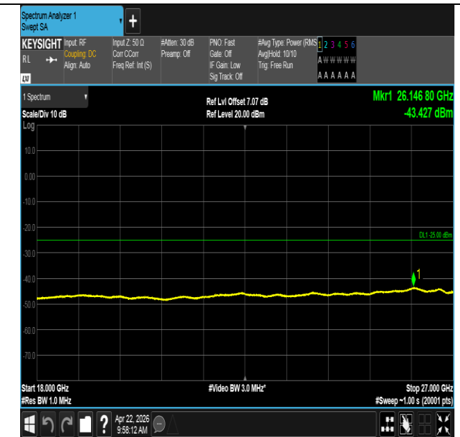
Band41-20MHz-16QAM-39750-100RB#0-18000~27000-PASS
