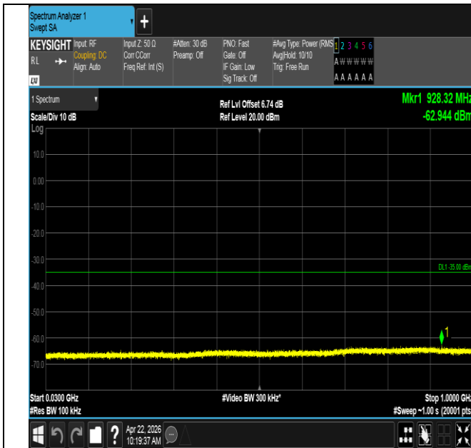
Band41-20MHz-QPSK-41490-100RB#0-30~1000-PASS
