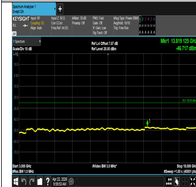
Band41-20MHz-QPSK-40620-1RB#0-3000~18000-PASS
