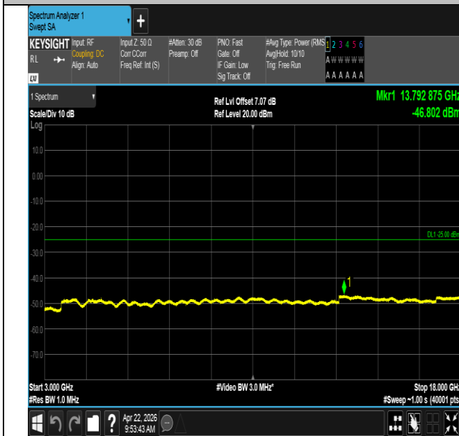
Band41-20MHz-16QAM-39750-1RB#99-3000~18000-PASS
