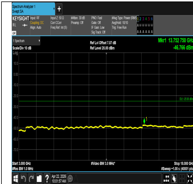
Band41-20MHz-16QAM-40620-1RB#0-3000~18000-PASS
