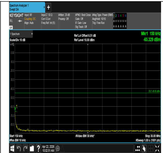
Band41-20MHz-QPSK-40620-1RB#99-0.15~30-PASS
