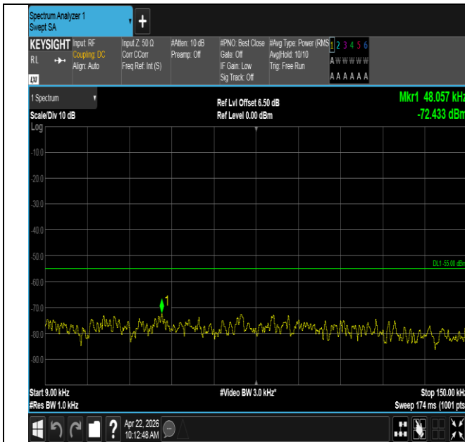
Band41-20MHz-16QAM-41490-1RB#0-0.009~0.15-PASS
