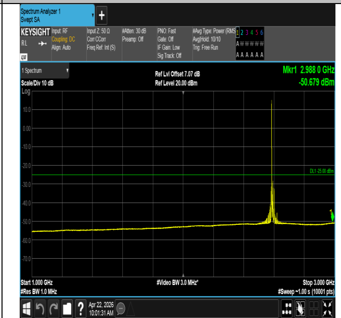
Band41-20MHz-16QAM-40620-1RB#0-1000~3000-PASS
