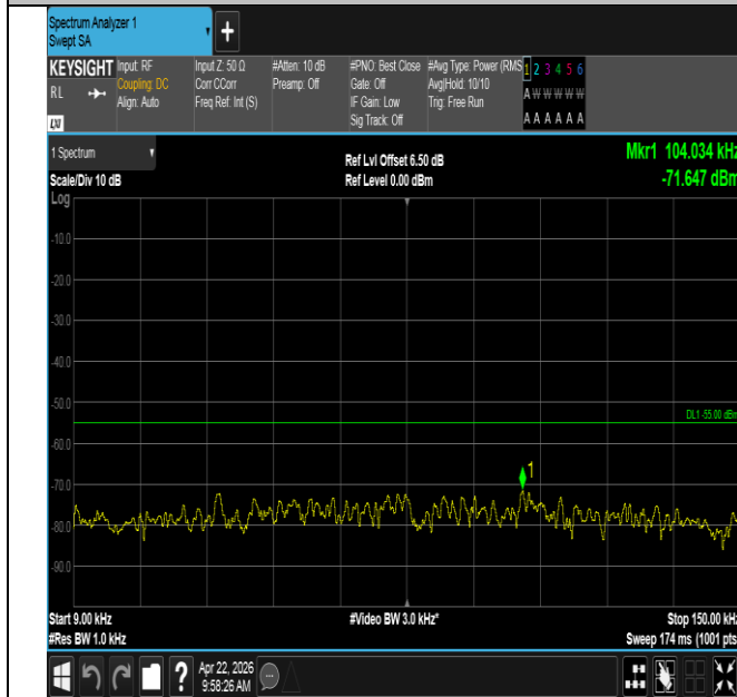
Band41-20MHz-QPSK-40620-1RB#0-0.009~0.15-PASS
