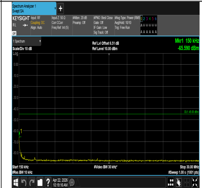
Band41-20MHz-QPSK-41490-100RB#0-0.15~30-PASS
