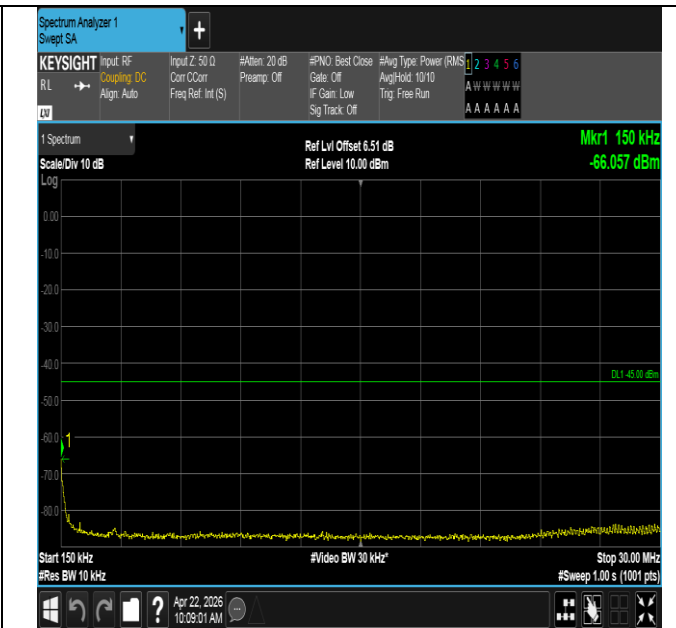
Band41-20MHz-16QAM-40620-100RB#0-0.15~30-PASS
