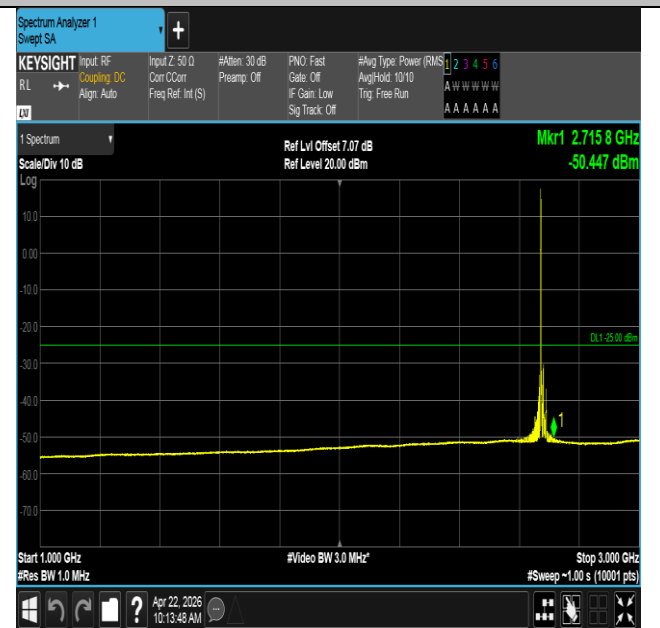
Band41-20MHz-16QAM-41490-1RB#0-1000~3000-PASS
