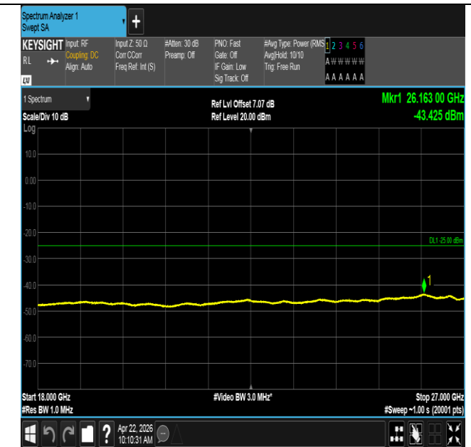
Band41-20MHz-16QAM-40620-100RB#0-18000~27000-PASS
