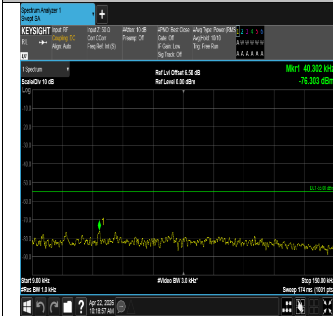
Band41-20MHz-QPSK-41490-100RB#0-0.009~0.15-PASS
