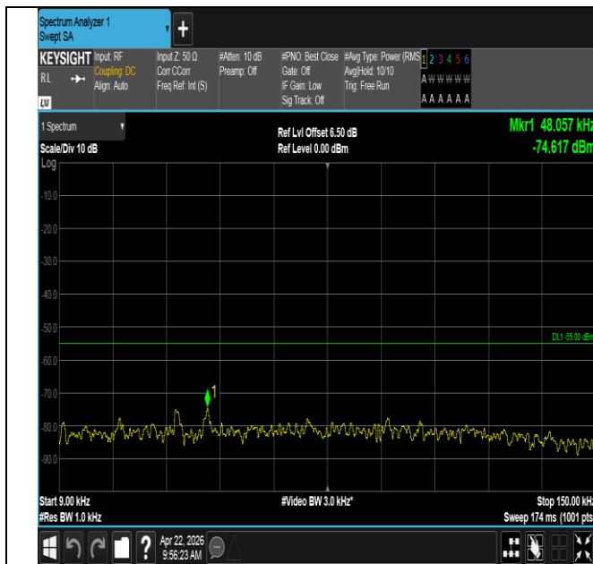
Band41-20MHz-16QAM-39750-100RB#0-0.009~0.15-PASS
