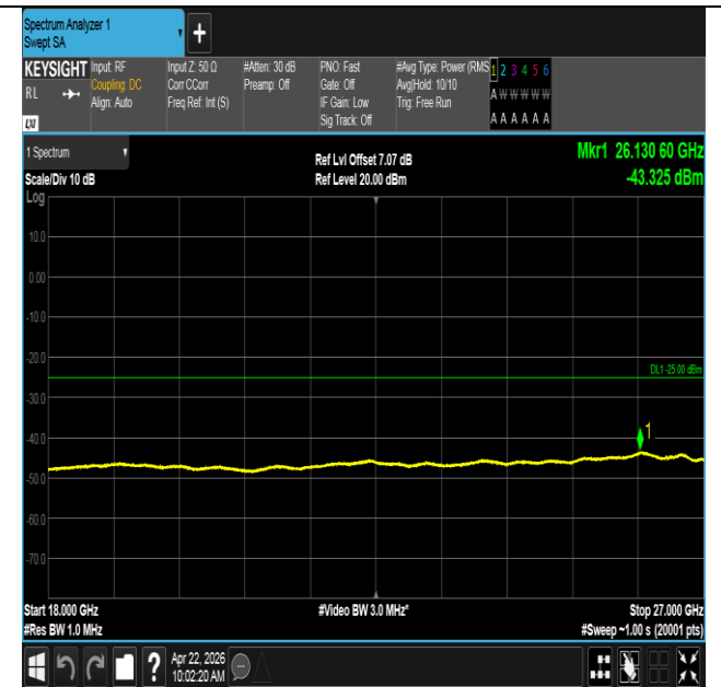
Band41-20MHz-16QAM-40620-1RB#0-18000~27000-PASS
