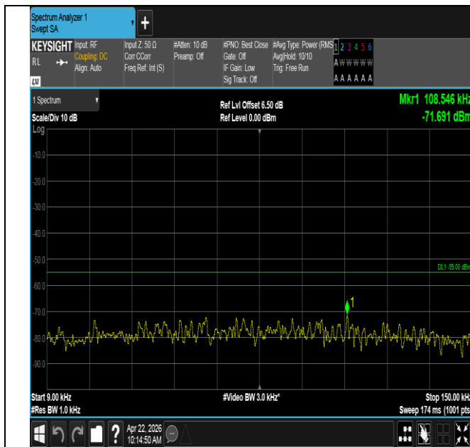
Band41-20MHz-QPSK-41490-1RB#99-0.009~0.15-PASS
