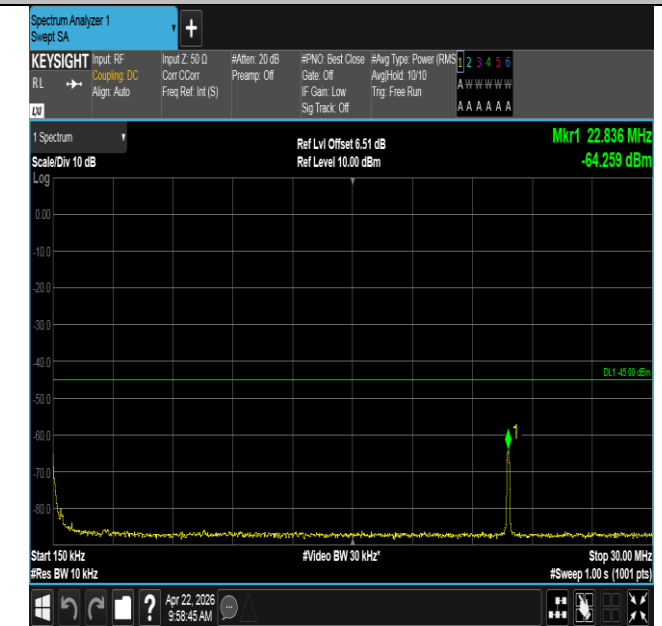
Band41-20MHz-QPSK-40620-1RB#0-0.15~30-PASS
