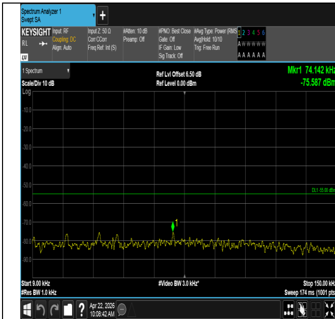
Band41-20MHz-16QAM-40620-100RB#0-0.009~0.15-PASS
