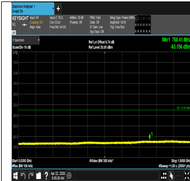
Band41-20MHz-QPSK-39750-100RB#0-30~1000-PASS
