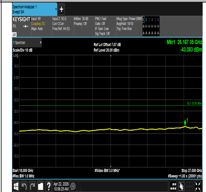
Band41-20MHz-16QAM-40620-1RB#99-18000~27000-PASS
