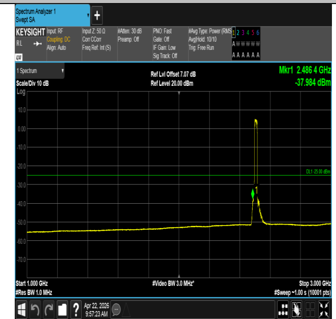
Band41-20MHz-16QAM-39750-100RB#0-1000~3000-PASS
