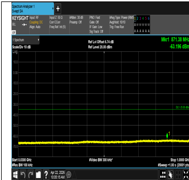
Band41-20MHz-16QAM-40620-1RB#99-30~1000-PASS
