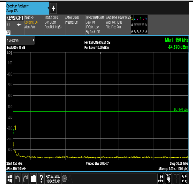
Band41-20MHz-16QAM-40620-1RB#99-0.15~30-PASS
