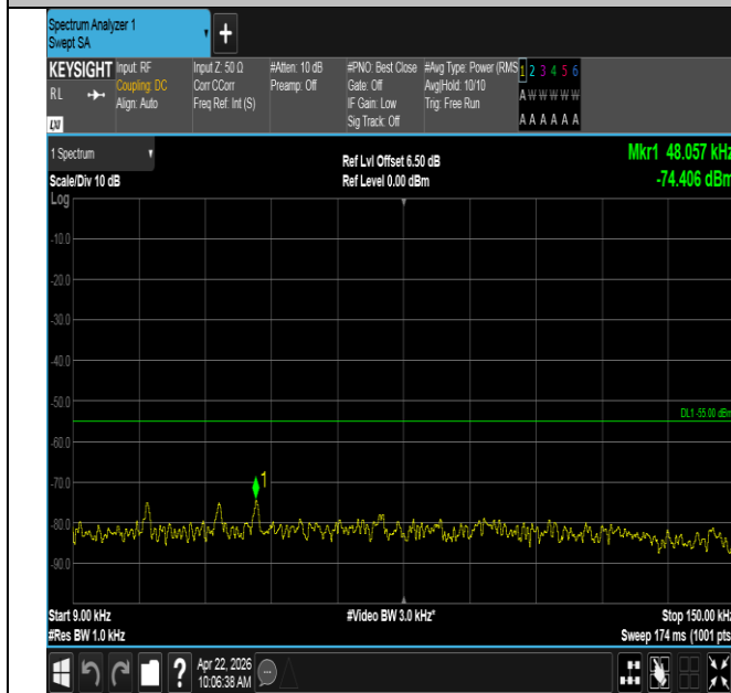
Band41-20MHz-QPSK-40620-100RB#0-0.009~0.15-PASS
