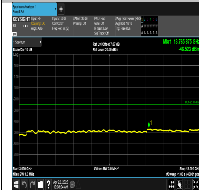
Band41-20MHz-QPSK-40620-100RB#0-3000~18000-PASS
