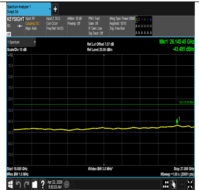
Band41-20MHz-16QAM-39750-1RB#0-18000~27000-PASS
