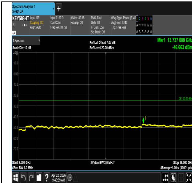
Band41-20MHz-16QAM-39750-1RB#0-3000~18000-PASS
