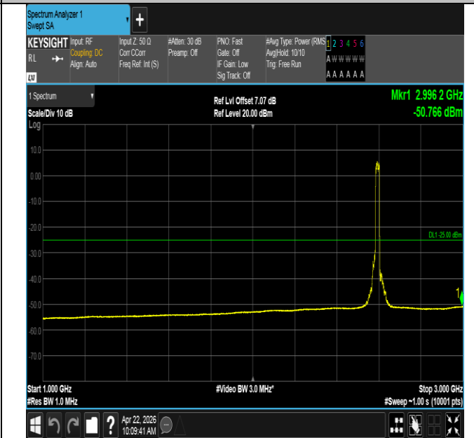
Band41-20MHz-16QAM-40620-100RB#0-1000~3000-PASS
