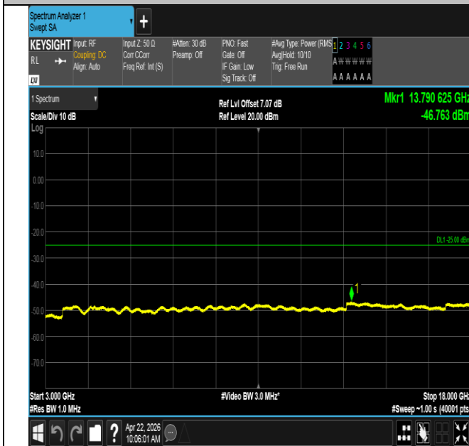
Band41-20MHz-16QAM-40620-1RB#99-3000~18000-PASS
