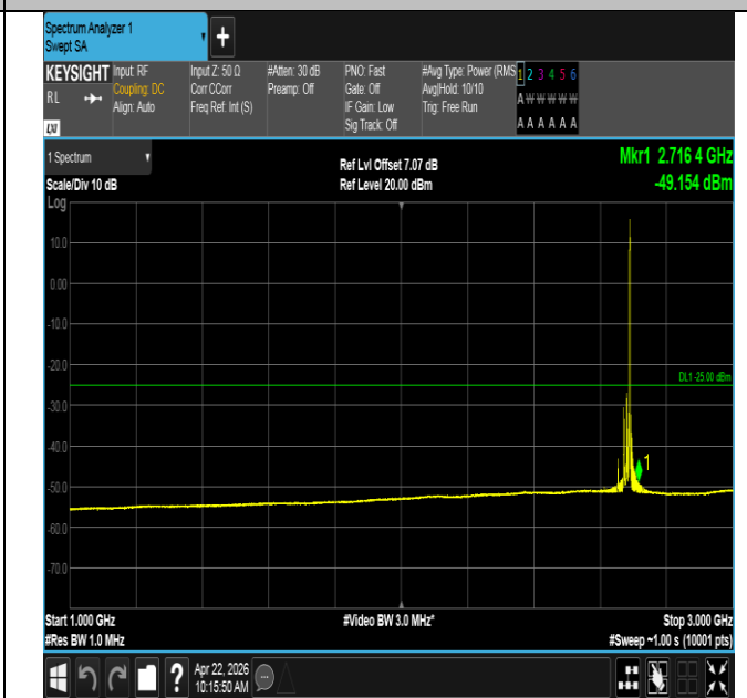
Band41-20MHz-QPSK-41490-1RB#99-1000~3000-PASS
