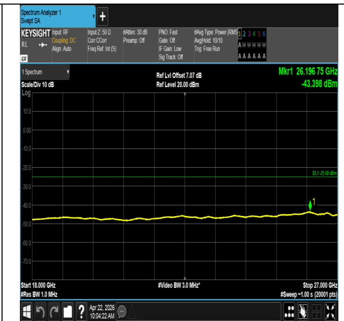
Band41-20MHz-QPSK-40620-1RB#99-18000~27000-PASS
