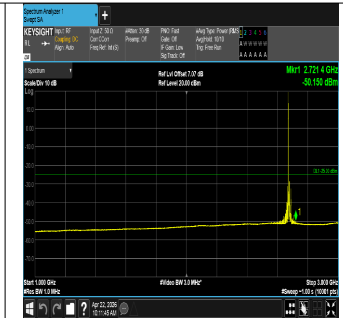
Band41-20MHz-QPSK-41490-1RB#0-1000~3000-PASS
