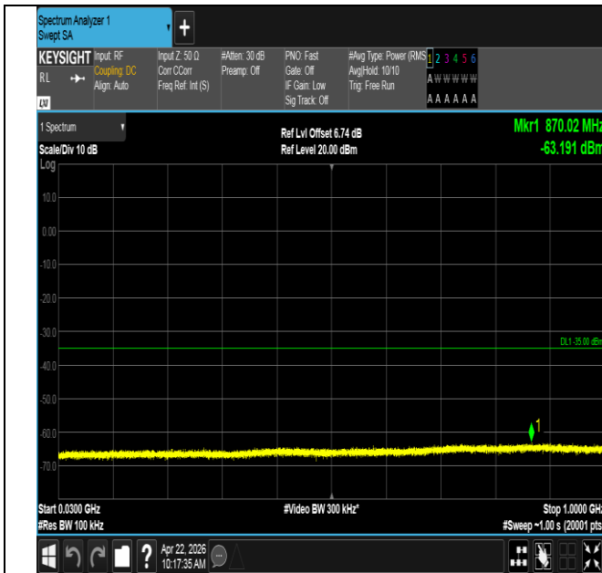
Band41-20MHz-16QAM-41490-1RB#99-30~1000-PASS
