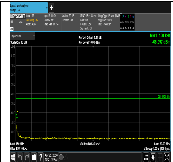
Band41-20MHz-16QAM-41490-100RB#0-0.15~30-PASS
