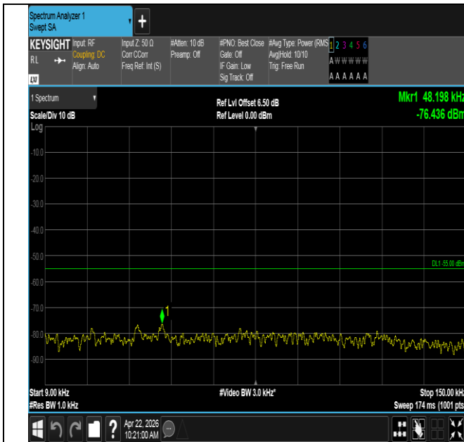
Band41-20MHz-16QAM-41490-100RB#0-0.009~0.15-PASS
