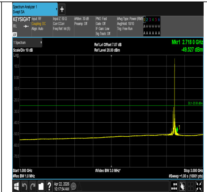
Band41-20MHz-16QAM-41490-1RB#99-1000~3000-PASS
