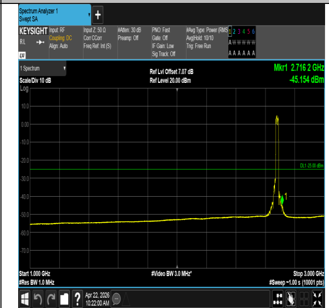
Band41-20MHz-16QAM-41490-100RB#0-1000~3000-PASS
