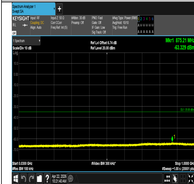
Band41-20MHz-16QAM-41490-100RB#0-30~1000-PASS
