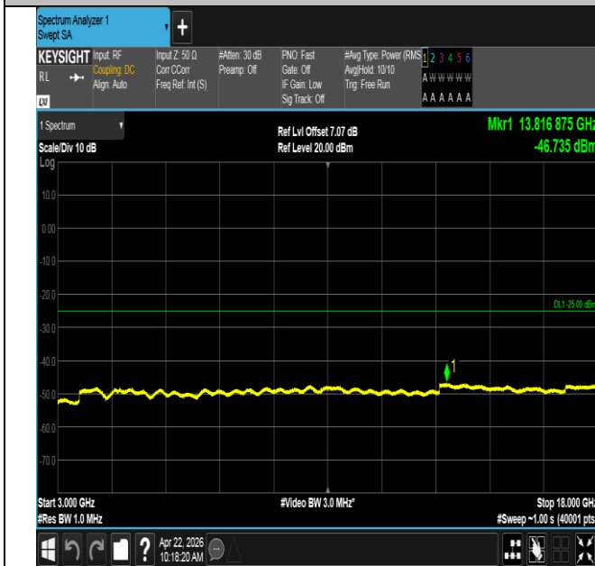
Band41-20MHz-16QAM-41490-1RB#99-3000~18000-PASS
