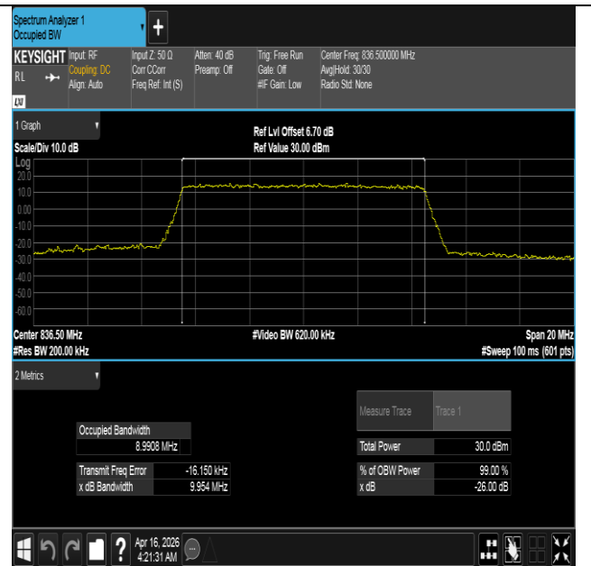
Band5-10MHz-16QAM-20525-50RB#0-PASS
