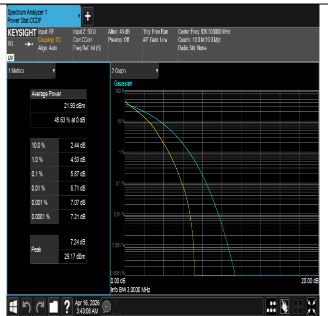
Band5-3MHz-QPSK-20525-15RB#0-PASS
