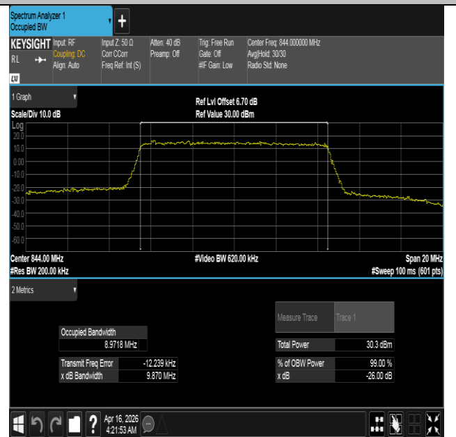
Band5-10MHz-16QAM-20600-50RB#0-PASS
