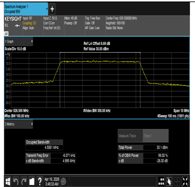
Band5-5MHz-16QAM-20425-25RB#0-PASS
