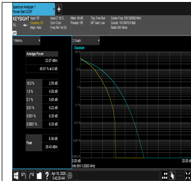
Band5-3MHz-QPSK-20525-1RB#0-PASS
