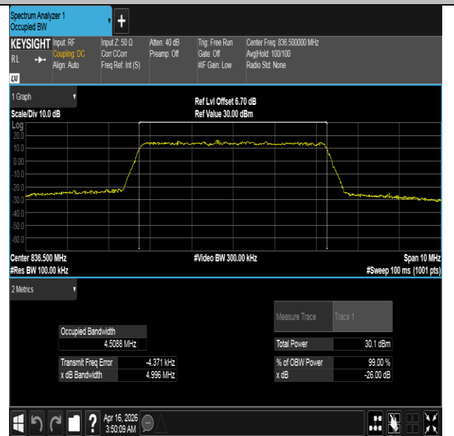
Band5-5MHz-16QAM-20525-25RB#0-PASS
