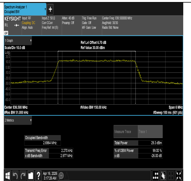
Band5-3MHz-16QAM-20525-15RB#0-PASS
