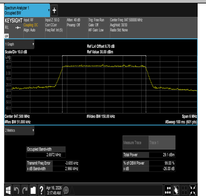
Band5-3MHz-16QAM-20635-15RB#0-PASS
