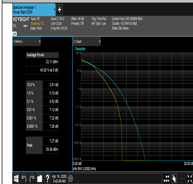
Band5-3MHz-16QAM-20525-1RB#0-PASS
