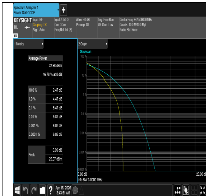
Band5-3MHz-QPSK-20635-1RB#0-PASS
