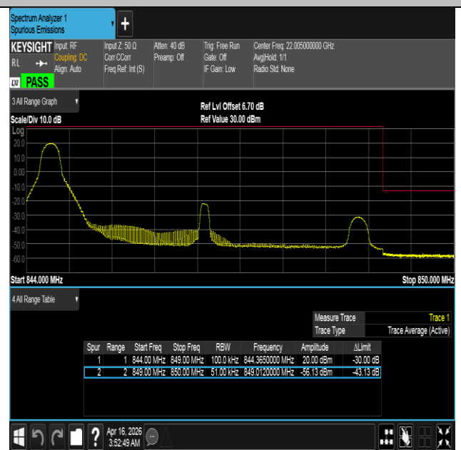
Band5-5MHz-16QAM-20625-1RB#0-PASS
