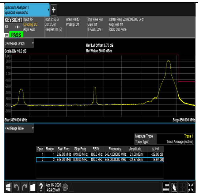
Band5-10MHz-QPSK-20600-1RB#49-PASS
