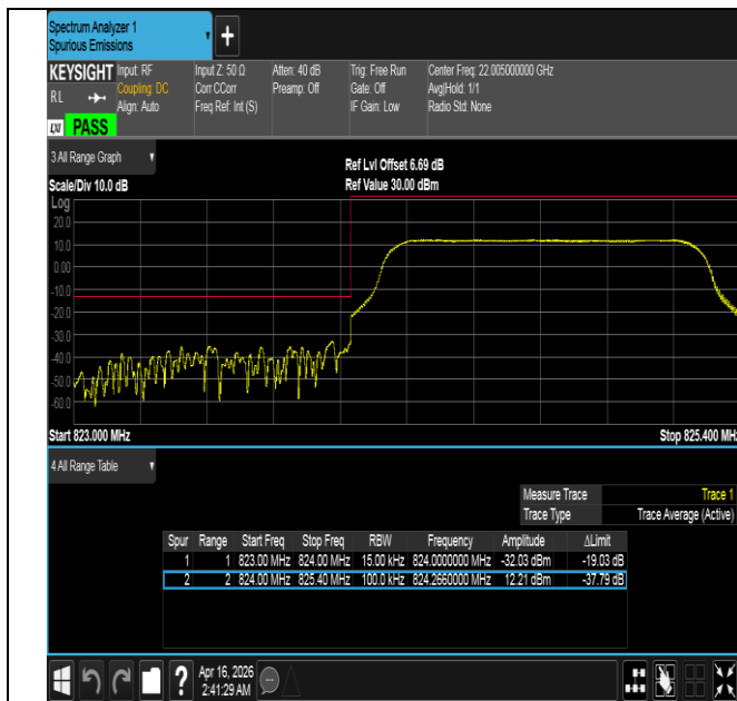
Band5-1.4MHz-QPSK-20407-6RB#0-PASS
