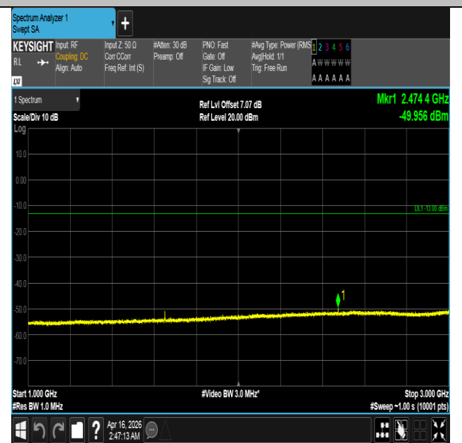
Band5-1.4MHz-QPSK-20407-6RB#0-1000~3000-PASS
