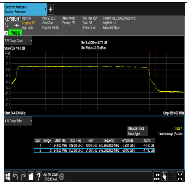
Band5-5MHz-16QAM-20625-25RB#0-PASS
