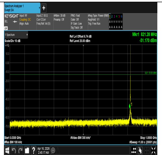
Band5-1.4MHz-QPSK-20407-1RB#5-30~1000-PASS
