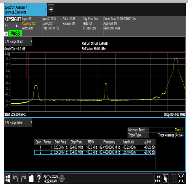
Band5-10MHz-QPSK-20450-1RB#49-PASS
