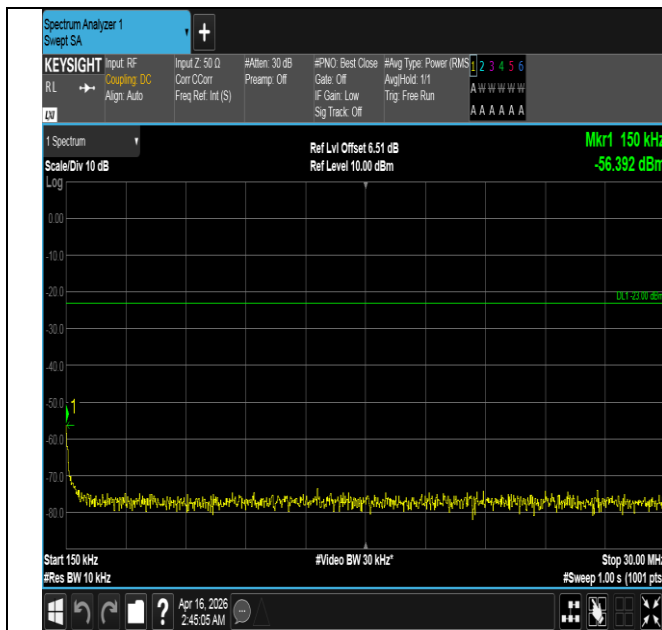
Band5-1.4MHz-QPSK-20407-1RB#5-0.15~30-PASS
