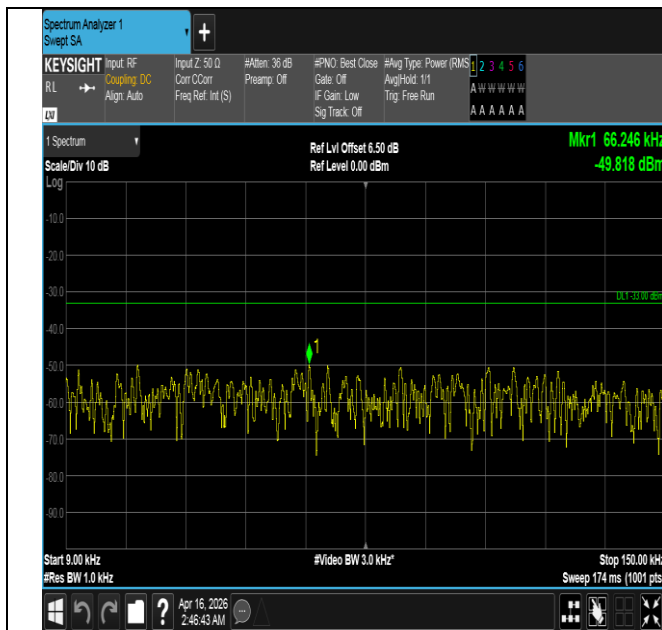
Band5-1.4MHz-QPSK-20407-6RB#0-0.009~0.15-PASS
