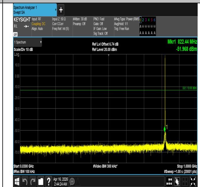
Band5-1.4MHz-16QAM-20407-1RB#0-30~1000-PASS
