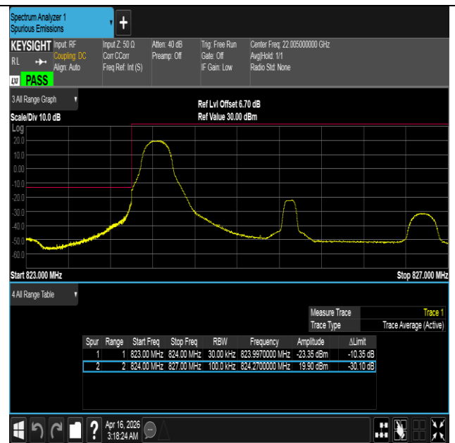
Band5-3MHz-16QAM-20415-1RB#0-PASS
