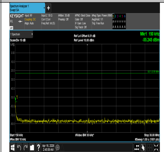
Band5-1.4MHz-16QAM-20407-1RB#5-0.15~30-PASS
