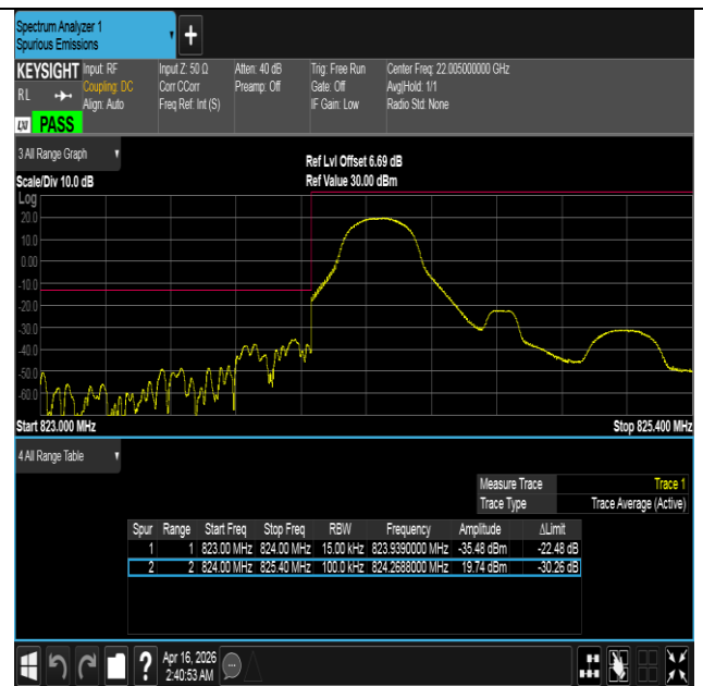
Band5-1.4MHz-16QAM-20407-1RB#0-PASS
