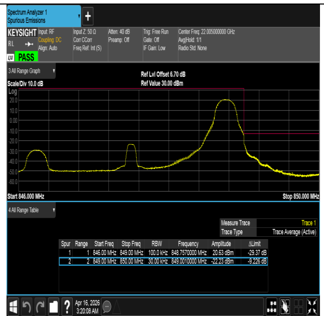
Band5-3MHz-QPSK-20635-1RB#14-PASS
