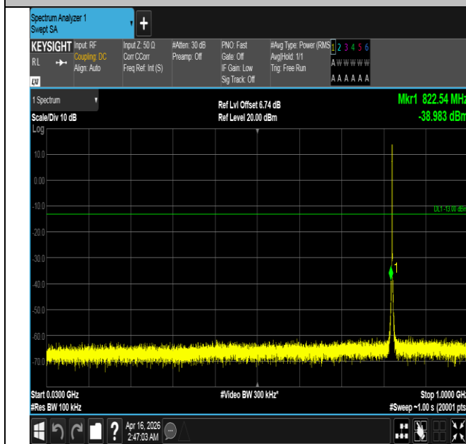
Band5-1.4MHz-QPSK-20407-6RB#0-30~1000-PASS
