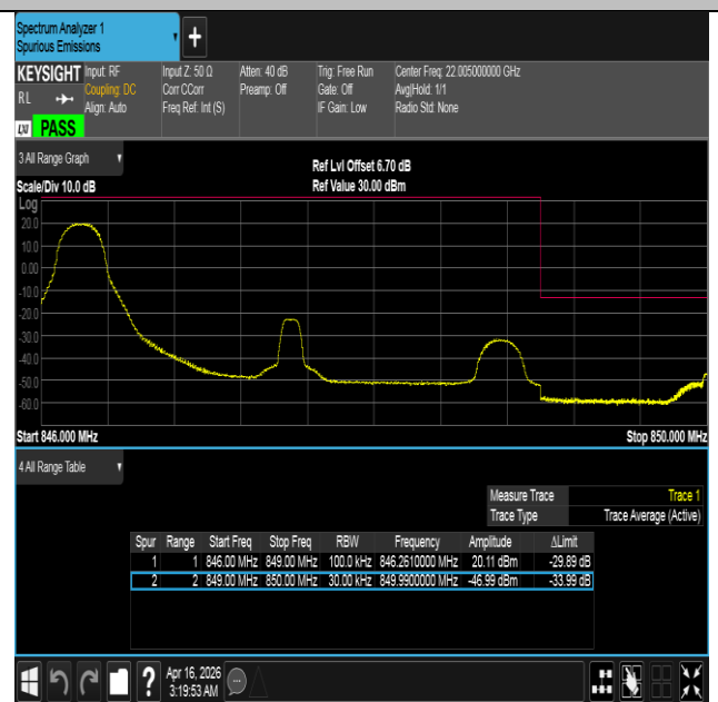
Band5-3MHz-16QAM-20635-1RB#0-PASS
