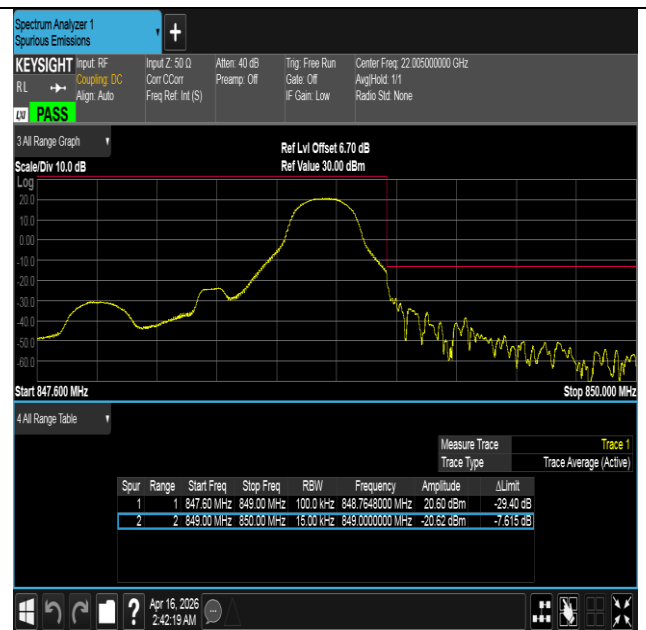
Band5-1.4MHz-QPSK-20643-1RB#5-PASS
