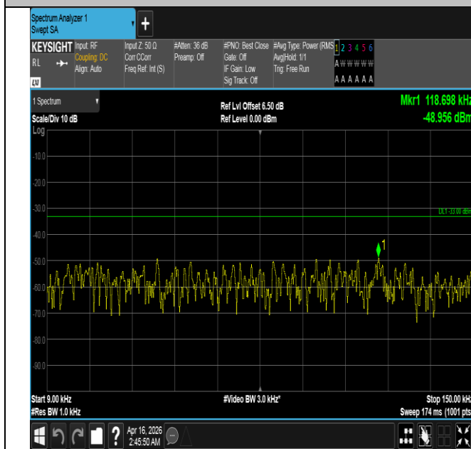
Band5-1.4MHz-16QAM-20407-1RB#5-0.009~0.15-PASS
