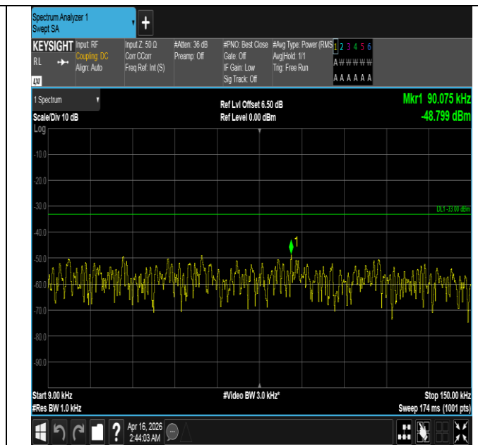
Band5-1.4MHz-16QAM-20407-1RB#0-0.009~0.15-PASS
