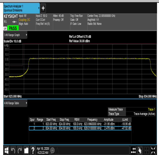
Band5-10MHz-16QAM-20450-50RB#0-PASS
