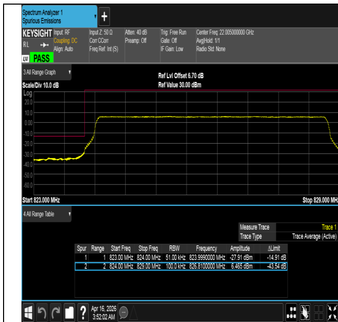
Band5-5MHz-QPSK-20425-25RB#0-PASS
