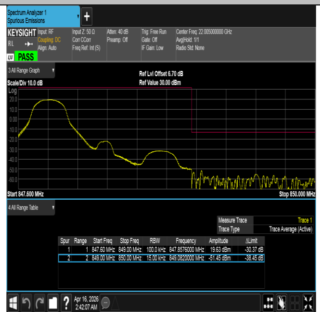
Band5-1.4MHz-16QAM-20643-1RB#0-PASS
