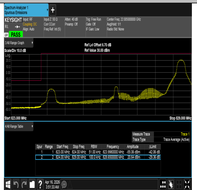
Band5-5MHz-QPSK-20425-1RB#24-PASS
