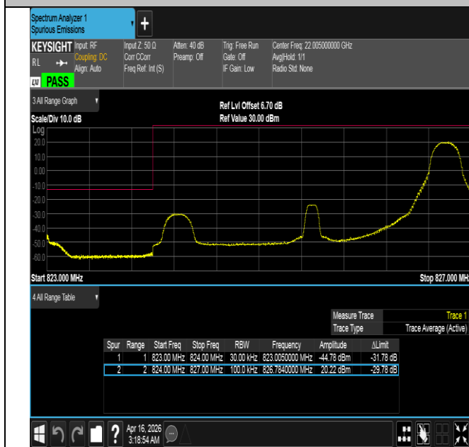
Band5-3MHz-16QAM-20415-1RB#14-PASS
