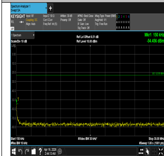
Band5-1.4MHz-16QAM-20407-1RB#0-0.15~30-PASS
