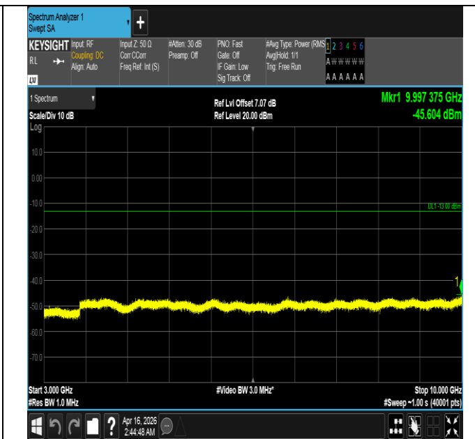
Band5-1.4MHz-16QAM-20407-1RB#0-3000~10000-PASS
