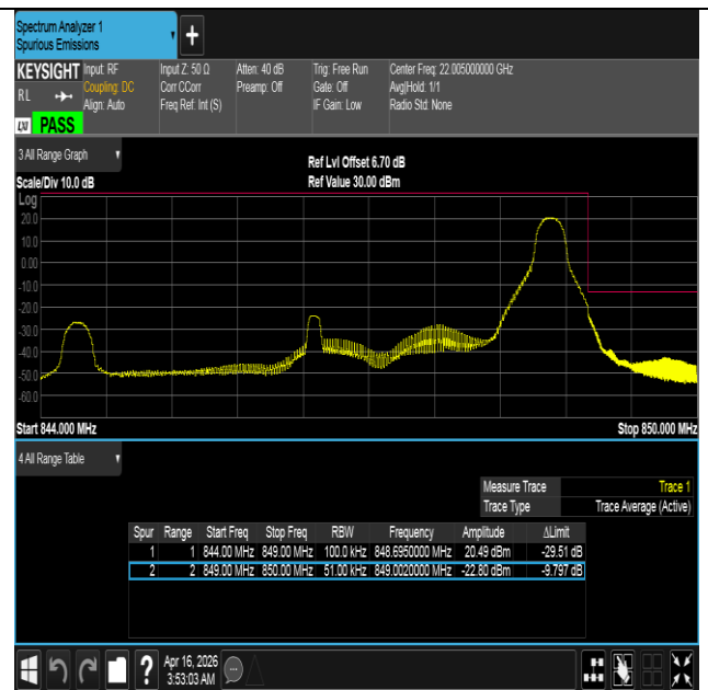
Band5-5MHz-QPSK-20625-1RB#24-PASS
