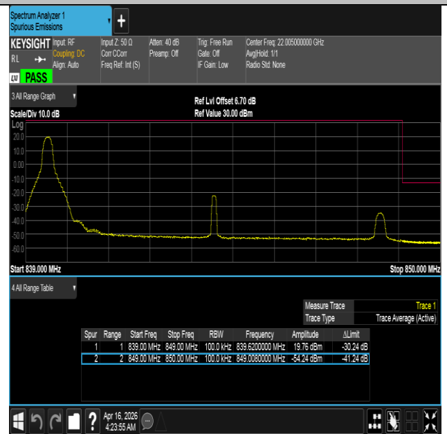
Band5-10MHz-16QAM-20600-1RB#0-PASS
