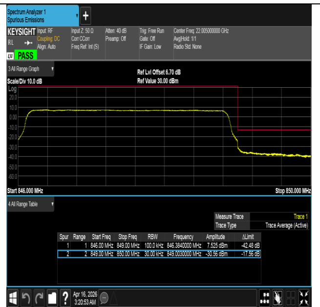
Band5-3MHz-16QAM-20635-15RB#0-PASS
