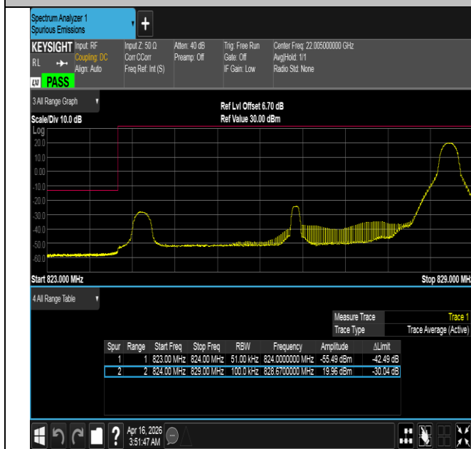
Band5-5MHz-16QAM-20425-1RB#24-PASS
