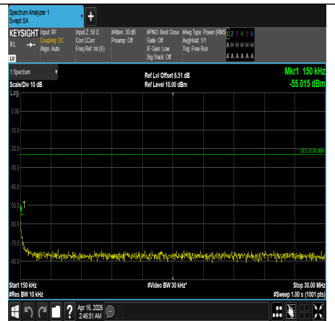
Band5-1.4MHz-QPSK-20407-6RB#0-0.15~30-PASS
