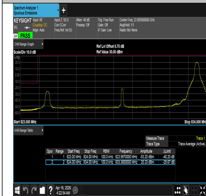
Band5-10MHz-16QAM-20450-1RB#49-PASS
