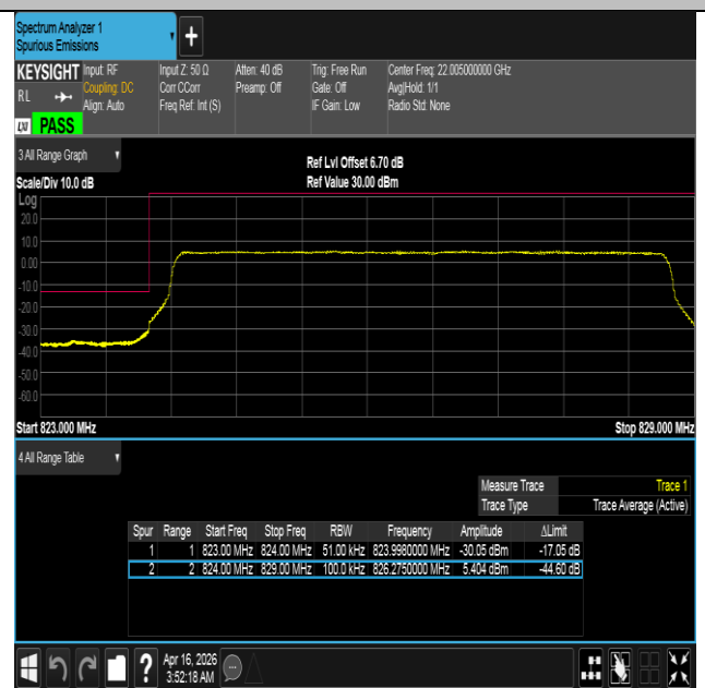
Band5-5MHz-16QAM-20425-25RB#0-PASS
