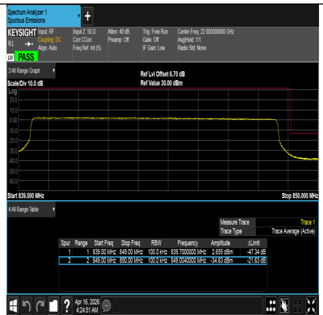
Band5-10MHz-16QAM-20600-50RB#0-PASS
