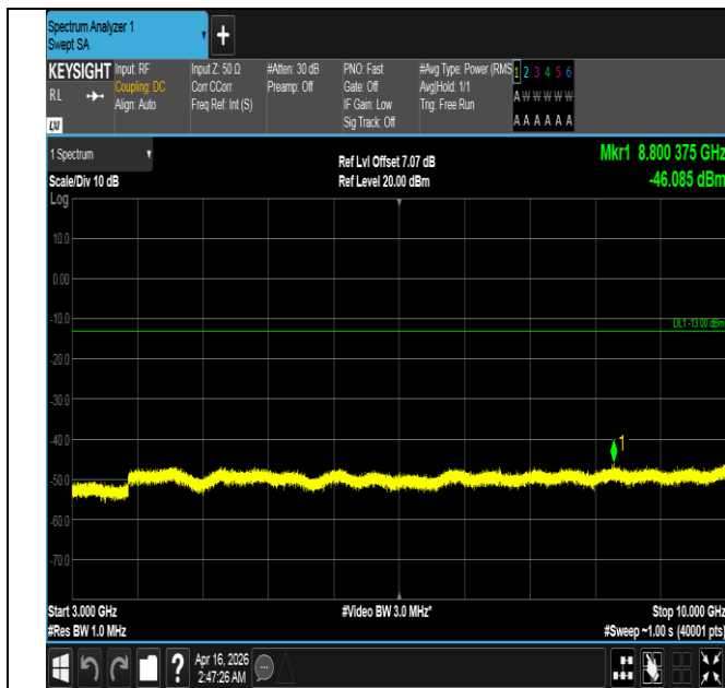
Band5-1.4MHz-QPSK-20407-6RB#0-3000~10000-PASS
