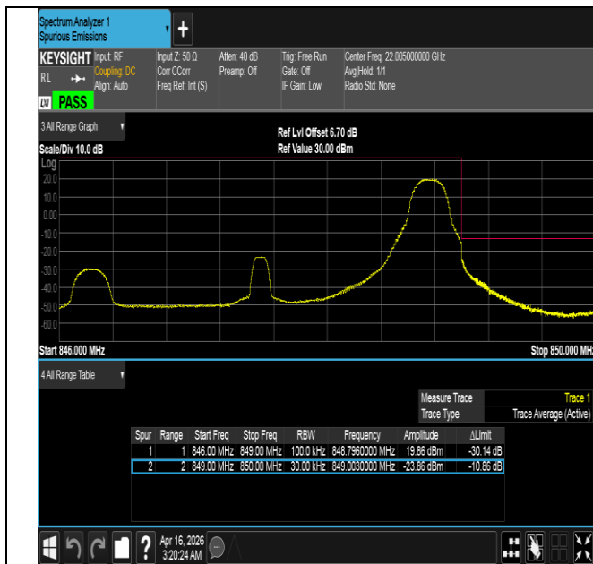
Band5-3MHz-16QAM-20635-1RB#14-PASS
