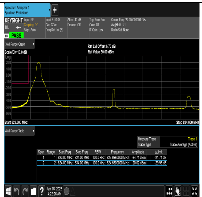
Band5-10MHz-16QAM-20450-1RB#0-PASS
