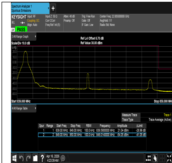
Band5-10MHz-QPSK-20600-1RB#0-PASS
