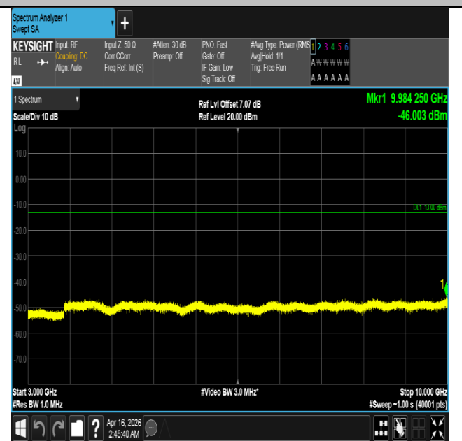
Band5-1.4MHz-QPSK-20407-1RB#5-3000~10000-PASS
