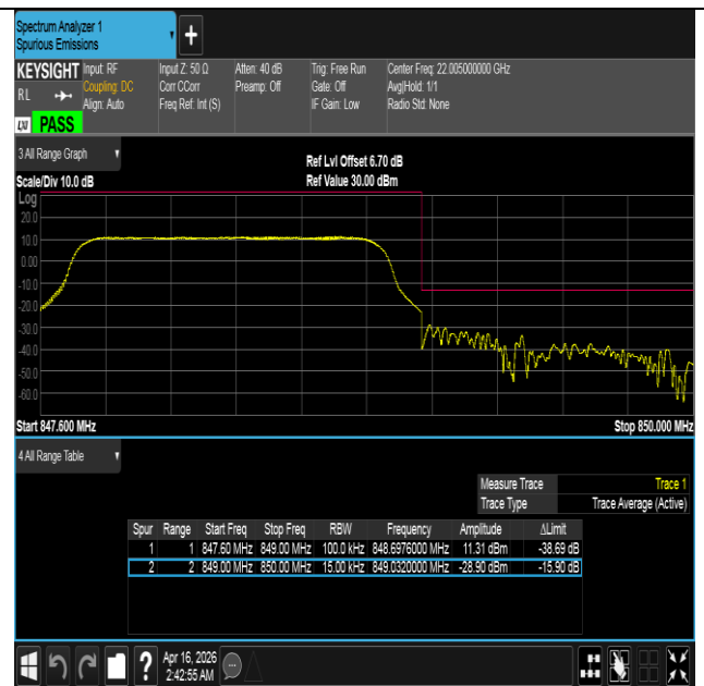
Band5-1.4MHz-16QAM-20643-6RB#0-PASS
