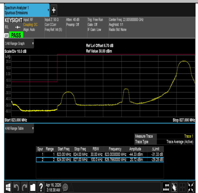
Band5-3MHz-QPSK-20415-1RB#14-PASS
