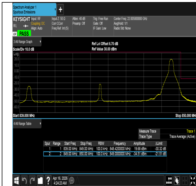
Band5-10MHz-16QAM-20600-1RB#49-PASS
