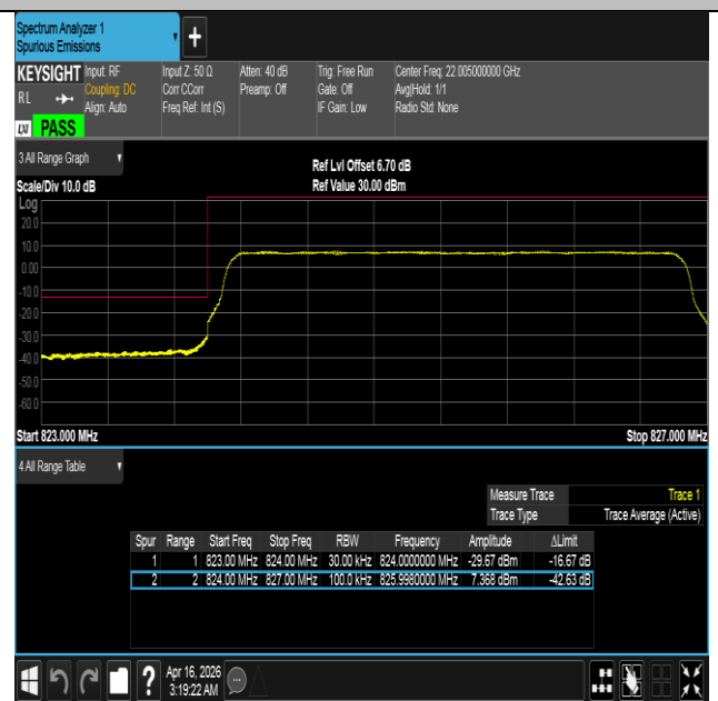
Band5-3MHz-16QAM-20415-15RB#0-PASS
