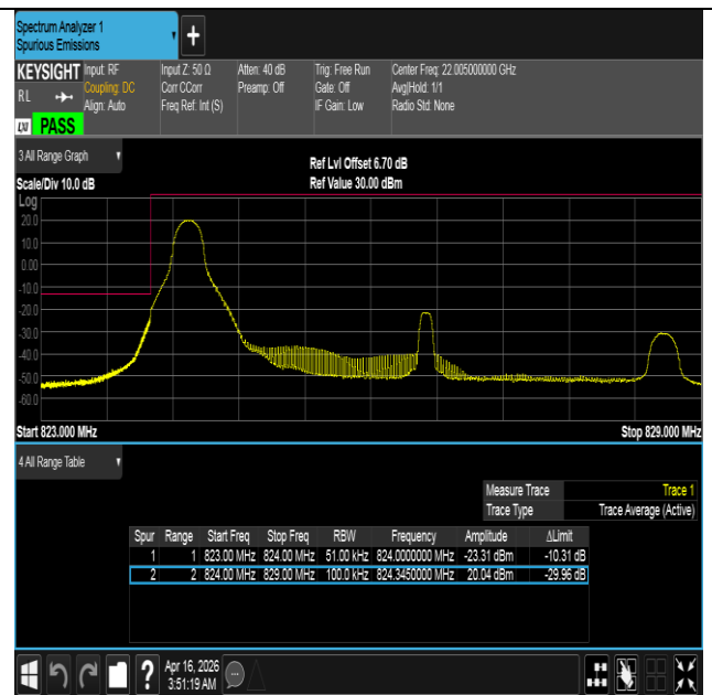
Band5-5MHz-16QAM-20425-1RB#0-PASS
