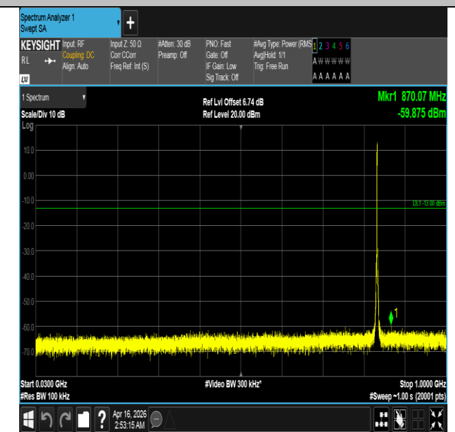
Band5-1.4MHz-16QAM-20525-6RB#0-30~1000-PASS
