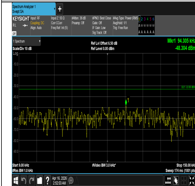
Band5-1.4MHz-QPSK-20525-6RB#0-0.009~0.15-PASS
