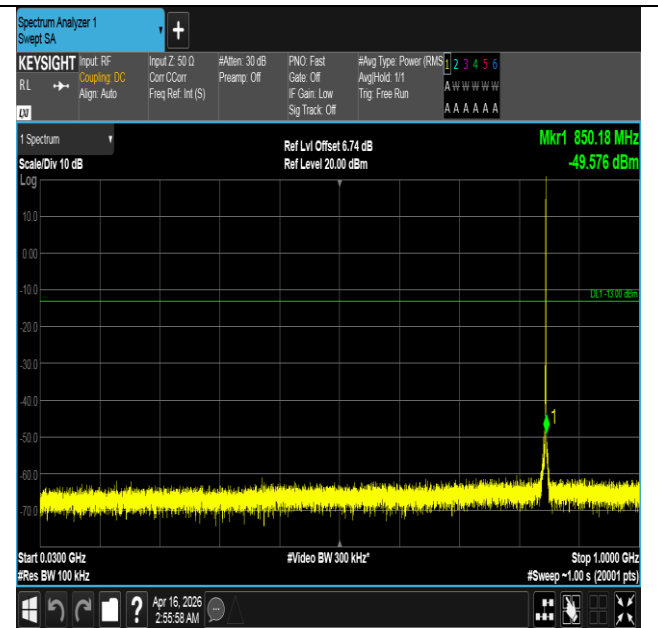
Band5-1.4MHz-QPSK-20643-1RB#5-30~1000-PASS
