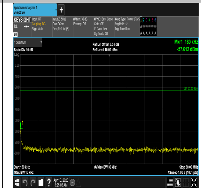
Band5-3MHz-QPSK-20415-15RB#0-0.15~30-PASS
