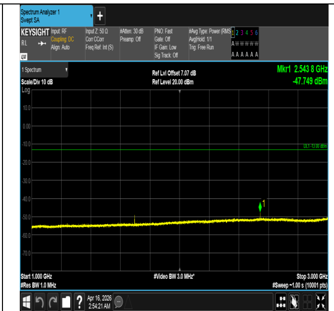
Band5-1.4MHz-QPSK-20643-1RB#0-1000~3000-PASS
