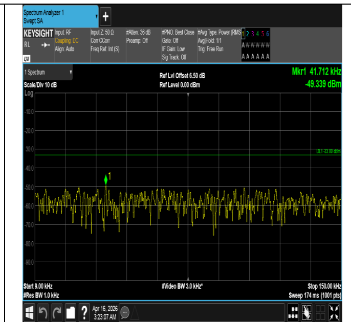
Band5-3MHz-QPSK-20415-1RB#14-0.009~0.15-PASS
