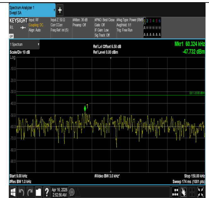
Band5-1.4MHz-16QAM-20525-6RB#0-0.009~0.15-PASS
