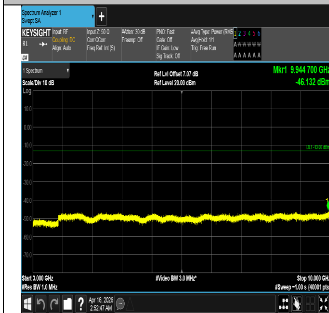
Band5-1.4MHz-QPSK-20525-6RB#0-3000~10000-PASS
