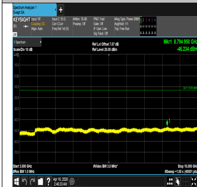
Band5-1.4MHz-16QAM-20407-1RB#5-3000~10000-PASS
