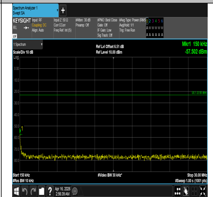
Band5-1.4MHz-16QAM-20643-1RB#5-0.15~30-PASS
