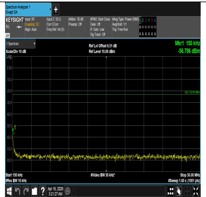
Band5-3MHz-QPSK-20415-1RB#0-0.15~30-PASS
