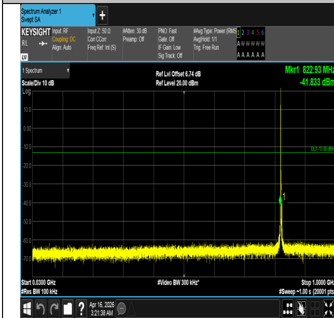
Band5-3MHz-QPSK-20415-1RB#0-30~1000-PASS
