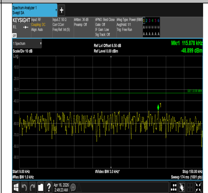
Band5-1.4MHz-16QAM-20525-1RB#0-0.009~0.15-PASS
