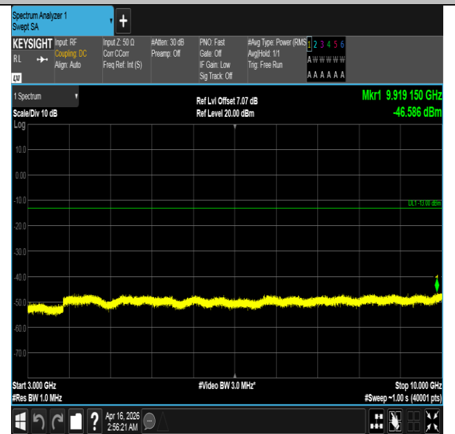
Band5-1.4MHz-QPSK-20643-1RB#5-3000~10000-PASS
