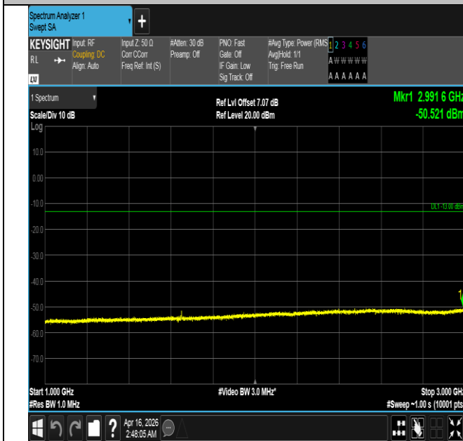
Band5-1.4MHz-16QAM-20407-6RB#0-1000~3000-PASS
