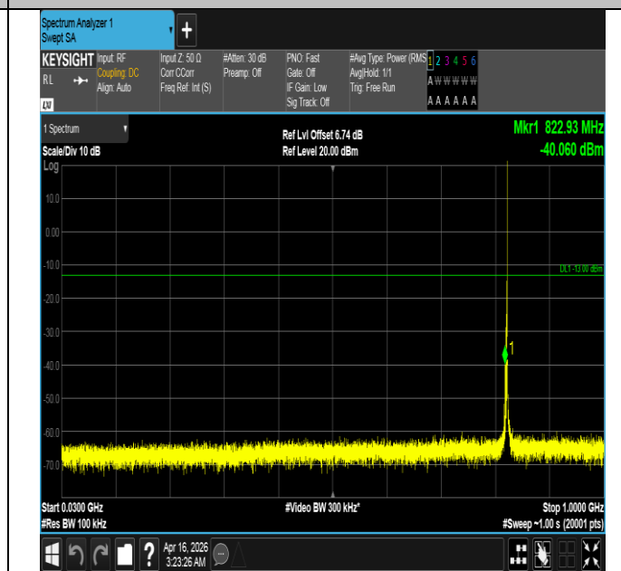
Band5-3MHz-QPSK-20415-1RB#14-30~1000-PASS
