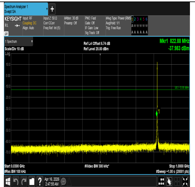
Band5-1.4MHz-16QAM-20407-6RB#0-30~1000-PASS
