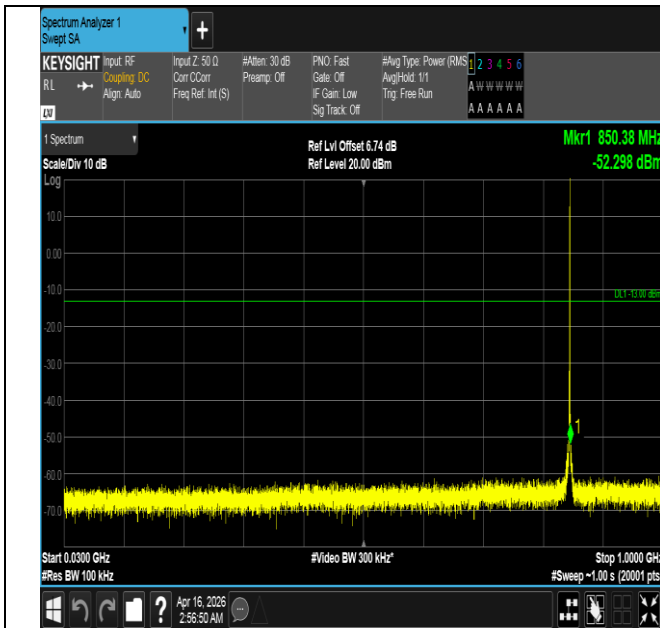
Band5-1.4MHz-16QAM-20643-1RB#5-30~1000-PASS
