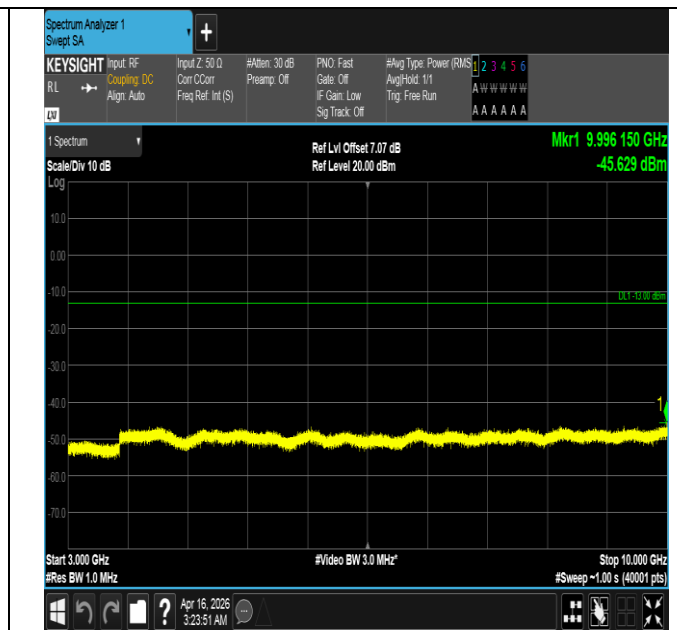
Band5-3MHz-QPSK-20415-1RB#14-3000~10000-PASS
