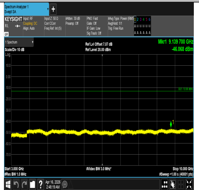
Band5-1.4MHz-16QAM-20407-6RB#0-3000~10000-PASS
