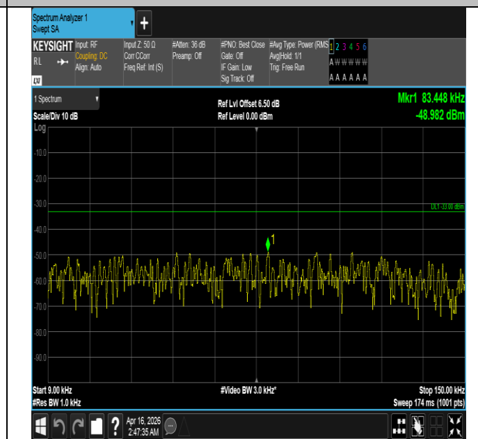
Band5-1.4MHz-16QAM-20407-6RB#0-0.009~0.15-PASS
