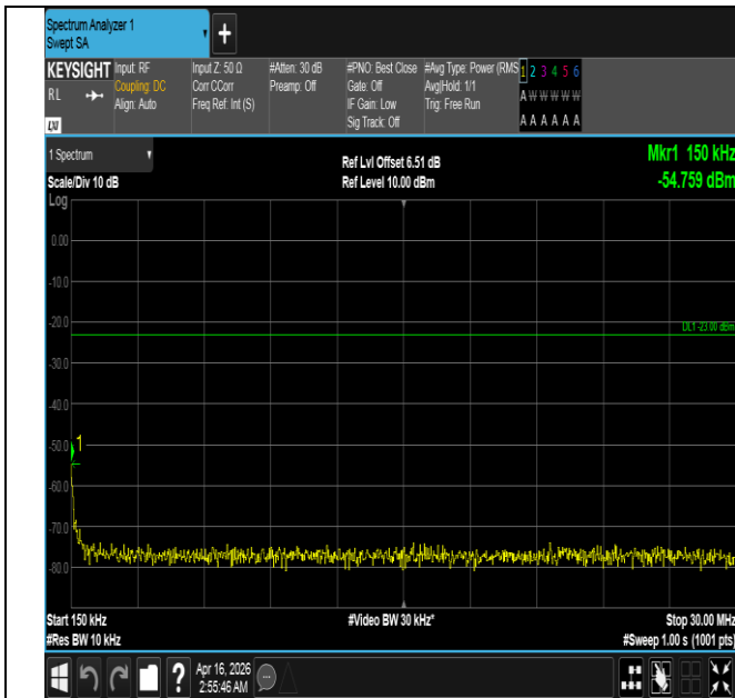
Band5-1.4MHz-QPSK-20643-1RB#5-0.15~30-PASS
