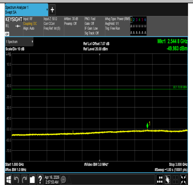
Band5-1.4MHz-QPSK-20643-6RB#0-1000~3000-PASS
