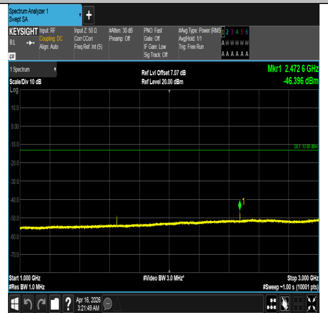
Band5-3MHz-QPSK-20415-1RB#0-1000~3000-PASS
