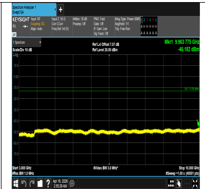
Band5-1.4MHz-16QAM-20643-1RB#0-3000~10000-PASS
