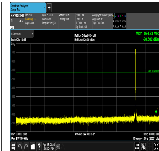
Band5-1.4MHz-QPSK-20525-6RB#0-30~1000-PASS
