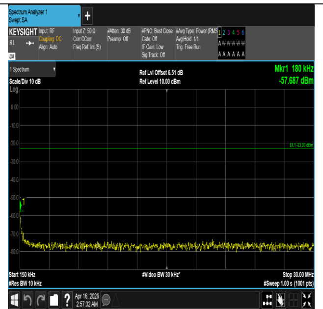
Band5-1.4MHz-QPSK-20643-6RB#0-0.15~30-PASS
