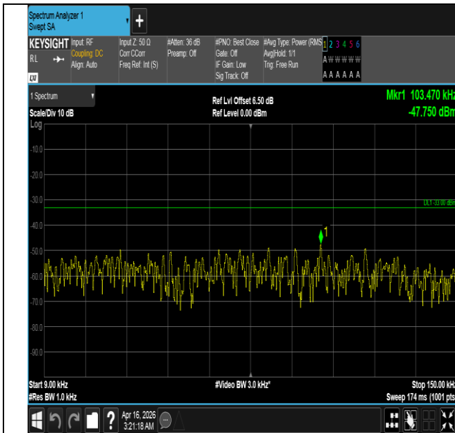
Band5-3MHz-QPSK-20415-1RB#0-0.009~0.15-PASS
