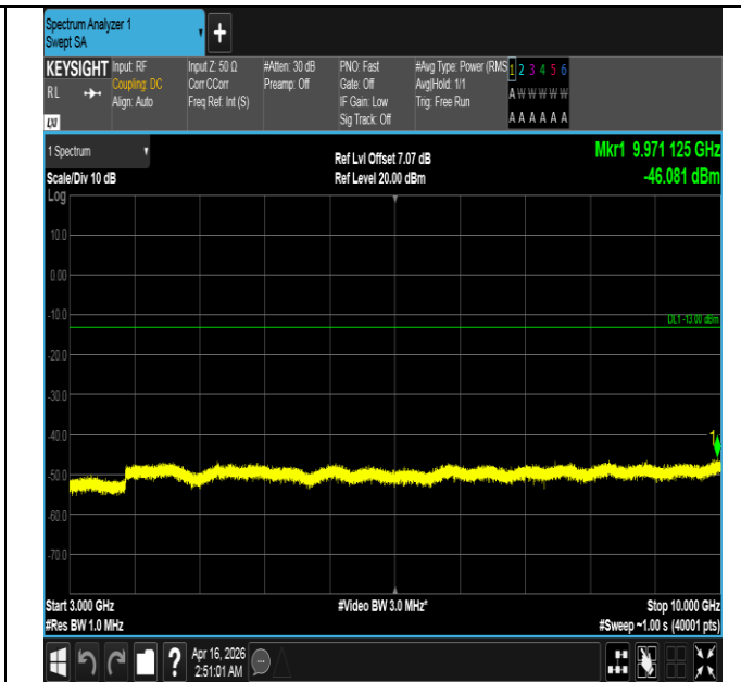
Band5-1.4MHz-QPSK-20525-1RB#5-3000~10000-PASS
