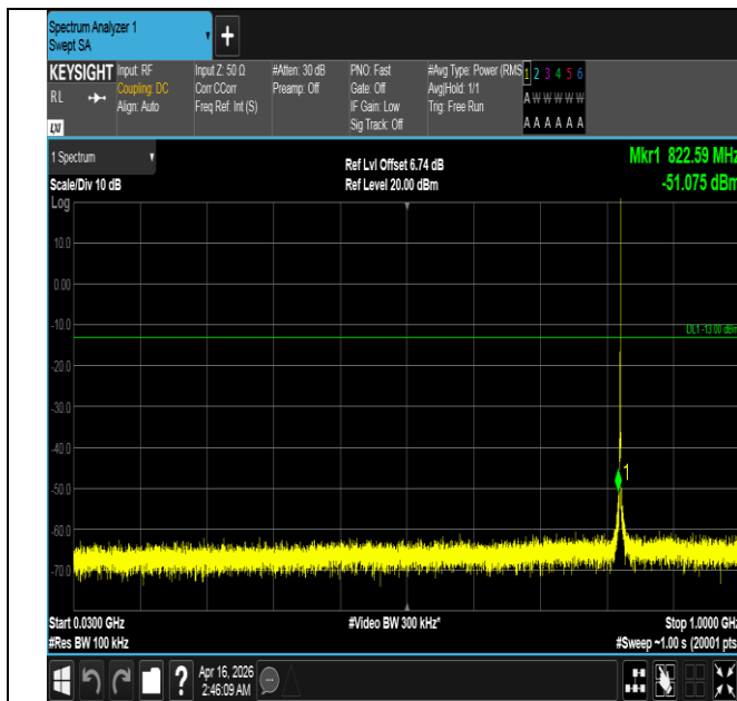
Band5-1.4MHz-16QAM-20407-1RB#5-30~1000-PASS
