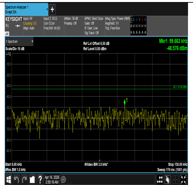
Band5-1.4MHz-QPSK-20525-1RB#5-0.009~0.15-PASS
