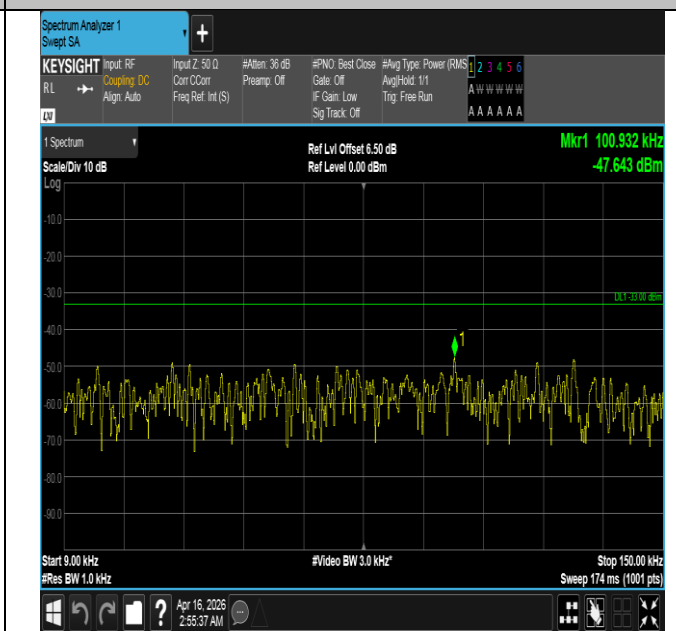
Band5-1.4MHz-QPSK-20643-1RB#5-0.009~0.15-PASS
