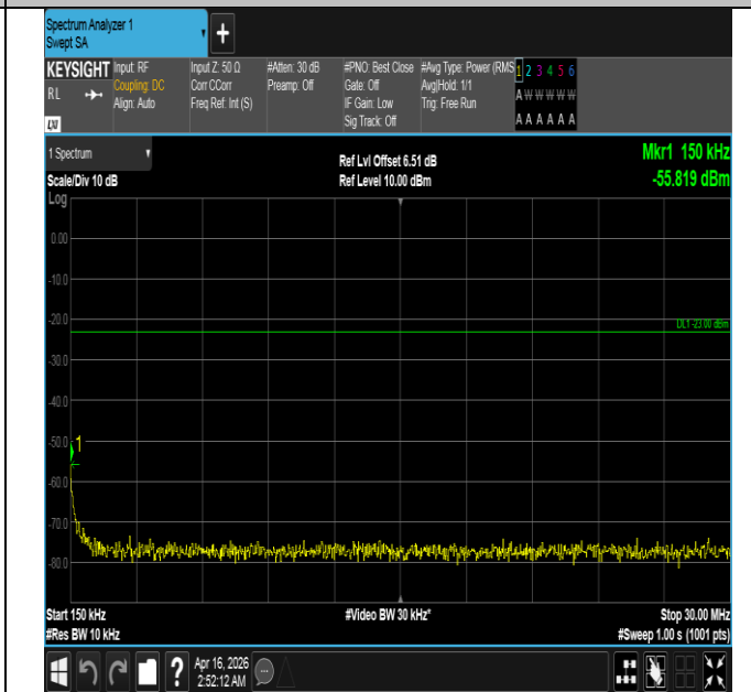
Band5-1.4MHz-QPSK-20525-6RB#0-0.15~30-PASS
