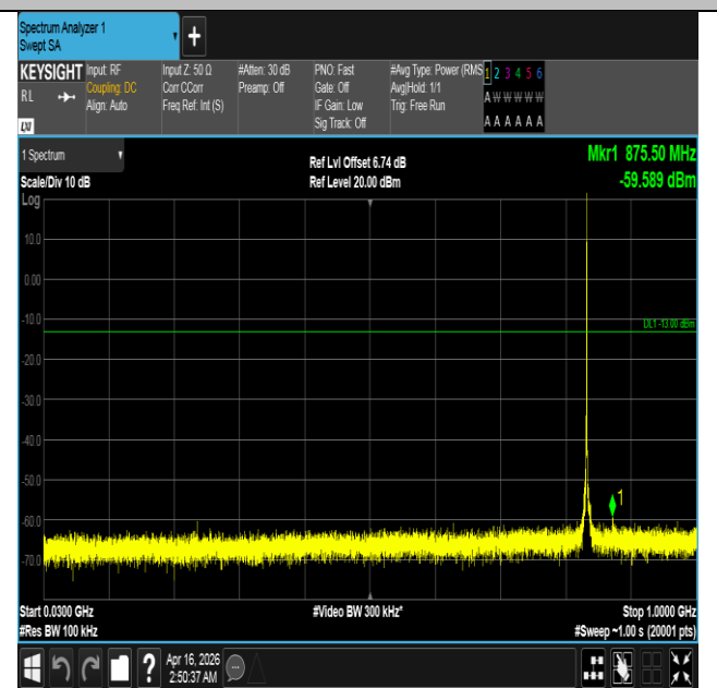
Band5-1.4MHz-QPSK-20525-1RB#5-30~1000-PASS
