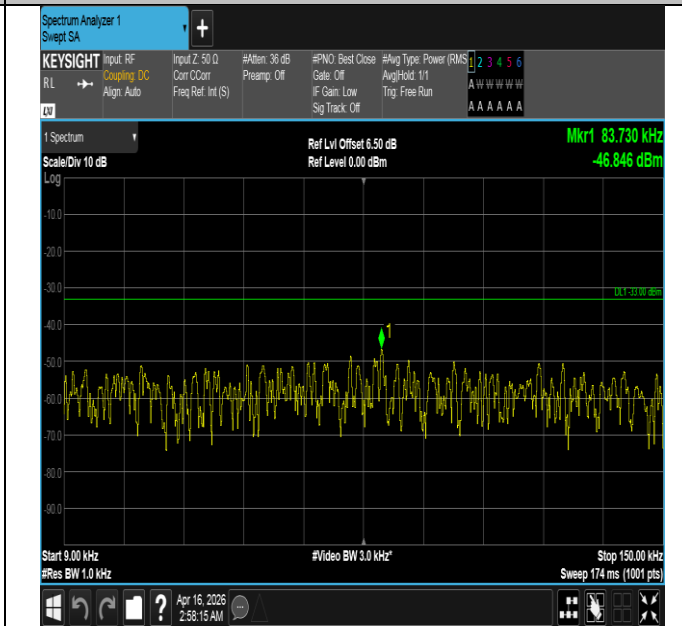
Band5-1.4MHz-16QAM-20643-6RB#0-0.009~0.15-PASS
