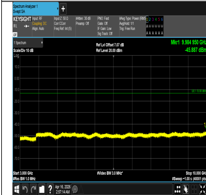
Band5-1.4MHz-16QAM-20643-1RB#5-3000~10000-PASS
