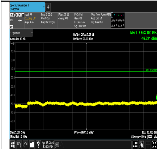
Band5-3MHz-QPSK-20635-15RB#0-3000~10000-PASS
