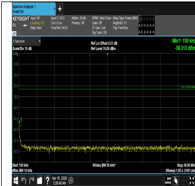
Band5-3MHz-QPSK-20525-1RB#14-0.15~30-PASS
