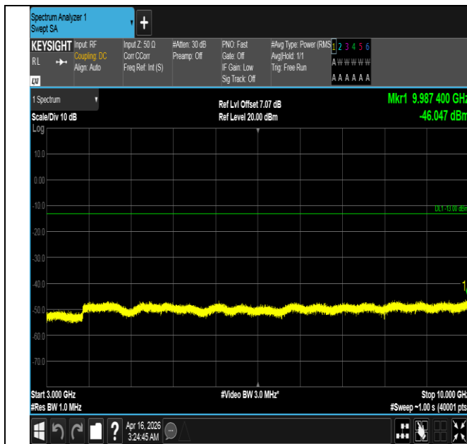
Band5-3MHz-16QAM-20415-1RB#14-3000~10000-PASS
