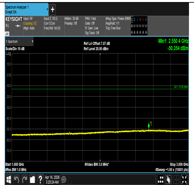
Band5-3MHz-QPSK-20415-15RB#0-1000~3000-PASS
