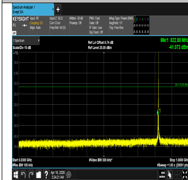
Band5-3MHz-16QAM-20415-1RB#14-30~1000-PASS
