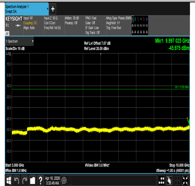
Band5-3MHz-16QAM-20635-1RB#0-3000~10000-PASS
