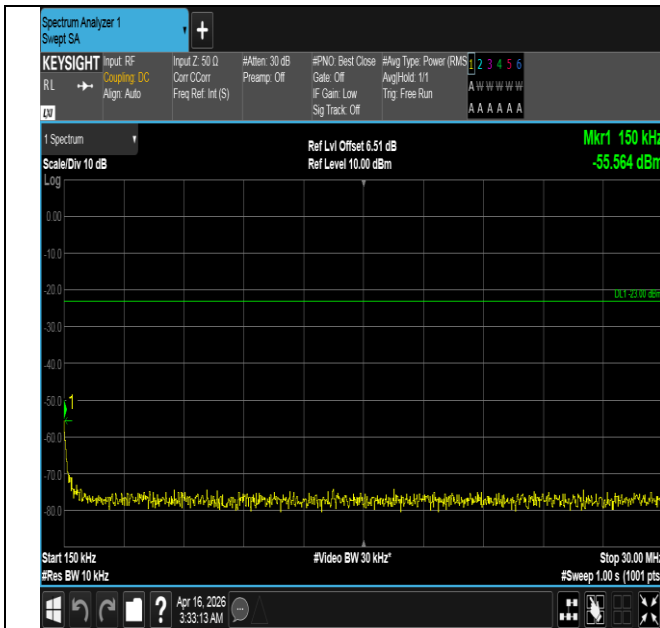
Band5-3MHz-16QAM-20635-1RB#0-0.15~30-PASS
