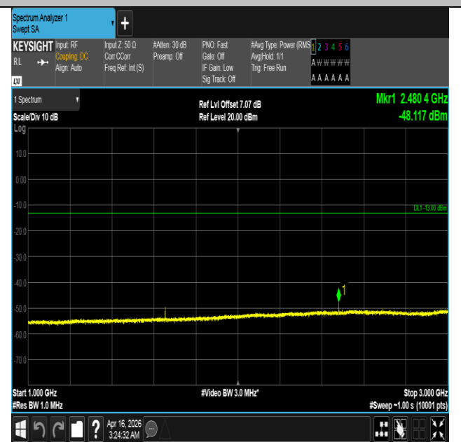
Band5-3MHz-16QAM-20415-1RB#14-1000~3000-PASS
