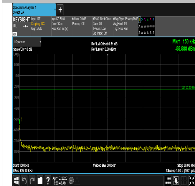
Band5-3MHz-16QAM-20635-15RB#0-0.15~30-PASS
