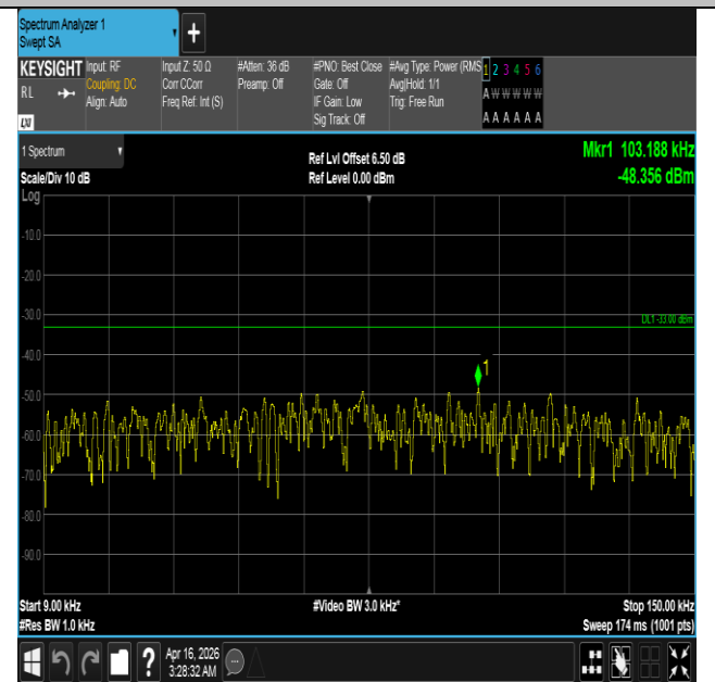
Band5-3MHz-QPSK-20525-1RB#14-0.009~0.15-PASS
