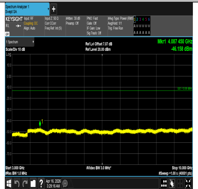
Band5-3MHz-QPSK-20525-1RB#14-3000~10000-PASS
