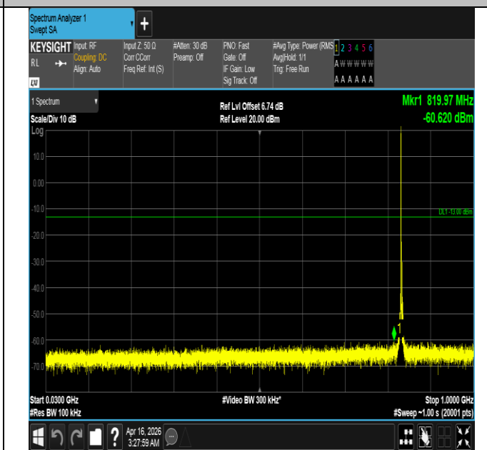
Band5-3MHz-16QAM-20525-1RB#0-30~1000-PASS
