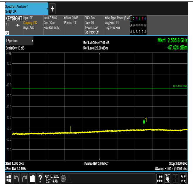
Band5-3MHz-QPSK-20525-1RB#0-1000~3000-PASS
