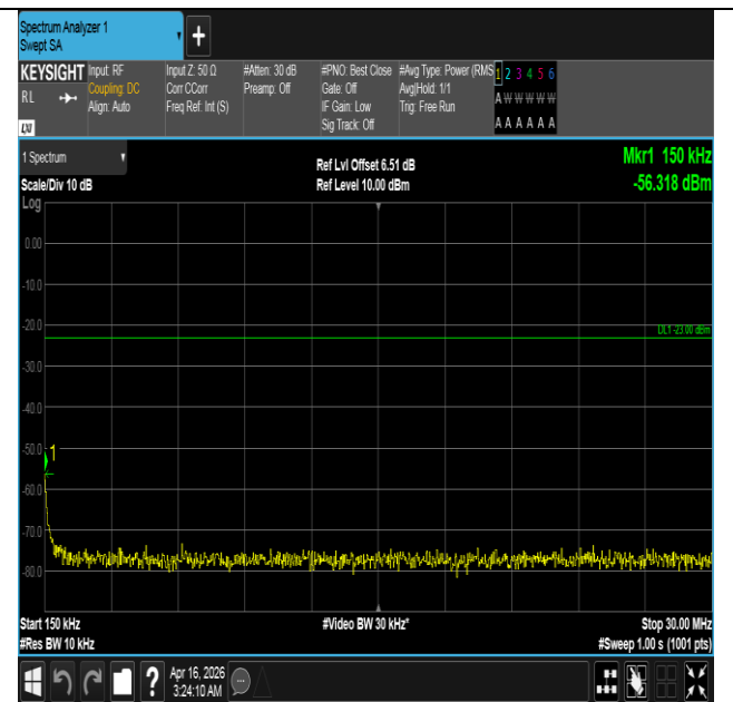
Band5-3MHz-16QAM-20415-1RB#14-0.15~30-PASS
