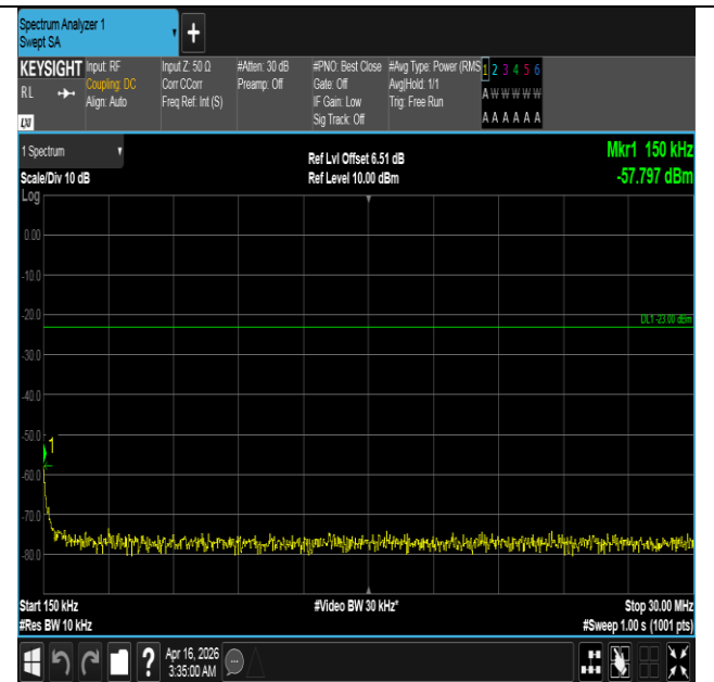
Band5-3MHz-16QAM-20635-1RB#14-0.15~30-PASS
