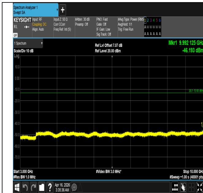
Band5-3MHz-16QAM-20635-1RB#14-3000~10000-PASS
