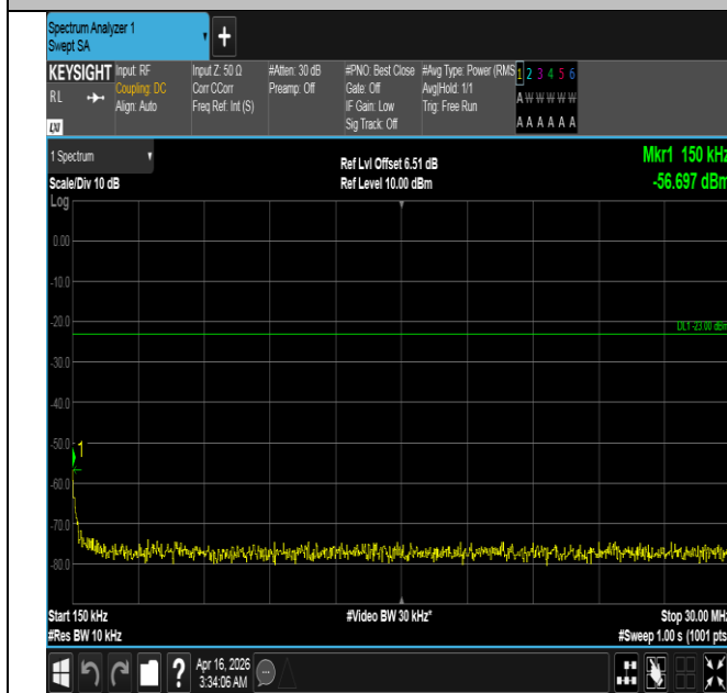
Band5-3MHz-QPSK-20635-1RB#14-0.15~30-PASS
