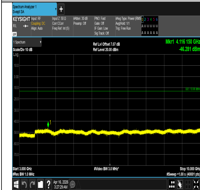
Band5-3MHz-QPSK-20525-1RB#0-3000~10000-PASS
