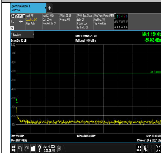
Band5-3MHz-16QAM-20415-15RB#0-0.15~30-PASS
