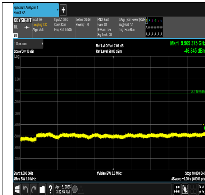
Band5-3MHz-QPSK-20635-1RB#0-3000~10000-PASS
