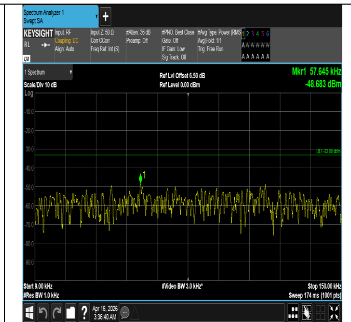
Band5-3MHz-16QAM-20635-15RB#0-0.009~0.15-PASS
