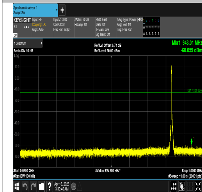
Band5-3MHz-QPSK-20525-15RB#0-30~1000-PASS
