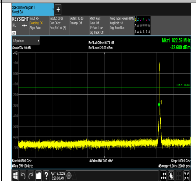
Band5-3MHz-16QAM-20415-15RB#0-30~1000-PASS
