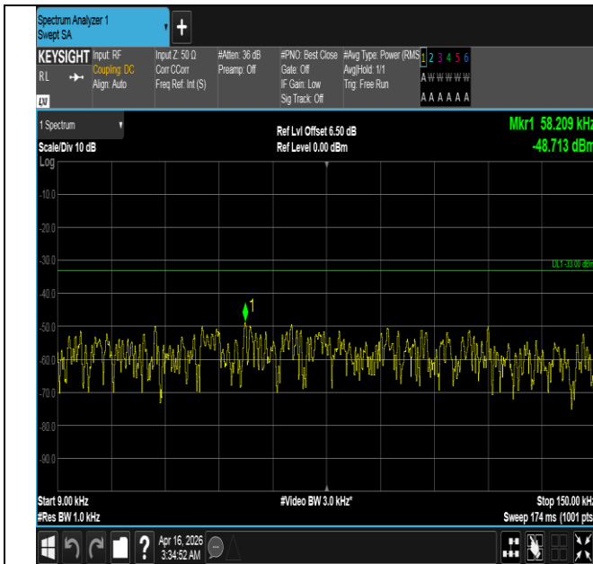
Band5-3MHz-16QAM-20635-1RB#14-0.009~0.15-PASS
