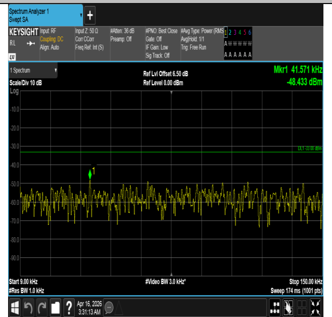
Band5-3MHz-16QAM-20525-15RB#0-0.009~0.15-PASS
