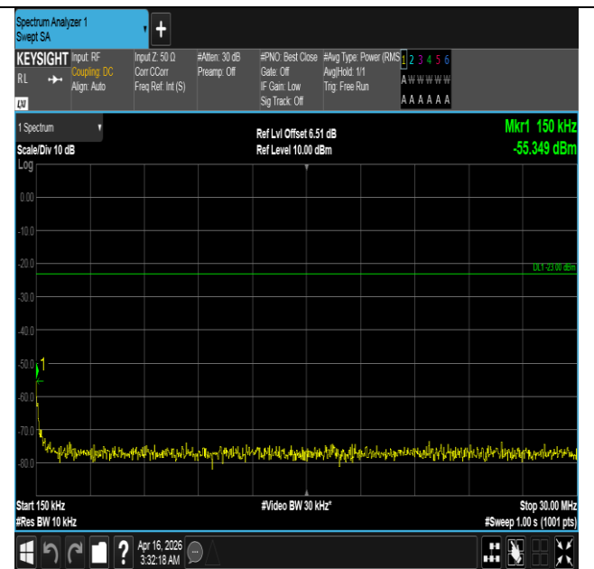
Band5-3MHz-QPSK-20635-1RB#0-0.15~30-PASS
