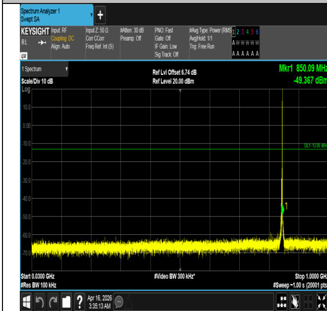
Band5-3MHz-16QAM-20635-1RB#14-30~1000-PASS
