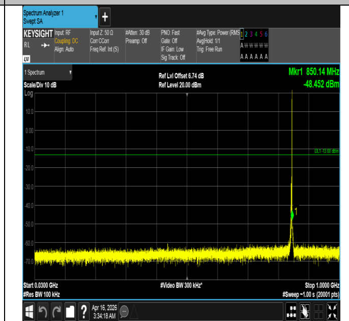
Band5-3MHz-QPSK-20635-1RB#14-30~1000-PASS
