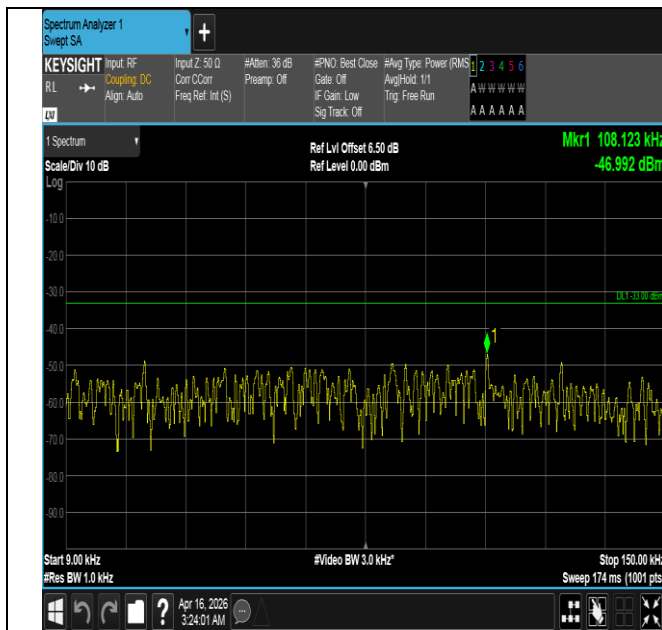
Band5-3MHz-16QAM-20415-1RB#14-0.009~0.15-PASS
