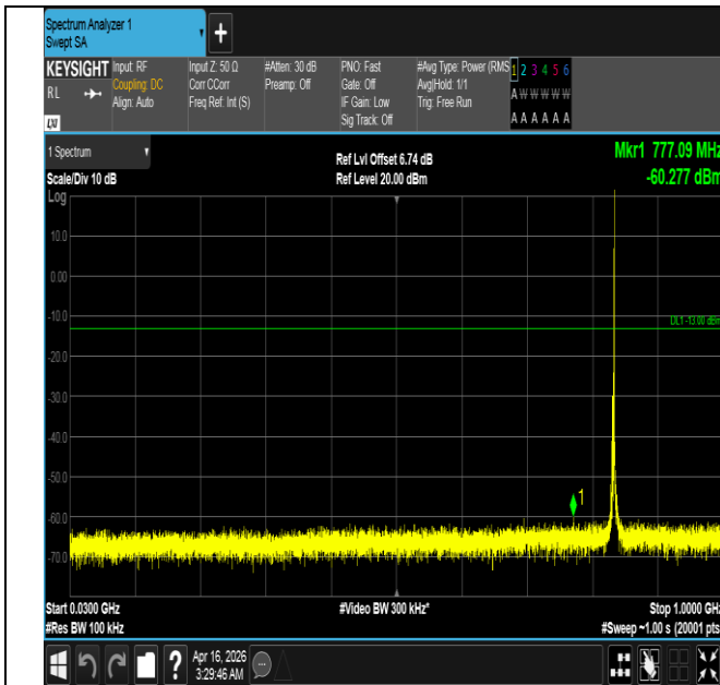
Band5-3MHz-16QAM-20525-1RB#14-30~1000-PASS
