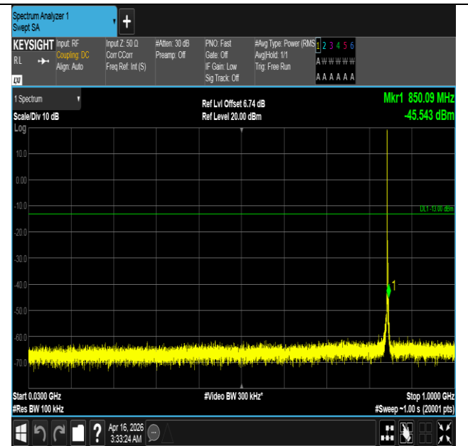
Band5-3MHz-16QAM-20635-1RB#0-30~1000-PASS
