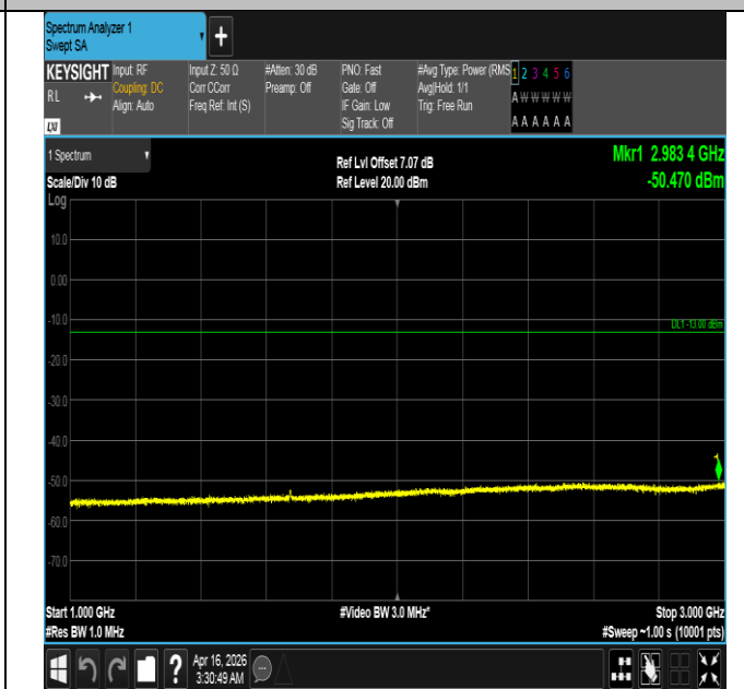
Band5-3MHz-QPSK-20525-15RB#0-1000~3000-PASS
