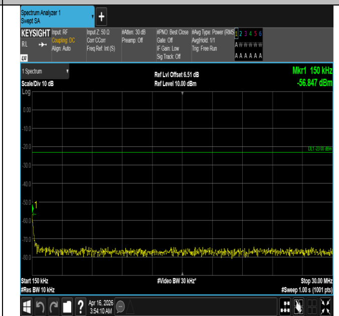
Band5-5MHz-QPSK-20425-1RB#0-0.15~30-PASS
