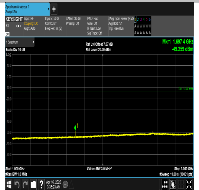
Band5-3MHz-16QAM-20635-1RB#14-1000~3000-PASS
