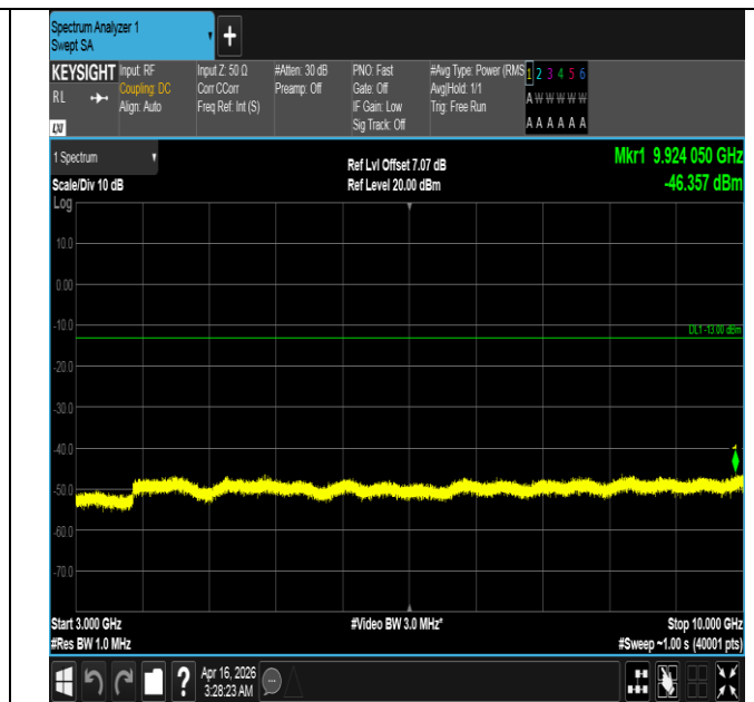
Band5-3MHz-16QAM-20525-1RB#0-3000~10000-PASS
