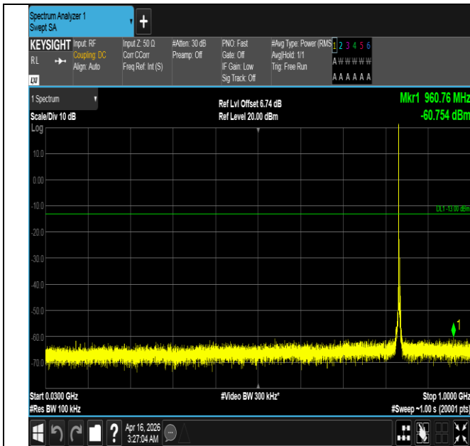
Band5-3MHz-QPSK-20525-1RB#0-30~1000-PASS
