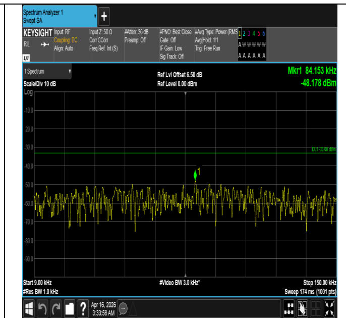
Band5-3MHz-QPSK-20635-1RB#14-0.009~0.15-PASS
