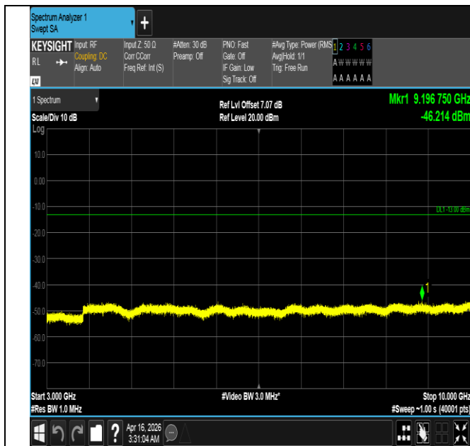
Band5-3MHz-QPSK-20525-15RB#0-3000~10000-PASS
