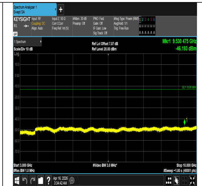
Band5-3MHz-QPSK-20635-1RB#14-3000~10000-PASS
