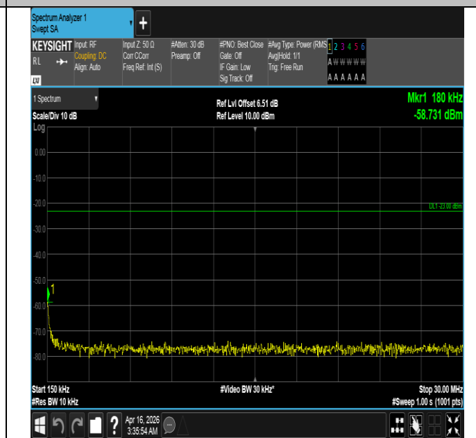
Band5-3MHz-QPSK-20635-15RB#0-0.15~30-PASS
