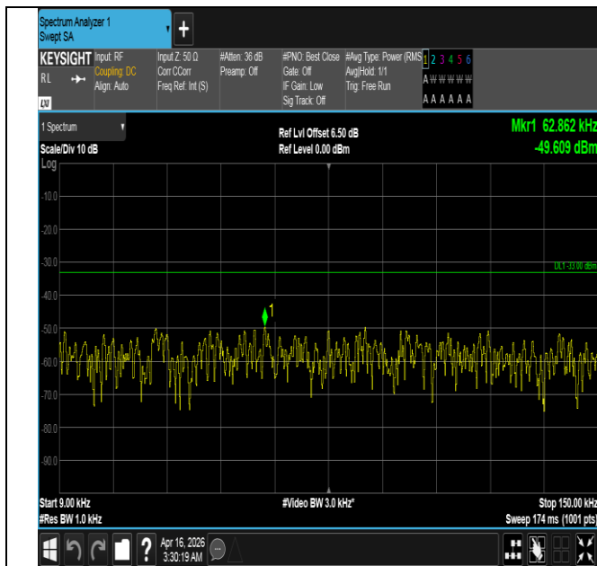
Band5-3MHz-QPSK-20525-15RB#0-0.009~0.15-PASS
