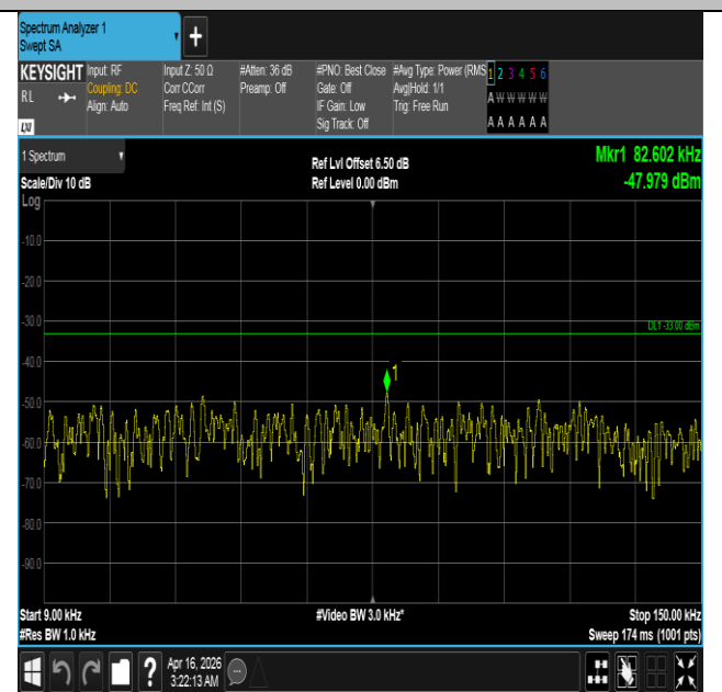
Band5-3MHz-16QAM-20415-1RB#0-0.009~0.15-PASS
