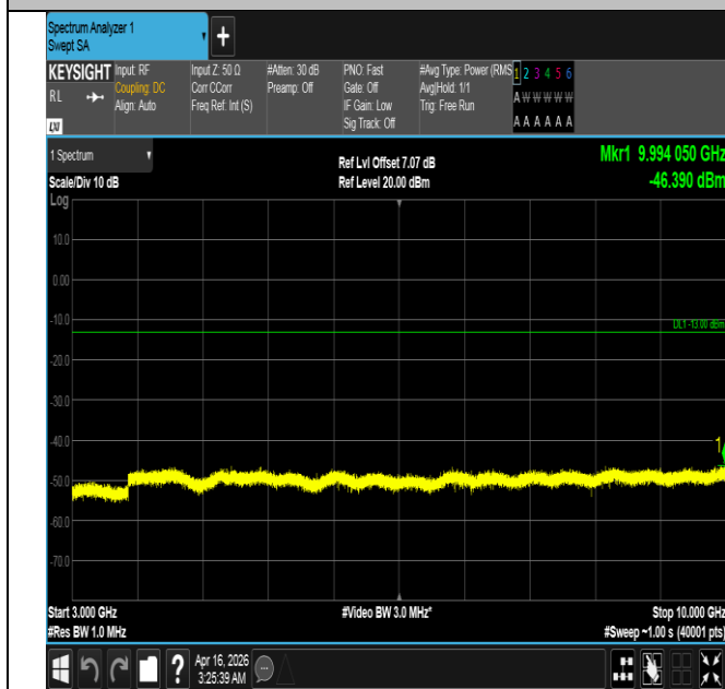
Band5-3MHz-QPSK-20415-15RB#0-3000~10000-PASS
