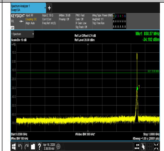
Band5-3MHz-16QAM-20635-15RB#0-30~1000-PASS
