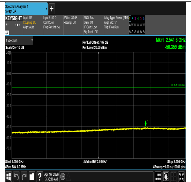
Band5-3MHz-QPSK-20635-15RB#0-1000~3000-PASS
