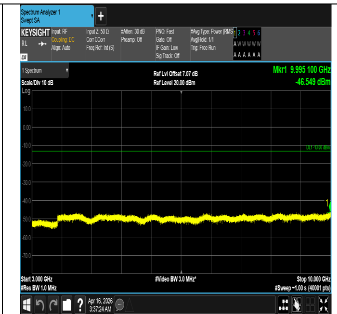
Band5-3MHz-16QAM-20635-15RB#0-3000~10000-PASS
