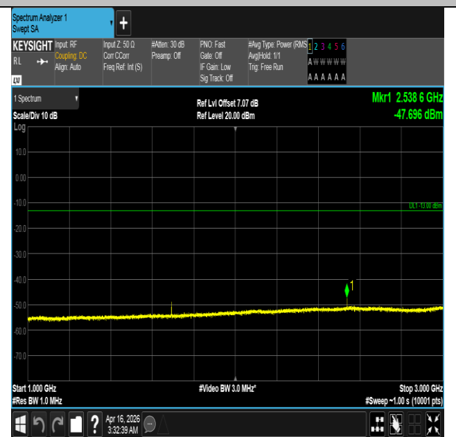
Band5-3MHz-QPSK-20635-1RB#0-1000~3000-PASS
