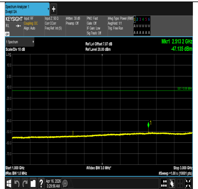
Band5-3MHz-16QAM-20525-1RB#14-1000~3000-PASS
