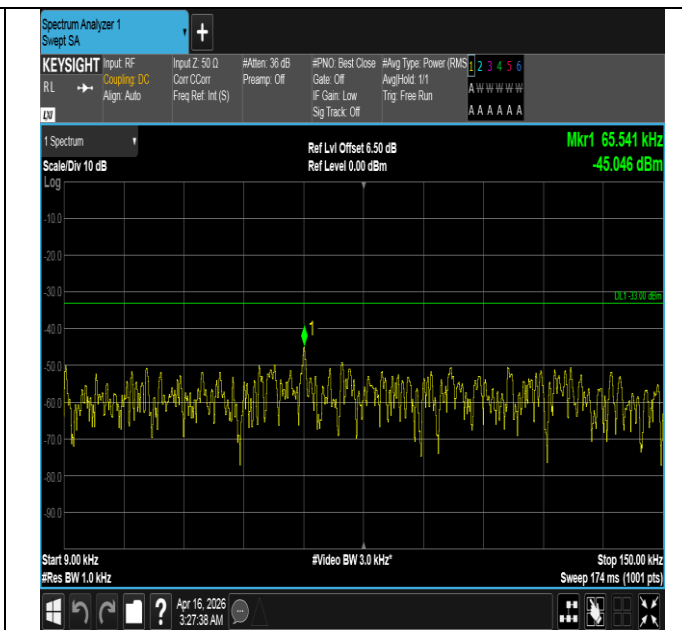
Band5-3MHz-16QAM-20525-1RB#0-0.009~0.15-PASS
