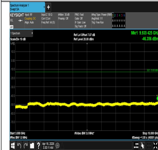
Band5-3MHz-16QAM-20525-1RB#14-3000~10000-PASS
