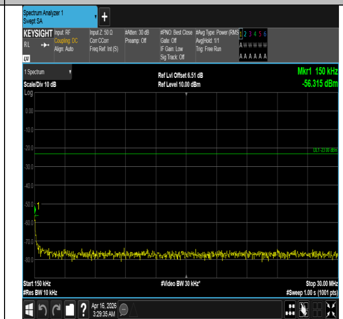
Band5-3MHz-16QAM-20525-1RB#14-0.15~30-PASS
