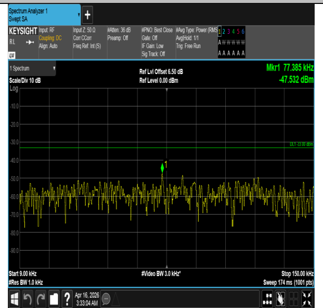
Band5-3MHz-16QAM-20635-1RB#0-0.009~0.15-PASS
