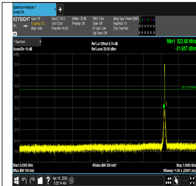
Band5-3MHz-QPSK-20415-15RB#0-30~1000-PASS
