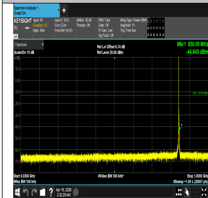
Band5-3MHz-QPSK-20635-1RB#0-30~1000-PASS
