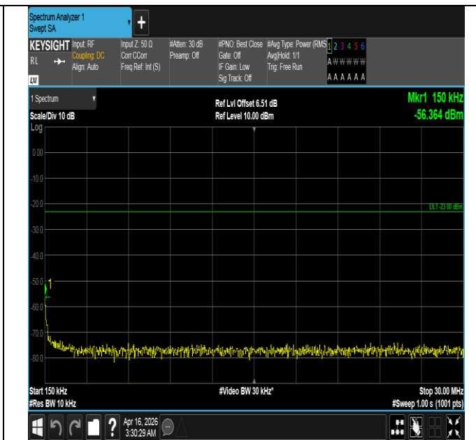
Band5-3MHz-QPSK-20525-15RB#0-0.15~30-PASS
