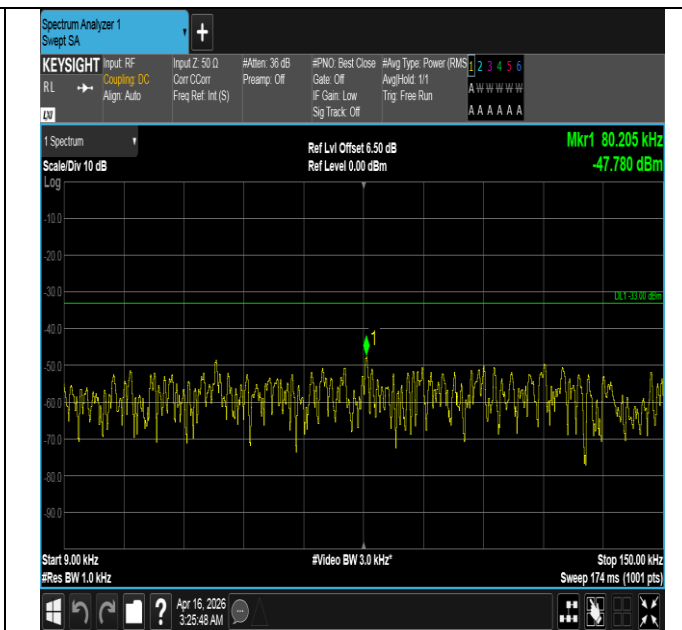
Band5-3MHz-16QAM-20415-15RB#0-0.009~0.15-PASS
