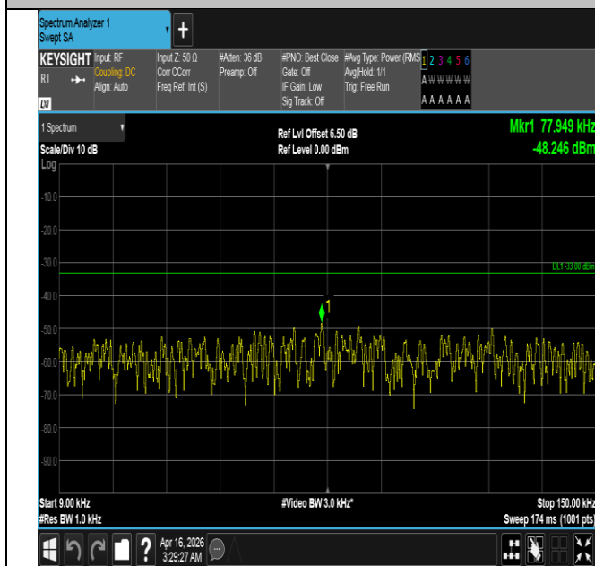
Band5-3MHz-16QAM-20525-1RB#14-0.009~0.15-PASS
