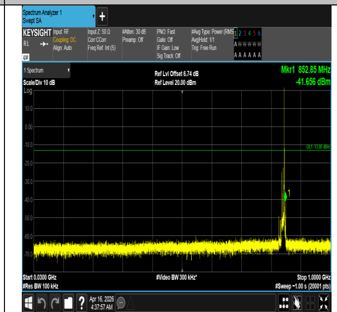
Band5-10MHz-QPSK-20600-1RB#49-30~1000-PASS
