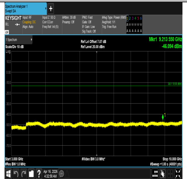
Band5-10MHz-QPSK-20525-1RB#49-3000~10000-PASS
