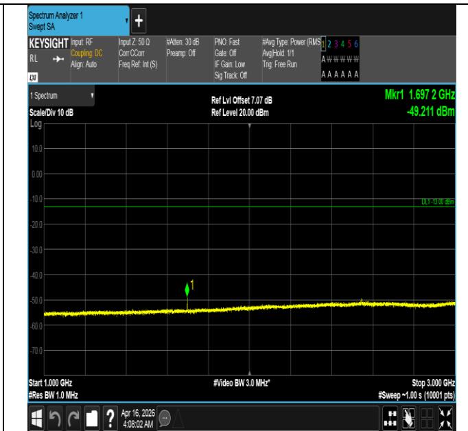
Band5-5MHz-16QAM-20625-1RB#24-1000~3000-PASS
