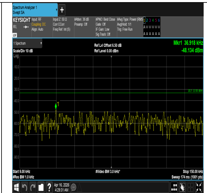
Band5-10MHz-16QAM-20450-50RB#0-0.009~0.15-PASS
