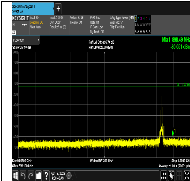
Band5-10MHz-QPSK-20525-1RB#0-30~1000-PASS
