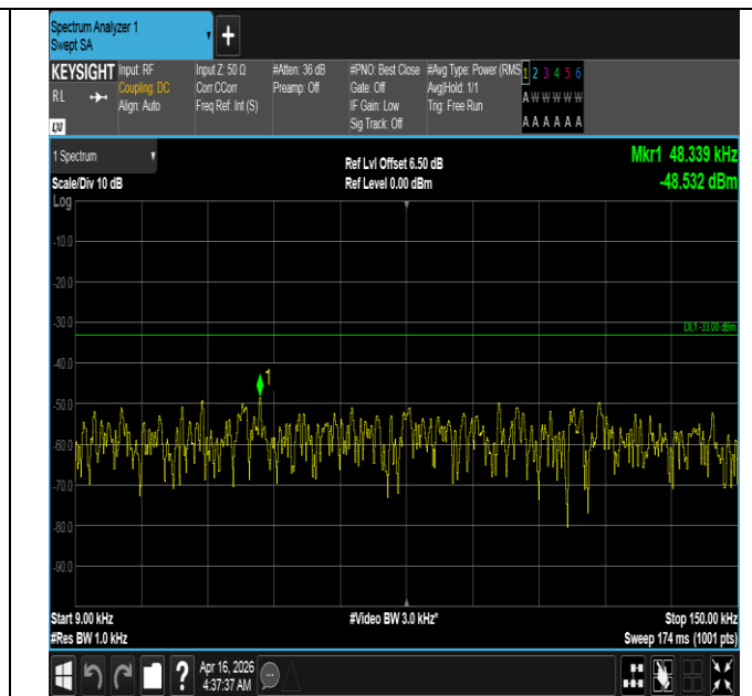
Band5-10MHz-QPSK-20600-1RB#49-0.009~0.15-PASS
