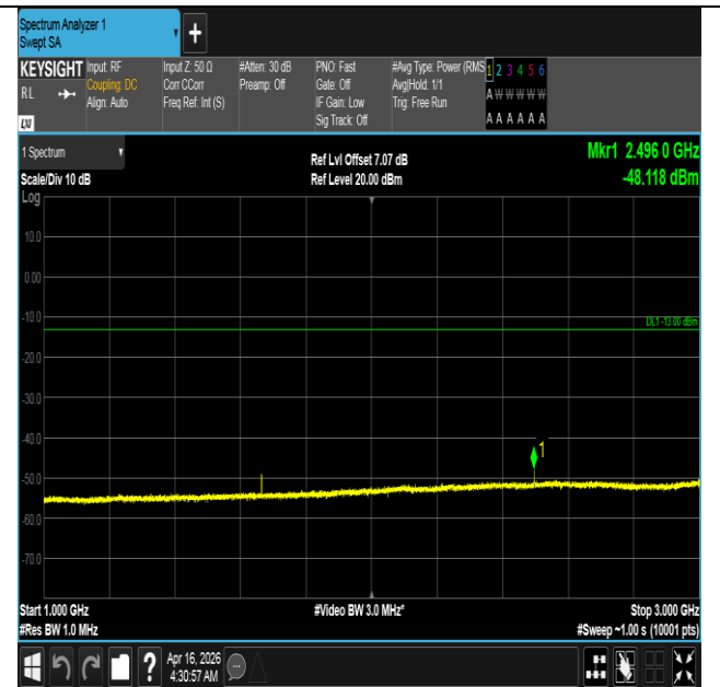
Band5-10MHz-QPSK-20525-1RB#0-1000~3000-PASS
