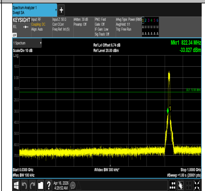
Band5-10MHz-16QAM-20450-50RB#0-30~1000-PASS
