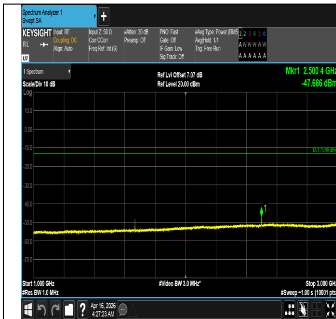
Band5-10MHz-QPSK-20450-1RB#49-1000~3000-PASS
