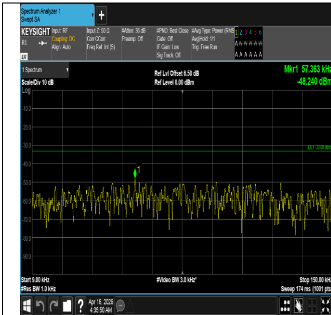
Band5-10MHz-QPSK-20600-1RB#0-0.009~0.15-PASS
