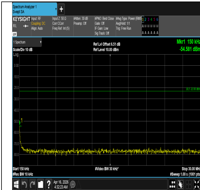
Band5-10MHz-QPSK-20525-1RB#49-0.15~30-PASS
