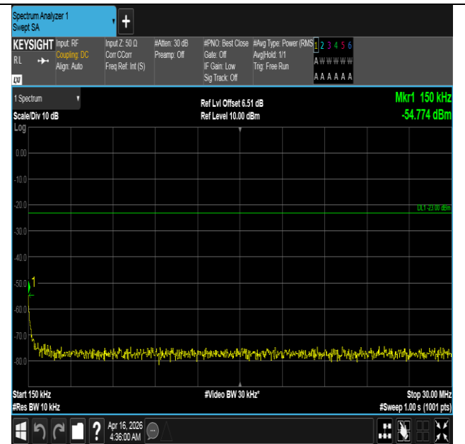
Band5-10MHz-QPSK-20600-1RB#0-0.15~30-PASS
