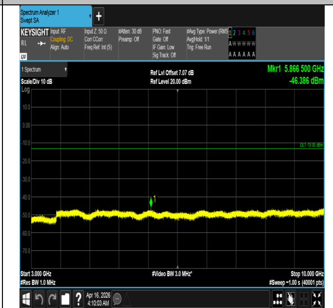
Band5-5MHz-16QAM-20625-25RB#0-3000~10000-PASS
