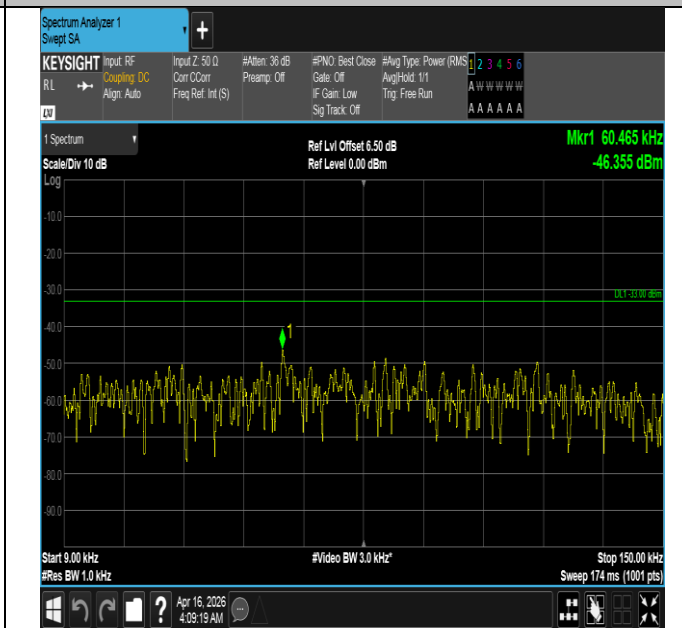
Band5-5MHz-16QAM-20625-25RB#0-0.009~0.15-PASS
