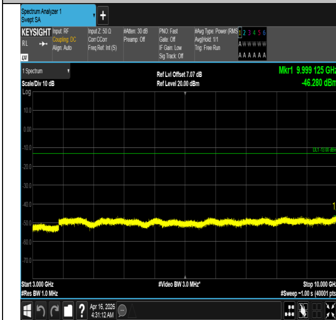
Band5-10MHz-QPSK-20525-1RB#0-3000~10000-PASS
