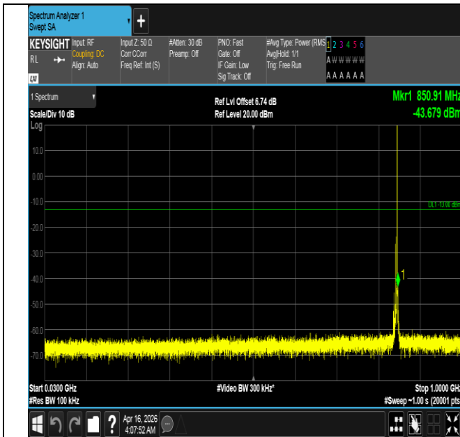
Band5-5MHz-16QAM-20625-1RB#24-30~1000-PASS
