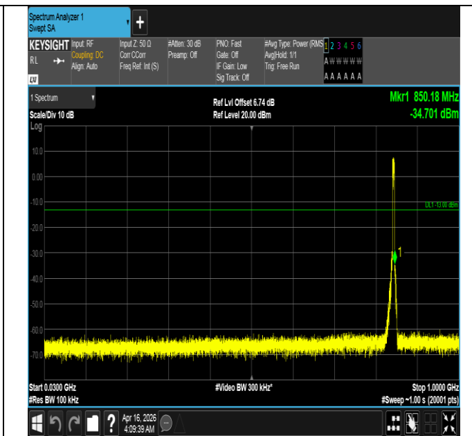
Band5-5MHz-16QAM-20625-25RB#0-30~1000-PASS
