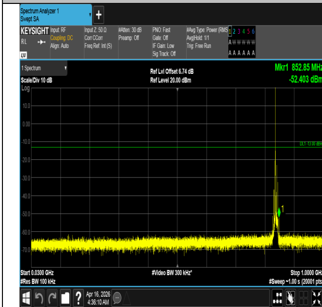
Band5-10MHz-QPSK-20600-1RB#0-30~1000-PASS
