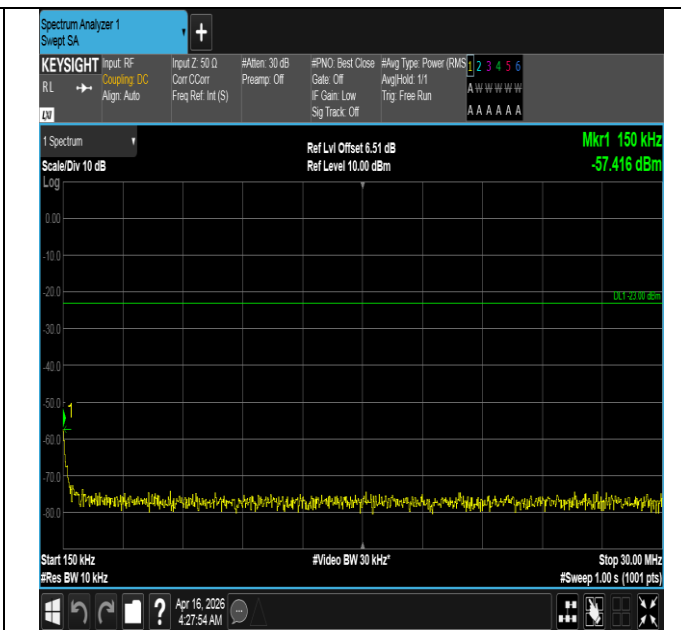
Band5-10MHz-16QAM-20450-1RB#49-0.15~30-PASS
