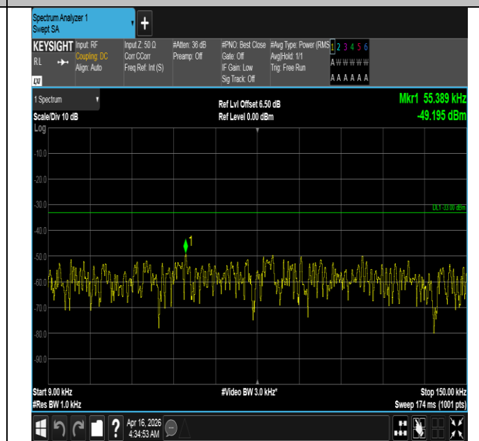
Band5-10MHz-16QAM-20525-50RB#0-0.009~0.15-PASS
