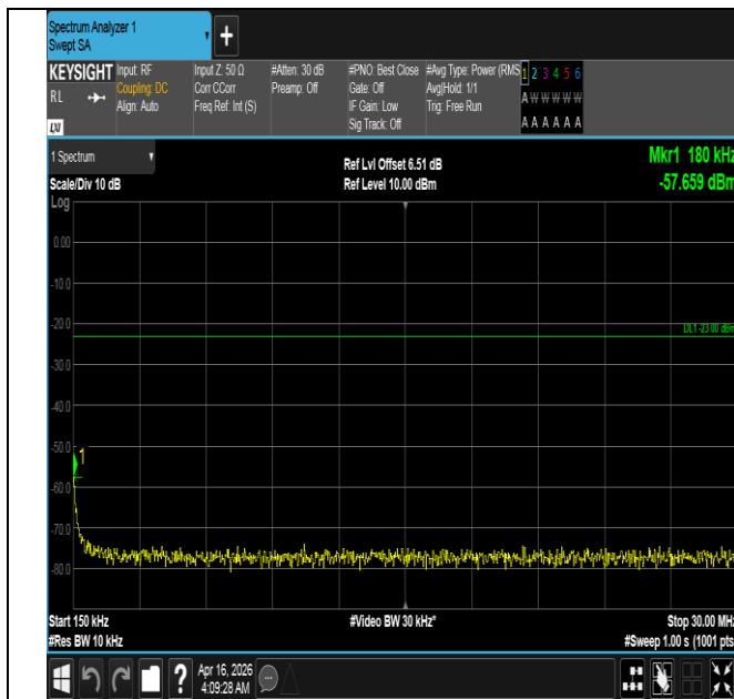
Band5-5MHz-16QAM-20625-25RB#0-0.15~30-PASS
