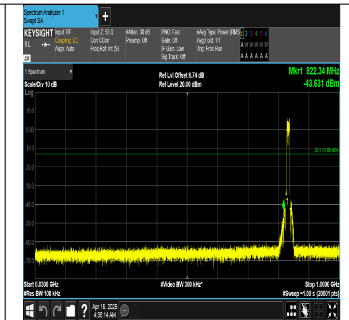
Band5-10MHz-16QAM-20525-50RB#0-30~1000-PASS
