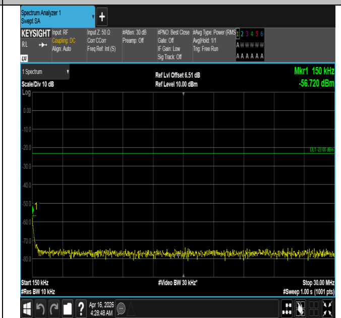
Band5-10MHz-QPSK-20450-50RB#0-0.15~30-PASS
