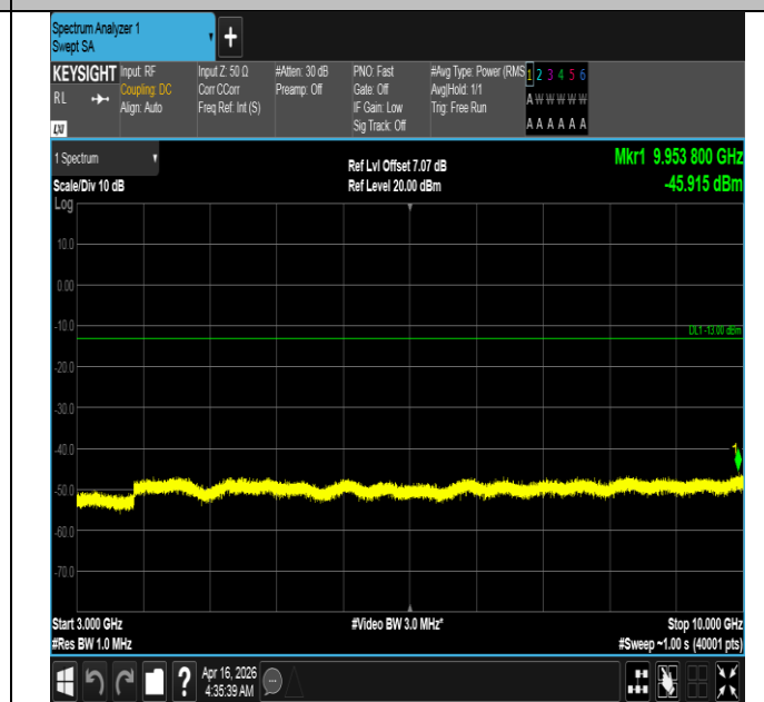
Band5-10MHz-16QAM-20525-50RB#0-3000~10000-PASS
