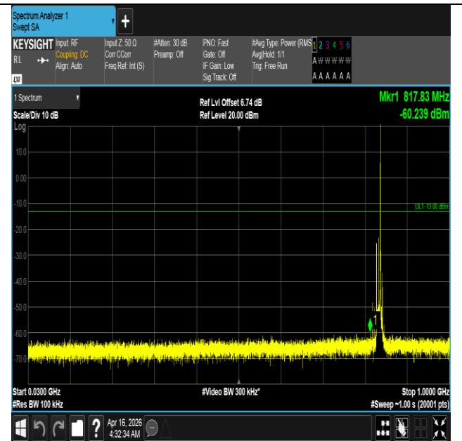
Band5-10MHz-QPSK-20525-1RB#49-30~1000-PASS
