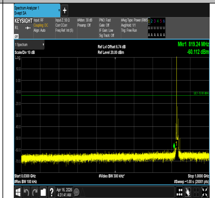
Band5-10MHz-16QAM-20525-1RB#0-30~1000-PASS
