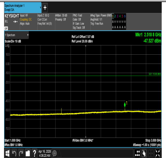
Band5-10MHz-QPSK-20600-1RB#0-1000~3000-PASS
