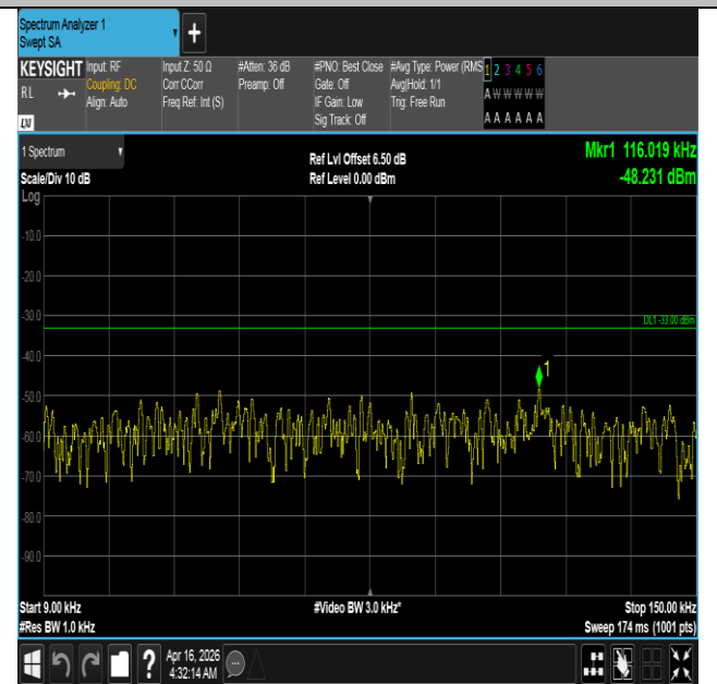
Band5-10MHz-QPSK-20525-1RB#49-0.009~0.15-PASS
