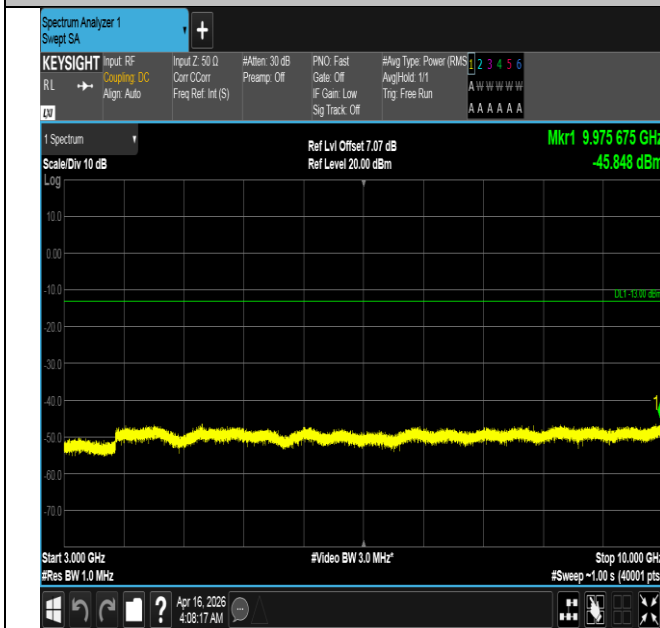
Band5-5MHz-16QAM-20625-1RB#24-3000~10000-PASS
