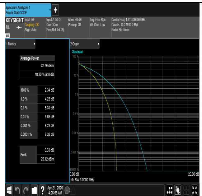
Band66-3MHz-QPSK-131987-15RB#0-PASS
