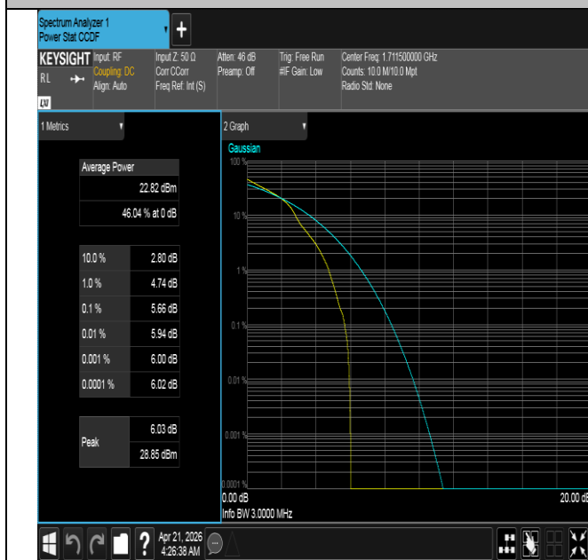
Band66-3MHz-16QAM-131987-1RB#0-PASS
