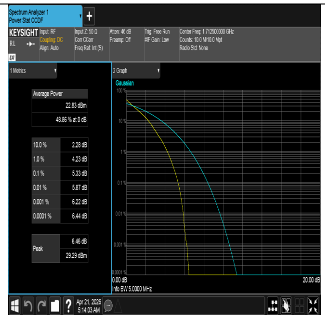
Band66-5MHz-QPSK-131997-25RB#0-PASS
