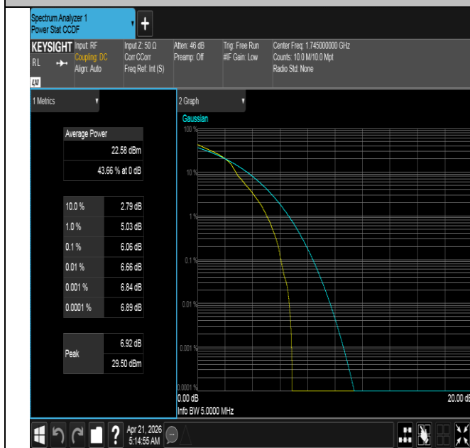
Band66-5MHz-16QAM-132322-1RB#0-PASS
