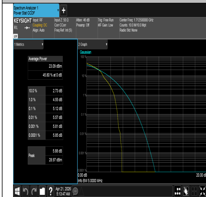
Band66-5MHz-16QAM-131997-1RB#0-PASS
