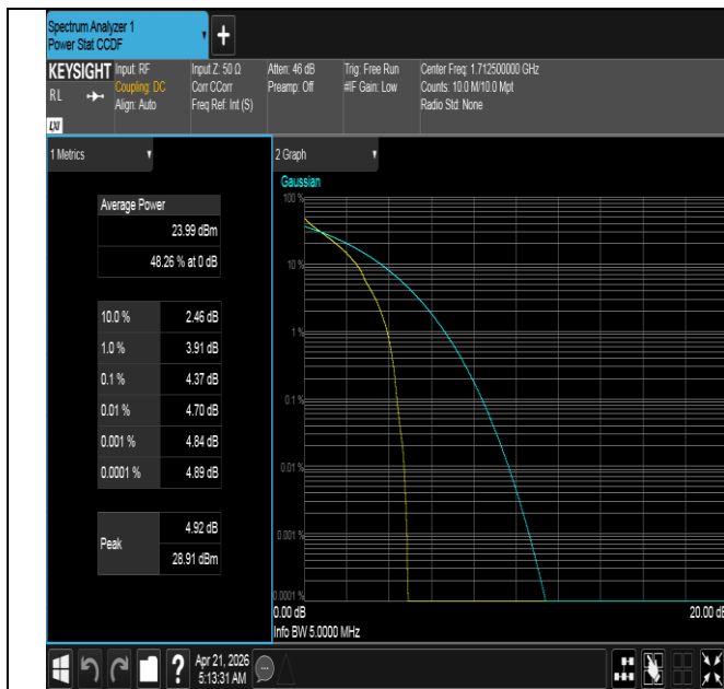
Band66-5MHz-QPSK-131997-1RB#0-PASS
