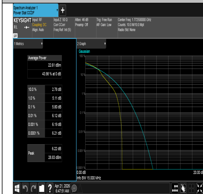
Band66-15MHz-16QAM-132597-1RB#0-PASS
