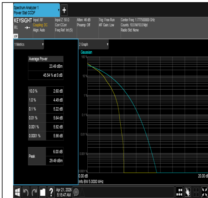
Band66-5MHz-QPSK-132647-1RB#0-PASS
