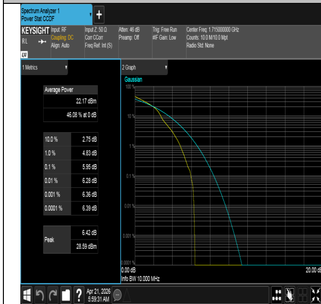
Band66-10MHz-16QAM-132022-1RB#0-PASS
