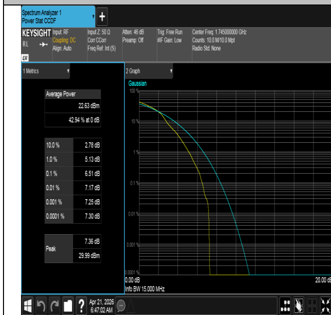
Band66-15MHz-16QAM-132322-1RB#0-PASS
