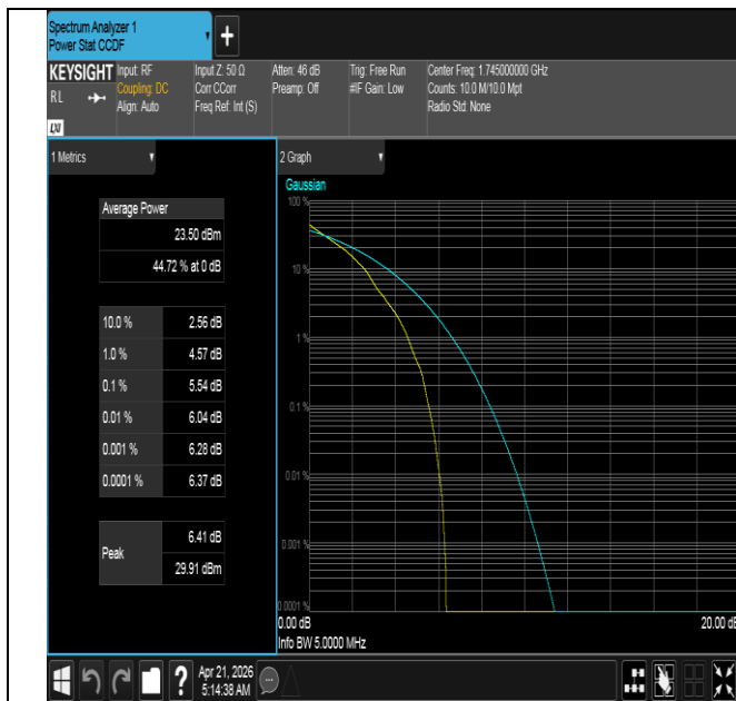
Band66-5MHz-QPSK-132322-1RB#0-PASS
