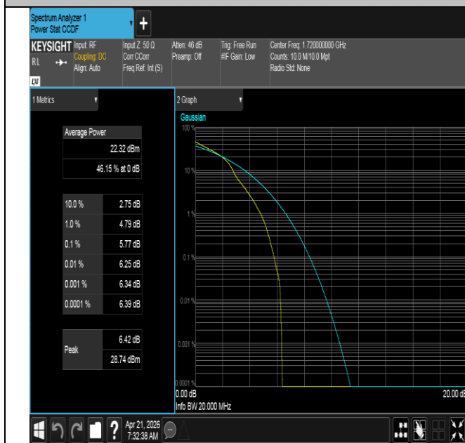
Band66-20MHz-16QAM-132072-1RB#0-PASS
