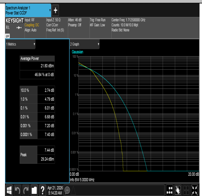
Band66-5MHz-16QAM-131997-25RB#0-PASS
