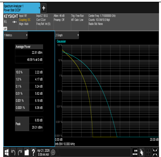
Band66-10MHz-QPSK-132022-50RB#0-PASS
