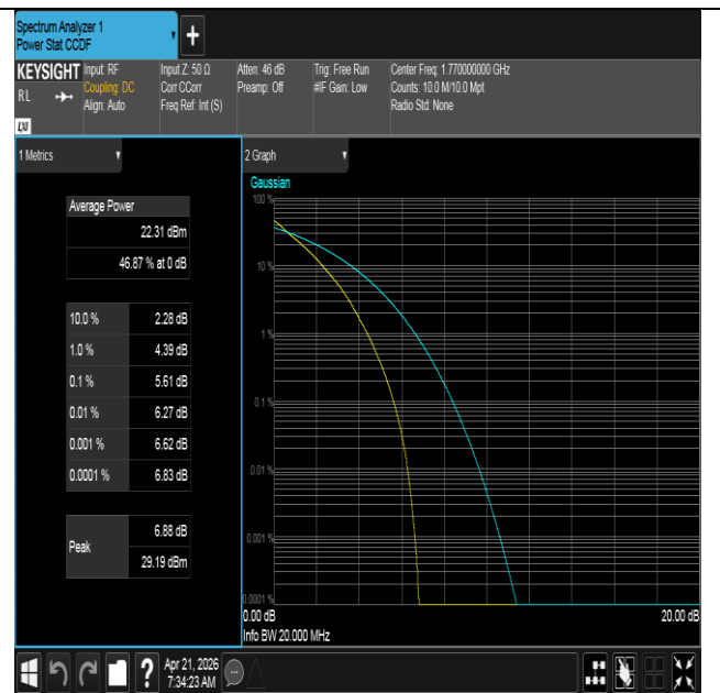
Band66-20MHz-QPSK-132572-100RB#0-PASS
