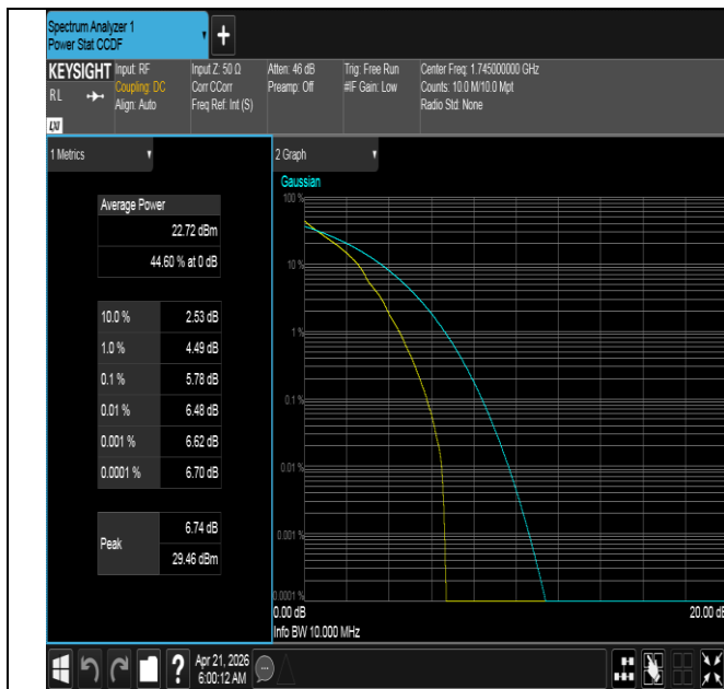
Band66-10MHz-QPSK-132322-1RB#0-PASS
