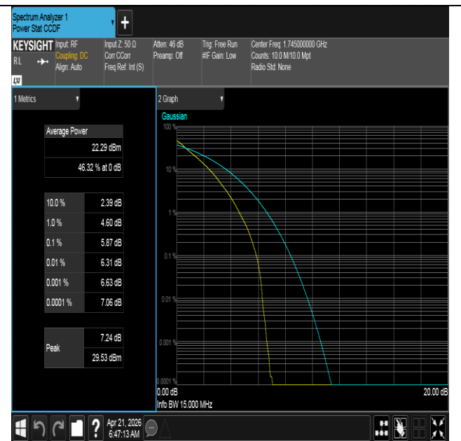
Band66-15MHz-QPSK-132322-75RB#0-PASS
