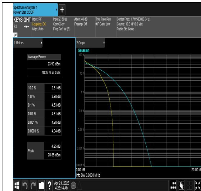
Band66-3MHz-QPSK-131987-1RB#0-PASS
