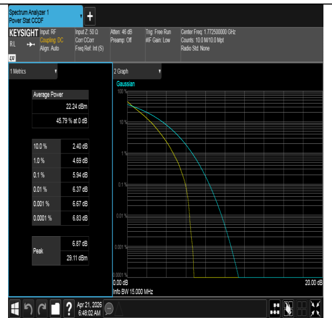
Band66-15MHz-QPSK-132597-75RB#0-PASS
