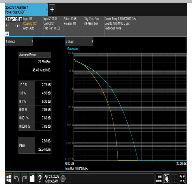
Band66-10MHz-16QAM-132622-50RB#0-PASS
