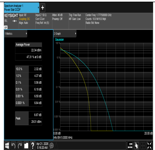
Band66-5MHz-QPSK-132647-25RB#0-PASS
