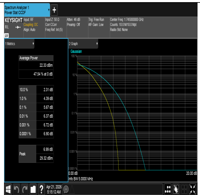
Band66-5MHz-QPSK-132322-25RB#0-PASS
