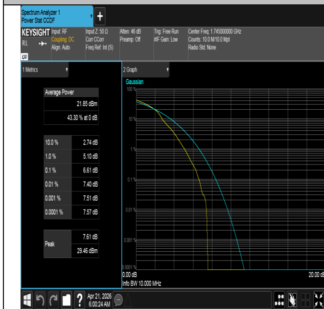
Band66-10MHz-16QAM-132322-1RB#0-PASS
