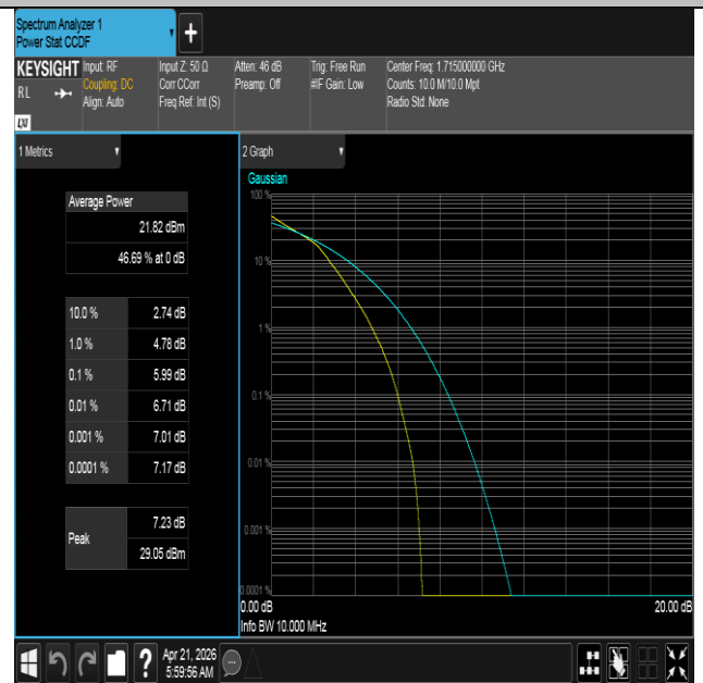
Band66-10MHz-16QAM-132022-50RB#0-PASS
