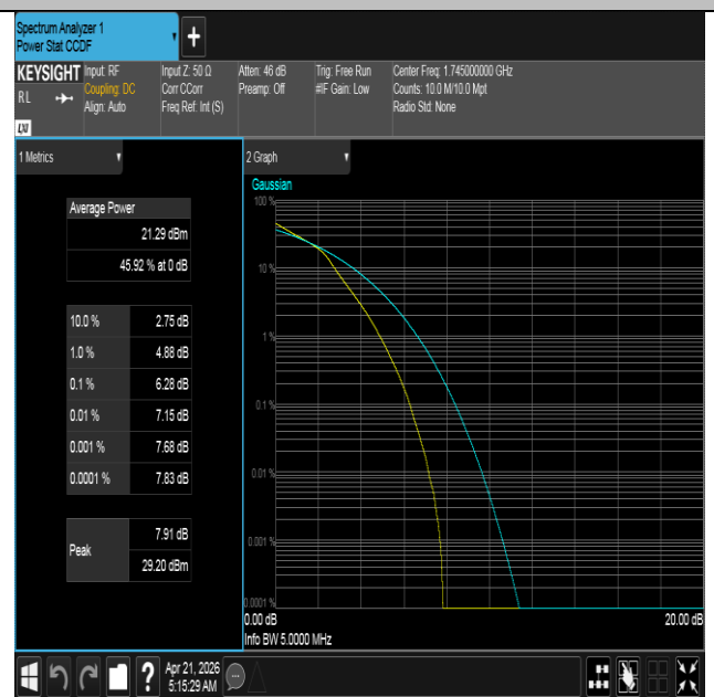
Band66-5MHz-16QAM-132322-25RB#0-PASS
