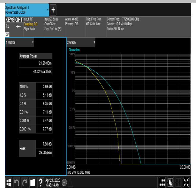
Band66-15MHz-16QAM-132597-75RB#0-PASS
