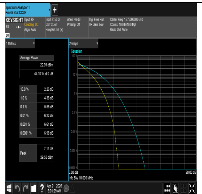
Band66-10MHz-QPSK-132622-50RB#0-PASS
