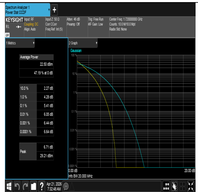
Band66-20MHz-QPSK-132072-100RB#0-PASS
