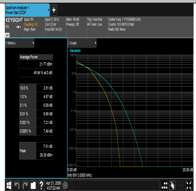
Band66-3MHz-16QAM-131987-15RB#0-PASS
