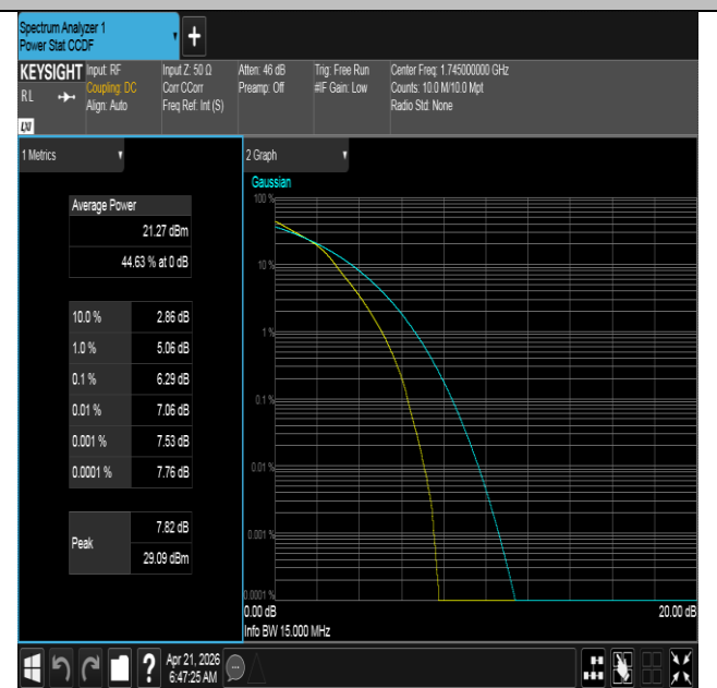
Band66-15MHz-16QAM-132322-75RB#0-PASS
