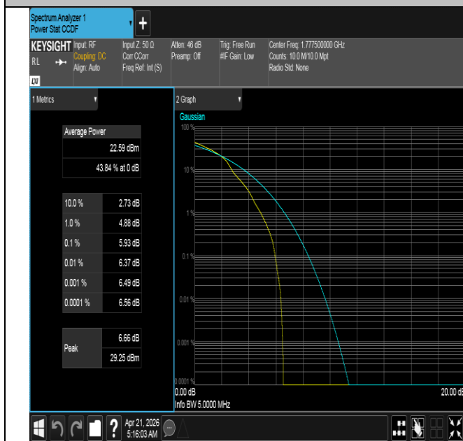
Band66-5MHz-16QAM-132647-1RB#0-PASS
