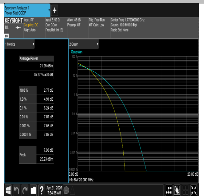
Band66-20MHz-16QAM-132572-100RB#0-PASS
