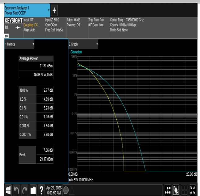
Band66-10MHz-16QAM-132322-50RB#0-PASS
