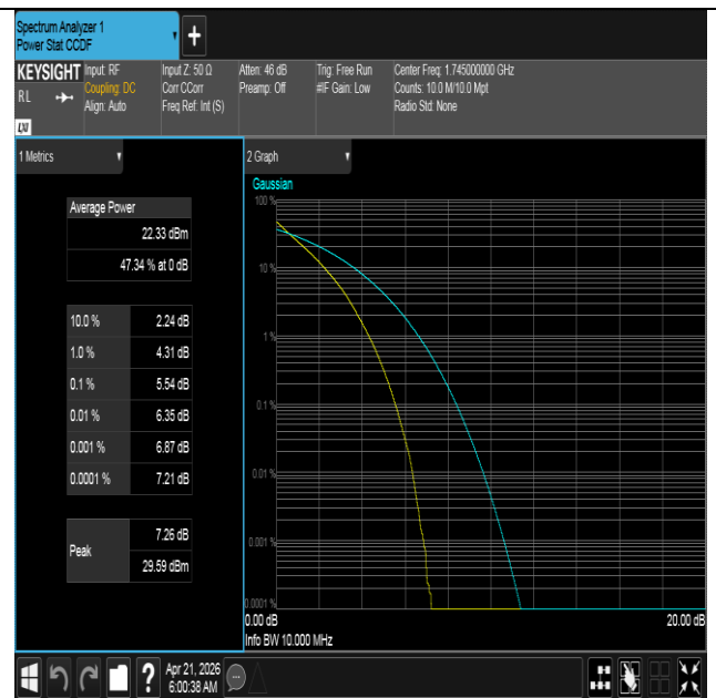
Band66-10MHz-QPSK-132322-50RB#0-PASS
