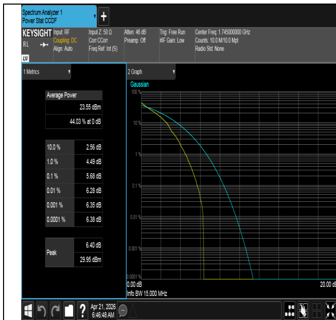
Band66-15MHz-QPSK-132322-1RB#0-PASS
