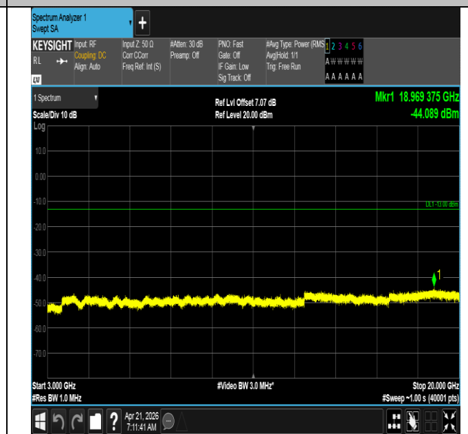
Band66-20MHz-QPSK-132572-1RB#99-3000~20000-PASS
