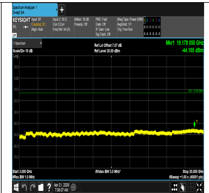
Band66-20MHz-QPSK-132322-1RB#99-3000~20000-PASS
