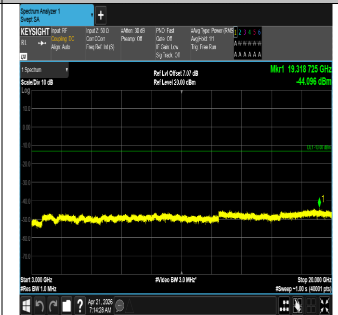
Band66-20MHz-16QAM-132572-100RB#0-3000~20000-PASS
