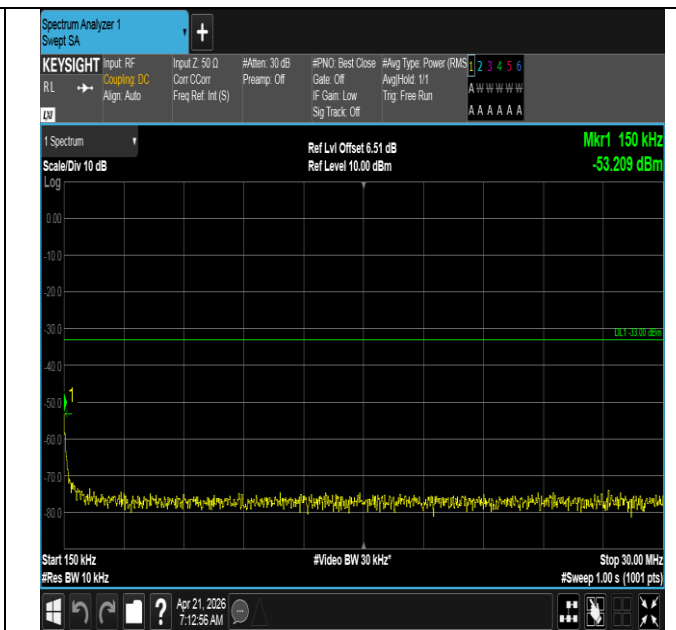
Band66-20MHz-QPSK-132572-100RB#0-0.15~30-PASS
