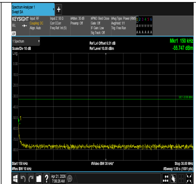
Band66-20MHz-16QAM-132322-1RB#99-0.15~30-PASS
