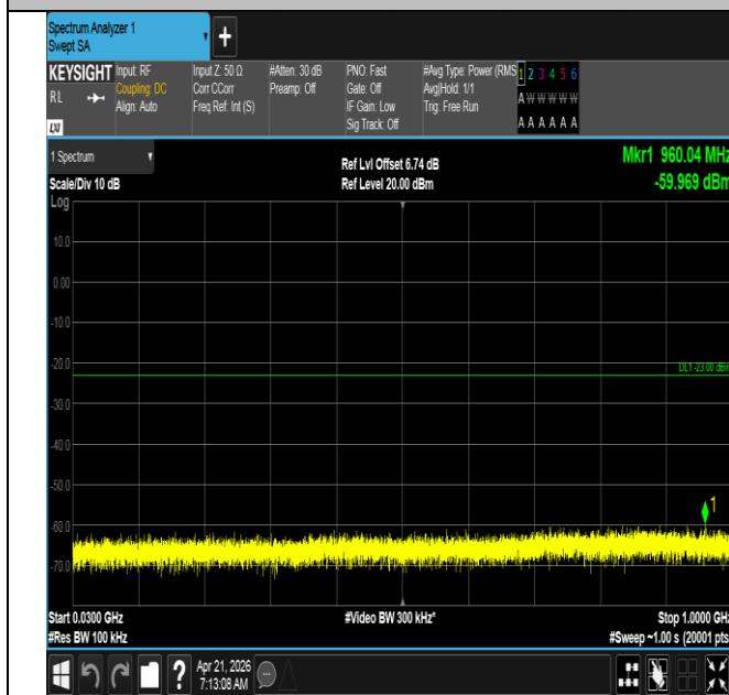
Band66-20MHz-QPSK-132572-100RB#0-30~1000-PASS
