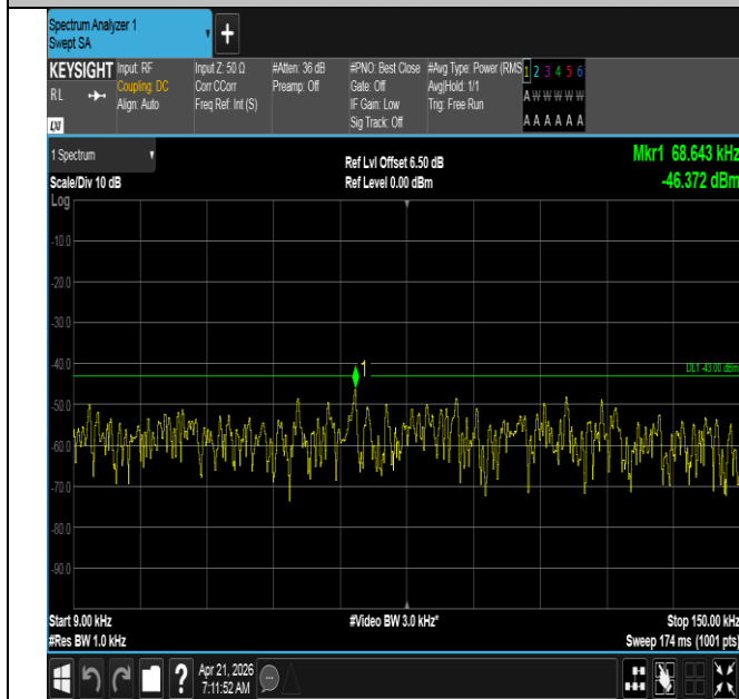
Band66-20MHz-16QAM-132572-1RB#99-0.009~0.15-PASS
