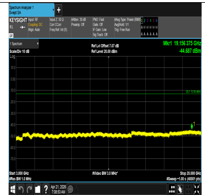
Band66-20MHz-16QAM-132322-100RB#0-3000~20000-PASS
