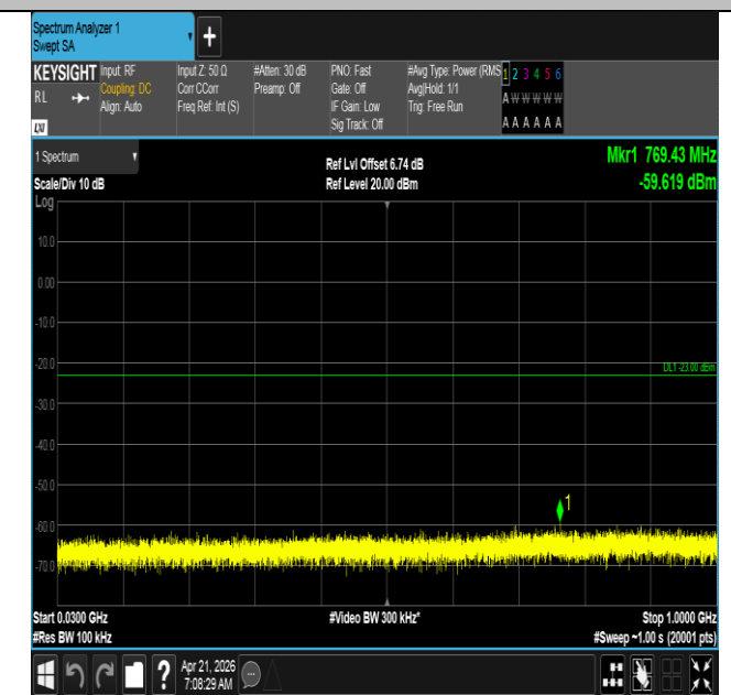
Band66-20MHz-16QAM-132322-100RB#0-30~1000-PASS
