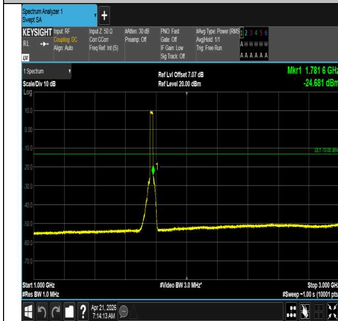
Band66-20MHz-16QAM-132572-100RB#0-1000~3000-PASS
