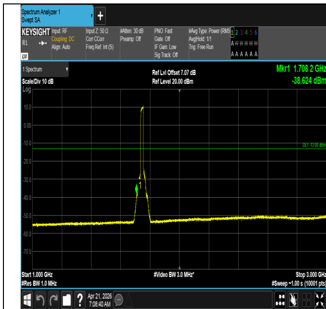
Band66-20MHz-16QAM-132322-100RB#0-1000~3000-PASS
