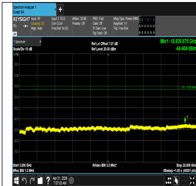
Band66-20MHz-16QAM-132322-1RB#99-3000~20000-PASS
