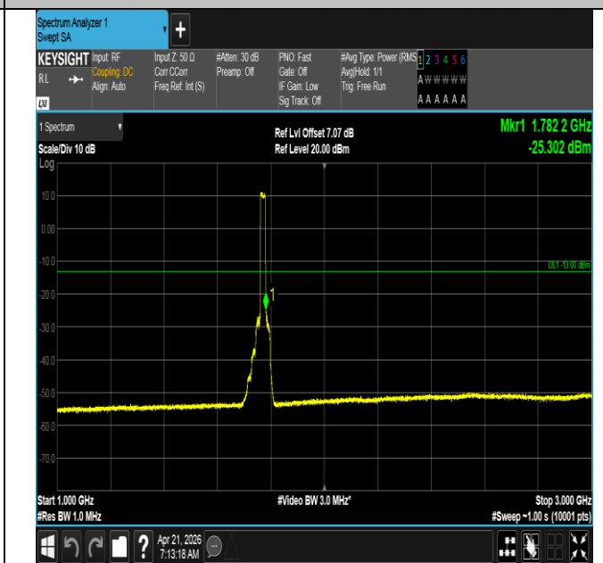
Band66-20MHz-QPSK-132572-100RB#0-1000~3000-PASS
