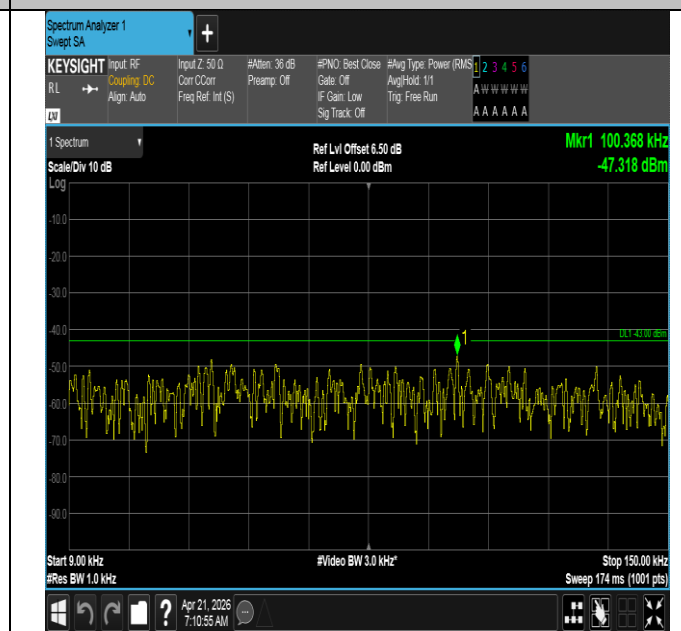
Band66-20MHz-QPSK-132572-1RB#99-0.009~0.15-PASS
