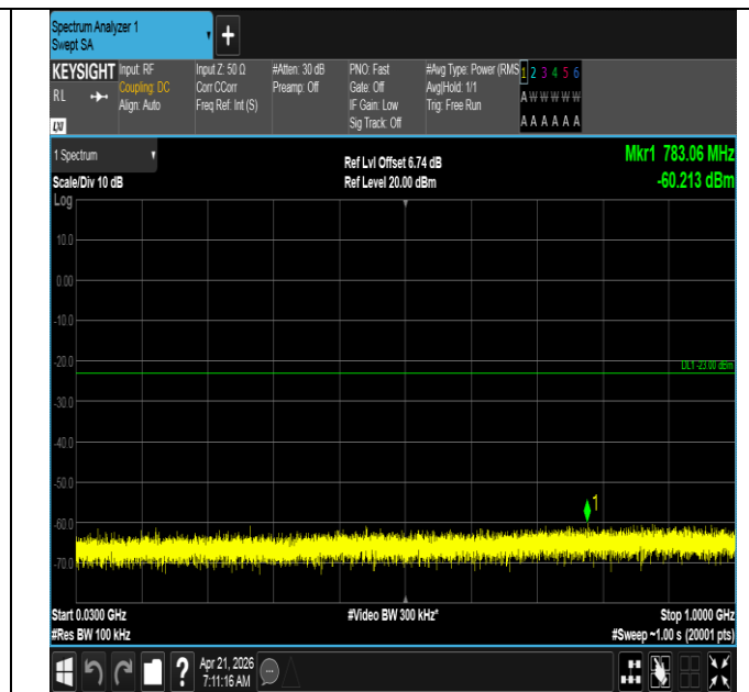
Band66-20MHz-QPSK-132572-1RB#99-30~1000-PASS
