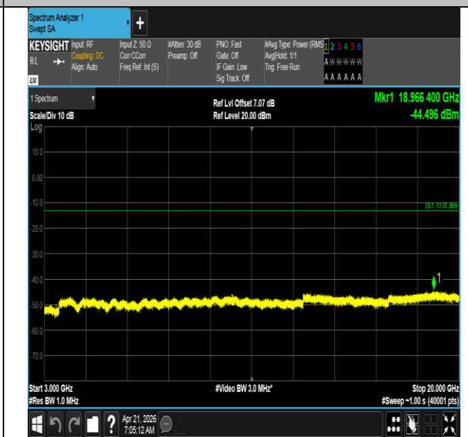
Band66-20MHz-16QAM-132322-1RB#0-3000~20000-PASS
