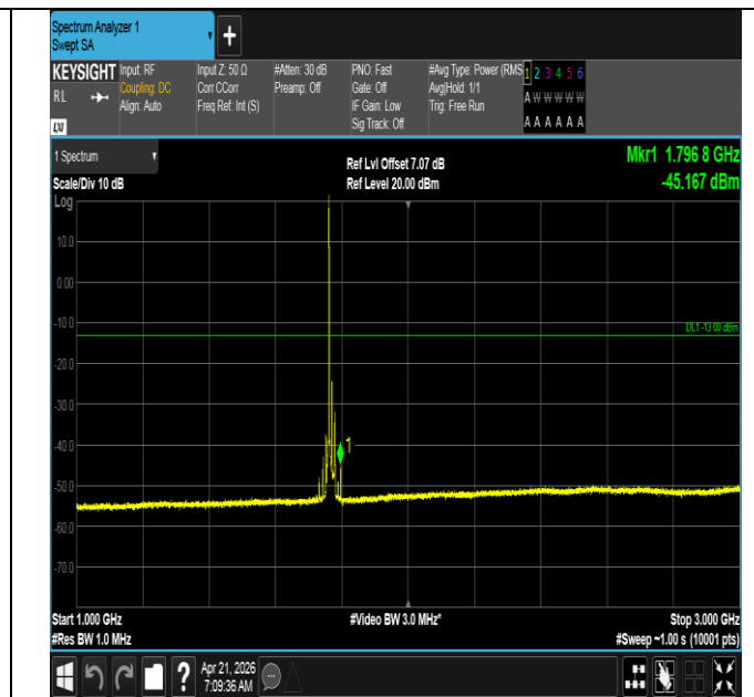
Band66-20MHz-QPSK-132572-1RB#0-1000~3000-PASS
