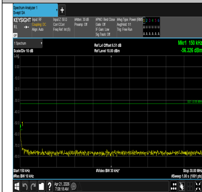
Band66-20MHz-16QAM-132322-100RB#0-0.15~30-PASS
