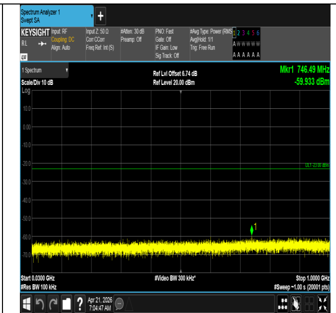
Band66-20MHz-16QAM-132322-1RB#0-30~1000-PASS
