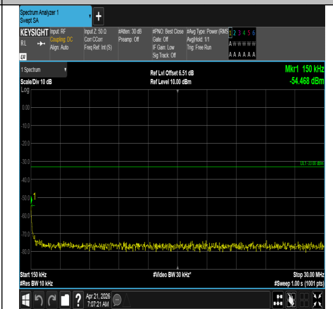
Band66-20MHz-QPSK-132322-100RB#0-0.15~30-PASS
