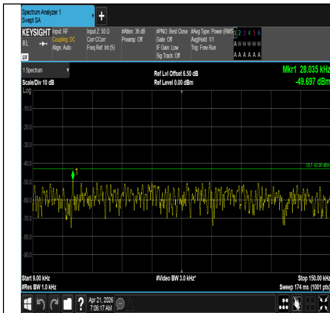
Band66-20MHz-16QAM-132322-1RB#99-0.009~0.15-PASS
