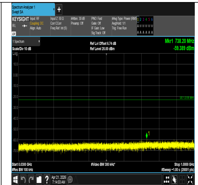
Band66-20MHz-16QAM-132572-100RB#0-30~1000-PASS
