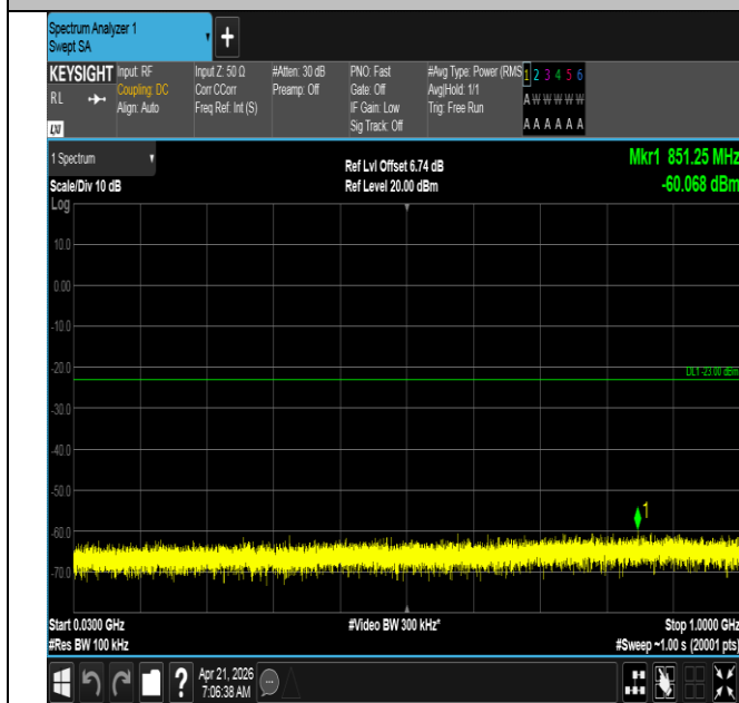
Band66-20MHz-16QAM-132322-1RB#99-30~1000-PASS
