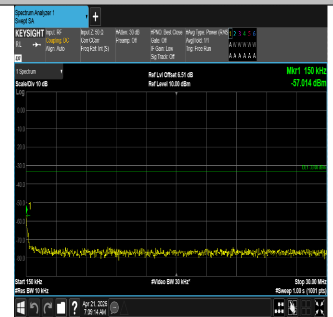
Band66-20MHz-QPSK-132572-1RB#0-0.15~30-PASS
