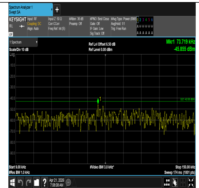
Band66-20MHz-16QAM-132322-100RB#0-0.009~0.15-PASS
