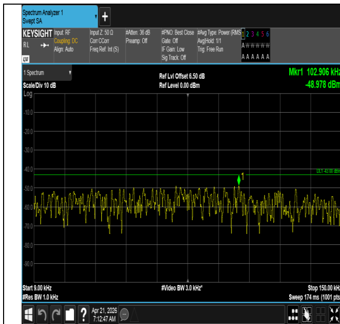
Band66-20MHz-QPSK-132572-100RB#0-0.009~0.15-PASS
