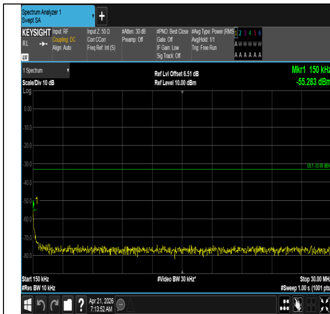
Band66-20MHz-16QAM-132572-100RB#0-0.15~30-PASS
