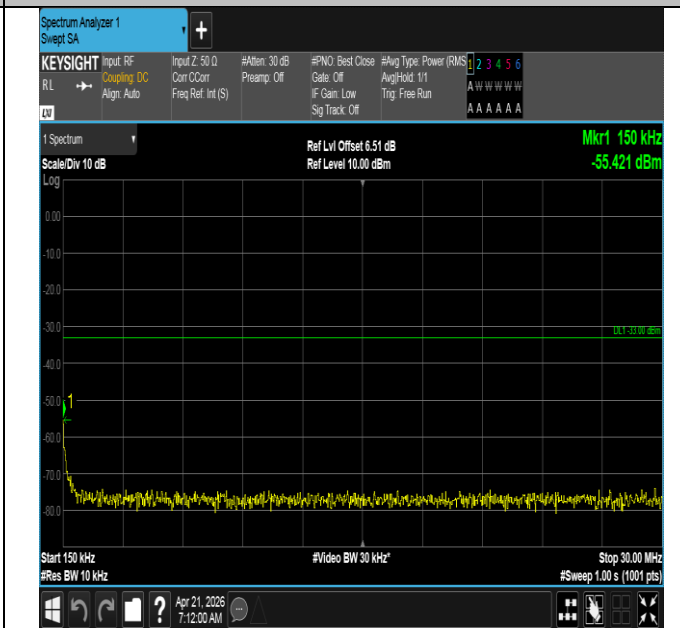
Band66-20MHz-16QAM-132572-1RB#99-0.15~30-PASS
