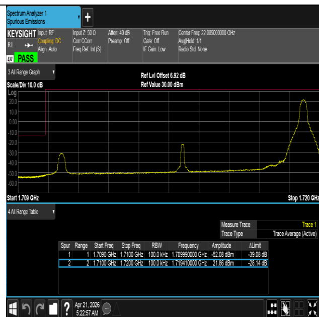
Band66-10MHz-QPSK-132022-1RB#49-PASS
