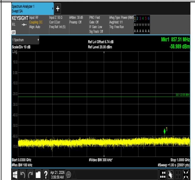
Band66-1.4MHz-QPSK-131979-1RB#5-30~1000-PASS
