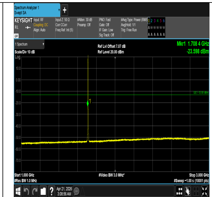
Band66-1.4MHz-QPSK-131979-6RB#0-1000~3000-PASS
