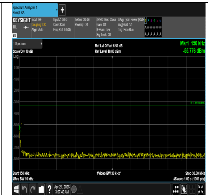
Band66-1.4MHz-16QAM-131979-1RB#5-0.15~30-PASS
