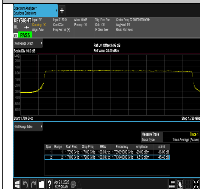
Band66-10MHz-QPSK-132022-50RB#0-PASS
