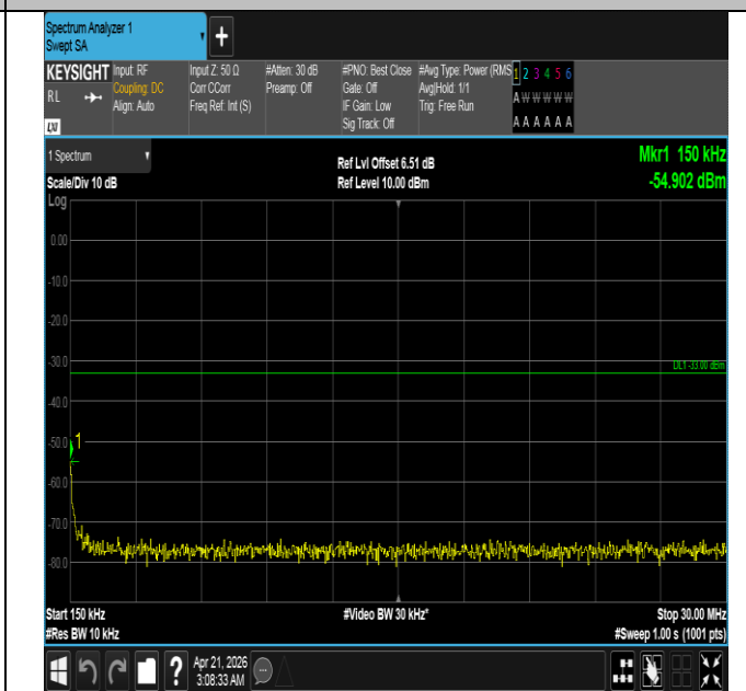
Band66-1.4MHz-QPSK-131979-6RB#0-0.15~30-PASS
