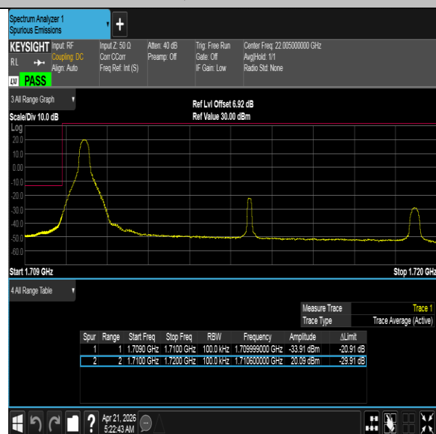
Band66-10MHz-16QAM-132022-1RB#0-PASS
