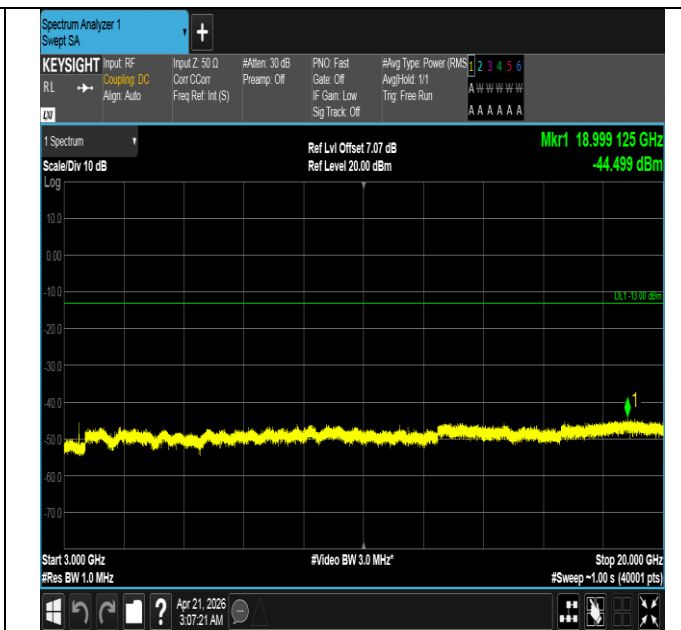
Band66-1.4MHz-QPSK-131979-1RB#5-3000~20000-PASS
