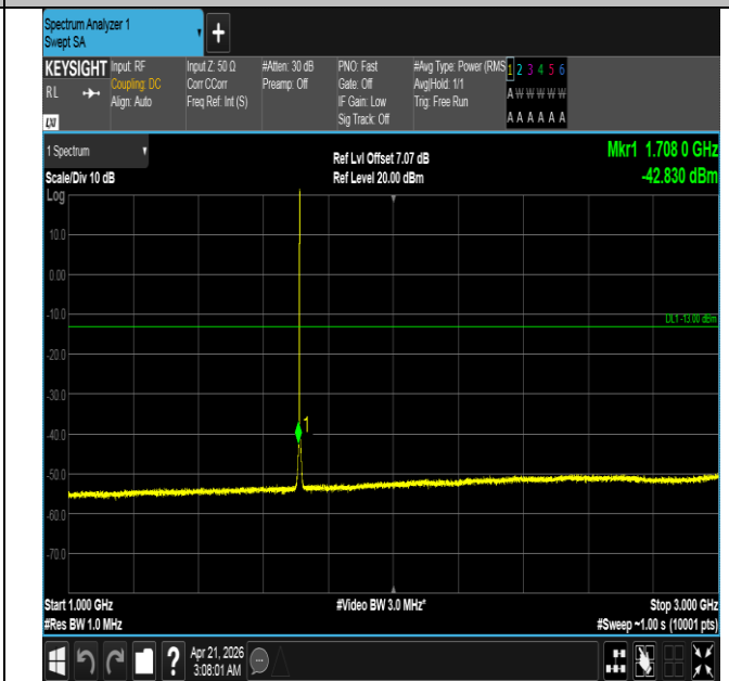
Band66-1.4MHz-16QAM-131979-1RB#5-1000~3000-PASS
