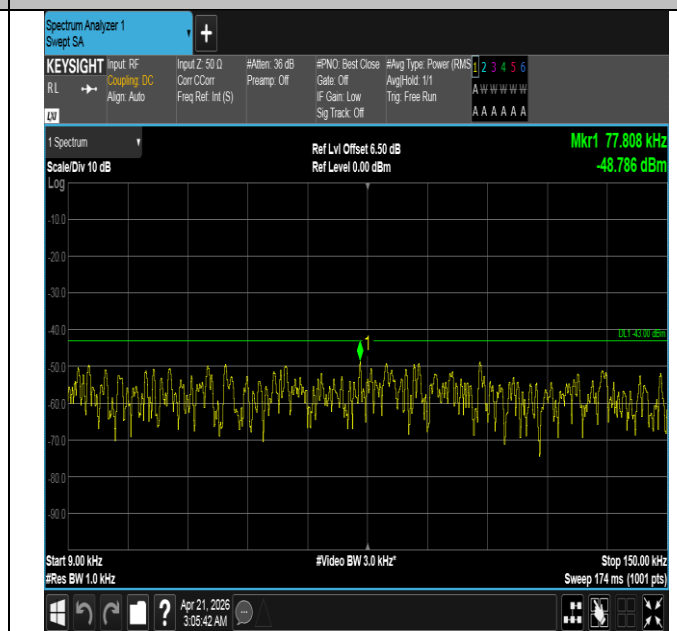
Band66-1.4MHz-16QAM-131979-1RB#0-0.009~0.15-PASS
