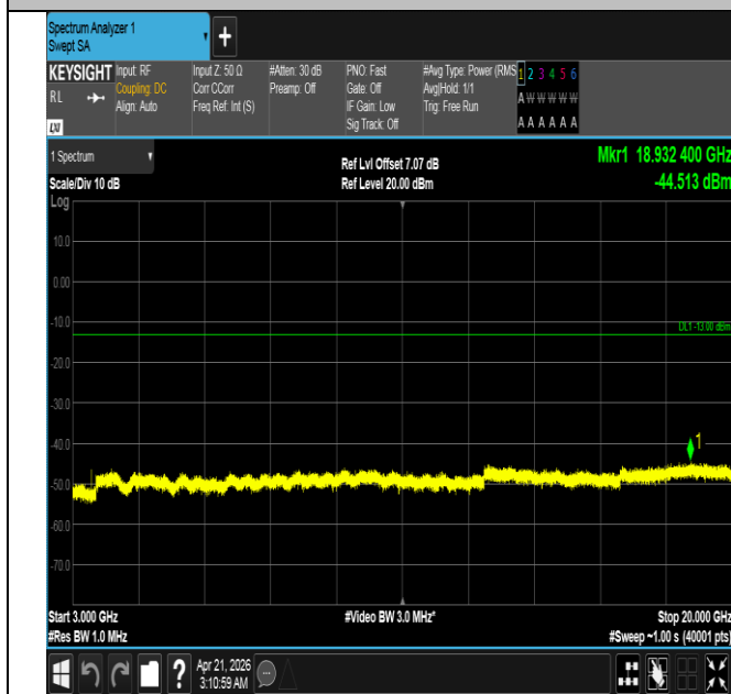
Band66-1.4MHz-QPSK-132322-1RB#0-3000~20000-PASS
