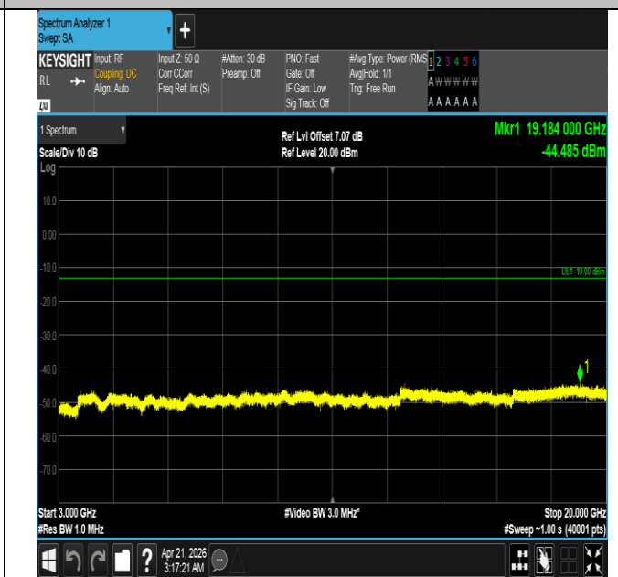
Band66-1.4MHz-16QAM-132665-1RB#0-3000~20000-PASS
