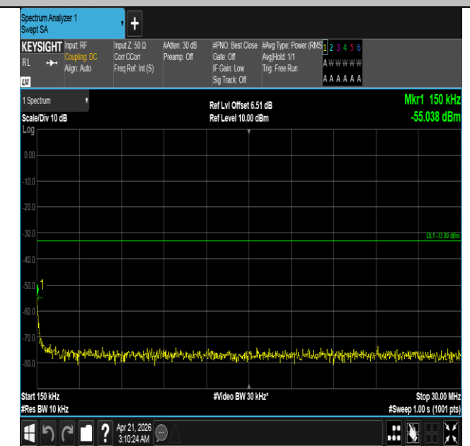
Band66-1.4MHz-QPSK-132322-1RB#0-0.15~30-PASS
