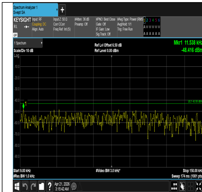
Band66-1.4MHz-QPSK-132665-1RB#0-0.009~0.15-PASS
