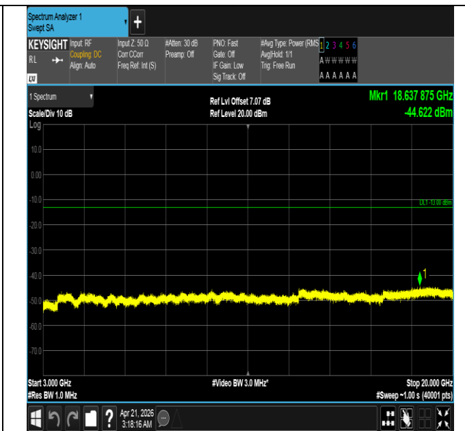
Band66-1.4MHz-QPSK-132665-1RB#5-3000~20000-PASS
