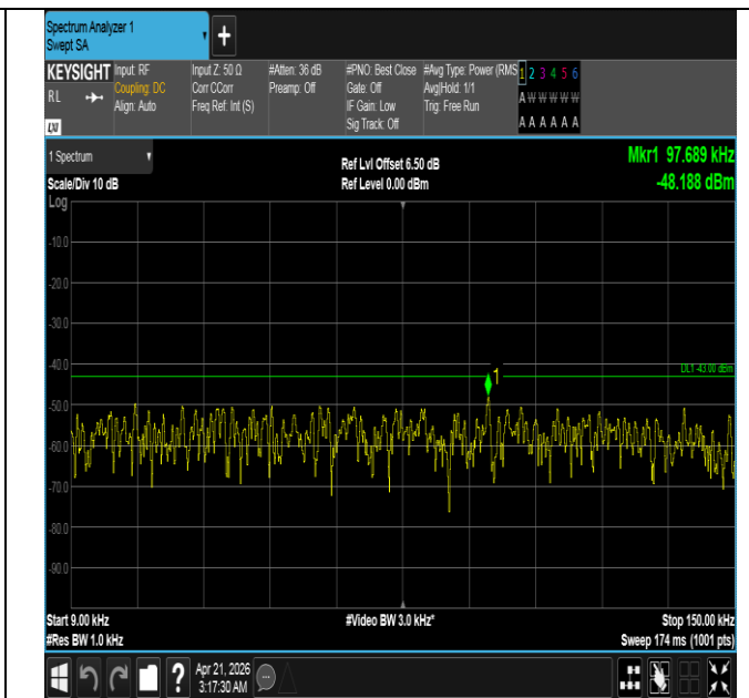
Band66-1.4MHz-QPSK-132665-1RB#5-0.009~0.15-PASS
