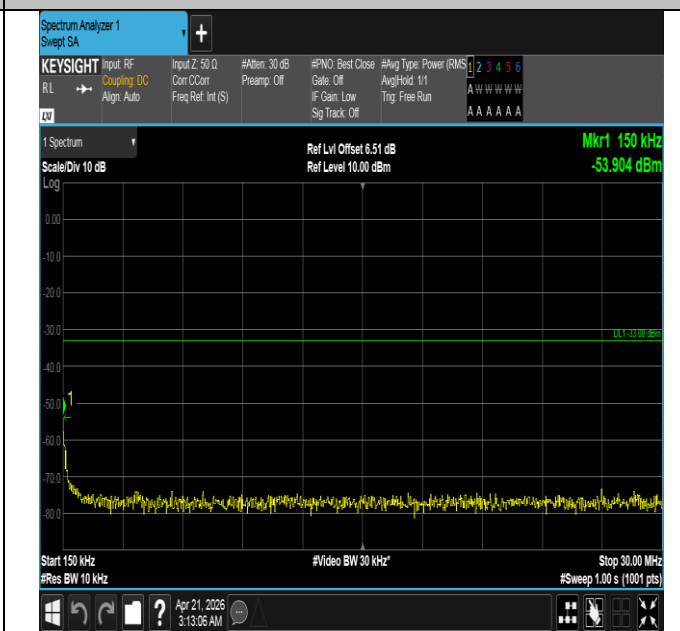
Band66-1.4MHz-16QAM-132322-1RB#5-0.15~30-PASS
