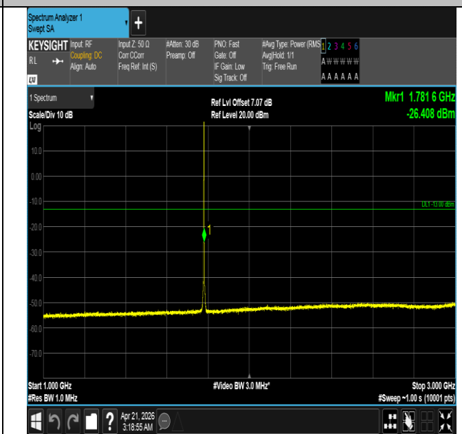
Band66-1.4MHz-16QAM-132665-1RB#5-1000~3000-PASS
