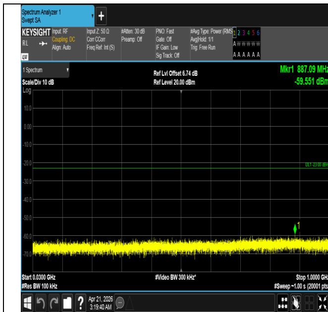
Band66-1.4MHz-QPSK-132665-6RB#0-30~1000-PASS
