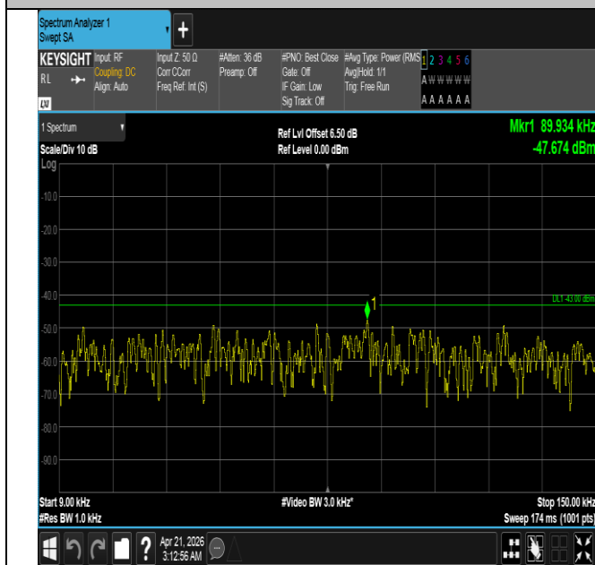
Band66-1.4MHz-16QAM-132322-1RB#5-0.009~0.15-PASS
