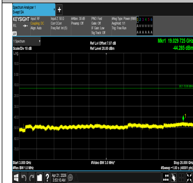
Band66-3MHz-QPSK-131987-1RB#0-3000~20000-PASS
