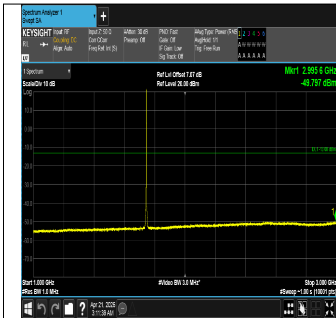
Band66-1.4MHz-16QAM-132322-1RB#0-1000~3000-PASS
