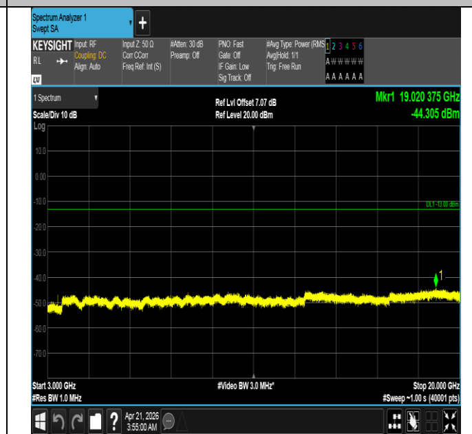
Band66-3MHz-QPSK-131987-1RB#14-3000~20000-PASS
