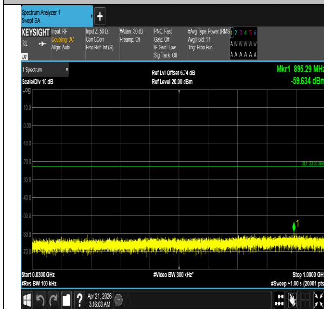
Band66-1.4MHz-QPSK-132665-1RB#0-30~1000-PASS
