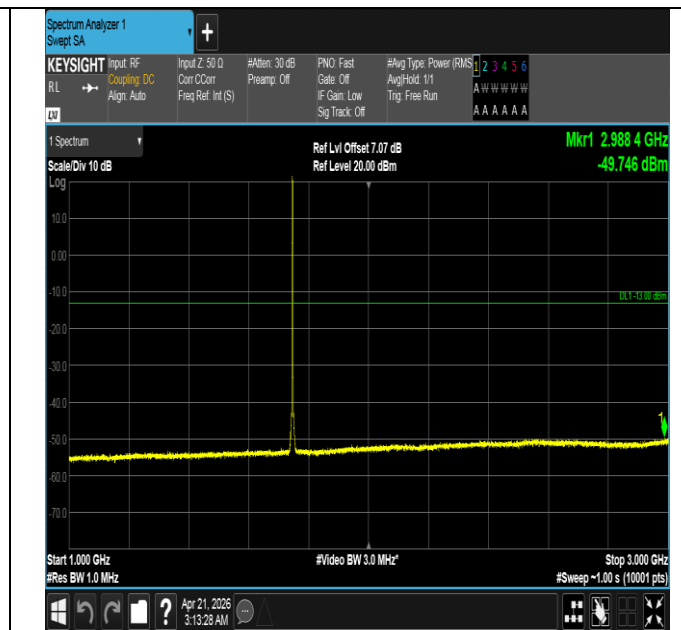
Band66-1.4MHz-16QAM-132322-1RB#5-1000~3000-PASS
