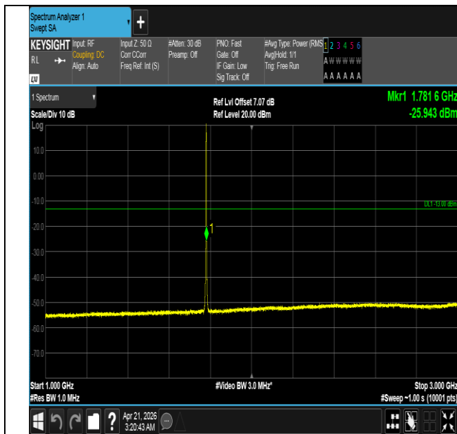
Band66-1.4MHz-16QAM-132665-6RB#0-1000~3000-PASS
