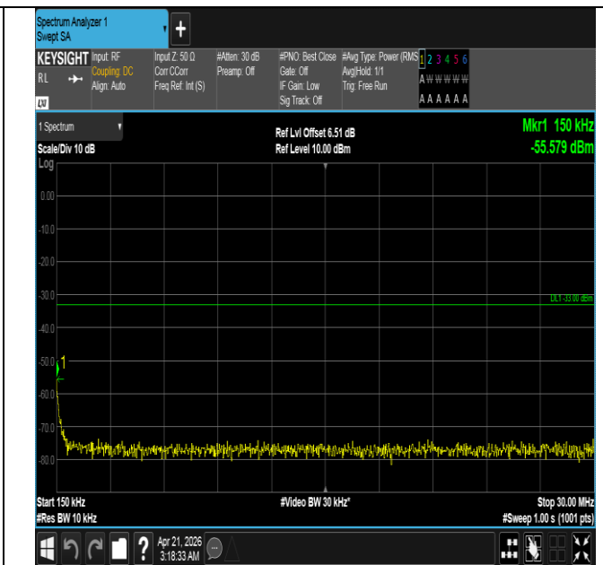
Band66-1.4MHz-16QAM-132665-1RB#5-0.15~30-PASS
