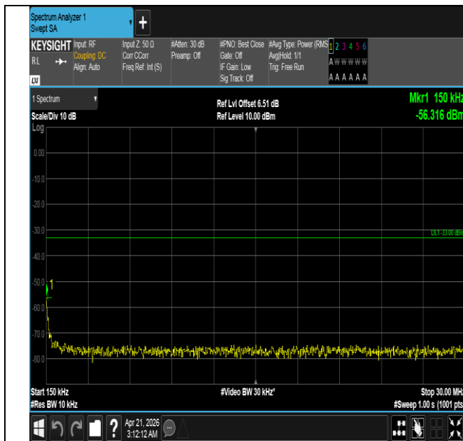
Band66-1.4MHz-QPSK-132322-1RB#5-0.15~30-PASS
