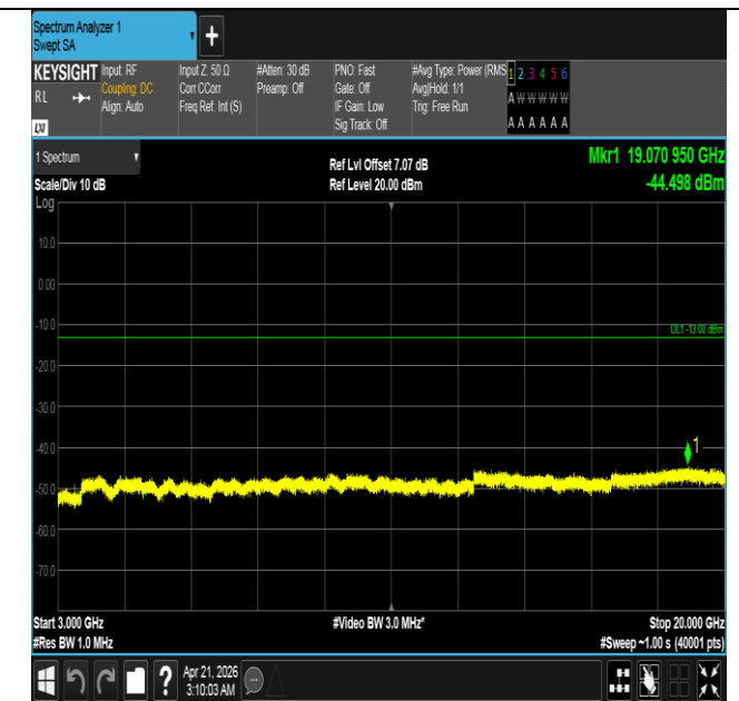
Band66-1.4MHz-16QAM-131979-6RB#0-3000~20000-PASS
