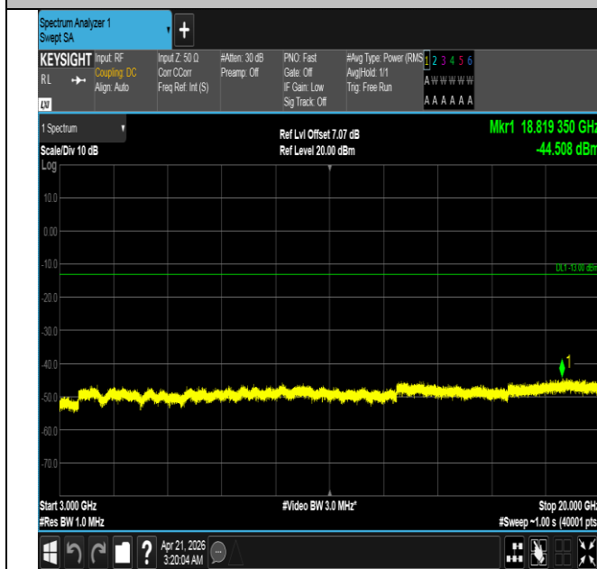
Band66-1.4MHz-QPSK-132665-6RB#0-3000~20000-PASS
