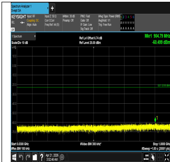
Band66-3MHz-QPSK-131987-1RB#0-30~1000-PASS
