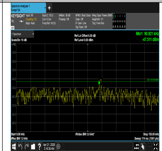
Band66-1.4MHz-16QAM-132665-1RB#0-0.009~0.15-PASS
