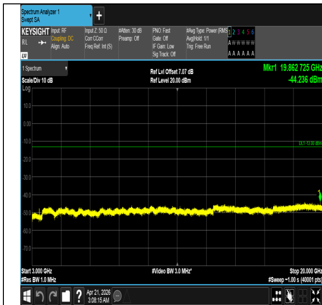
Band66-1.4MHz-16QAM-131979-1RB#5-3000~20000-PASS
