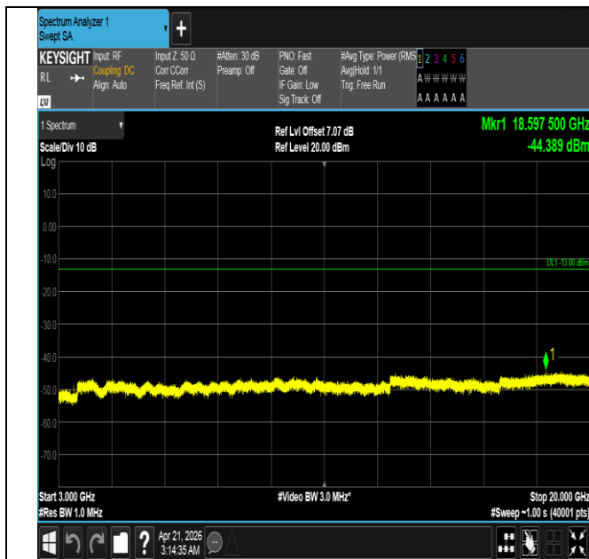
Band66-1.4MHz-QPSK-132322-6RB#0-3000~20000-PASS
