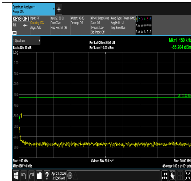
Band66-1.4MHz-16QAM-132665-1RB#0-0.15~30-PASS
