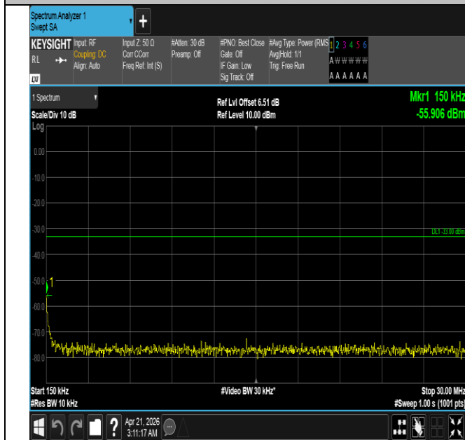
Band66-1.4MHz-16QAM-132322-1RB#0-0.15~30-PASS
