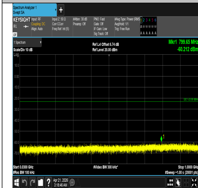
Band66-1.4MHz-16QAM-132665-1RB#5-30~1000-PASS
