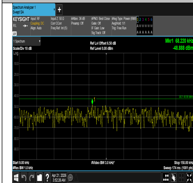
Band66-3MHz-QPSK-131987-1RB#0-0.009~0.15-PASS
