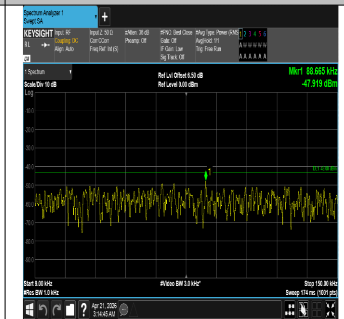
Band66-1.4MHz-16QAM-132322-6RB#0-0.009~0.15-PASS
