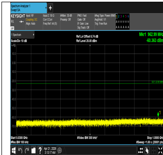
Band66-1.4MHz-16QAM-132322-1RB#5-30~1000-PASS
