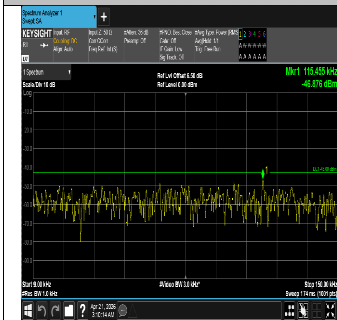
Band66-1.4MHz-QPSK-132322-1RB#0-0.009~0.15-PASS
