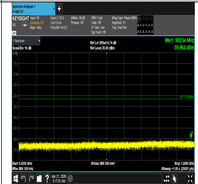
Band66-1.4MHz-QPSK-132665-1RB#5-30~1000-PASS
