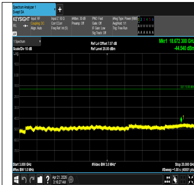
Band66-1.4MHz-QPSK-132665-1RB#0-3000~20000-PASS
