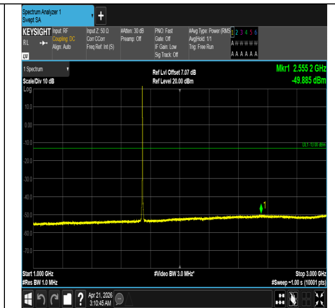
Band66-1.4MHz-QPSK-132322-1RB#0-1000~3000-PASS
