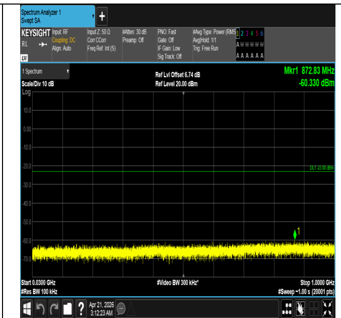
Band66-1.4MHz-QPSK-132322-1RB#5-30~1000-PASS
