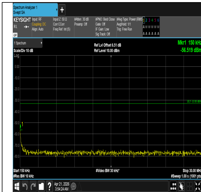
Band66-3MHz-QPSK-131987-1RB#14-0.15~30-PASS
