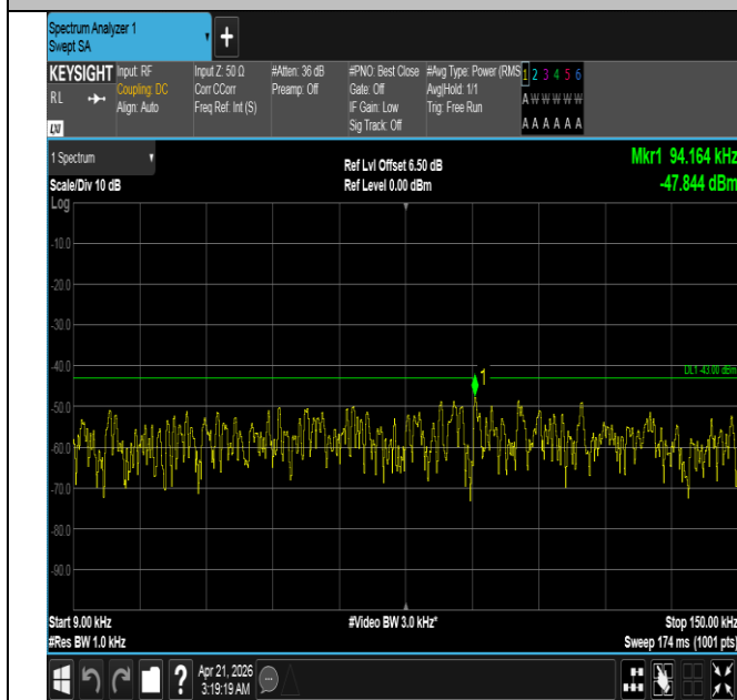
Band66-1.4MHz-QPSK-132665-6RB#0-0.009~0.15-PASS
