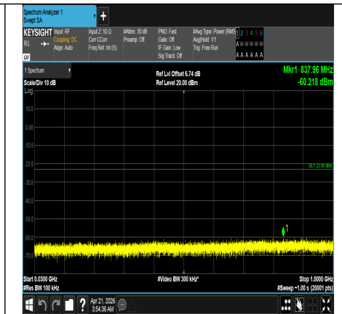
Band66-3MHz-QPSK-131987-1RB#14-30~1000-PASS
