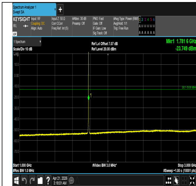
Band66-1.4MHz-QPSK-132665-1RB#5-1000~3000-PASS
