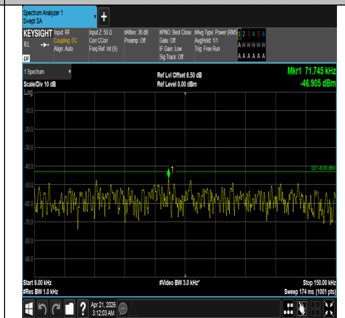
Band66-1.4MHz-QPSK-132322-1RB#5-0.009~0.15-PASS
