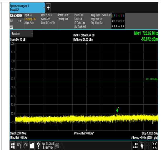
Band66-1.4MHz-16QAM-132665-1RB#0-30~1000-PASS
