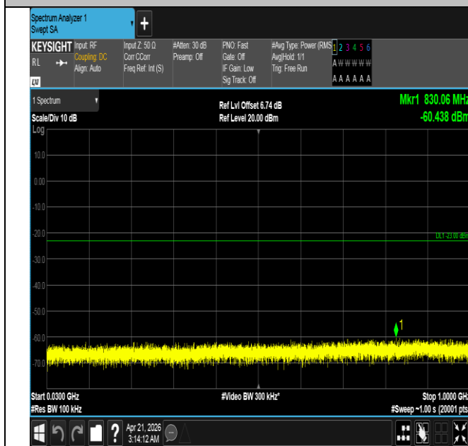
Band66-1.4MHz-QPSK-132322-6RB#0-30~1000-PASS
