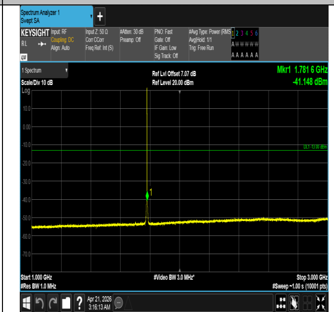
Band66-1.4MHz-QPSK-132665-1RB#0-1000~3000-PASS
