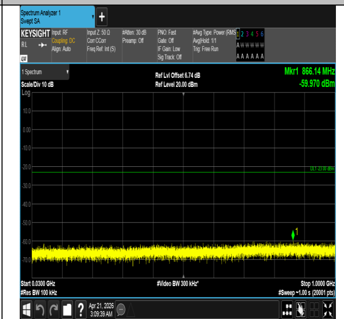
Band66-1.4MHz-16QAM-131979-6RB#0-30~1000-PASS
