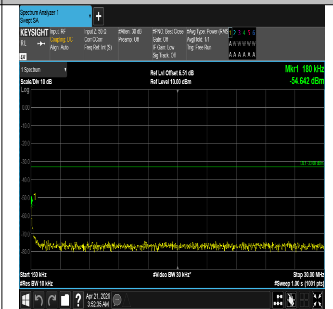
Band66-3MHz-QPSK-131987-1RB#0-0.15~30-PASS
