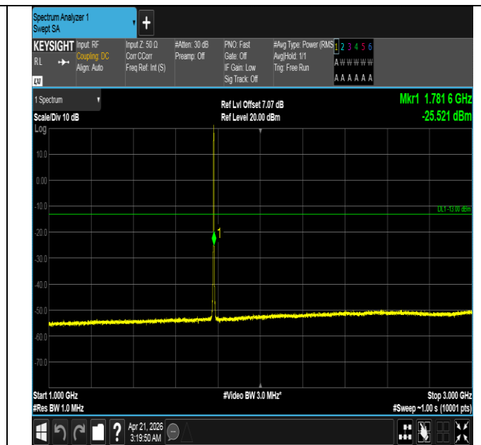
Band66-1.4MHz-QPSK-132665-6RB#0-1000~3000-PASS
