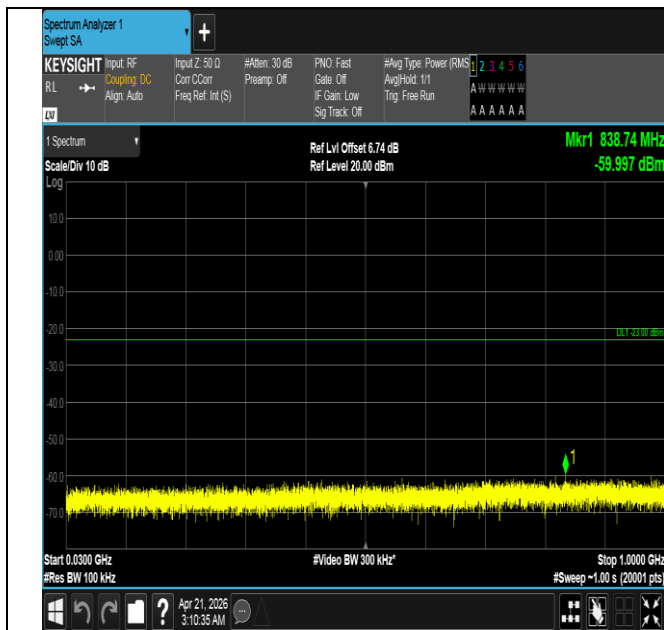
Band66-1.4MHz-QPSK-132322-1RB#0-30~1000-PASS
