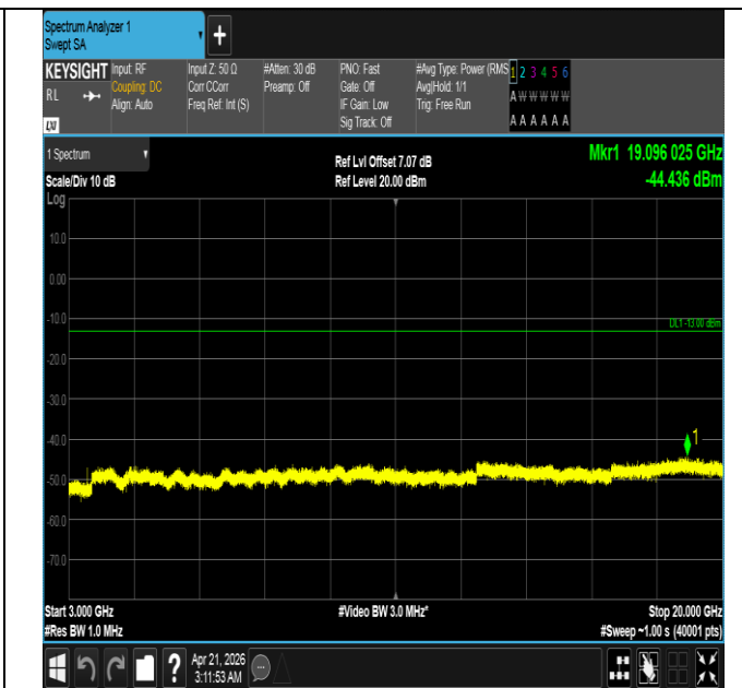
Band66-1.4MHz-16QAM-132322-1RB#0-3000~20000-PASS
