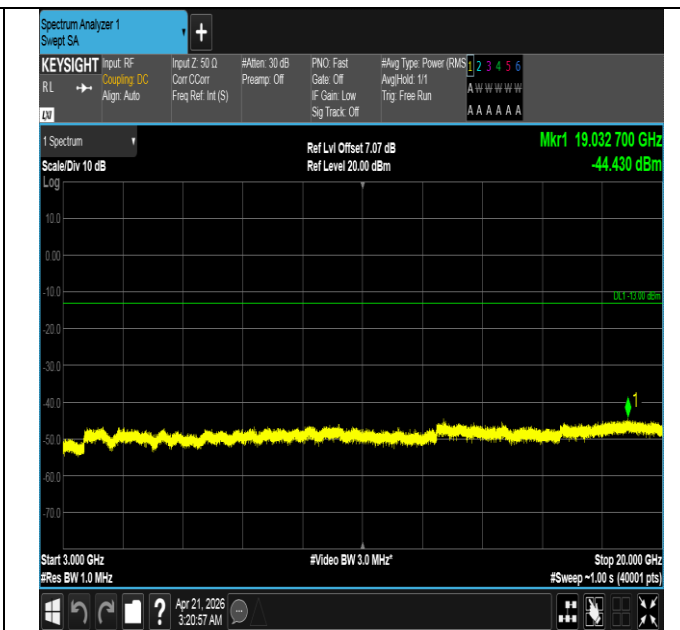
Band66-1.4MHz-16QAM-132665-6RB#0-3000~20000-PASS
