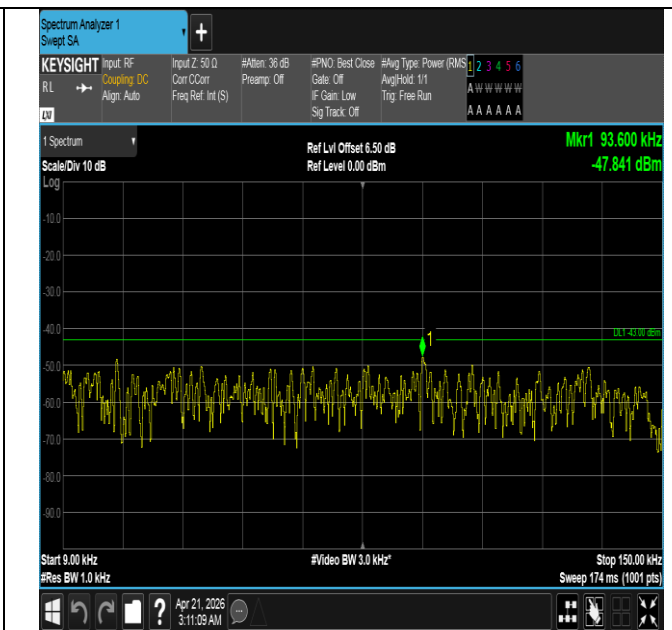
Band66-1.4MHz-16QAM-132322-1RB#0-0.009~0.15-PASS
