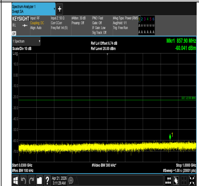
Band66-1.4MHz-16QAM-132322-1RB#0-30~1000-PASS
