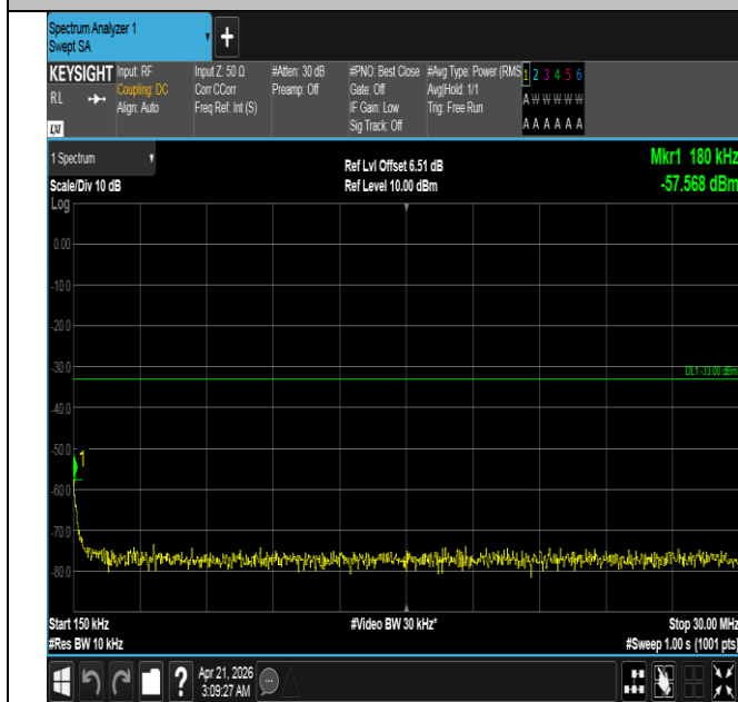
Band66-1.4MHz-16QAM-131979-6RB#0-0.15~30-PASS
