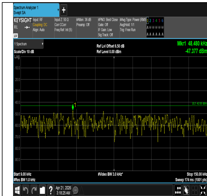
Band66-1.4MHz-16QAM-132665-1RB#5-0.009~0.15-PASS
