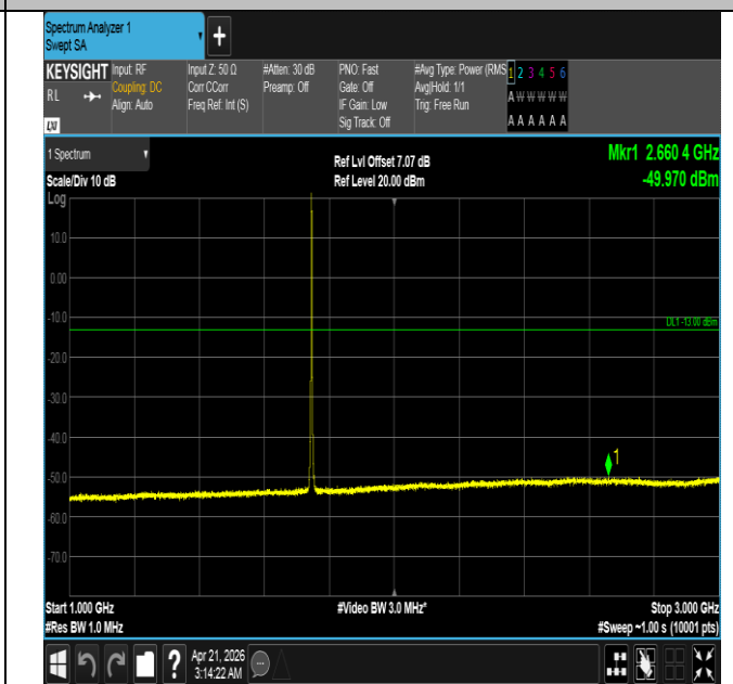
Band66-1.4MHz-QPSK-132322-6RB#0-1000~3000-PASS
