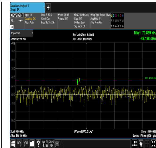
Band66-1.4MHz-QPSK-132322-6RB#0-0.009~0.15-PASS
