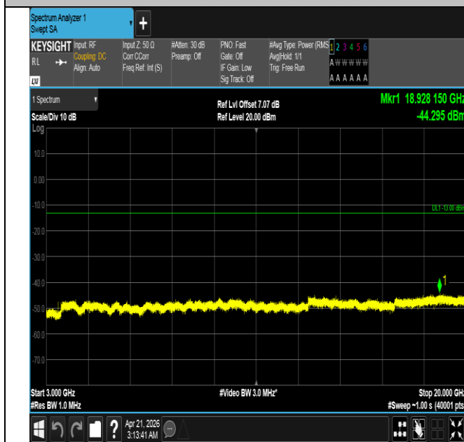
Band66-1.4MHz-16QAM-132322-1RB#5-3000~20000-PASS
