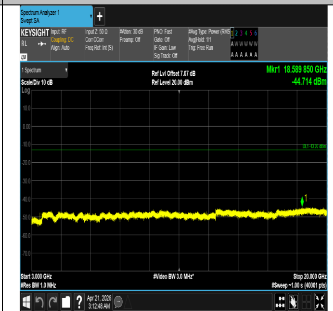
Band66-1.4MHz-QPSK-132322-1RB#5-3000~20000-PASS
