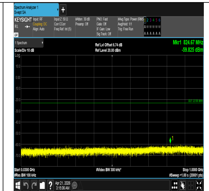
Band66-1.4MHz-16QAM-132322-6RB#0-30~1000-PASS
