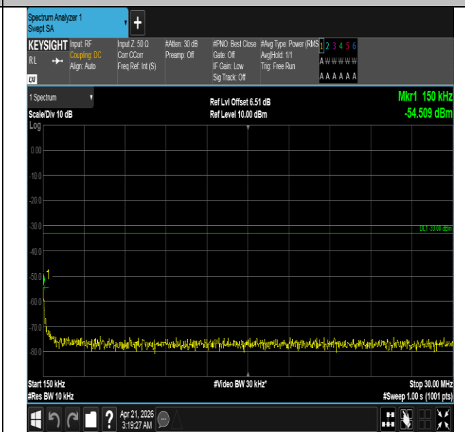
Band66-1.4MHz-QPSK-132665-6RB#0-0.15~30-PASS
