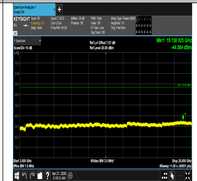
Band66-1.4MHz-16QAM-132322-6RB#0-3000~20000-PASS
