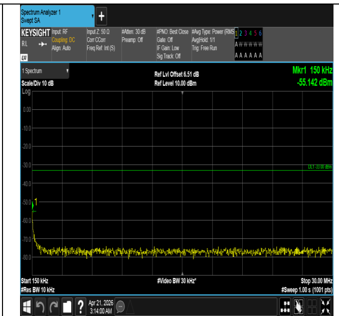
Band66-1.4MHz-QPSK-132322-6RB#0-0.15~30-PASS
