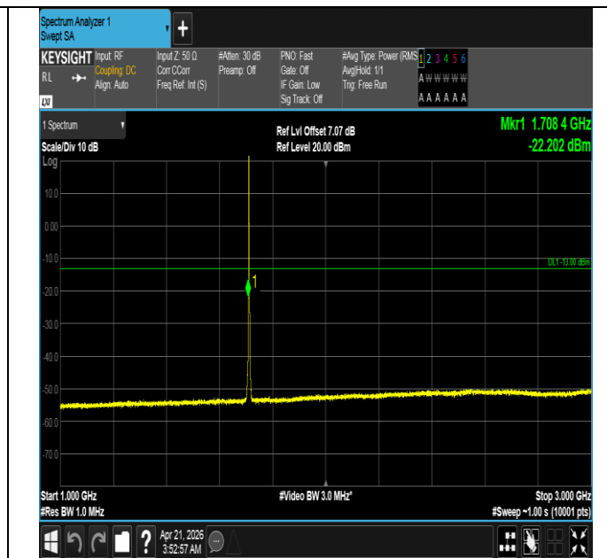
Band66-3MHz-QPSK-131987-1RB#0-1000~3000-PASS
