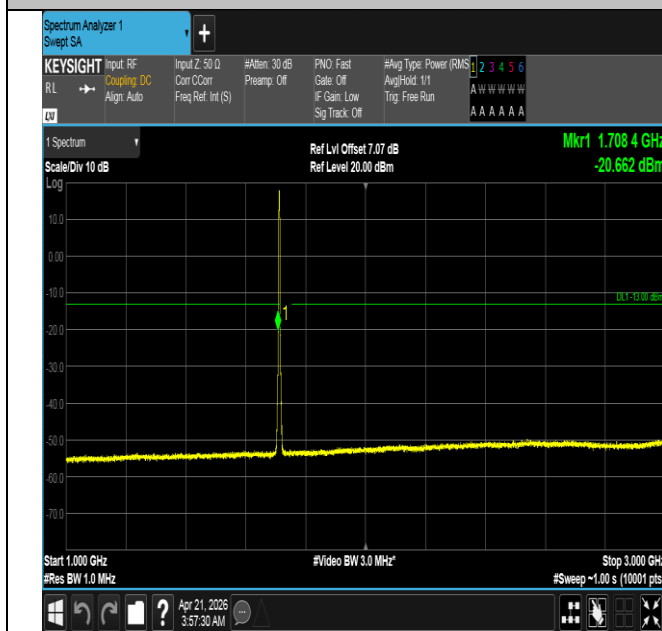
Band66-3MHz-16QAM-131987-15RB#0-1000~3000-PASS
