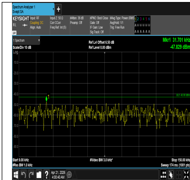
Band66-3MHz-16QAM-132322-1RB#14-0.009~0.15-PASS
