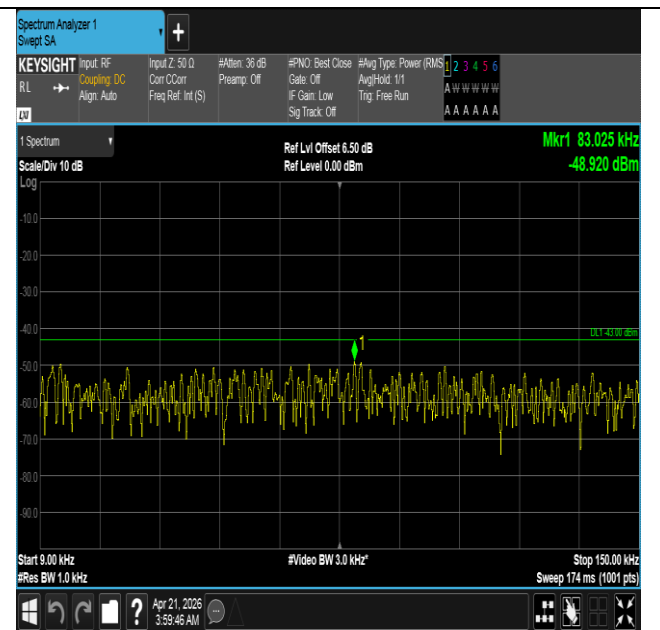
Band66-3MHz-QPSK-132322-1RB#14-0.009~0.15-PASS
