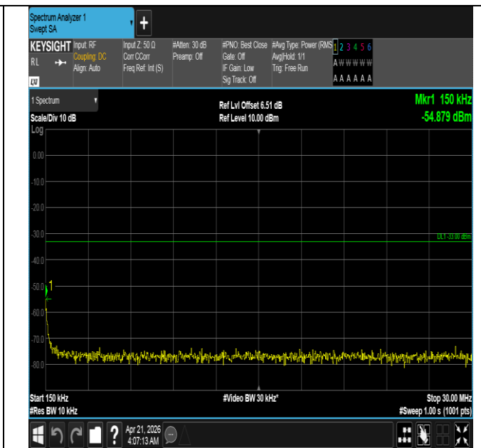
Band66-3MHz-QPSK-132657-15RB#0-0.15~30-PASS
