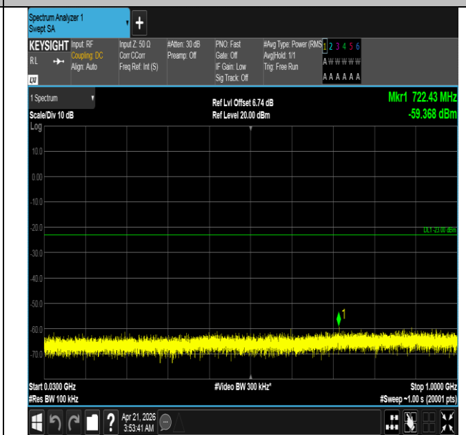
Band66-3MHz-16QAM-131987-1RB#0-30~1000-PASS
