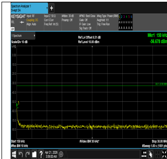
Band66-3MHz-16QAM-132322-1RB#0-0.15~30-PASS
