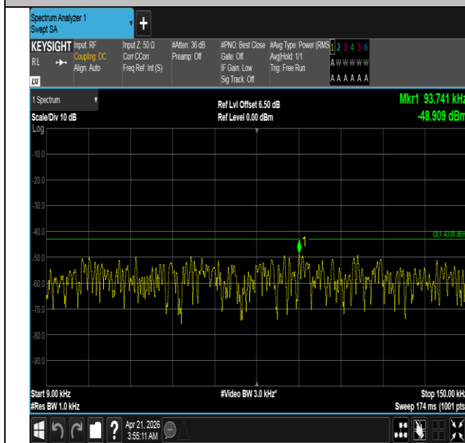
Band66-3MHz-16QAM-131987-1RB#14-0.009~0.15-PASS
