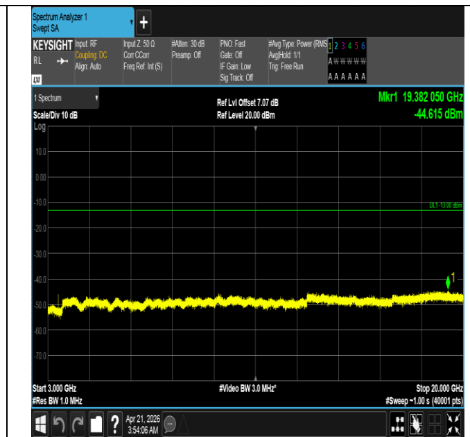
Band66-3MHz-16QAM-131987-1RB#0-3000~20000-PASS
