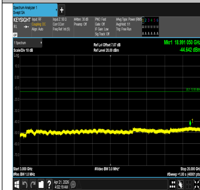
Band66-3MHz-QPSK-132322-15RB#0-3000~20000-PASS
