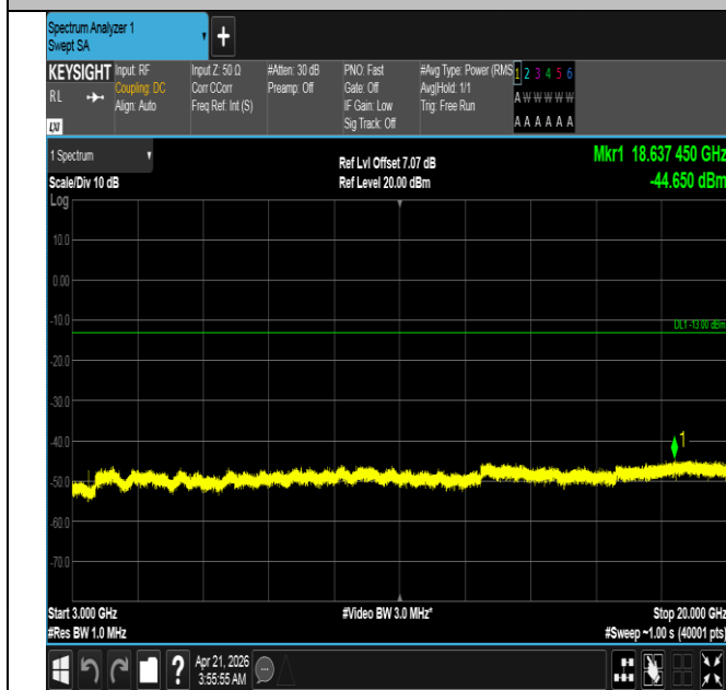
Band66-3MHz-16QAM-131987-1RB#14-3000~20000-PASS
