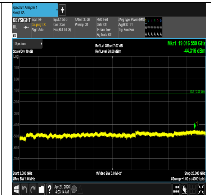
Band66-3MHz-16QAM-132322-15RB#0-3000~20000-PASS
