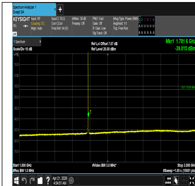
Band66-3MHz-16QAM-132657-1RB#0-1000~3000-PASS
