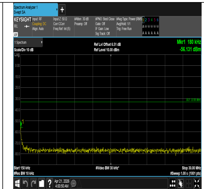
Band66-3MHz-16QAM-132322-1RB#14-0.15~30-PASS
