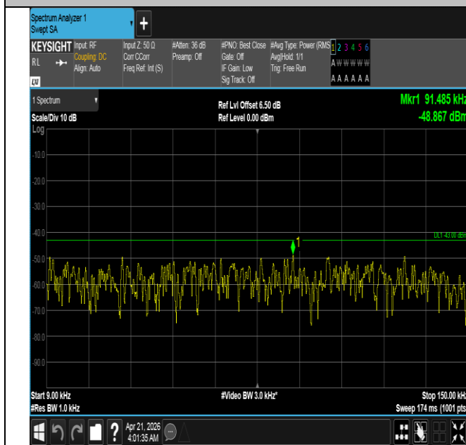
Band66-3MHz-QPSK-132322-15RB#0-0.009~0.15-PASS
