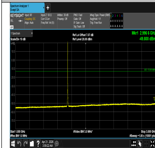
Band66-3MHz-16QAM-132322-1RB#0-1000~3000-PASS
