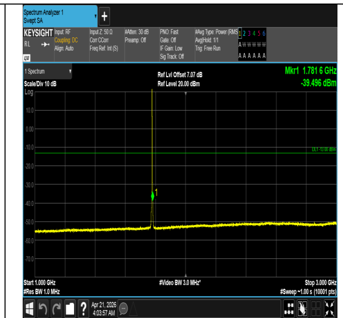
Band66-3MHz-QPSK-132657-1RB#0-1000~3000-PASS
