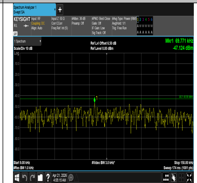
Band66-3MHz-QPSK-132657-1RB#14-0.009~0.15-PASS
