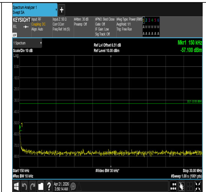
Band66-3MHz-QPSK-131987-15RB#0-0.15~30-PASS
