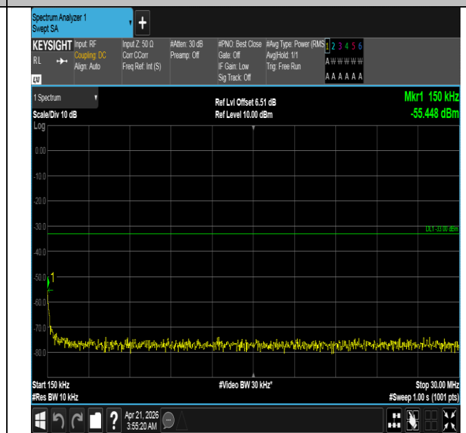
Band66-3MHz-16QAM-131987-1RB#14-0.15~30-PASS
