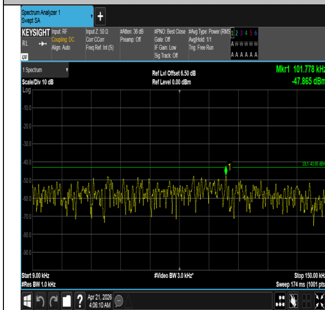
Band66-3MHz-16QAM-132657-1RB#14-0.009~0.15-PASS
