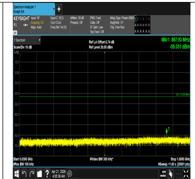
Band66-3MHz-QPSK-132657-1RB#14-30~1000-PASS
