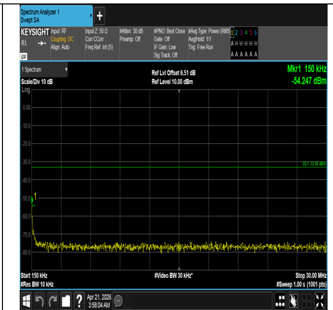
Band66-3MHz-QPSK-132322-1RB#0-0.15~30-PASS
