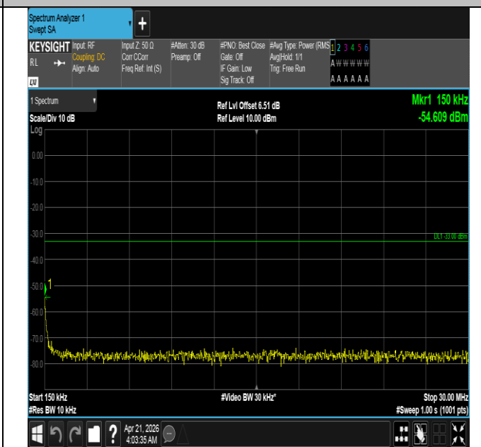
Band66-3MHz-QPSK-132657-1RB#0-0.15~30-PASS
