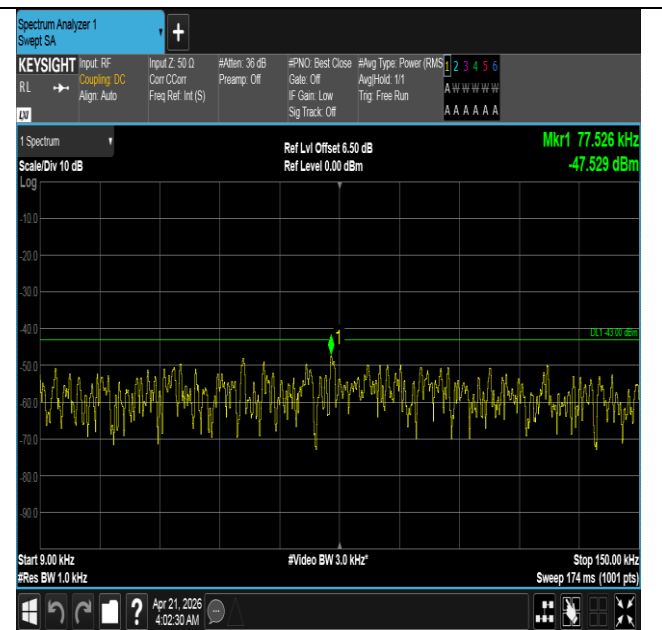
Band66-3MHz-16QAM-132322-15RB#0-0.009~0.15-PASS
