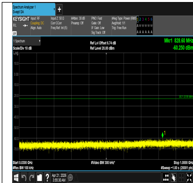
Band66-3MHz-16QAM-131987-1RB#14-30~1000-PASS
