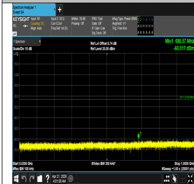
Band66-3MHz-16QAM-132322-1RB#14-30~1000-PASS
