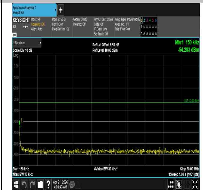
Band66-3MHz-QPSK-132322-15RB#0-0.15~30-PASS
