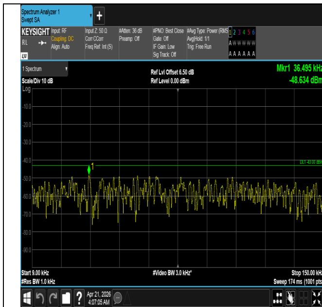
Band66-3MHz-QPSK-132657-15RB#0-0.009~0.15-PASS
