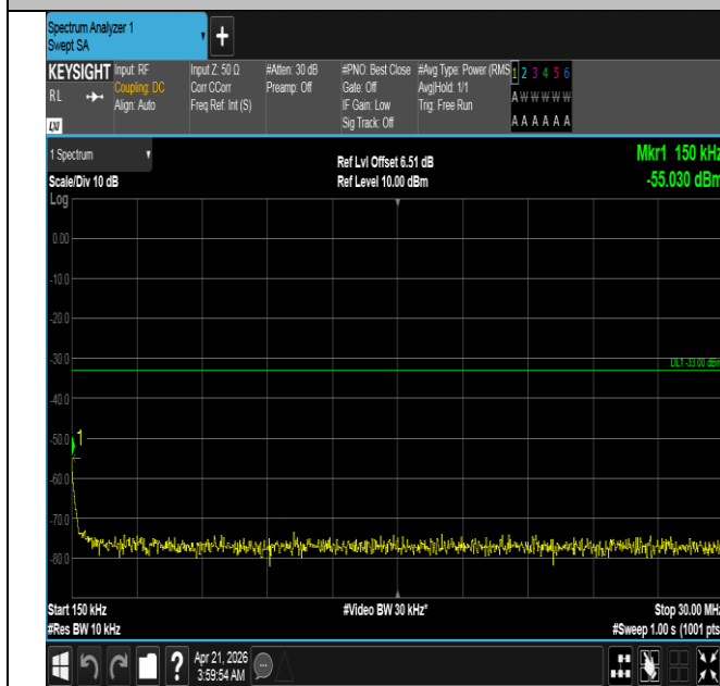
Band66-3MHz-QPSK-132322-1RB#14-0.15~30-PASS
