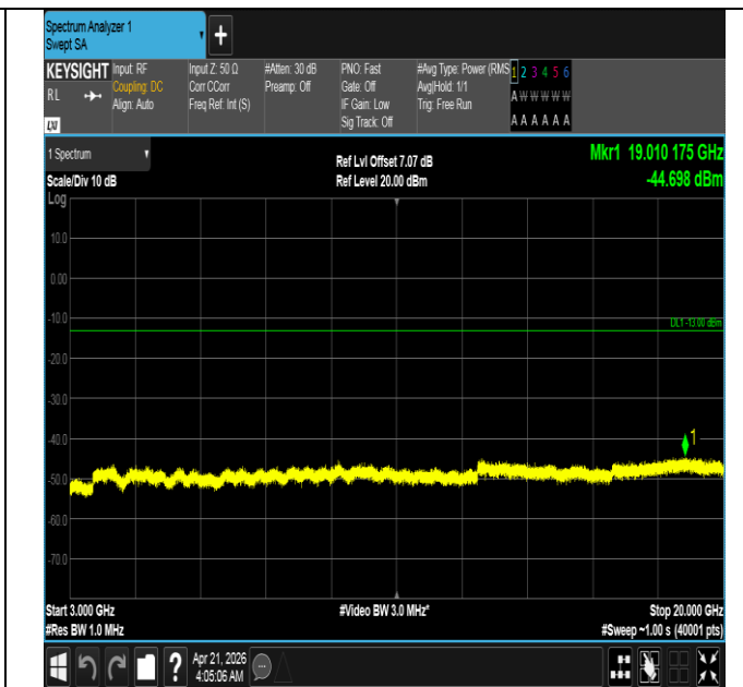
Band66-3MHz-16QAM-132657-1RB#0-3000~20000-PASS
