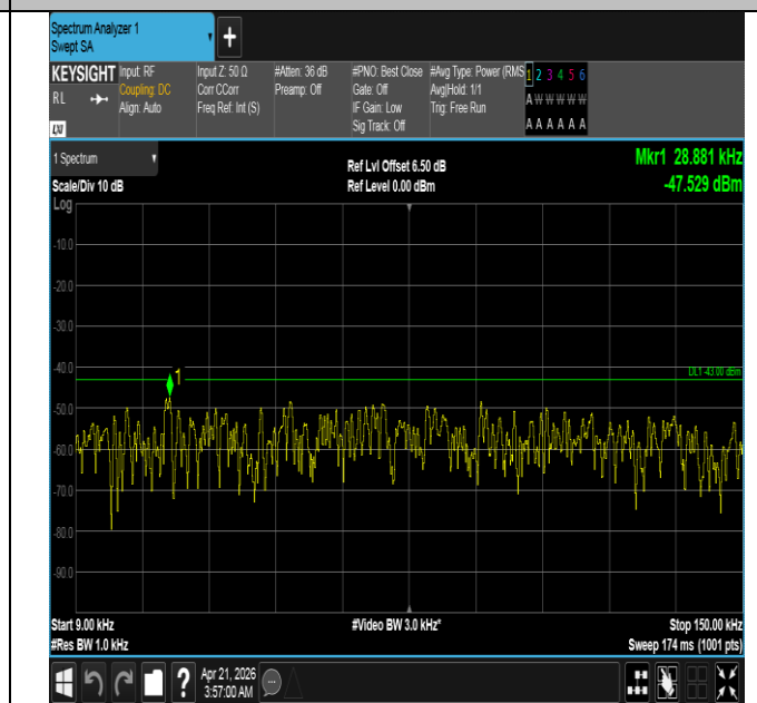
Band66-3MHz-16QAM-131987-15RB#0-0.009~0.15-PASS
