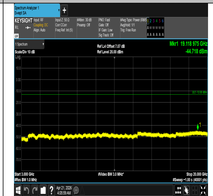
Band66-3MHz-QPSK-132657-1RB#14-3000~20000-PASS
