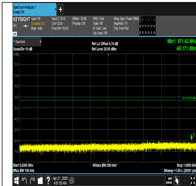
Band66-3MHz-QPSK-132322-15RB#0-30~1000-PASS
