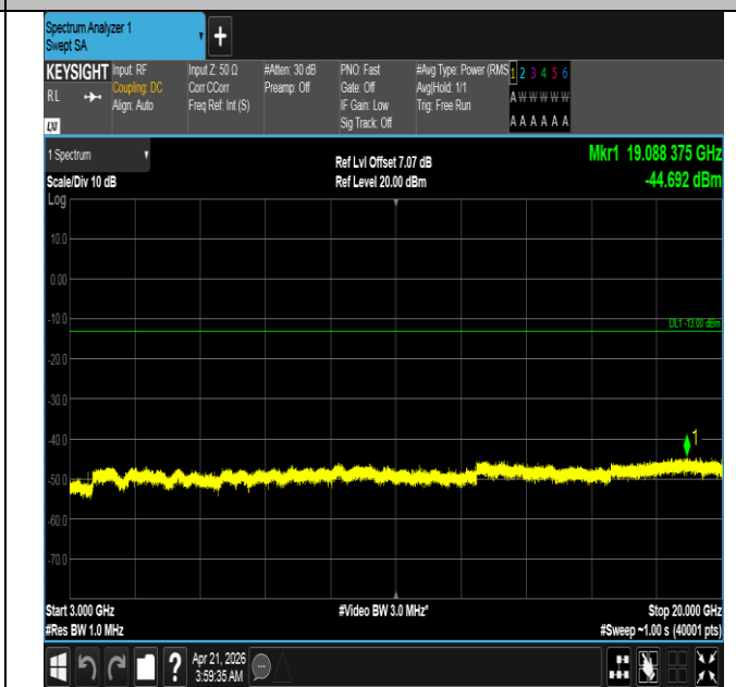
Band66-3MHz-16QAM-132322-1RB#0-3000~20000-PASS
