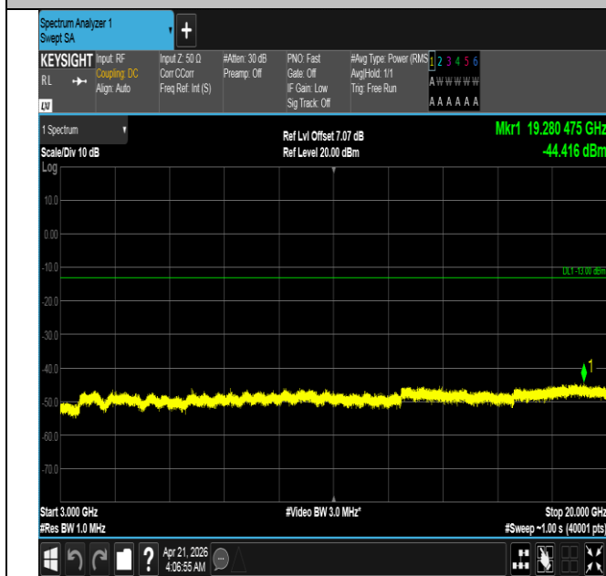
Band66-3MHz-16QAM-132657-1RB#14-3000~20000-PASS
