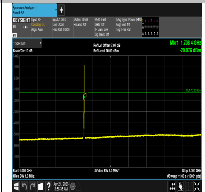
Band66-3MHz-QPSK-131987-15RB#0-1000~3000-PASS
