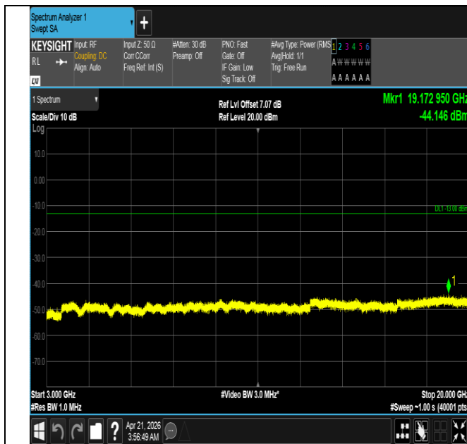
Band66-3MHz-QPSK-131987-15RB#0-3000~20000-PASS
