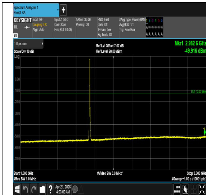
Band66-3MHz-16QAM-132322-15RB#0-1000~3000-PASS
