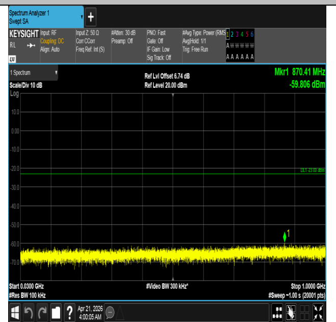
Band66-3MHz-QPSK-132322-1RB#14-30~1000-PASS
