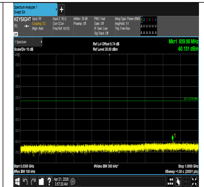
Band66-3MHz-16QAM-131987-15RB#0-30~1000-PASS
