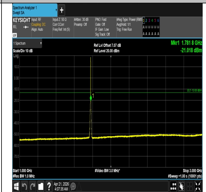
Band66-3MHz-QPSK-132657-15RB#0-1000~3000-PASS
