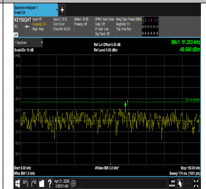
Band66-3MHz-16QAM-132322-1RB#0-0.009~0.15-PASS
