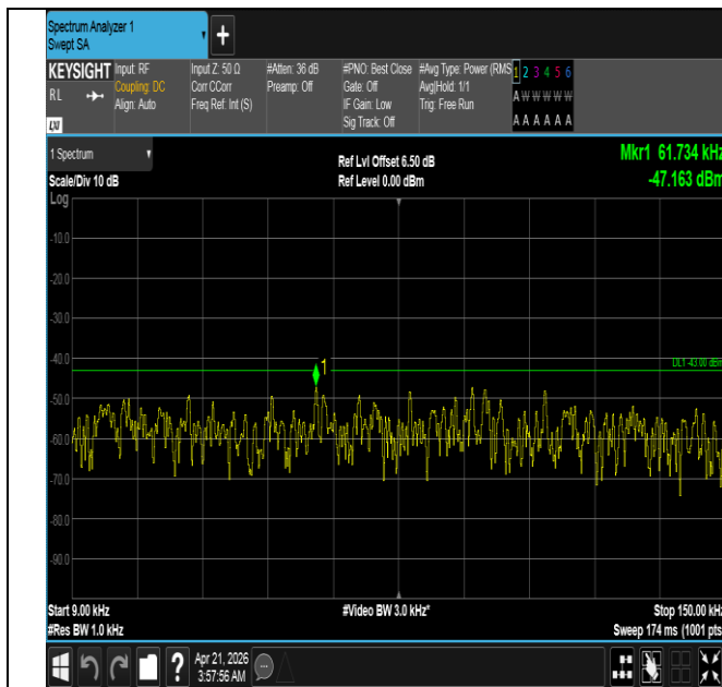
Band66-3MHz-QPSK-132322-1RB#0-0.009~0.15-PASS
