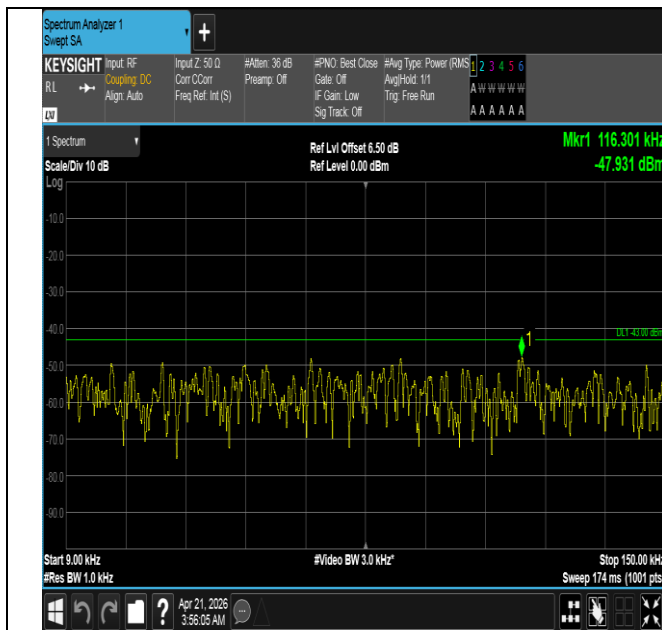
Band66-3MHz-QPSK-131987-15RB#0-0.009~0.15-PASS
