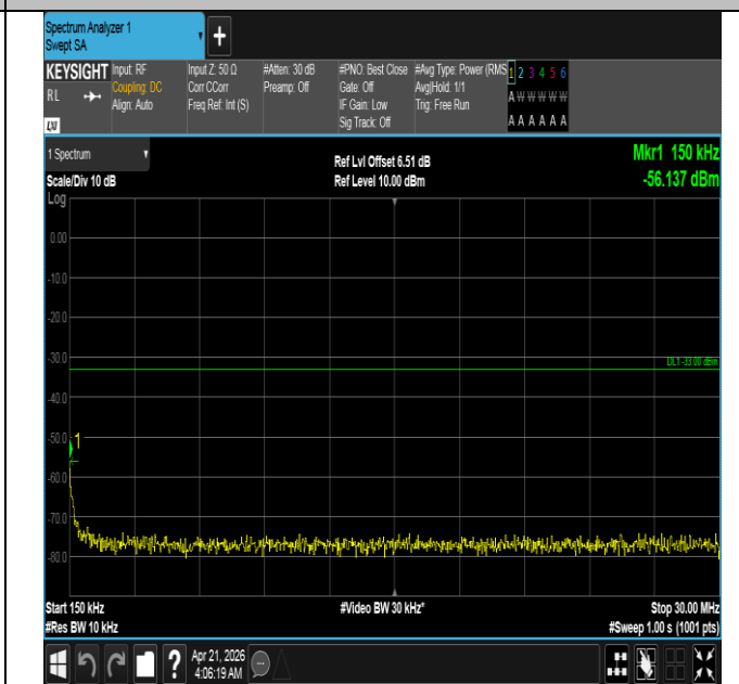
Band66-3MHz-16QAM-132657-1RB#14-0.15~30-PASS
