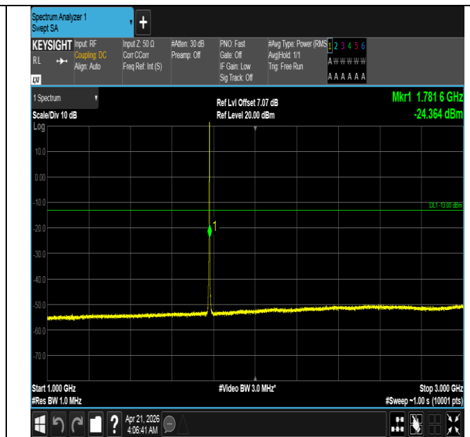
Band66-3MHz-16QAM-132657-1RB#14-1000~3000-PASS
