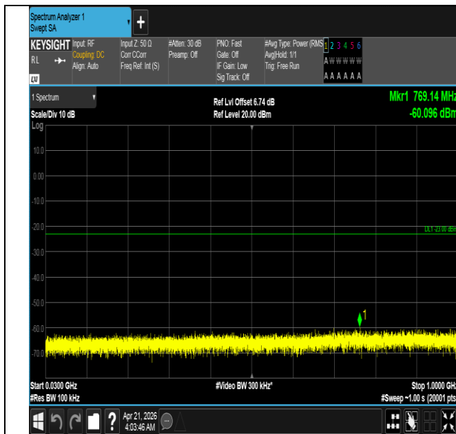
Band66-3MHz-QPSK-132657-1RB#0-30~1000-PASS
