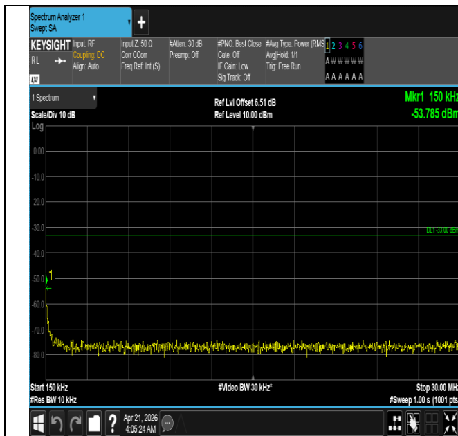
Band66-3MHz-QPSK-132657-1RB#14-0.15~30-PASS
