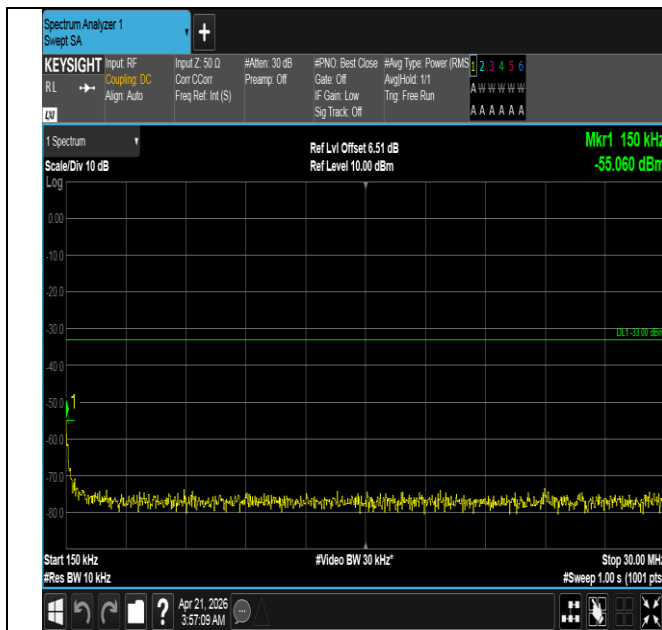
Band66-3MHz-16QAM-131987-15RB#0-0.15~30-PASS
