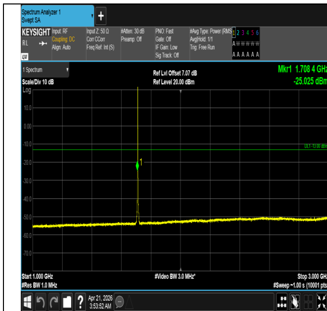
Band66-3MHz-16QAM-131987-1RB#0-1000~3000-PASS
