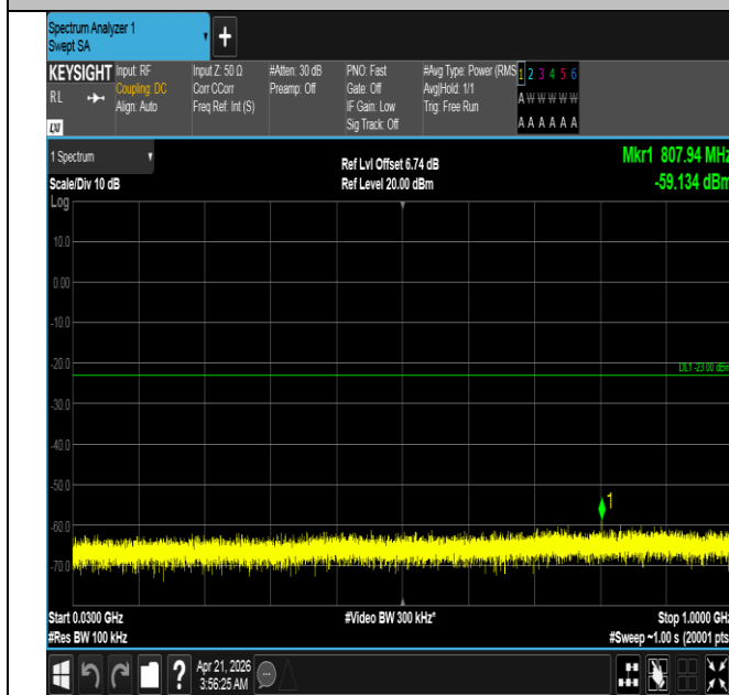
Band66-3MHz-QPSK-131987-15RB#0-30~1000-PASS
