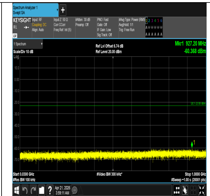
Band66-3MHz-16QAM-132322-1RB#0-30~1000-PASS
