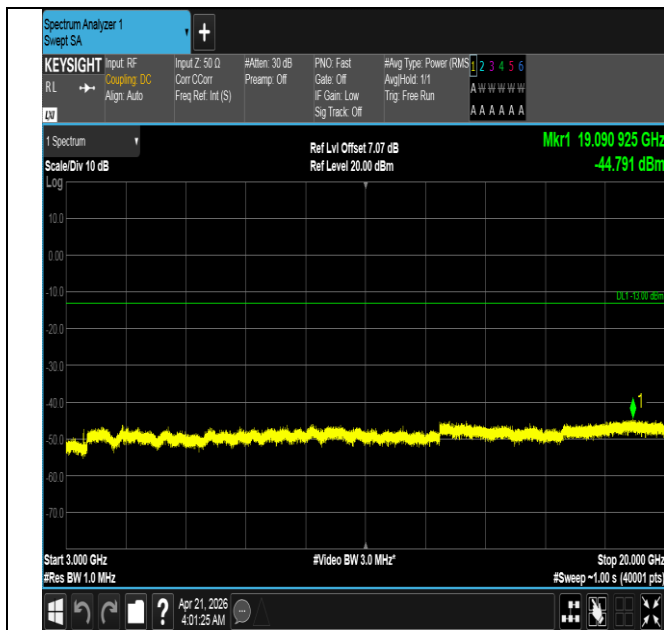
Band66-3MHz-16QAM-132322-1RB#14-3000~20000-PASS
