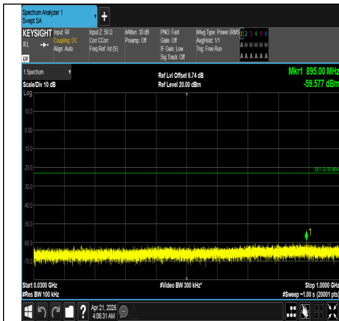
Band66-3MHz-16QAM-132657-1RB#14-30~1000-PASS
