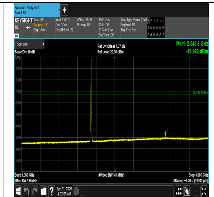
Band66-3MHz-QPSK-132322-15RB#0-1000~3000-PASS
