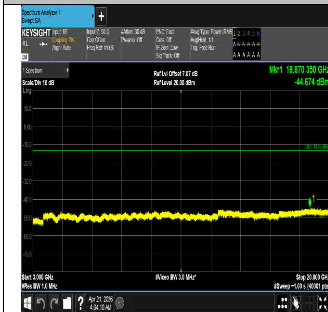
Band66-3MHz-QPSK-132657-1RB#0-3000~20000-PASS
