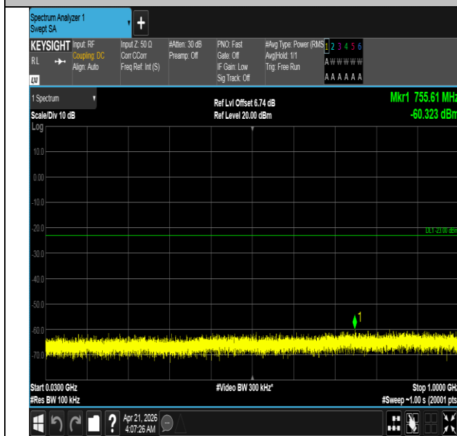
Band66-3MHz-QPSK-132657-15RB#0-30~1000-PASS
