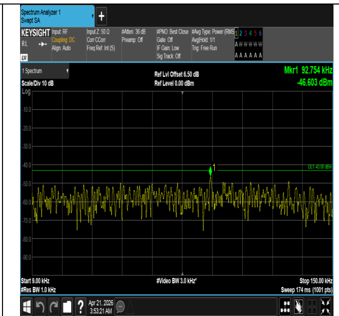
Band66-3MHz-16QAM-131987-1RB#0-0.009~0.15-PASS
