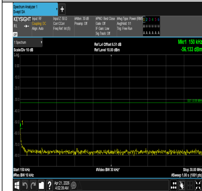
Band66-3MHz-16QAM-132322-15RB#0-0.15~30-PASS
