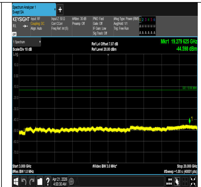
Band66-3MHz-QPSK-132322-1RB#14-3000~20000-PASS
