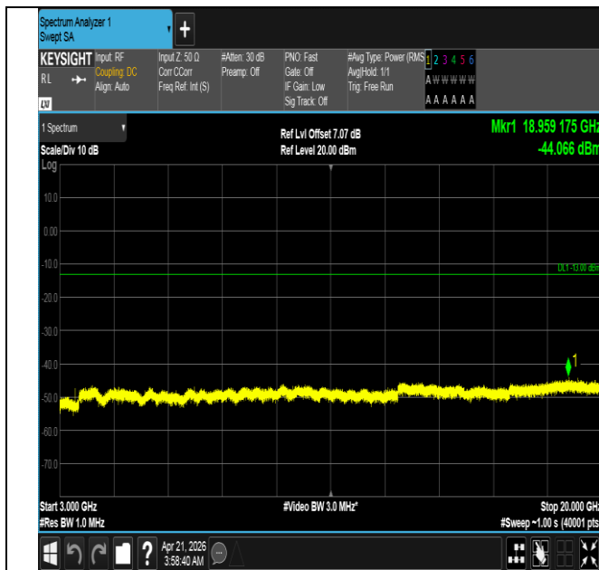
Band66-3MHz-QPSK-132322-1RB#0-3000~20000-PASS
