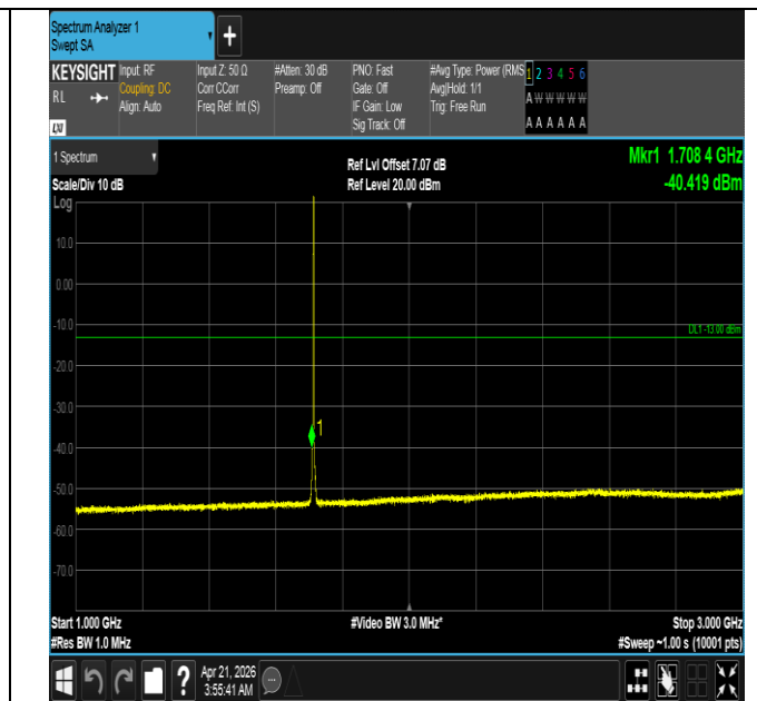
Band66-3MHz-16QAM-131987-1RB#14-1000~3000-PASS
