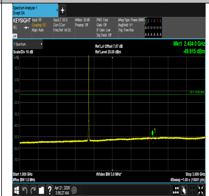
Band66-3MHz-QPSK-132322-1RB#0-1000~3000-PASS
