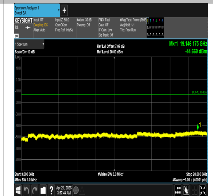
Band66-3MHz-16QAM-131987-15RB#0-3000~20000-PASS
