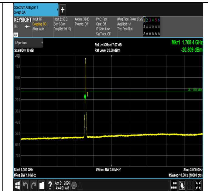
Band66-5MHz-QPSK-131997-25RB#0-1000~3000-PASS
