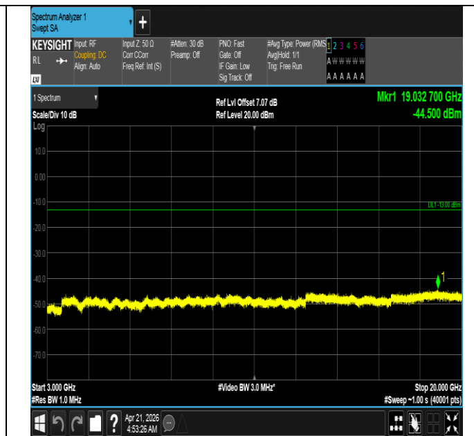
Band66-5MHz-QPSK-132647-1RB#24-3000~20000-PASS
