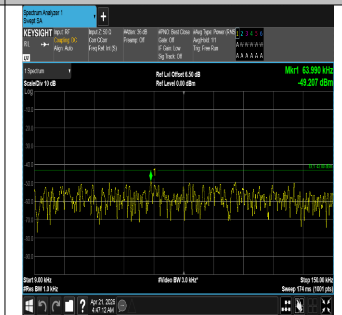
Band66-5MHz-QPSK-132322-1RB#24-0.009~0.15-PASS
