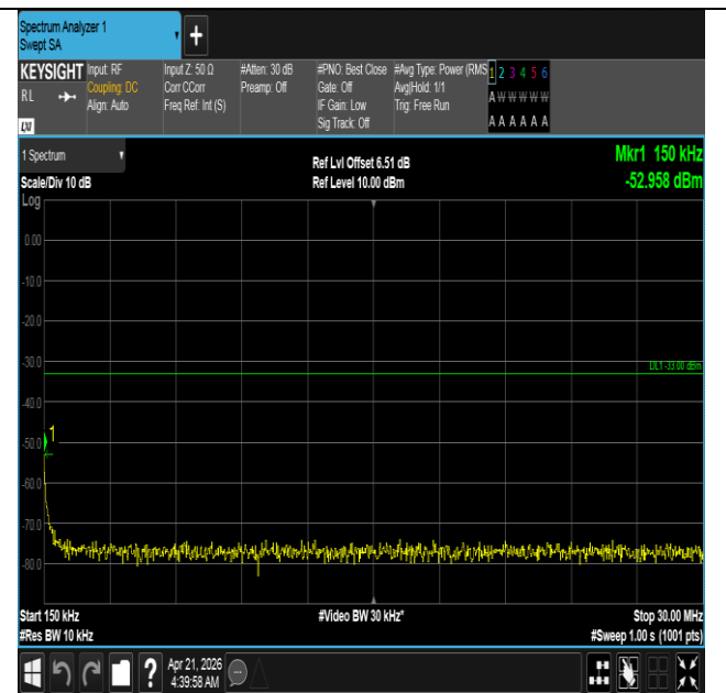
Band66-5MHz-QPSK-131997-1RB#0-0.15~30-PASS
