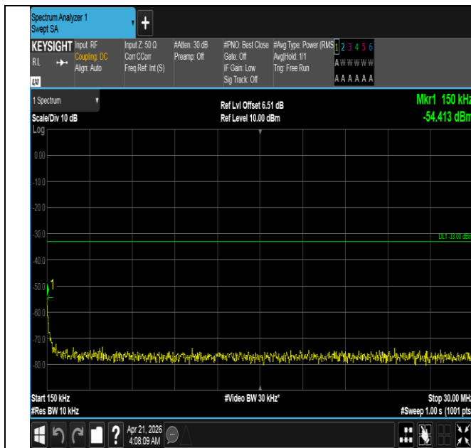
Band66-3MHz-16QAM-132657-15RB#0-0.15~30-PASS
