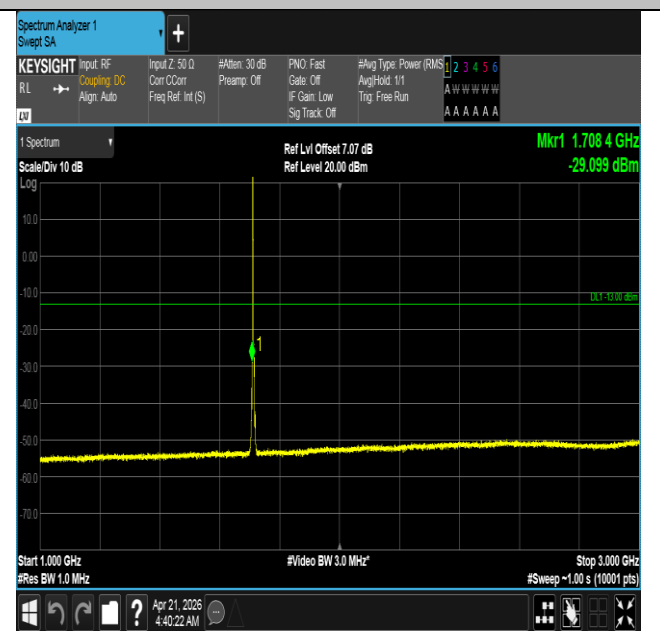
Band66-5MHz-QPSK-131997-1RB#0-1000~3000-PASS
