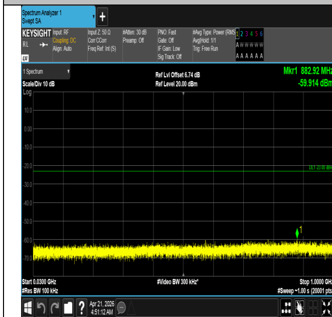
Band66-5MHz-QPSK-132647-1RB#0-30~1000-PASS
