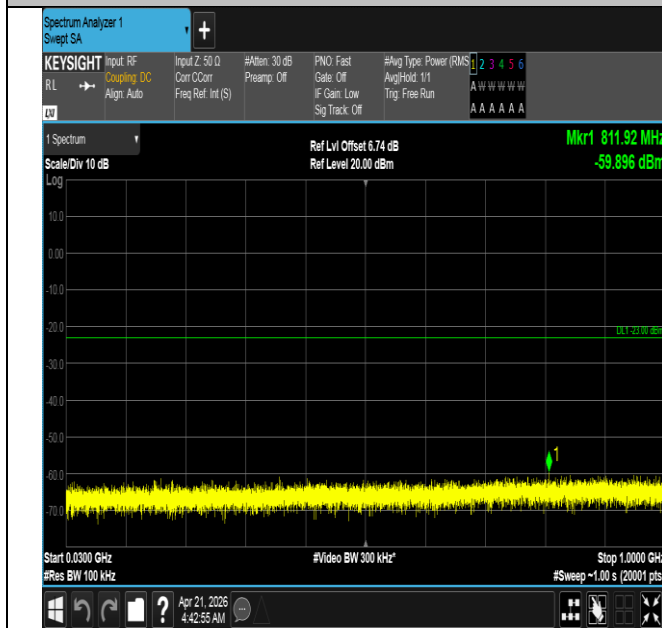
Band66-5MHz-16QAM-131997-1RB#24-30~1000-PASS
