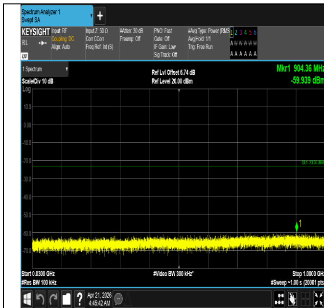
Band66-5MHz-QPSK-132322-1RB#0-30~1000-PASS
