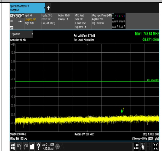
Band66-5MHz-QPSK-131997-1RB#24-30~1000-PASS
