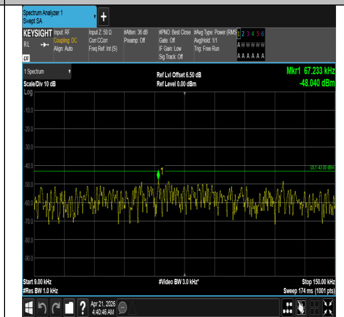
Band66-5MHz-16QAM-131997-1RB#0-0.009~0.15-PASS
