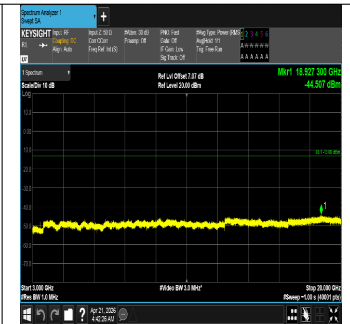
Band66-5MHz-QPSK-131997-1RB#24-3000~20000-PASS
