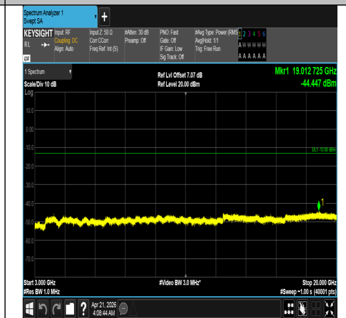
Band66-3MHz-16QAM-132657-15RB#0-3000~20000-PASS
