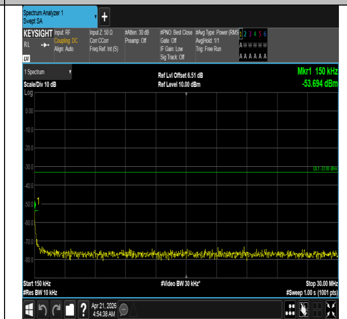
Band66-5MHz-QPSK-132647-25RB#0-0.15~30-PASS
