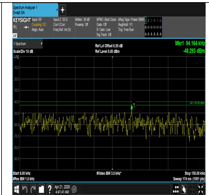
Band66-5MHz-QPSK-131997-1RB#24-0.009~0.15-PASS
