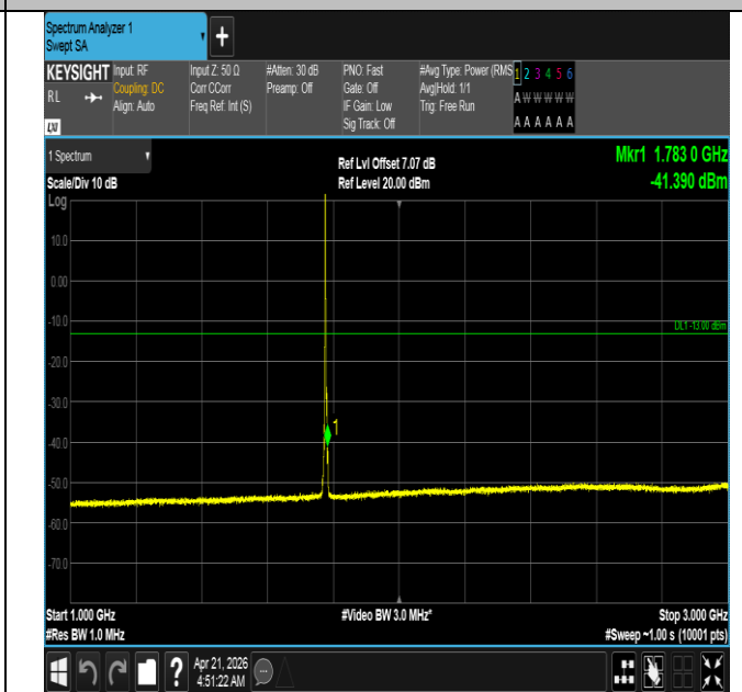
Band66-5MHz-QPSK-132647-1RB#0-1000~3000-PASS
