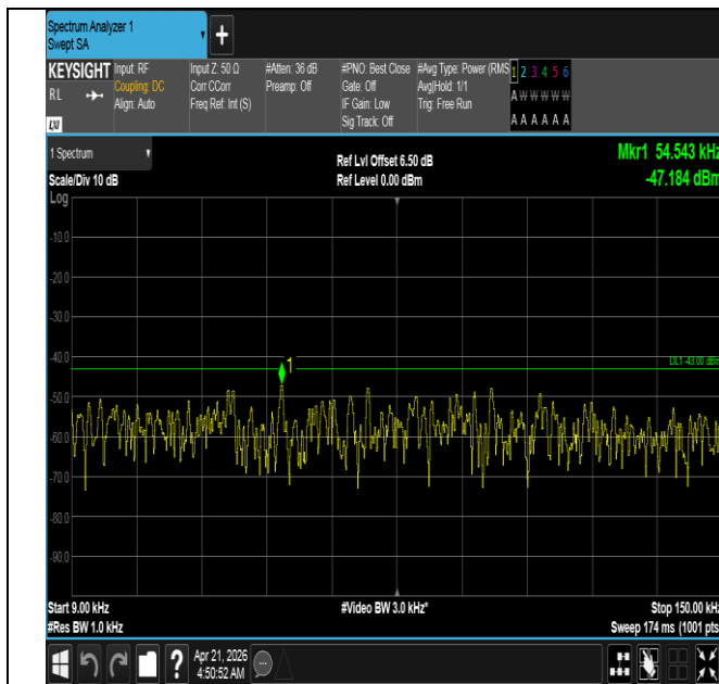
Band66-5MHz-QPSK-132647-1RB#0-0.009~0.15-PASS
