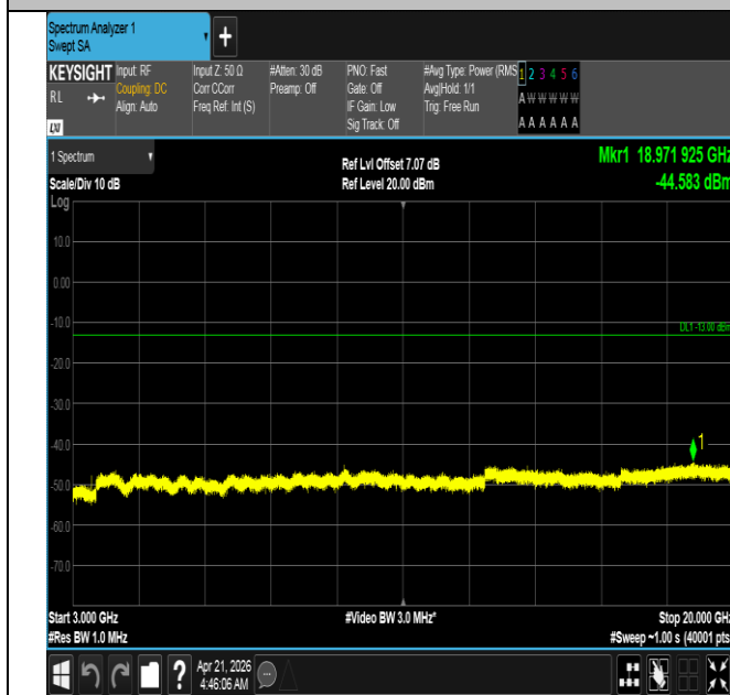
Band66-5MHz-QPSK-132322-1RB#0-3000~20000-PASS
