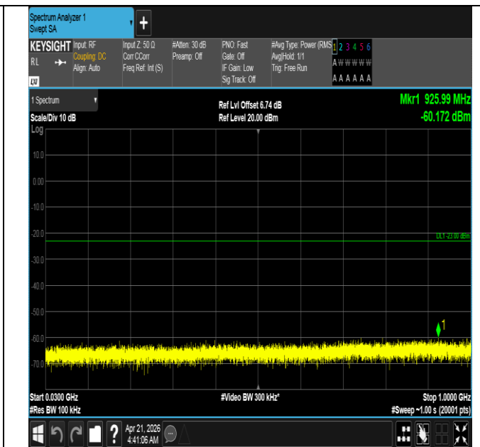
Band66-5MHz-16QAM-131997-1RB#0-30~1000-PASS
