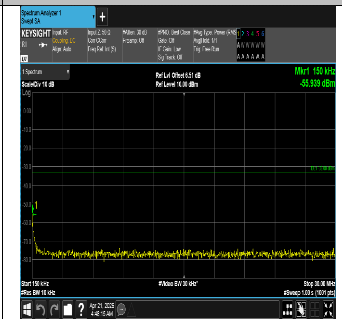
Band66-5MHz-16QAM-132322-1RB#24-0.15~30-PASS
