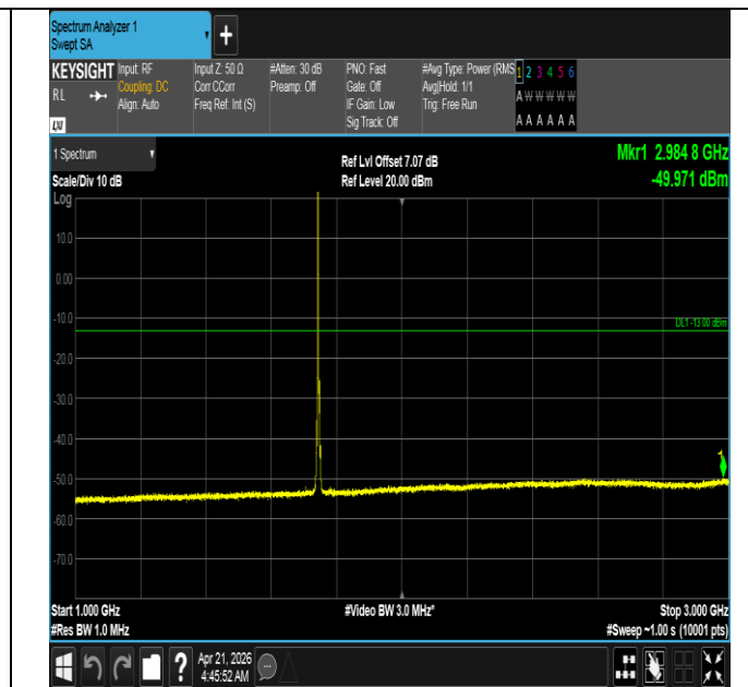
Band66-5MHz-QPSK-132322-1RB#0-1000~3000-PASS
