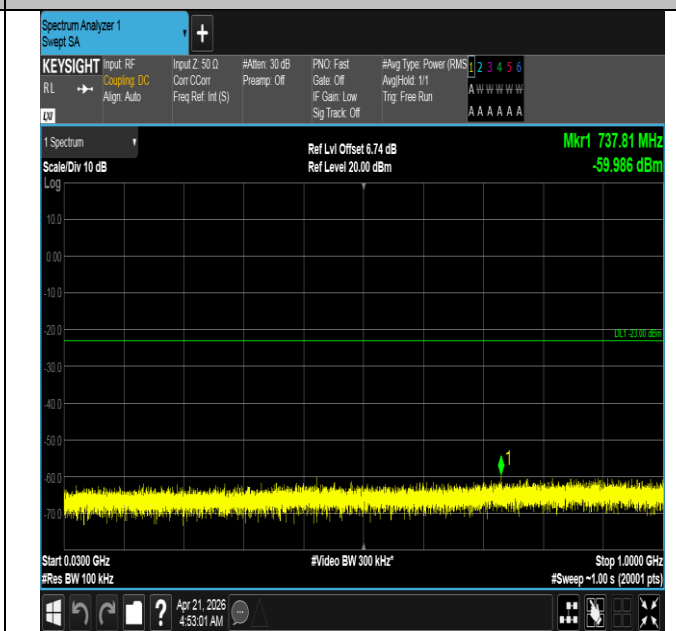
Band66-5MHz-QPSK-132647-1RB#24-30~1000-PASS
