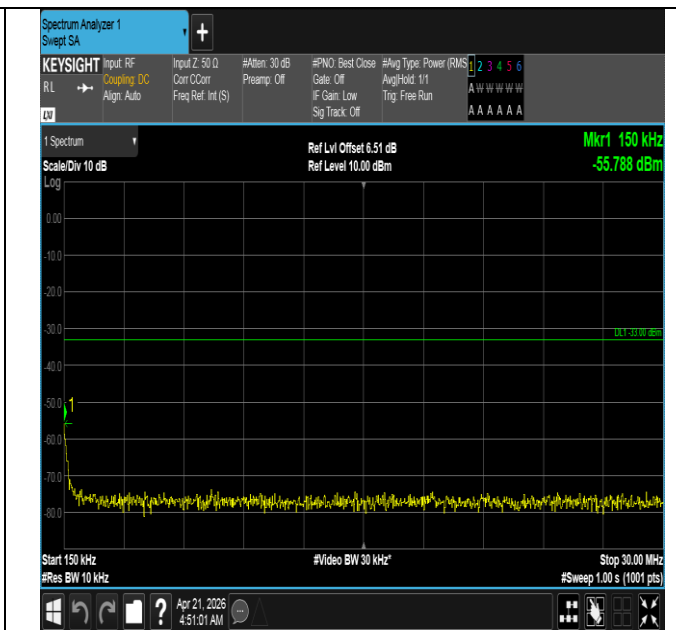
Band66-5MHz-QPSK-132647-1RB#0-0.15~30-PASS
