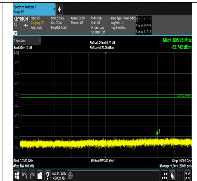
Band66-3MHz-16QAM-132657-15RB#0-30~1000-PASS
