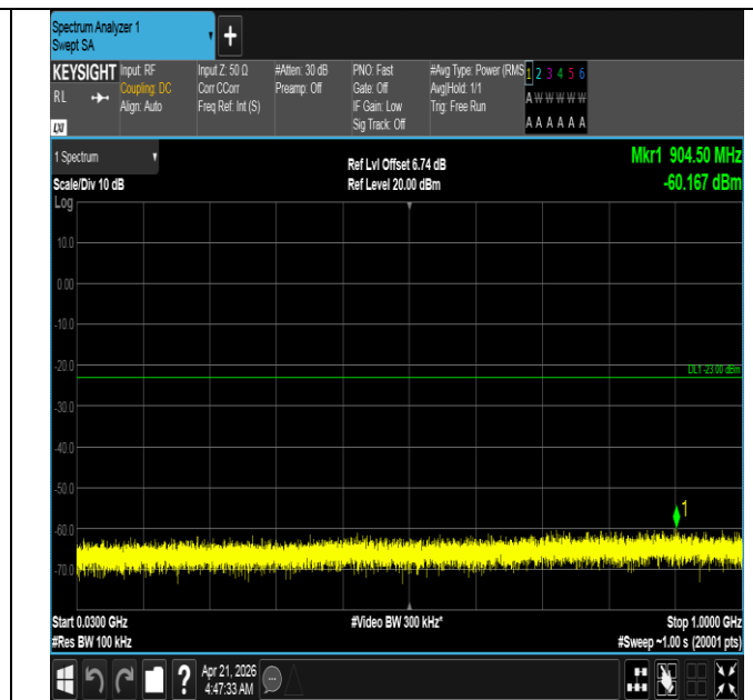
Band66-5MHz-QPSK-132322-1RB#24-30~1000-PASS
