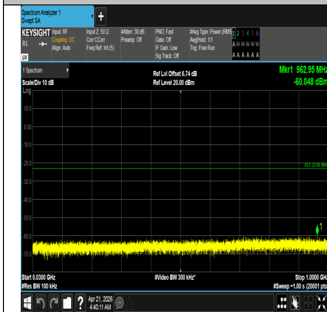
Band66-5MHz-QPSK-131997-1RB#0-30~1000-PASS
