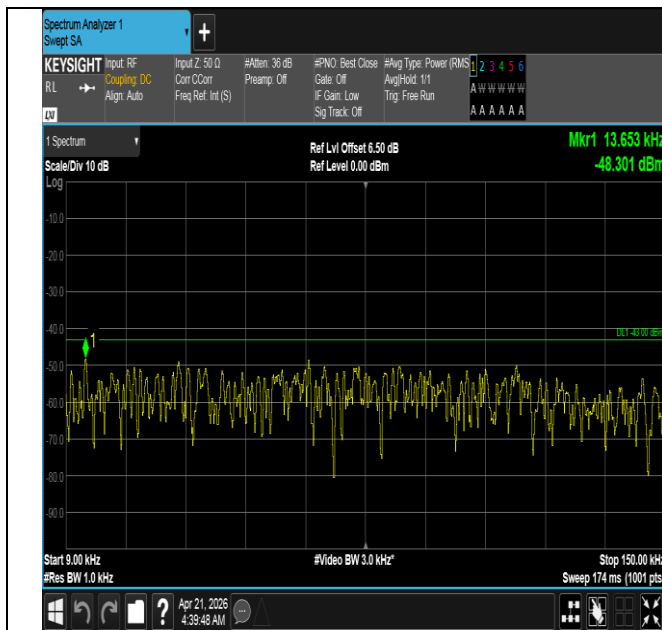
Band66-5MHz-QPSK-131997-1RB#0-0.009~0.15-PASS
