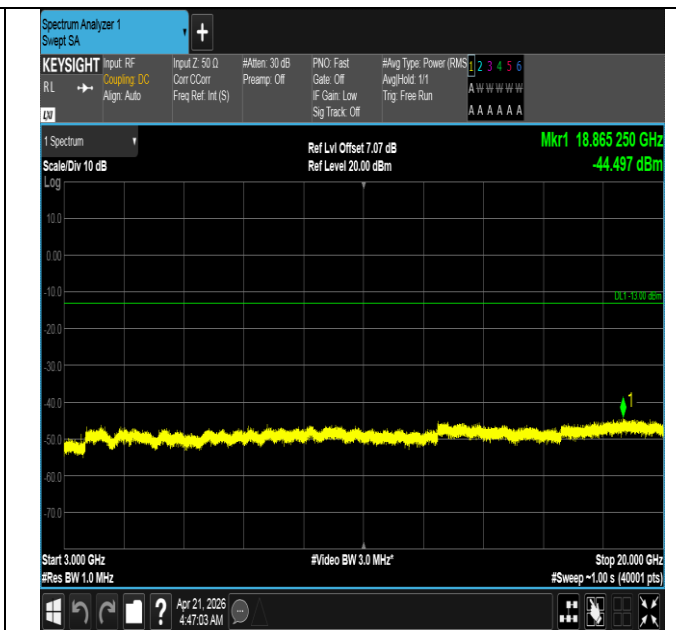
Band66-5MHz-16QAM-132322-1RB#0-3000~20000-PASS
