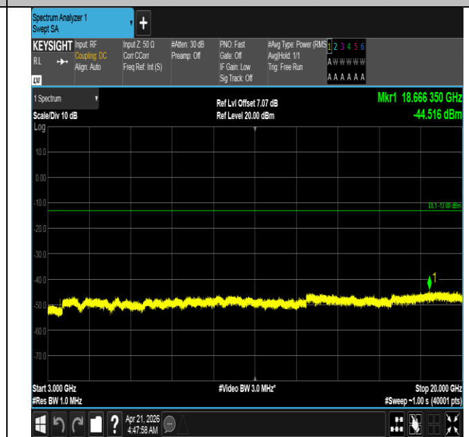
Band66-5MHz-QPSK-132322-1RB#24-3000~20000-PASS
