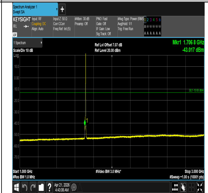
Band66-5MHz-16QAM-131997-1RB#24-1000~3000-PASS
