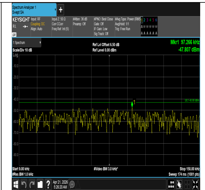
Band66-10MHz-16QAM-132022-1RB#0-0.009~0.15-PASS
