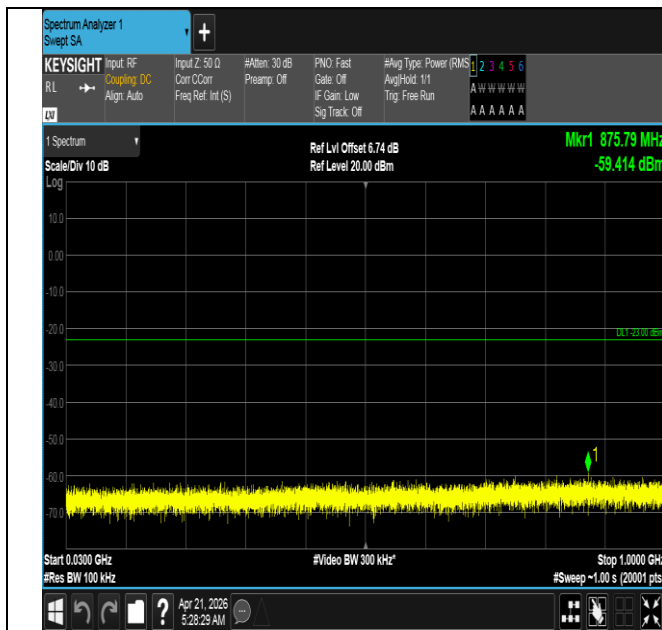
Band66-10MHz-16QAM-132022-1RB#49-30~1000-PASS
