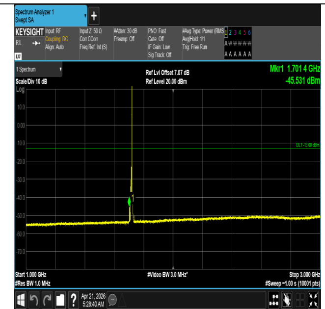
Band66-10MHz-16QAM-132022-1RB#49-1000~3000-PASS
