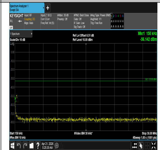
Band66-10MHz-QPSK-132022-1RB#0-0.15~30-PASS
