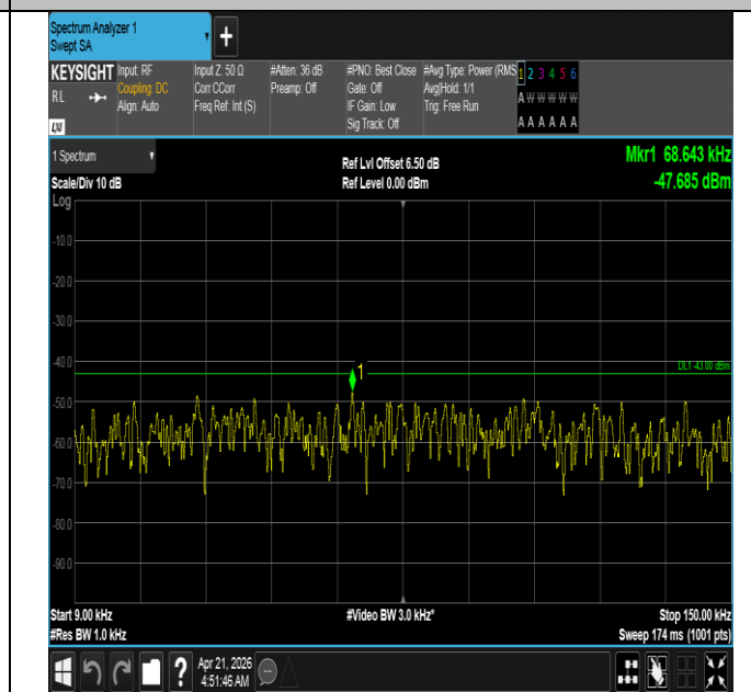
Band66-5MHz-16QAM-132647-1RB#0-0.009~0.15-PASS
