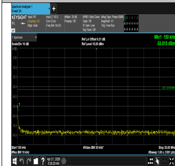
Band66-10MHz-16QAM-132022-1RB#0-0.15~30-PASS
