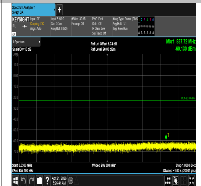
Band66-10MHz-16QAM-132022-1RB#0-30~1000-PASS
