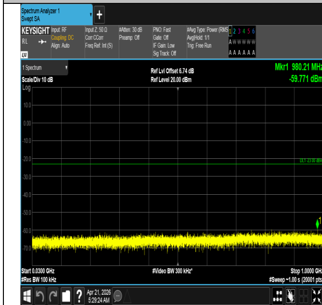
Band66-10MHz-QPSK-132022-50RB#0-30~1000-PASS
