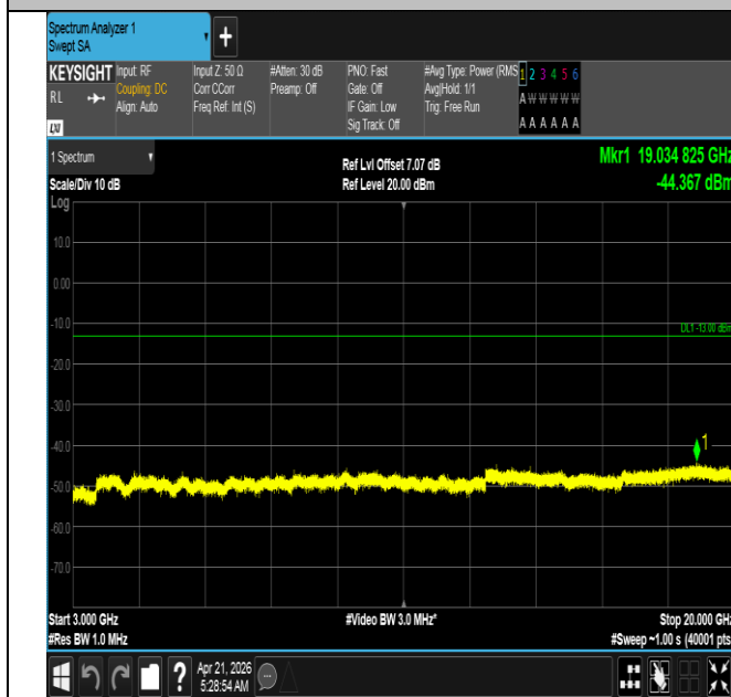
Band66-10MHz-16QAM-132022-1RB#49-3000~20000-PASS
