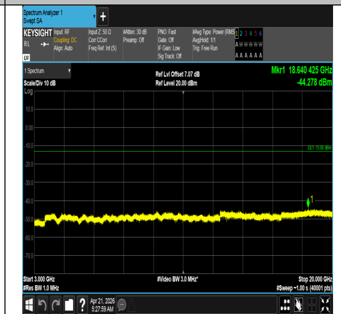
Band66-10MHz-QPSK-132022-1RB#49-3000~20000-PASS
