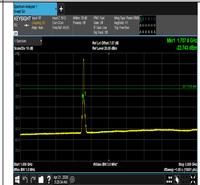
Band66-10MHz-QPSK-132022-50RB#0-1000~3000-PASS
