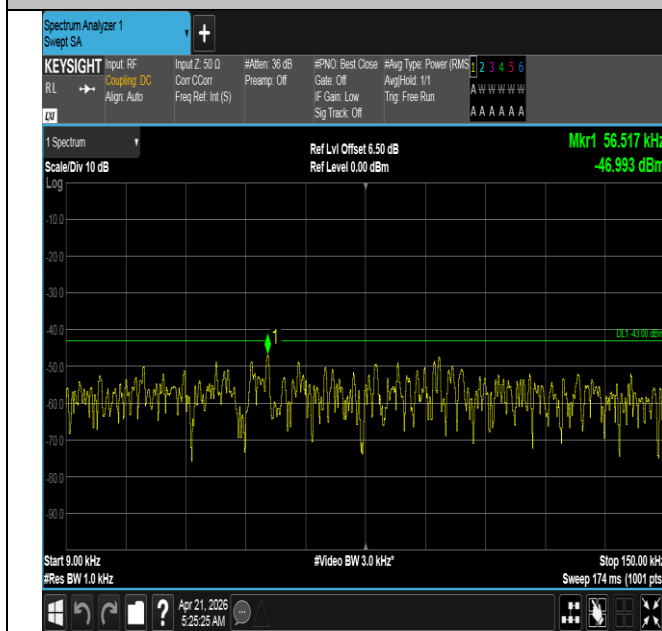
Band66-10MHz-QPSK-132022-1RB#0-0.009~0.15-PASS
