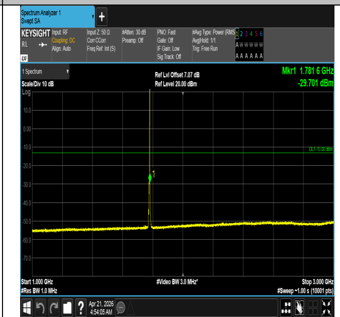
Band66-5MHz-16QAM-132647-1RB#24-1000~3000-PASS
