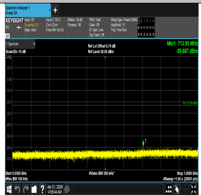
Band66-5MHz-16QAM-132647-25RB#0-30~1000-PASS
