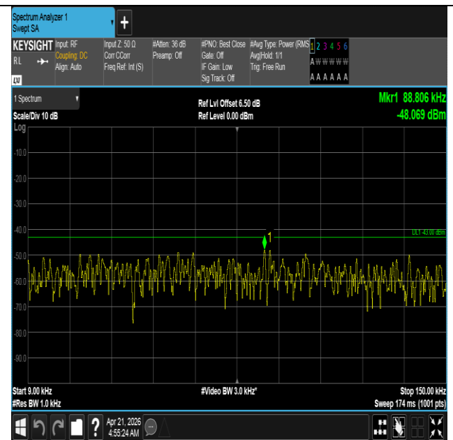
Band66-5MHz-16QAM-132647-25RB#0-0.009~0.15-PASS
