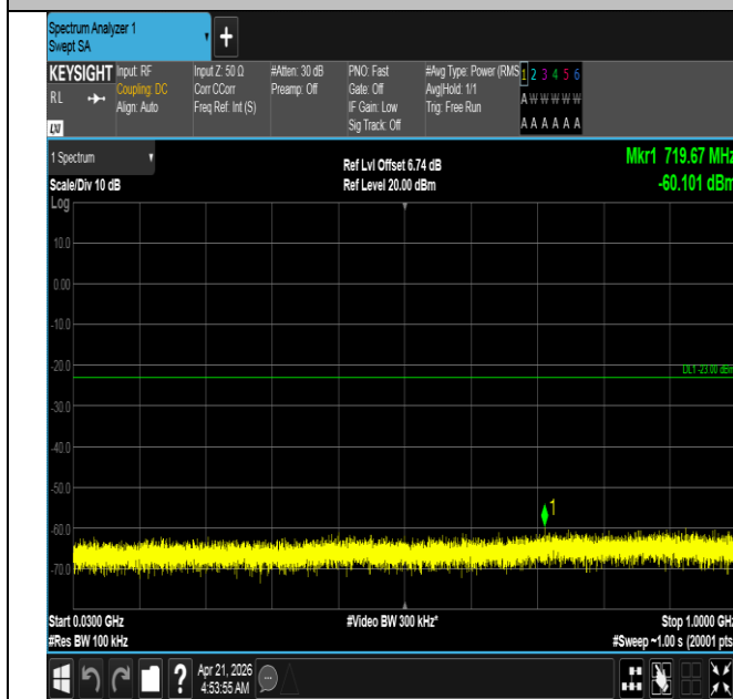
Band66-5MHz-16QAM-132647-1RB#24-30~1000-PASS
