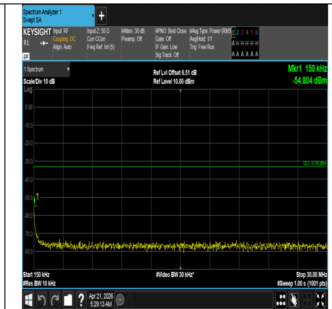
Band66-10MHz-QPSK-132022-50RB#0-0.15~30-PASS
