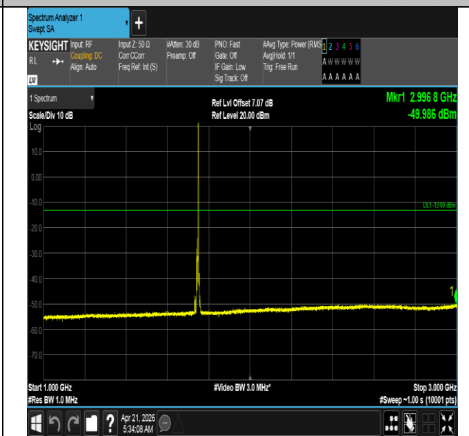
Band66-10MHz-16QAM-132322-1RB#49-1000~3000-PASS
