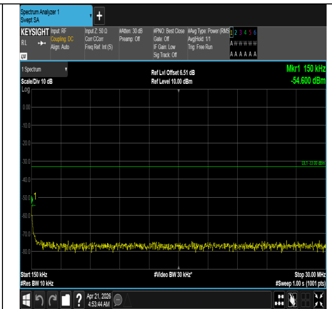
Band66-5MHz-16QAM-132647-1RB#24-0.15~30-PASS
