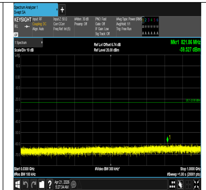
Band66-10MHz-QPSK-132022-1RB#49-30~1000-PASS
