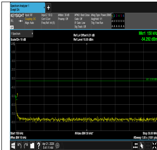
Band66-10MHz-16QAM-132622-50RB#0-0.15~30-PASS
