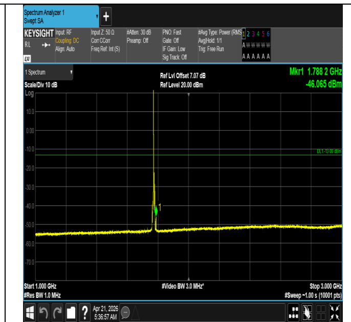
Band66-10MHz-QPSK-132622-1RB#0-1000~3000-PASS
