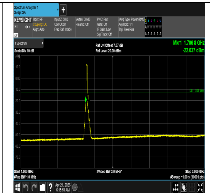
Band66-15MHz-QPSK-132047-75RB#0-1000~3000-PASS
