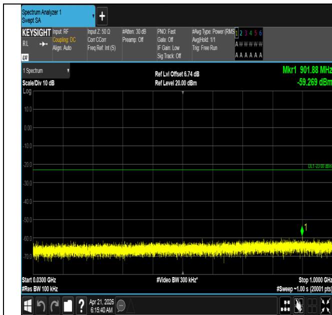
Band66-15MHz-QPSK-132047-75RB#0-30~1000-PASS
