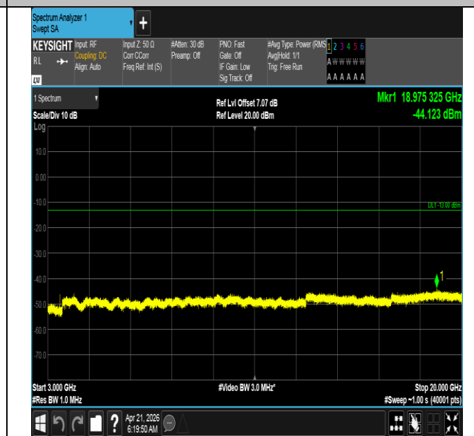
Band66-15MHz-QPSK-132322-1RB#74-3000~20000-PASS
