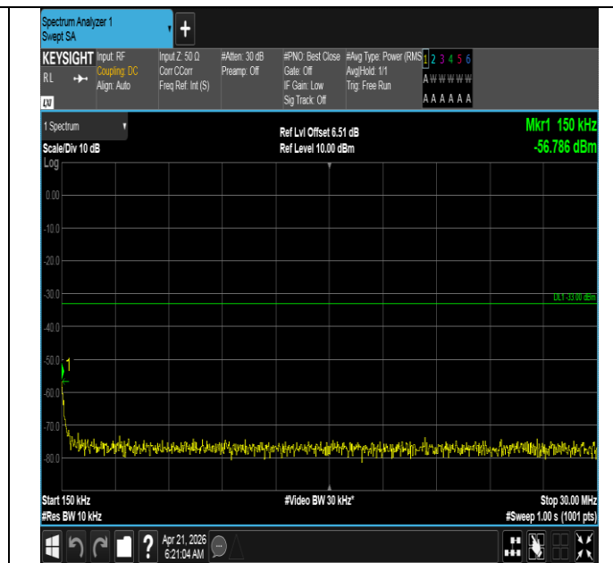
Band66-15MHz-QPSK-132322-75RB#0-0.15~30-PASS
