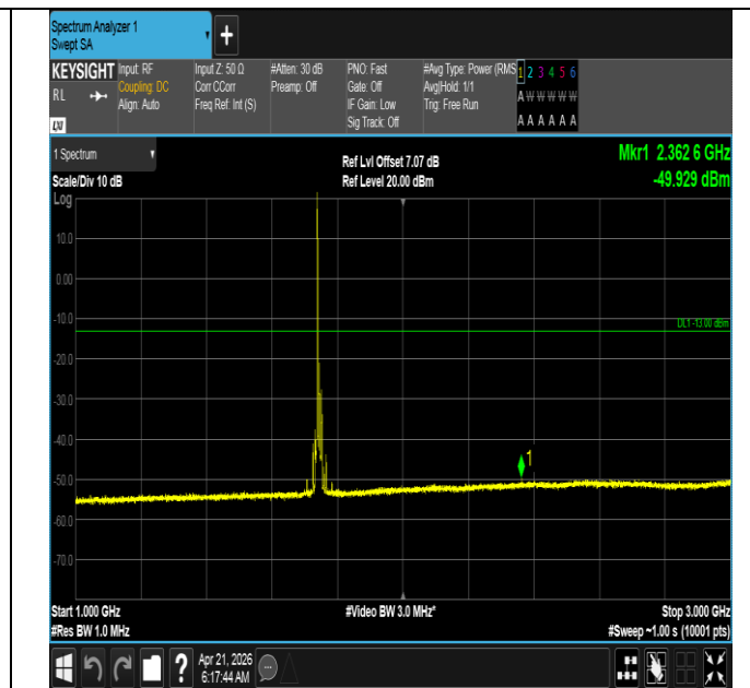
Band66-15MHz-QPSK-132322-1RB#0-1000~3000-PASS
