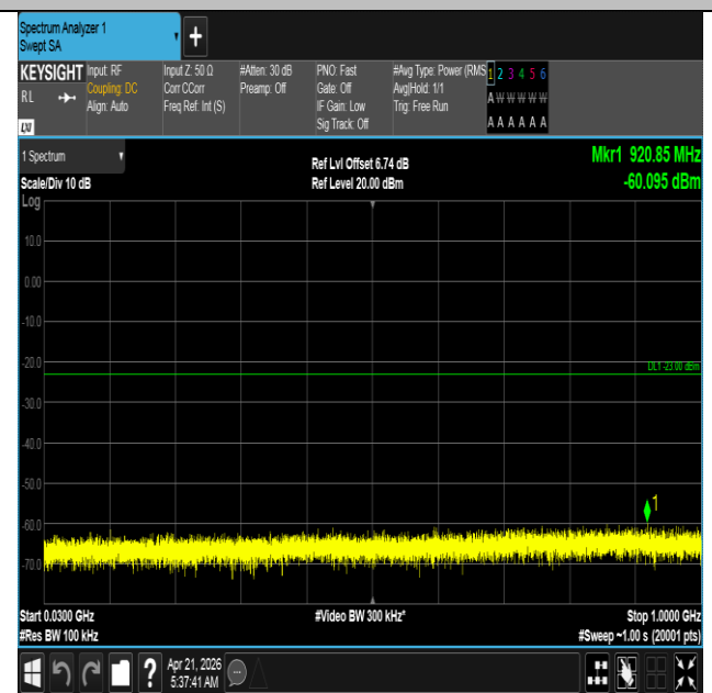
Band66-10MHz-16QAM-132622-1RB#0-30~1000-PASS
