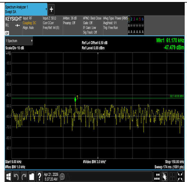
Band66-10MHz-16QAM-132622-1RB#0-0.009~0.15-PASS
