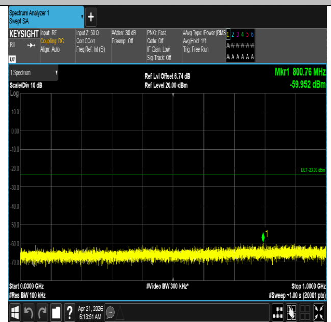
Band66-15MHz-QPSK-132047-1RB#74-30~1000-PASS
