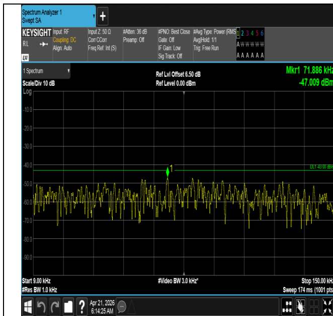
Band66-15MHz-16QAM-132047-1RB#74-0.009~0.15-PASS
