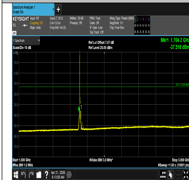
Band66-15MHz-16QAM-132047-1RB#0-1000~3000-PASS
