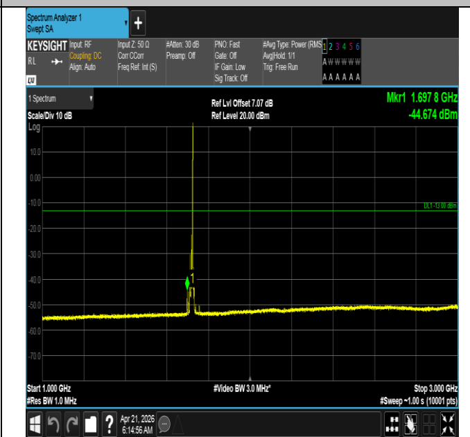
Band66-15MHz-16QAM-132047-1RB#74-1000~3000-PASS
