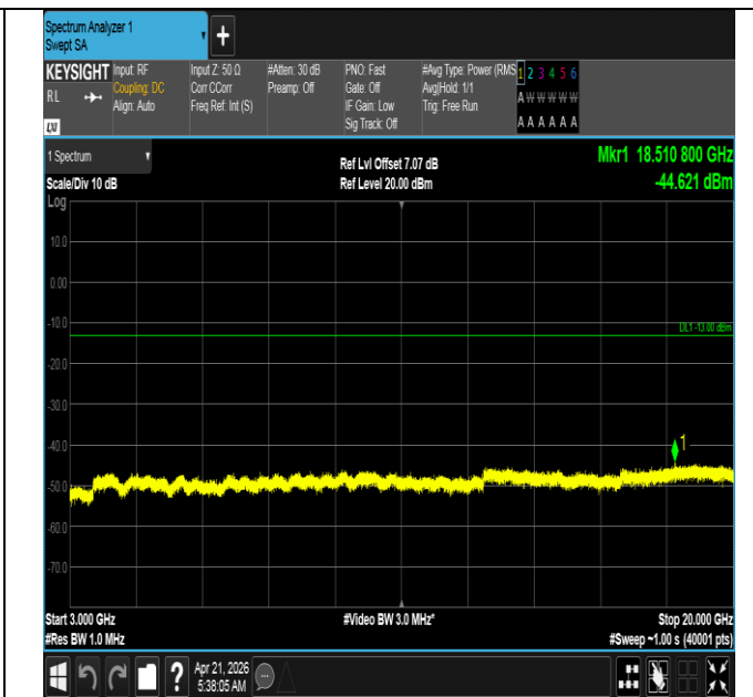
Band66-10MHz-16QAM-132622-1RB#0-3000~20000-PASS
