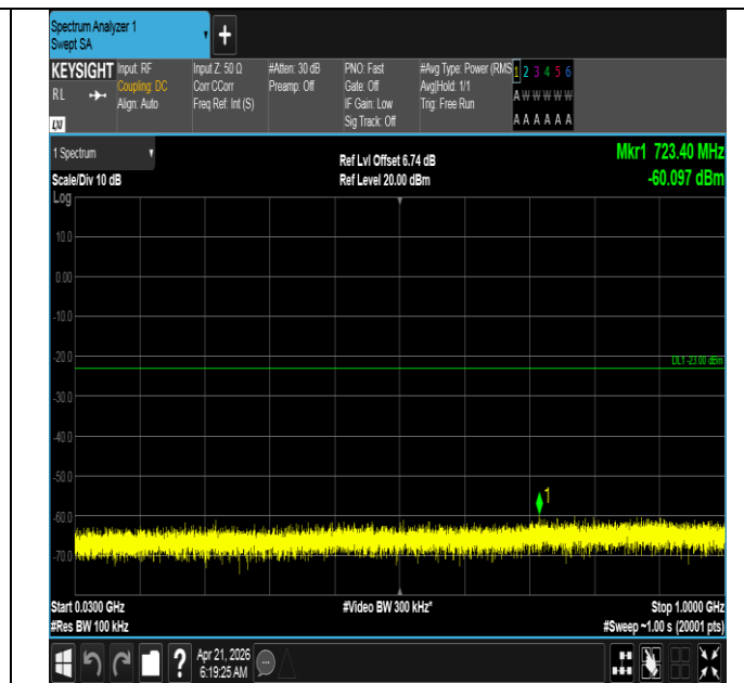
Band66-15MHz-QPSK-132322-1RB#74-30~1000-PASS
