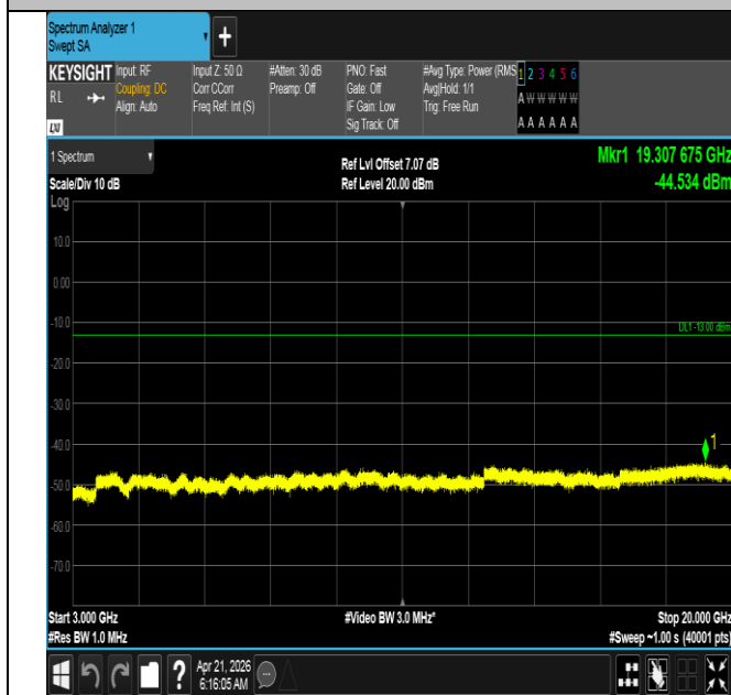
Band66-15MHz-QPSK-132047-75RB#0-3000~20000-PASS
