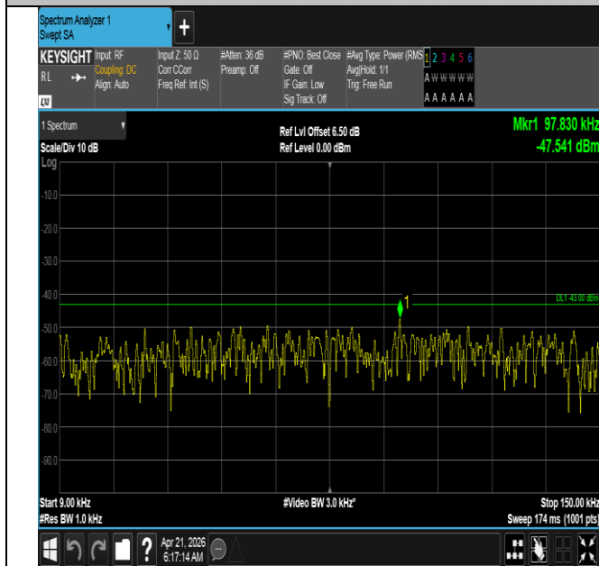
Band66-15MHz-QPSK-132322-1RB#0-0.009~0.15-PASS
