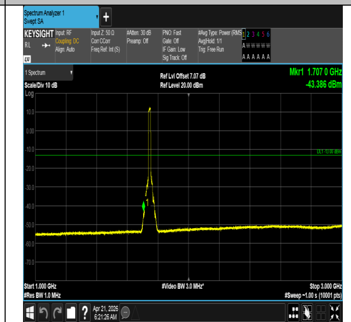
Band66-15MHz-QPSK-132322-75RB#0-1000~3000-PASS
