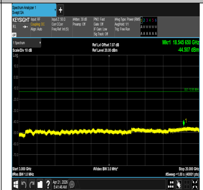
Band66-10MHz-16QAM-132622-50RB#0-3000~20000-PASS
