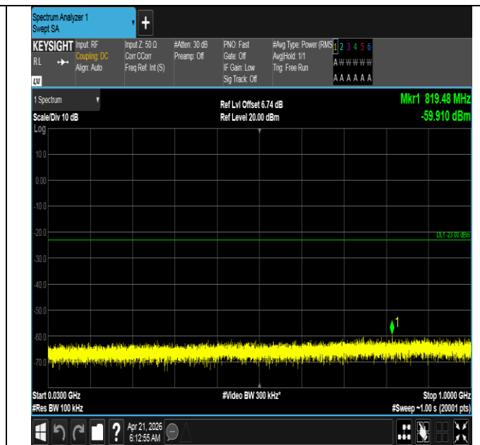
Band66-15MHz-16QAM-132047-1RB#0-30~1000-PASS
