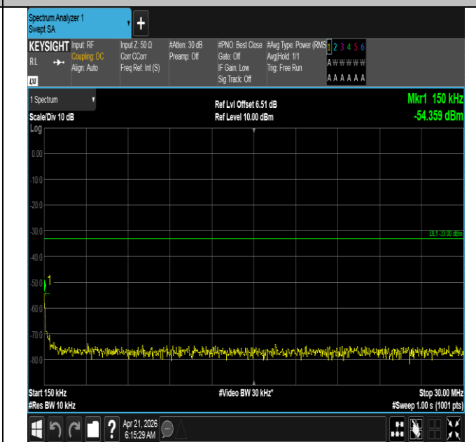
Band66-15MHz-QPSK-132047-75RB#0-0.15~30-PASS
