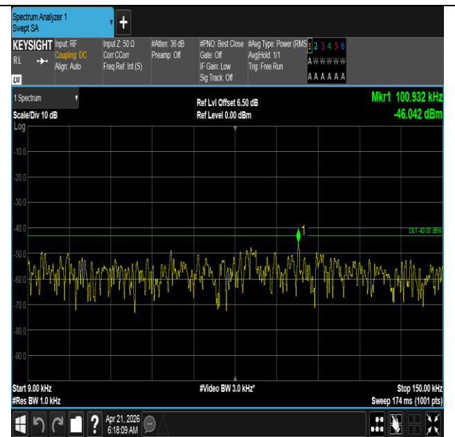
Band66-15MHz-16QAM-132322-1RB#0-0.009~0.15-PASS
