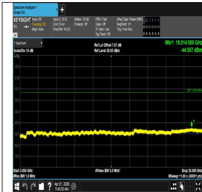
Band66-10MHz-QPSK-132622-50RB#0-3000~20000-PASS
