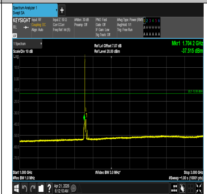
Band66-15MHz-QPSK-132047-1RB#0-1000~3000-PASS
