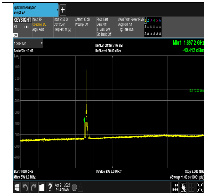
Band66-15MHz-QPSK-132047-1RB#74-1000~3000-PASS
