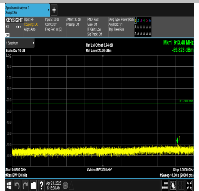
Band66-15MHz-16QAM-132322-1RB#0-30~1000-PASS
