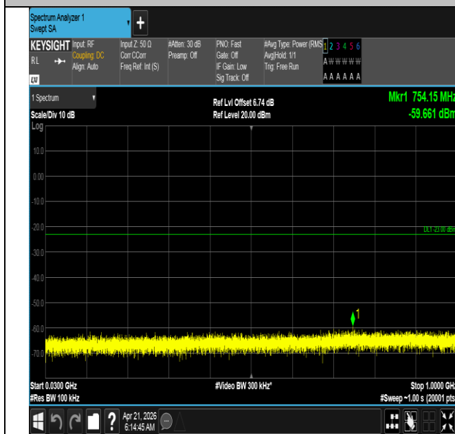
Band66-15MHz-16QAM-132047-1RB#74-30~1000-PASS
