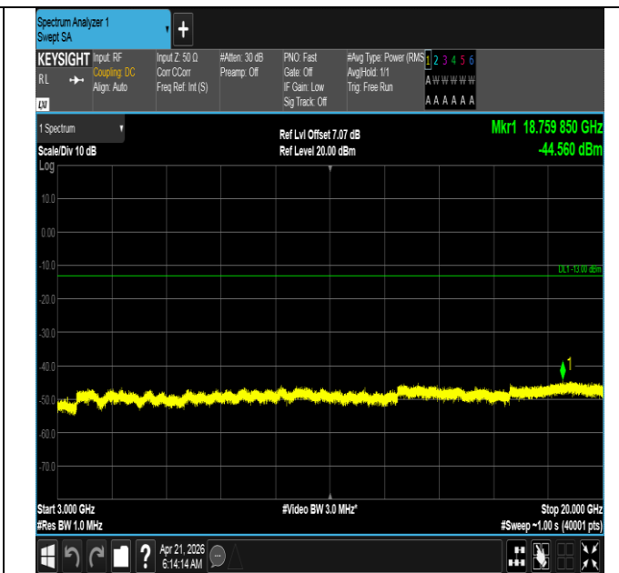
Band66-15MHz-QPSK-132047-1RB#74-3000~20000-PASS
