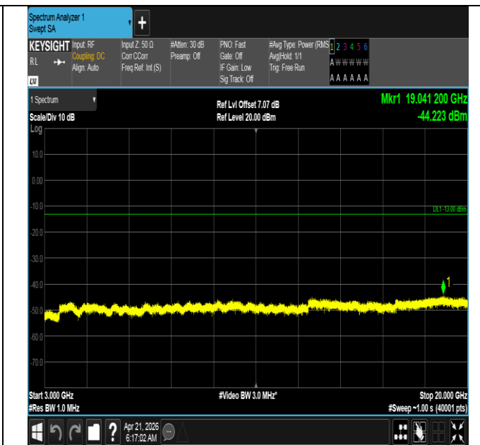
Band66-15MHz-16QAM-132047-75RB#0-3000~20000-PASS
