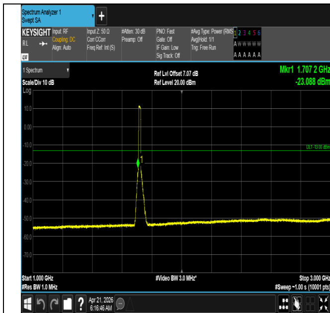
Band66-15MHz-16QAM-132047-75RB#0-1000~3000-PASS
