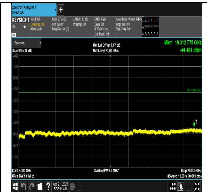
Band66-10MHz-16QAM-132322-50RB#0-3000~20000-PASS
