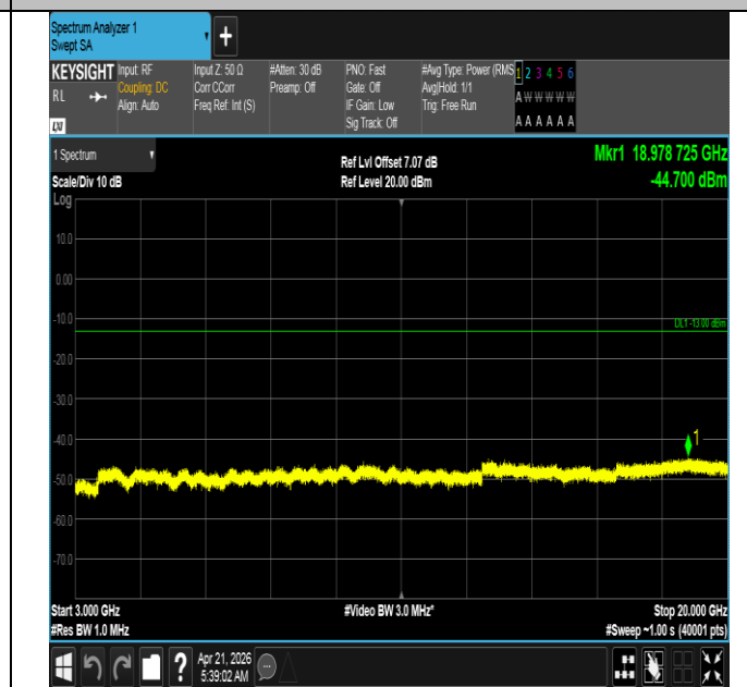
Band66-10MHz-QPSK-132622-1RB#49-3000~20000-PASS
