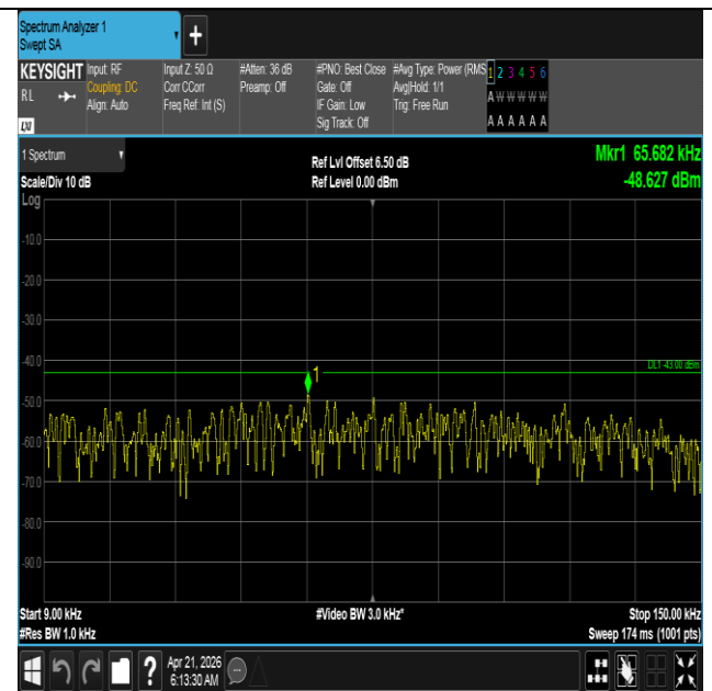
Band66-15MHz-QPSK-132047-1RB#74-0.009~0.15-PASS
