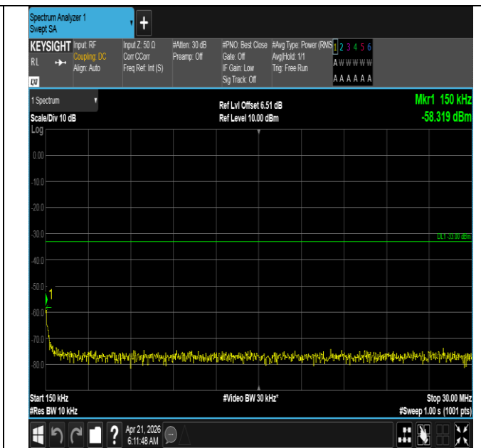
Band66-15MHz-QPSK-132047-1RB#0-0.15~30-PASS
