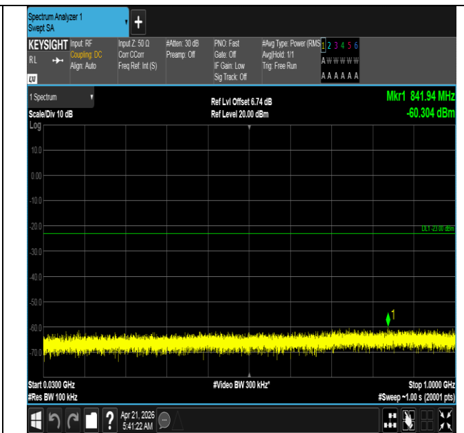
Band66-10MHz-16QAM-132622-50RB#0-30~1000-PASS
