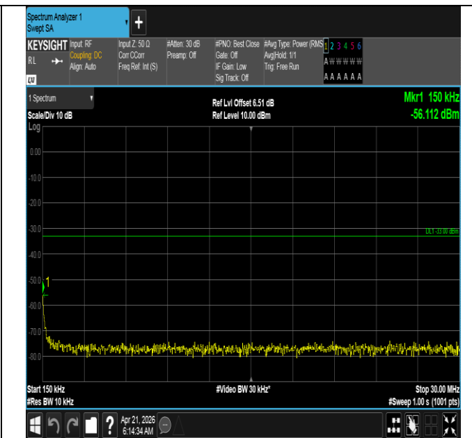
Band66-15MHz-16QAM-132047-1RB#74-0.15~30-PASS
