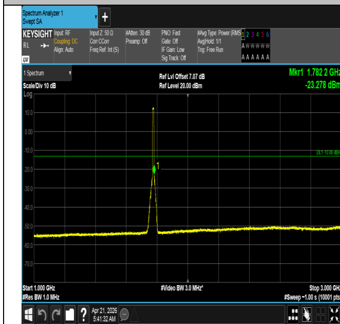
Band66-10MHz-16QAM-132622-50RB#0-1000~3000-PASS
