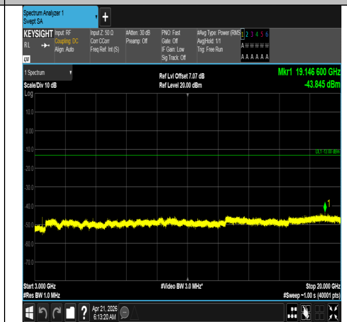
Band66-15MHz-16QAM-132047-1RB#0-3000~20000-PASS
