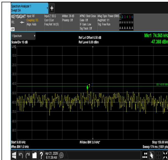
Band66-15MHz-QPSK-132047-1RB#0-0.009~0.15-PASS
