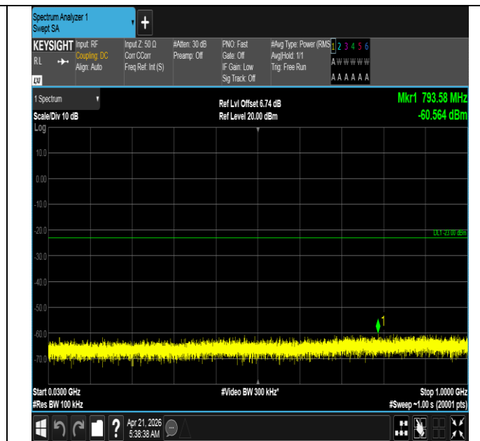
Band66-10MHz-QPSK-132622-1RB#49-30~1000-PASS
