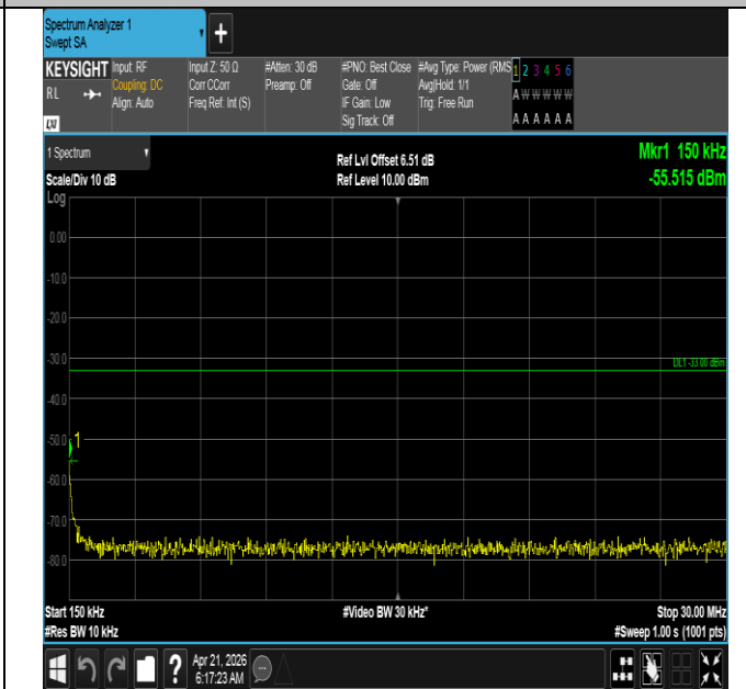
Band66-15MHz-QPSK-132322-1RB#0-0.15~30-PASS
