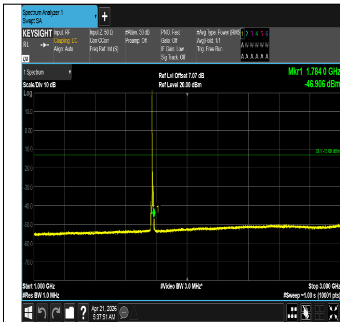
Band66-10MHz-16QAM-132622-1RB#0-1000~3000-PASS
