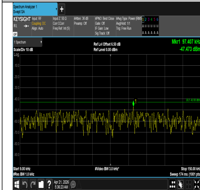
Band66-10MHz-QPSK-132622-1RB#0-0.009~0.15-PASS
