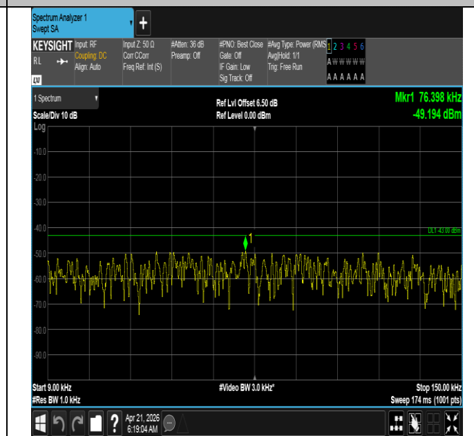
Band66-15MHz-QPSK-132322-1RB#74-0.009~0.15-PASS
