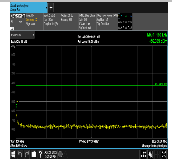
Band66-10MHz-16QAM-132622-1RB#49-0.15~30-PASS
