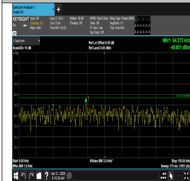
Band66-15MHz-QPSK-132047-75RB#0-0.009~0.15-PASS
