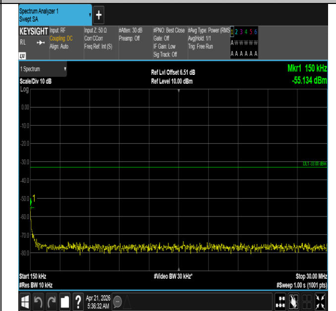
Band66-10MHz-QPSK-132622-1RB#0-0.15~30-PASS
