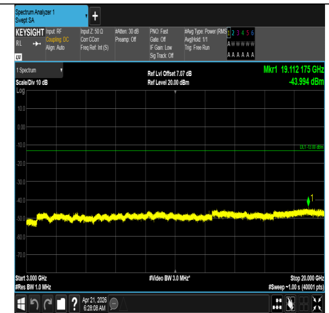
Band66-15MHz-16QAM-132597-75RB#0-3000~20000-PASS
