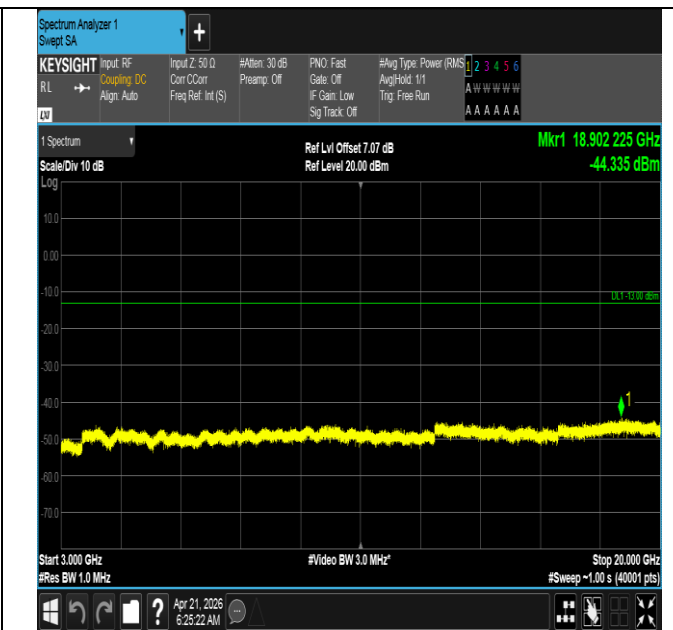
Band66-15MHz-QPSK-132597-1RB#74-3000~20000-PASS
