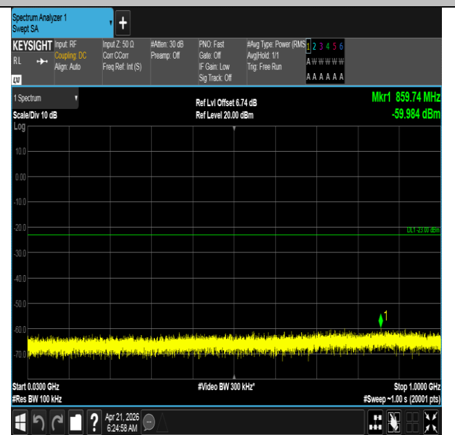
Band66-15MHz-QPSK-132597-1RB#74-30~1000-PASS
