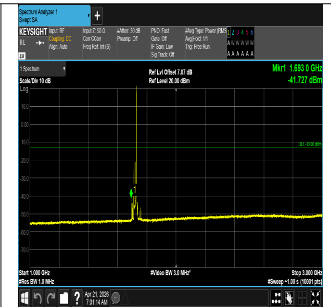
Band66-20MHz-16QAM-132072-1RB#99-1000~3000-PASS
