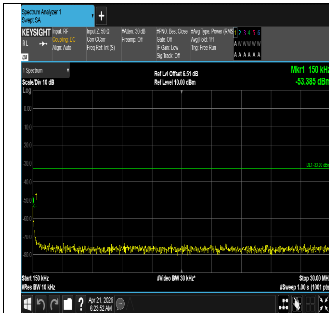
Band66-15MHz-16QAM-132597-1RB#0-0.15~30-PASS
