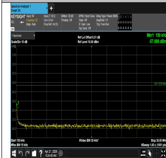
Band66-15MHz-QPSK-132597-1RB#74-0.15~30-PASS
