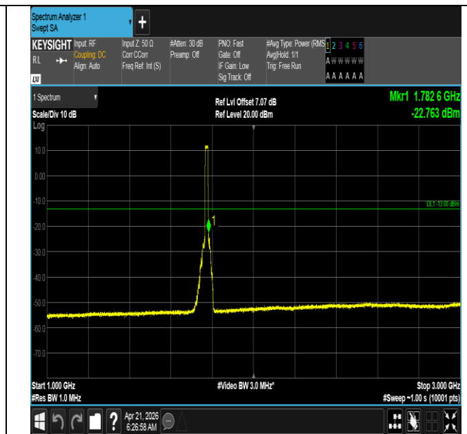
Band66-15MHz-QPSK-132597-75RB#0-1000~3000-PASS
