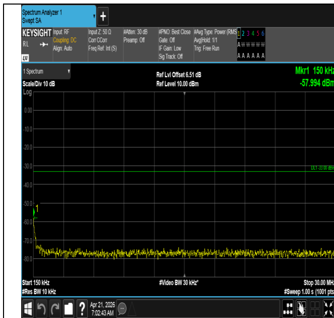
Band66-20MHz-16QAM-132072-100RB#0-0.15~30-PASS
