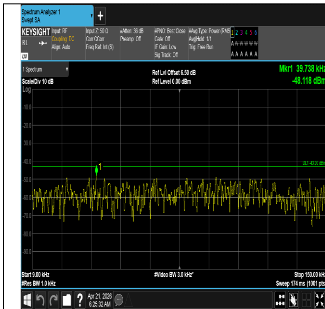
Band66-15MHz-16QAM-132597-1RB#74-0.009~0.15-PASS
