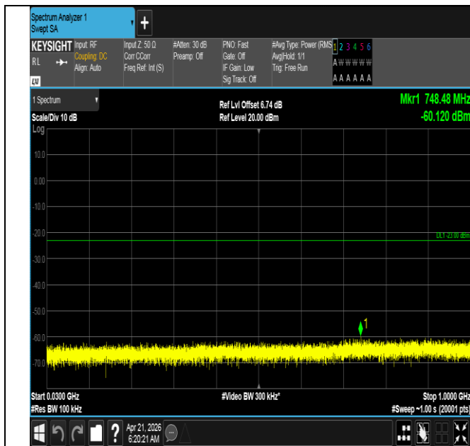
Band66-15MHz-16QAM-132322-1RB#74-30~1000-PASS
