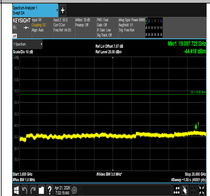
Band66-20MHz-16QAM-132072-100RB#0-3000~20000-PASS
