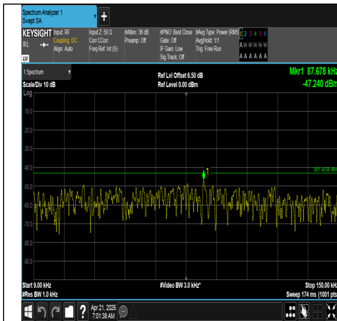
Band66-20MHz-QPSK-132072-100RB#0-0.009~0.15-PASS
