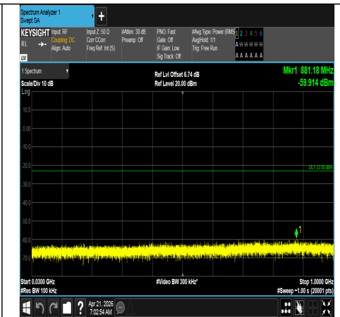
Band66-20MHz-16QAM-132072-100RB#0-30~1000-PASS
