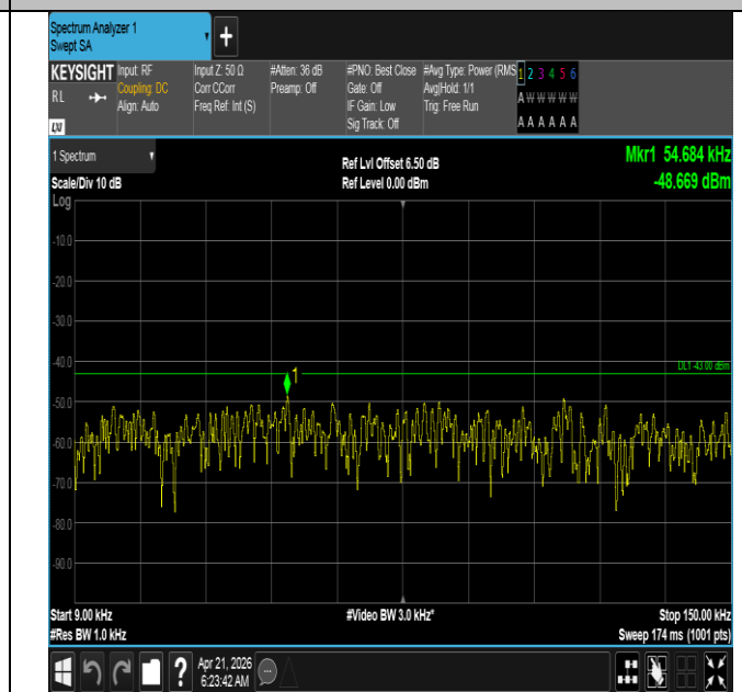
Band66-15MHz-16QAM-132597-1RB#0-0.009~0.15-PASS
