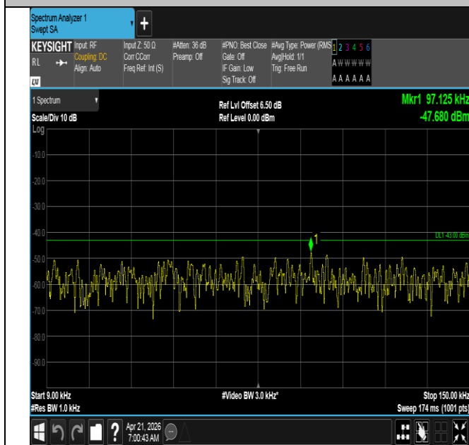
Band66-20MHz-16QAM-132072-1RB#99-0.009~0.15-PASS
