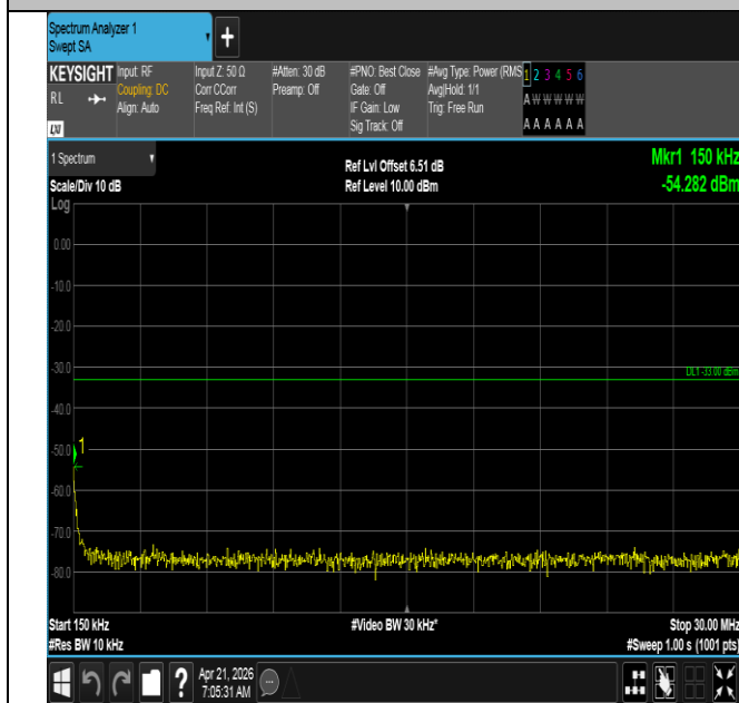
Band66-20MHz-QPSK-132322-1RB#99-0.15~30-PASS
