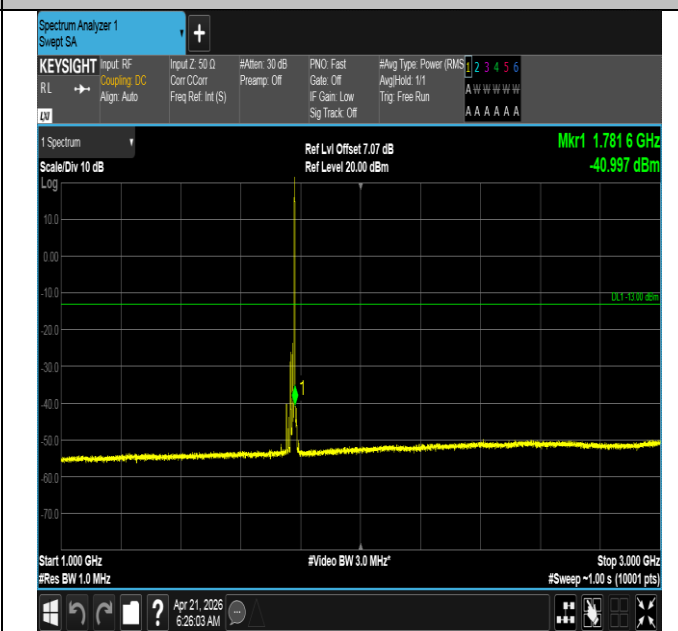
Band66-15MHz-16QAM-132597-1RB#74-1000~3000-PASS
