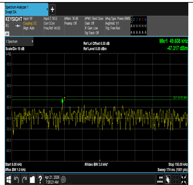
Band66-20MHz-QPSK-132322-1RB#99-0.009~0.15-PASS
