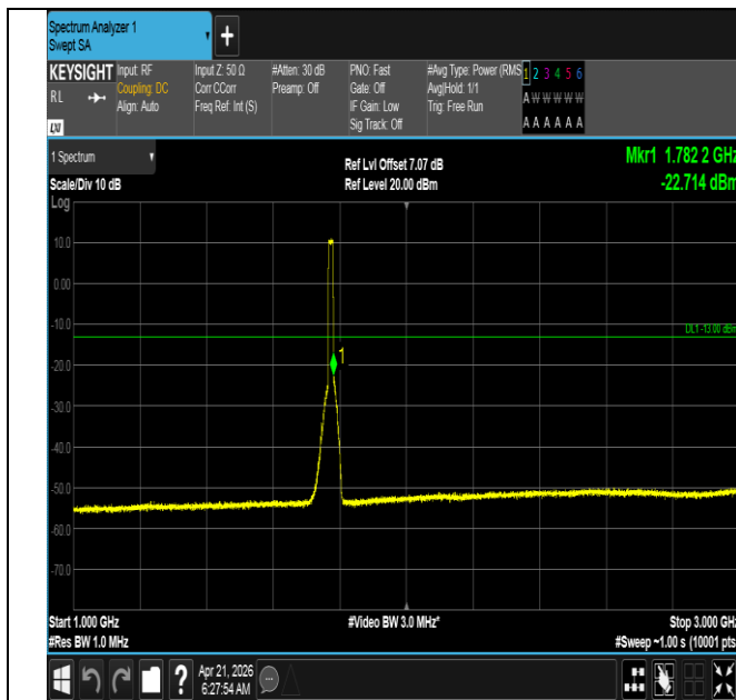
Band66-15MHz-16QAM-132597-75RB#0-1000~3000-PASS
