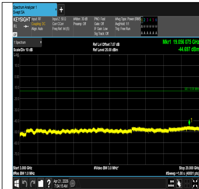
Band66-20MHz-QPSK-132322-1RB#0-3000~20000-PASS
