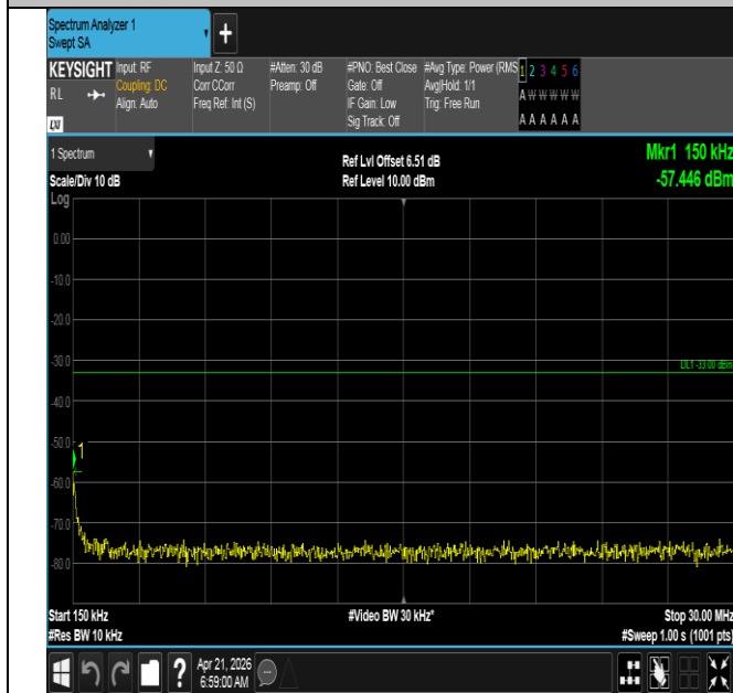
Band66-20MHz-16QAM-132072-1RB#0-0.15~30-PASS
