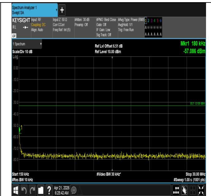
Band66-15MHz-16QAM-132597-1RB#74-0.15~30-PASS
