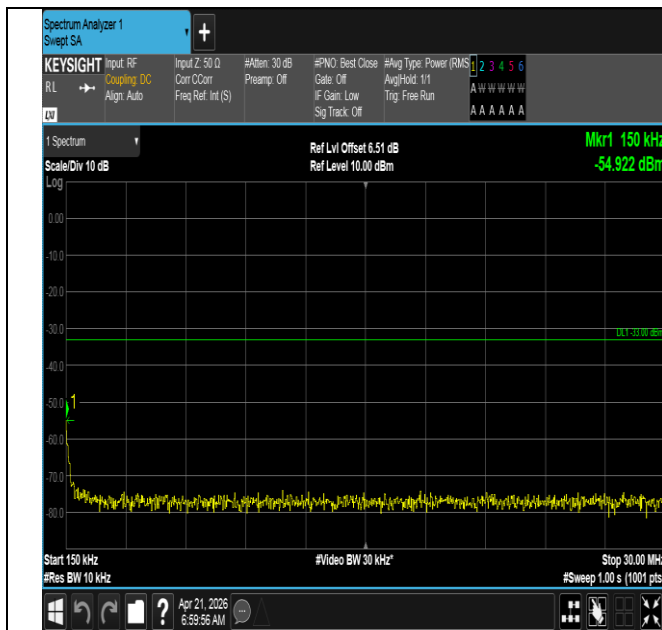
Band66-20MHz-QPSK-132072-1RB#99-0.15~30-PASS
