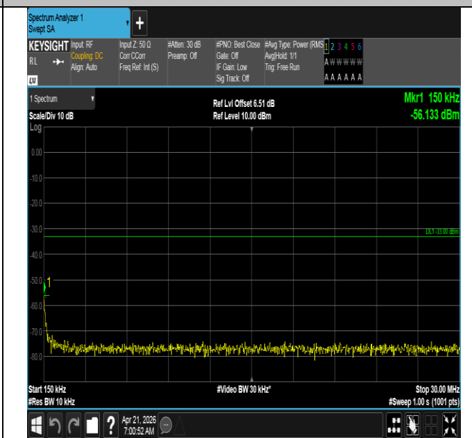
Band66-20MHz-16QAM-132072-1RB#99-0.15~30-PASS
