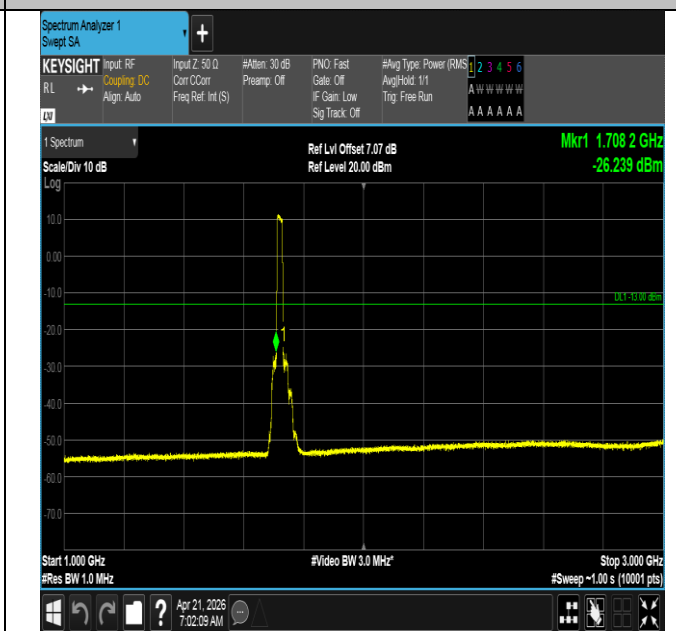
Band66-20MHz-QPSK-132072-100RB#0-1000~3000-PASS
