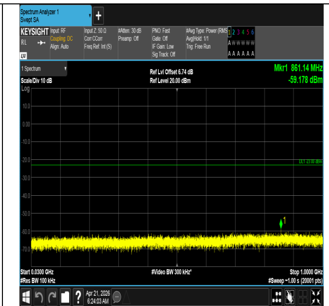
Band66-15MHz-16QAM-132597-1RB#0-30~1000-PASS
