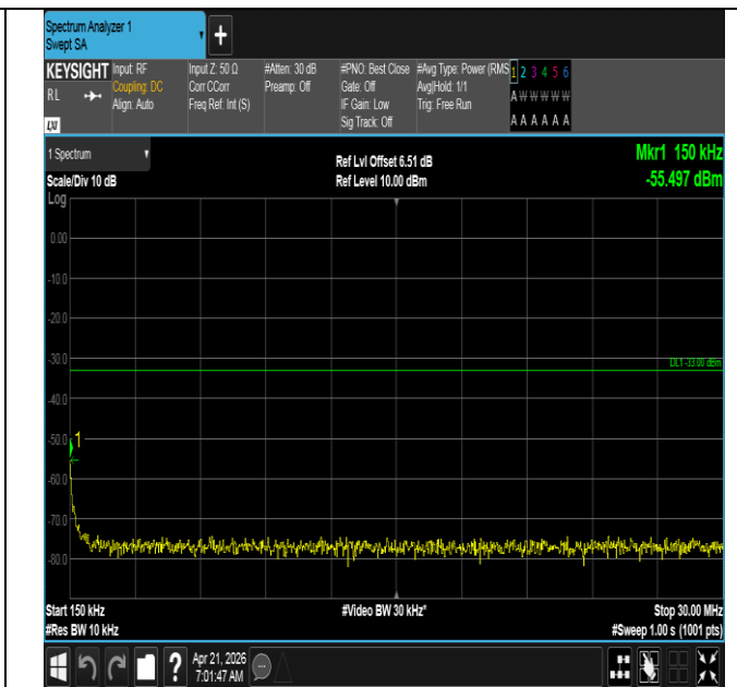
Band66-20MHz-QPSK-132072-100RB#0-0.15~30-PASS
