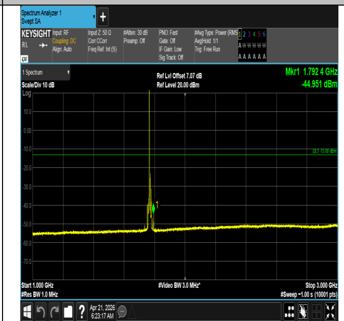
Band66-15MHz-QPSK-132597-1RB#0-1000~3000-PASS
