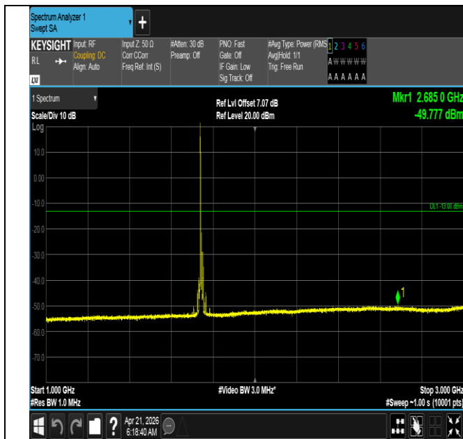
Band66-15MHz-16QAM-132322-1RB#0-1000~3000-PASS
