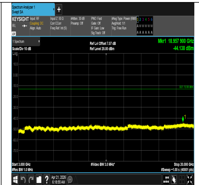
Band66-15MHz-16QAM-132322-1RB#0-3000~20000-PASS
