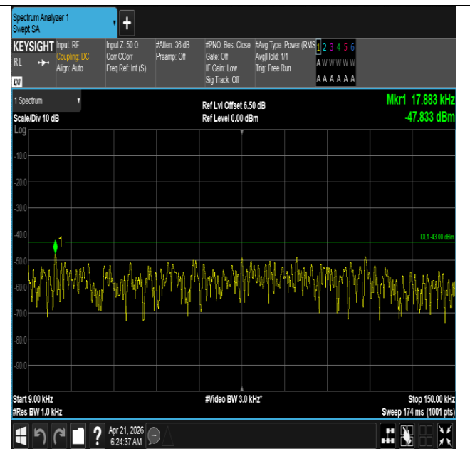
Band66-15MHz-QPSK-132597-1RB#74-0.009~0.15-PASS
