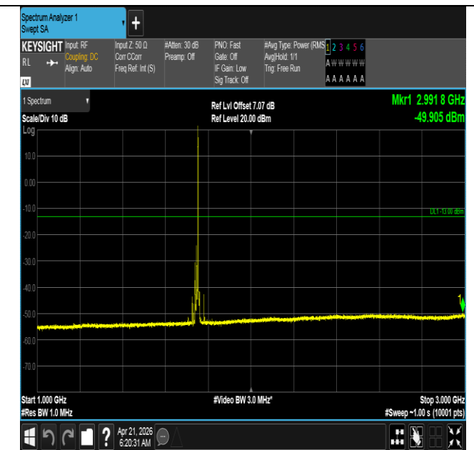
Band66-15MHz-16QAM-132322-1RB#74-1000~3000-PASS
