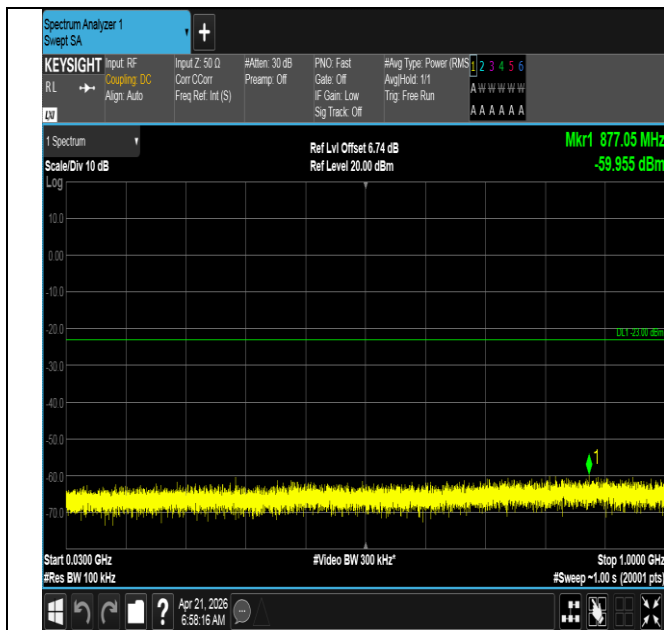
Band66-20MHz-QPSK-132072-1RB#0-30~1000-PASS
