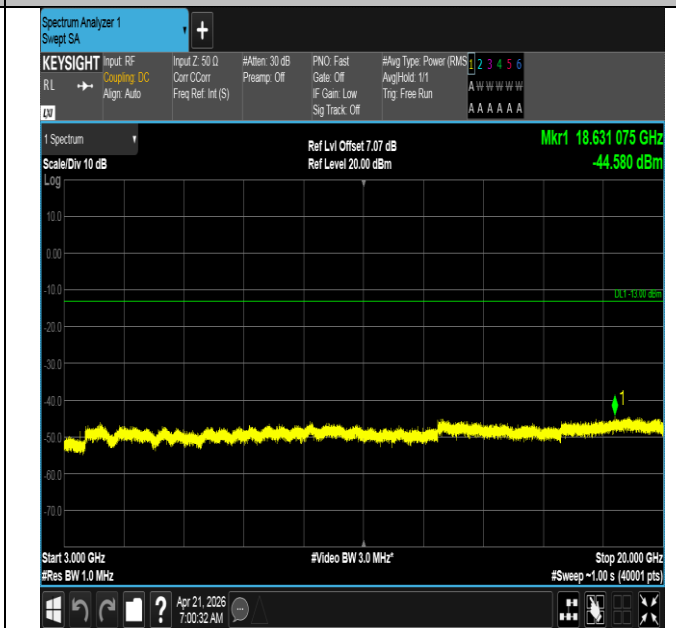
Band66-20MHz-QPSK-132072-1RB#99-3000~20000-PASS
