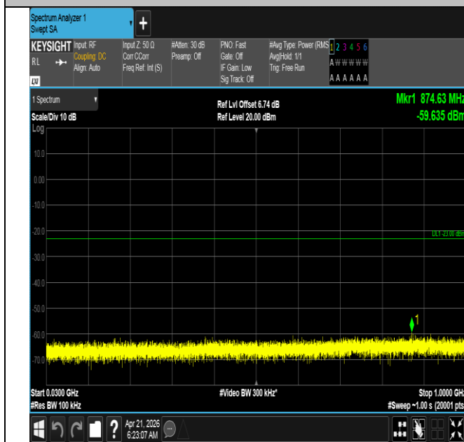
Band66-15MHz-QPSK-132597-1RB#0-30~1000-PASS
