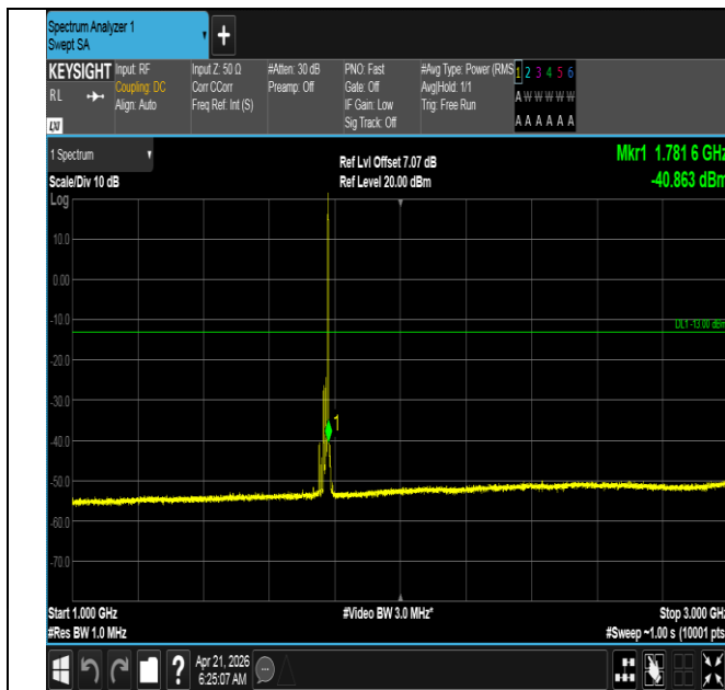
Band66-15MHz-QPSK-132597-1RB#74-1000~3000-PASS
