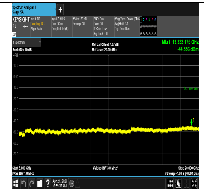
Band66-20MHz-16QAM-132072-1RB#0-3000~20000-PASS
