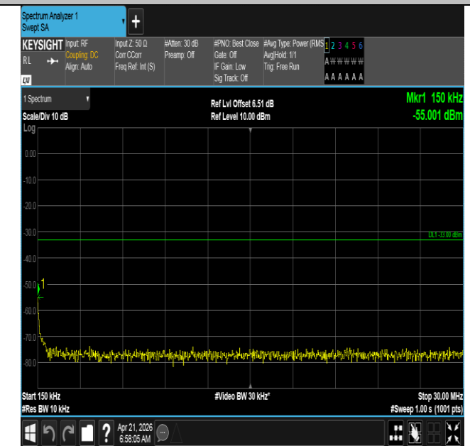
Band66-20MHz-QPSK-132072-1RB#0-0.15~30-PASS
