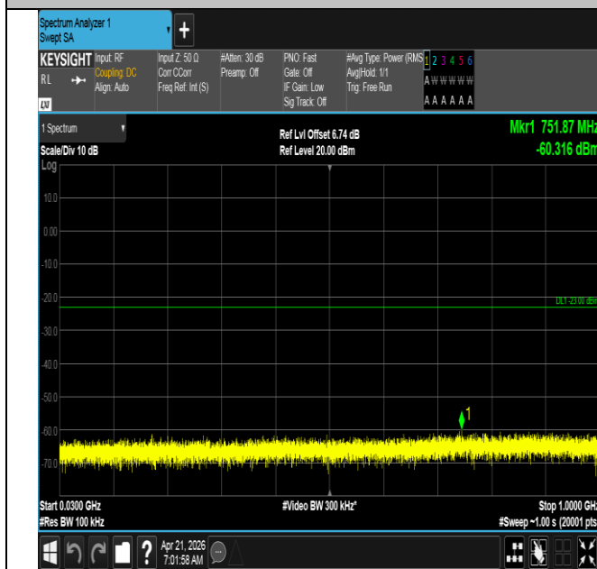
Band66-20MHz-QPSK-132072-100RB#0-30~1000-PASS
