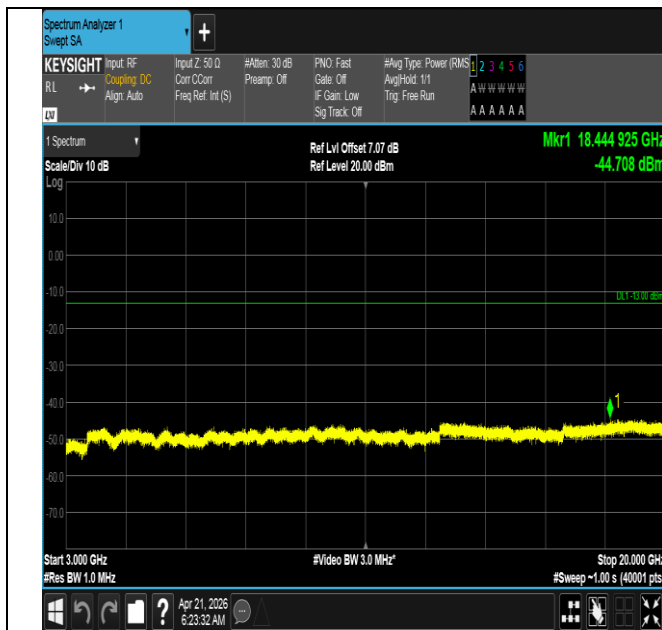
Band66-15MHz-QPSK-132597-1RB#0-3000~20000-PASS
