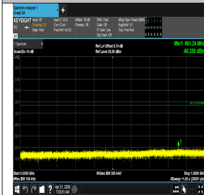
Band66-20MHz-QPSK-132322-1RB#0-30~1000-PASS
