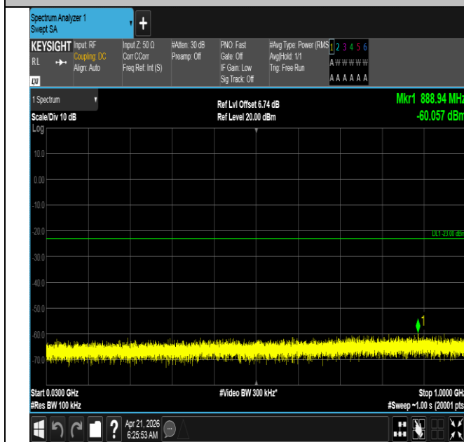
Band66-15MHz-16QAM-132597-1RB#74-30~1000-PASS
