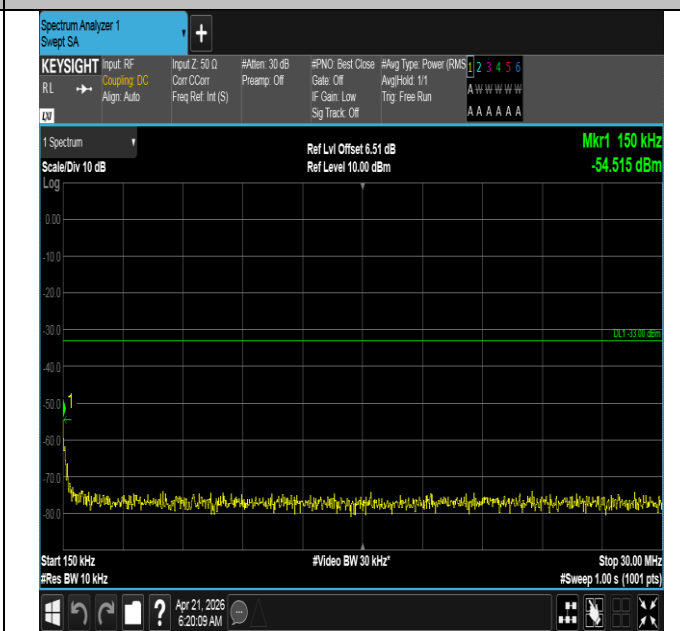
Band66-15MHz-16QAM-132322-1RB#74-0.15~30-PASS
