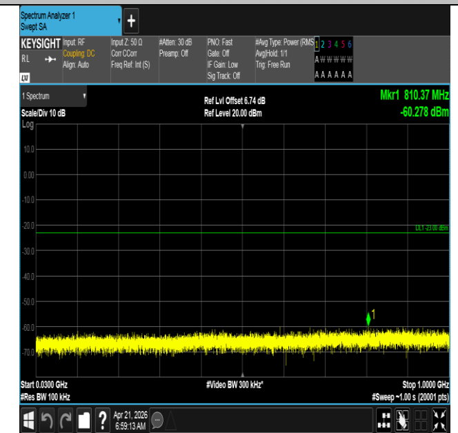
Band66-20MHz-16QAM-132072-1RB#0-30~1000-PASS
