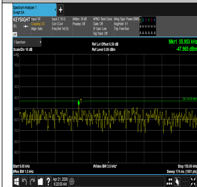
Band66-15MHz-16QAM-132322-1RB#74-0.009~0.15-PASS
