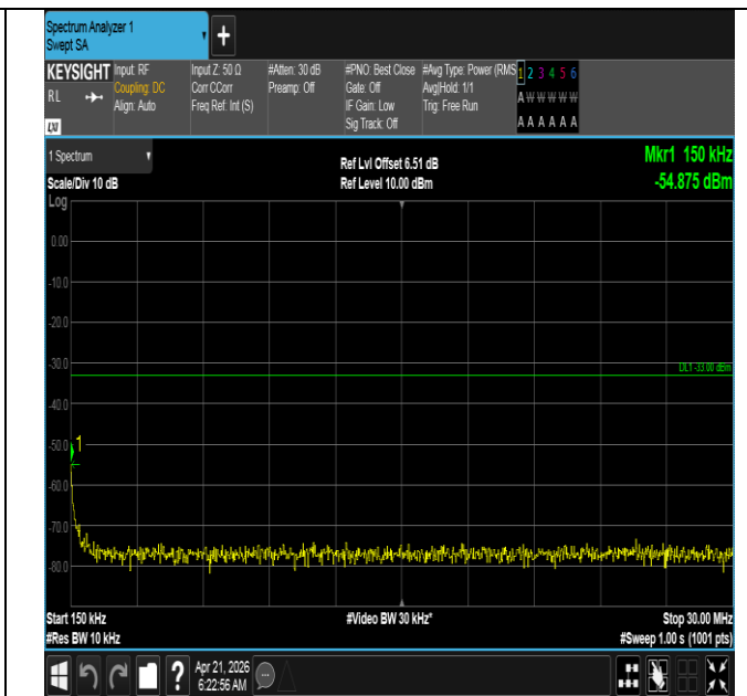
Band66-15MHz-QPSK-132597-1RB#0-0.15~30-PASS
