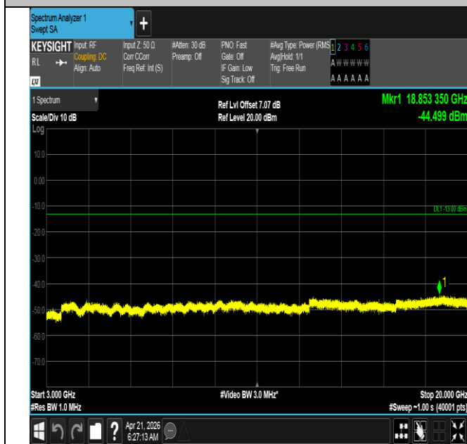
Band66-15MHz-QPSK-132597-75RB#0-3000~20000-PASS
