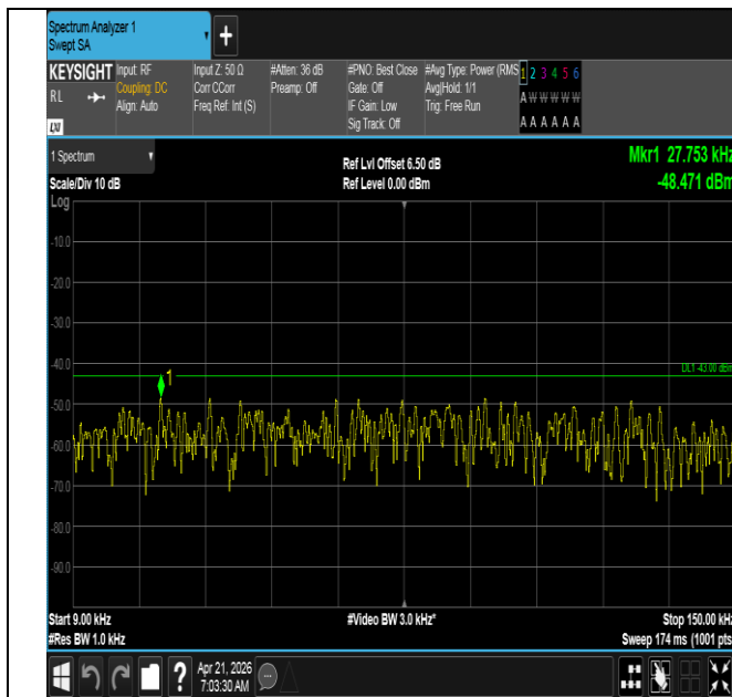
Band66-20MHz-QPSK-132322-1RB#0-0.009~0.15-PASS
