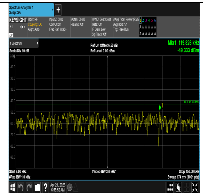
Band66-20MHz-16QAM-132072-1RB#0-0.009~0.15-PASS
