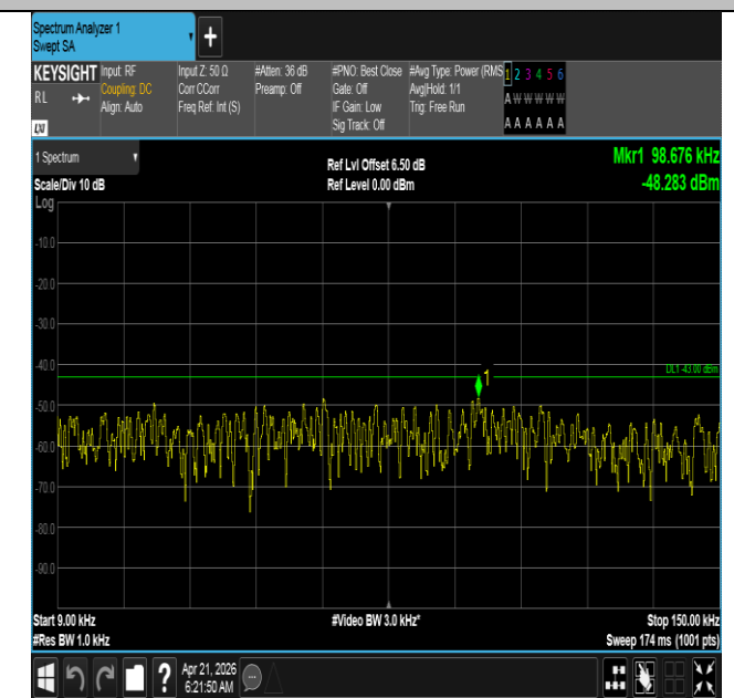
Band66-15MHz-16QAM-132322-75RB#0-0.009~0.15-PASS
