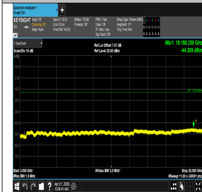
Band66-20MHz-QPSK-132072-1RB#0-3000~20000-PASS
