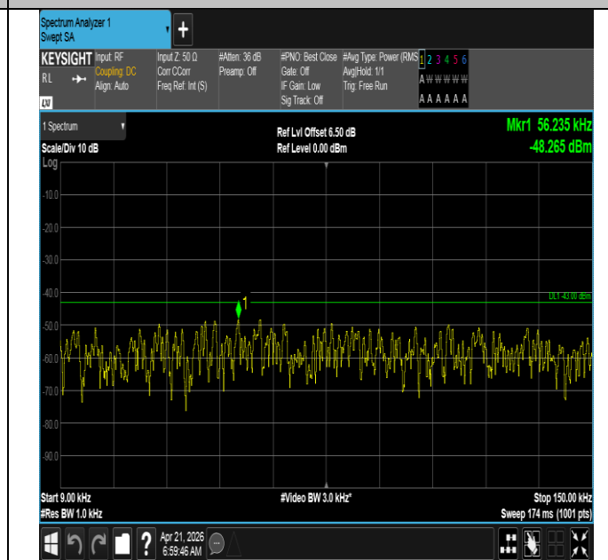
Band66-20MHz-QPSK-132072-1RB#99-0.009~0.15-PASS
