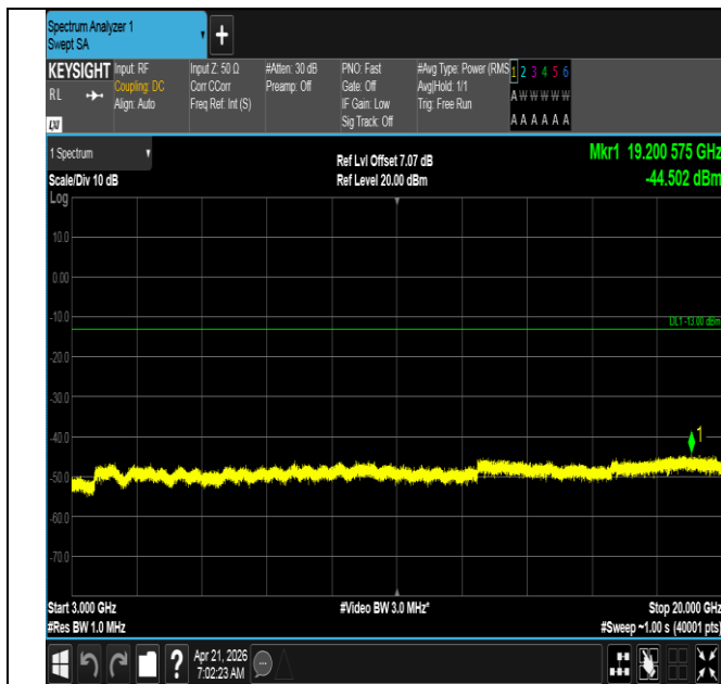
Band66-20MHz-QPSK-132072-100RB#0-3000~20000-PASS
