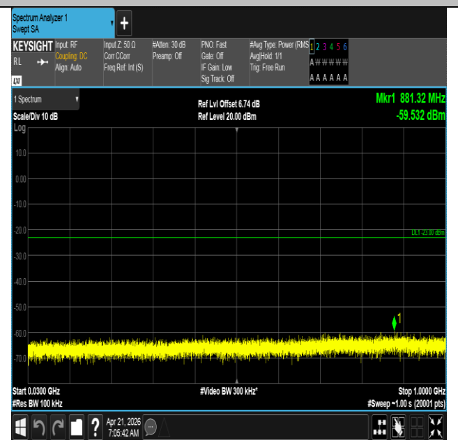
Band66-20MHz-QPSK-132322-1RB#99-30~1000-PASS
