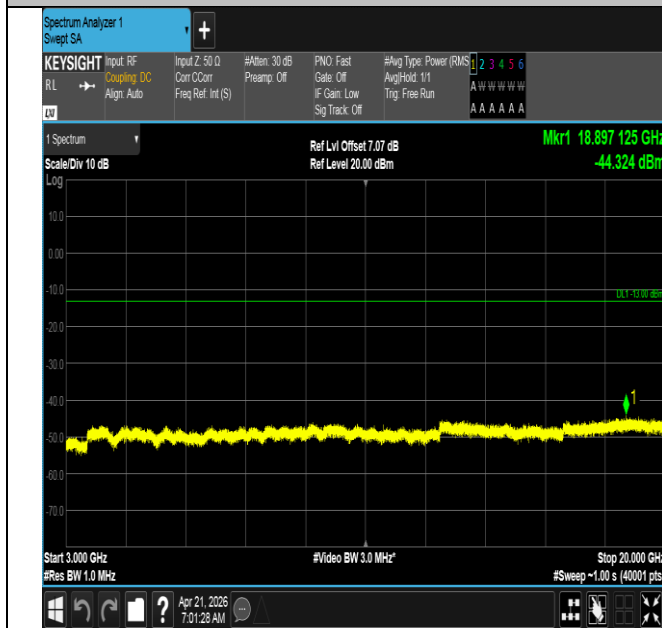
Band66-20MHz-16QAM-132072-1RB#99-3000~20000-PASS
