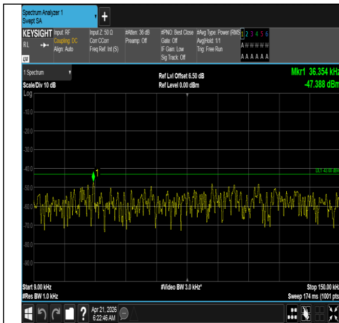
Band66-15MHz-QPSK-132597-1RB#0-0.009~0.15-PASS
