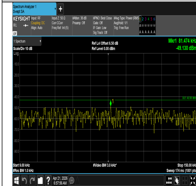
Band66-20MHz-QPSK-132072-1RB#0-0.009~0.15-PASS
