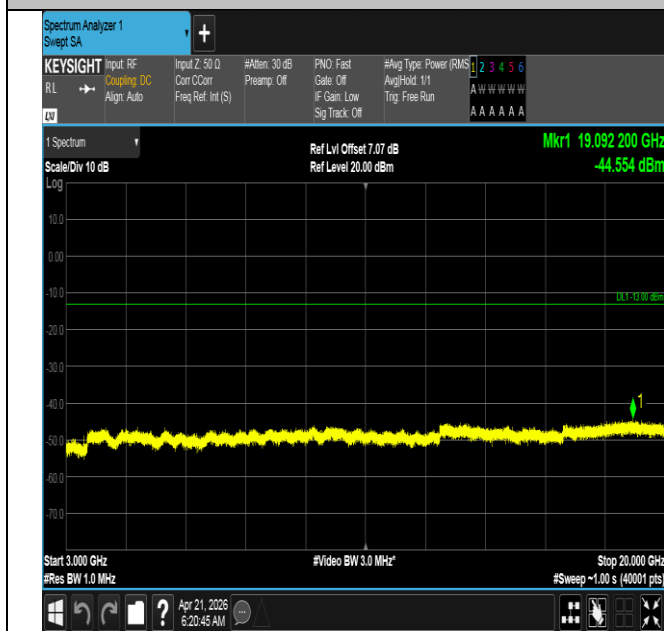
Band66-15MHz-16QAM-132322-1RB#74-3000~20000-PASS
