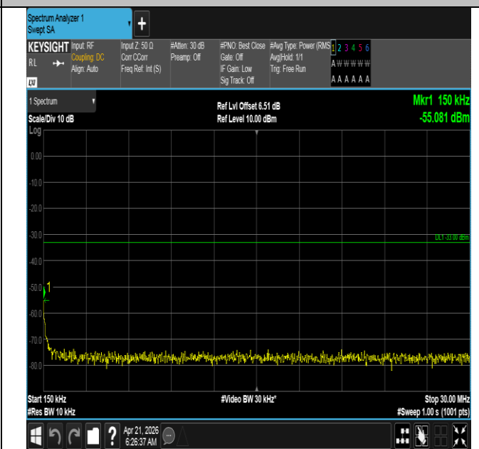
Band66-15MHz-QPSK-132597-75RB#0-0.15~30-PASS
