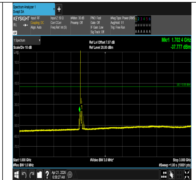
Band66-20MHz-QPSK-132072-1RB#0-1000~3000-PASS
