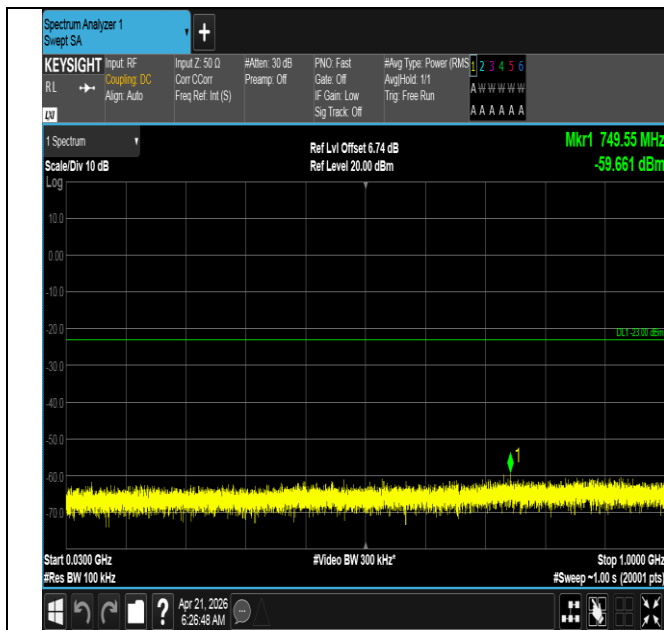
Band66-15MHz-QPSK-132597-75RB#0-30~1000-PASS
