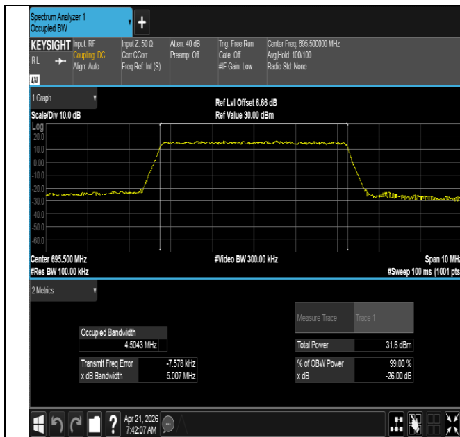
Band71-5MHz-QPSK-133447-25RB#0-PASS
