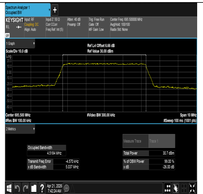
Band71-5MHz-16QAM-133447-25RB#0-PASS
