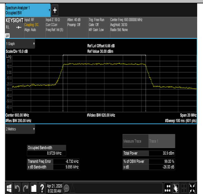
Band71-10MHz-16QAM-133422-50RB#0-PASS
