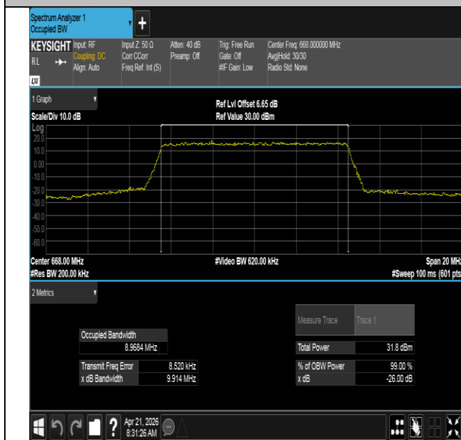
Band71-10MHz-QPSK-133172-50RB#0-PASS
