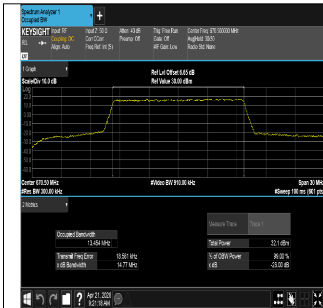
Band71-15MHz-QPSK-133197-75RB#0-PASS
