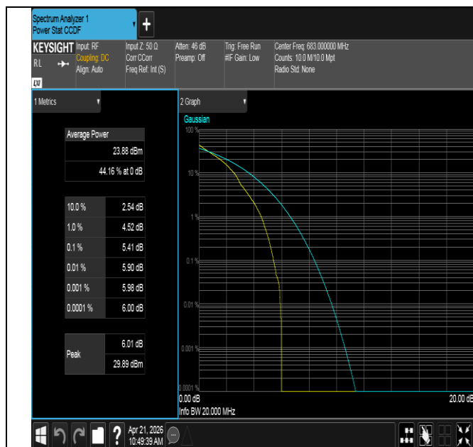
Band71-20MHz-QPSK-133322-1RB#0-PASS
