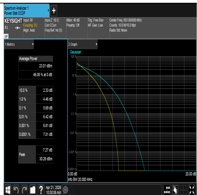
Band71-20MHz-QPSK-133322-100RB#0-PASS
