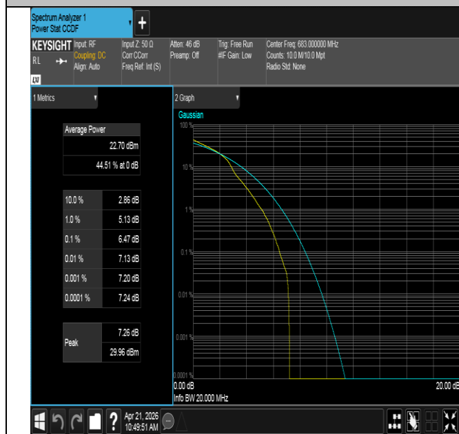
Band71-20MHz-16QAM-133322-1RB#0-PASS
