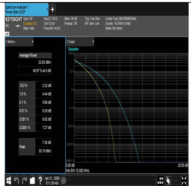
Band71-10MHz-QPSK-133172-50RB#0-PASS
