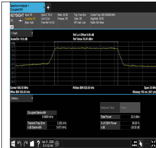
Band71-10MHz-QPSK-133297-50RB#0-PASS
