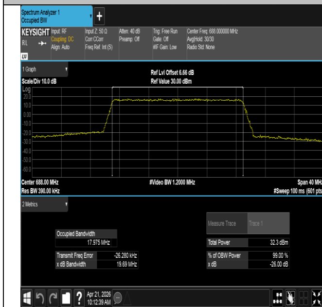
Band71-20MHz-QPSK-133372-100RB#0-PASS
