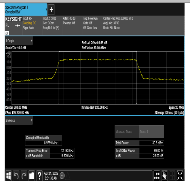
Band71-10MHz-16QAM-133172-50RB#0-PASS
