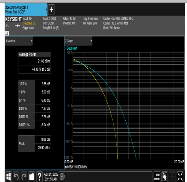
Band71-10MHz-16QAM-133172-50RB#0-PASS
