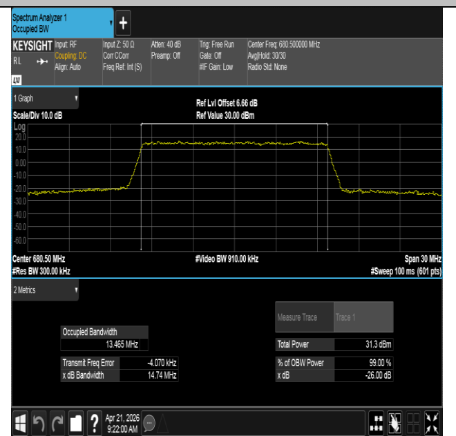
Band71-15MHz-16QAM-133297-75RB#0-PASS
