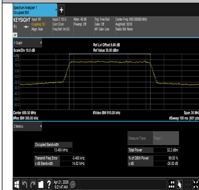
Band71-15MHz-QPSK-133297-75RB#0-PASS
