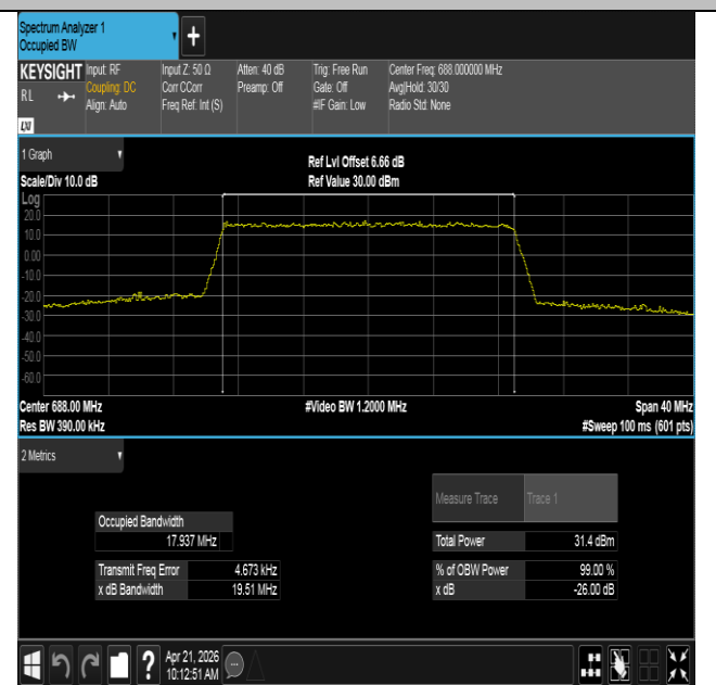
Band71-20MHz-16QAM-133372-100RB#0-PASS
