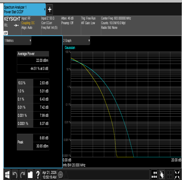
Band71-20MHz-16QAM-133322-100RB#0-PASS
