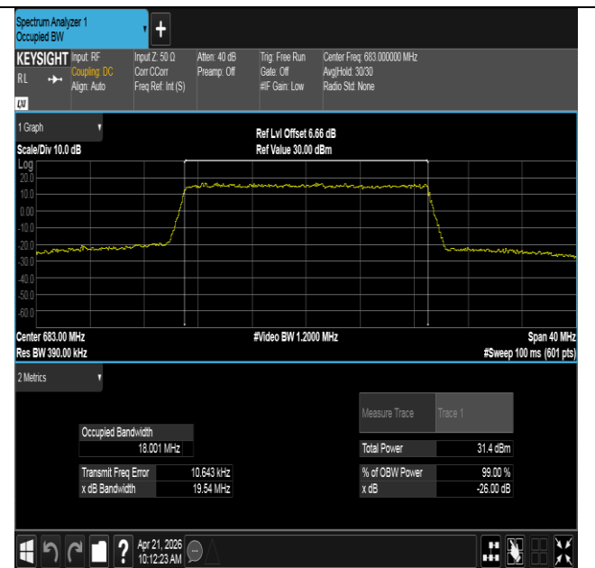
Band71-20MHz-16QAM-133322-100RB#0-PASS
