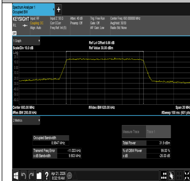
Band71-10MHz-QPSK-133422-50RB#0-PASS
