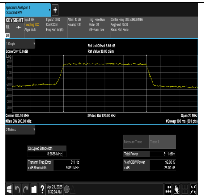
Band71-10MHz-16QAM-133297-50RB#0-PASS
