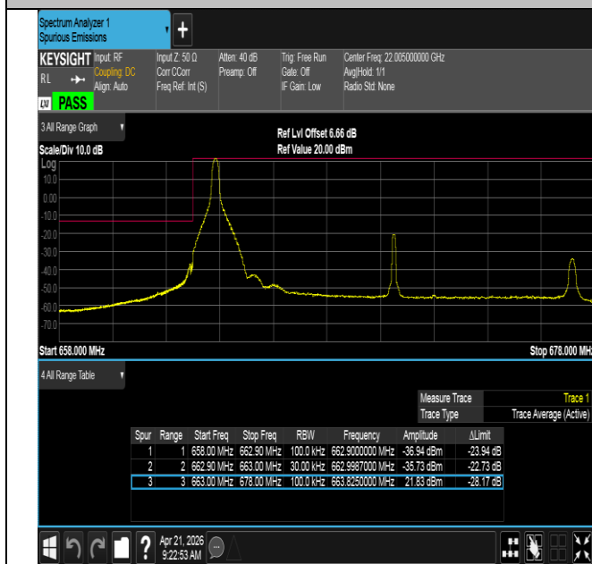
Band71-15MHz-QPSK-133197-1RB#0-PASS
