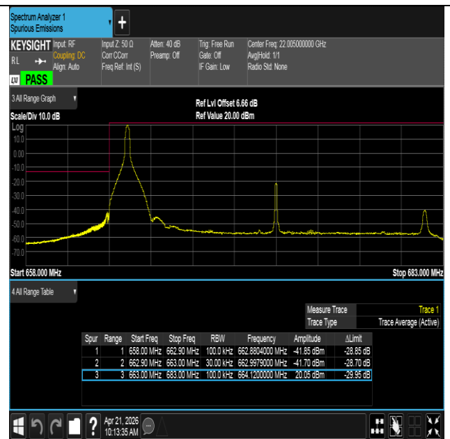
Band71-20MHz-16QAM-133222-1RB#0-PASS
