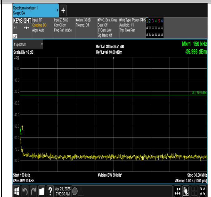
Band71-5MHz-QPSK-133147-25RB#0-0.15~30-PASS
