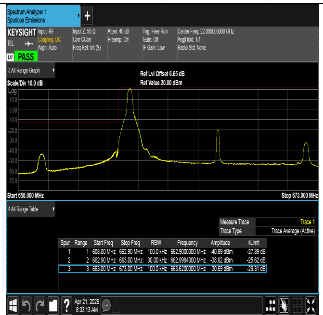
Band71-10MHz-16QAM-133172-1RB#0-PASS
