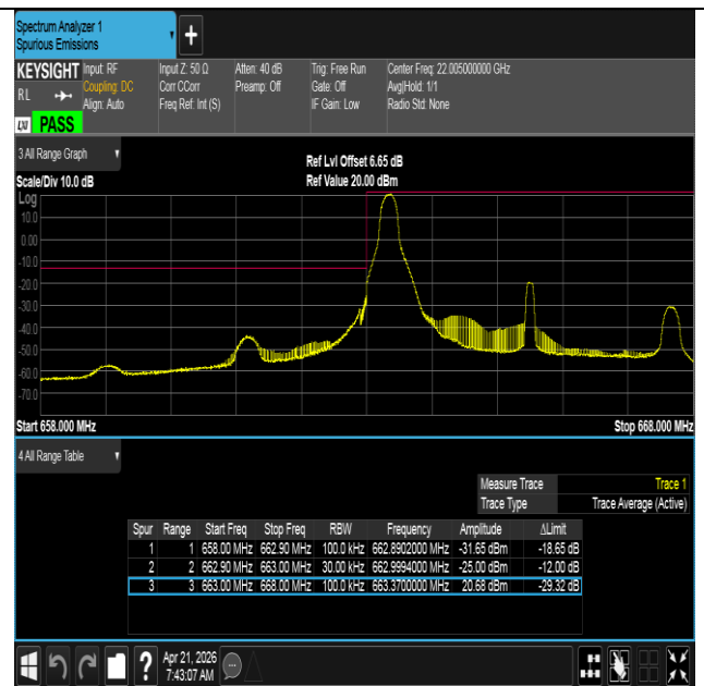
Band71-5MHz-16QAM-133147-1RB#0-PASS
