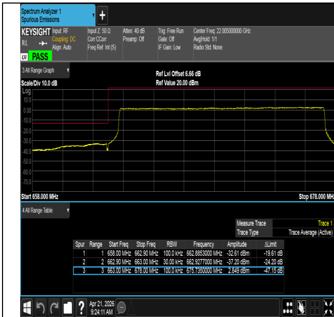
Band71-15MHz-QPSK-133197-75RB#0-PASS
