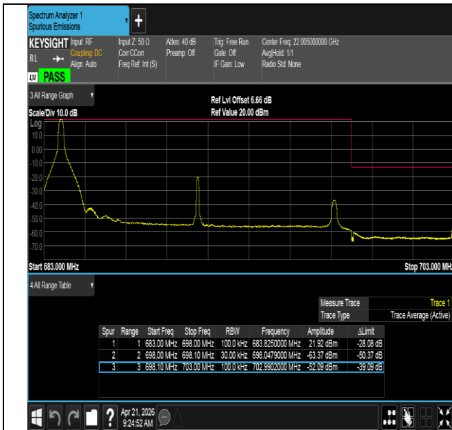
Band71-15MHz-QPSK-133397-1RB#0-PASS
