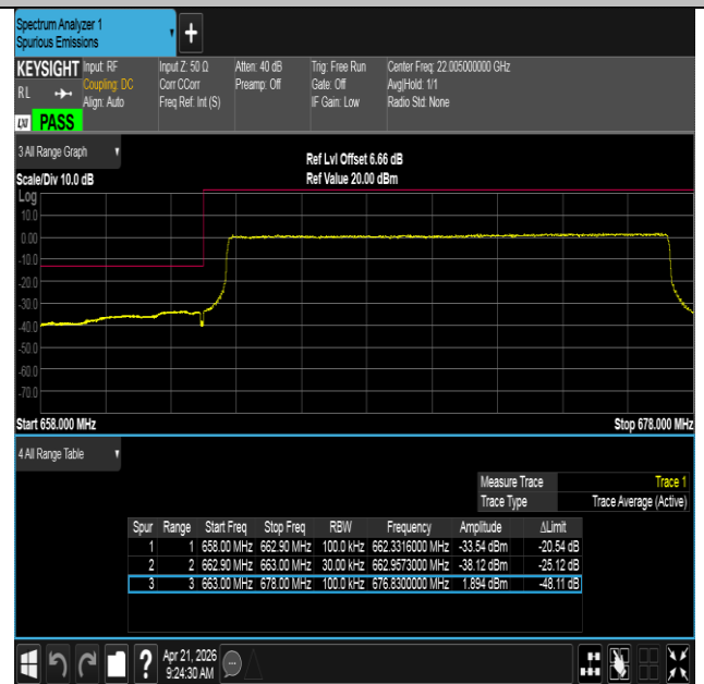
Band71-15MHz-16QAM-133197-75RB#0-PASS
