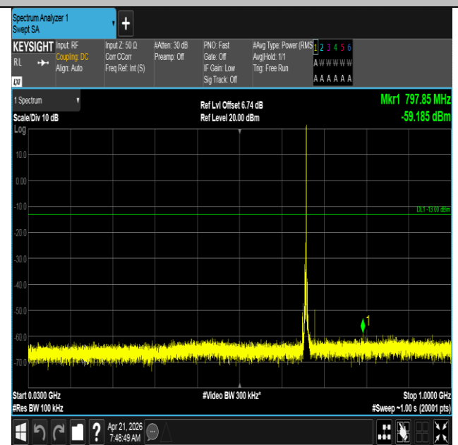
Band71-5MHz-QPSK-133147-1RB#24-30~1000-PASS
