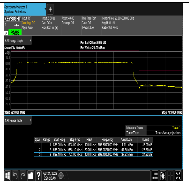
Band71-15MHz-16QAM-133397-75RB#0-PASS
