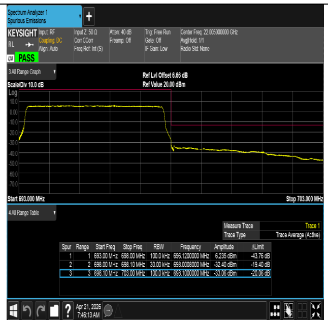
Band71-5MHz-16QAM-133447-25RB#0-PASS
