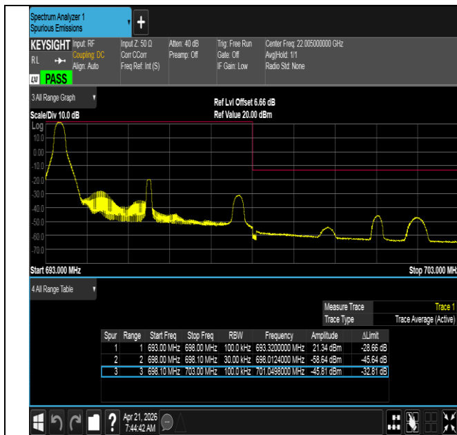
Band71-5MHz-QPSK-133447-1RB#0-PASS
