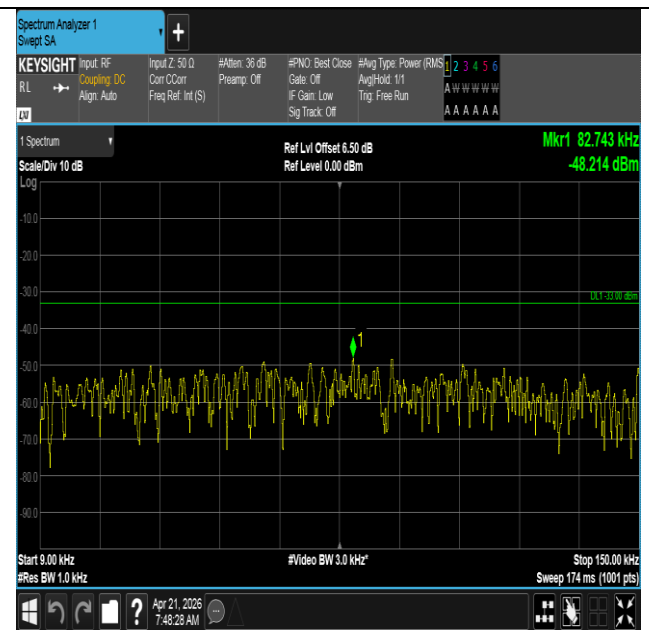
Band71-5MHz-QPSK-133147-1RB#24-0.009~0.15-PASS
