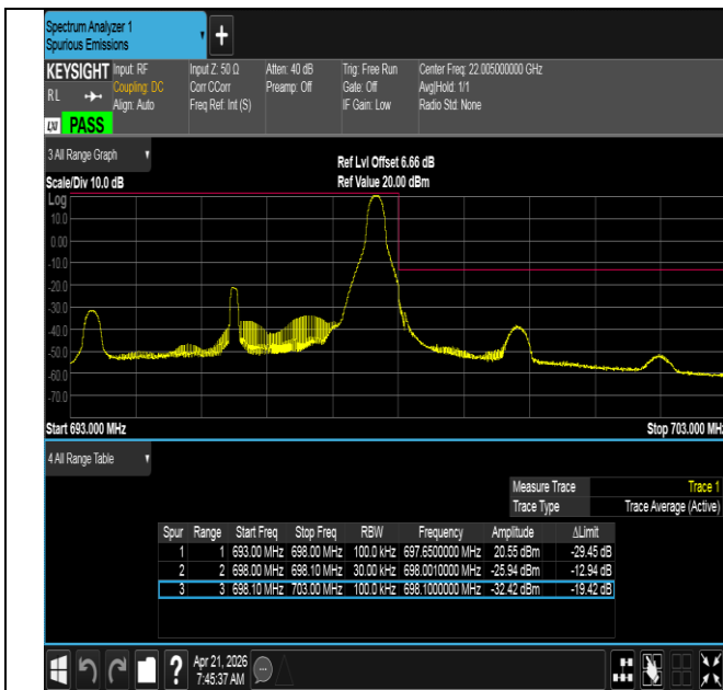
Band71-5MHz-16QAM-133447-1RB#24-PASS
