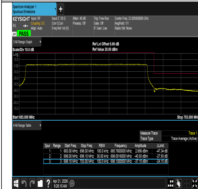
Band71-15MHz-QPSK-133397-75RB#0-PASS
