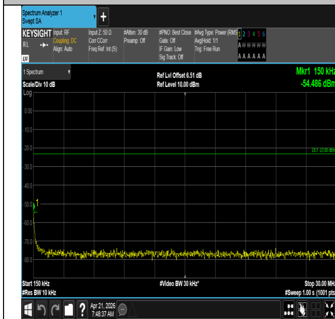
Band71-5MHz-QPSK-133147-1RB#24-0.15~30-PASS
