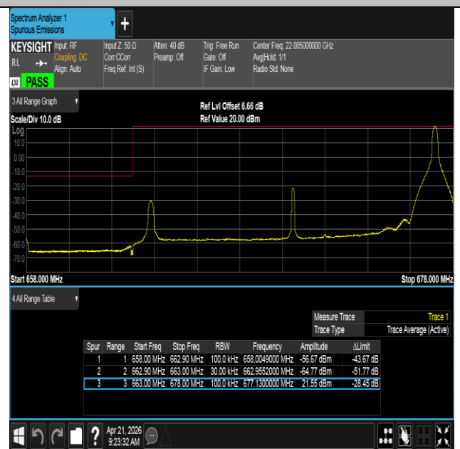
Band71-15MHz-QPSK-133197-1RB#74-PASS
