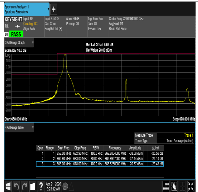
Band71-15MHz-16QAM-133197-1RB#0-PASS
