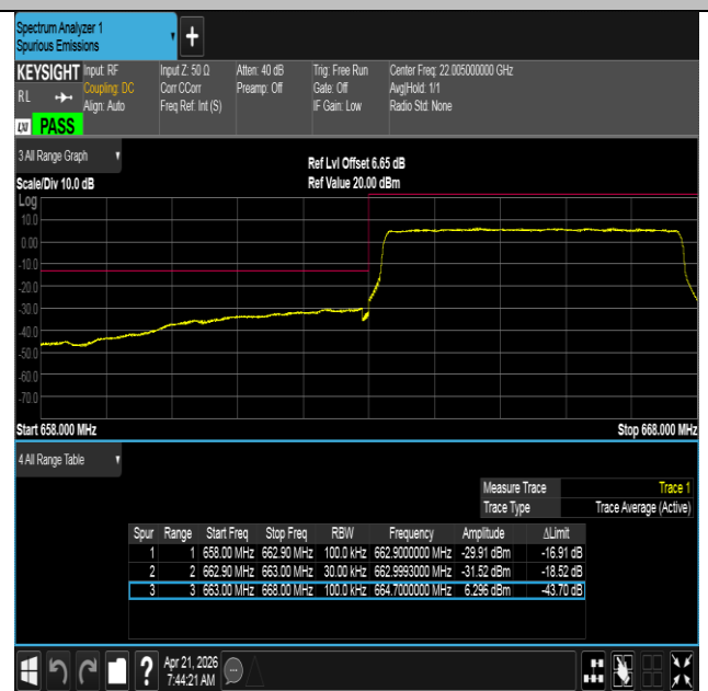
Band71-5MHz-16QAM-133147-25RB#0-PASS
