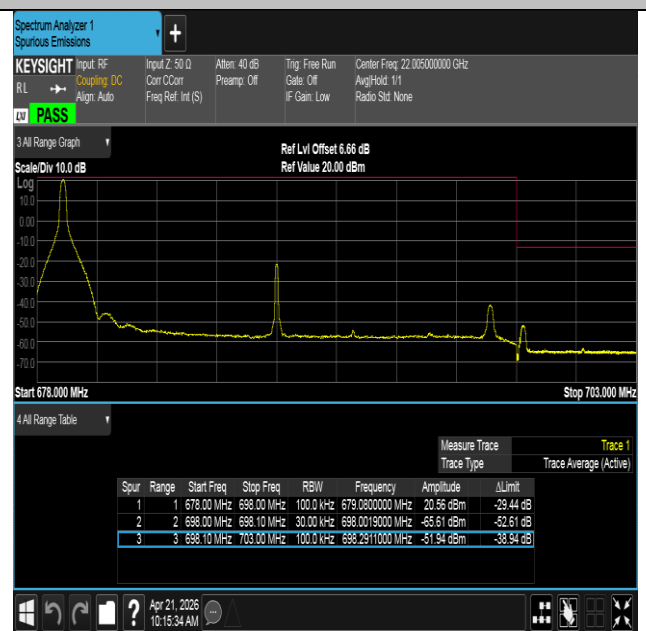
Band71-20MHz-16QAM-133372-1RB#0-PASS
