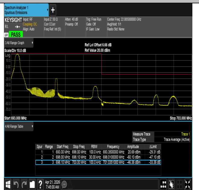
Band71-5MHz-16QAM-133447-1RB#0-PASS
