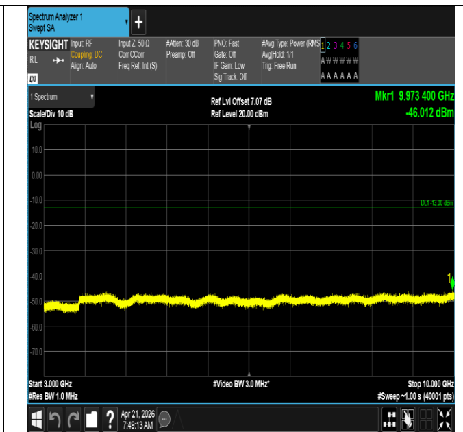
Band71-5MHz-QPSK-133147-1RB#24-3000~10000-PASS
