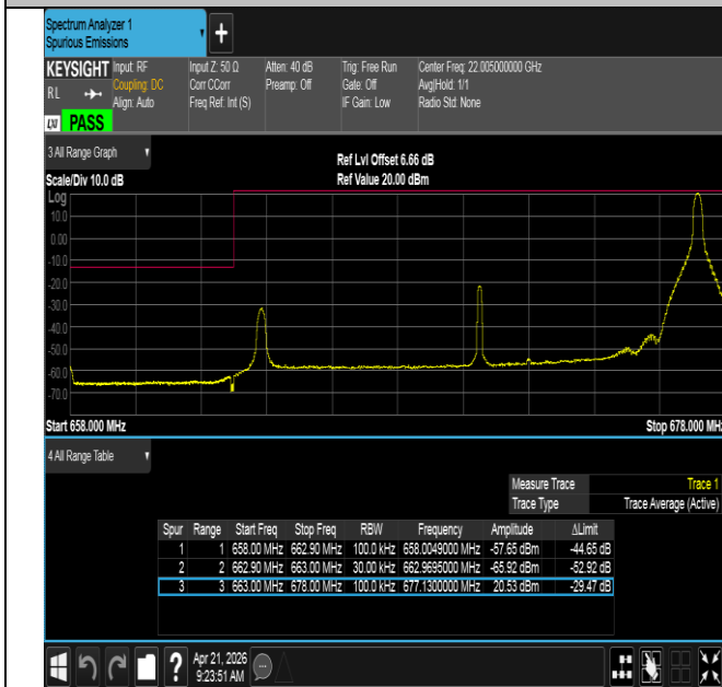
Band71-15MHz-16QAM-133197-1RB#74-PASS
