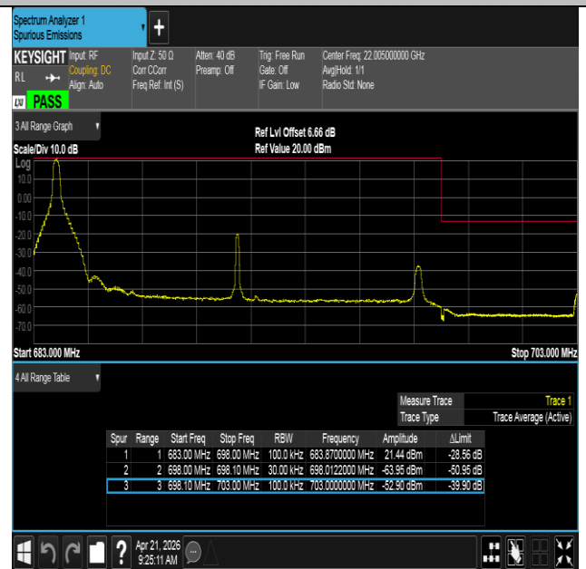
Band71-15MHz-16QAM-133397-1RB#0-PASS
