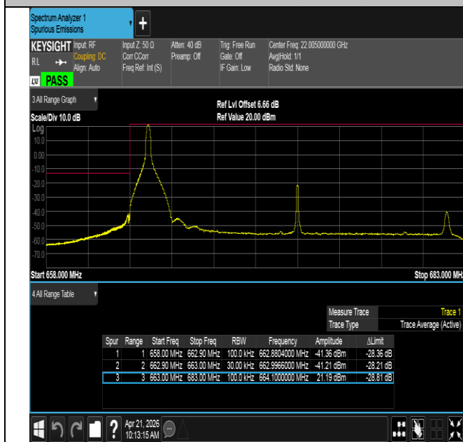
Band71-20MHz-QPSK-133222-1RB#0-PASS
