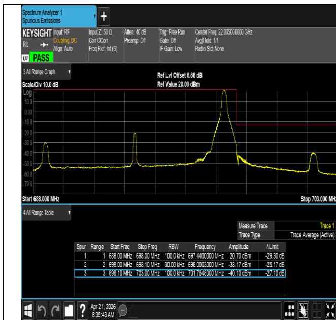
Band71-10MHz-16QAM-133422-1RB#49-PASS
