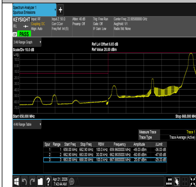
Band71-5MHz-16QAM-133147-1RB#24-PASS
