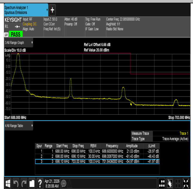
Band71-10MHz-16QAM-133422-1RB#0-PASS
