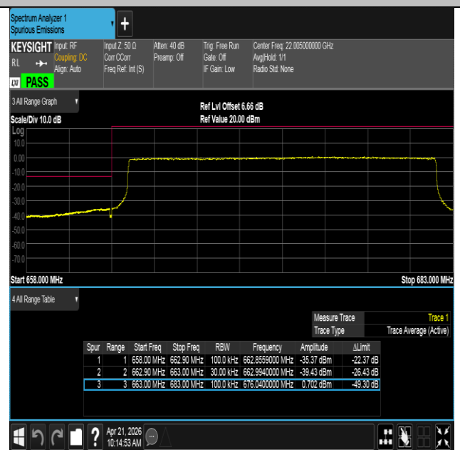
Band71-20MHz-16QAM-133222-100RB#0-PASS
