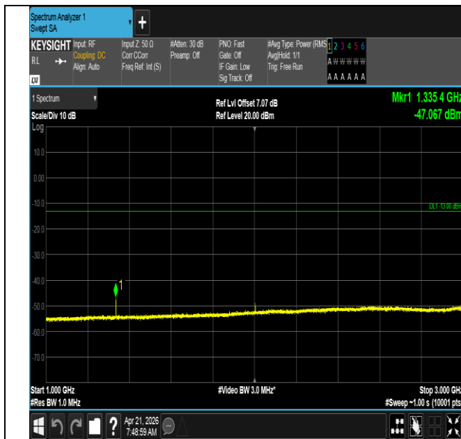
Band71-5MHz-QPSK-133147-1RB#24-1000~3000-PASS
