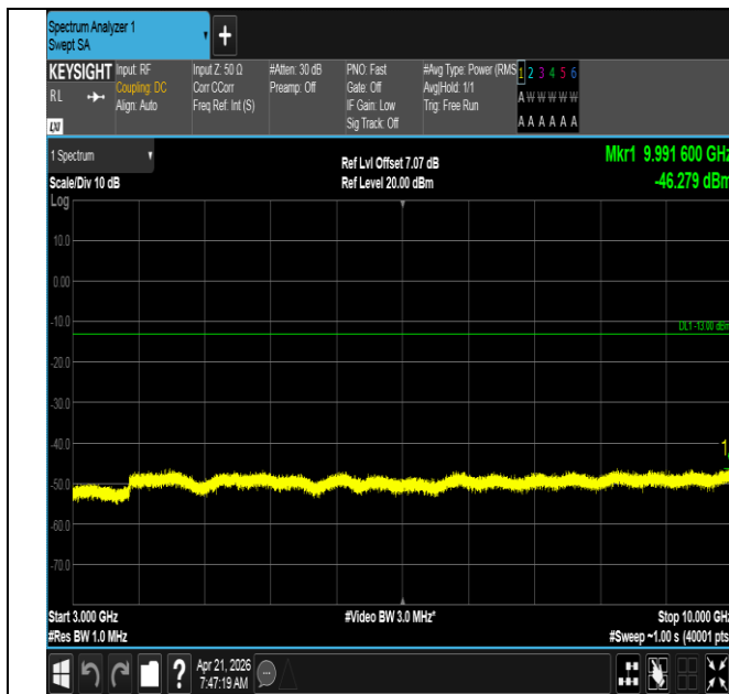
Band71-5MHz-QPSK-133147-1RB#0-3000~10000-PASS
