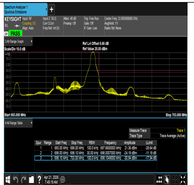
Band71-5MHz-QPSK-133447-1RB#24-PASS
