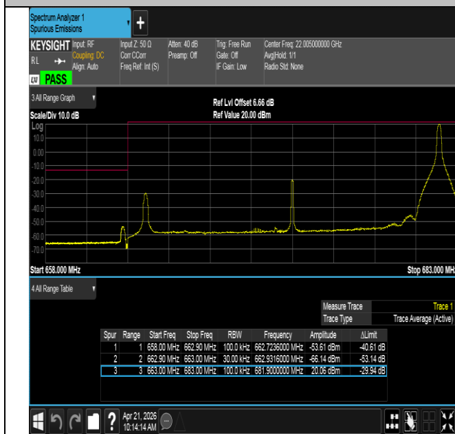
Band71-20MHz-16QAM-133222-1RB#99-PASS
