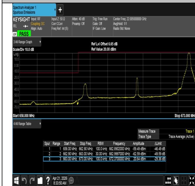
Band71-10MHz-16QAM-133172-1RB#49-PASS
