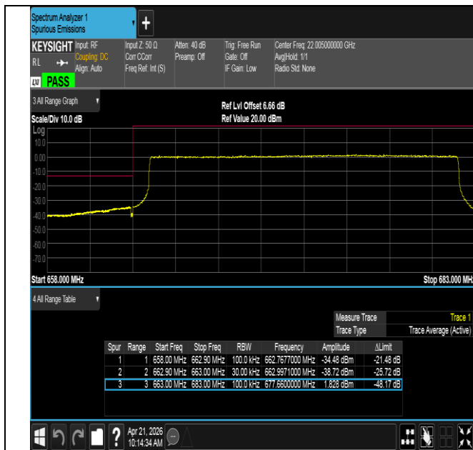
Band71-20MHz-QPSK-133222-100RB#0-PASS
