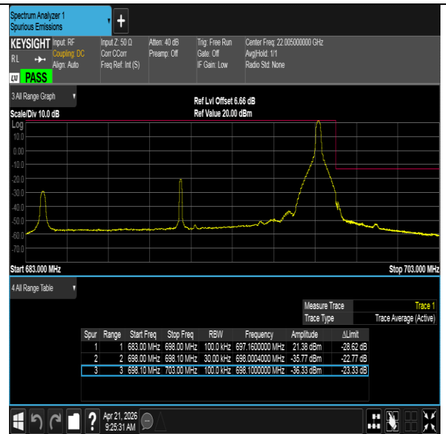
Band71-15MHz-QPSK-133397-1RB#74-PASS
