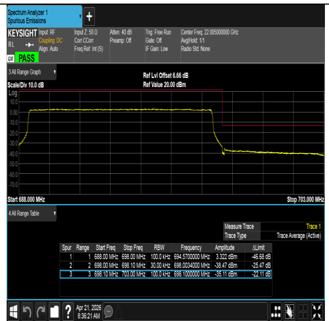
Band71-10MHz-16QAM-133422-50RB#0-PASS
